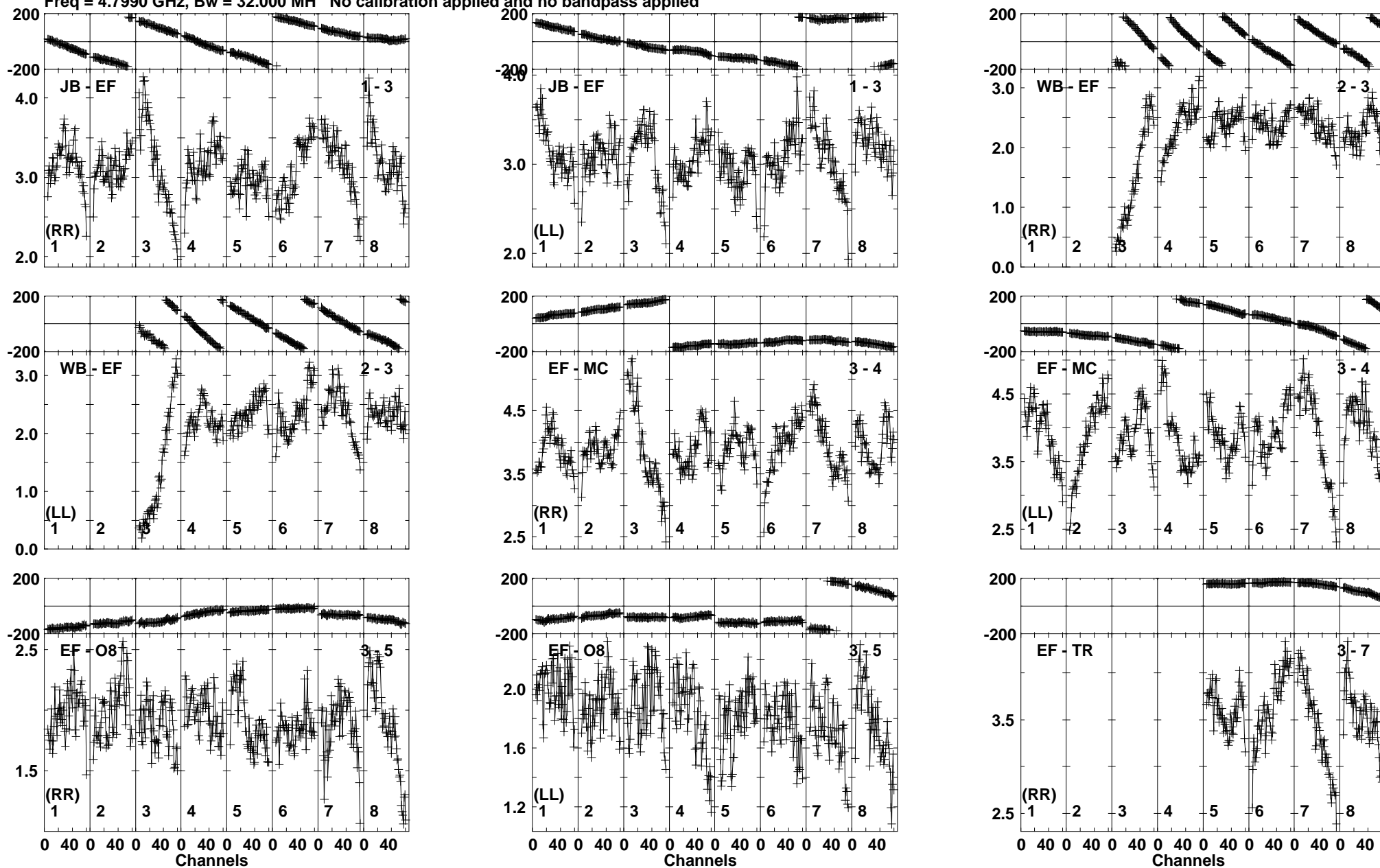
Lower frame: Milli Ampl Jy Top frame: Phas deg Vector averaged cross-power spectrum Baseline: JB (01) - EF (03) Timerange: 00/23:57:41 to 00/23:58:10
