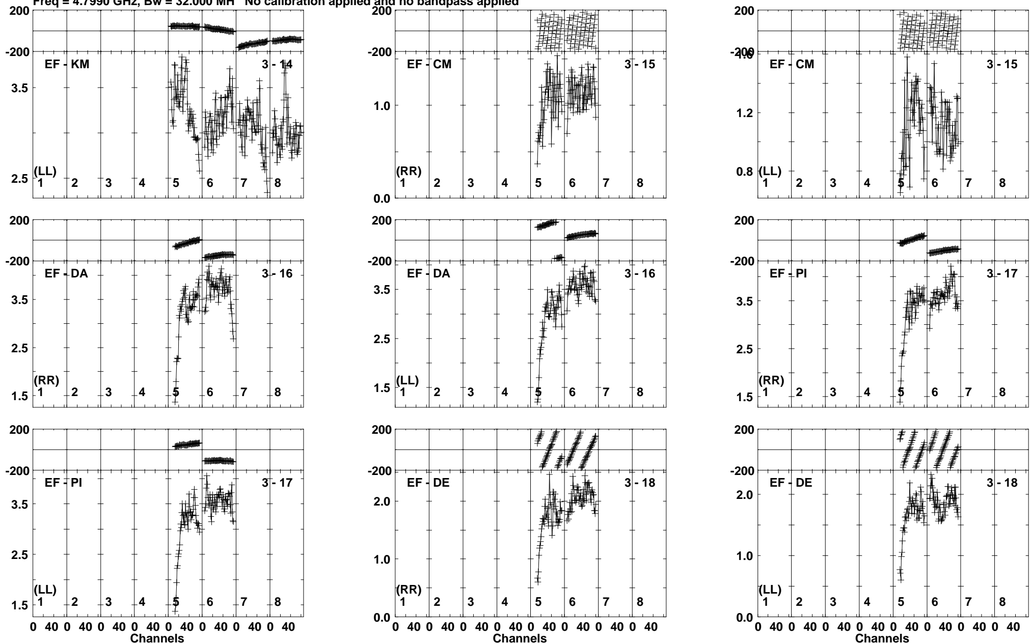
Lower frame: Milli Ampl Jy Top frame: Phas deg Vector averaged cross-power spectrum Baseline: EF (03) - KM (14) Timerange: 01/01:02:46 to 01/01:03:15
