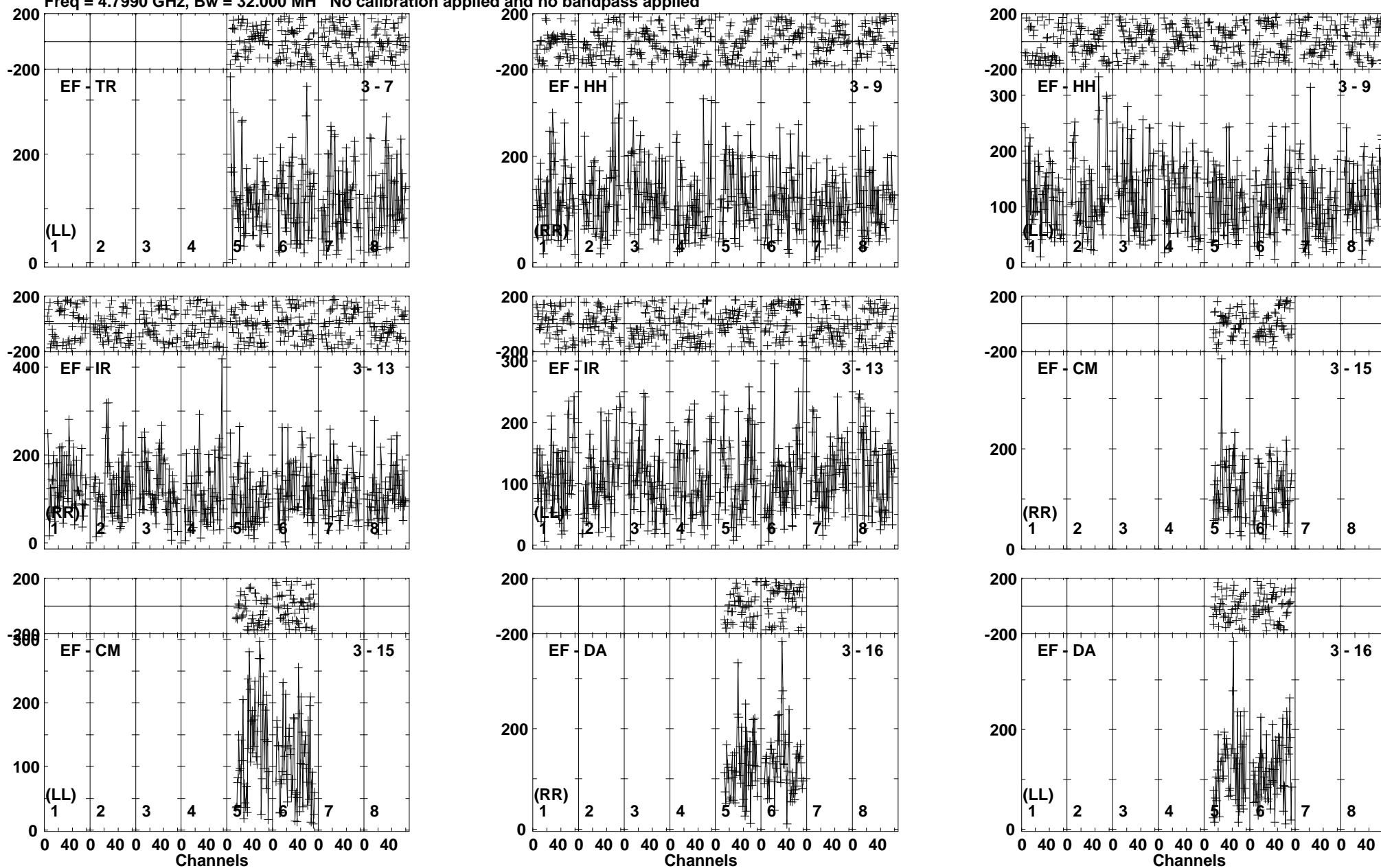
Lower frame: Micro Ampl Jy Top frame: Phas deg Vector averaged cross-power spectrum Baseline: EF (03) - TR (07) Timerange: 01/05:32:05 to 01/05:34:14
