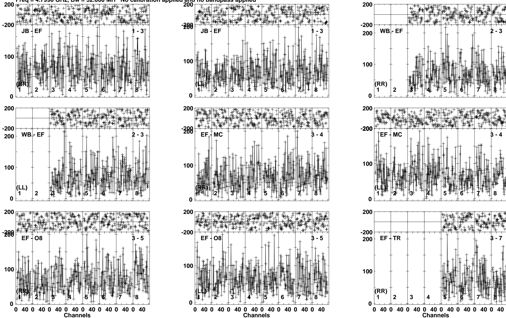
Lower frame: Micro Ampl Jy Top frame: Phas deg Vector averaged cross-power spectrum Baseline: JB (01) - EF (03) Timerange: 01/01:53:55 to 01/01:58:54
