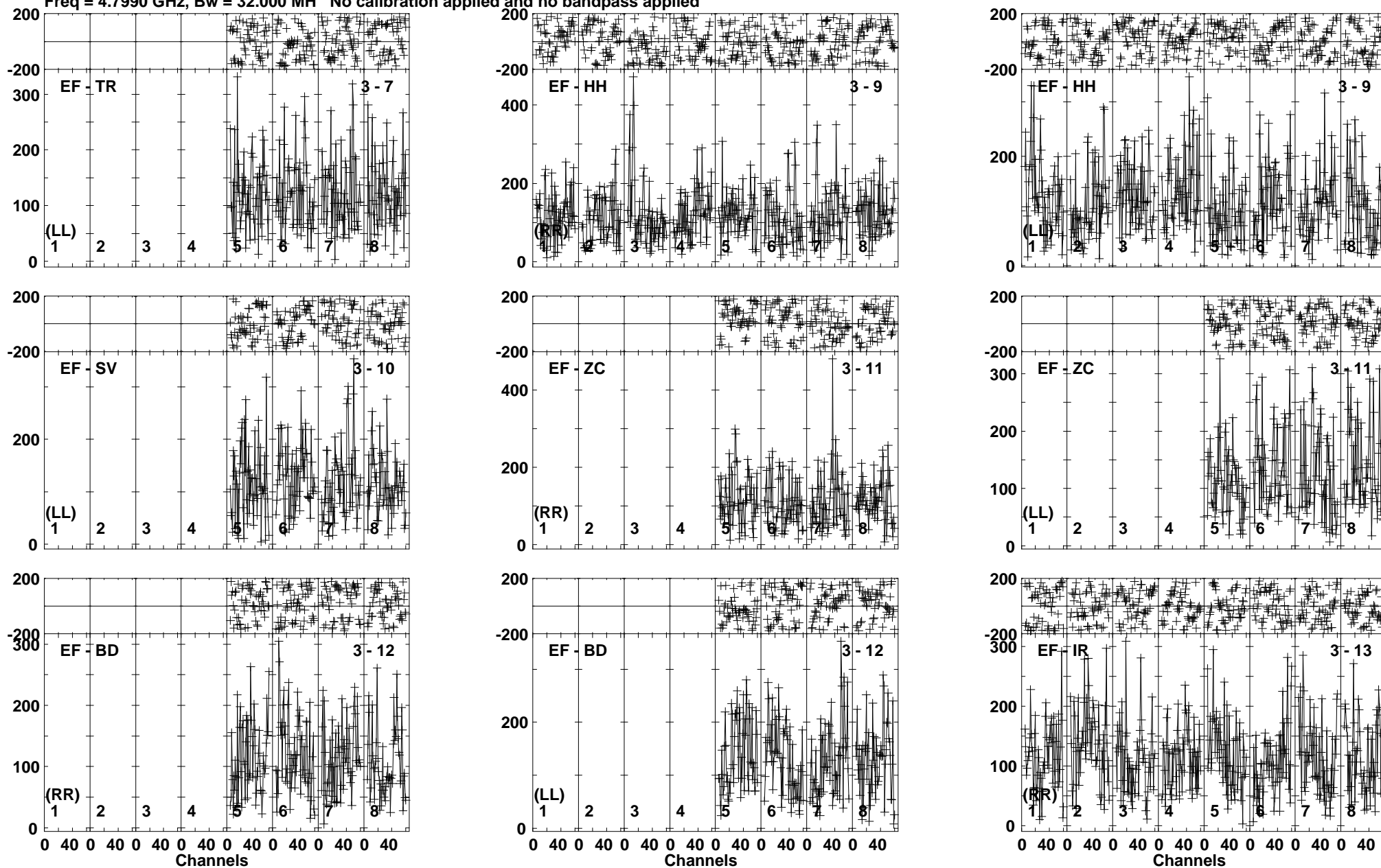
Lower frame: Micro Ampl Jy Top frame: Phas deg Vector averaged cross-power spectrum Baseline: EF (03) - TR (07) Timerange: 01/00:01:21 to 01/00:03:29
