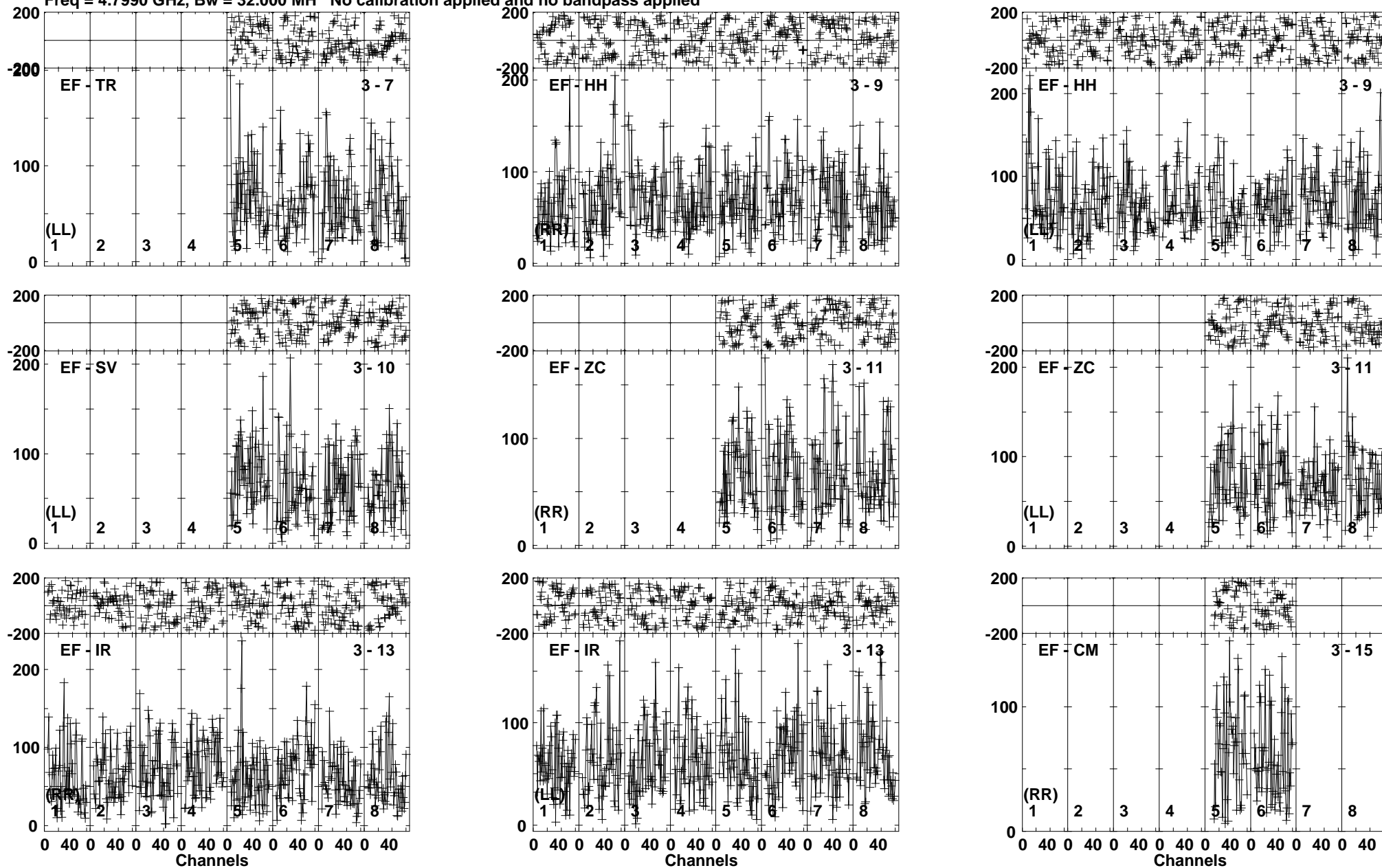
Lower frame: Micro Ampl Jy Top frame: Phas deg Vector averaged cross-power spectrum Baseline: EF (03) - TR (07) Timerange: 01/03:25:15 to 01/03:30:14
