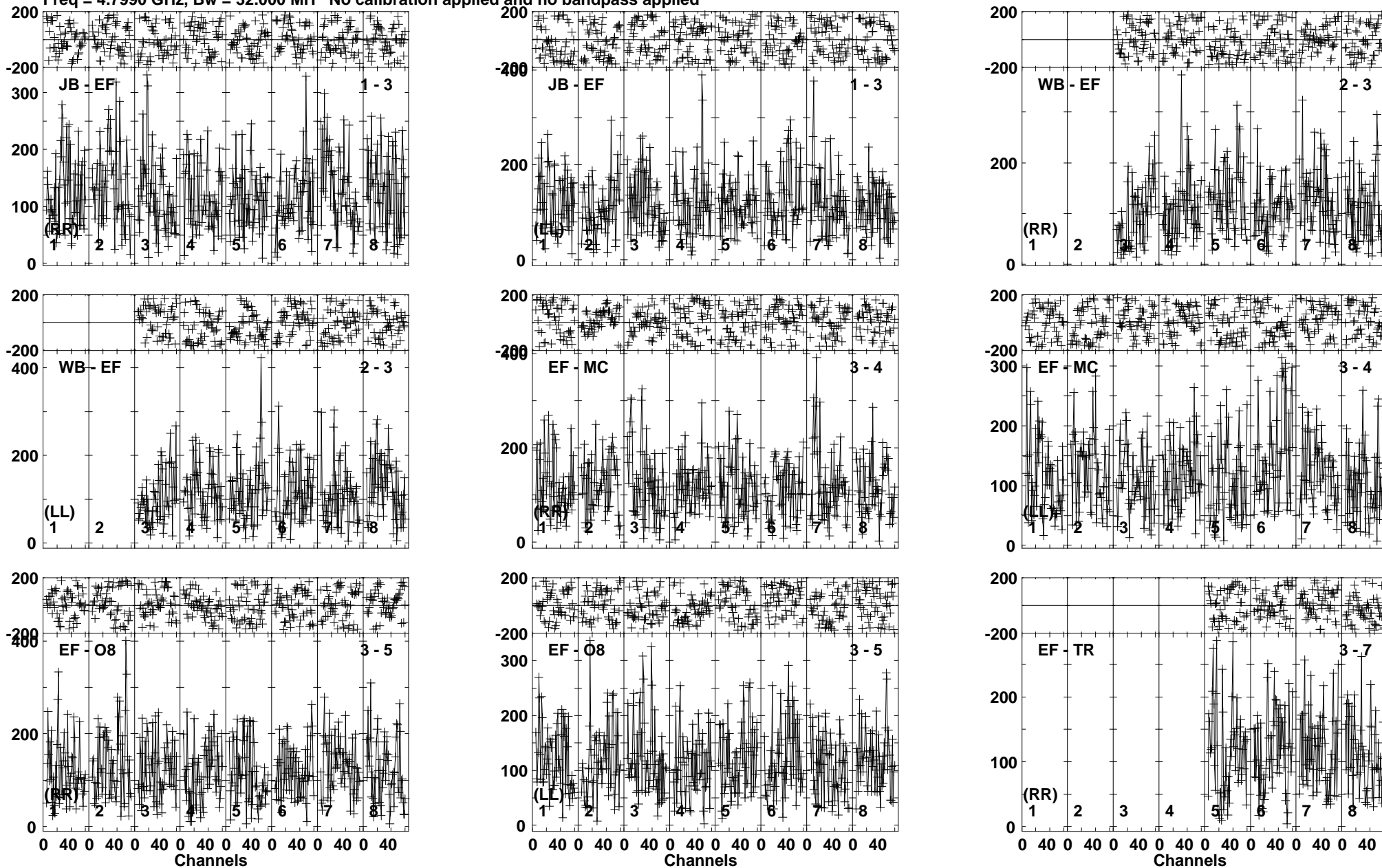
Lower frame: Micro Ampl Jy Top frame: Phas deg Vector averaged cross-power spectrum Baseline: JB (01) - EF (03) Timerange: 01/06:02:16 to 01/06:04:24
