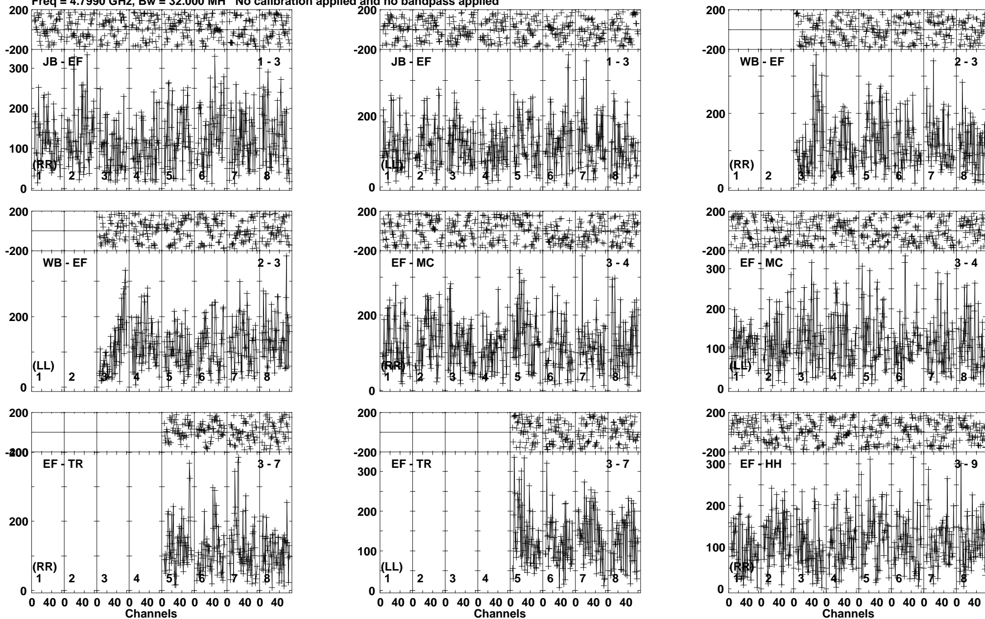
Lower frame: Micro Ampl Jy Top frame: Phas deg Vector averaged cross-power spectrum Baseline: JB (01) - EF (03) Timerange: 01/06:39:35 to 01/06:41:44
