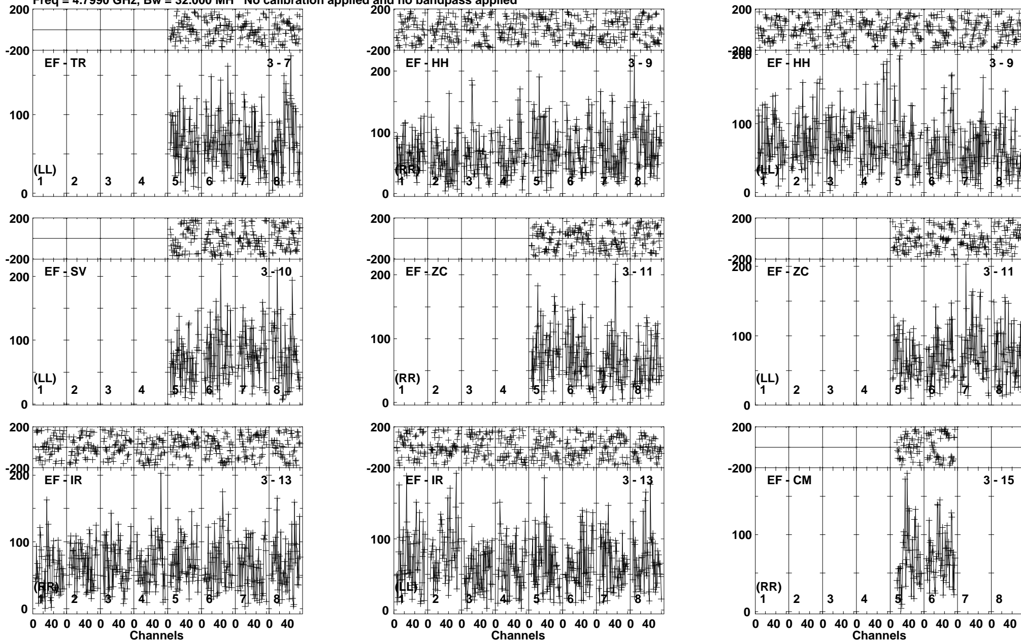
Lower frame: Micro Ampl Jy Top frame: Phas deg Vector averaged cross-power spectrum Baseline: EF (03) - TR (07) Timerange: 01/03:18:35 to 01/03:23:34
