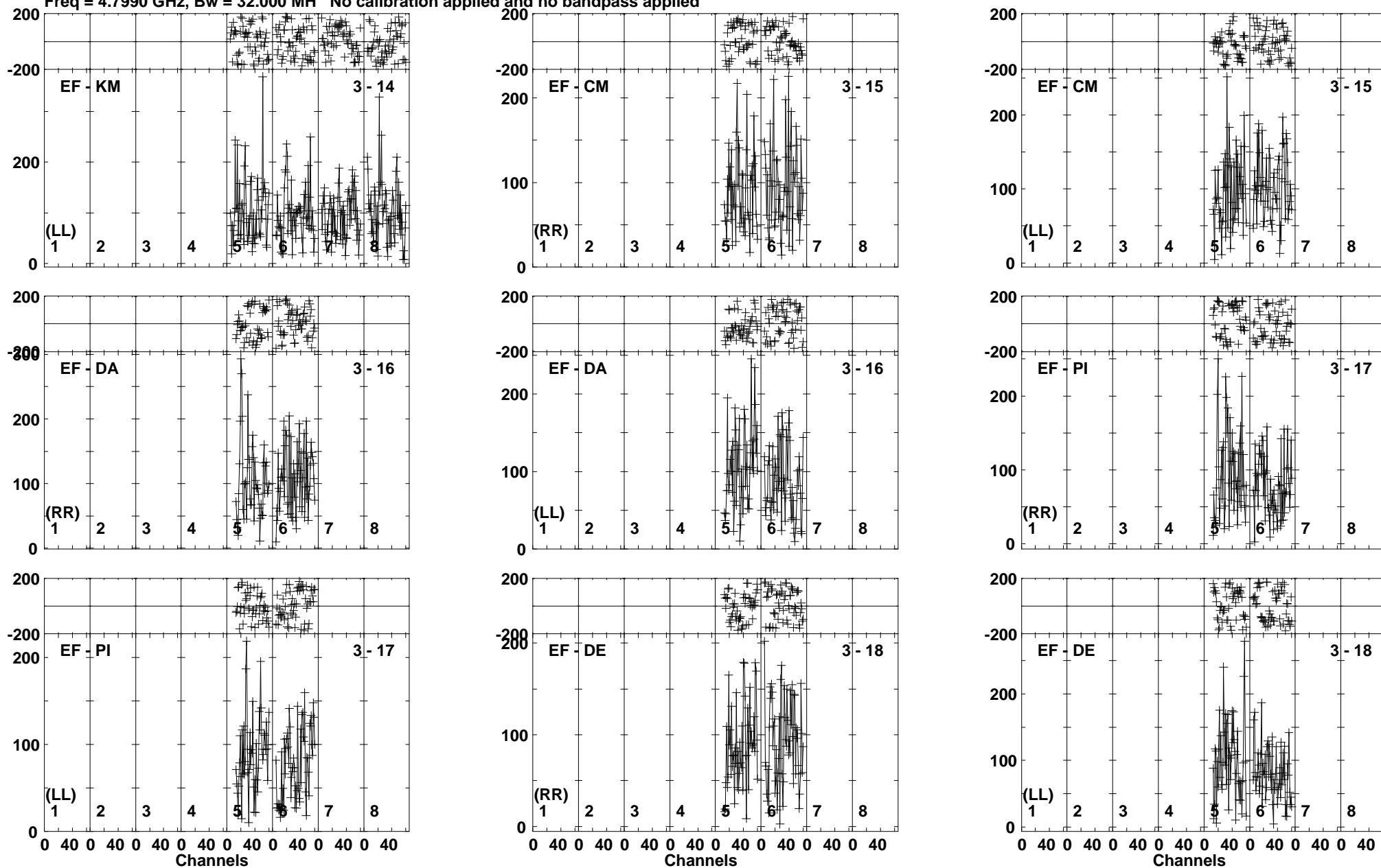
Lower frame: Micro Ampl Jy Top frame: Phas deg Vector averaged cross-power spectrum Baseline: EF (03) - KM (14) Timerange: 01/01:05:45 to 01/01:08:15
