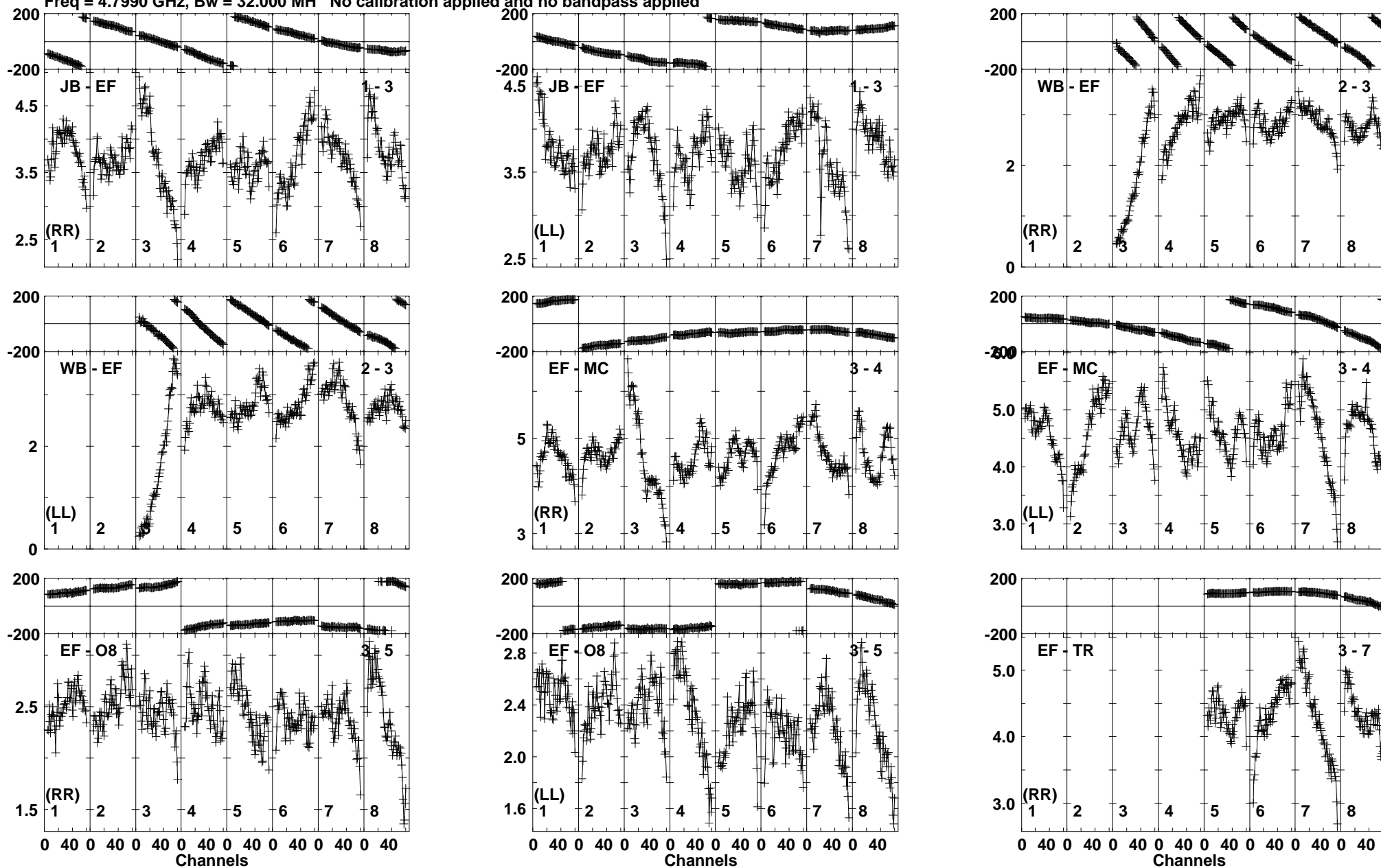
Lower frame: Milli Ampl Jy Top frame: Phas deg Vector averaged cross-power spectrum Baseline: JB (01) - EF (03) Timerange: 01/00:55:56 to 01/00:56:54
