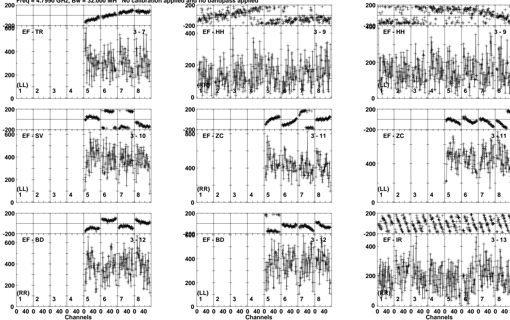
Lower frame: Micro Ampl Jy Top frame: Phas deg Vector averaged cross-power spectrum Baseline: EF (03) - TR (07) Timerange: 00/23:19:11 to 00/23:21:20
