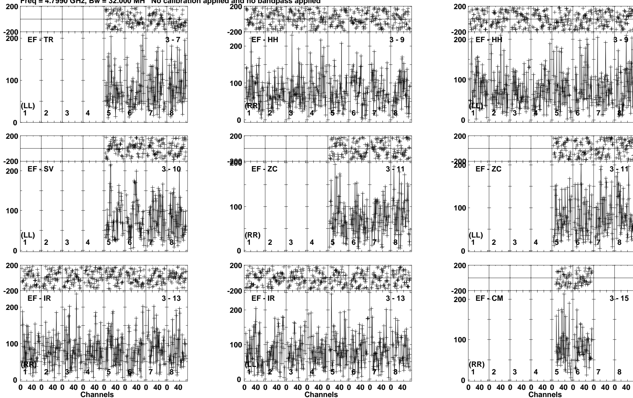
Lower frame: Micro Ampl Jy Top frame: Phas deg Vector averaged cross-power spectrum Baseline: EF (03) - TR (07) Timerange: 01/04:13:35 to 01/04:17:04
