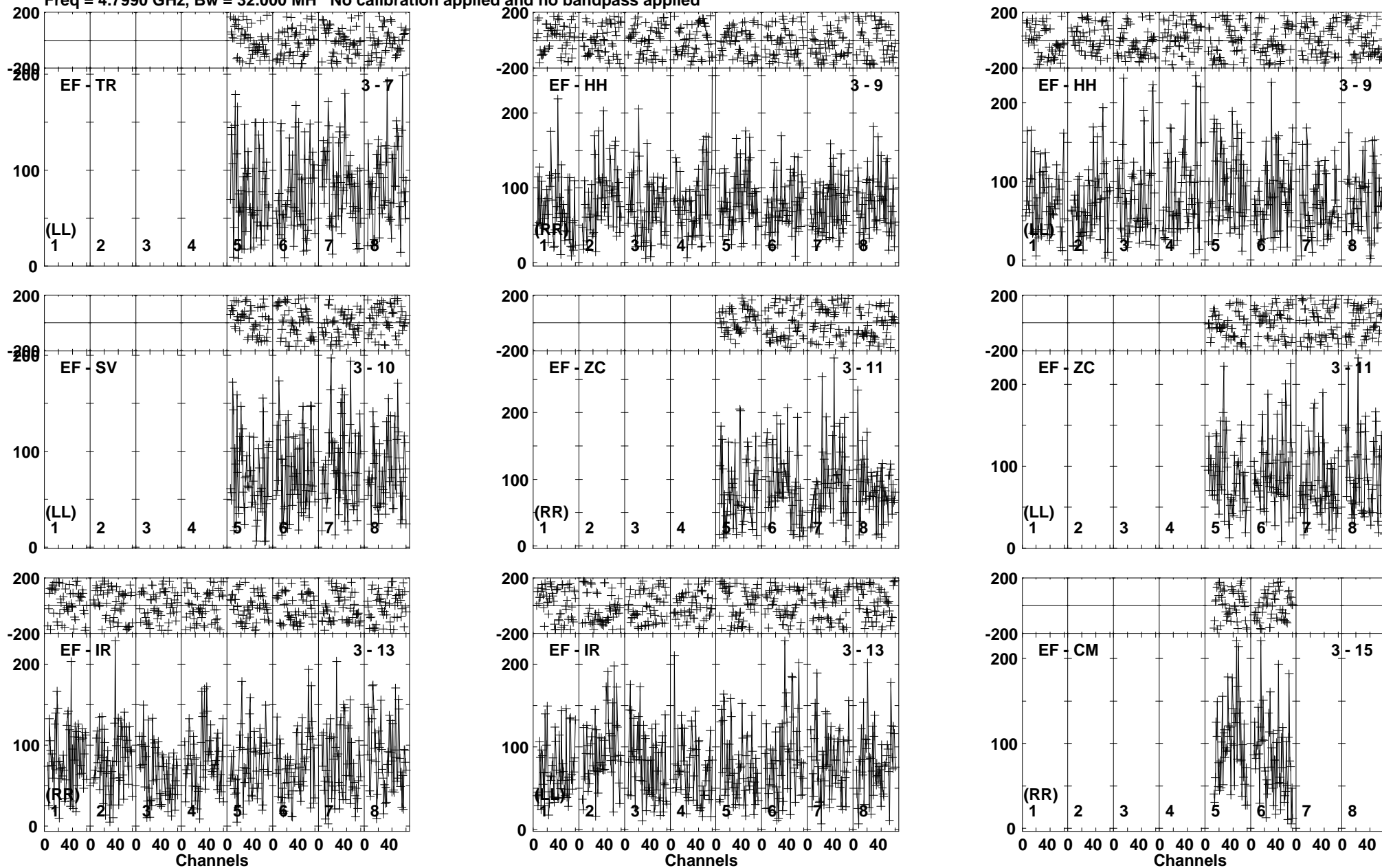
Lower frame: Micro Ampl Jy Top frame: Phas deg Vector averaged cross-power spectrum Baseline: EF (03) - TR (07) Timerange: 01/03:14:06 to 01/03:17:35
