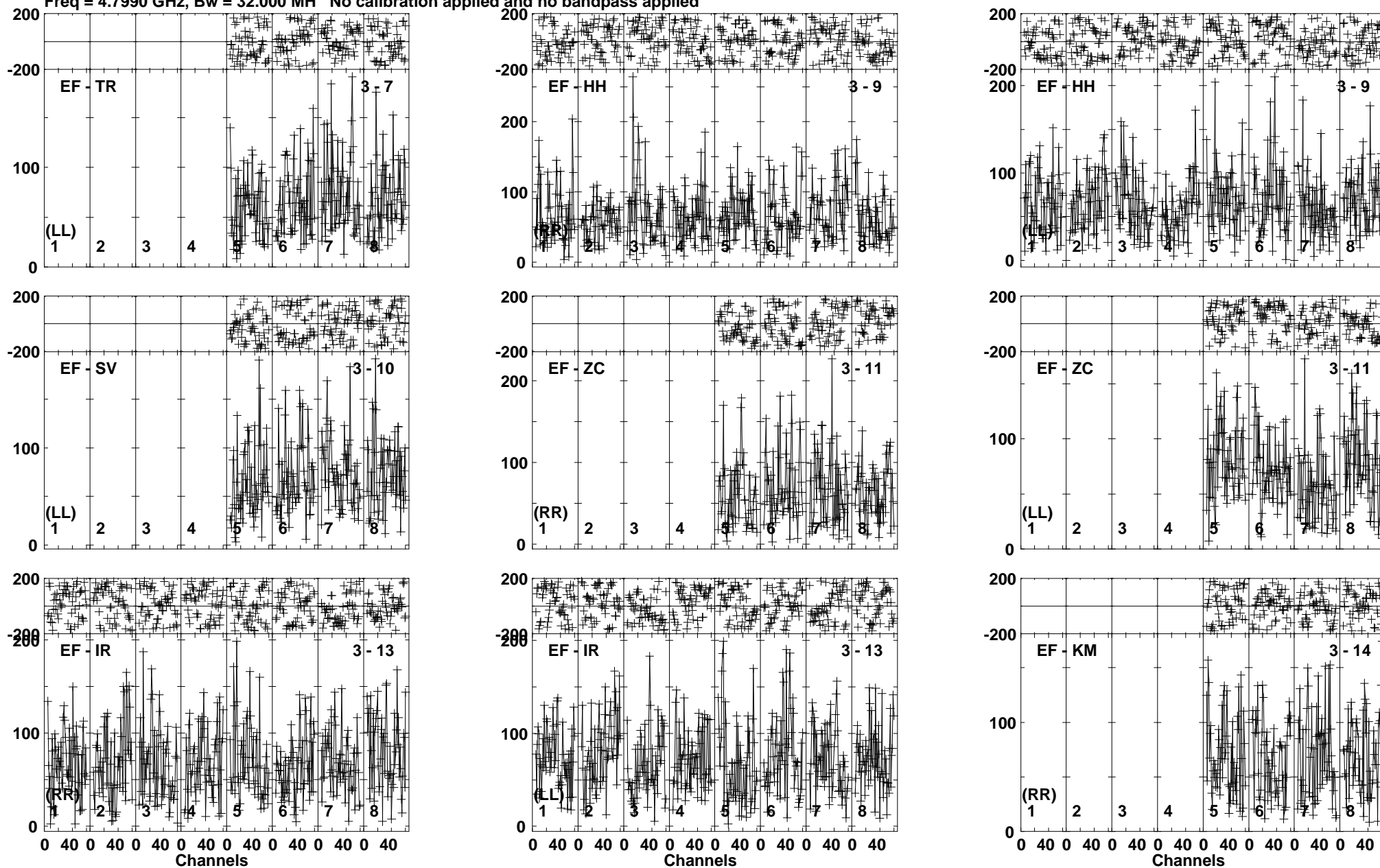
Lower frame: Micro Ampl Jy Top frame: Phas deg Vector averaged cross-power spectrum Baseline: EF (03) - TR (07) Timerange: 01/01:09:15 to 01/01:14:14
