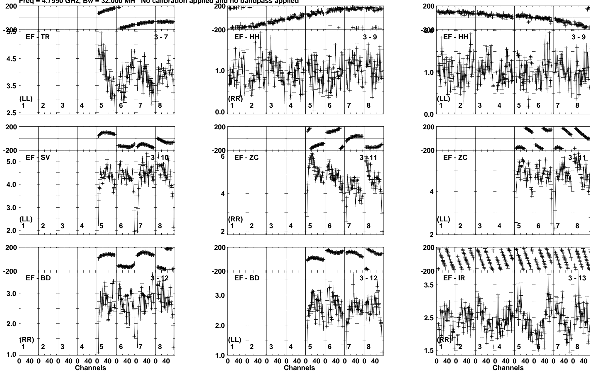
Lower frame: Milli Ampl Jy Top frame: Phas deg Vector averaged cross-power spectrum Baseline: EF (03) - TR (07) Timerange: 01/00:06:41 to 01/00:07:39
