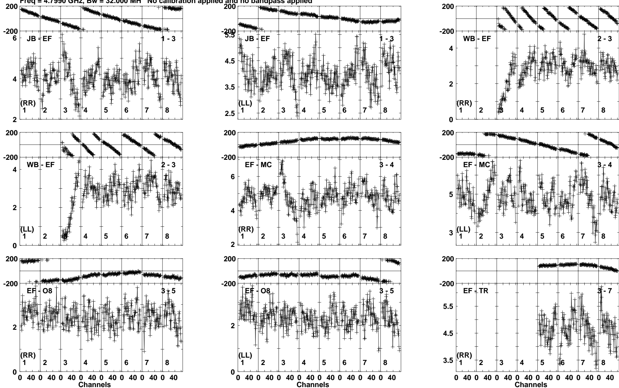
Lower frame: Milli Ampl Jy Top frame: Phas deg Vector averaged cross-power spectrum Baseline: JB (01) - EF (03) Timerange: 01/02:24:16 to 01/02:25:14
