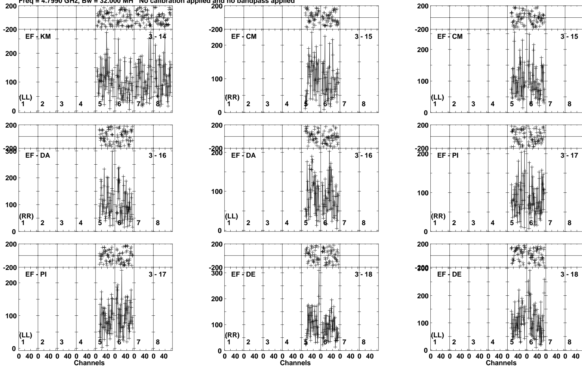
Lower frame: Micro Ampl Jy Top frame: Phas deg Vector averaged cross-power spectrum Baseline: EF (03) - KM (14) Timerange: 01/00:46:45 to 01/00:49:15
