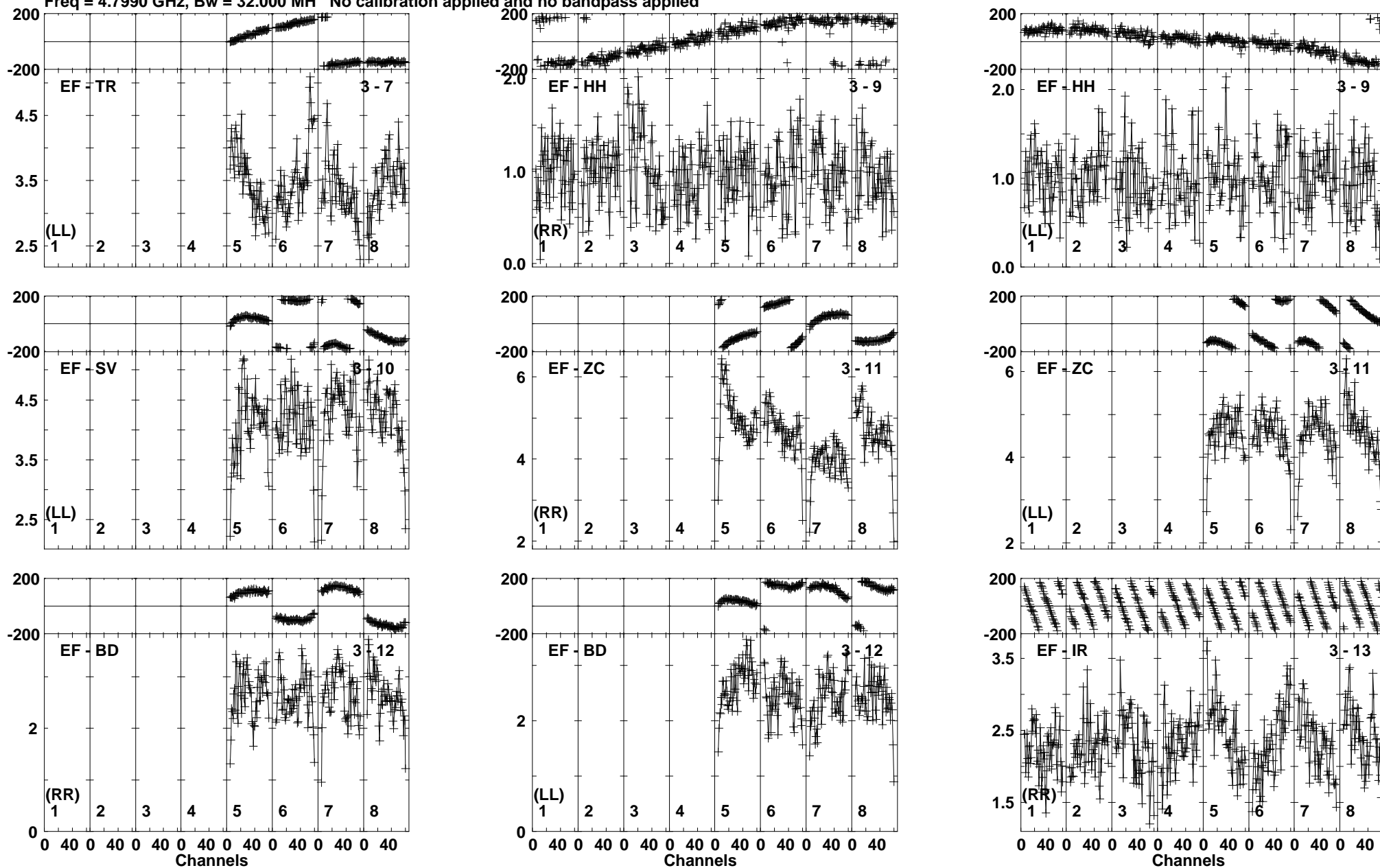
Lower frame: Milli Ampl Jy Top frame: Phas deg Vector averaged cross-power spectrum Baseline: EF (03) - TR (07) Timerange: 01/00:00:20 to 01/00:01:19
