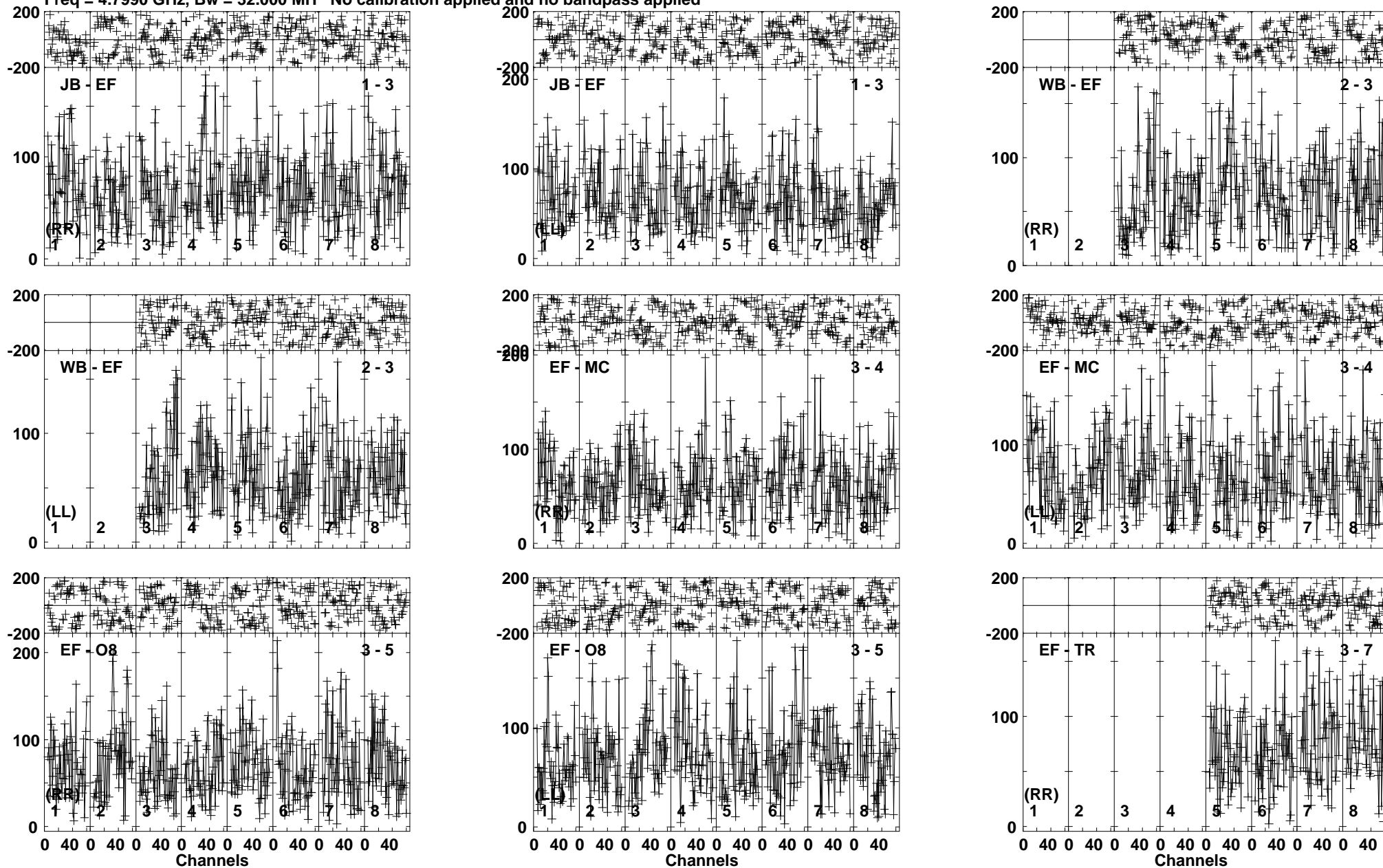
Lower frame: Micro Ampl Jy Top frame: Phas deg Vector averaged cross-power spectrum Baseline: JB (01) - EF (03) Timerange: 01/01:47:15 to 01/01:52:14
