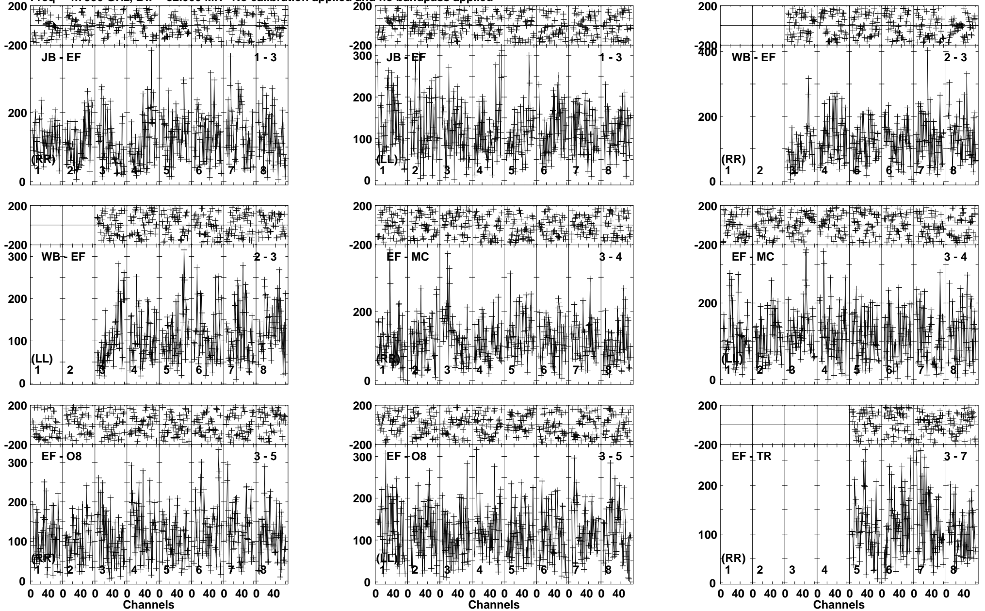
Lower frame: Micro Ampl Jy Top frame: Phas deg Vector averaged cross-power spectrum Baseline: JB (01) - EF (03) Timerange: 01/06:29:15 to 01/06:31:24
