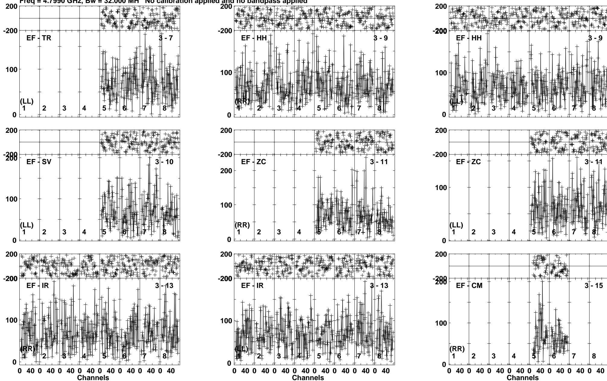
Lower frame: Micro Ampl Jy Top frame: Phas deg Vector averaged cross-power spectrum Baseline: EF (03) - TR (07) Timerange: 01/02:06:15 to 01/02:11:14
