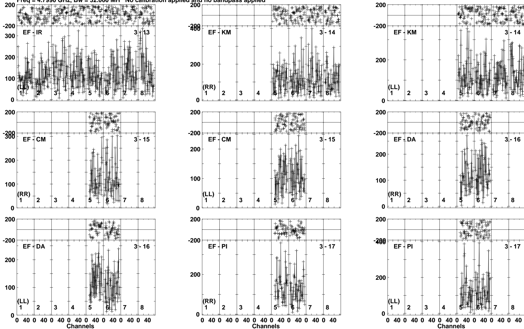
Lower frame: Micro Ampl Jy Top frame: Phas deg Vector averaged cross-power spectrum Baseline: EF (03) - IR (13) Timerange: 01/00:01:21 to 01/00:03:29
