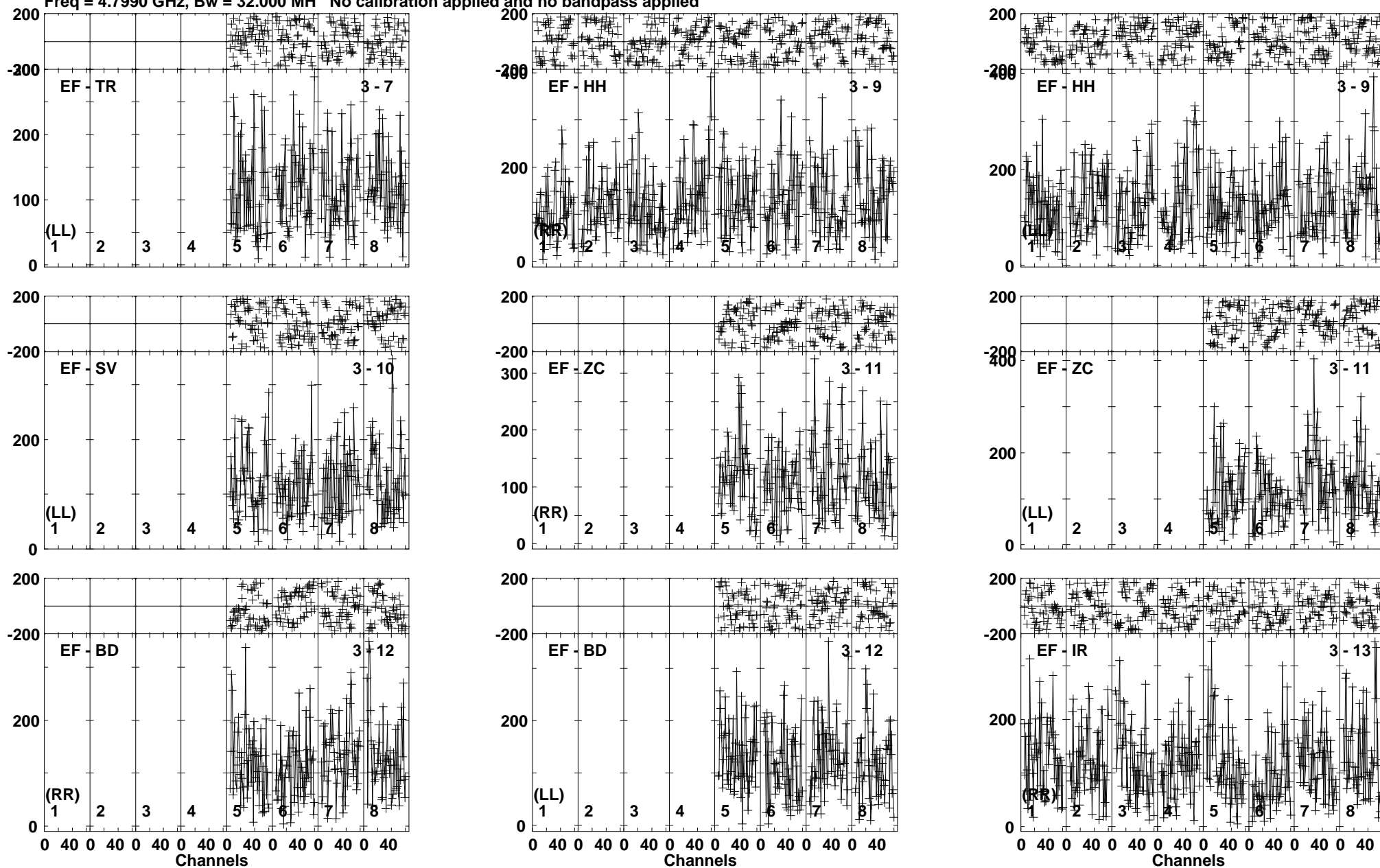
Lower frame: Micro Ampl Jy Top frame: Phas deg Vector averaged cross-power spectrum Baseline: EF (03) - TR (07) Timerange: 00/22:59:31 to 00/23:01:39
