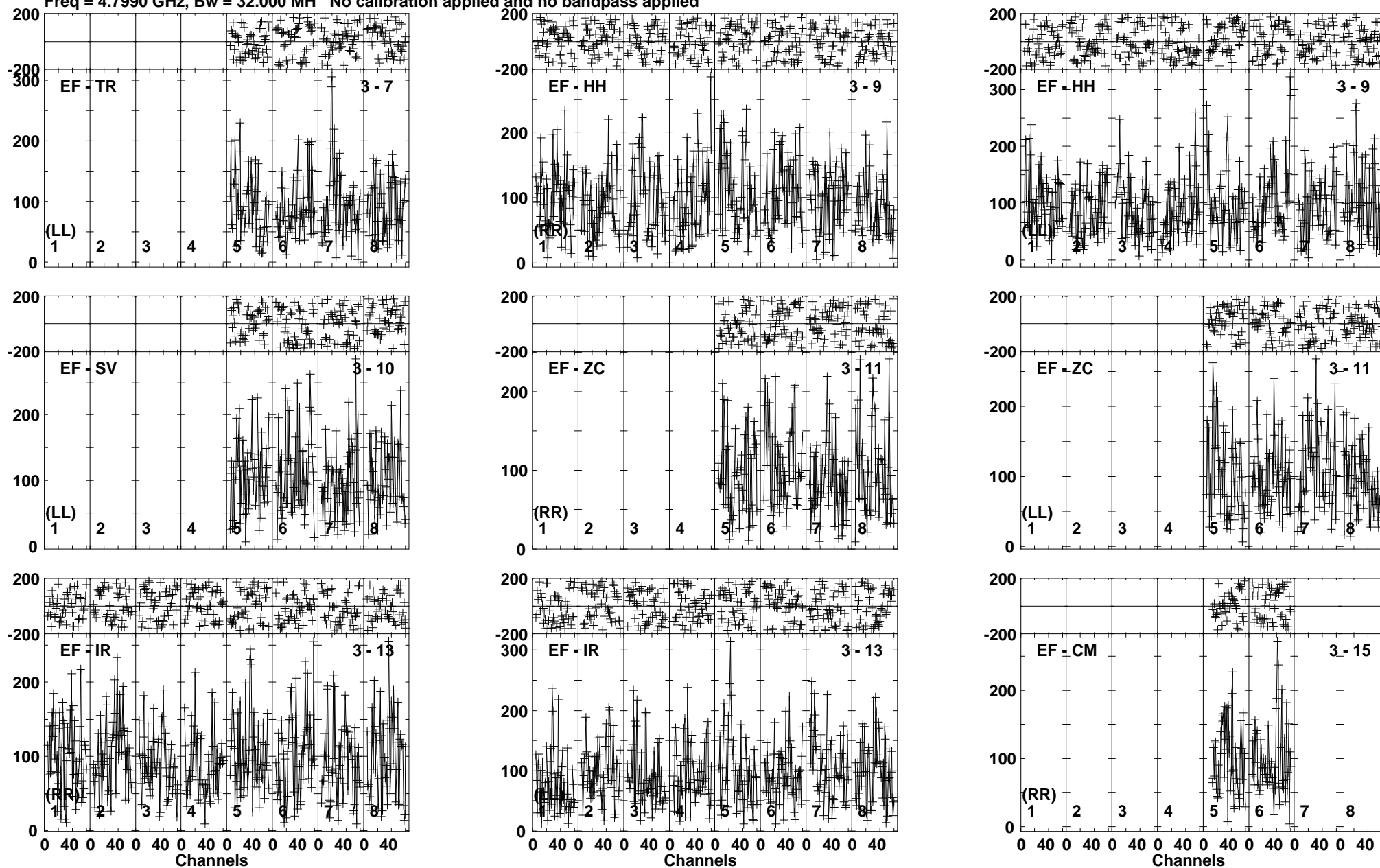
Lower frame: Micro Ampl Jy Top frame: Phas deg Vector averaged cross-power spectrum Baseline: EF (03) - TR (07) Timerange: 01/02:02:45 to 01/02:05:15
