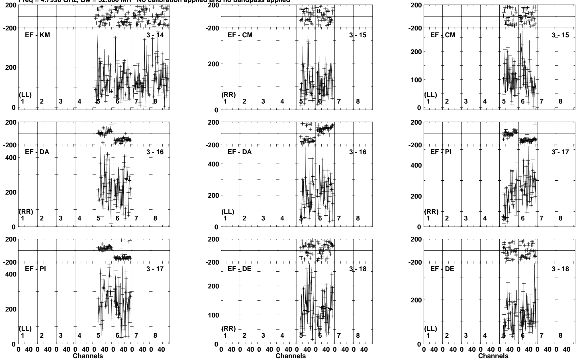
Lower frame: Micro Ampl Jy Top frame: Phas deg Vector averaged cross-power spectrum Baseline: EF (03) - KM (14) Timerange: 01/00:31:46 to 01/00:33:54
