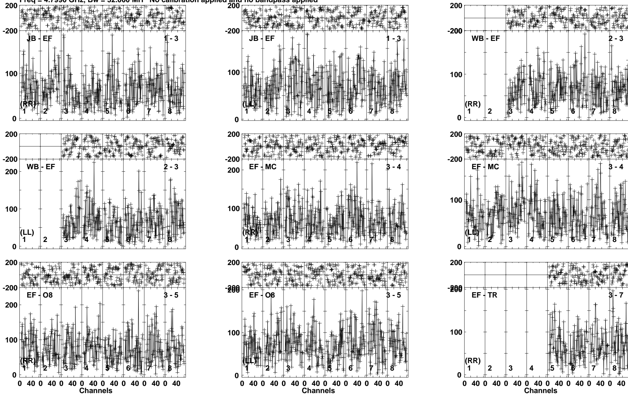
Lower frame: Micro Ampl Jy Top frame: Phas deg Vector averaged cross-power spectrum Baseline: JB (01) - EF (03) Timerange: 01/03:58:15 to 01/04:03:14
