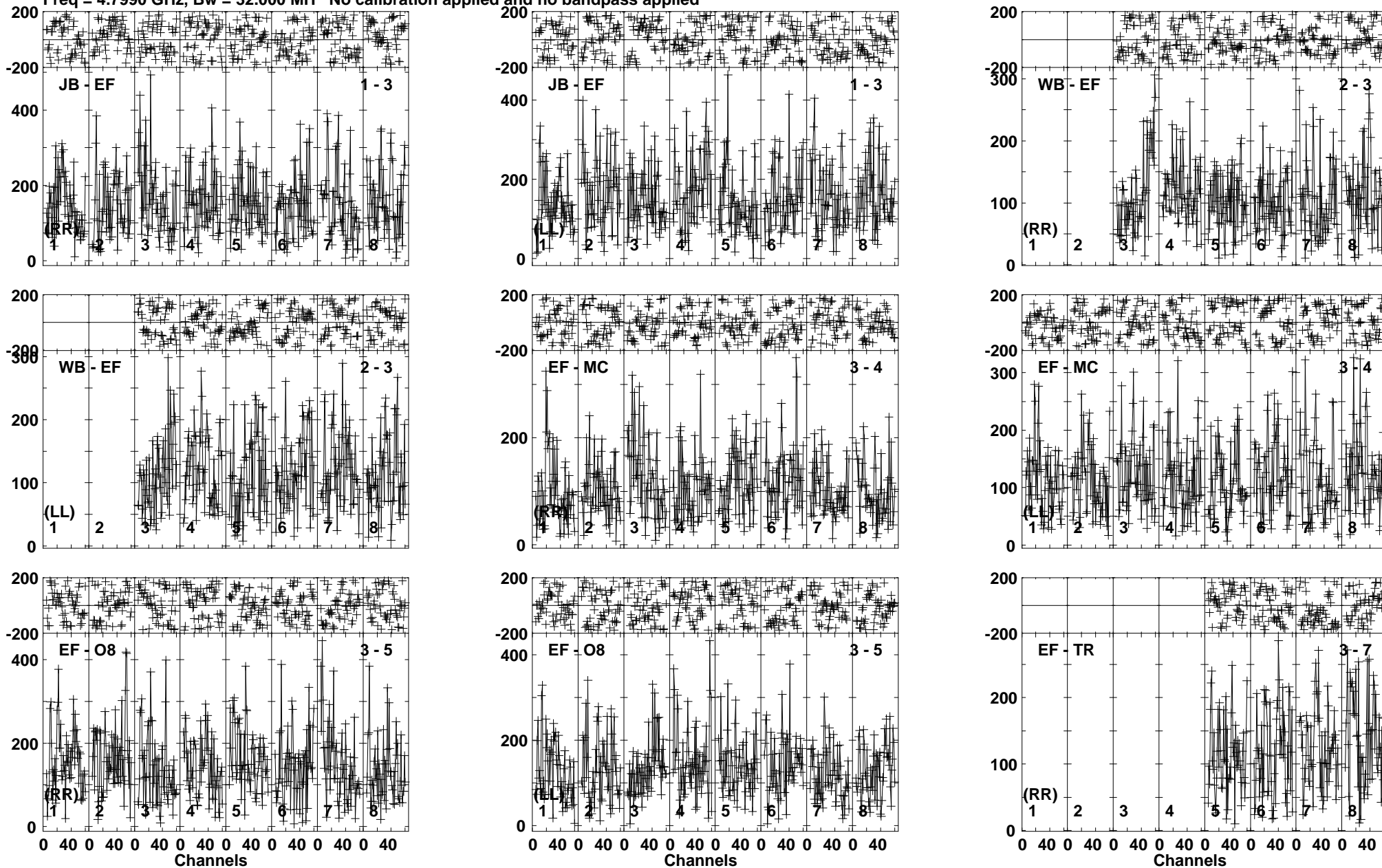
Lower frame: Micro Ampl Jy Top frame: Phas deg Vector averaged cross-power spectrum Baseline: JB (01) - EF (03) Timerange: 01/05:14:45 to 01/05:16:54
