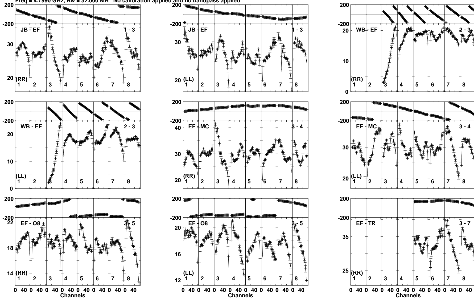
Lower frame: Milli Ampl Jy Top frame: Phas deg Vector averaged cross-power spectrum Baseline: JB (01) - EF (03) Timerange: 01/02:44:36 to 01/02:47:35
