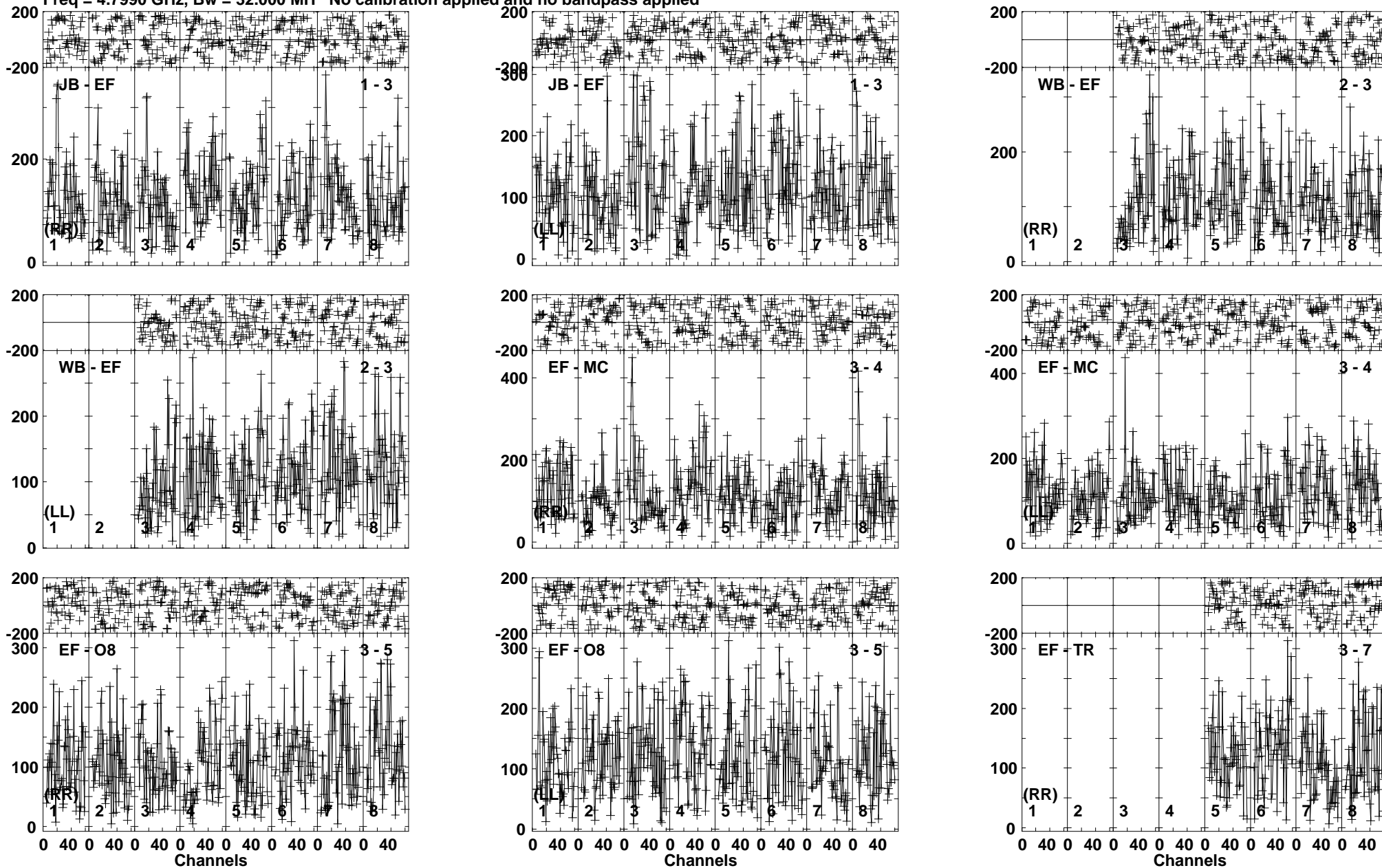
Lower frame: Micro Ampl Jy Top frame: Phas deg Vector averaged cross-power spectrum Baseline: JB (01) - EF (03) Timerange: 01/06:22:15 to 01/06:24:24
