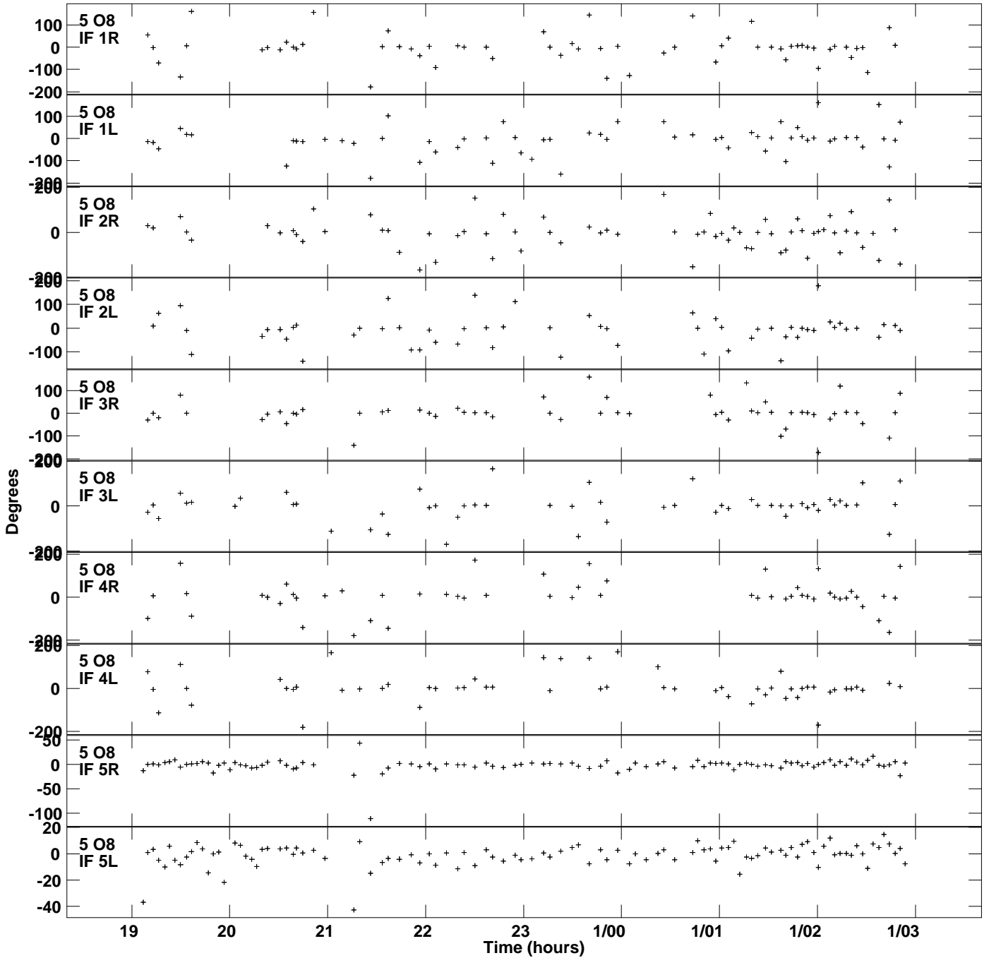
Plot file version 7 created 14-NOV-2019 18:57:45 Gain phs vs UTC time for J0300-0846.MULTI.1 SN 1 Rpol & Lpol IF 1 - 8
