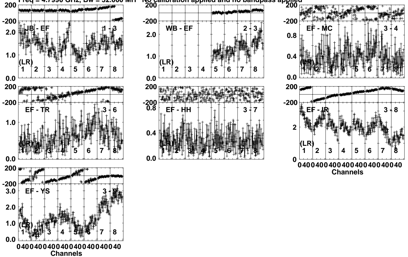
Lower frame: Milli Ampl Jy Top frame: Phas deg Vector averaged cross-power spectrum Several baselines displayed Timerange: 00/20:37:10 to 00/20:37:59
