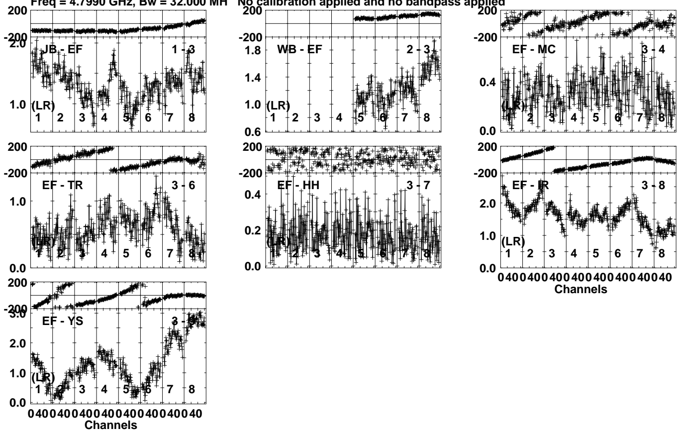
Lower frame: Milli Ampl Jy Top frame: Phas deg Vector averaged cross-power spectrum Several baselines displayed Timerange: 00/21:39:41 to 00/21:40:19
