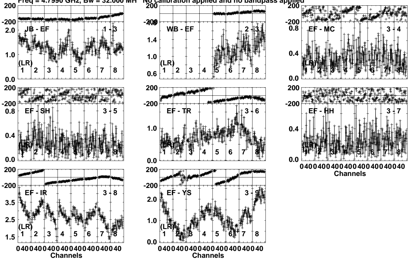
Lower frame: Milli Ampl Jy Top frame: Phas deg Vector averaged cross-power spectrum Several baselines displayed Timerange: 00/16:46:40 to 00/16:47:19
