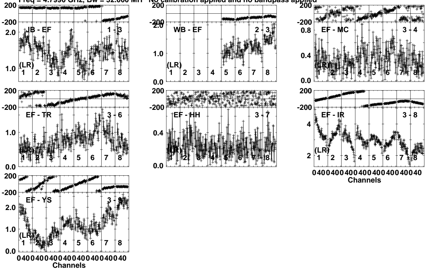
Lower frame: Milli Ampl Jy Top frame: Phas deg Vector averaged cross-power spectrum Several baselines displayed Timerange: 00/18:22:10 to 00/18:22:59
