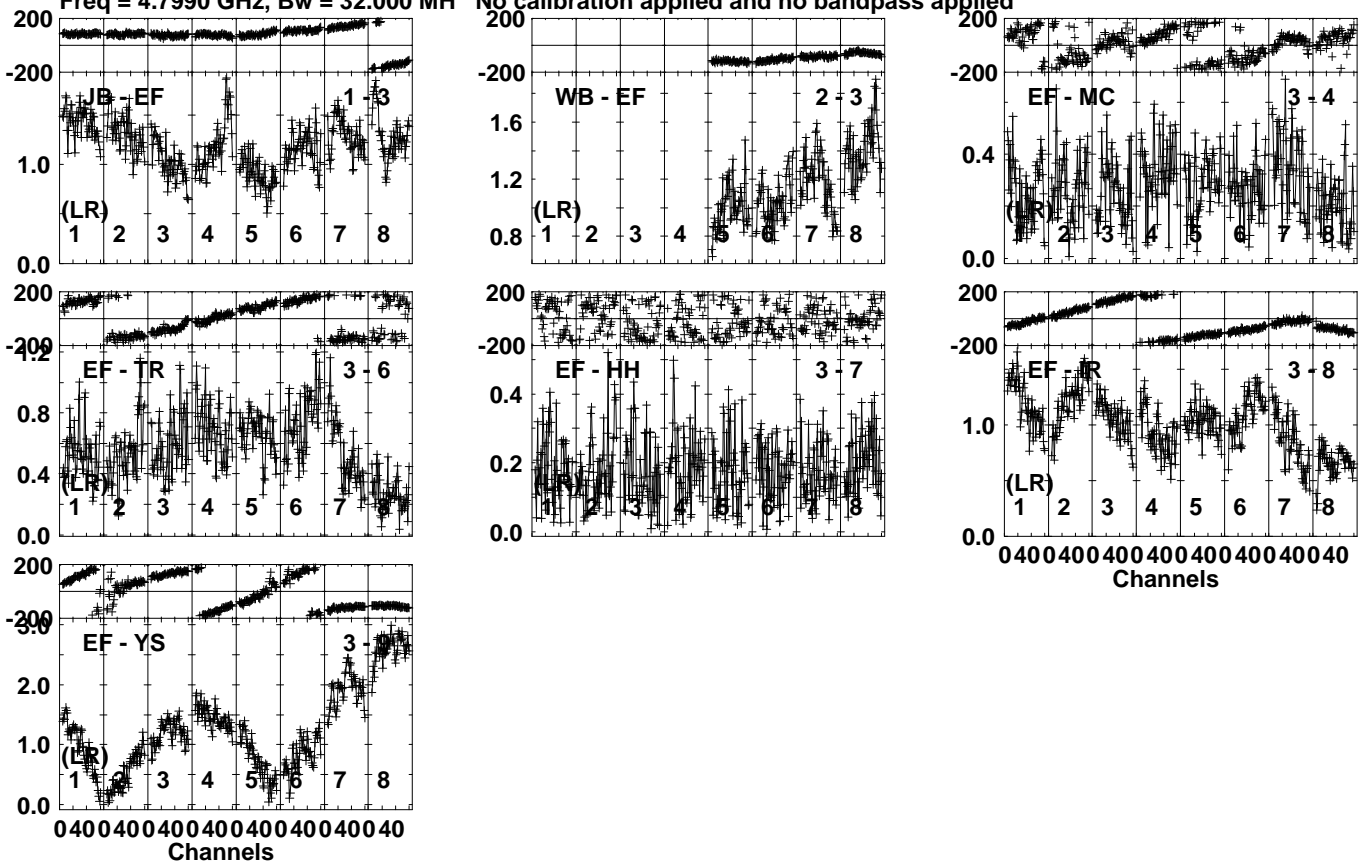
Lower frame: Milli Ampl Jy Top frame: Phas deg Vector averaged cross-power spectrum Several baselines displayed Timerange: 00/22:13:11 to 00/22:13:50
