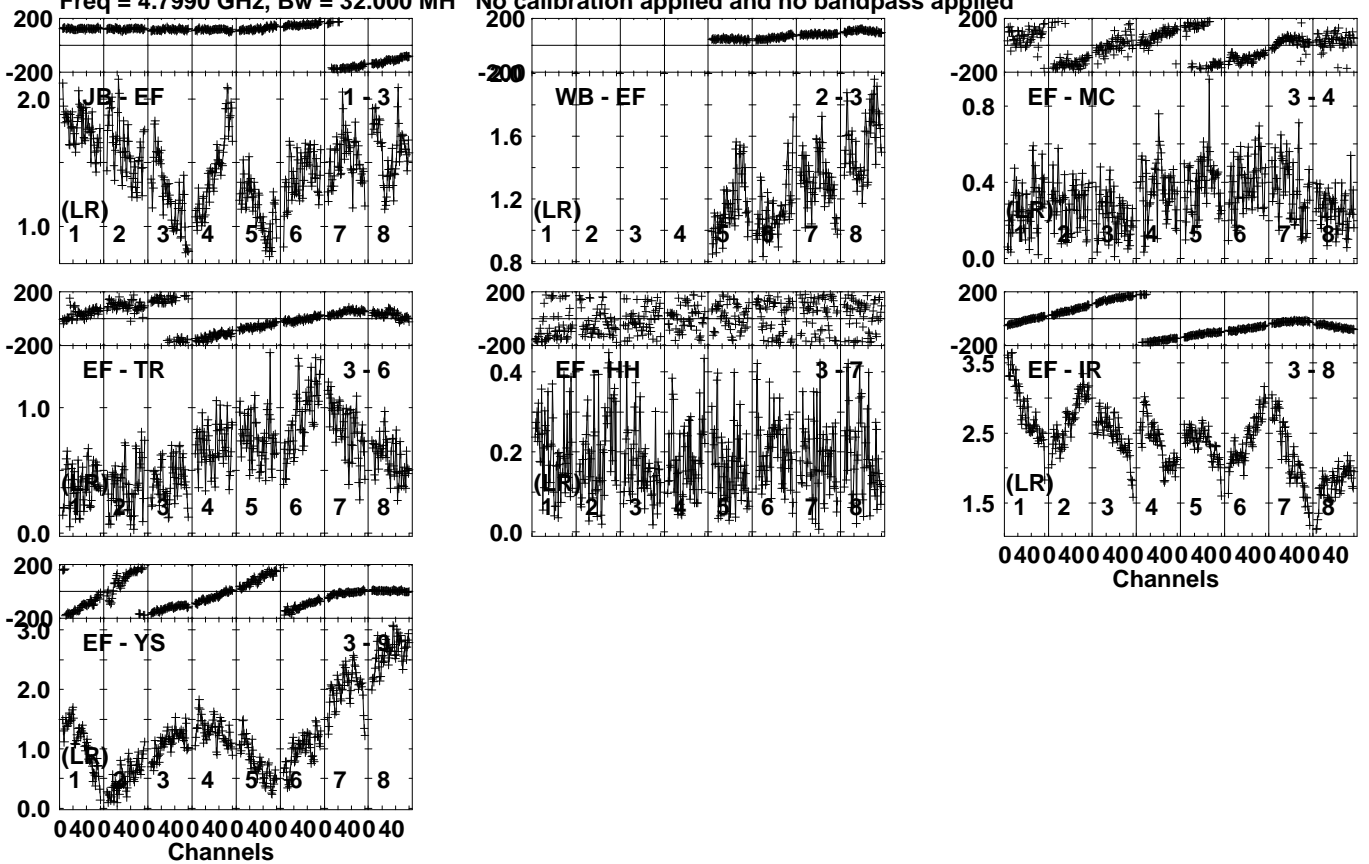
Lower frame: Milli Ampl Jy Top frame: Phas deg Vector averaged cross-power spectrum Several baselines displayed Timerange: 00/20:20:11 to 00/20:20:50
