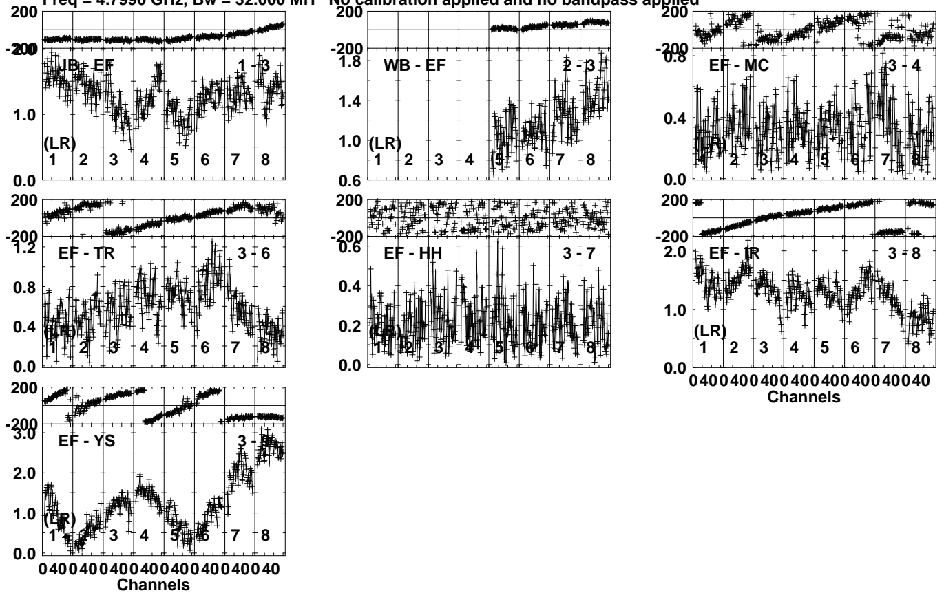
Lower frame: Milli Ampl Jy Top frame: Phas deg Vector averaged cross-power spectrum Several baselines displayed Timerange: 00/21:50:11 to 00/21:50:50
