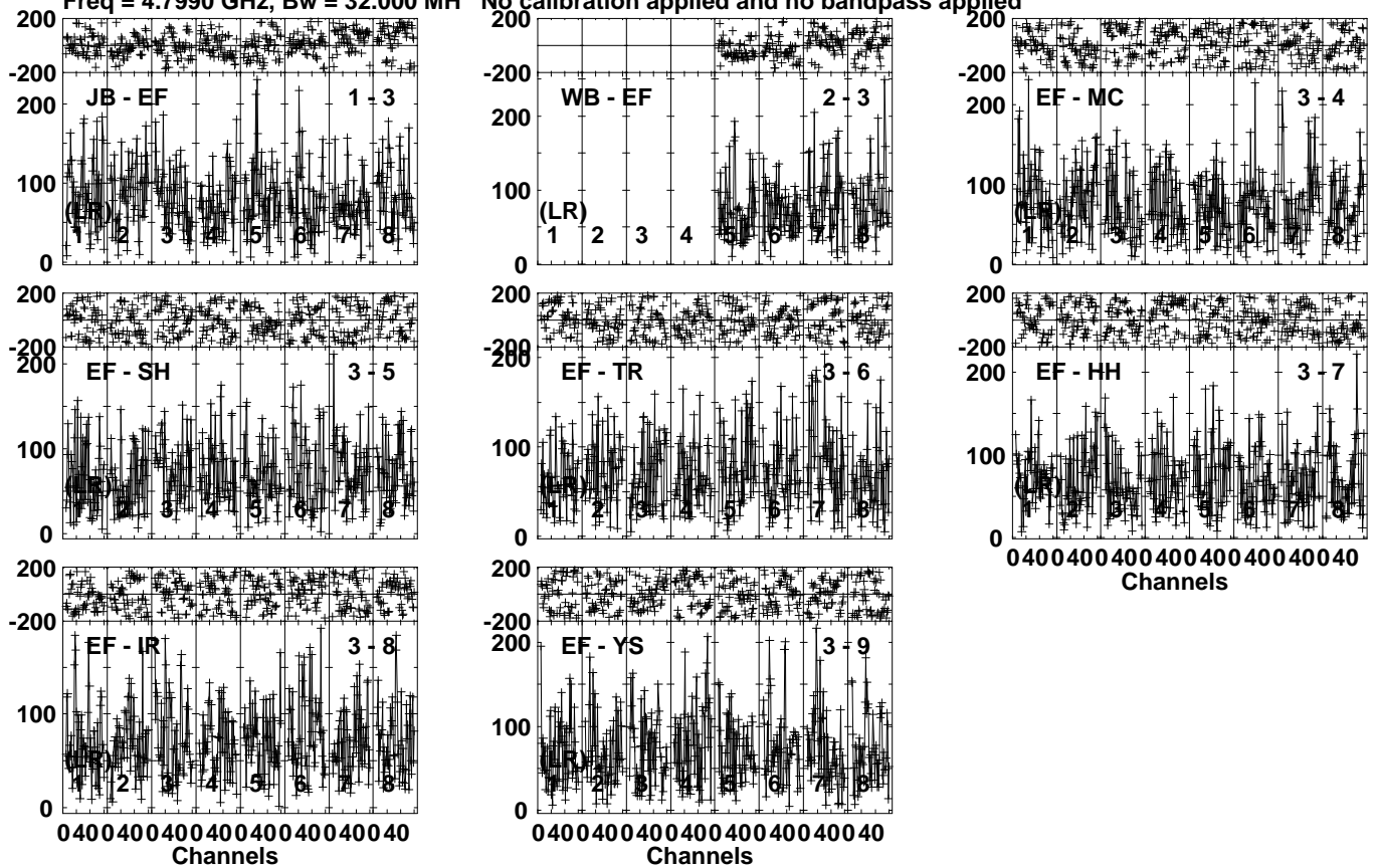
Lower frame: Micro Ampl Jy Top frame: Phas deg Vector averaged cross-power spectrum Several baselines displayed Timerange: 00/16:47:40 to 00/16:51:50
