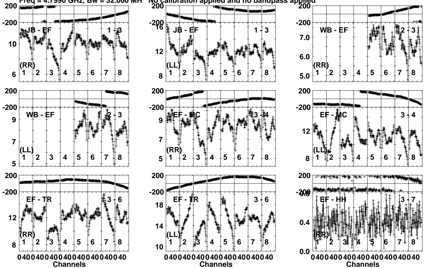
Lower frame: Milli Ampl Jy Top frame: Phas deg Vector averaged cross-power spectrum Several baselines displayed Timerange: 00/18:16:40 to 00/18:17:19
