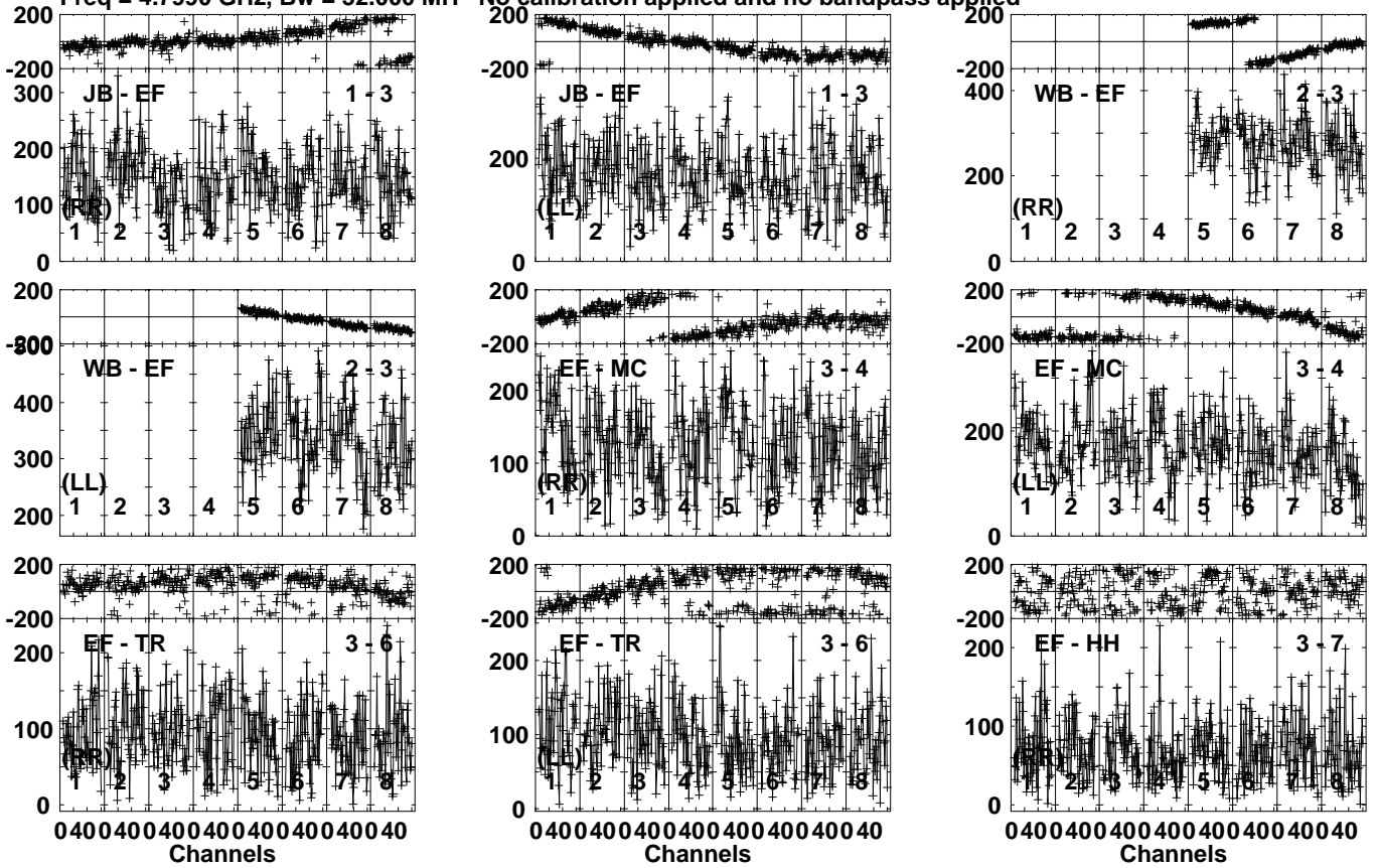
Lower frame: Micro Ampl Jy Top frame: Phas deg Vector averaged cross-power spectrum Several baselines displayed Timerange: 00:19:53:20 to 00:19:57:30
