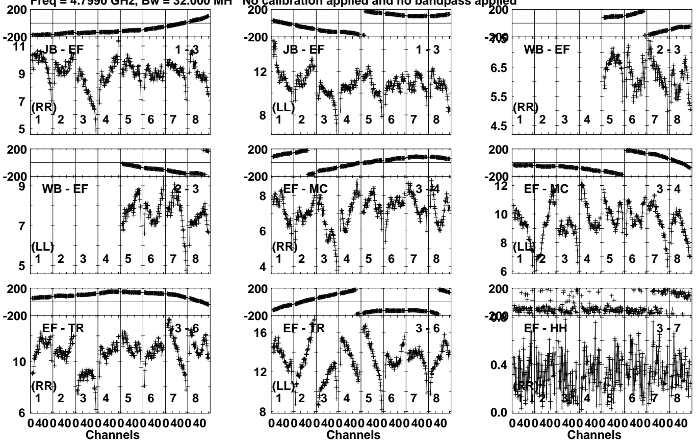
Lower frame: Milli Ampl Jy Top frame: Phas deg Vector averaged cross-power spectrum Several baselines displayed Timerange: 00/21:55:40 to 00/21:56:30
