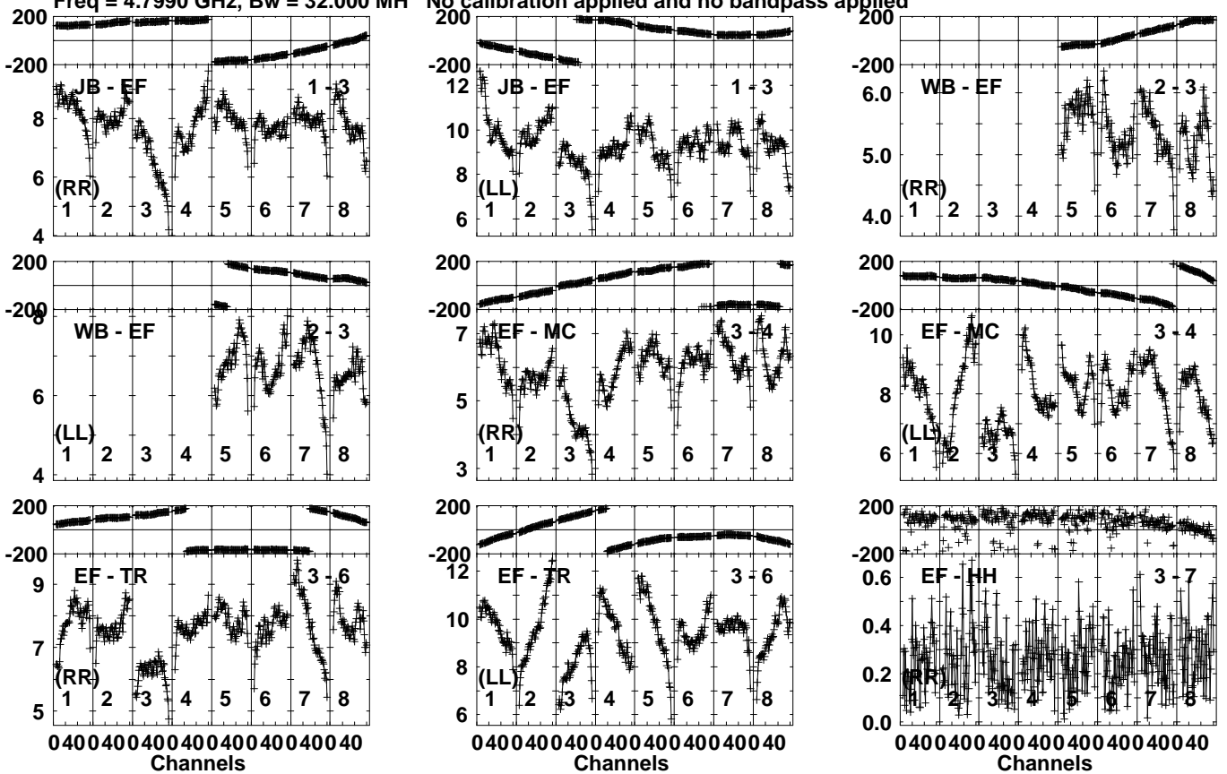
Lower frame: Milli Ampl Jy Top frame: Phas deg Vector averaged cross-power spectrum Several baselines displayed Timerange: 00/22:46:40 to 00/22:47:19
