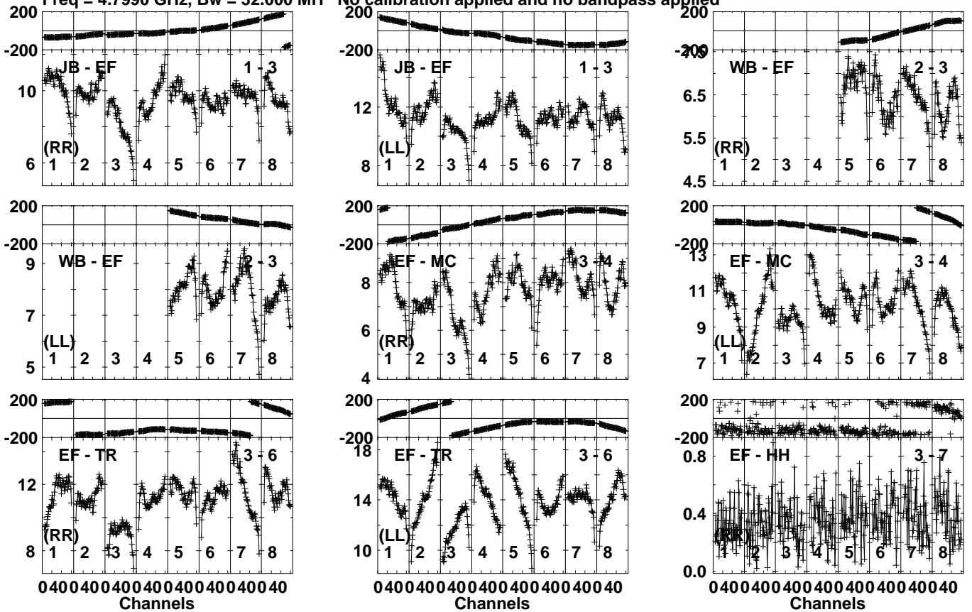
Lower frame: Milli Ampl Jy Top frame: Phas deg Vector averaged cross-power spectrum Several baselines displayed Timerange: 00/21:33:40 to 00/21:34:30
