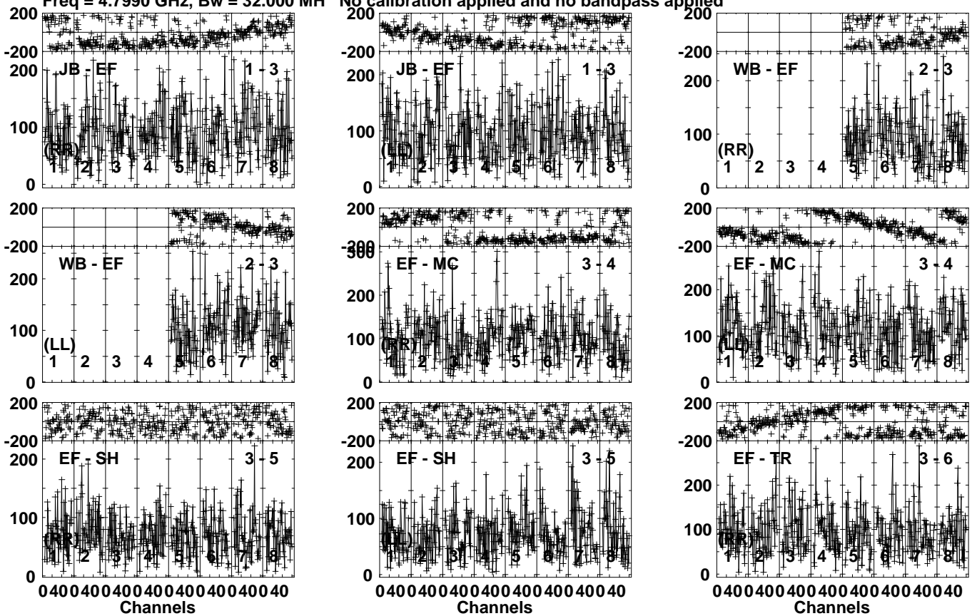
Lower frame: Micro Ampl Jy Top frame: Phas deg Vector averaged cross-power spectrum Several baselines displayed Timerange: 00/16:30:50 to 00/16:34:30
