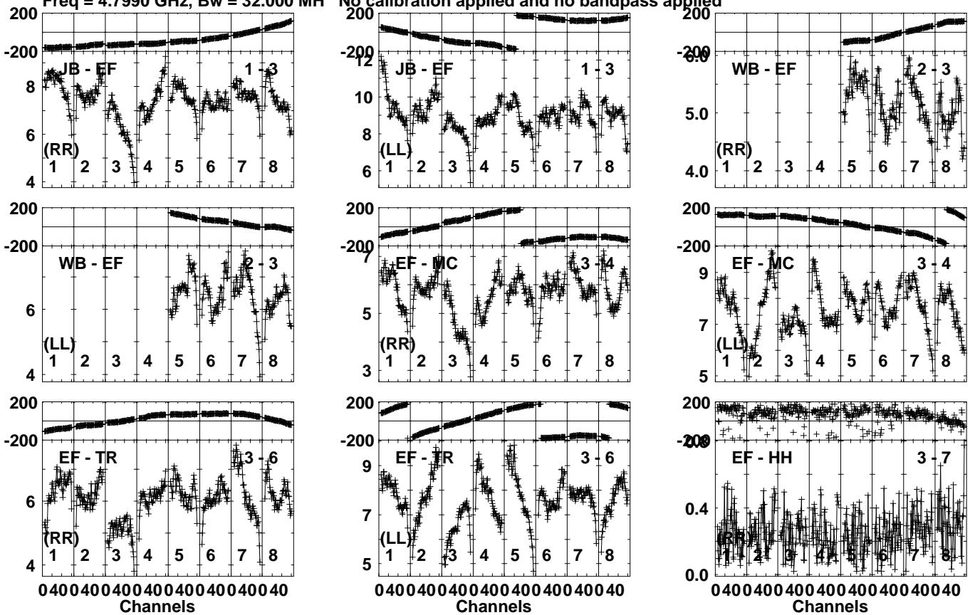
Lower frame: Milli Ampl Jy Top frame: Phas deg Vector averaged cross-power spectrum Several baselines displayed Timerange: 00/22:58:11 to 00/22:58:50
