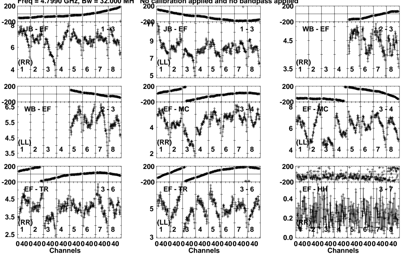
Lower frame: Milli Ampl Jy Top frame: Phas deg Vector averaged cross-power spectrum Several baselines displayed Timerange: 00/23:20:11 to 00/23:20:50
