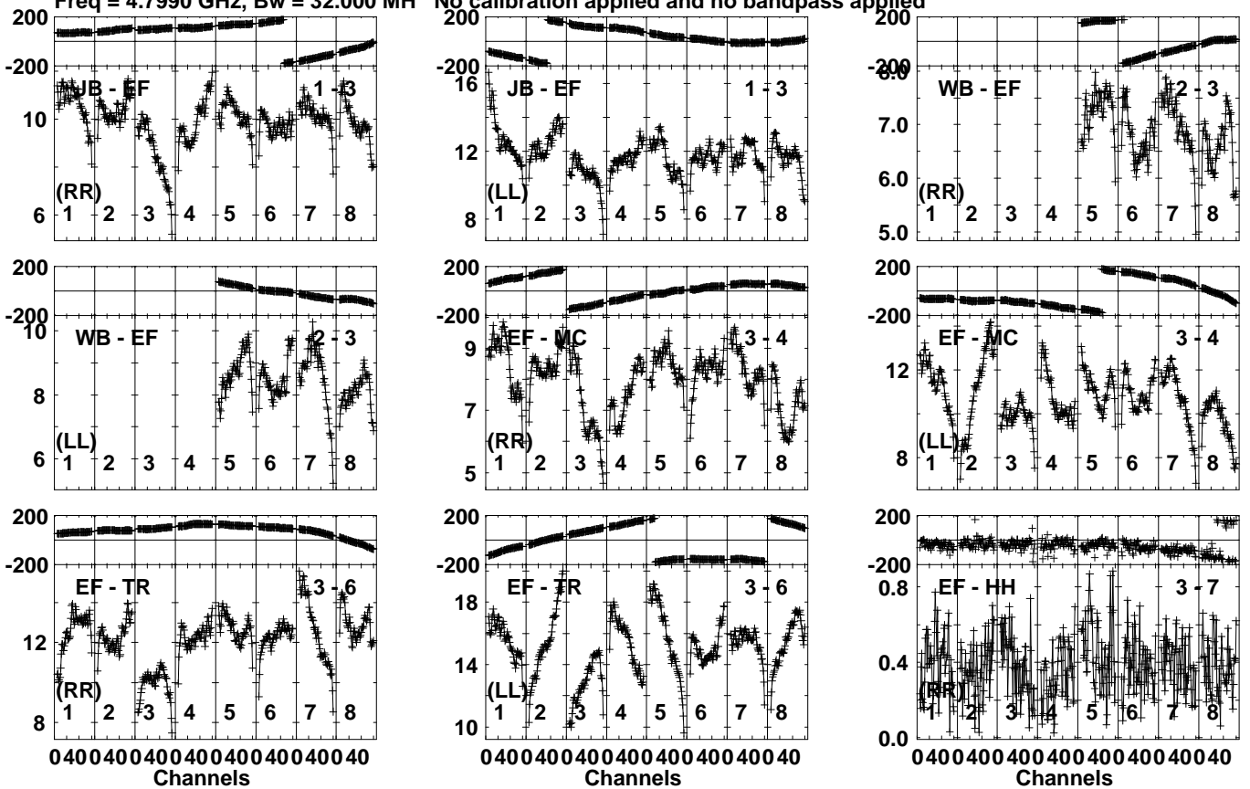
Lower frame: Milli Ampl Jy Top frame: Phas deg Vector averaged cross-power spectrum Several baselines displayed Timerange: 00/20:43:11 to 00/20:43:50
