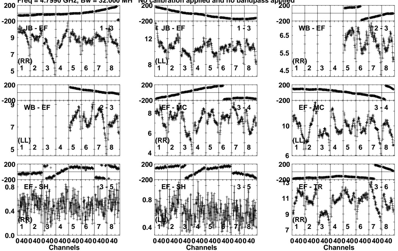
Lower frame: Milli Ampl Jy Top frame: Phas deg Vector averaged cross-power spectrum Several baselines displayed Timerange: 00/16:35:11 to 00/16:35:50
