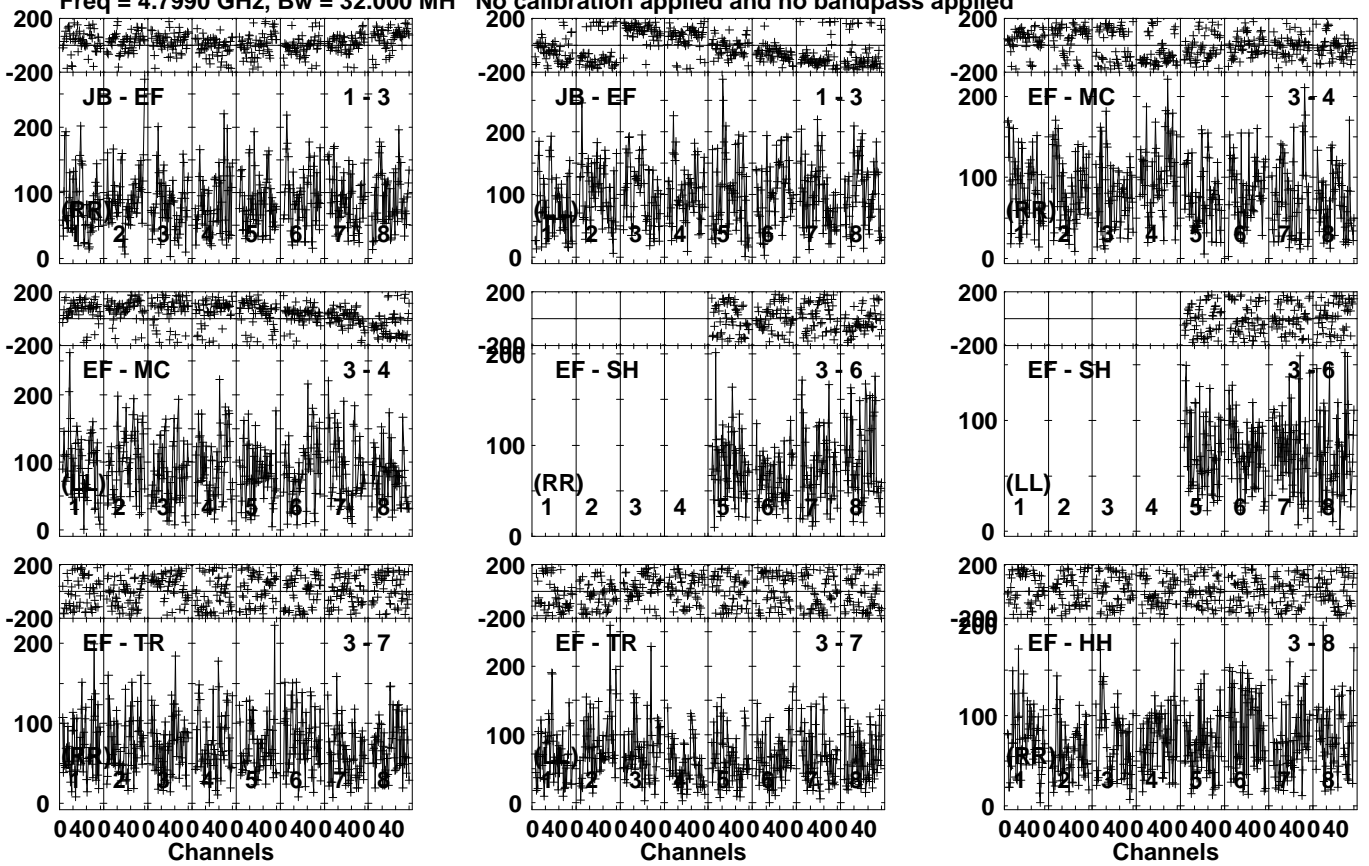
Lower frame: Micro Ampl Jy Top frame: Phas deg Vector averaged cross-power spectrum Several baselines displayed Timerange: 00/15:19:50 to 00/15:24:00
