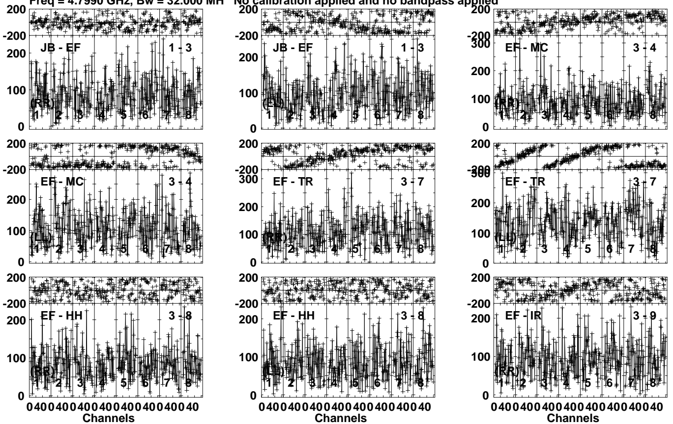
Lower frame: Micro Ampl Jy Top frame: Phas deg Vector averaged cross-power spectrum Several baselines displayed Timerange: 00/20:45:50 to 00/20:49:30
