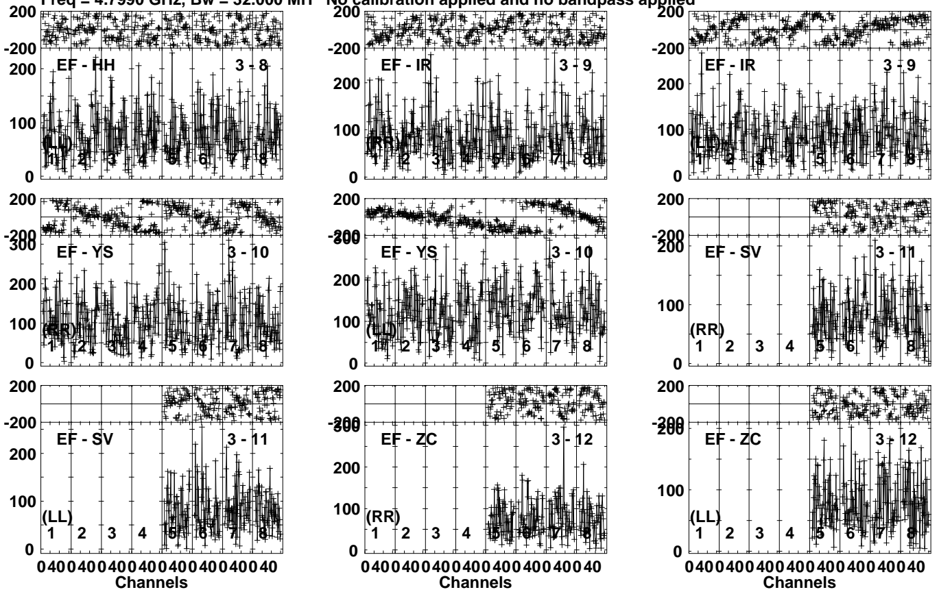
Lower frame: Micro Ampl Jy Top frame: Phas deg Vector averaged cross-power spectrum Several baselines displayed Timerange: 00/15:30:50 to 00/15:34:30
