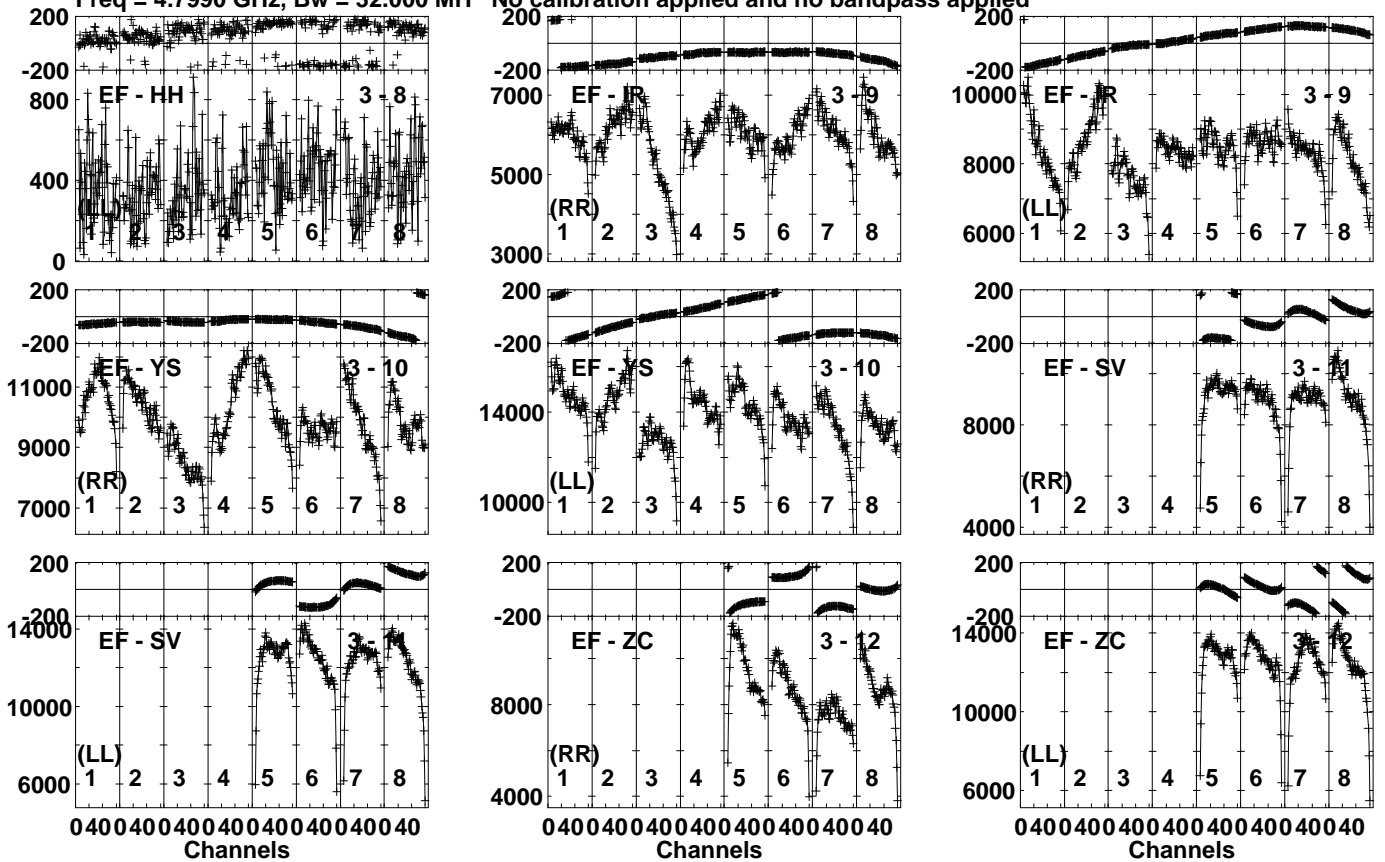
Lower frame: Micro Ampl Jy Top frame: Phas deg Vector averaged cross-power spectrum Several baselines displayed Timerange: 00/15:01:41 to 00/15:02:19
