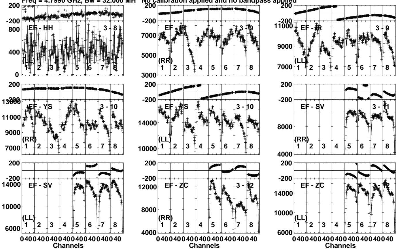
Lower frame: Micro Ampl Jy Top frame: Phas deg Vector averaged cross-power spectrum Several baselines displayed Timerange: 00/15:13:11 to 00/15:13:49
