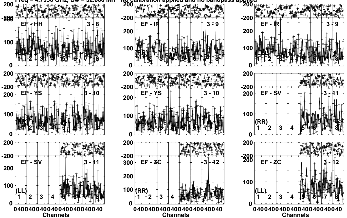
Lower frame: Micro Ampl Jy Top frame: Phas deg Vector averaged cross-power spectrum Several baselines displayed Timerange: 00/14:39:40 to 00/14:43:50
