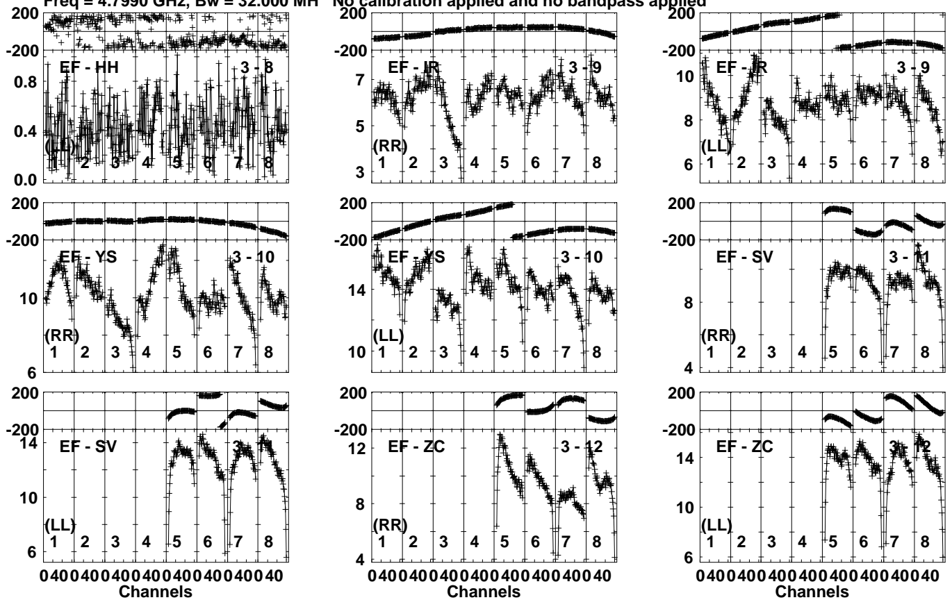
Lower frame: Milli Ampl Jy Top frame: Phas deg Vector averaged cross-power spectrum Several baselines displayed Timerange: 00/15:07:10 to 00/15:08:00
