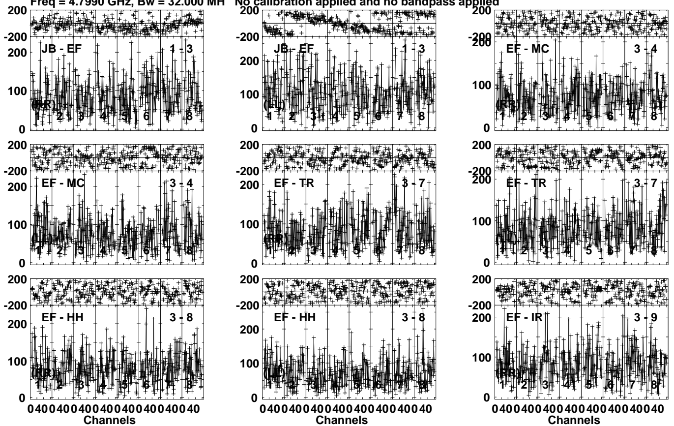
Lower frame: Micro Ampl Jy Top frame: Phas deg Vector averaged cross-power spectrum Several baselines displayed Timerange: 00/16:10:40 to 00/16:14:20
