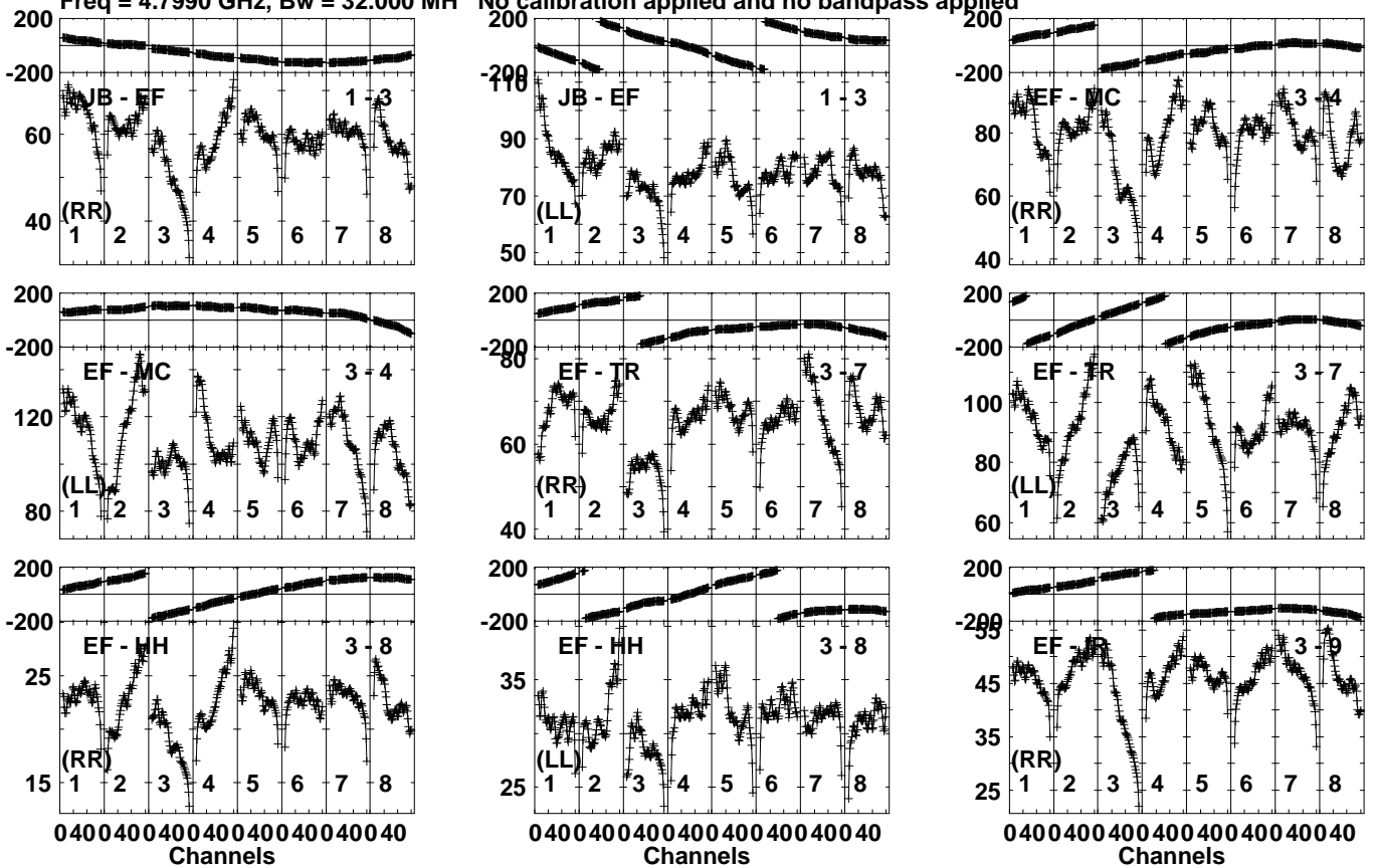
Lower frame: Milli Ampl Jy Top frame: Phas deg Vector averaged cross-power spectrum Several baselines displayed Timerange: 00/22:25:30 to 00/22:28:10
