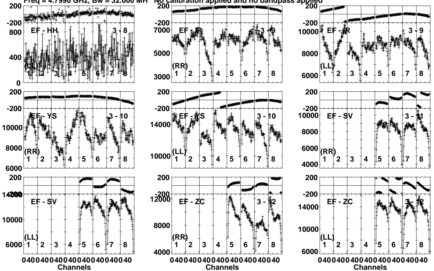
Lower frame: Micro Ampl Jy Top frame: Phas deg Vector averaged cross-power spectrum Several baselines displayed Timerange: 00/14:50:10 to 00/14:50:50
