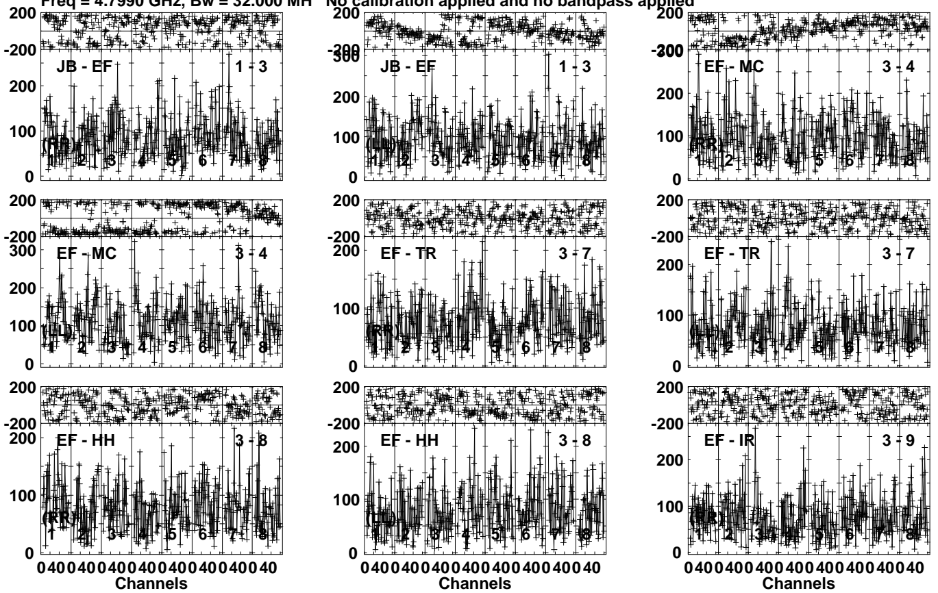
Lower frame: Micro Ampl Jy Top frame: Phas deg Vector averaged cross-power spectrum Several baselines displayed Timerange: 00/16:55:40 to 00/16:59:20
