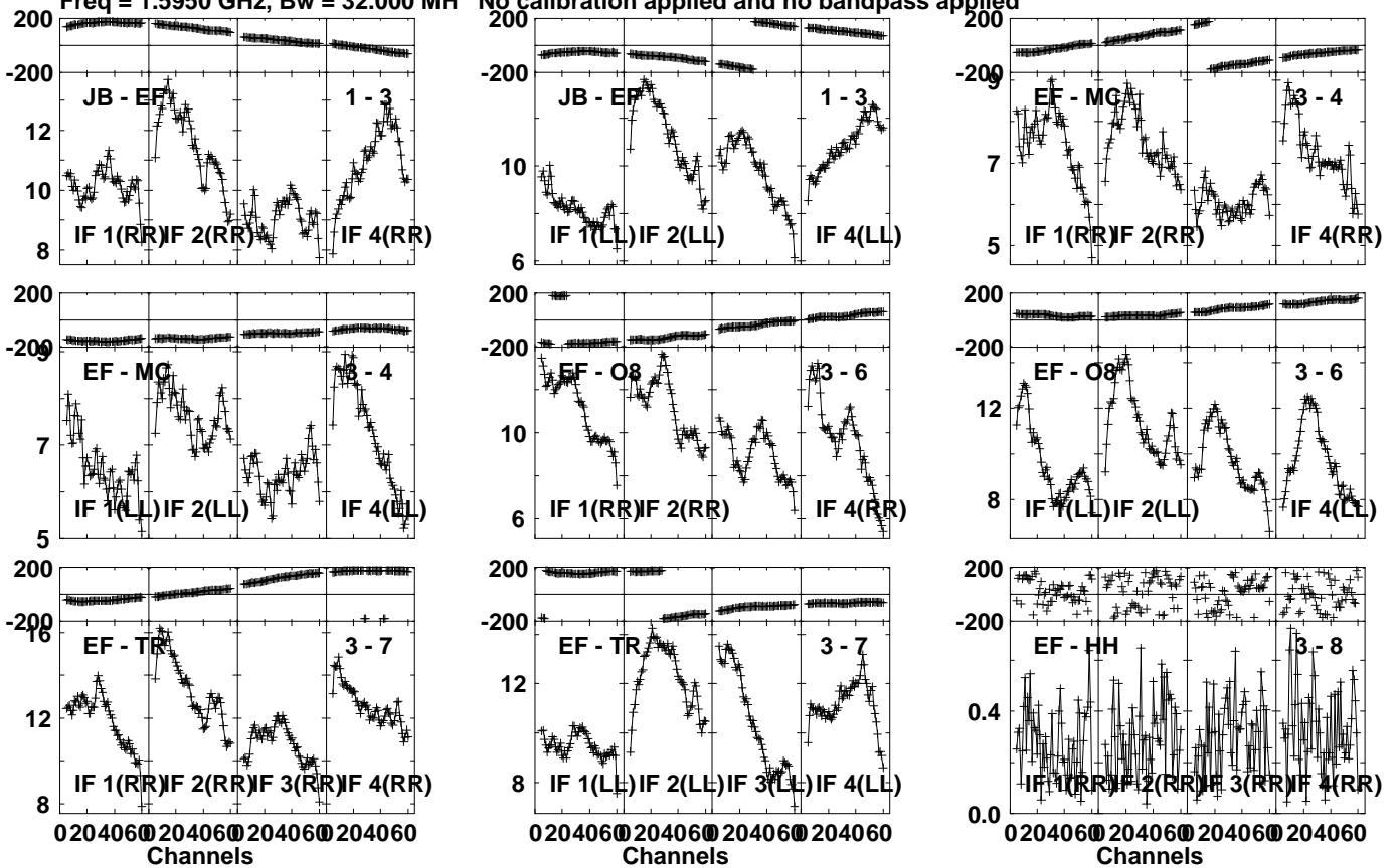
Lower frame: Milli Ampl Jy Top frame: Phas deg Vector averaged cross-power spectrum Several baselines displayed Timerange: 00/17:14:40 to 00/17:15:29
