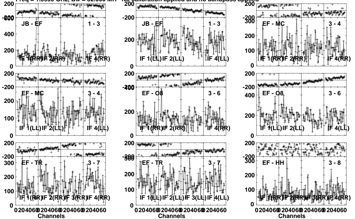
Lower frame: Micro Ampl Jy Top frame: Phas deg Vector averaged cross-power spectrum Several baselines displayed Timerange: 00/13:30:50 to 00/13:34:30
