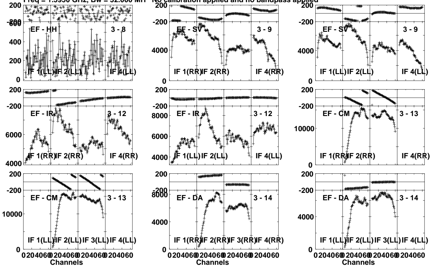
Lower frame: Micro Ampl Jy Top frame: Phas deg Vector averaged cross-power spectrum Several baselines displayed Timerange: 00/14:43:11 to 00/14:43:50
