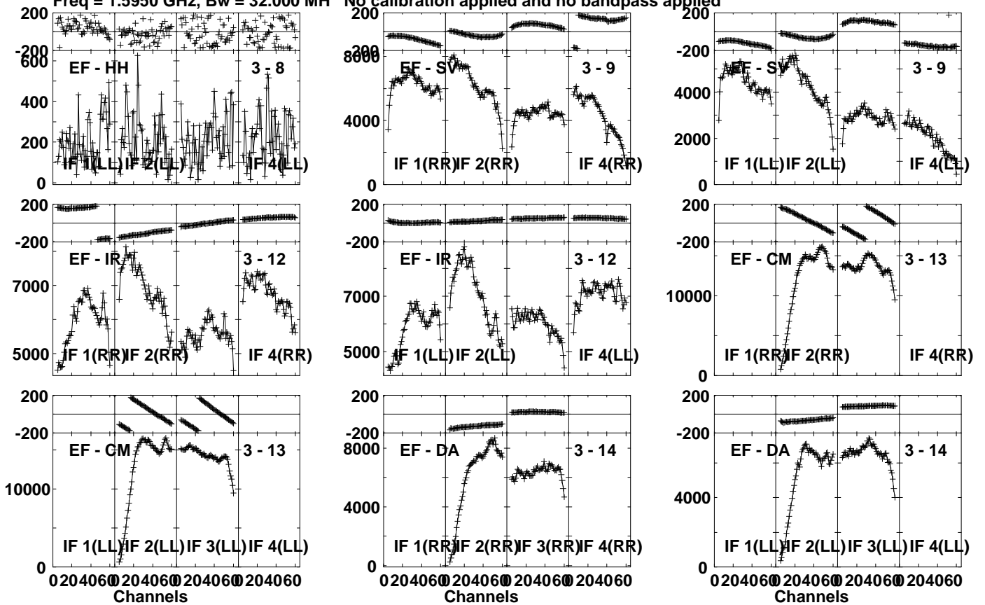
Lower frame: Micro Ampl Jy Top frame: Phas deg Vector averaged cross-power spectrum Several baselines displayed Timerange: 00/15:50:11 to 00/15:50:49
