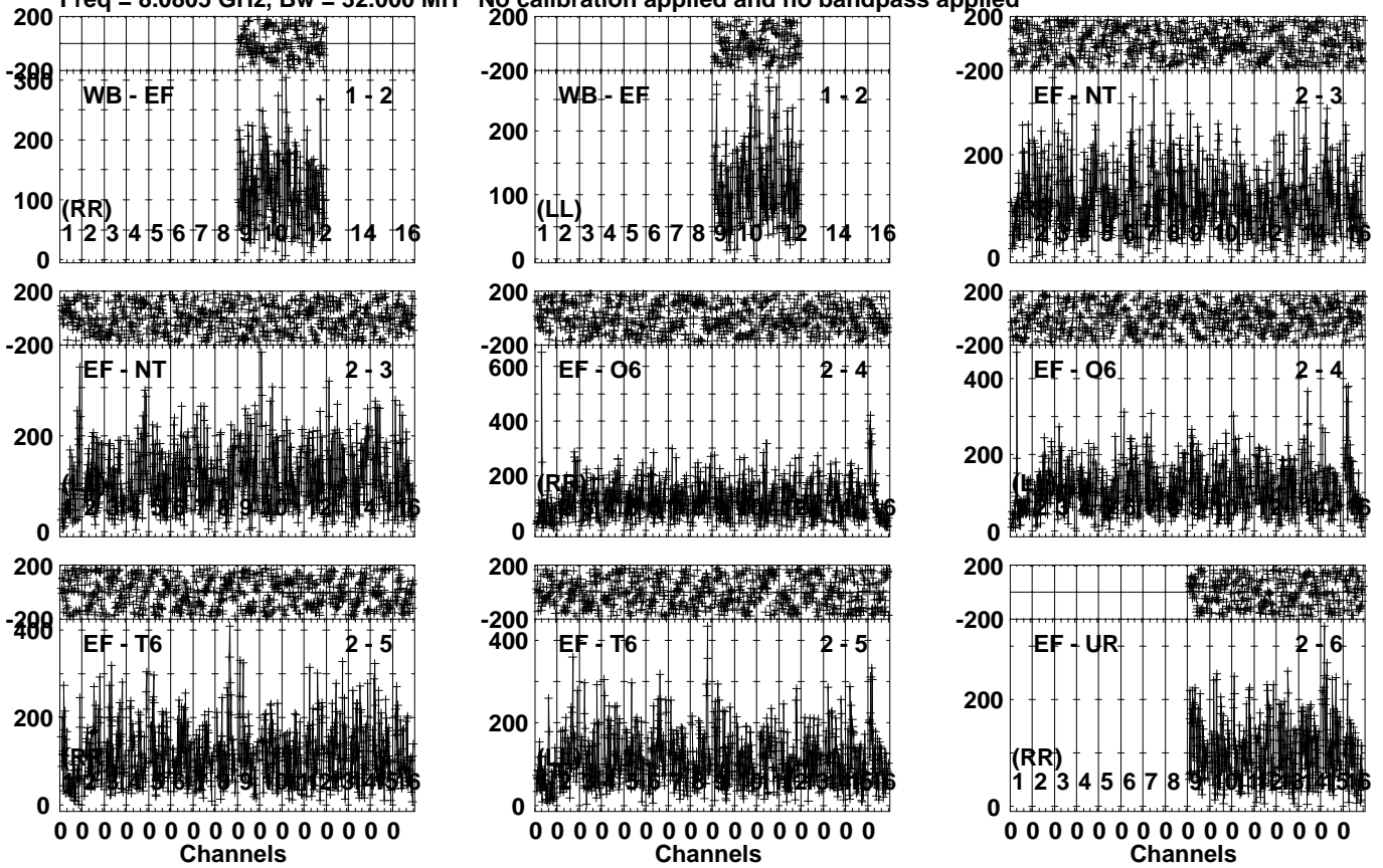
Lower frame: Micro Ampl Jy Top frame: Phas deg Vector averaged cross-power spectrum Several baselines displayed Timerange: 00/11:10:25 to 00/11:12:34
