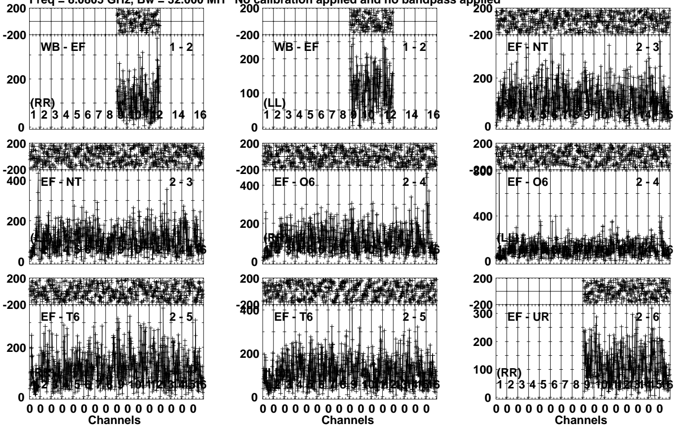
Lower frame: Micro Ampl Jy Top frame: Phas deg Vector averaged cross-power spectrum Several baselines displayed Timerange: 00/11:26:21 to 00/11:28:30
