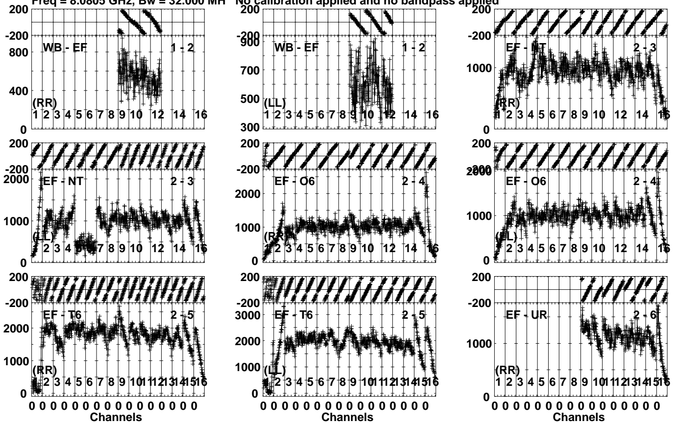
Lower frame: Micro Ampl Jy Top frame: Phas deg Vector averaged cross-power spectrum Several baselines displayed Timerange: 00/11:55:02 to 00/11:56:19
