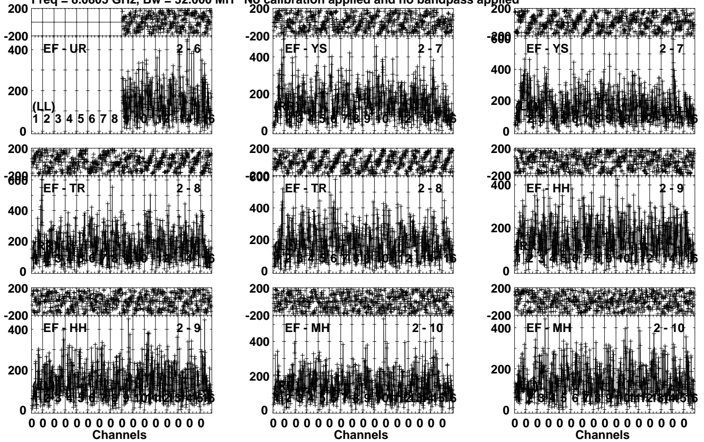
Lower frame: Micro Ampl Jy Top frame: Phas deg Vector averaged cross-power spectrum Several baselines displayed Timerange: 00/12:49:25 to 00/12:50:55
