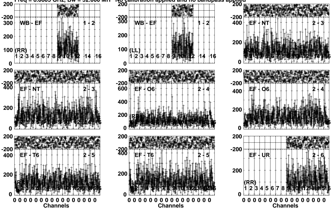
Lower frame: Micro Ampl Jy Top frame: Phas deg Vector averaged cross-power spectrum Several baselines displayed Timerange: 00/12:28:17 to 00/12:30:25
