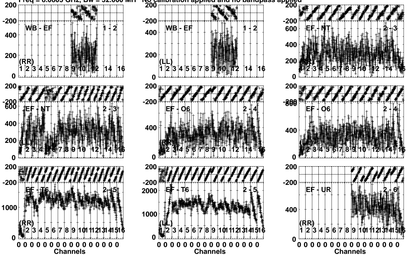
Lower frame: Micro Ampl Jy Top frame: Phas deg Vector averaged cross-power spectrum Several baselines displayed Timerange: 00/10:03:52 to 00/10:05:34
