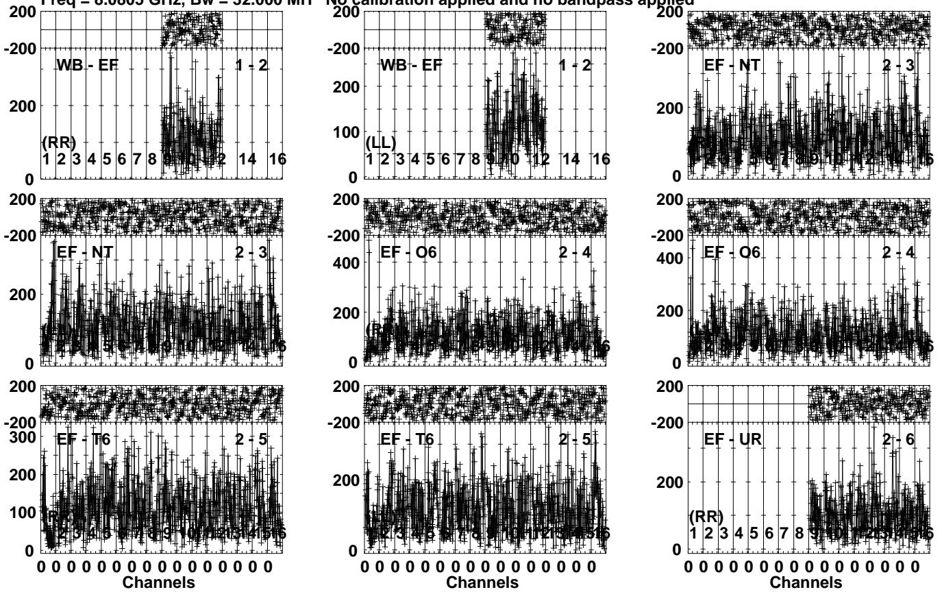
Lower frame: Micro Ampl Jy Top frame: Phas deg Vector averaged cross-power spectrum Several baselines displayed Timerange: 00/09:51:32 to 00/09:53:40
