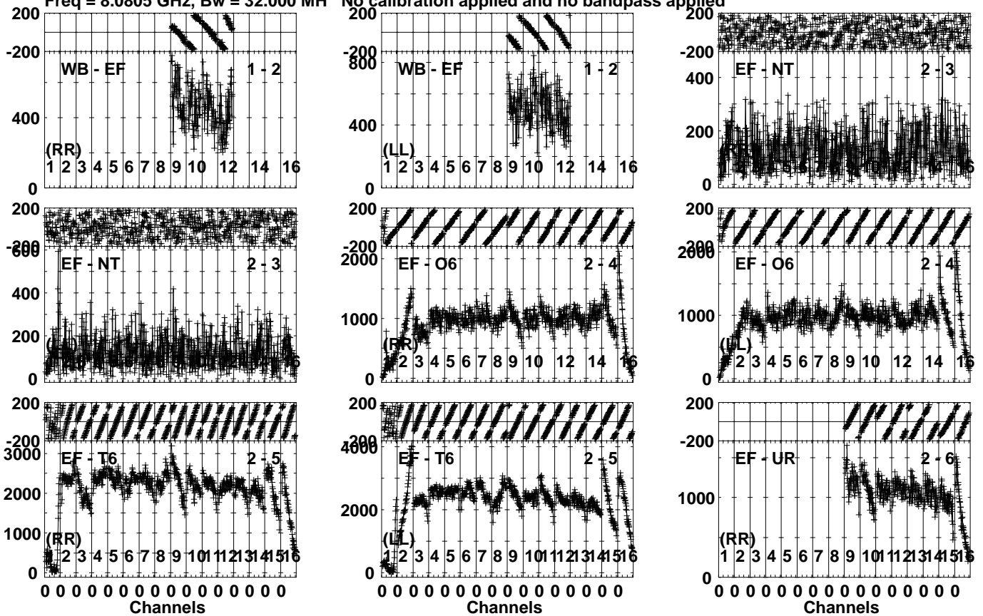
Lower frame: Micro Ampl Jy Top frame: Phas deg Vector averaged cross-power spectrum Several baselines displayed Timerange: 00/11:13:07 to 00/11:14:25
