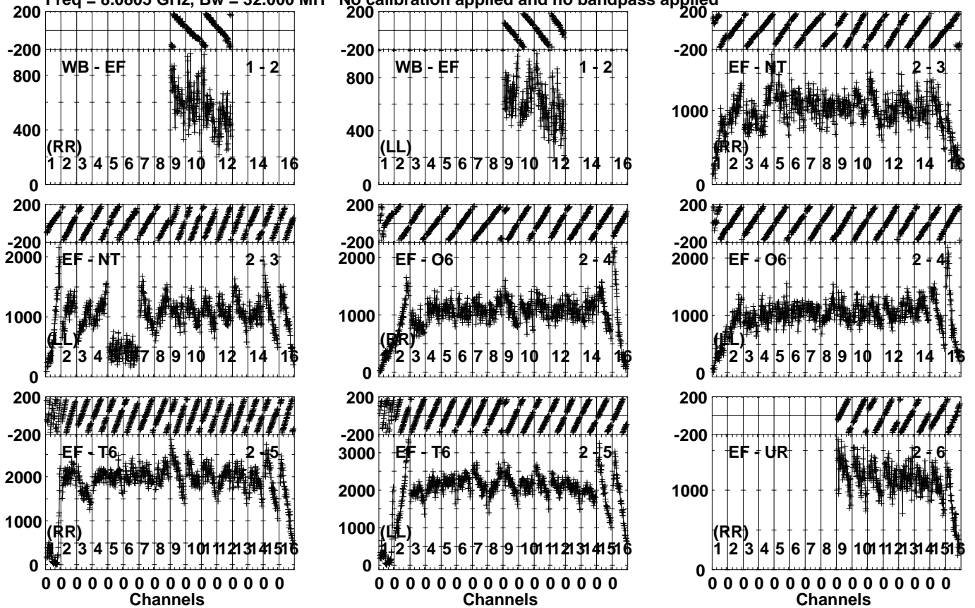
Lower frame: Micro Ampl Jy Top frame: Phas deg Vector averaged cross-power spectrum Several baselines displayed Timerange: 00/12:38:56 to 00/12:40:14
