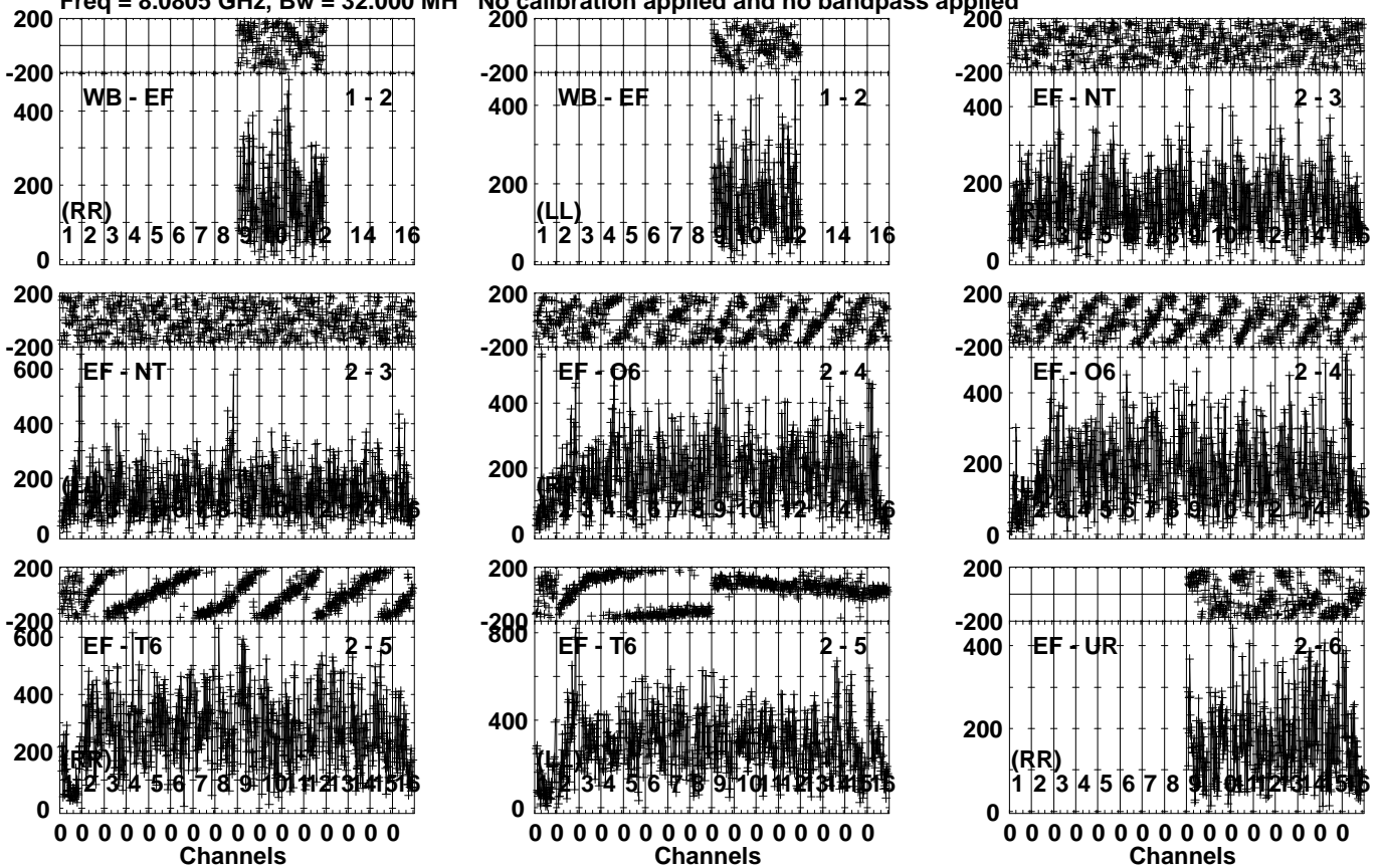
Lower frame: Micro Ampl Jy Top frame: Phas deg Vector averaged cross-power spectrum Several baselines displayed Timerange: 00/10:34:56 to 00/10:36:25
