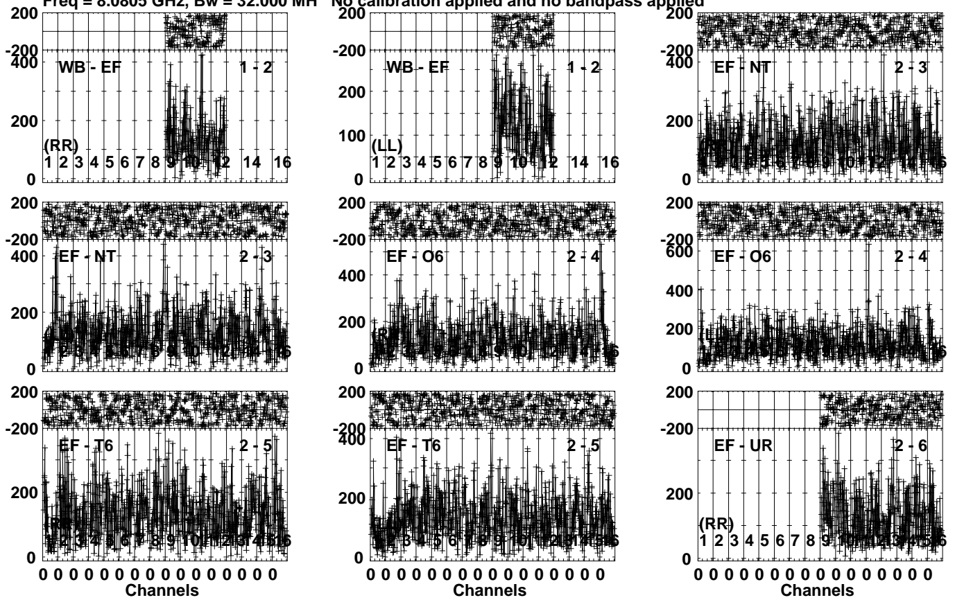
Lower frame: Micro Ampl Jy Top frame: Phas deg Vector averaged cross-power spectrum Several baselines displayed Timerange: 00/12:40:16 to 00/12:42:24
