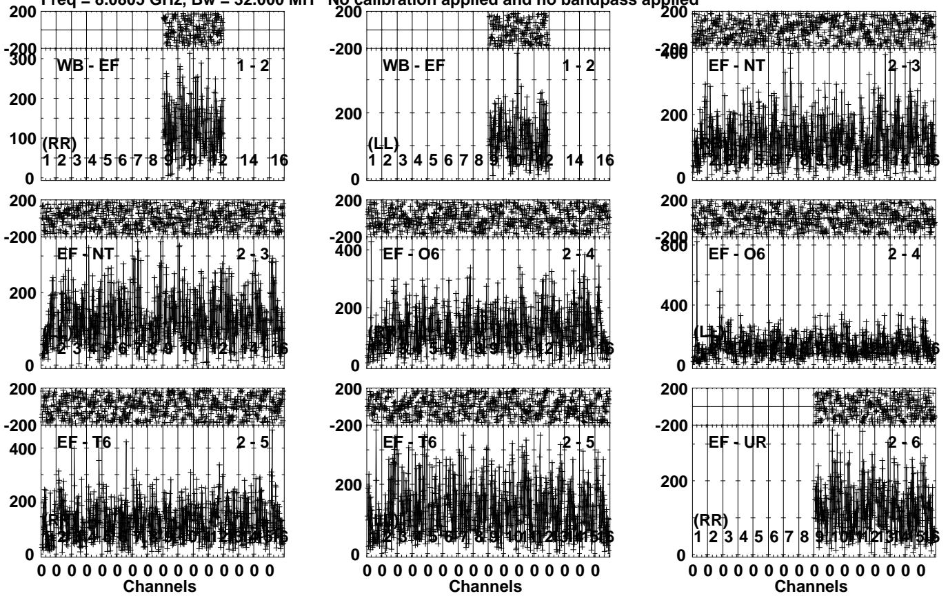
Lower frame: Micro Ampl Jy Top frame: Phas deg Vector averaged cross-power spectrum Several baselines displayed Timerange: 00/12:08:20 to 00/12:10:30
