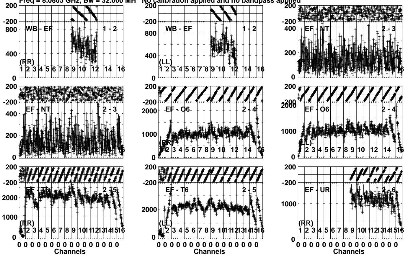
Lower frame: Micro Ampl Jy Top frame: Phas deg Vector averaged cross-power spectrum Several baselines displayed Timerange: 00/11:29:01 to 00/11:30:20
