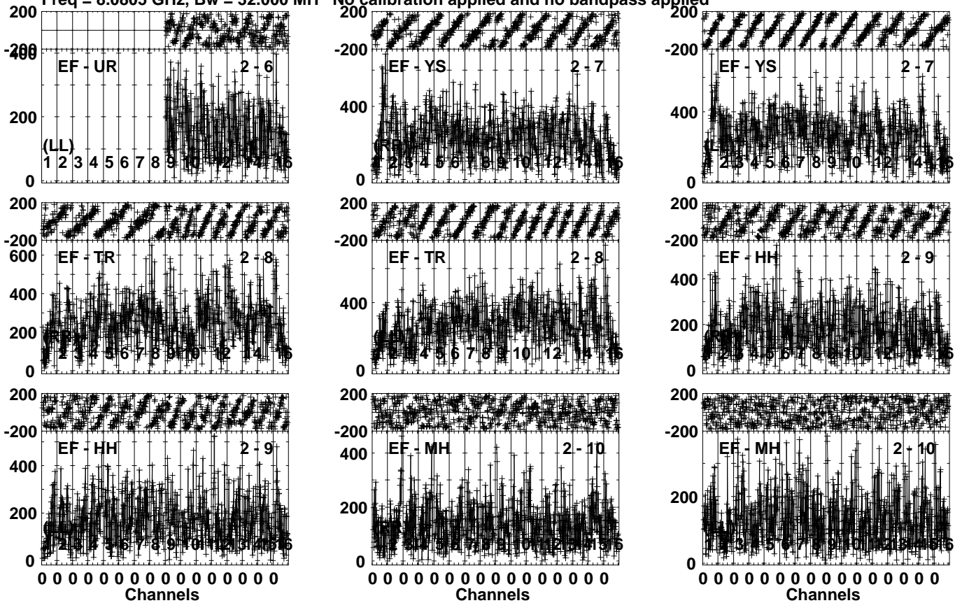
Lower frame: Micro Ampl Jy Top frame: Phas deg Vector averaged cross-power spectrum Several baselines displayed Timerange: 00/10:31:36 to 00/10:33:05
