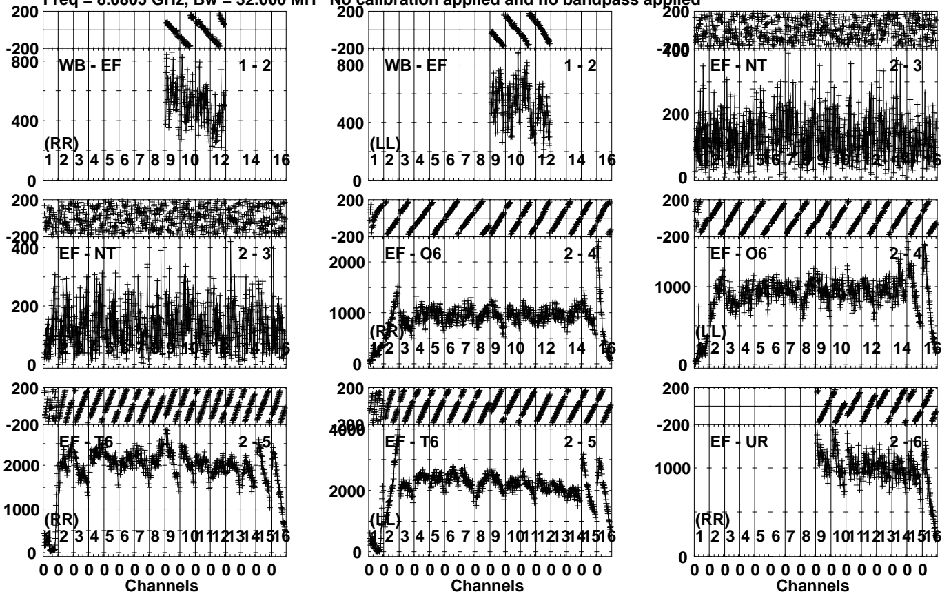
Lower frame: Micro Ampl Jy Top frame: Phas deg Vector averaged cross-power spectrum Several baselines displayed Timerange: 00/10:18:06 to 00/10:19:24
