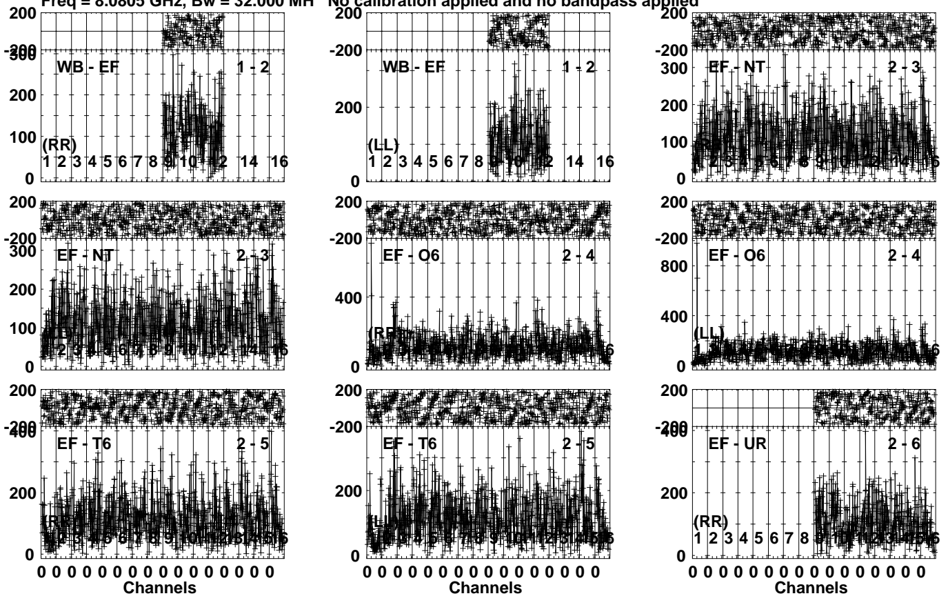
Lower frame: Micro Ampl Jy Top frame: Phas deg Vector averaged cross-power spectrum Several baselines displayed Timerange: 00/10:27:27 to 00/10:29:35
