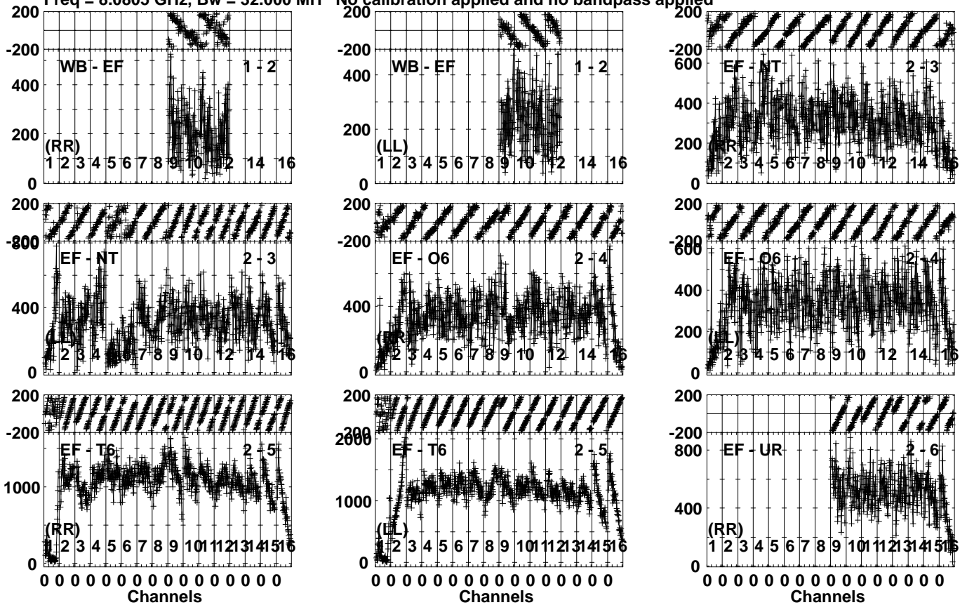
Lower frame: Micro Ampl Jy Top frame: Phas deg Vector averaged cross-power spectrum Several baselines displayed Timerange: 00/12:16:41 to 00/12:18:24
