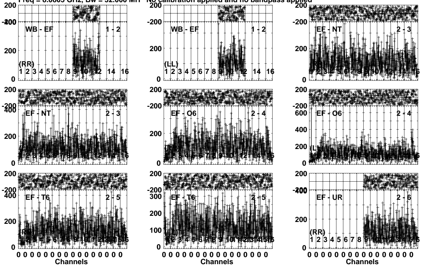
Lower frame: Micro Ampl Jy Top frame: Phas deg Vector averaged cross-power spectrum Several baselines displayed Timerange: 00/09:47:32 to 00/09:49:39
