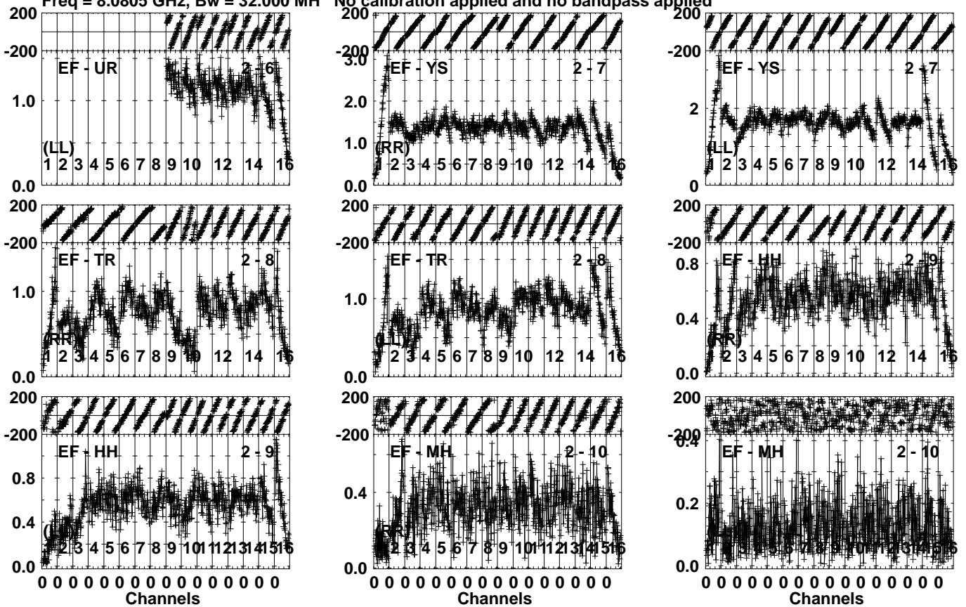
Lower frame: Milli Ampl Jy Top frame: Phas deg Vector averaged cross-power spectrum Several baselines displayed Timerange: 00/11:13:07 to 00/11:14:25
