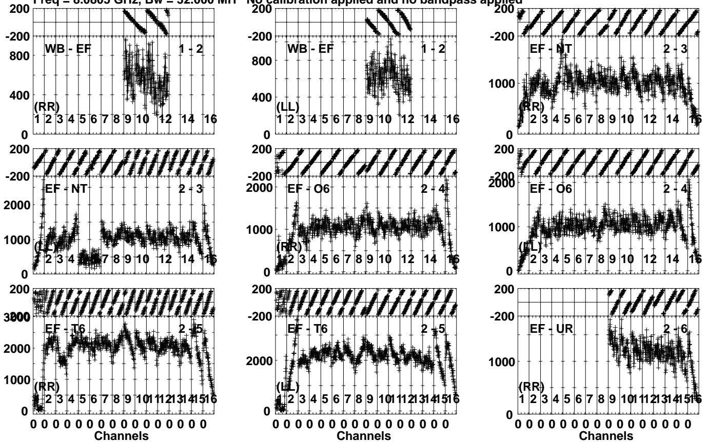
Lower frame: Micro Ampl Jy Top frame: Phas deg Vector averaged cross-power spectrum Several baselines displayed Timerange: 00/12:30:57 to 00/12:32:15
