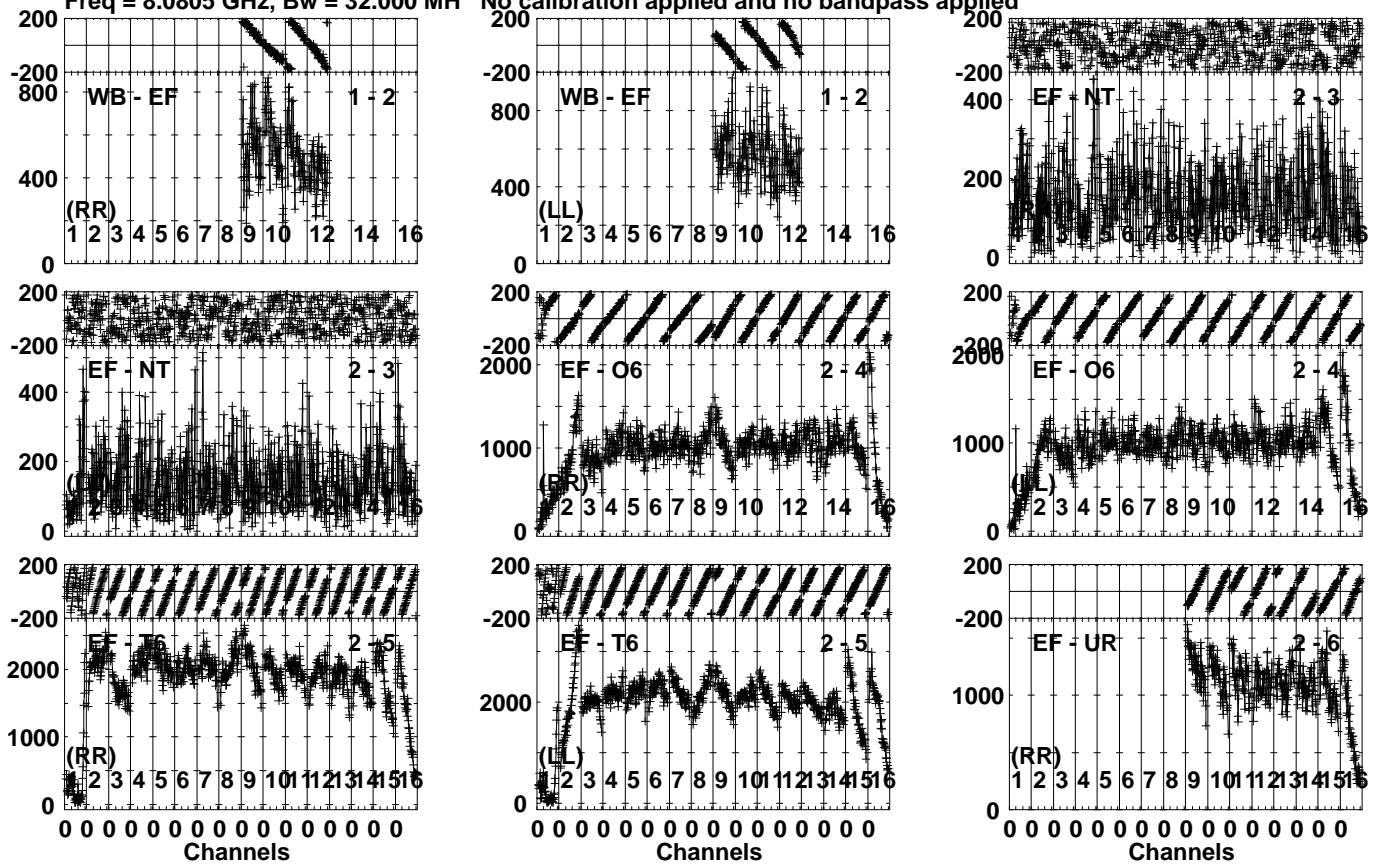
Lower frame: Micro Ampl Jy Top frame: Phas deg Vector averaged cross-power spectrum Several baselines displayed Timerange: 00/11:33:02 to 00/11:34:20
