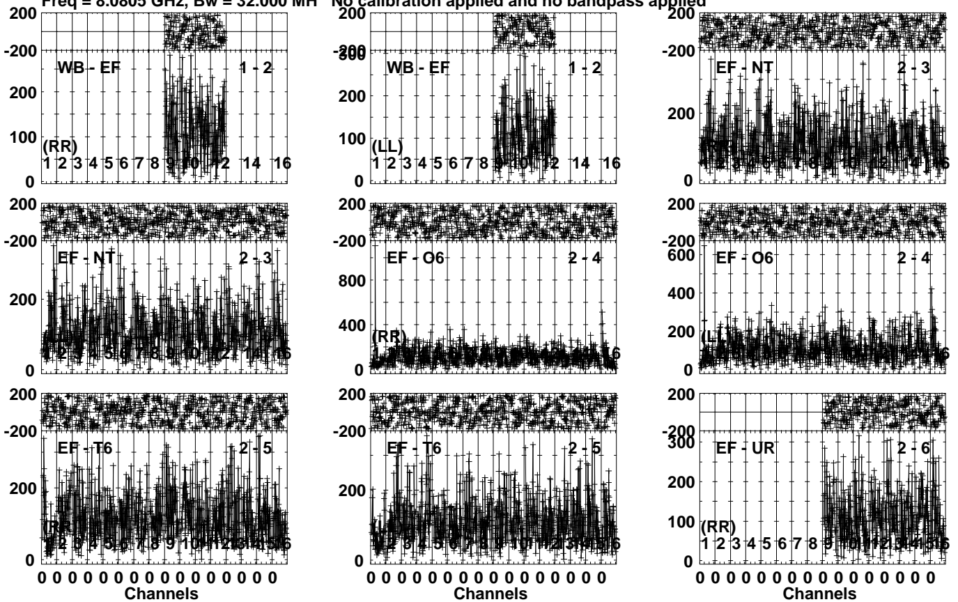
Lower frame: Micro Ampl Jy Top frame: Phas deg Vector averaged cross-power spectrum Several baselines displayed Timerange: 00/11:22:21 to 00/11:24:30
