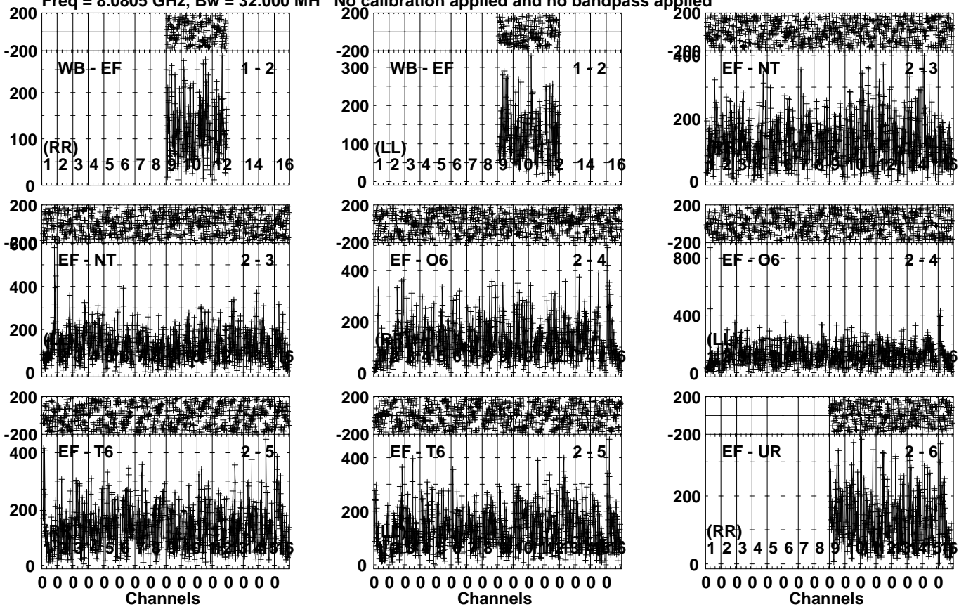
Lower frame: Micro Ampl Jy Top frame: Phas deg Vector averaged cross-power spectrum Several baselines displayed Timerange: 00/12:00:21 to 00/12:02:29
