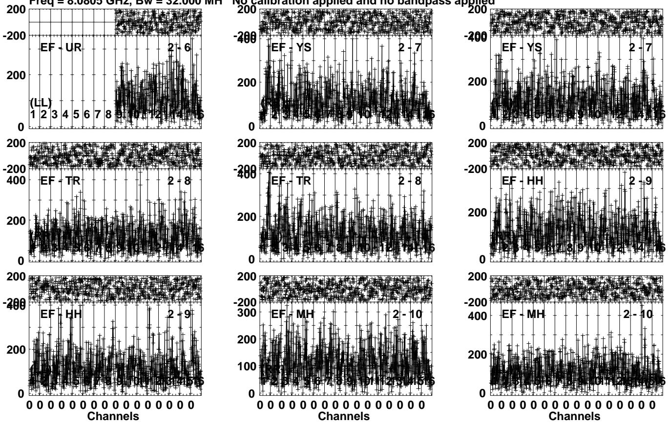
Lower frame: Micro Ampl Jy Top frame: Phas deg Vector averaged cross-power spectrum Several baselines displayed Timerange: 00/10:54:26 to 00/10:56:35
