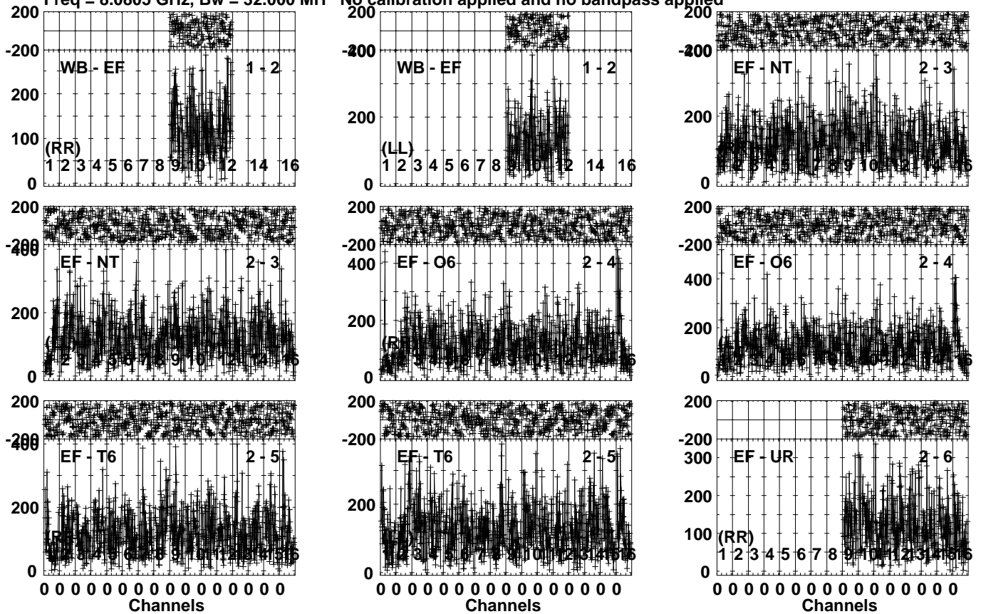
Lower frame: Micro Ampl Jy Top frame: Phas deg Vector averaged cross-power spectrum Several baselines displayed Timerange: 00/12:04:21 to 00/12:06:30
