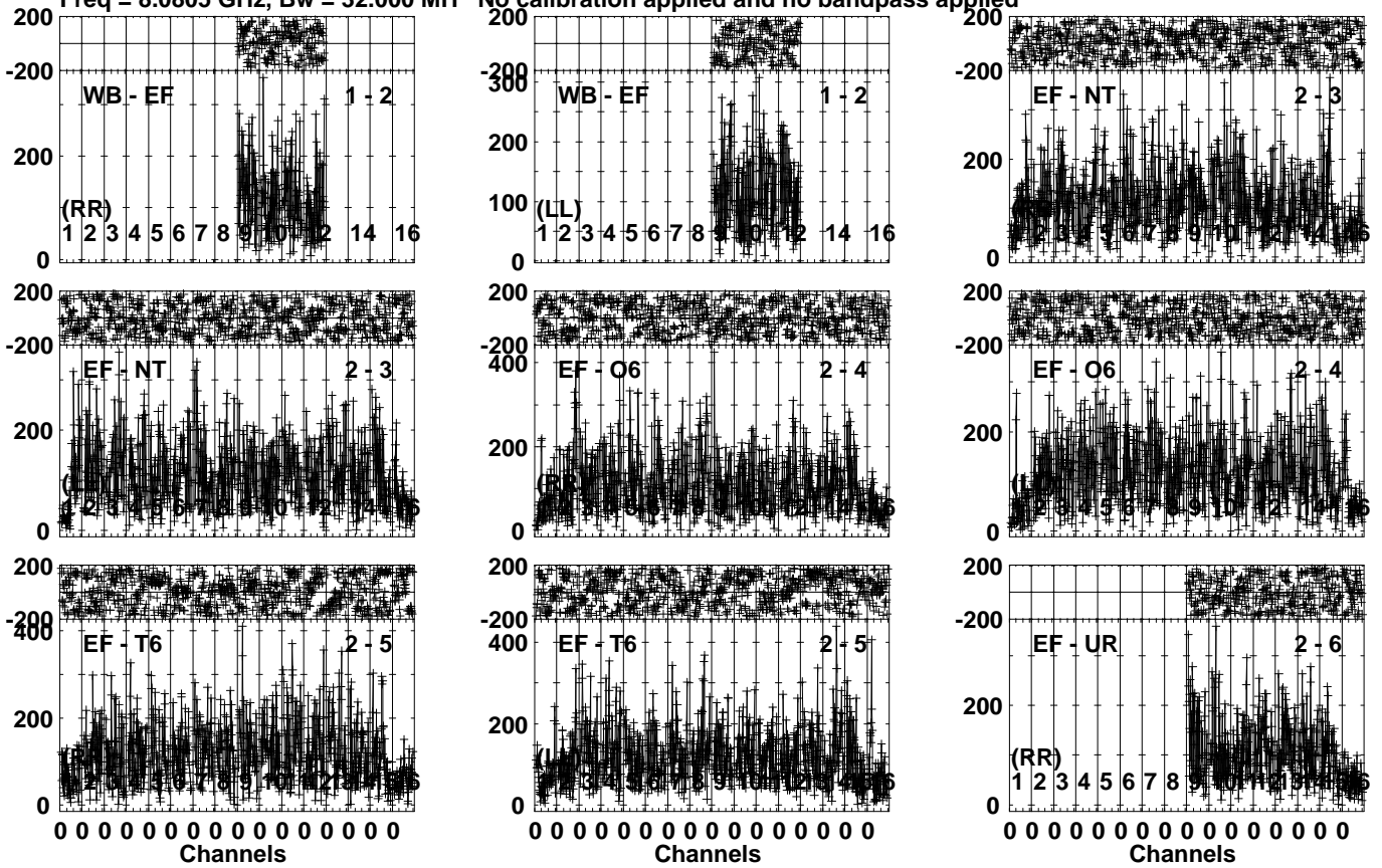
Lower frame: Micro Ampl Jy Top frame: Phas deg Vector averaged cross-power spectrum Several baselines displayed Timerange: 00/09:39:31 to 00/09:41:39
