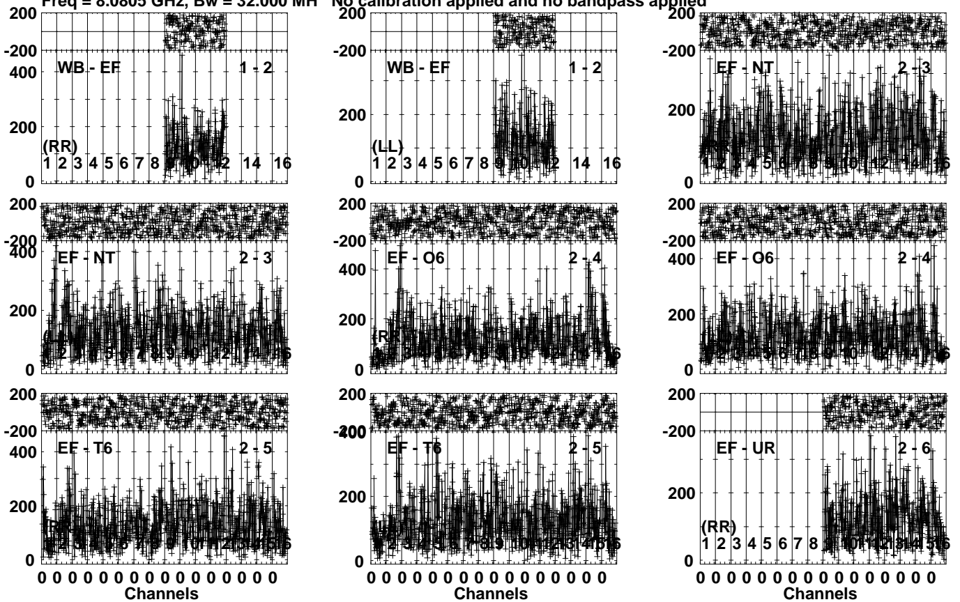
Lower frame: Micro Ampl Jy Top frame: Phas deg Vector averaged cross-power spectrum Several baselines displayed Timerange: 00/12:32:16 to 00/12:34:24
