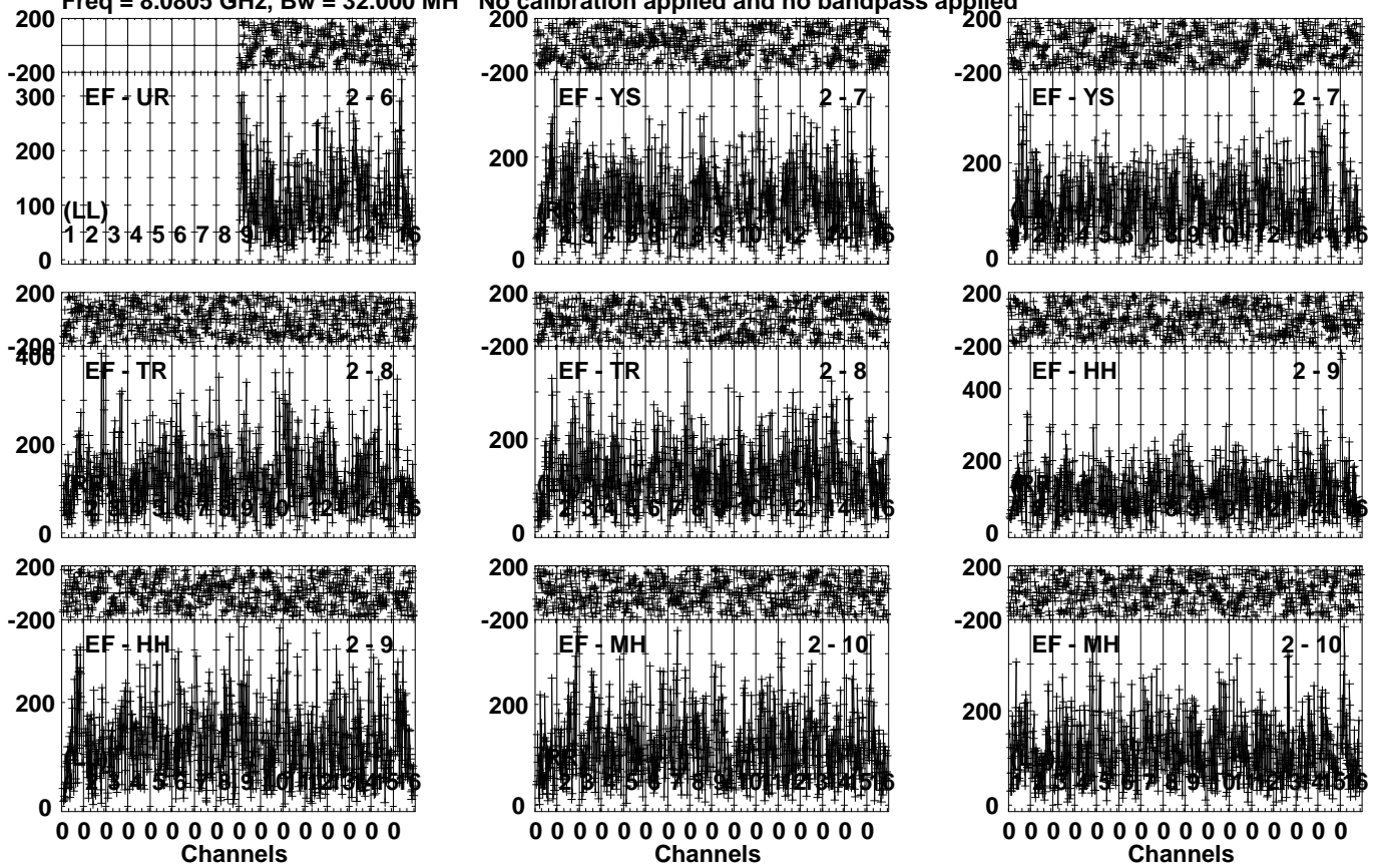
Lower frame: Micro Ampl Jy Top frame: Phas deg Vector averaged cross-power spectrum Several baselines displayed Timerange: 00/11:38:22 to 00/11:40:29
