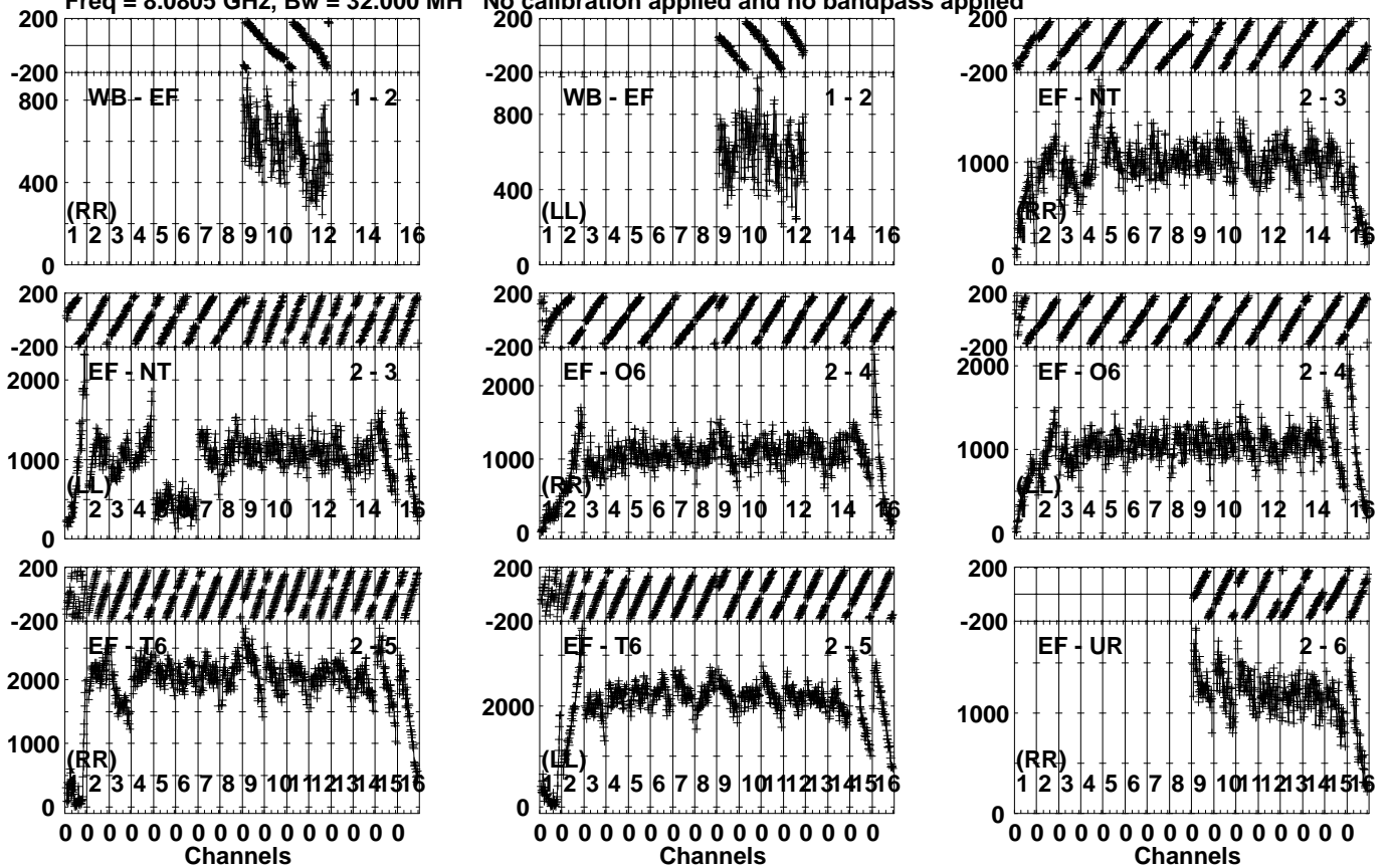
Lower frame: Micro Ampl Jy Top frame: Phas deg Vector averaged cross-power spectrum Several baselines displayed Timerange: 00/12:42:56 to 00/12:44:15
