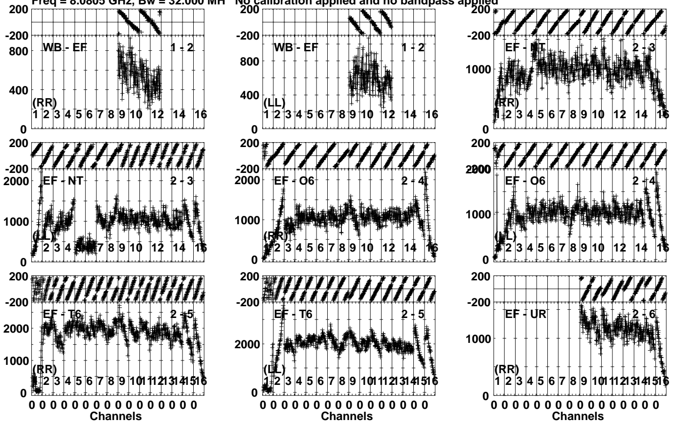
Lower frame: Micro Ampl Jy Top frame: Phas deg Vector averaged cross-power spectrum Several baselines displayed Timerange: 00/11:59:02 to 00/12:00:20
