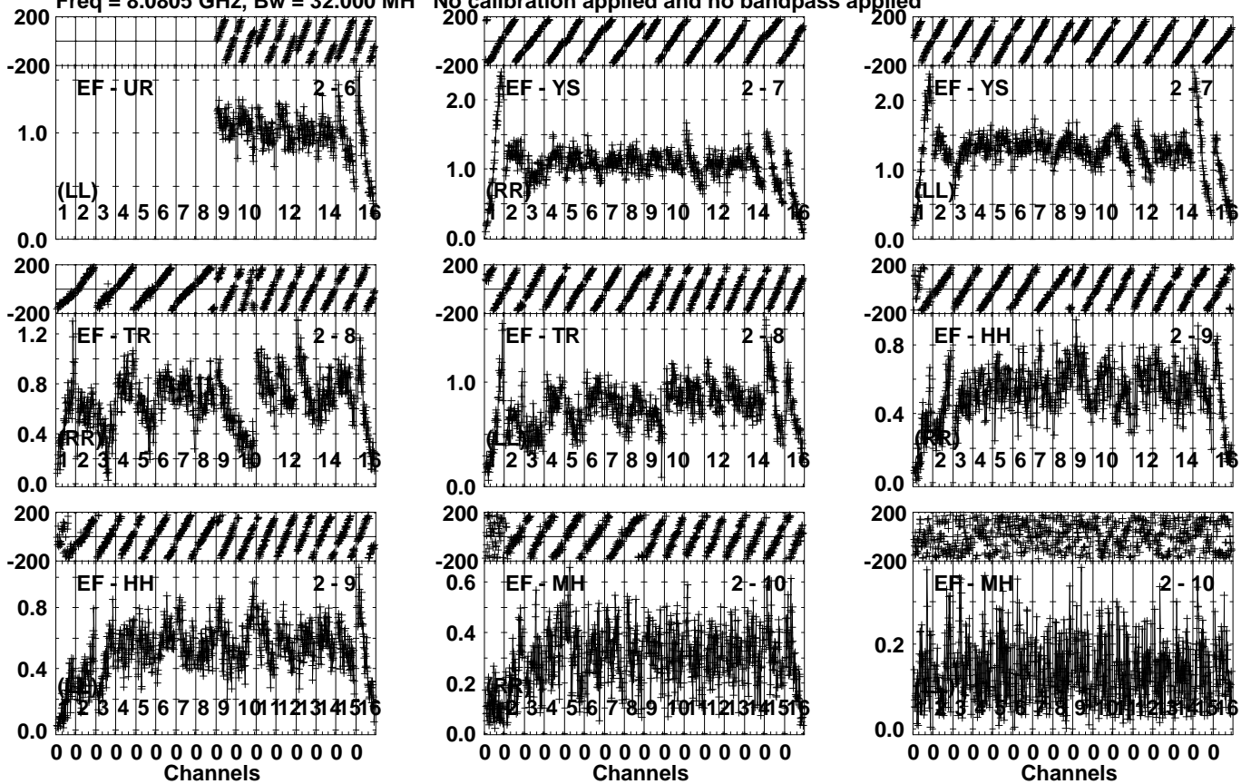
Lower frame: Milli Ampl Jy Top frame: Phas deg Vector averaged cross-power spectrum Several baselines displayed Timerange: 00/10:10:07 to 00/10:11:24
