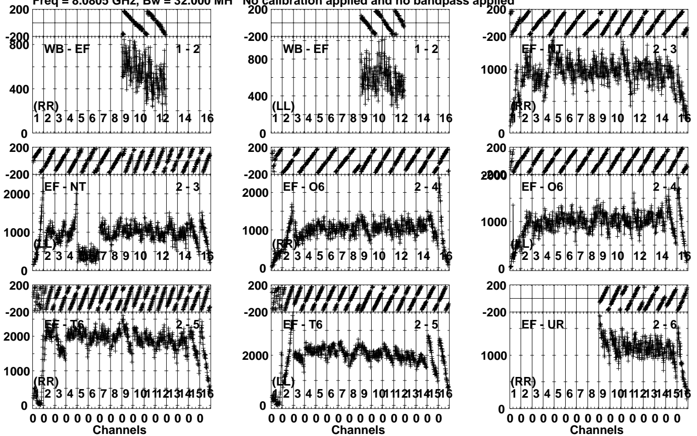
Lower frame: Micro Ampl Jy Top frame: Phas deg Vector averaged cross-power spectrum Several baselines displayed Timerange: 00/11:37:02 to 00/11:38:20
