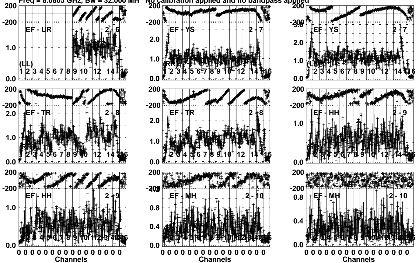
Lower frame: Milli Ampl Jy Top frame: Phas deg Vector averaged cross-power spectrum Several baselines displayed Timerange: 00/09:34:21 to 00/09:35:34
