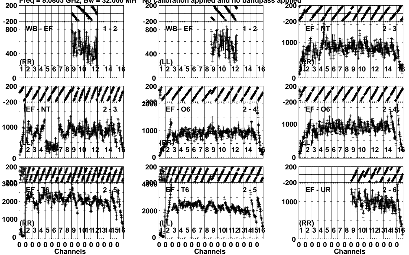
Lower frame: Micro Ampl Jy Top frame: Phas deg Vector averaged cross-power spectrum Several baselines displayed Timerange: 00/09:46:12 to 00/09:47:29
