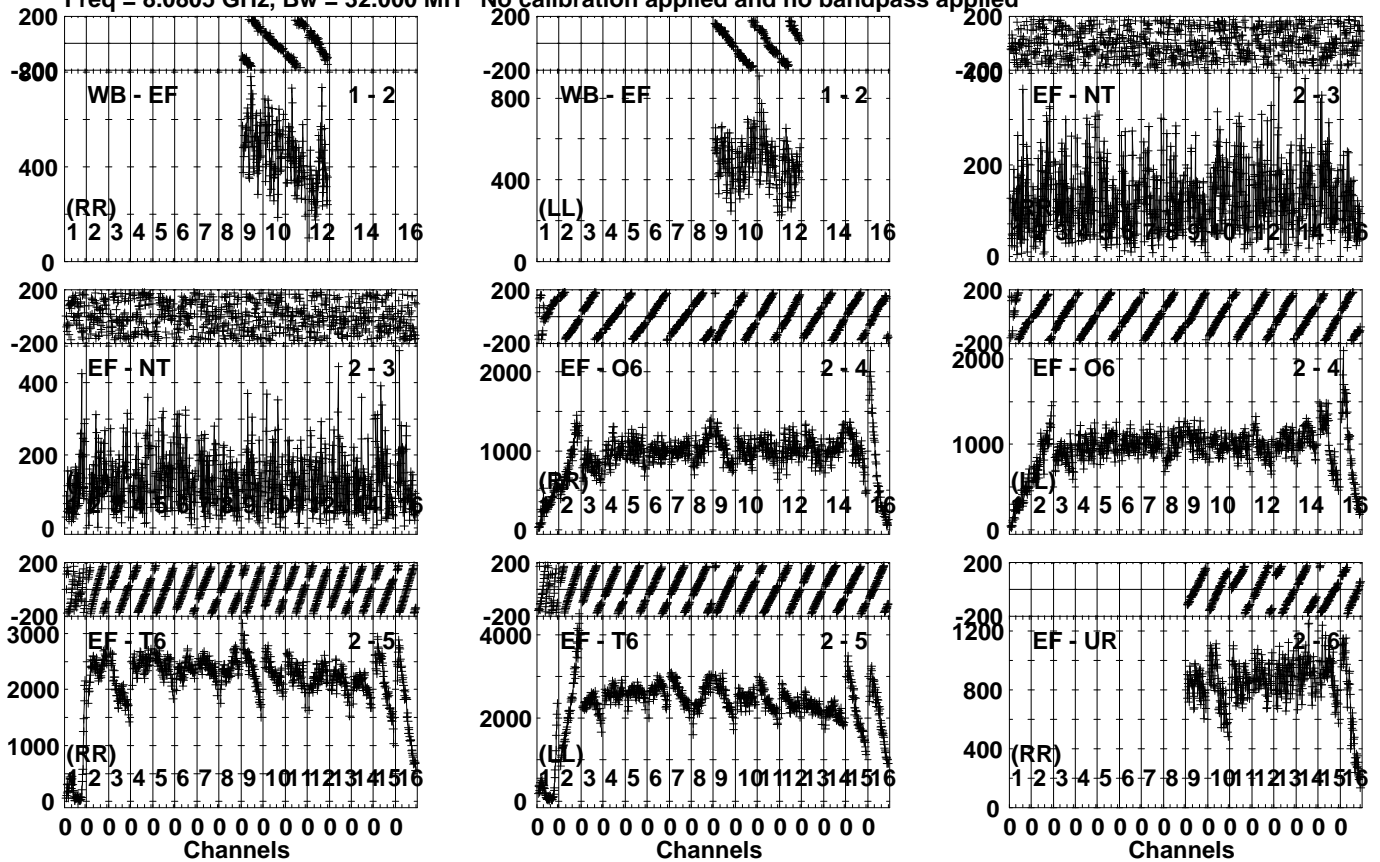
Lower frame: Micro Ampl Jy Top frame: Phas deg Vector averaged cross-power spectrum Several baselines displayed Timerange: 00/10:57:06 to 00/10:58:25
