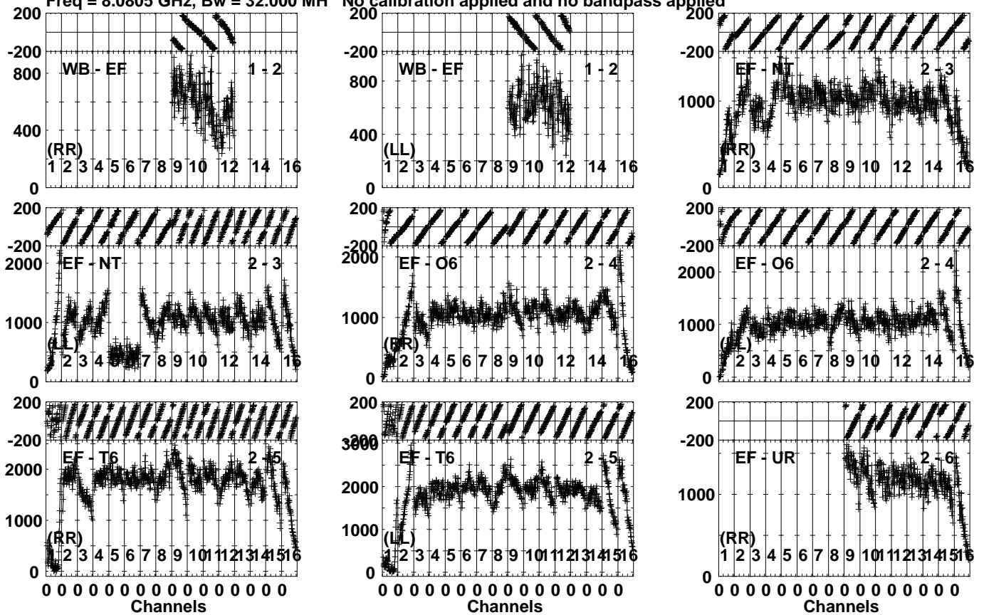
Lower frame: Micro Ampl Jy Top frame: Phas deg Vector averaged cross-power spectrum Several baselines displayed Timerange: 00/13:05:26 to 00/13:06:45
