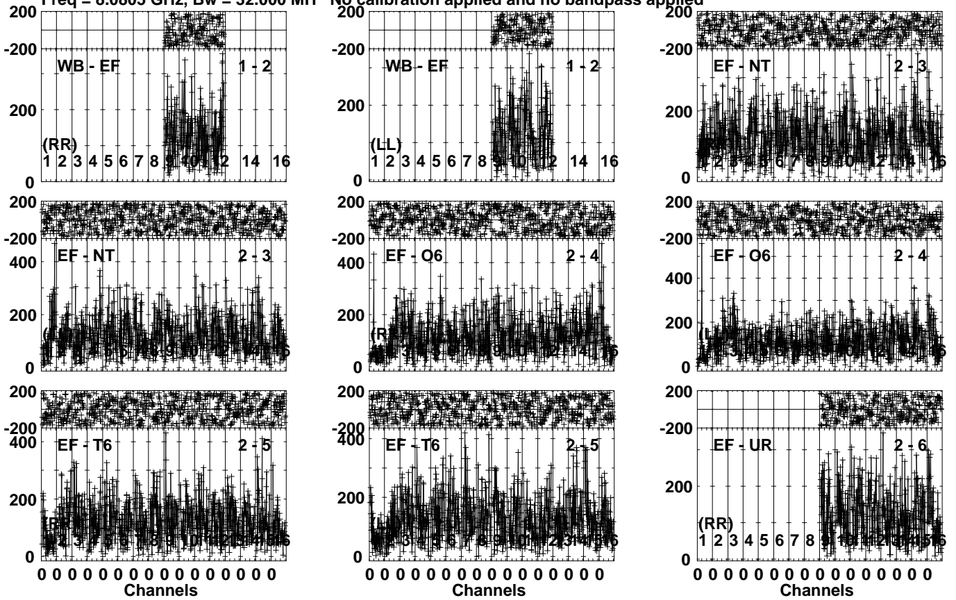
Lower frame: Micro Ampl Jy Top frame: Phas deg Vector averaged cross-power spectrum Several baselines displayed Timerange: 00/12:20:16 to 00/12:22:24
