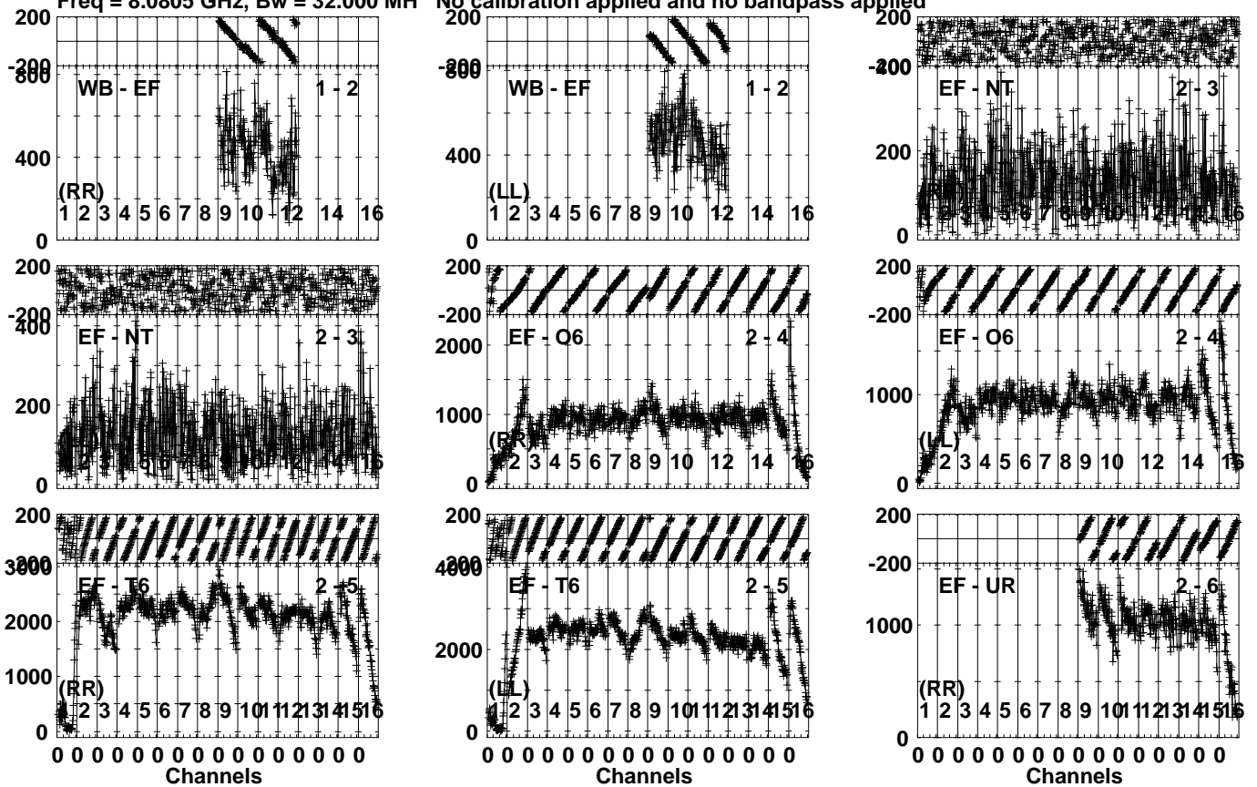
Lower frame: Micro Ampl Jy Top frame: Phas deg Vector averaged cross-power spectrum Several baselines displayed Timerange: 00/10:53:06 to 00/10:54:24
