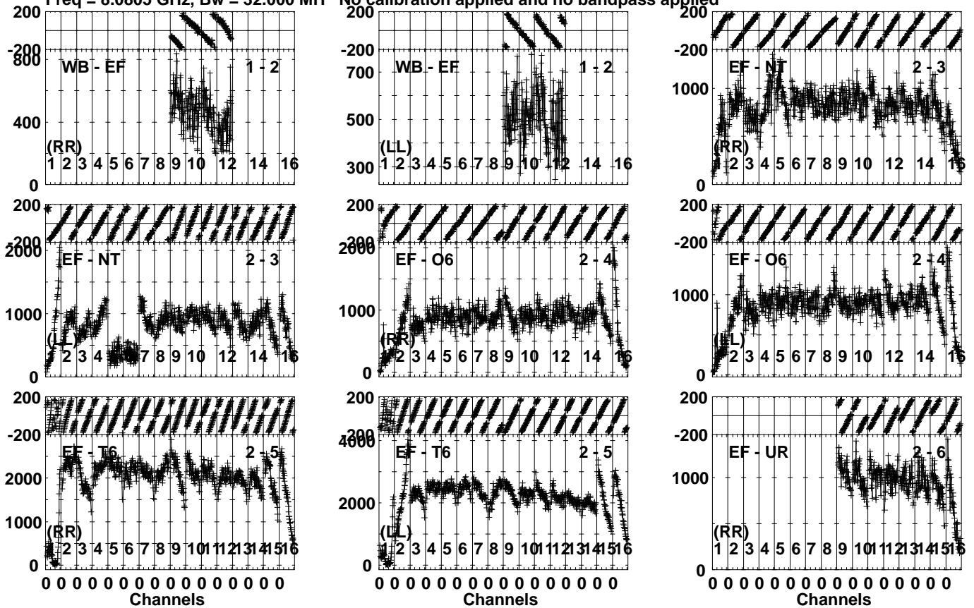
Lower frame: Micro Ampl Jy Top frame: Phas deg Vector averaged cross-power spectrum Several baselines displayed Timerange: 00/09:58:11 to 00/09:59:29
