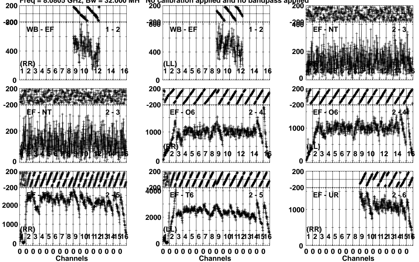
Lower frame: Micro Ampl Jy Top frame: Phas deg Vector averaged cross-power spectrum Several baselines displayed Timerange: 00/11:05:07 to 00/11:06:25
