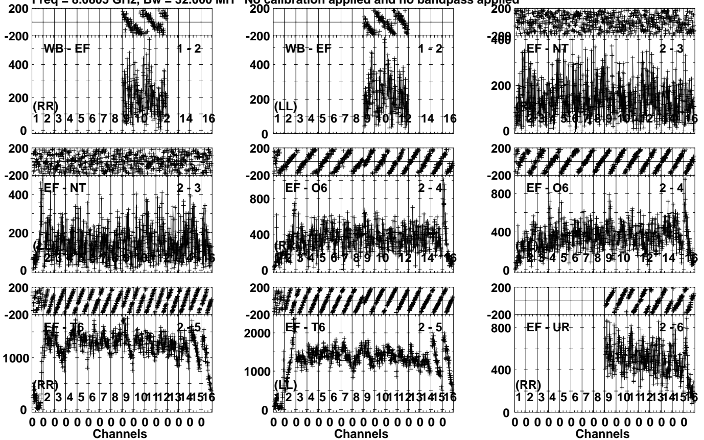
Lower frame: Micro Ampl Jy Top frame: Phas deg Vector averaged cross-power spectrum Several baselines displayed Timerange: 00/11:14:47 to 00/11:16:29
