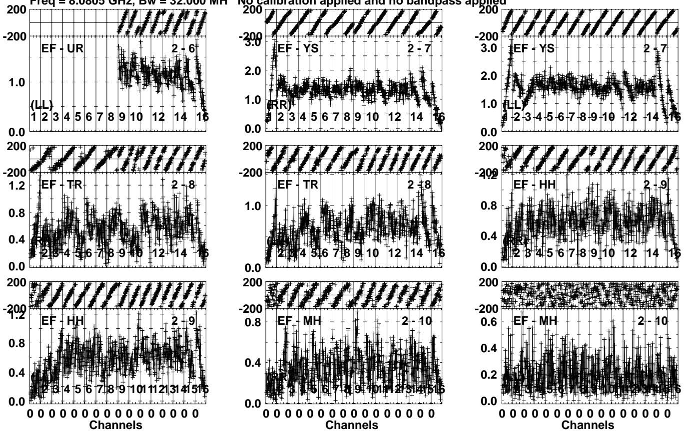
Lower frame: Milli Ampl Jy Top frame: Phas deg Vector averaged cross-power spectrum Several baselines displayed Timerange: 00/10:48:57 to 00/10:50:25
