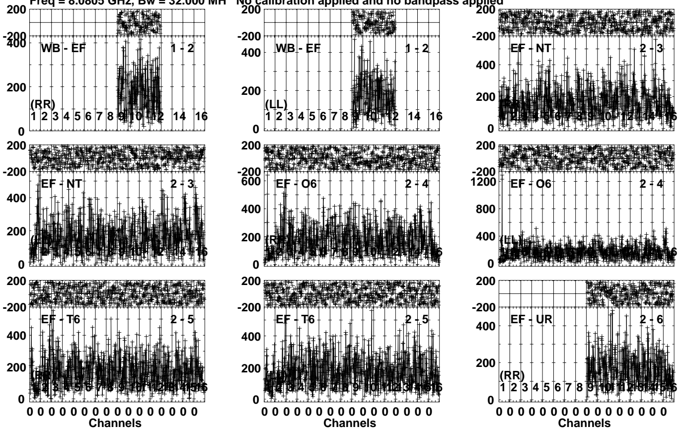
Lower frame: Micro Ampl Jy Top frame: Phas deg Vector averaged cross-power spectrum Several baselines displayed Timerange: 00/12:51:06 to 00/12:52:34
