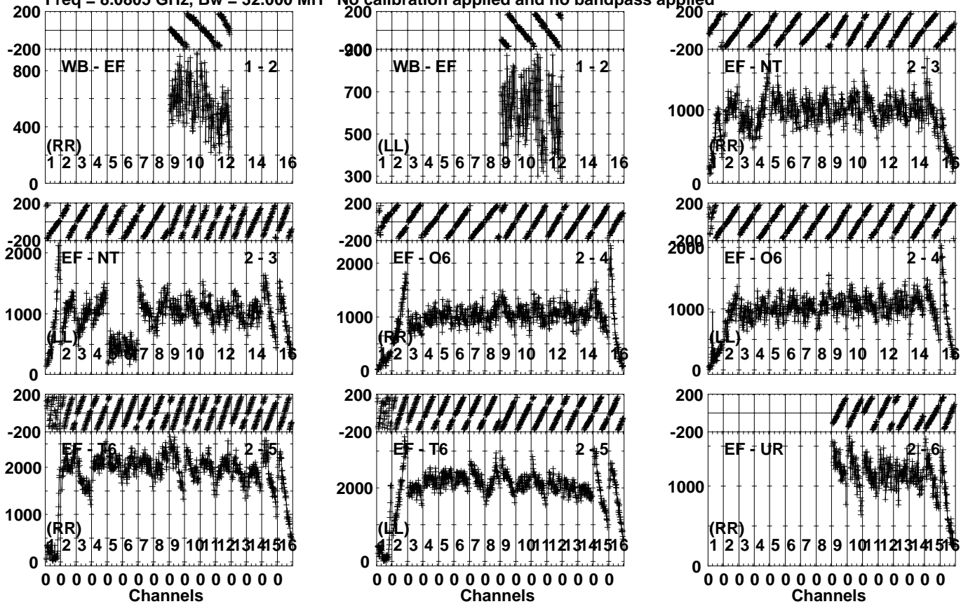
Lower frame: Micro Ampl Jy Top frame: Phas deg Vector averaged cross-power spectrum Several baselines displayed Timerange: 00/12:11:02 to 00/12:12:20
