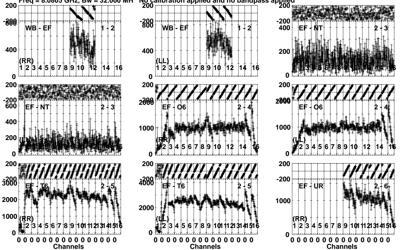
Lower frame: Micro Ampl Jy Top frame: Phas deg Vector averaged cross-power spectrum Several baselines displayed Timerange: 00/11:09:07 to 00/11:10:24
