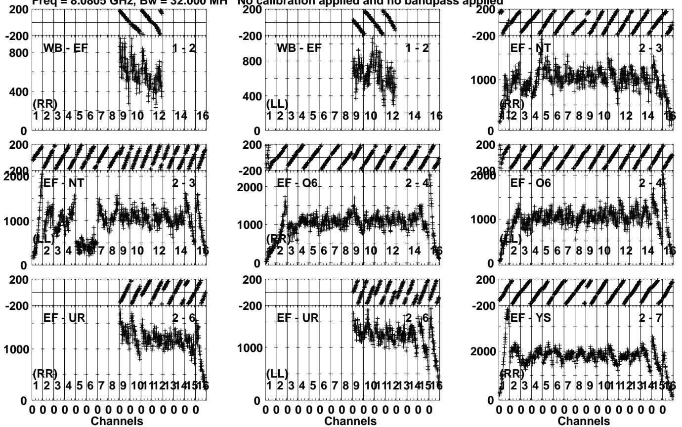
Lower frame: Micro Ampl Jy Top frame: Phas deg Vector averaged cross-power spectrum Several baselines displayed Timerange: 00/13:17:27 to 00/13:18:44
