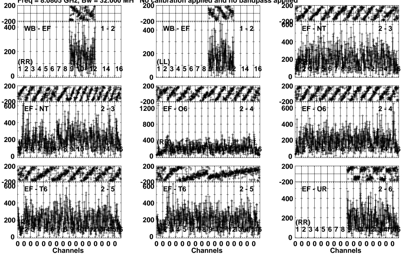
Lower frame: Micro Ampl Jy Top frame: Phas deg Vector averaged cross-power spectrum Several baselines displayed Timerange: 00/12:47:46 to 00/12:49:14
