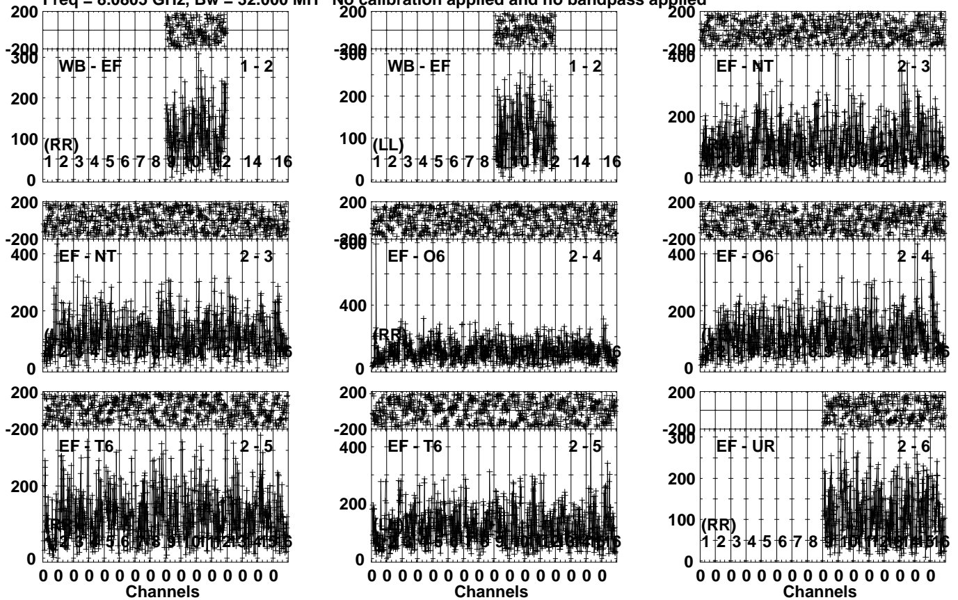
Lower frame: Micro Ampl Jy Top frame: Phas deg Vector averaged cross-power spectrum Several baselines displayed Timerange: 00/11:18:21 to 00/11:20:30
