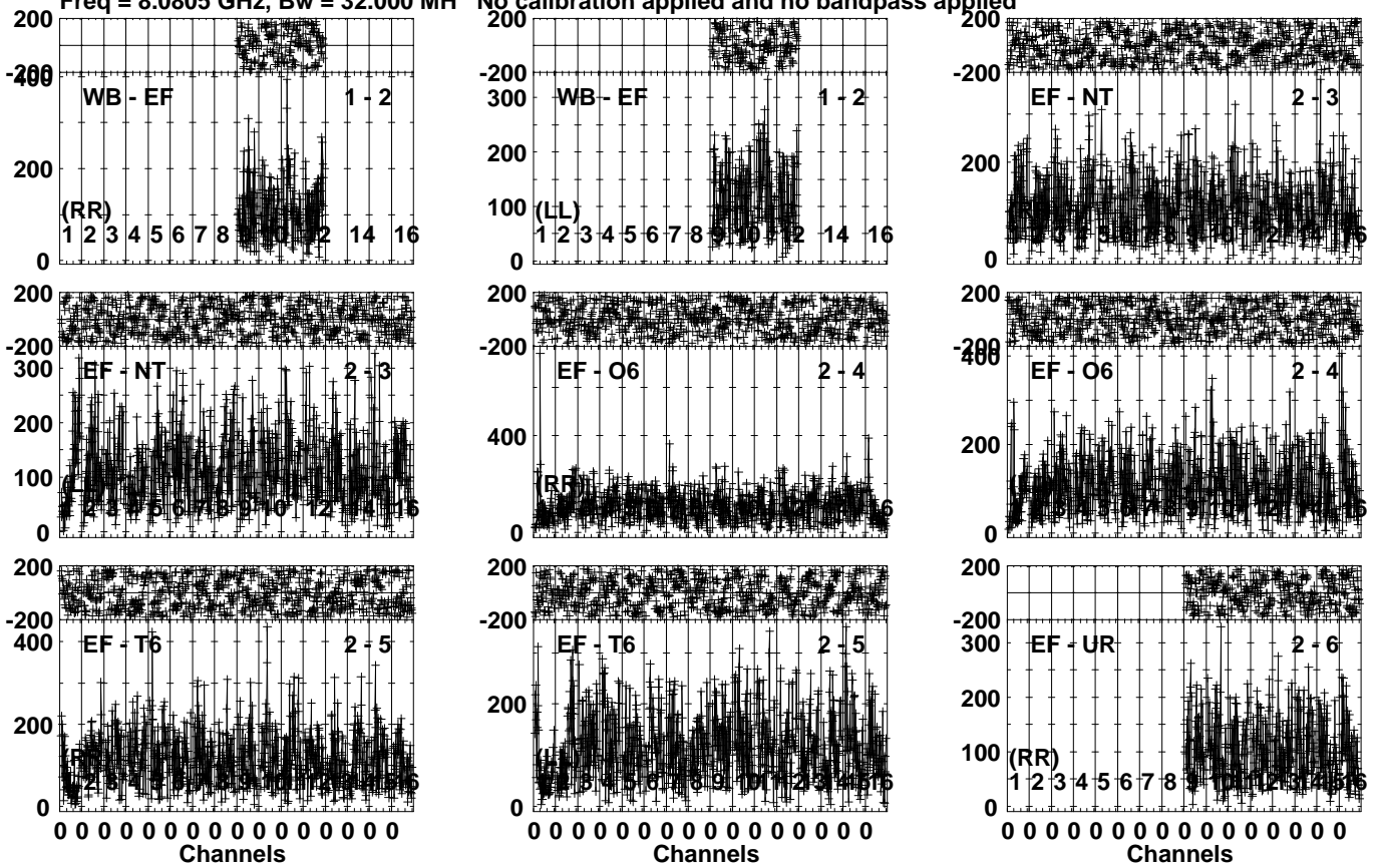
Lower frame: Micro Ampl Jy Top frame: Phas deg Vector averaged cross-power spectrum Several baselines displayed Timerange: 00/11:02:27 to 00/11:04:35
