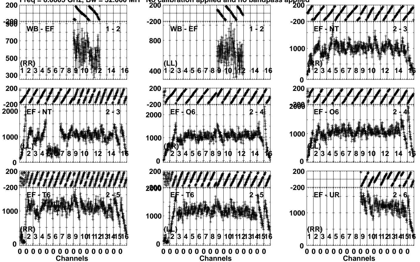
Lower frame: Micro Ampl Jy Top frame: Phas deg Vector averaged cross-power spectrum Several baselines displayed Timerange: 00/13:13:26 to 00/13:14:45
