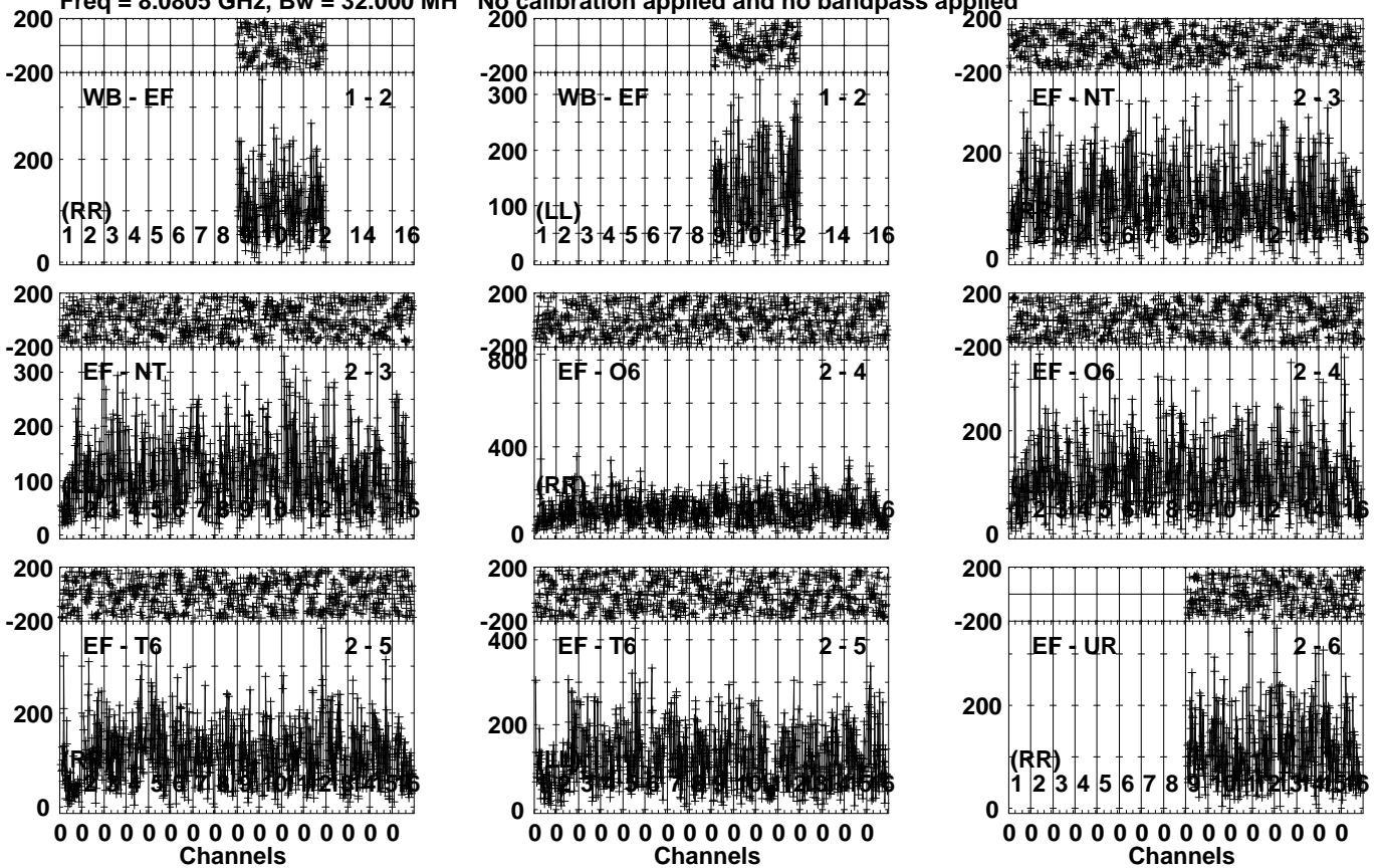
Lower frame: Micro Ampl Jy Top frame: Phas deg Vector averaged cross-power spectrum Several baselines displayed Timerange: 00/11:30:20 to 00/11:32:29
