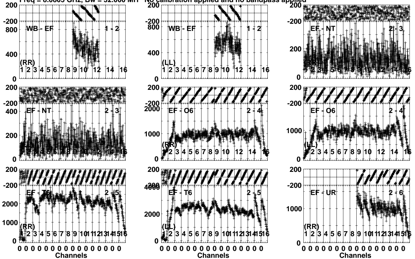
Lower frame: Micro Ampl Jy Top frame: Phas deg Vector averaged cross-power spectrum Several baselines displayed Timerange: 00/10:26:06 to 00/10:27:25
