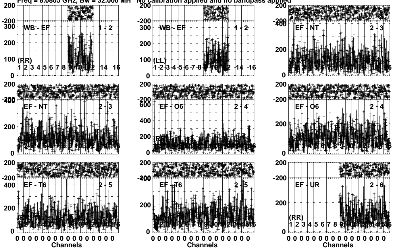
Lower frame: Micro Ampl Jy Top frame: Phas deg Vector averaged cross-power spectrum Several baselines displayed Timerange: 00/13:14:47 to 00/13:16:55
