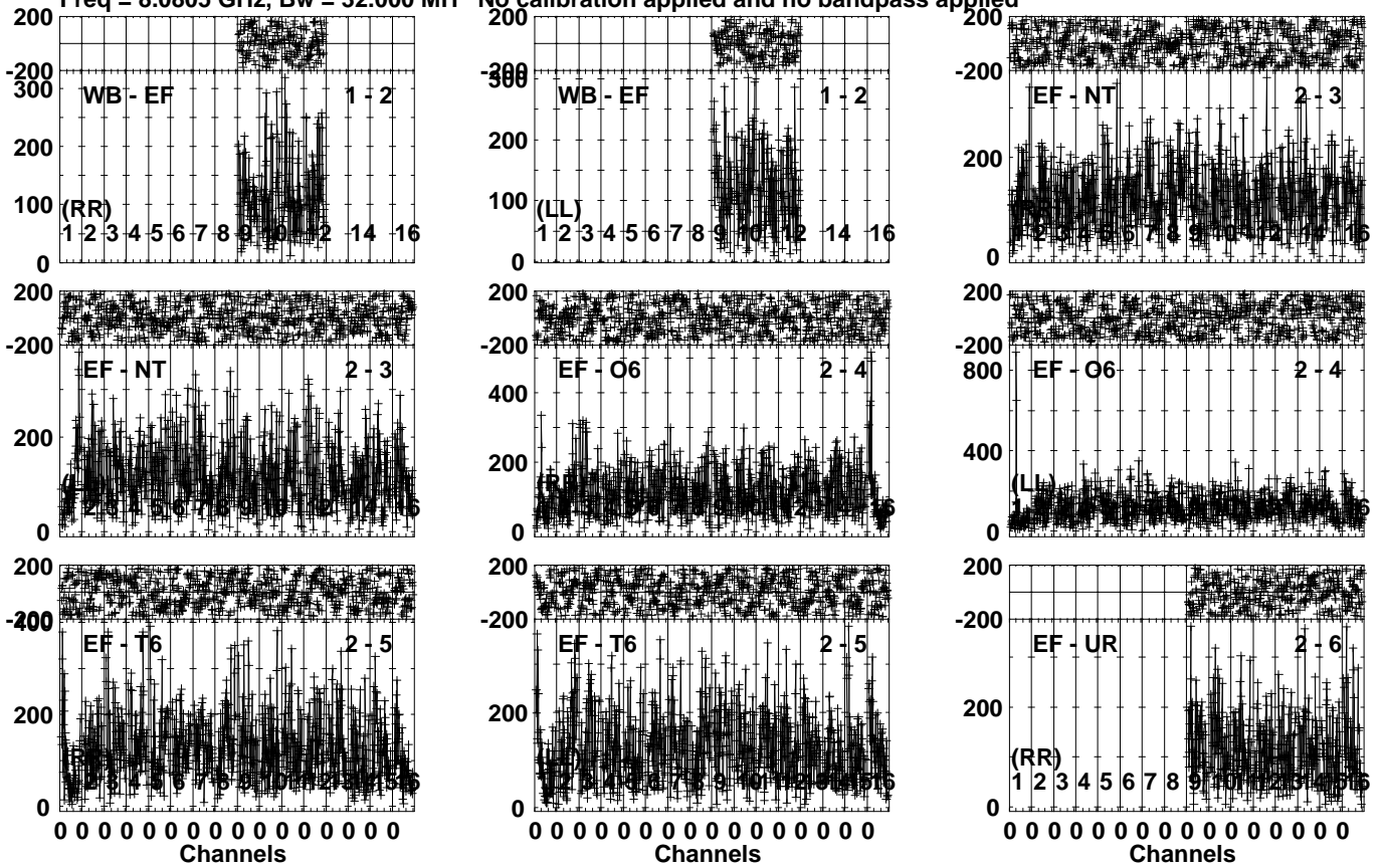
Lower frame: Micro Ampl Jy Top frame: Phas deg Vector averaged cross-power spectrum Several baselines displayed Timerange: 00/09:55:30 to 00/09:57:40
