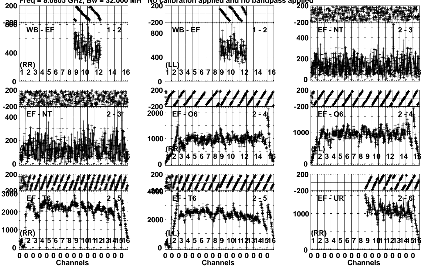
Lower frame: Micro Ampl Jy Top frame: Phas deg Vector averaged cross-power spectrum Several baselines displayed Timerange: 00/11:01:07 to 00/11:02:25
