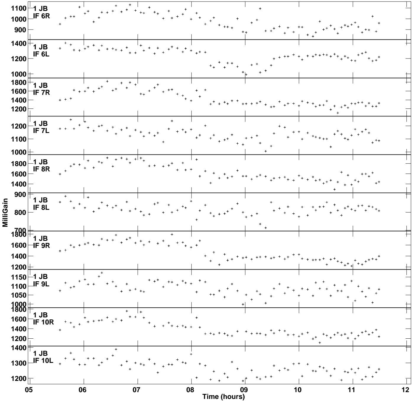
Plot file version 2 created 09-MAR-2023 14:53:34 Gain amp vs UTC time for J191142+1952.MULTI.1 SN 2 Rpol & Lpol IF 1 - 16
