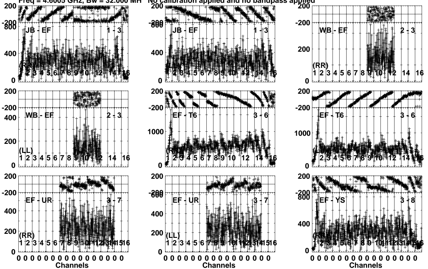
Lower frame: Micro Ampl Jy Top frame: Phas deg Vector averaged cross-power spectrum Several baselines displayed Timerange: 00/06:17:42 to 00/06:18:54
