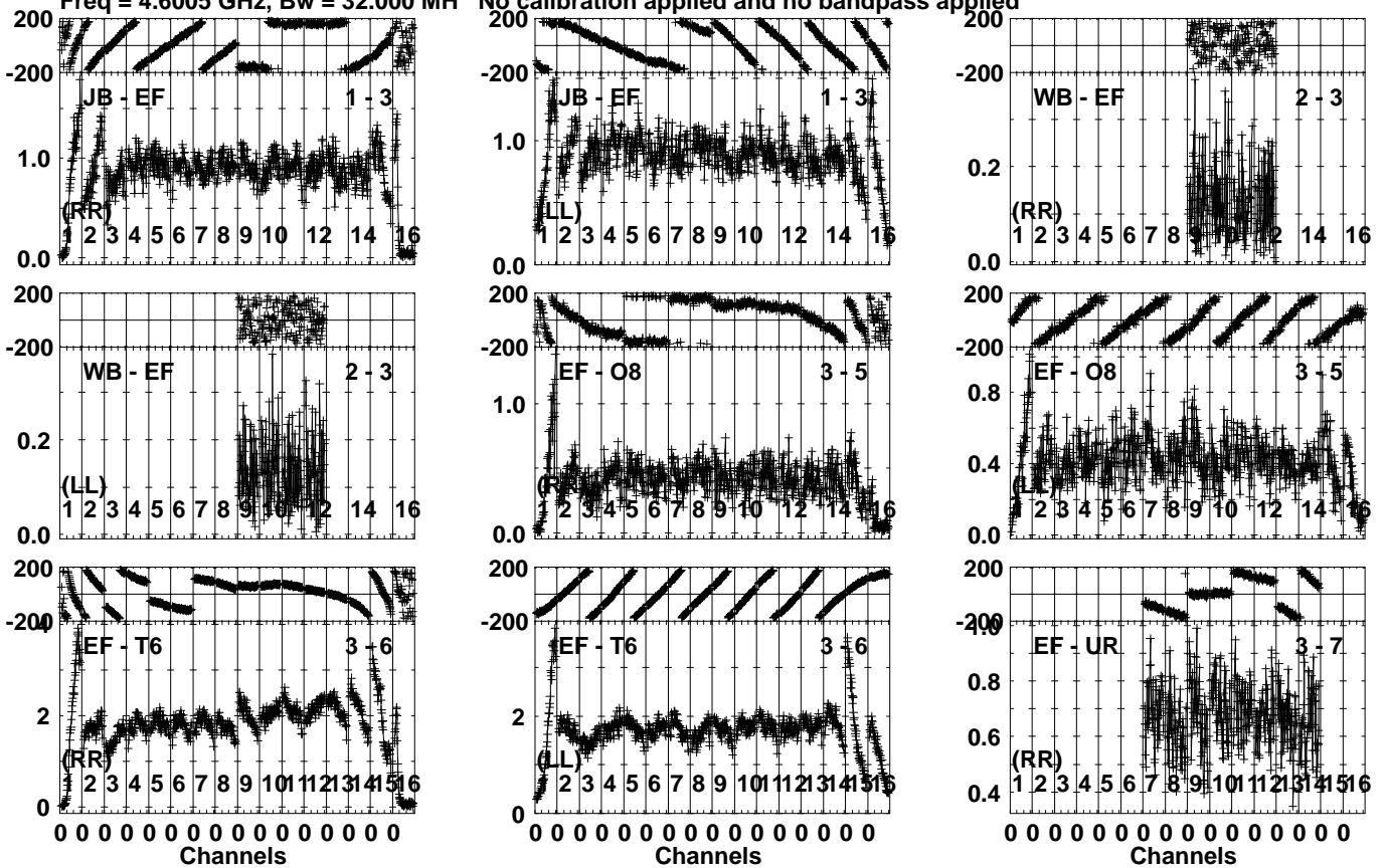
Lower frame: Milli Ampl Jy Top frame: Phas deg Vector averaged cross-power spectrum Several baselines displayed Timerange: 00/07:37:26 to 00/07:38:54
