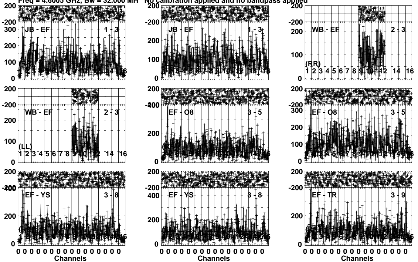
Lower frame: Micro Ampl Jy Top frame: Phas deg Vector averaged cross-power spectrum Several baselines displayed Timerange: 00/11:11:17 to 00/11:13:30
