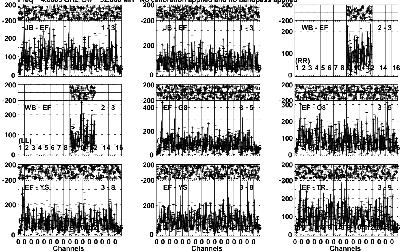
Lower frame: Micro Ampl Jy Top frame: Phas deg Vector averaged cross-power spectrum Several baselines displayed Timerange: 00/10:19:46 to 00/10:22:15
