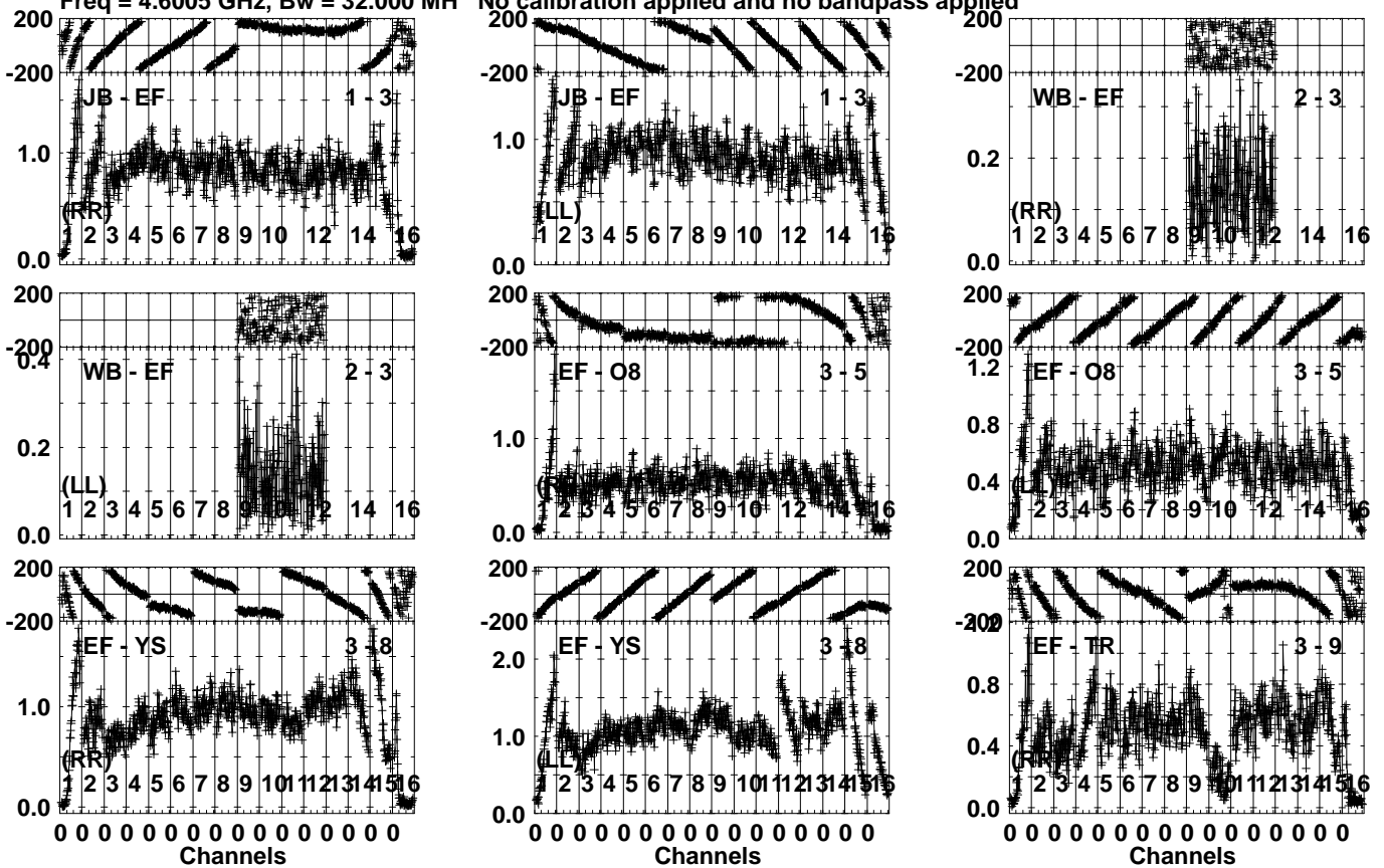
Lower frame: Milli Ampl Jy Top frame: Phas deg Vector averaged cross-power spectrum Several baselines displayed Timerange: 00/11:17:11 to 00/11:18:39
