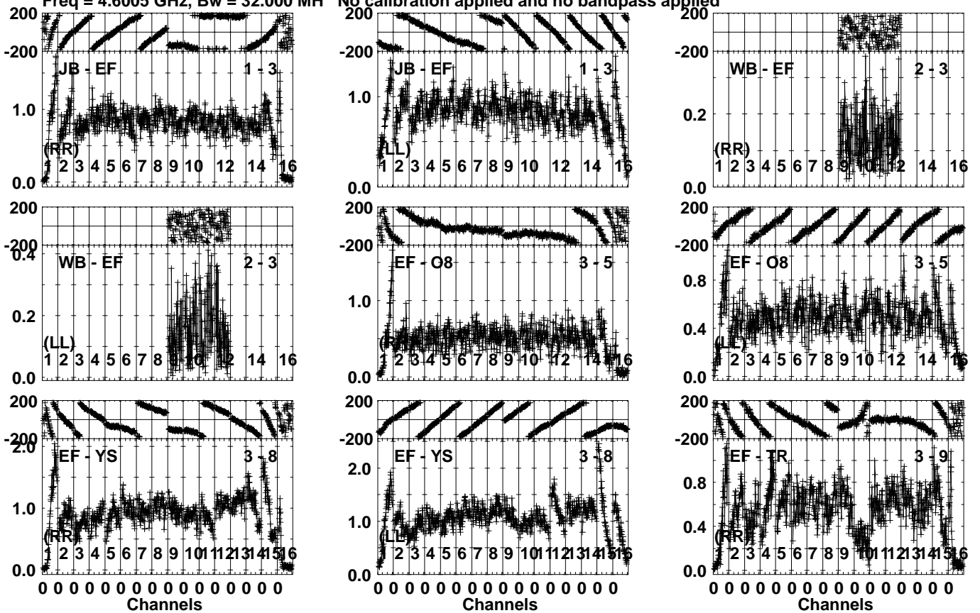
Lower frame: Milli Ampl Jy Top frame: Phas deg Vector averaged cross-power spectrum Several baselines displayed Timerange: 00/11:02:02 to 00/11:03:14
