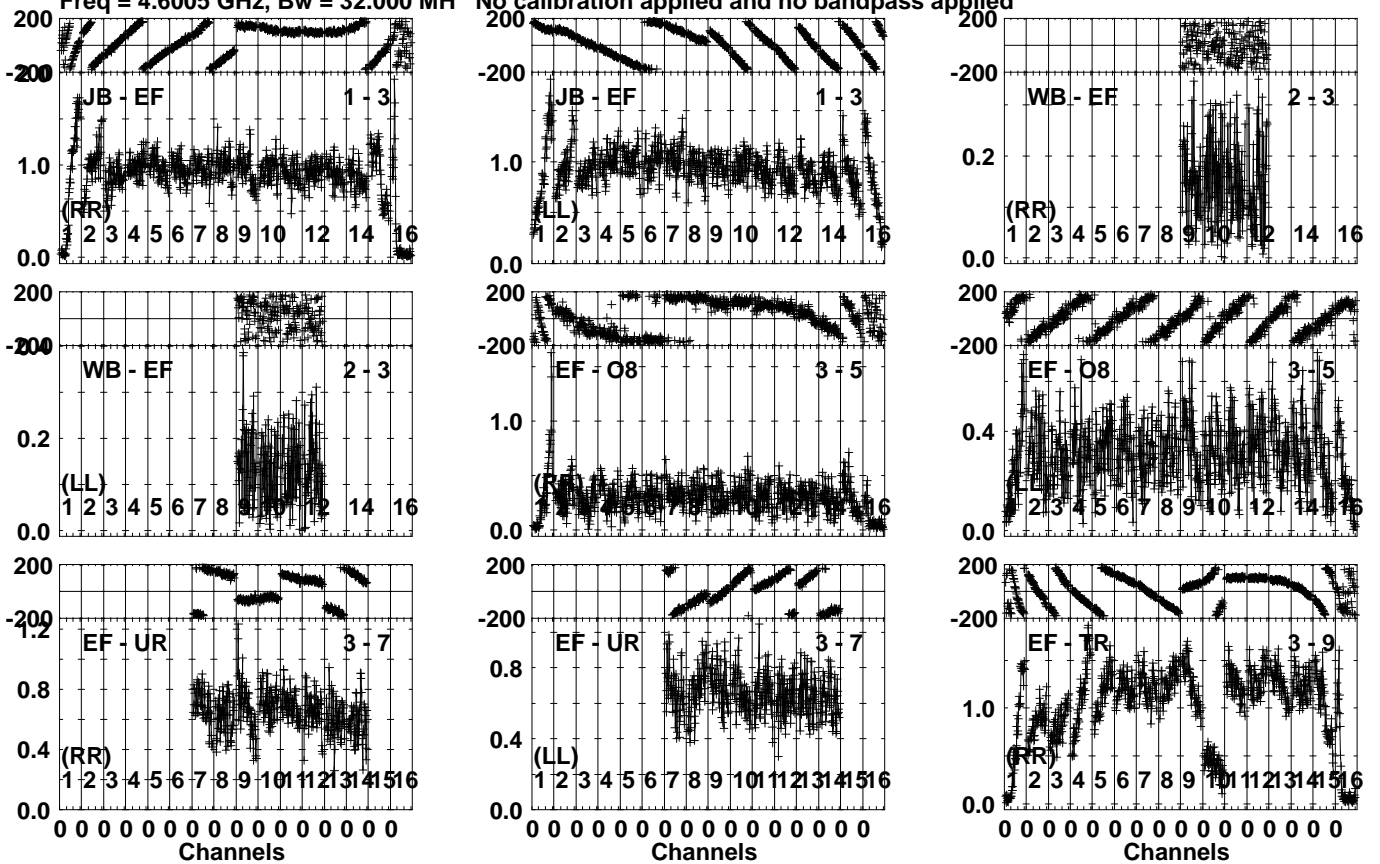
Lower frame: Milli Ampl Jy Top frame: Phas deg Vector averaged cross-power spectrum Several baselines displayed Timerange: 00/09:28:11 to 00/09:29:25
