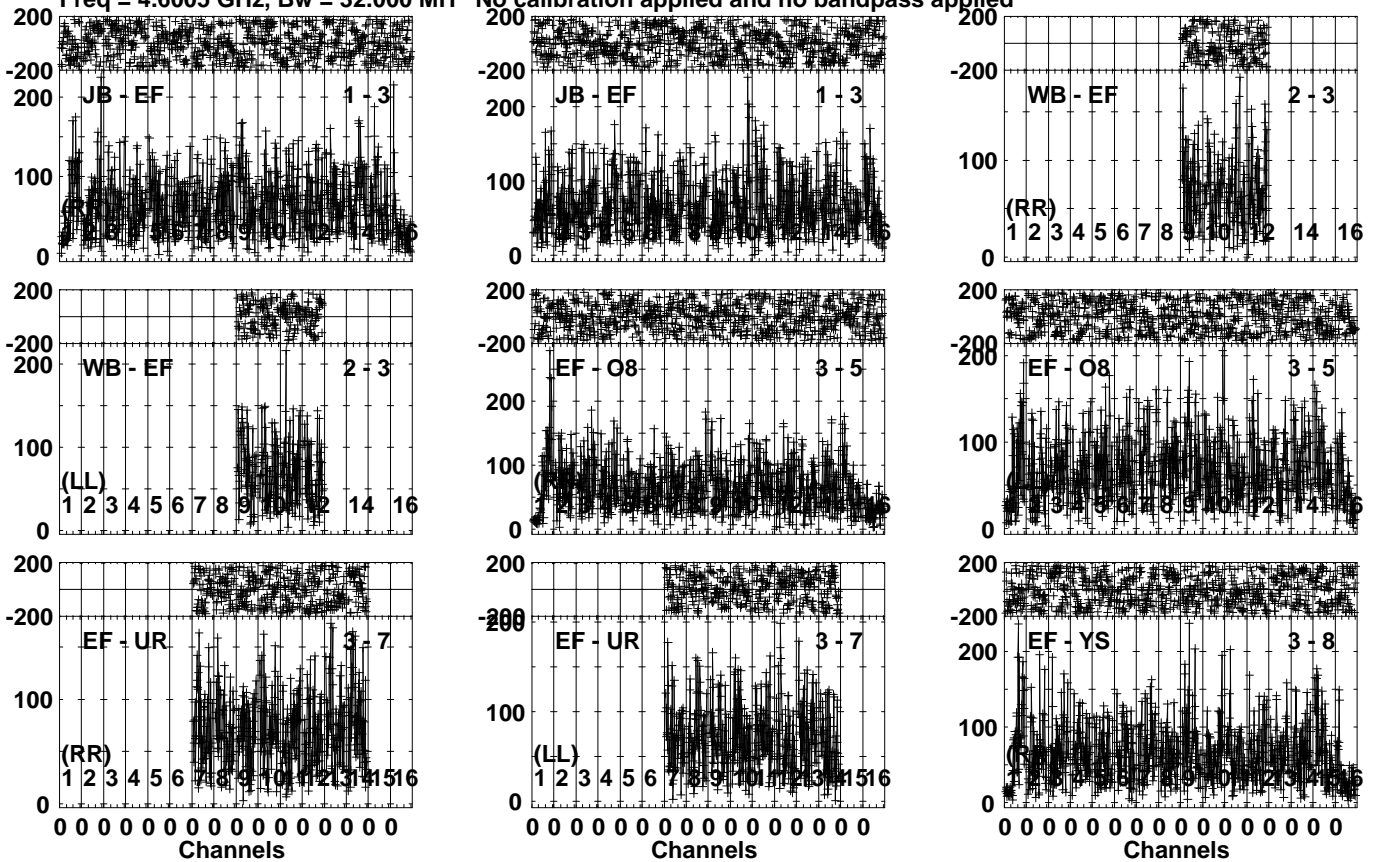
Lower frame: Micro Ampl Jy Top frame: Phas deg Vector averaged cross-power spectrum Several baselines displayed Timerange: 00/09:48:47 to 00/09:53:00
