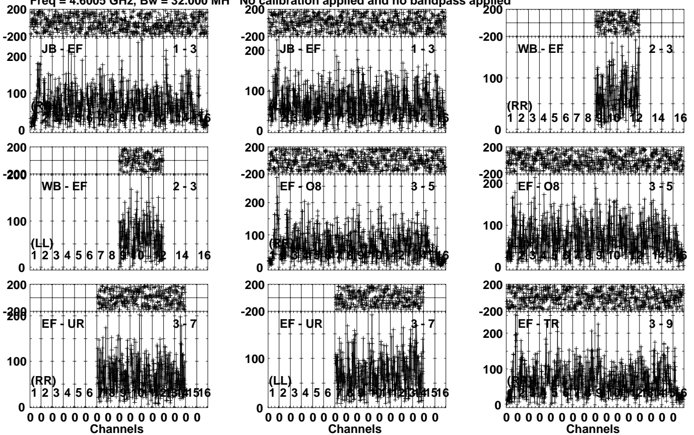
Lower frame: Micro Ampl Jy Top frame: Phas deg Vector averaged cross-power spectrum Several baselines displayed Timerange: 00/08:31:56 to 00/08:36:10
