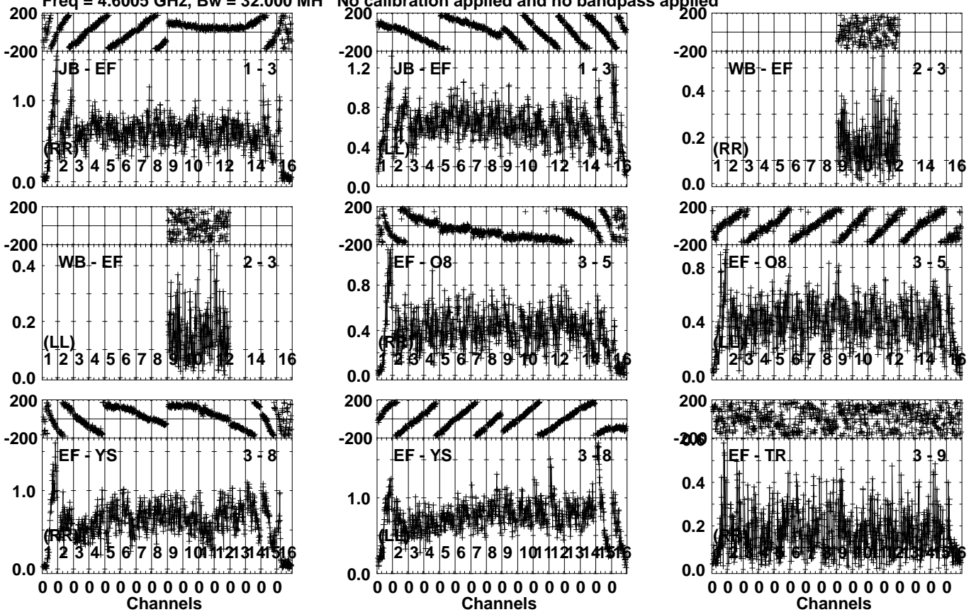
Lower frame: Milli Ampl Jy Top frame: Phas deg Vector averaged cross-power spectrum Several baselines displayed Timerange: 00/11:15:27 to 00/11:16:40
