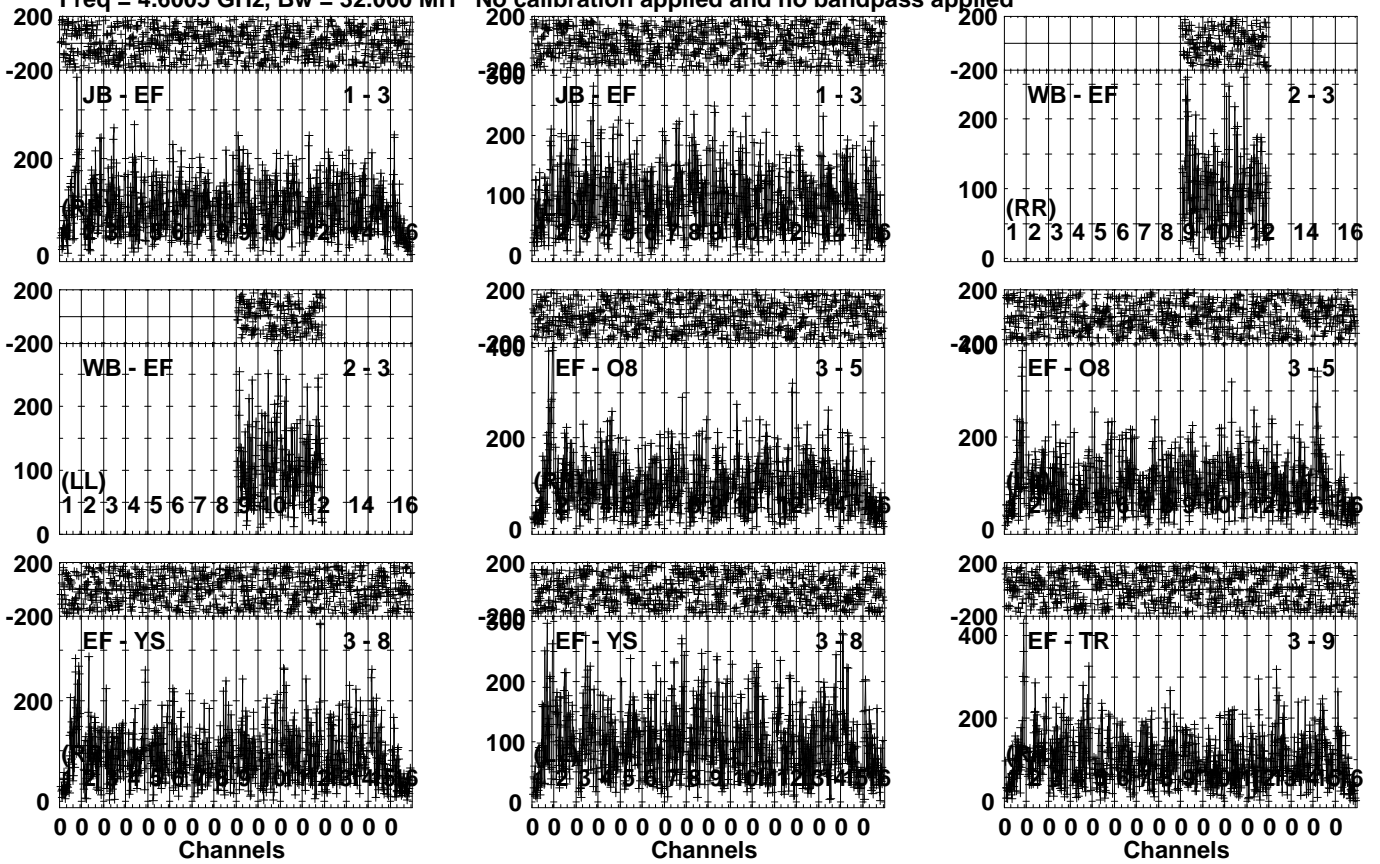
Lower frame: Micro Ampl Jy Top frame: Phas deg Vector averaged cross-power spectrum Several baselines displayed Timerange: 00/11:22:56 to 00/11:25:10
