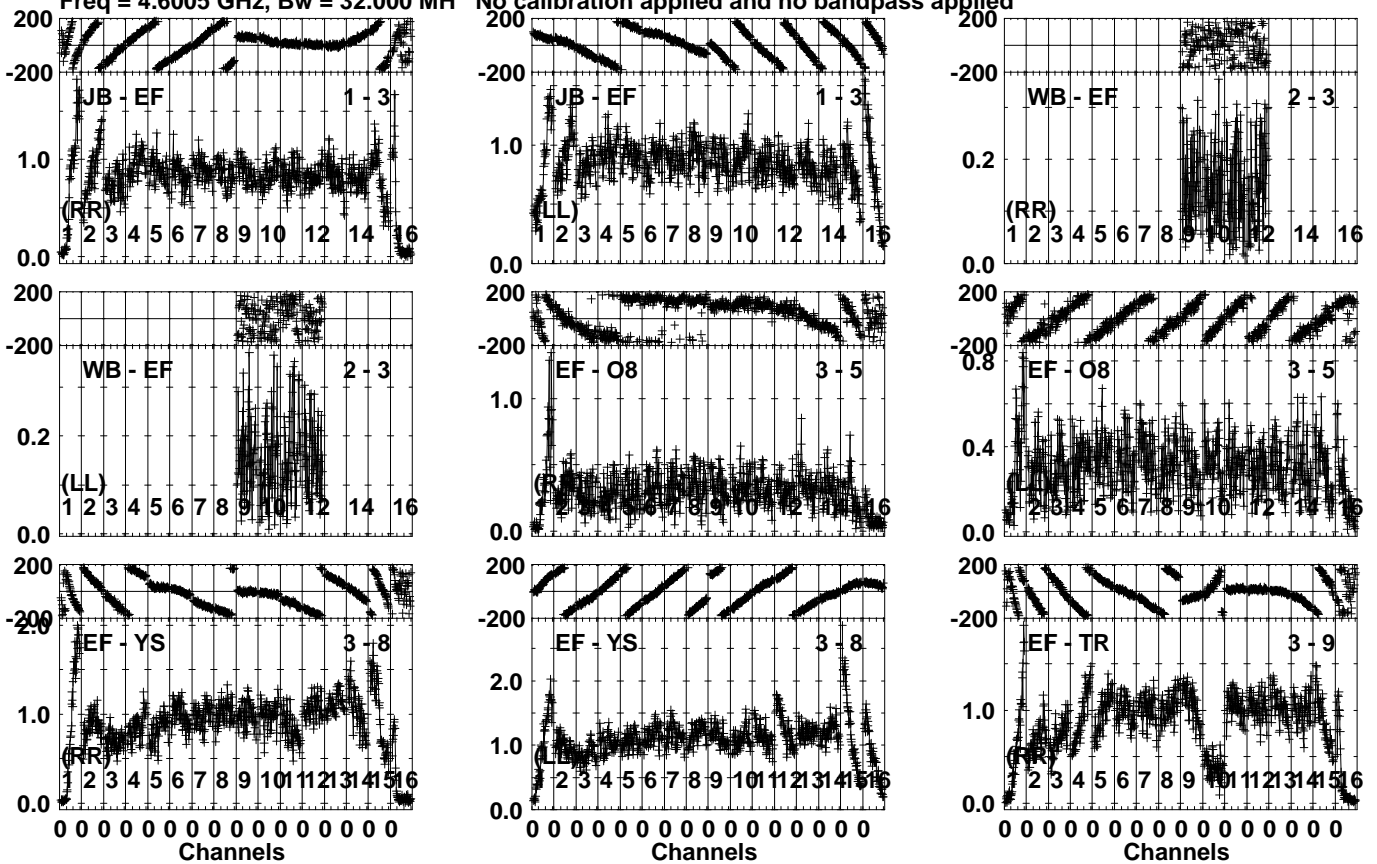
Lower frame: Milli Ampl Jy Top frame: Phas deg Vector averaged cross-power spectrum Several baselines displayed Timerange: 00/10:14:56 to 00/10:16:10
