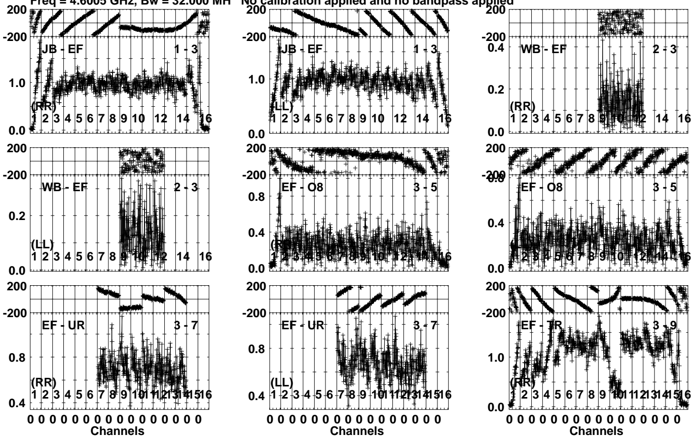
Lower frame: Milli Ampl Jy Top frame: Phas deg Vector averaged cross-power spectrum Several baselines displayed Timerange: 00/08:36:26 to 00/08:37:39
