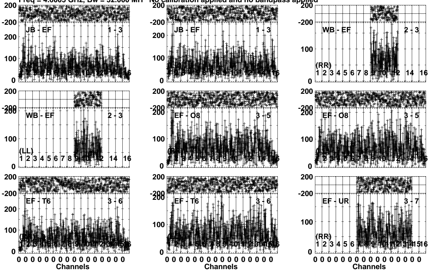
Lower frame: Micro Ampl Jy Top frame: Phas deg Vector averaged cross-power spectrum Several baselines displayed Timerange: 00/07:45:11 to 00/07:49:24
