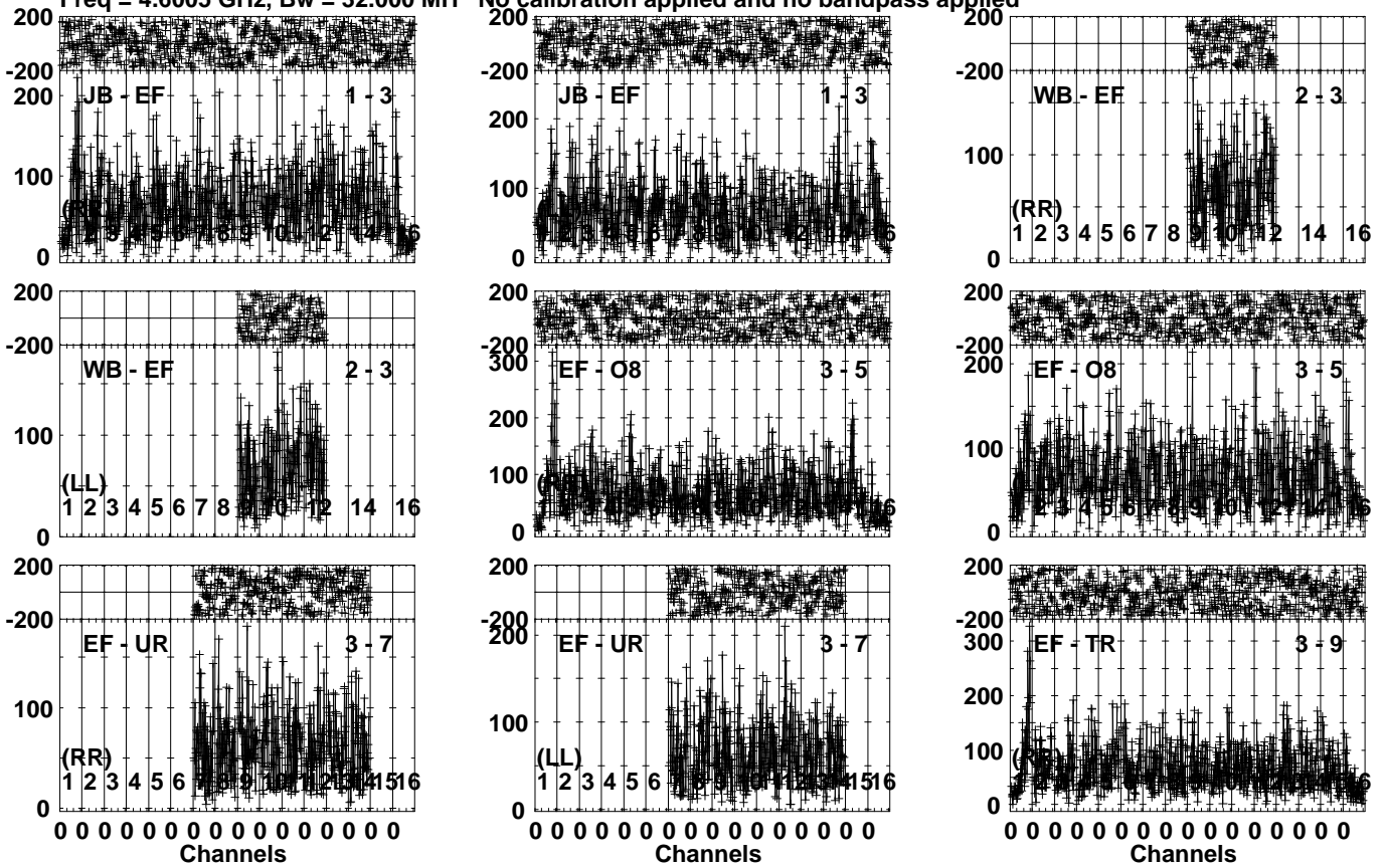
Lower frame: Micro Ampl Jy Top frame: Phas deg Vector averaged cross-power spectrum Several baselines displayed Timerange: 00/08:46:16 to 00/08:50:30
