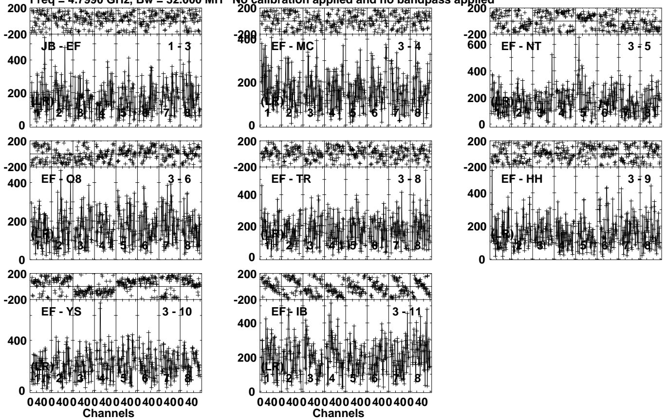
Lower frame: Micro Ampl Jy Top frame: Phas deg Vector averaged cross-power spectrum Several baselines displayed Timerange: 01/00:04:01 to 01/00:05:49
