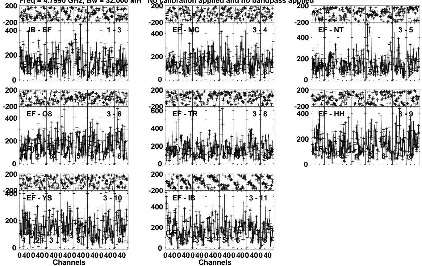
Lower frame: Micro Ampl Jy Top frame: Phas deg Vector averaged cross-power spectrum Several baselines displayed Timerange: 00/21:05:21 to 00/21:06:29
