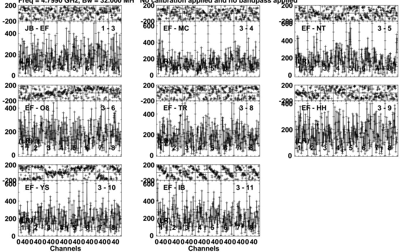
Lower frame: Micro Ampl Jy Top frame: Phas deg Vector averaged cross-power spectrum Several baselines displayed Timerange: 01/00:25:47 to 01/00:26:49
