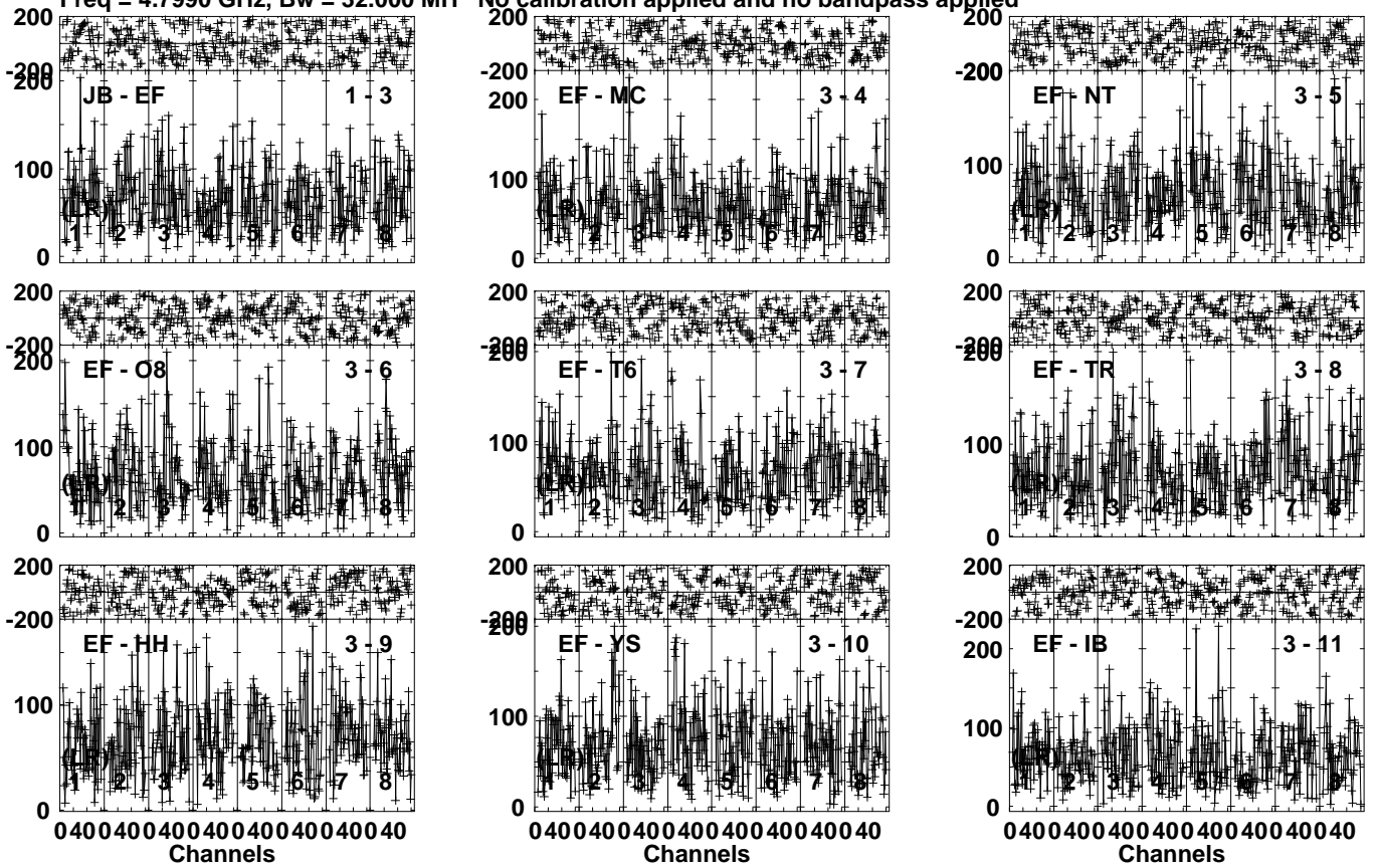
Lower frame: Micro Ampl Jy Top frame: Phas deg Vector averaged cross-power spectrum Several baselines displayed Timerange: 00/21:43:07 to 00/21:47:39
