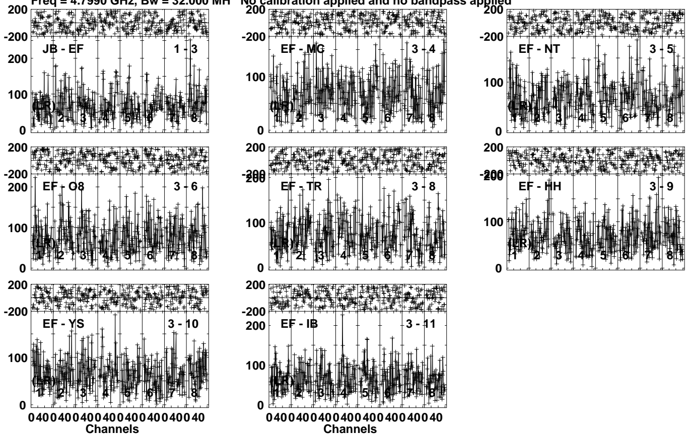
Lower frame: Micro Ampl Jy Top frame: Phas deg Vector averaged cross-power spectrum Several baselines displayed Timerange: 00/19:50:31 to 00/19:55:03
