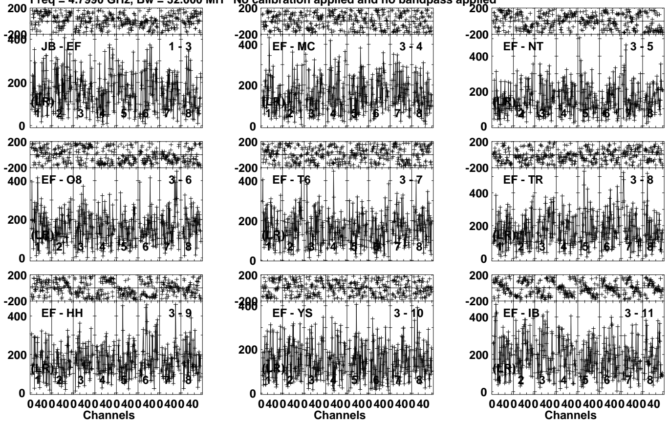
Lower frame: Micro Ampl Jy Top frame: Phas deg Vector averaged cross-power spectrum Several baselines displayed Timerange: 00/22:33:37 to 00/22:34:39
