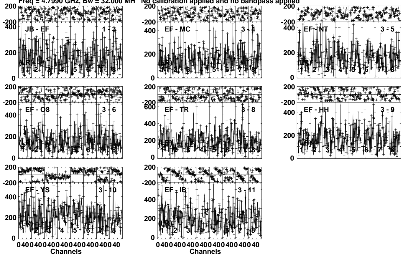
Lower frame: Micro Ampl Jy Top frame: Phas deg Vector averaged cross-power spectrum Several baselines displayed Timerange: 01/00:46:57 to 01/00:47:59
