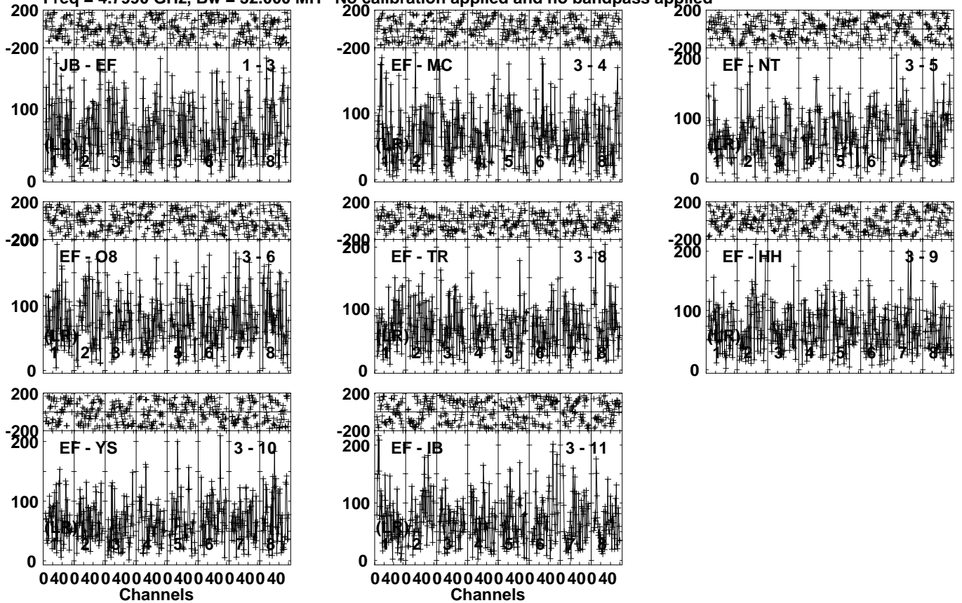
Lower frame: Micro Ampl Jy Top frame: Phas deg Vector averaged cross-power spectrum Several baselines displayed Timerange: 00/20:20:57 to 00/20:25:29
