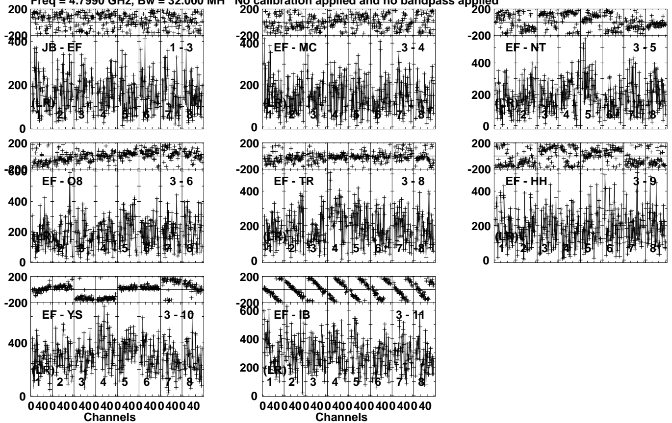
Lower frame: Micro Ampl Jy Top frame: Phas deg Vector averaged cross-power spectrum Several baselines displayed Timerange: 01/00:32:51 to 01/00:34:33
