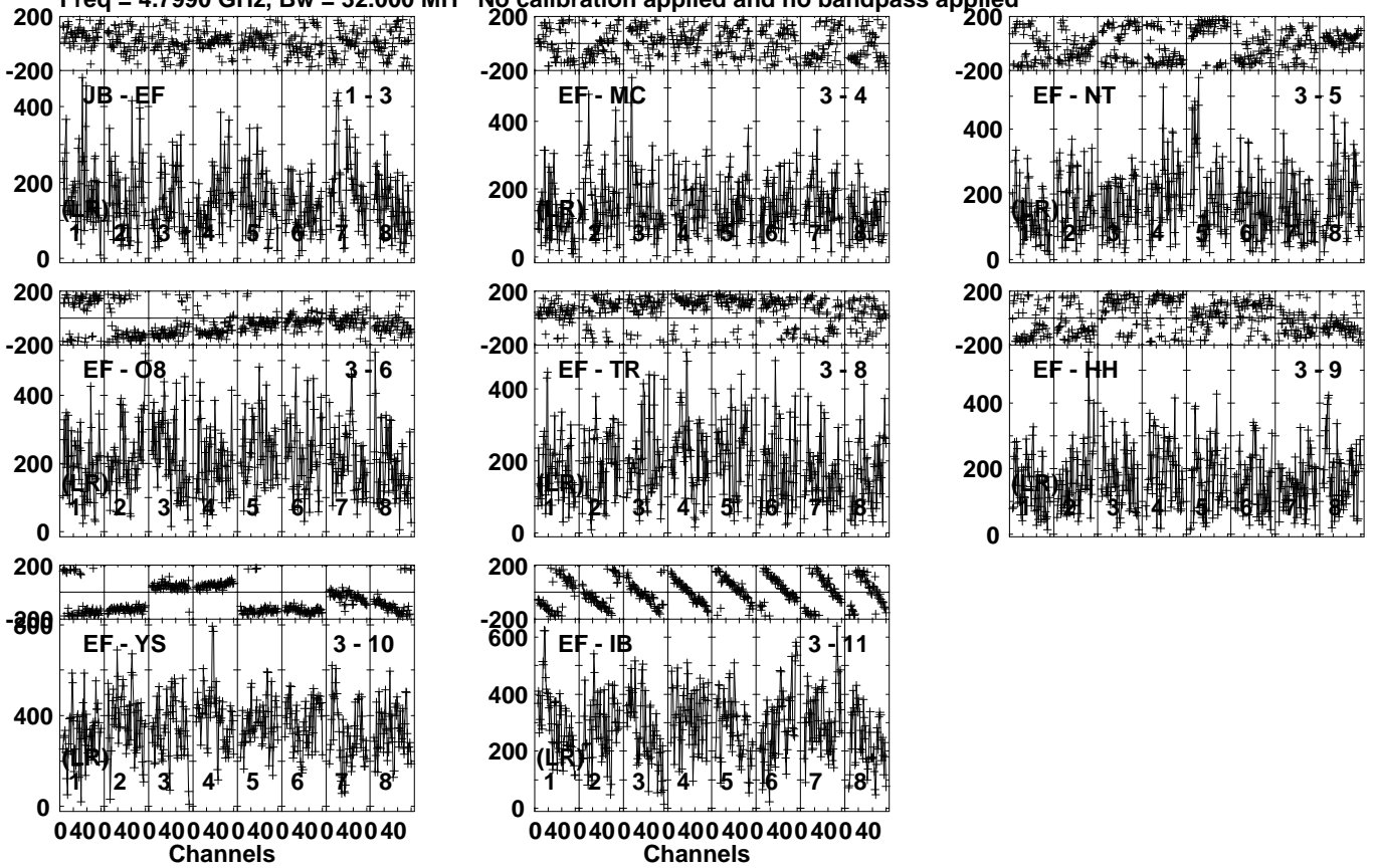
Lower frame: Micro Ampl Jy Top frame: Phas deg Vector averaged cross-power spectrum Several baselines displayed Timerange: 01/01:18:27 to 01/01:20:09
