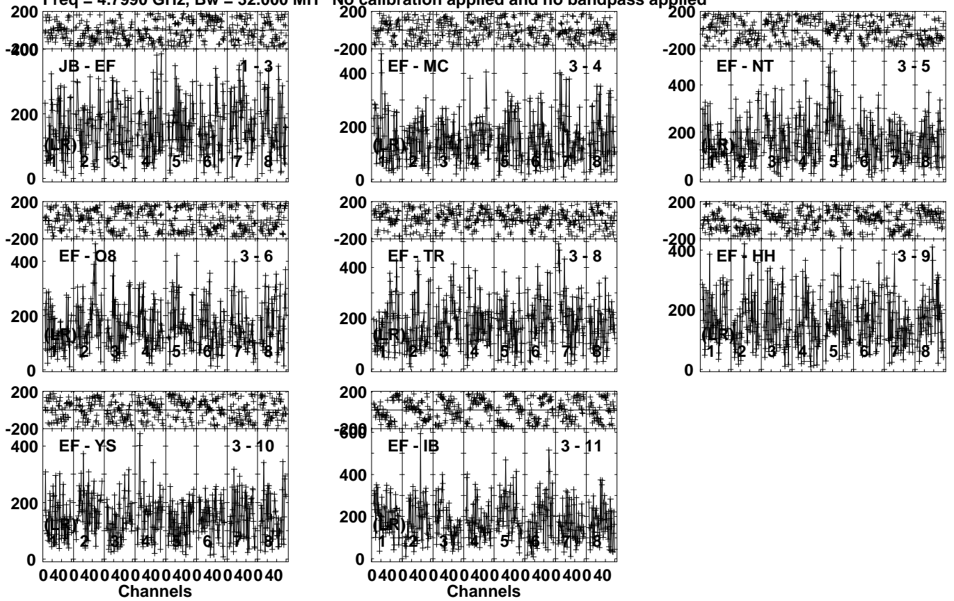
Lower frame: Micro Ampl Jy Top frame: Phas deg Vector averaged cross-power spectrum Several baselines displayed Timerange: 00/19:55:27 to 00/19:56:29
