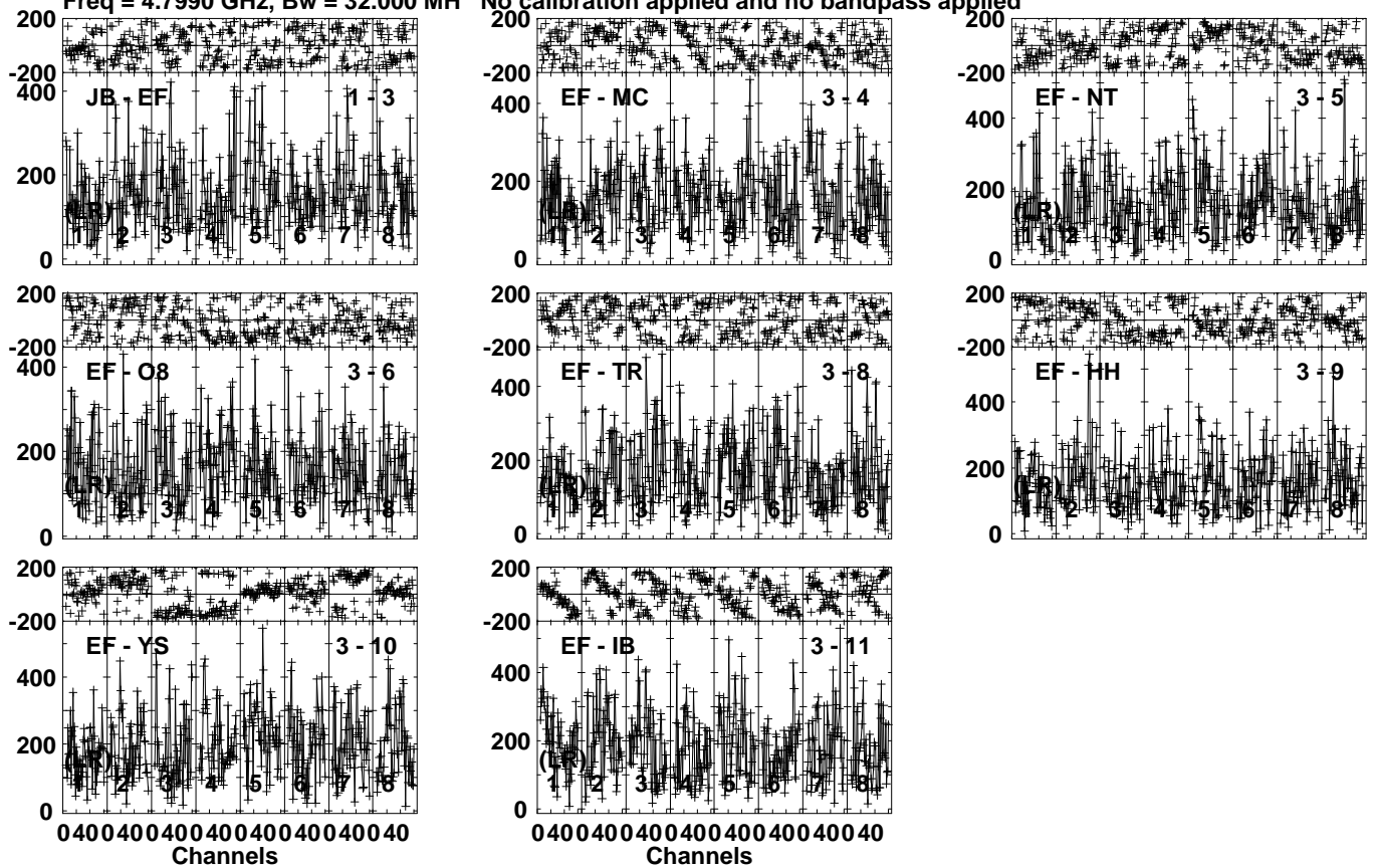
Lower frame: Micro Ampl Jy Top frame: Phas deg Vector averaged cross-power spectrum Several baselines displayed Timerange: 00/23:19:11 to 00/23:20:13
