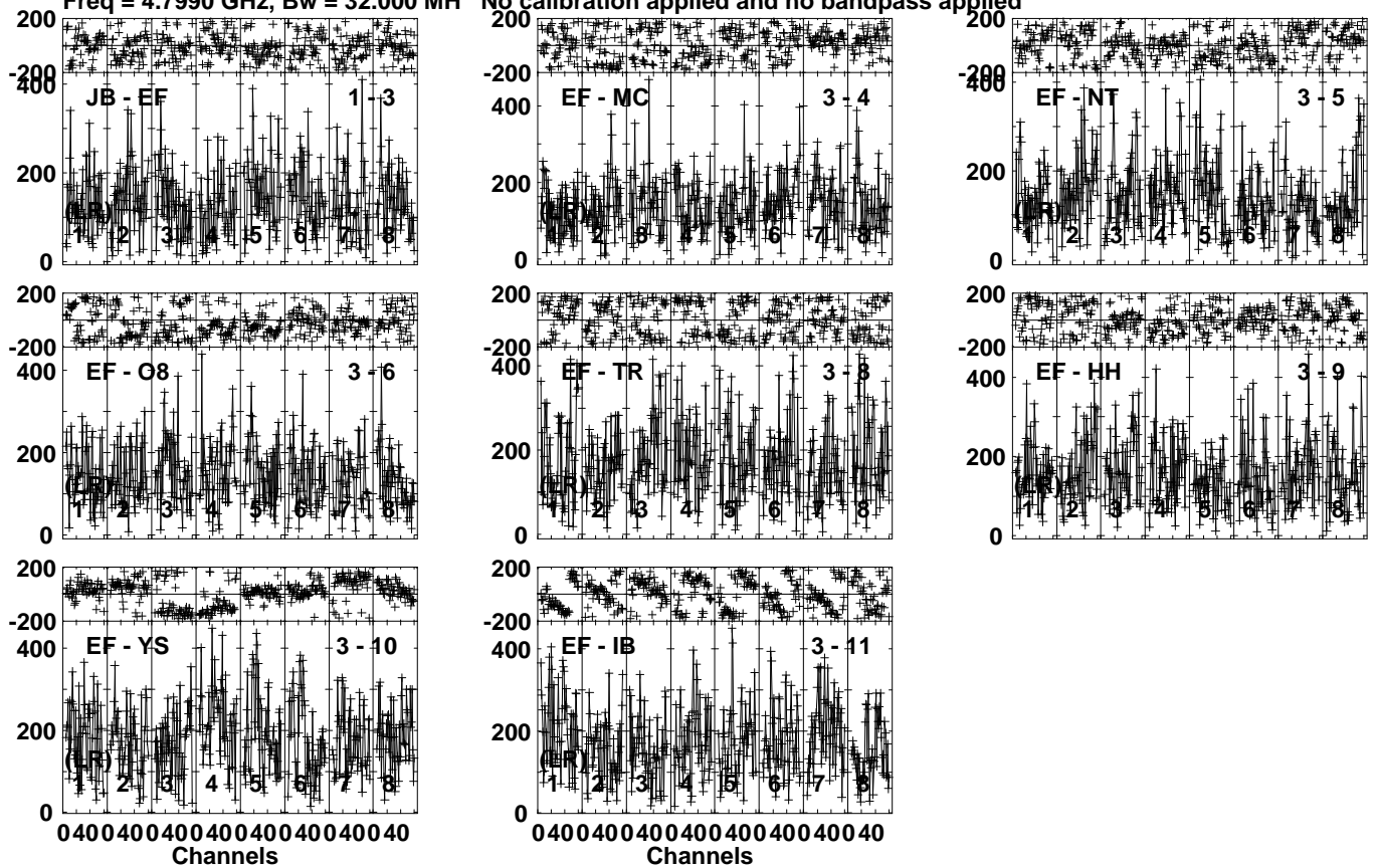
Lower frame: Micro Ampl Jy Top frame: Phas deg Vector averaged cross-power spectrum Several baselines displayed Timerange: 00/23:34:11 to 00/23:35:13
