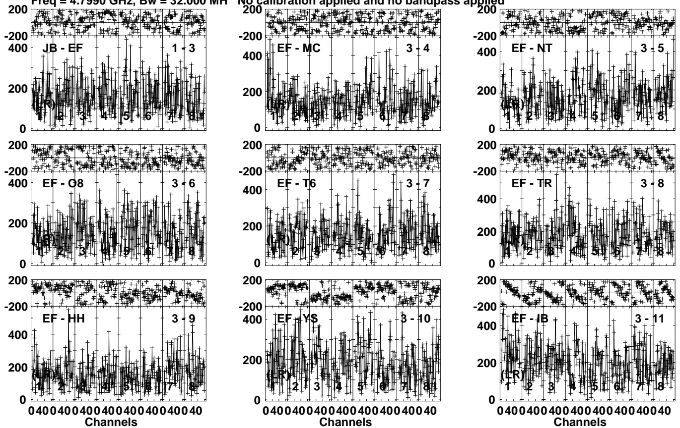
Lower frame: Micro Ampl Jy Top frame: Phas deg Vector averaged cross-power spectrum Several baselines displayed Timerange: 00/22:48:37 to 00/22:49:39
