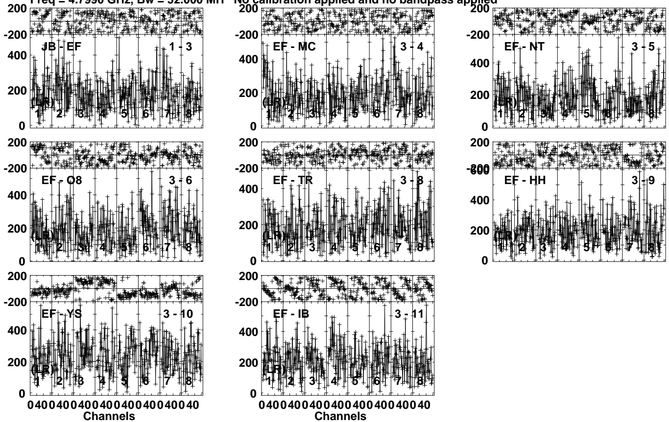
Lower frame: Micro Ampl Jy Top frame: Phas deg Vector averaged cross-power spectrum Several baselines displayed Timerange: 01/01:20:31 to 01/01:21:33
