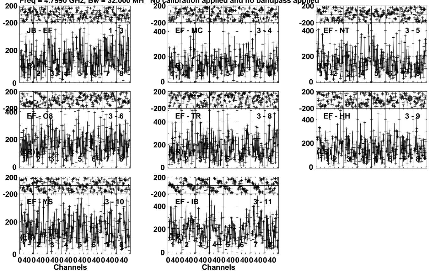
Lower frame: Micro Ampl Jy Top frame: Phas deg Vector averaged cross-power spectrum Several baselines displayed Timerange: 00/20:25:51 to 00/20:26:53
