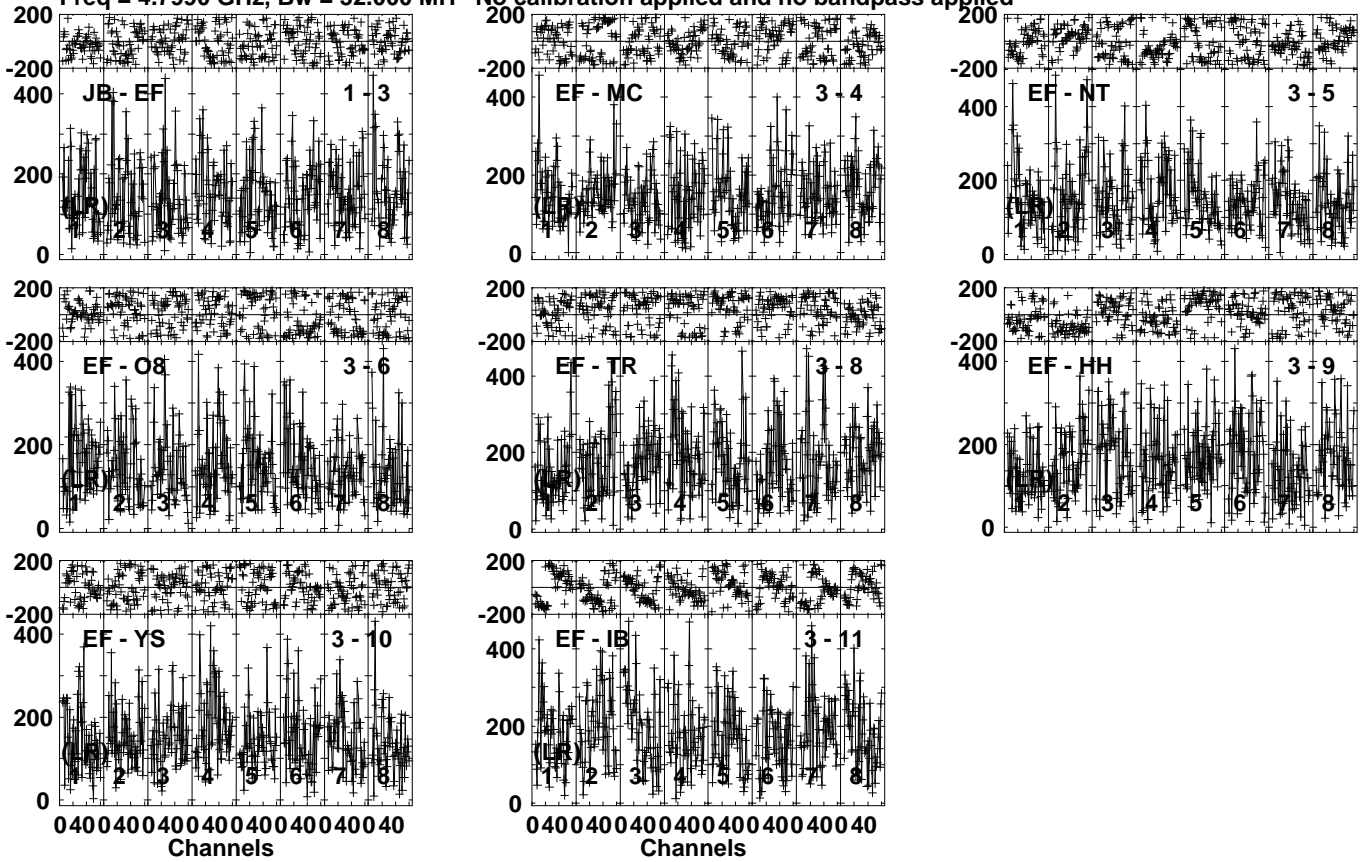
Lower frame: Micro Ampl Jy Top frame: Phas deg Vector averaged cross-power spectrum Several baselines displayed Timerange: 00/20:10:51 to 00/20:11:53
