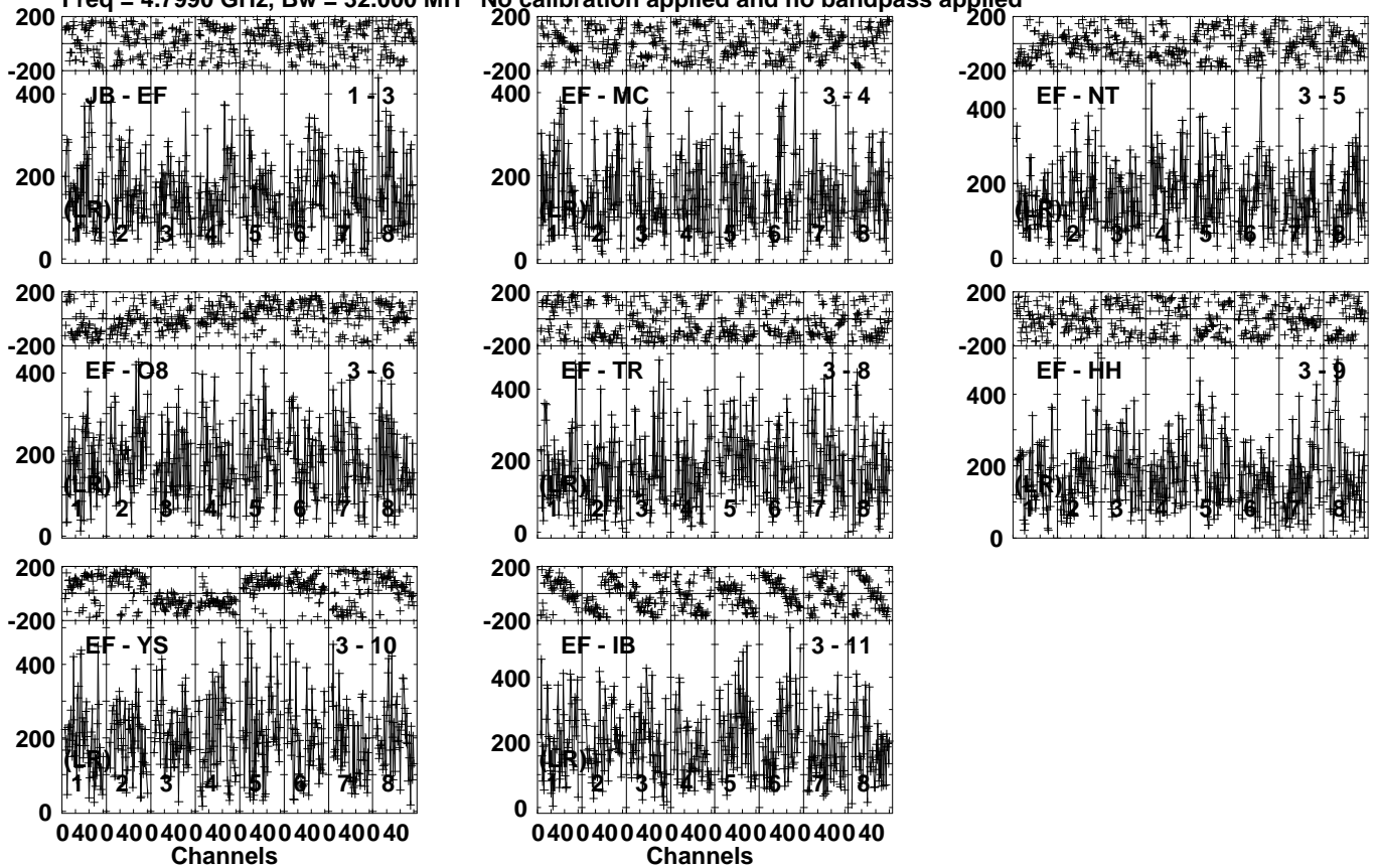
Lower frame: Micro Ampl Jy Top frame: Phas deg Vector averaged cross-power spectrum Several baselines displayed Timerange: 01/00:40:57 to 01/00:41:59
