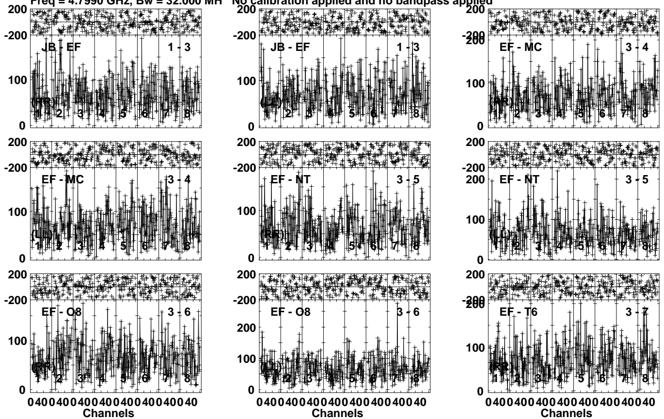
Lower frame: Micro Ampl Jy Top frame: Phas deg Vector averaged cross-power spectrum Several baselines displayed Timerange: 00/22:07:17 to 00/22:11:49
