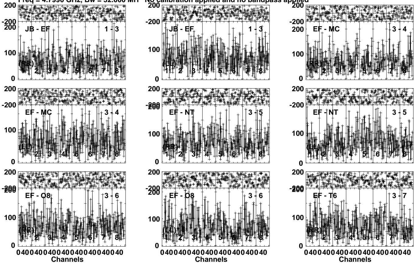
Lower frame: Micro Ampl Jy Top frame: Phas deg Vector averaged cross-power spectrum Several baselines displayed Timerange: 00/21:21:41 to 00/21:26:13
