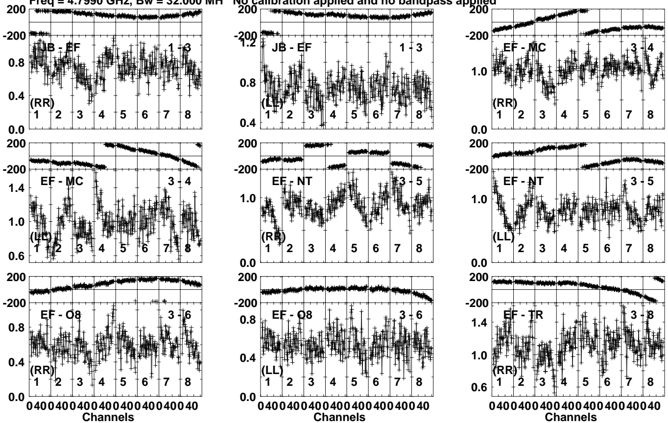
Lower frame: Milli Ampl Jy Top frame: Phas deg Vector averaged cross-power spectrum Several baselines displayed Timerange: 00/20:16:51 to 00/20:17:53
