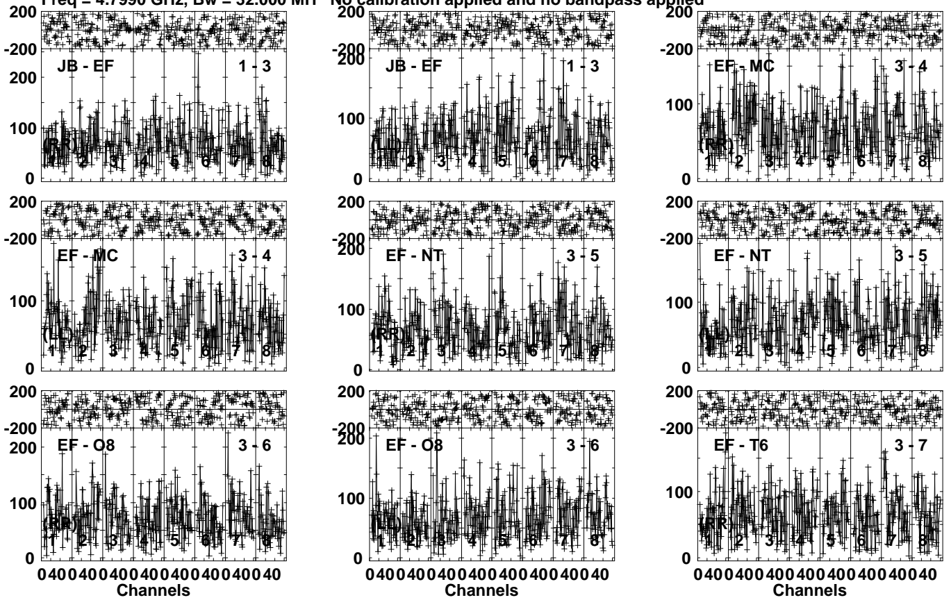
Lower frame: Micro Ampl Jy Top frame: Phas deg Vector averaged cross-power spectrum Several baselines displayed Timerange: 00/22:52:51 to 00/22:57:23
