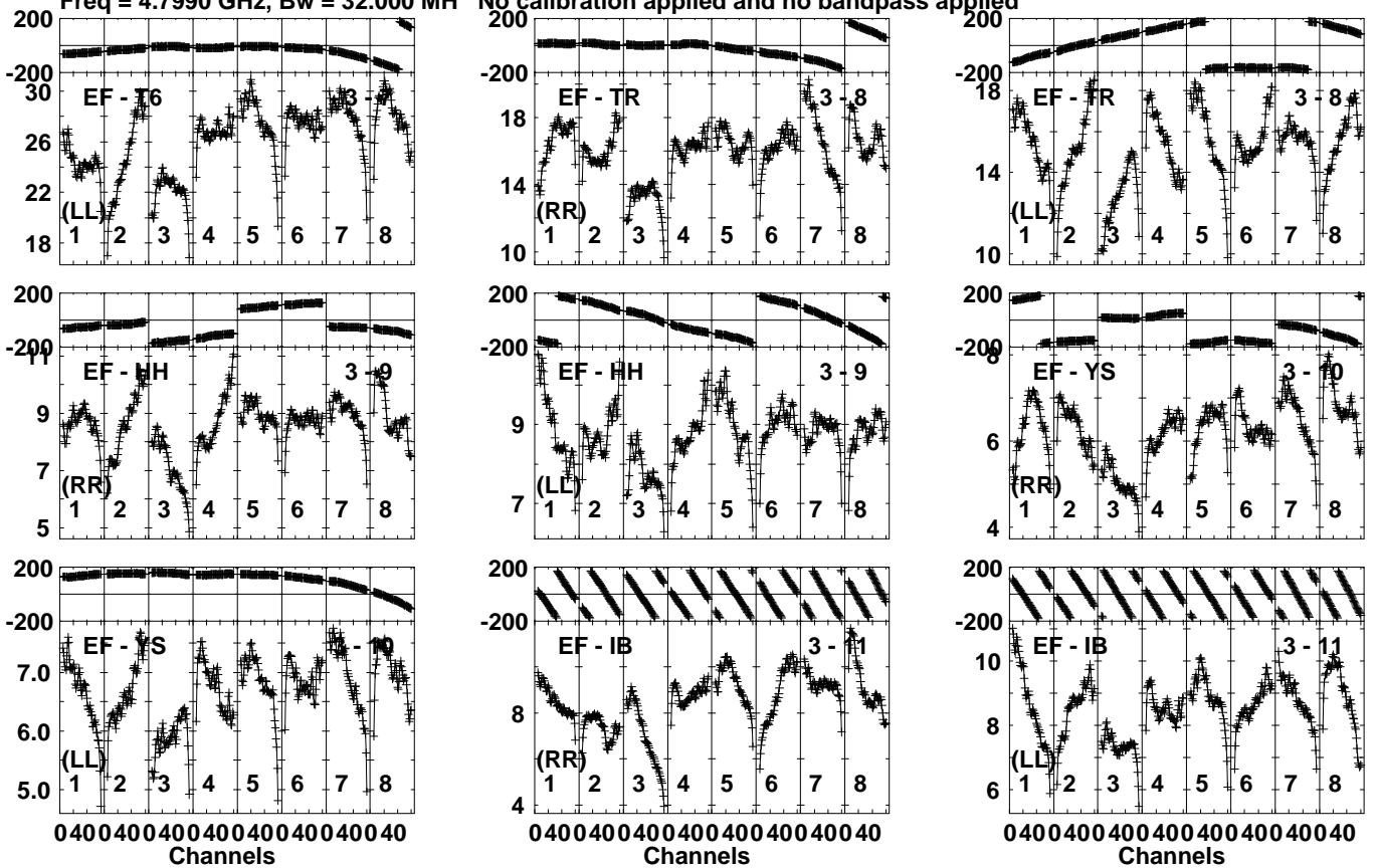
Lower frame: Milli Ampl Jy Top frame: Phas deg Vector averaged cross-power spectrum Several baselines displayed Timerange: 01/02:32:19 to 01/02:36:09
