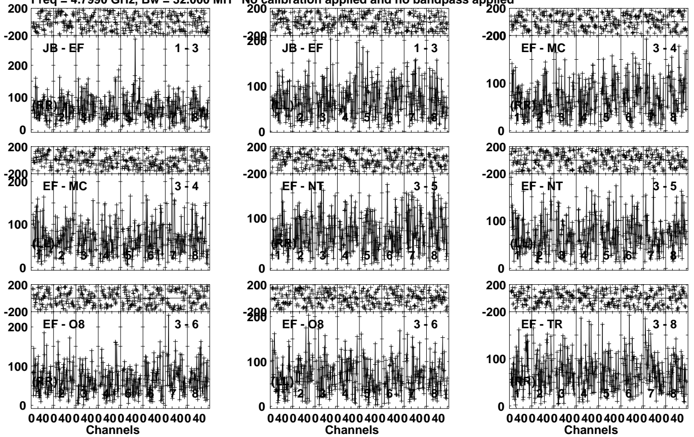
Lower frame: Micro Ampl Jy Top frame: Phas deg Vector averaged cross-power spectrum Several baselines displayed Timerange: 00/23:35:17 to 00/23:39:49
