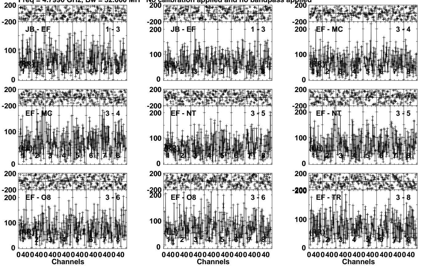
Lower frame: Micro Ampl Jy Top frame: Phas deg Vector averaged cross-power spectrum Several baselines displayed Timerange: 00/20:26:57 to 00/20:31:29
