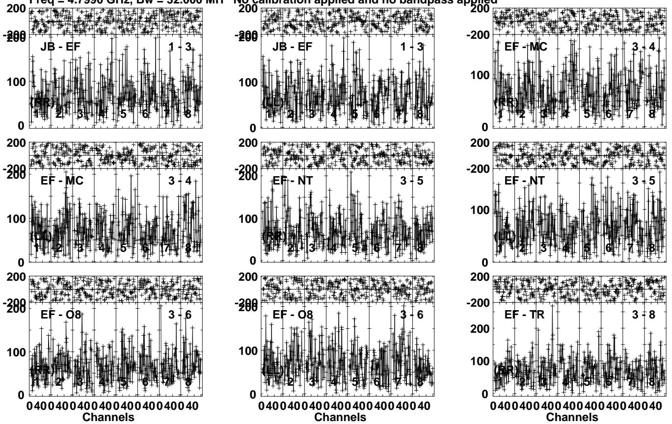
Lower frame: Micro Ampl Jy Top frame: Phas deg Vector averaged cross-power spectrum Several baselines displayed Timerange: 00/23:41:17 to 00/23:45:49
