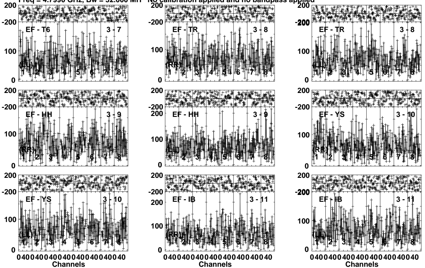
Lower frame: Micro Ampl Jy Top frame: Phas deg Vector averaged cross-power spectrum Several baselines displayed Timerange: 00/22:28:41 to 00/22:33:13
