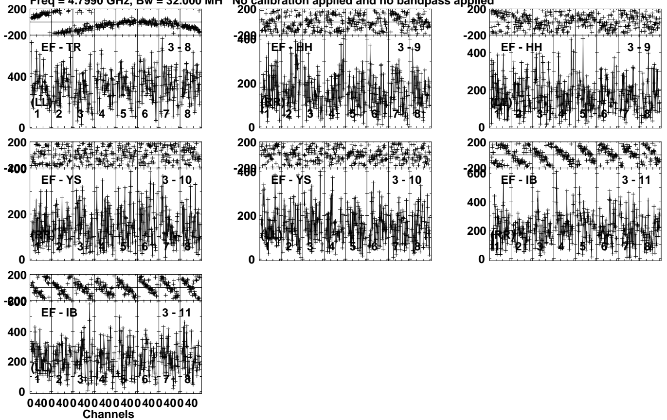
Lower frame: Micro Ampl Jy Top frame: Phas deg Vector averaged cross-power spectrum Several baselines displayed Timerange: 00/20:17:57 to 00/20:19:23
