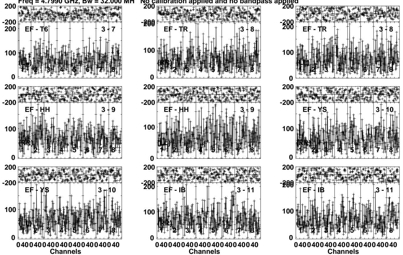
Lower frame: Micro Ampl Jy Top frame: Phas deg Vector averaged cross-power spectrum Several baselines displayed Timerange: 00/22:22:41 to 00/22:27:13
