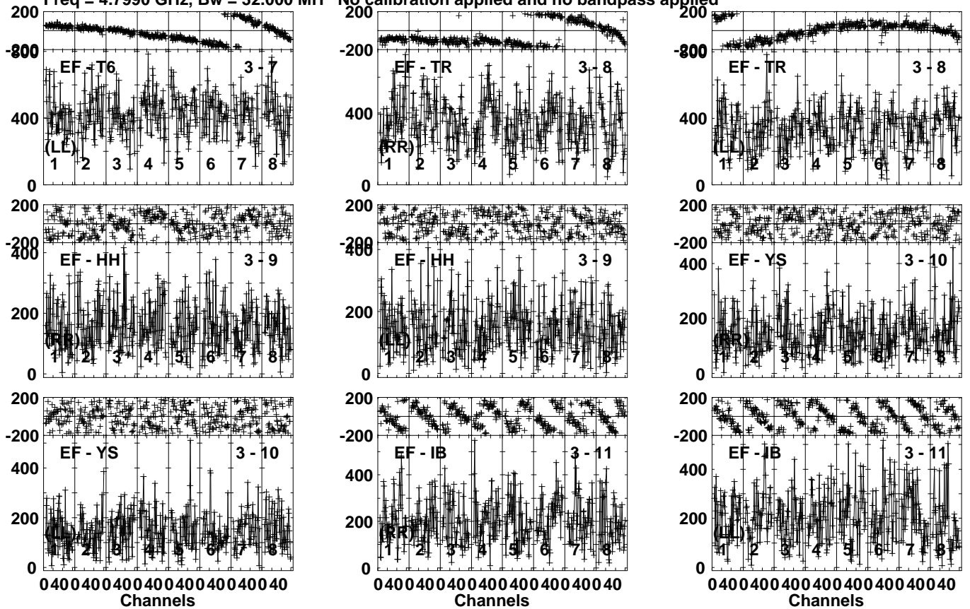
Lower frame: Micro Ampl Jy Top frame: Phas deg Vector averaged cross-power spectrum Several baselines displayed Timerange: 00/21:49:07 to 00/21:50:33
