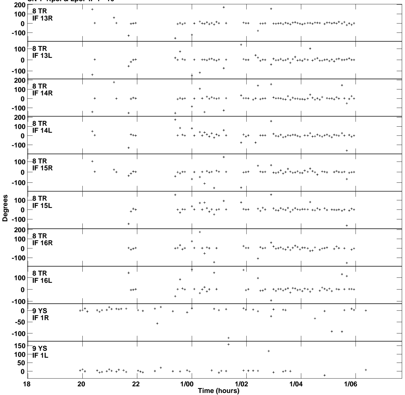
Plot file version 17 created 18-APR-2024 16:52:10 Gain phs vs UTC time for J1129+0951.MULTI.1 SN 1 Rpol & Lpol IF 1 - 16
