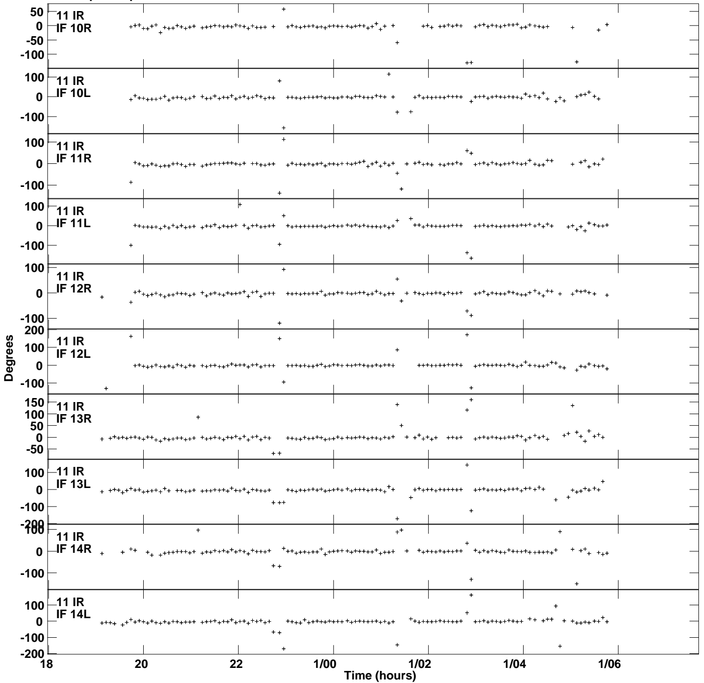
Plot file version 26 created 18-APR-2024 16:52:10 Gain phs vs UTC time for J1129+0951.MULTI.1 SN 1 Rpol & Lpol IF 1 - 16
