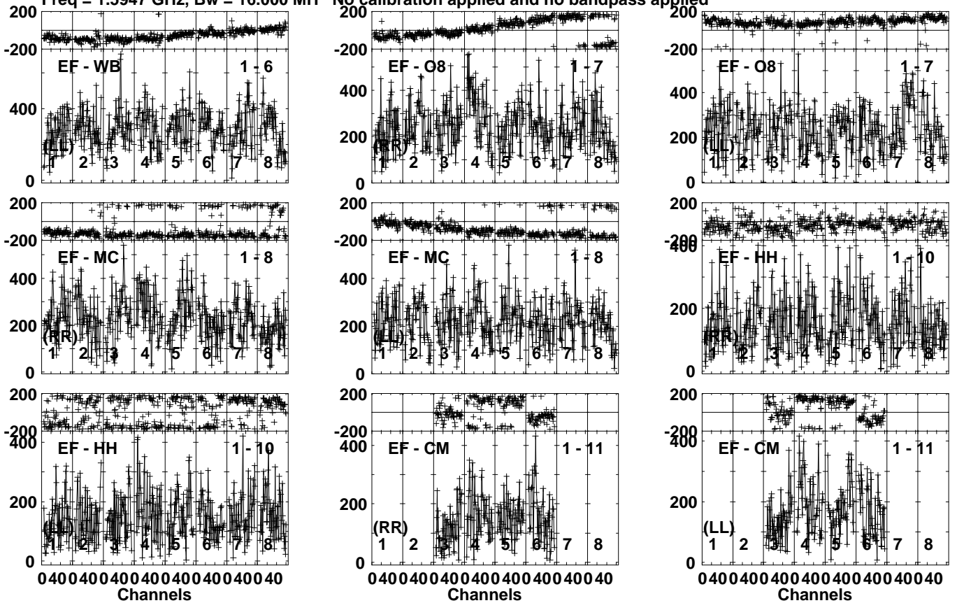
Lower frame: Micro Ampl Jy Top frame: Phas deg Vector averaged cross-power spectrum Several baselines displayed Timerange: 00/10:32:57 to 00/10:36:29
