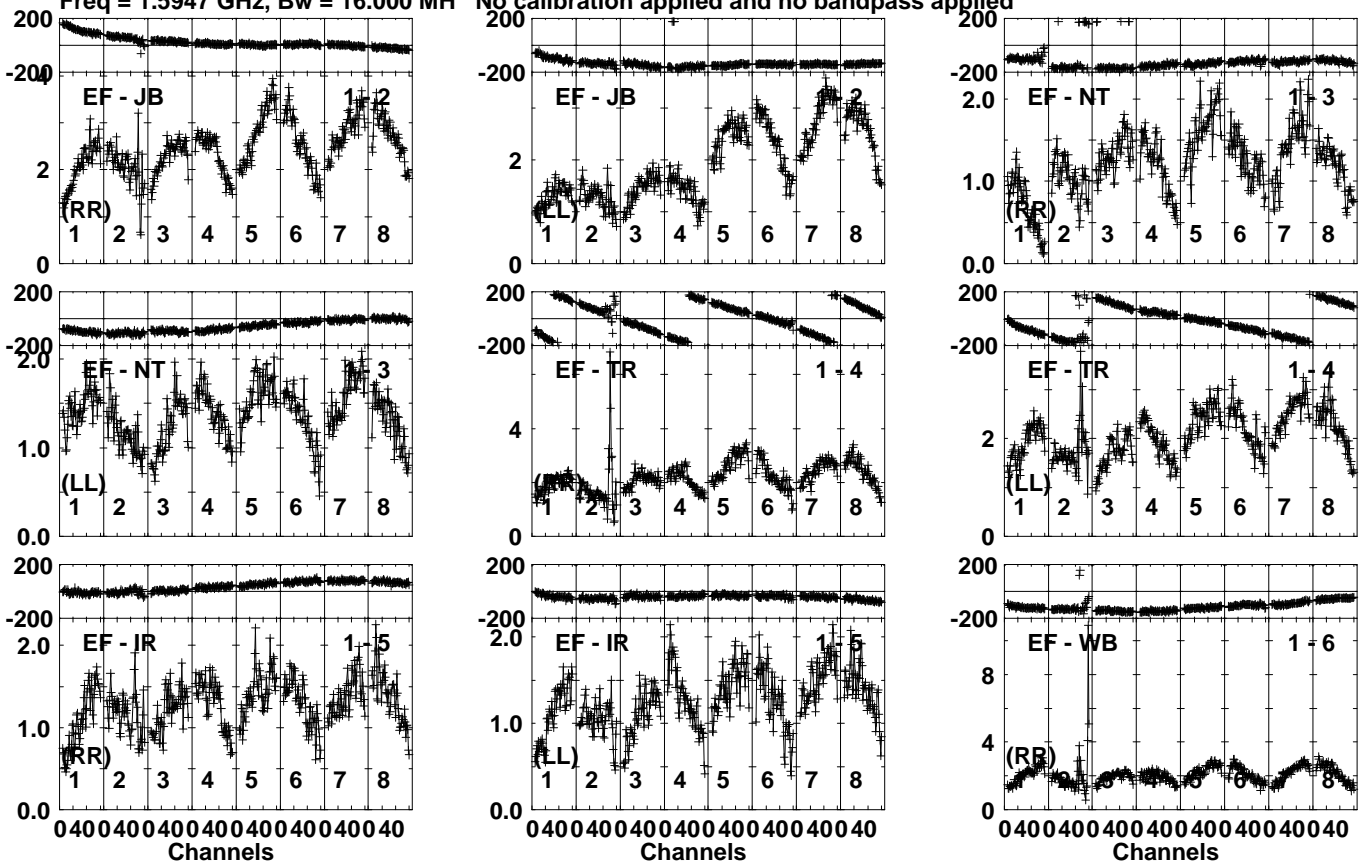
Lower frame: Milli Ampl Jy Top frame: Phas deg Vector averaged cross-power spectrum Several baselines displayed Timerange: 00/14:27:37 to 00/14:28:53
