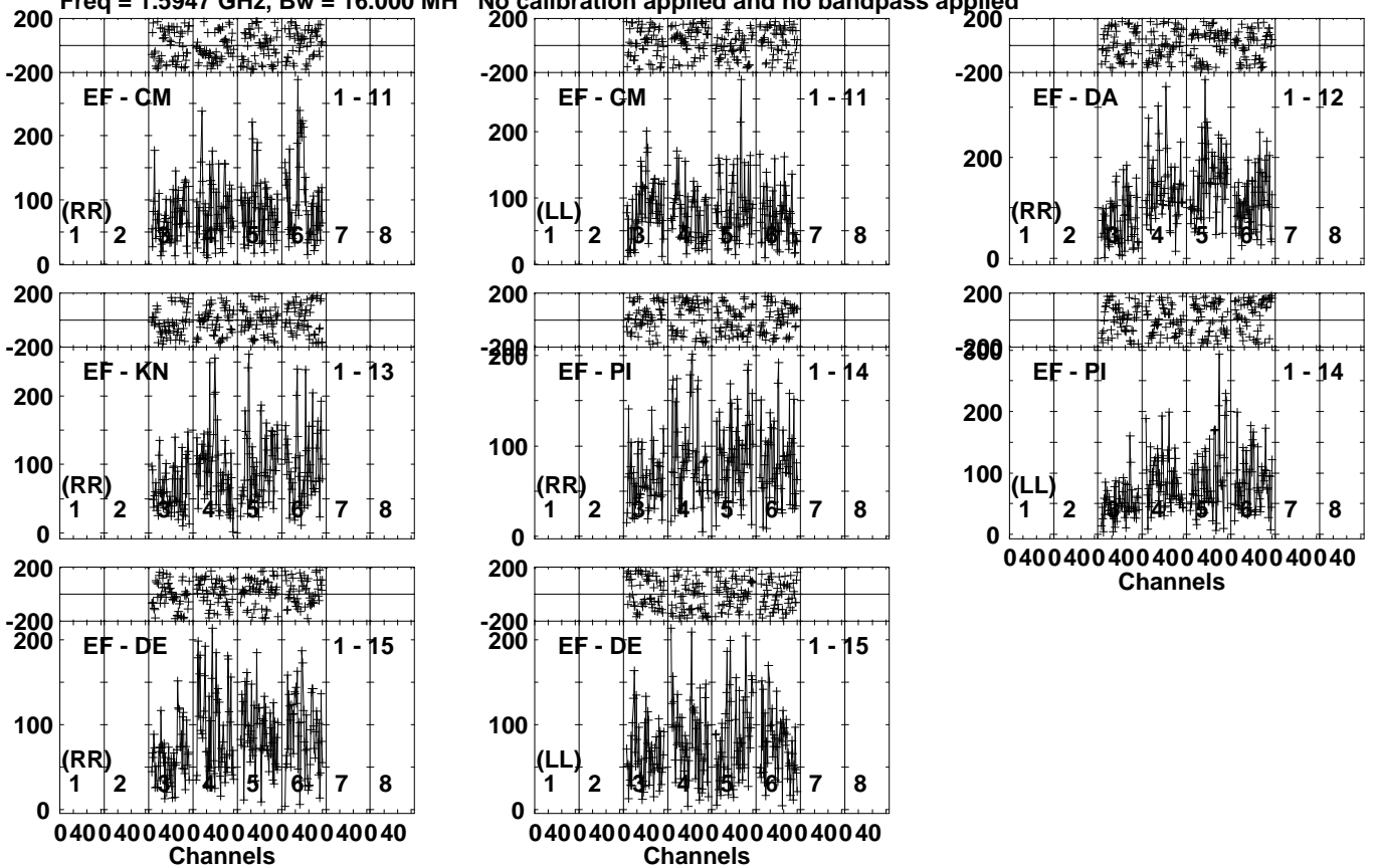
Lower frame: Micro Ampl Jy Top frame: Phas deg Vector averaged cross-power spectrum Several baselines displayed Timerange: 00/07:52:13 to 00/07:58:09
