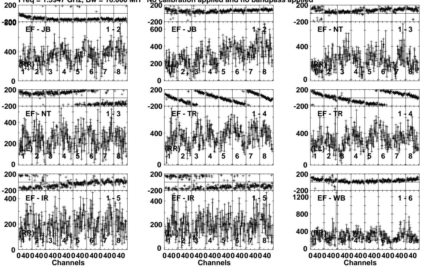
Lower frame: Micro Ampl Jy Top frame: Phas deg Vector averaged cross-power spectrum Several baselines displayed Timerange: 00/12:51:57 to 00/12:55:29
