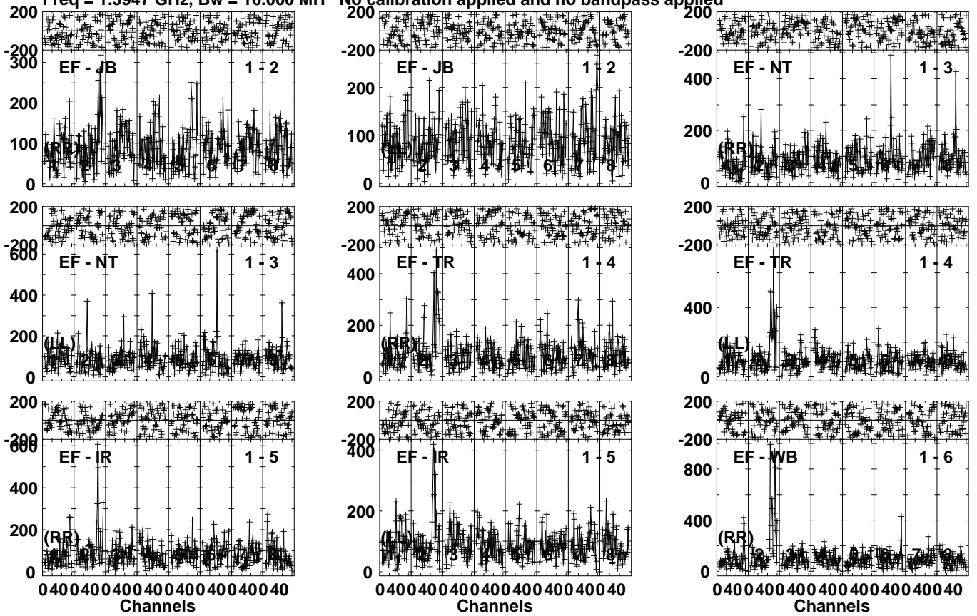
Lower frame: Micro Ampl Jy Top frame: Phas deg Vector averaged cross-power spectrum Several baselines displayed Timerange: 00/12:22:17 to 00/12:28:13
