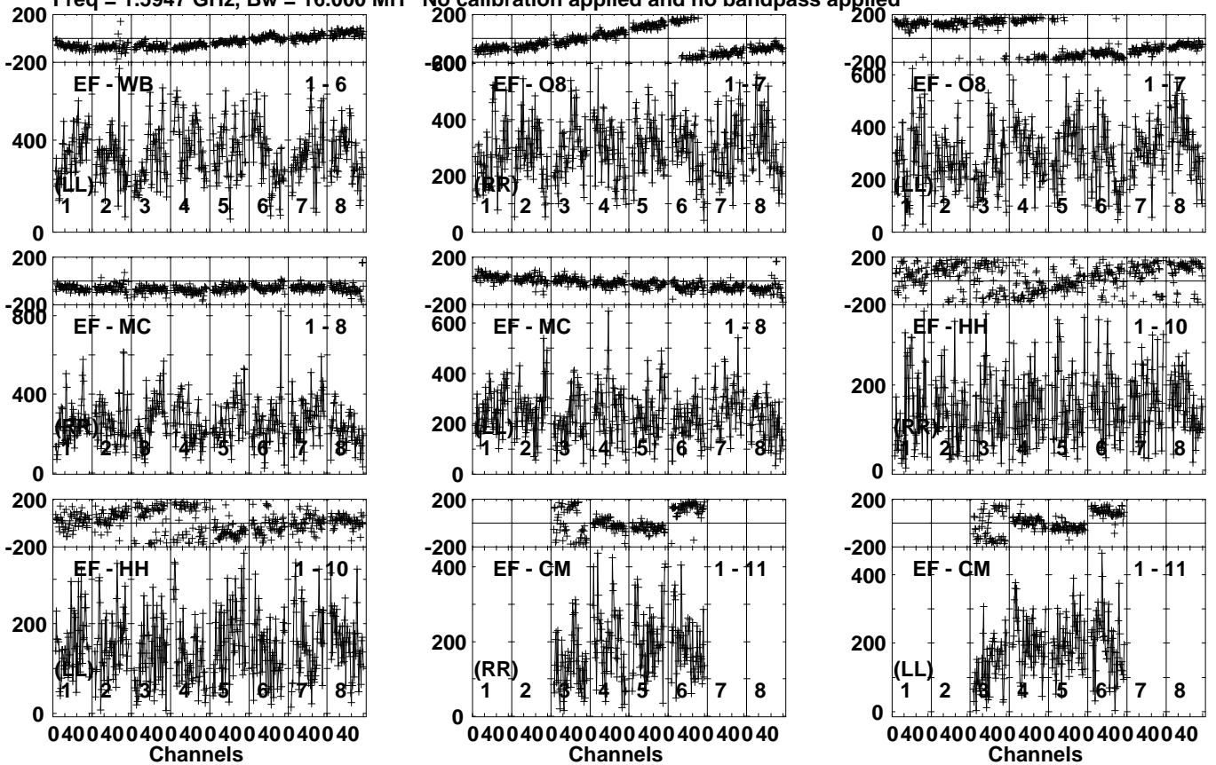
Lower frame: Micro Ampl Jy Top frame: Phas deg Vector averaged cross-power spectrum Several baselines displayed Timerange: 00/13:26:50 to 00/13:30:22
