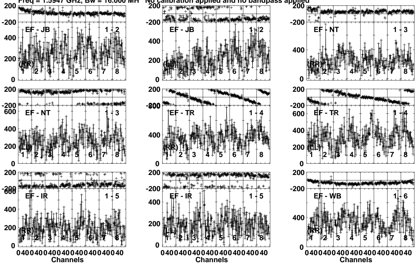
Lower frame: Micro Ampl Jy Top frame: Phas deg Vector averaged cross-power spectrum Several baselines displayed Timerange: 00:12:17:15 to 00:12:20:45
