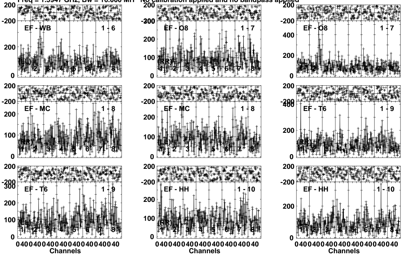
Lower frame: Micro Ampl Jy Top frame: Phas deg Vector averaged cross-power spectrum Several baselines displayed Timerange: 00/08:34:19 to 00/08:40:13
