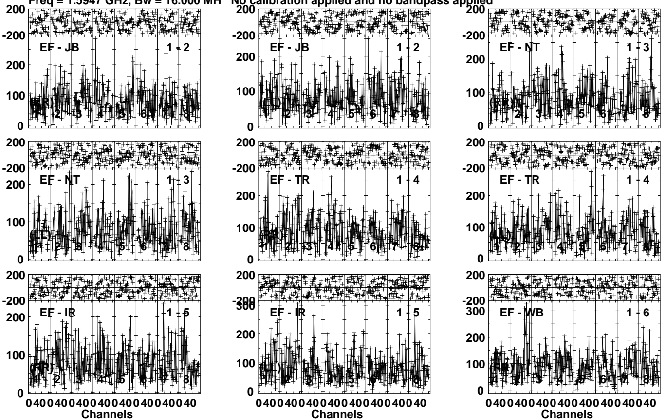
Lower frame: Micro Ampl Jy Top frame: Phas deg Vector averaged cross-power spectrum Several baselines displayed Timerange: 00/10:10:55 to 00/10:16:49
