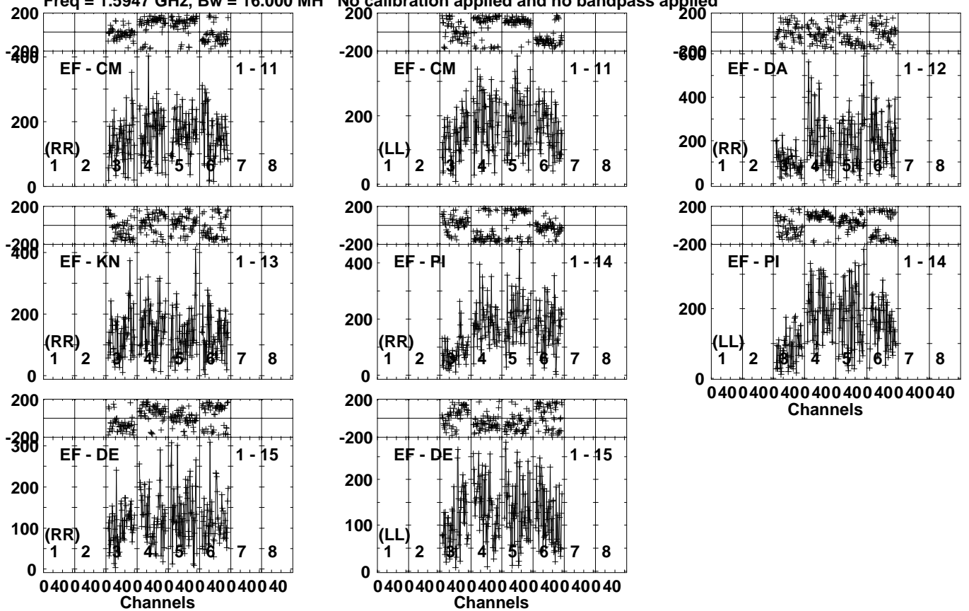
Lower frame: Micro Ampl Jy Top frame: Phas deg Vector averaged cross-power spectrum Several baselines displayed Timerange: 00/09:23:40 to 00/09:27:12
