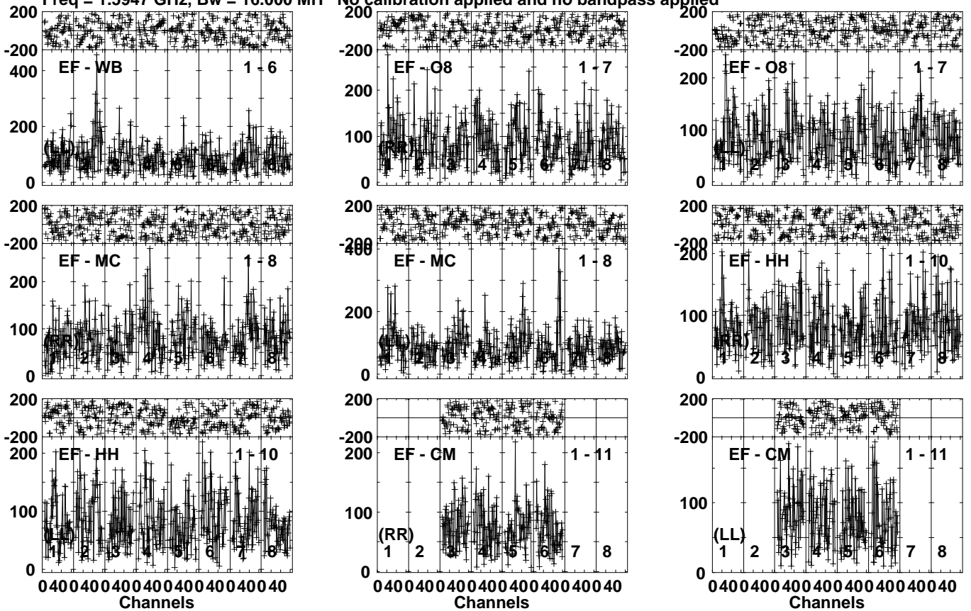
Lower frame: Micro Ampl Jy Top frame: Phas deg Vector averaged cross-power spectrum Several baselines displayed Timerange: 00/10:38:11 to 00/10:44:07
