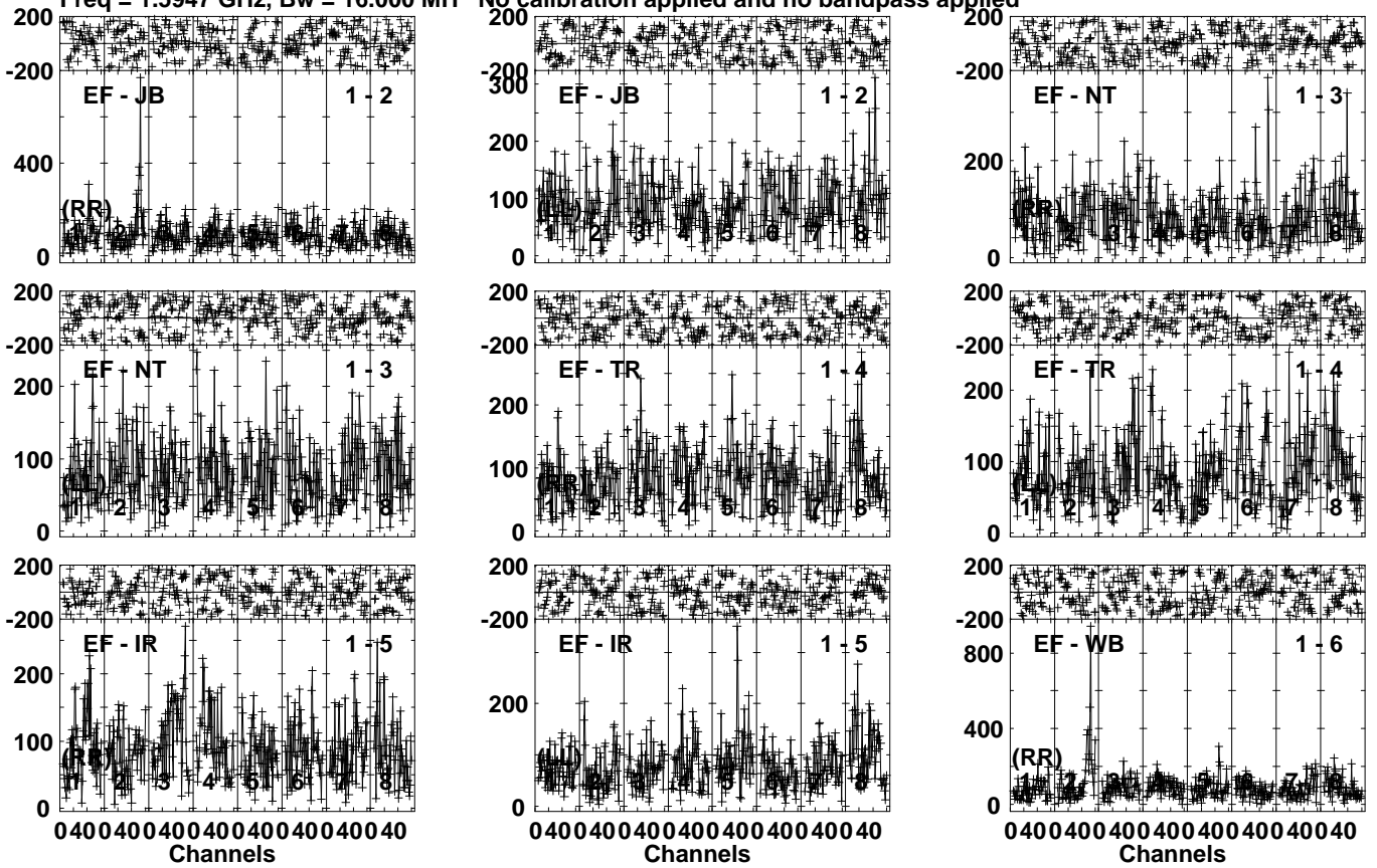
Lower frame: Micro Ampl Jy Top frame: Phas deg Vector averaged cross-power spectrum Several baselines displayed Timerange: 00/07:17:29 to 00/07:23:23
