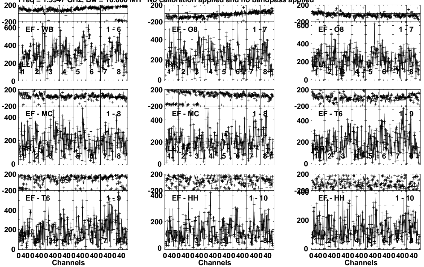
Lower frame: Micro Ampl Jy Top frame: Phas deg Vector averaged cross-power spectrum Several baselines displayed Timerange: 00/08:14:20 to 00/08:17:50
