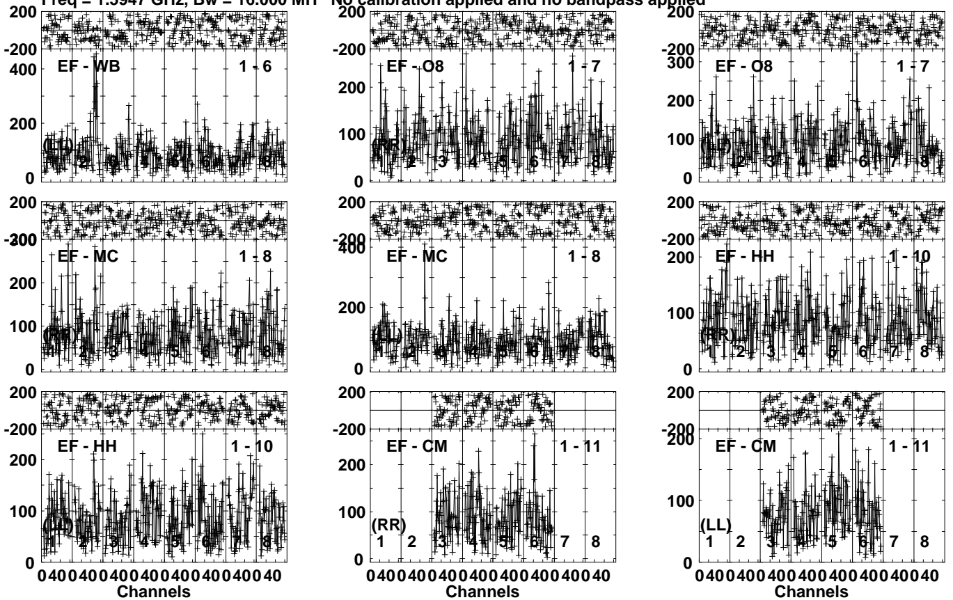
Lower frame: Micro Ampl Jy Top frame: Phas deg Vector averaged cross-power spectrum Several baselines displayed Timerange: 00/11:20:17 to 00/11:26:11
