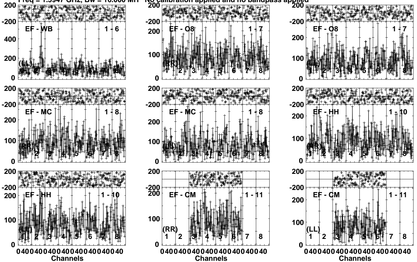
Lower frame: Micro Ampl Jy Top frame: Phas deg Vector averaged cross-power spectrum Several baselines displayed Timerange: 00/13:31:56 to 00/13:37:50
