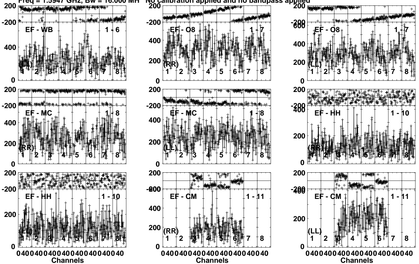
Lower frame: Micro Ampl Jy Top frame: Phas deg Vector averaged cross-power spectrum Several baselines displayed Timerange: 00/14:01:34 to 00/14:05:06
