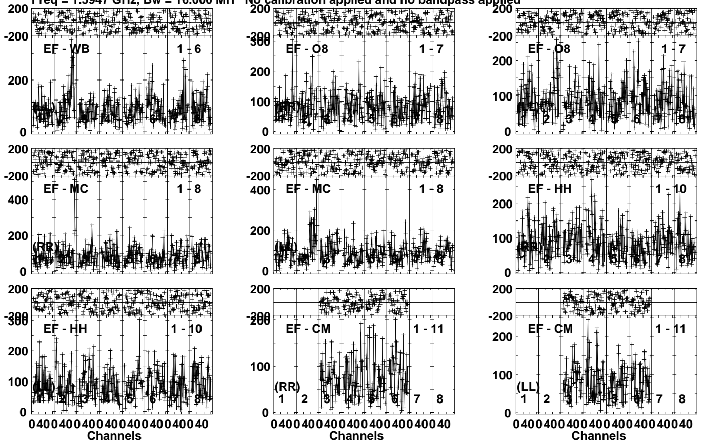
Lower frame: Micro Ampl Jy Top frame: Phas deg Vector averaged cross-power spectrum Several baselines displayed Timerange: 00/13:19:21 to 00/13:25:15
