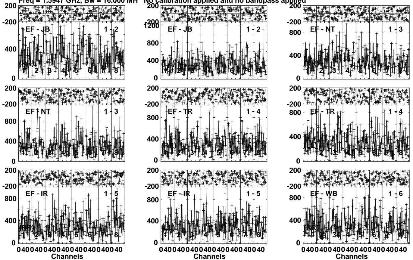
Lower frame: Micro Ampl Jy Top frame: Phas deg Vector averaged cross-power spectrum Several baselines displayed Timerange: 00/15:49:09 to 00/15:50:21
