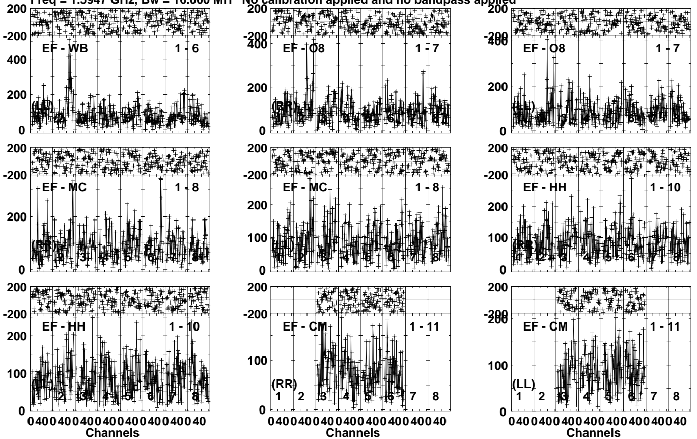
Lower frame: Micro Ampl Jy Top frame: Phas deg Vector averaged cross-power spectrum Several baselines displayed Timerange: 00/14:28:57 to 00/14:34:53
