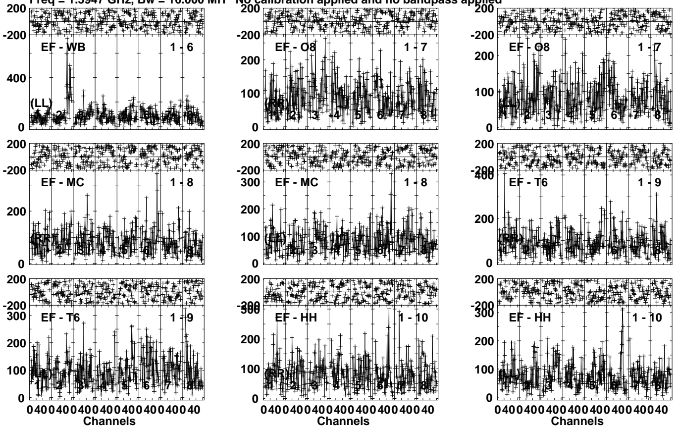
Lower frame: Micro Ampl Jy Top frame: Phas deg Vector averaged cross-power spectrum Several baselines displayed Timerange: 00/07:44:46 to 00/07:50:42
