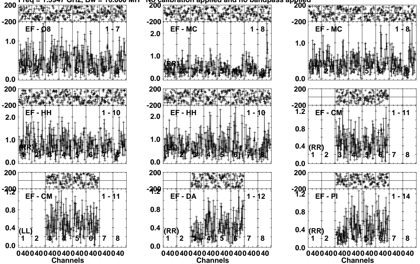
Lower frame: Milli Ampl Jy Top frame: Phas deg Vector averaged cross-power spectrum Several baselines displayed Timerange: 00/15:34:42 to 00/15:35:54
