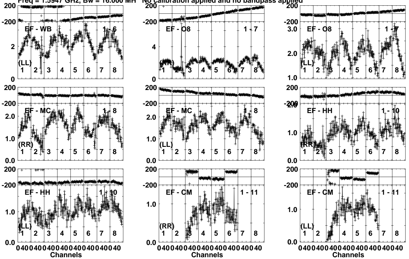
Lower frame: Milli Ampl Jy Top frame: Phas deg Vector averaged cross-power spectrum Several baselines displayed Timerange: 00/10:10:01 to 00/10:10:49
