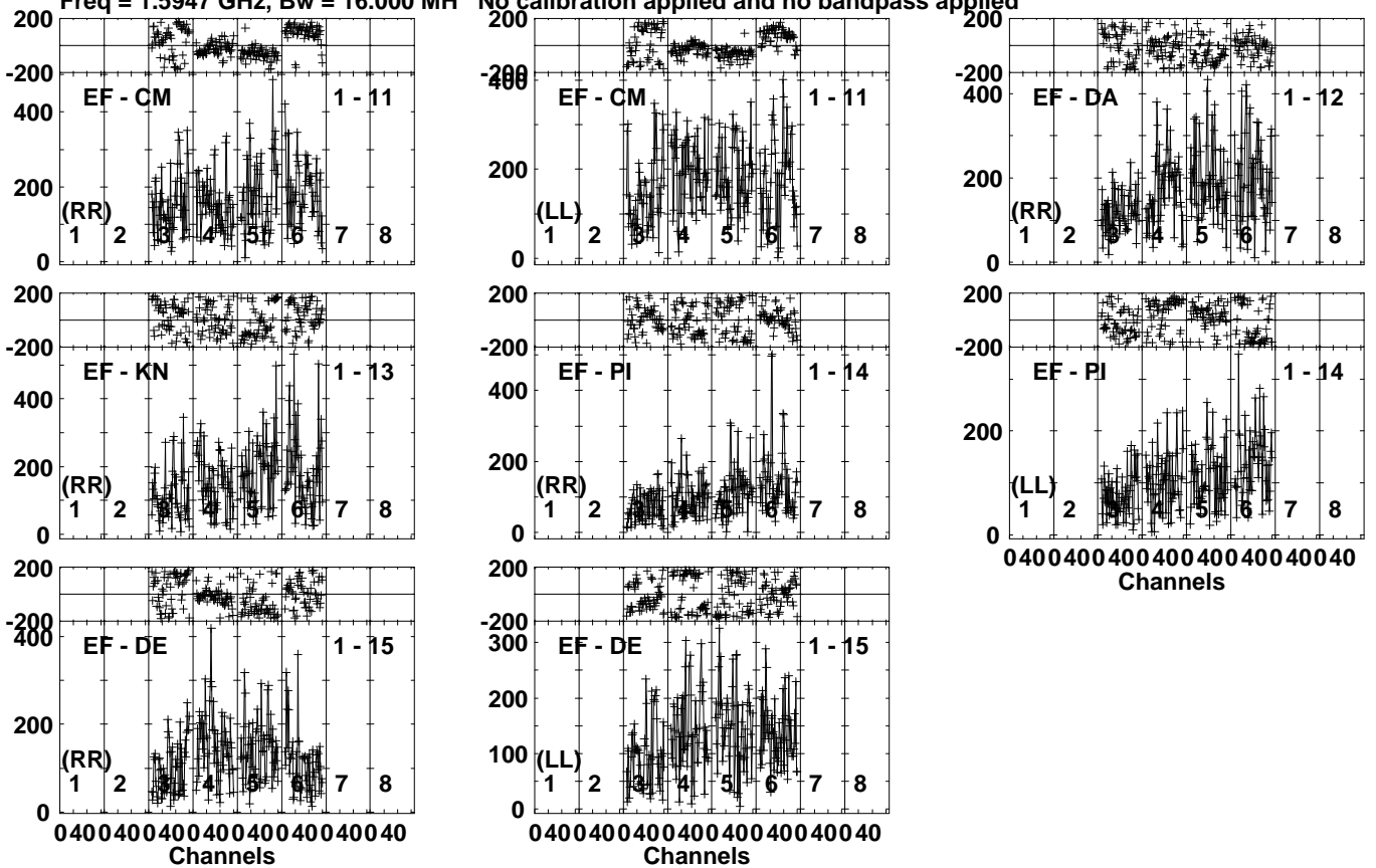
Lower frame: Micro Ampl Jy Top frame: Phas deg Vector averaged cross-power spectrum Several baselines displayed Timerange: 00/08:49:04 to 00/08:52:36
