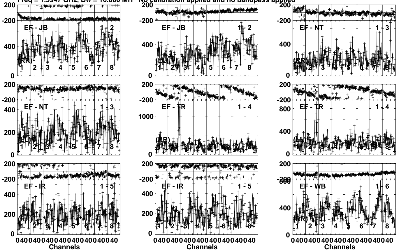
Lower frame: Micro Ampl Jy Top frame: Phas deg Vector averaged cross-power spectrum Several baselines displayed Timerange: 00/11:42:26 to 00/11:45:54
