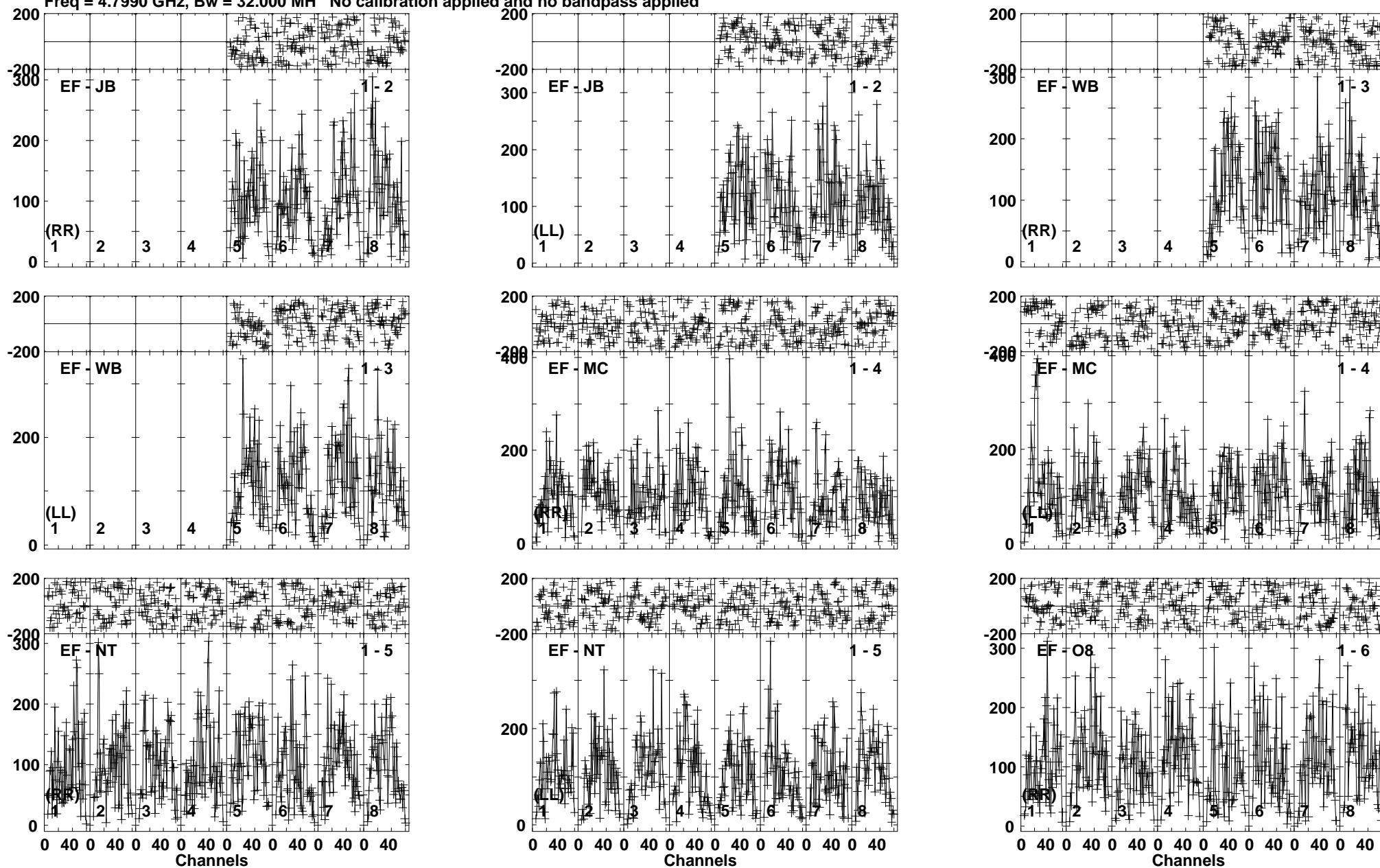
Lower frame: Micro Ampl Jy Top frame: Phas deg Vector averaged cross-power spectrum Baseline: EF (01) - JB (02) Timerange: 00/23:15:01 to 00/23:17:29
