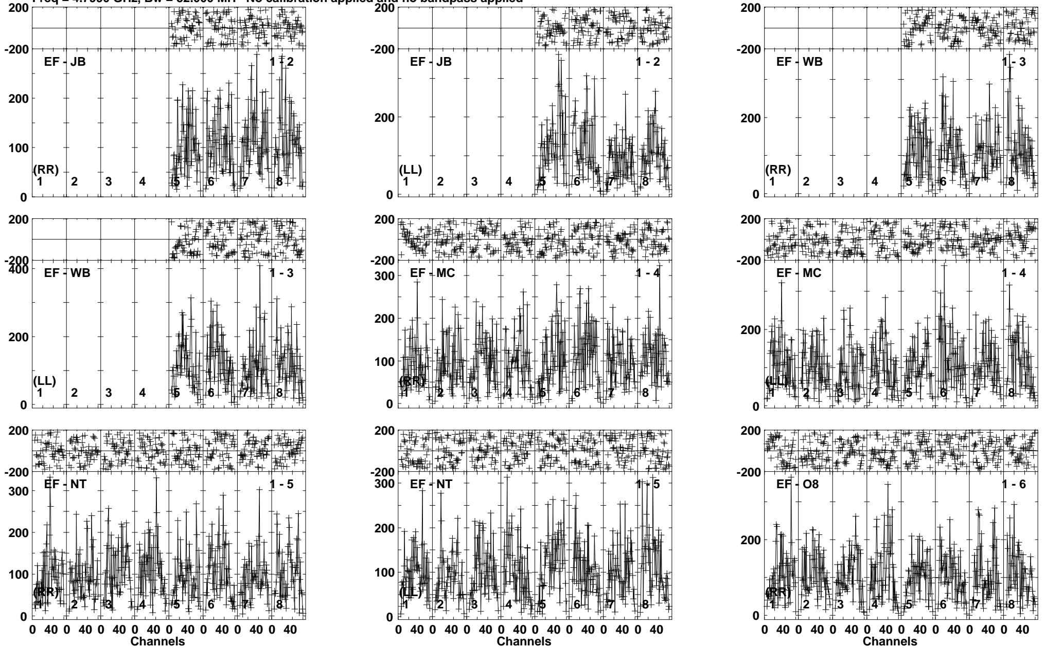
Lower frame: Micro Ampl Jy Top frame: Phas deg Vector averaged cross-power spectrum Baseline: EF (01) - JB (02) Timerange: 00/19:43:01 to 00/19:45:29
