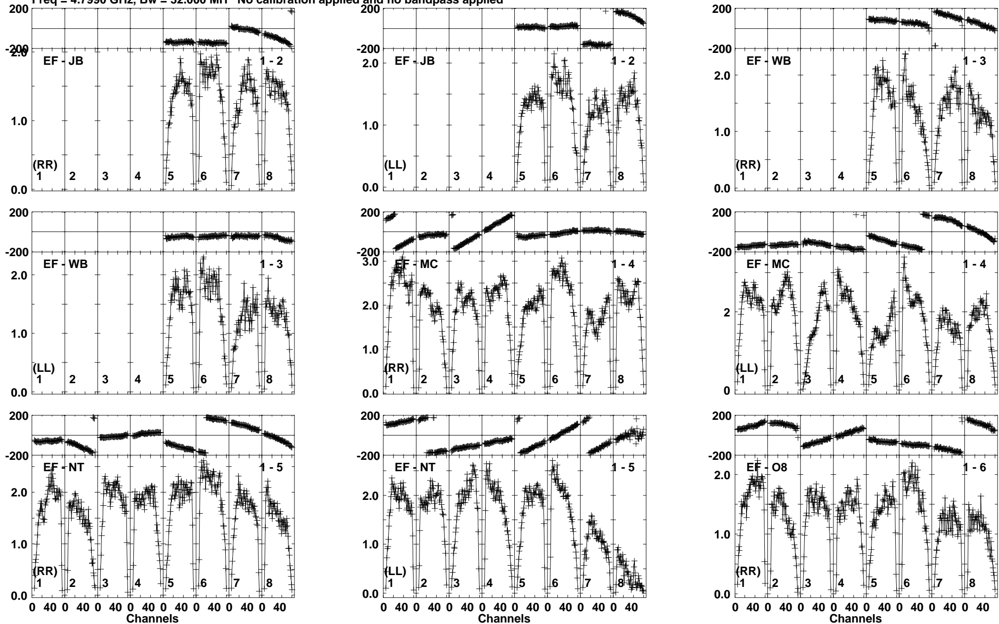
Lower frame: Milli Ampl Jy Top frame: Phas deg Vector averaged cross-power spectrum Baseline: EF (01) - JB (02) Timerange: 00/19:01:31 to 00/19:02:59
