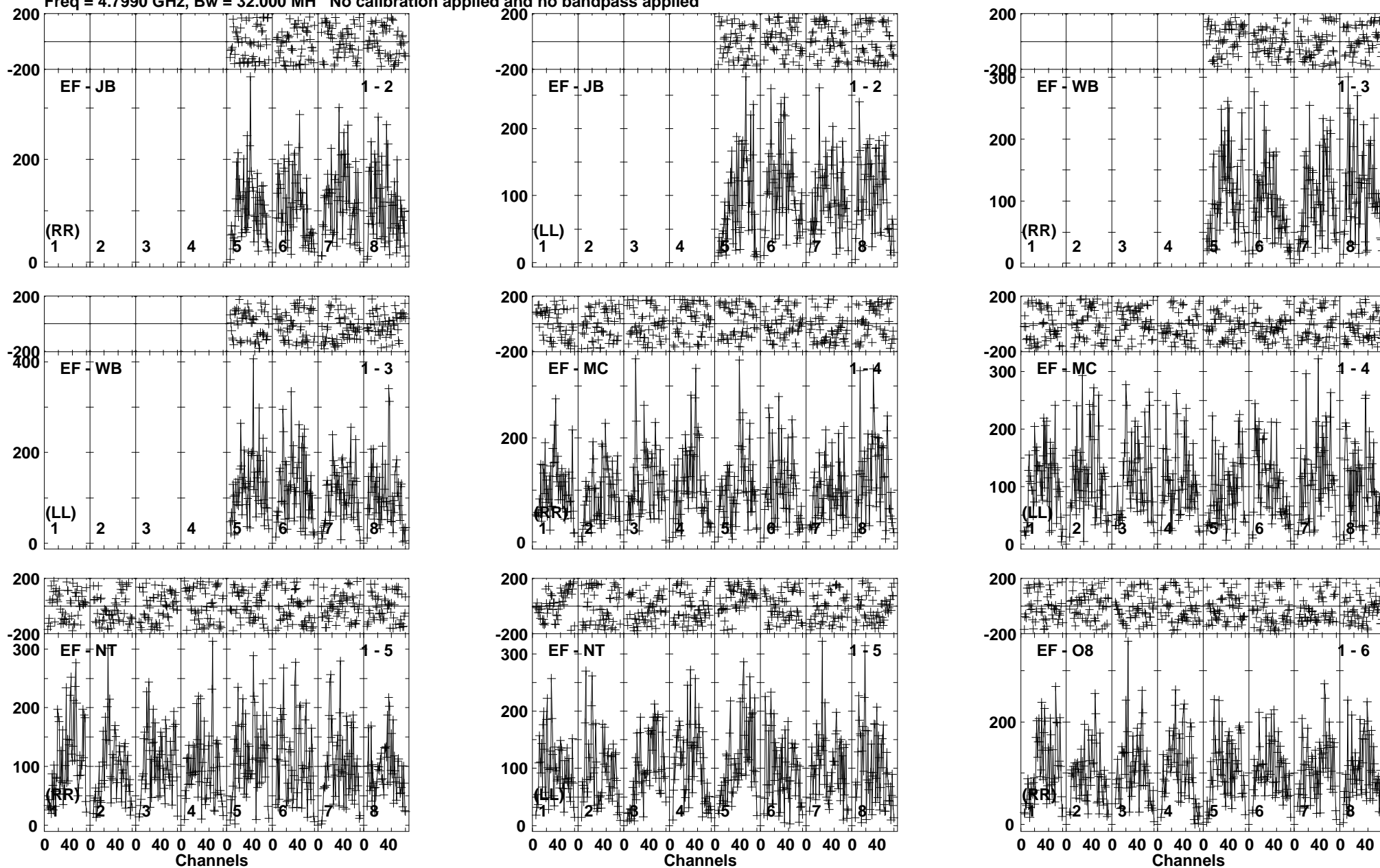
Lower frame: Micro Ampl Jy Top frame: Phas deg Vector averaged cross-power spectrum Baseline: EF (01) - JB (02) Timerange: 00/19:55:01 to 00/19:57:29
