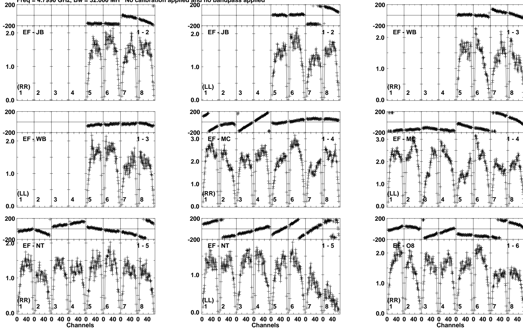
Lower frame: Milli Ampl Jy Top frame: Phas deg Vector averaged cross-power spectrum Baseline: EF (01) - JB (02) Timerange: 00:22:10:01 to 00:22:10:59
