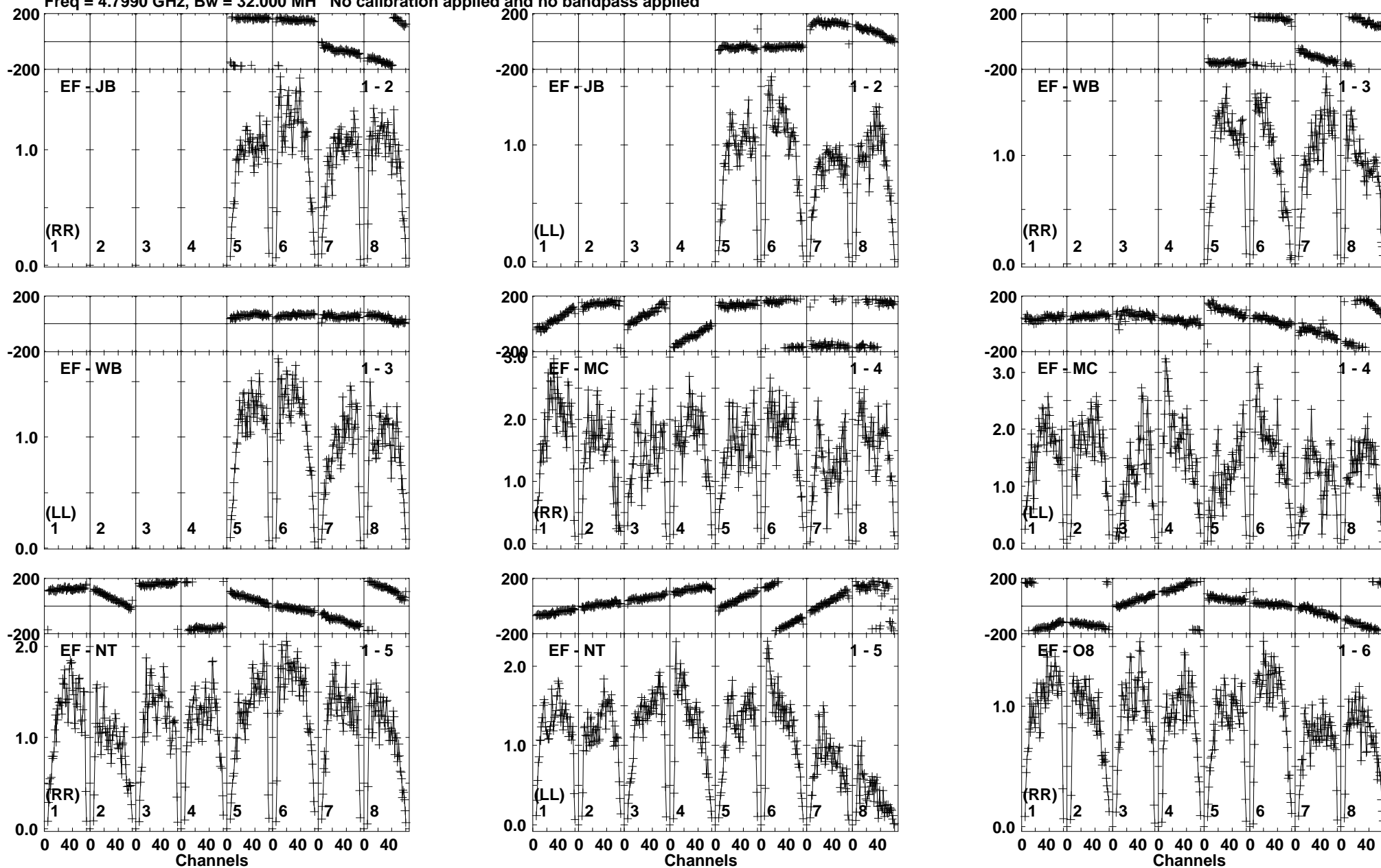
Lower frame: Milli Ampl Jy Top frame: Phas deg Vector averaged cross-power spectrum Baseline: EF (01) - JB (02) Timerange: 00/18:10:02 to 00/18:10:58
