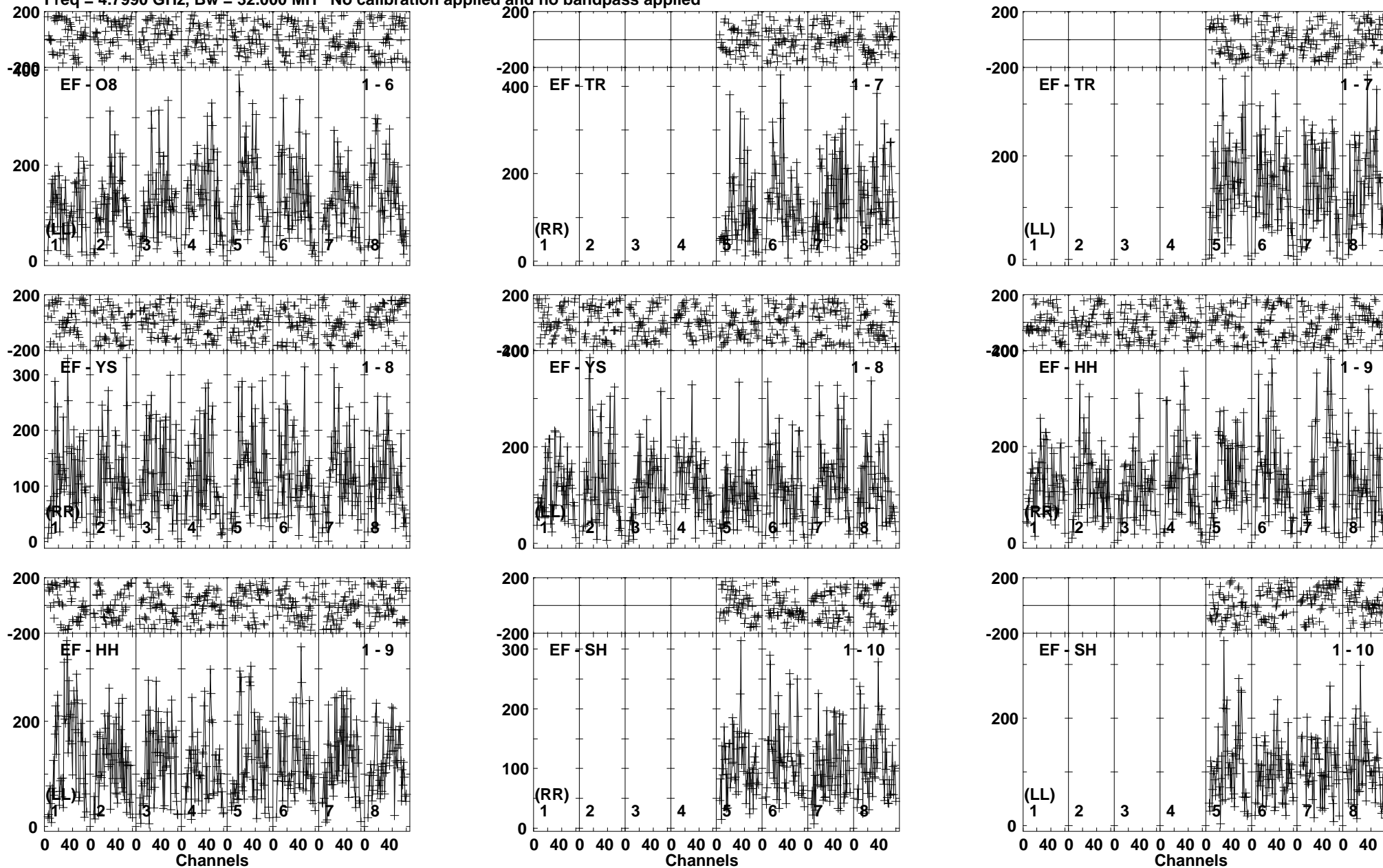
Lower frame: Micro Ampl Jy Top frame: Phas deg Vector averaged cross-power spectrum Baseline: EF (01) - O8 (06) Timerange: 00/18:11:02 to 00/18:13:18
