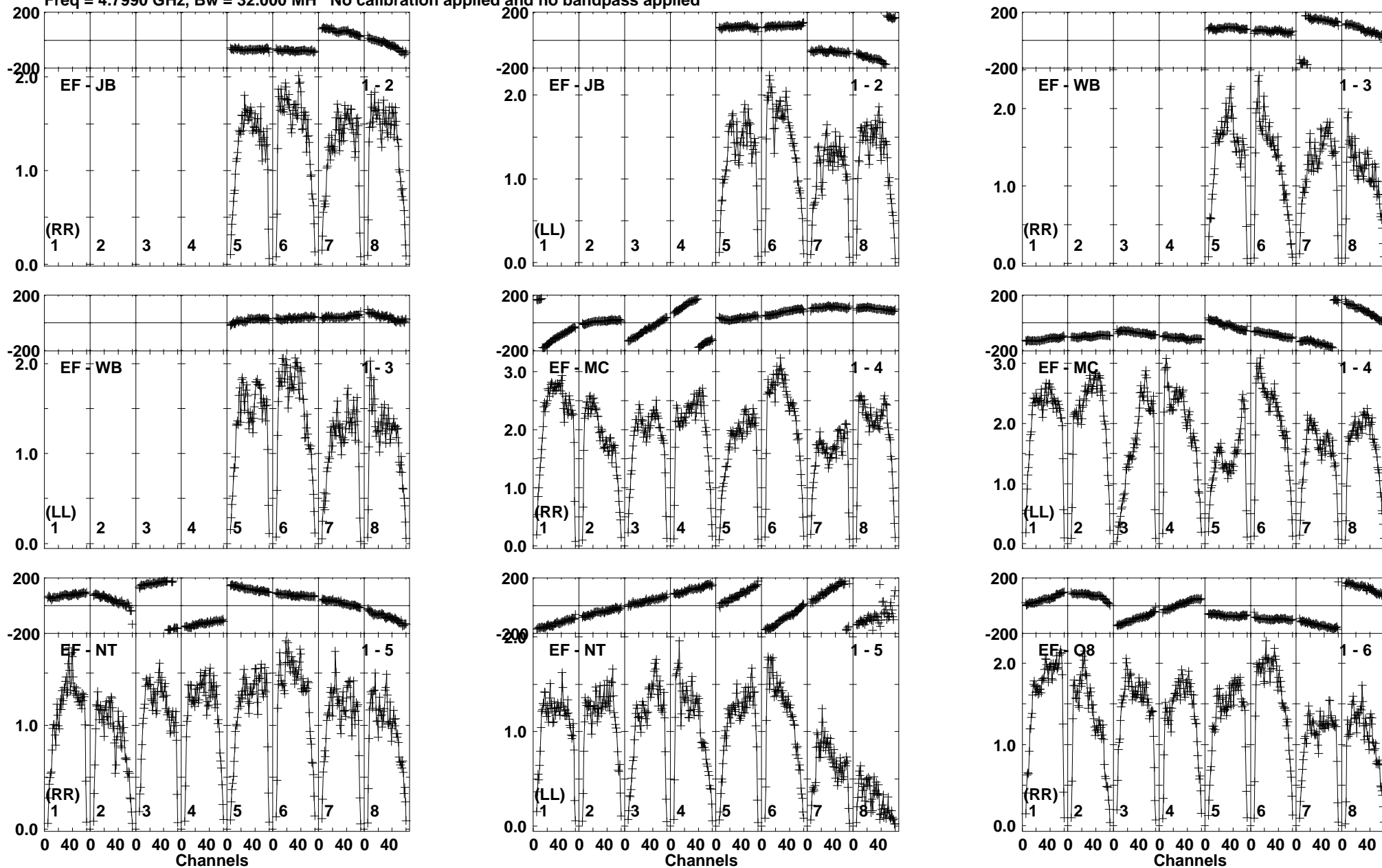
Lower frame: Milli Ampl Jy Top frame: Phas deg Vector averaged cross-power spectrum Baseline: EF (01) - JB (02) Timerange: 00/22:13:31 to 00/22:14:59
