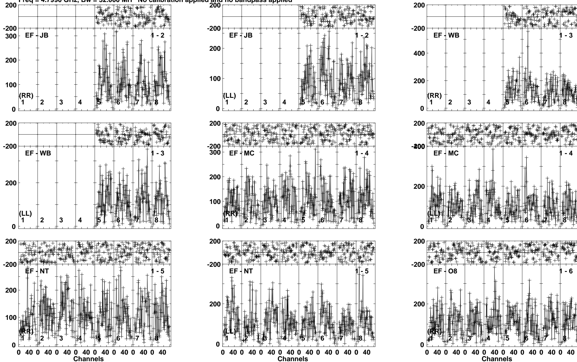
Lower frame: Micro Ampl Jy Top frame: Phas deg Vector averaged cross-power spectrum Baseline: EF (01) - JB (02) Timerange: 00/23:23:01 to 00/23:25:29
