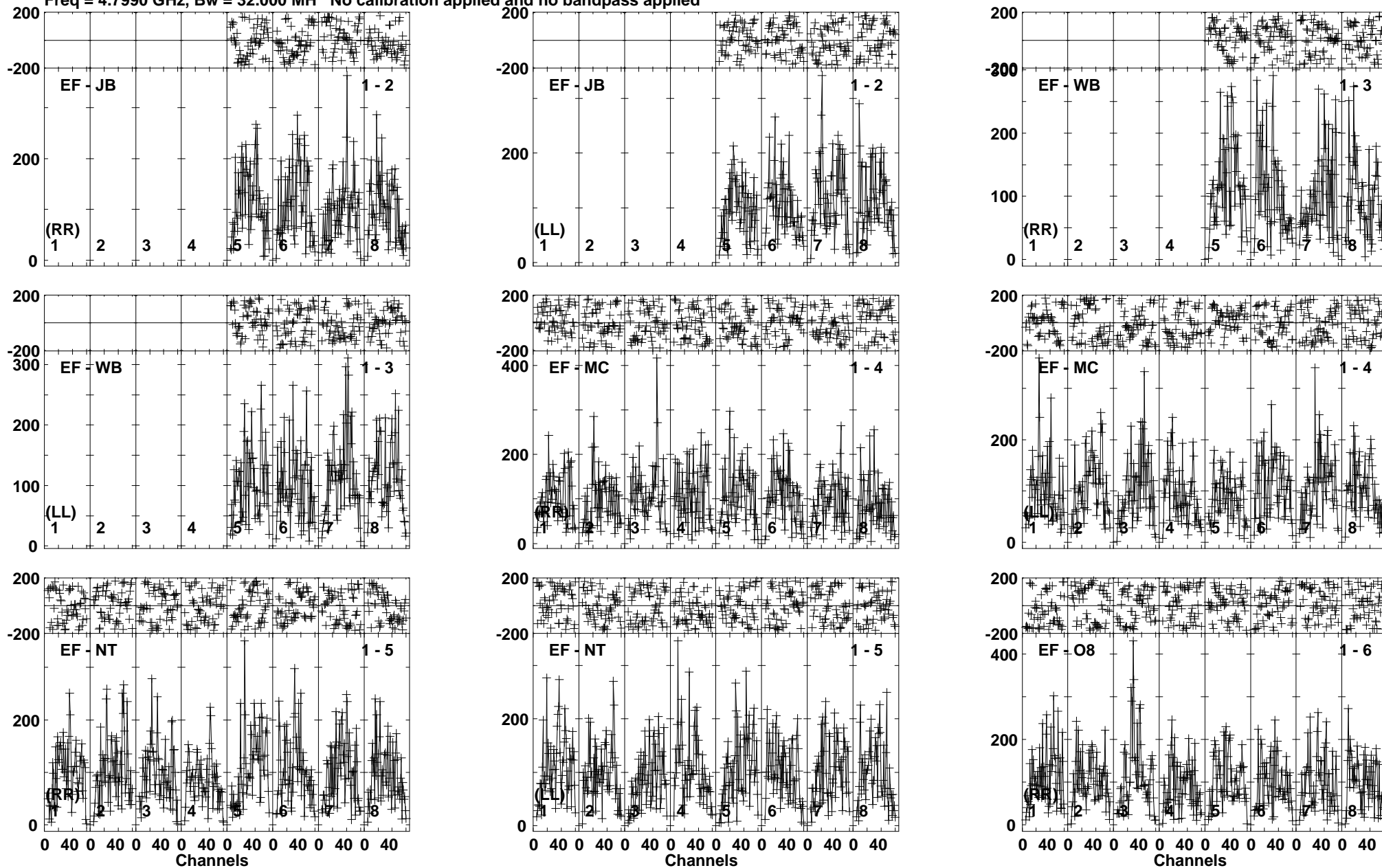
Lower frame: Micro Ampl Jy Top frame: Phas deg Vector averaged cross-power spectrum Baseline: EF (01) - JB (02) Timerange: 00/20:31:01 to 00/20:33:29
