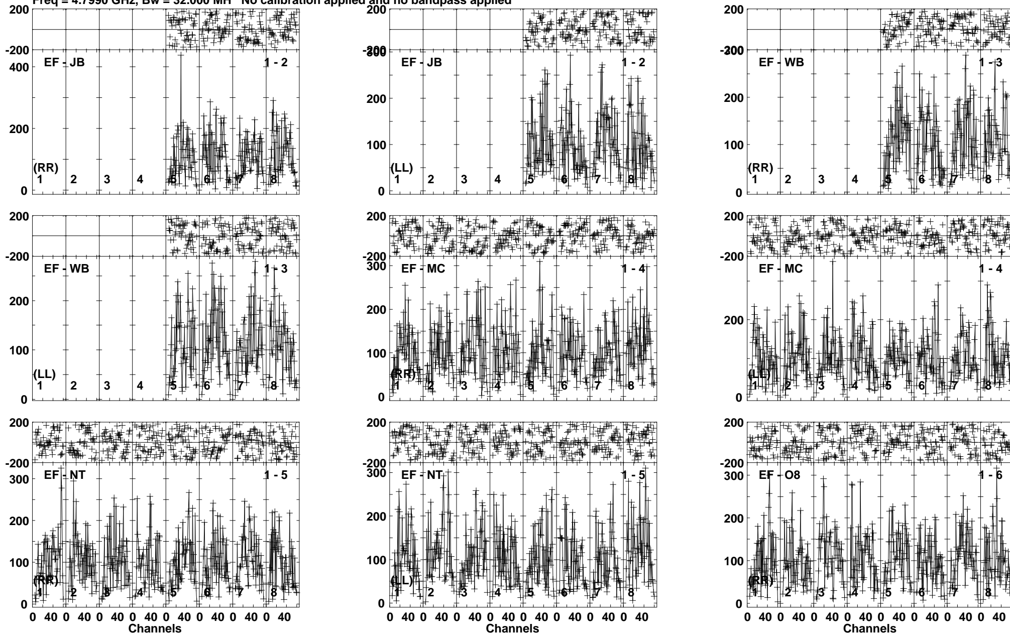
Lower frame: Micro Ampl Jy Top frame: Phas deg Vector averaged cross-power spectrum Baseline: EF (01) - JB (02) Timerange: 00/19:07:01 to 00/19:09:29
