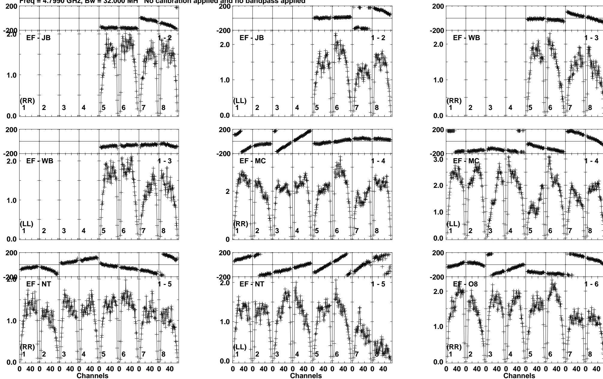
Lower frame: Milli Ampl Jy Top frame: Phas deg Vector averaged cross-power spectrum Baseline: EF (01) - JB (02) Timerange: 00/22:05:31 to 00/22:06:59
