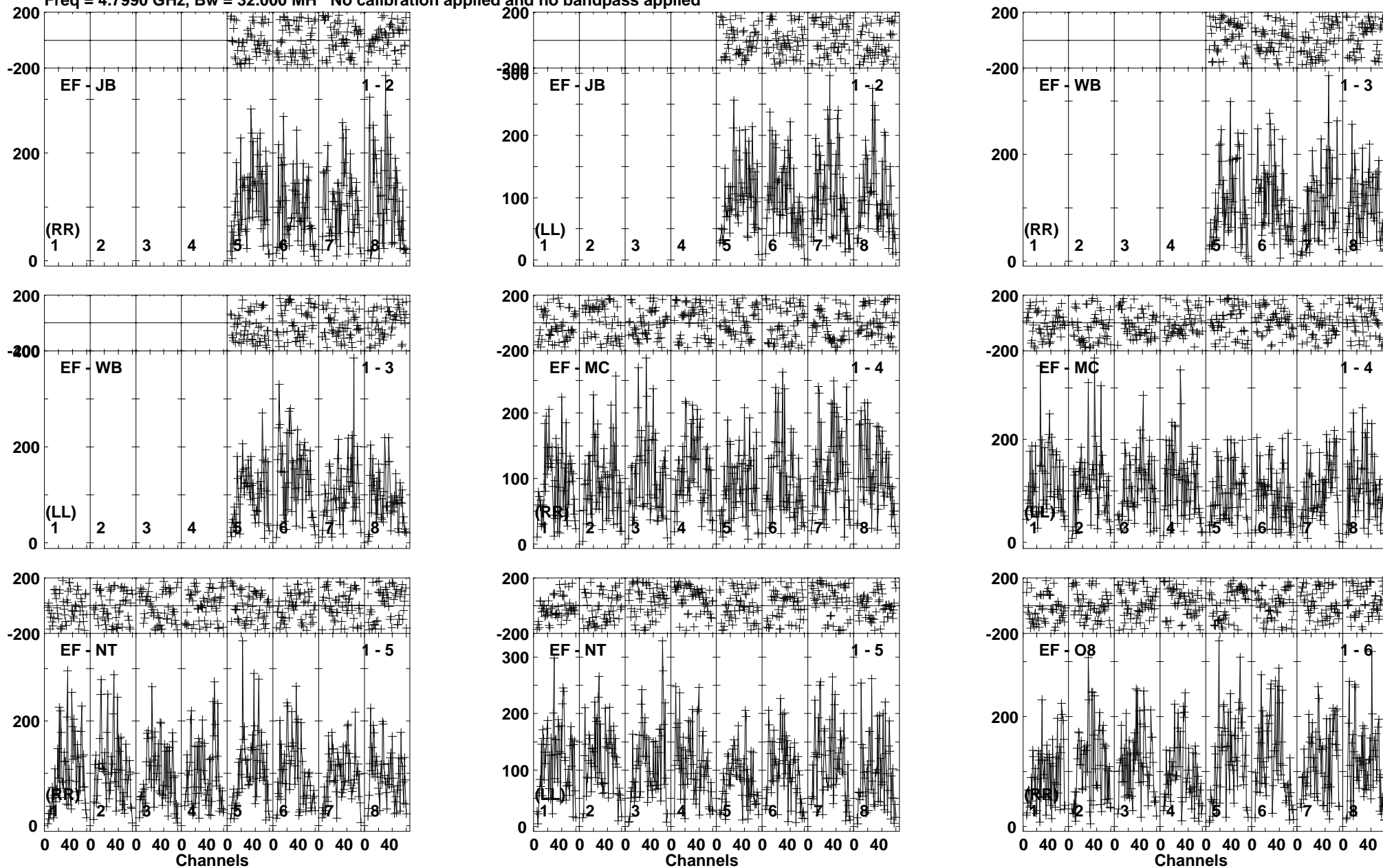
Lower frame: Micro Ampl Jy Top frame: Phas deg Vector averaged cross-power spectrum Baseline: EF (01) - JB (02) Timerange: 00/19:23:01 to 00/19:25:29
