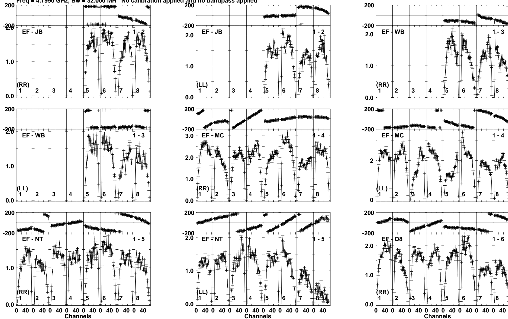
Lower frame: Milli Ampl Jy Top frame: Phas deg Vector averaged cross-power spectrum Baseline: EF (01) - JB (02) Timerange: 00/21:57:31 to 00/21:58:59
