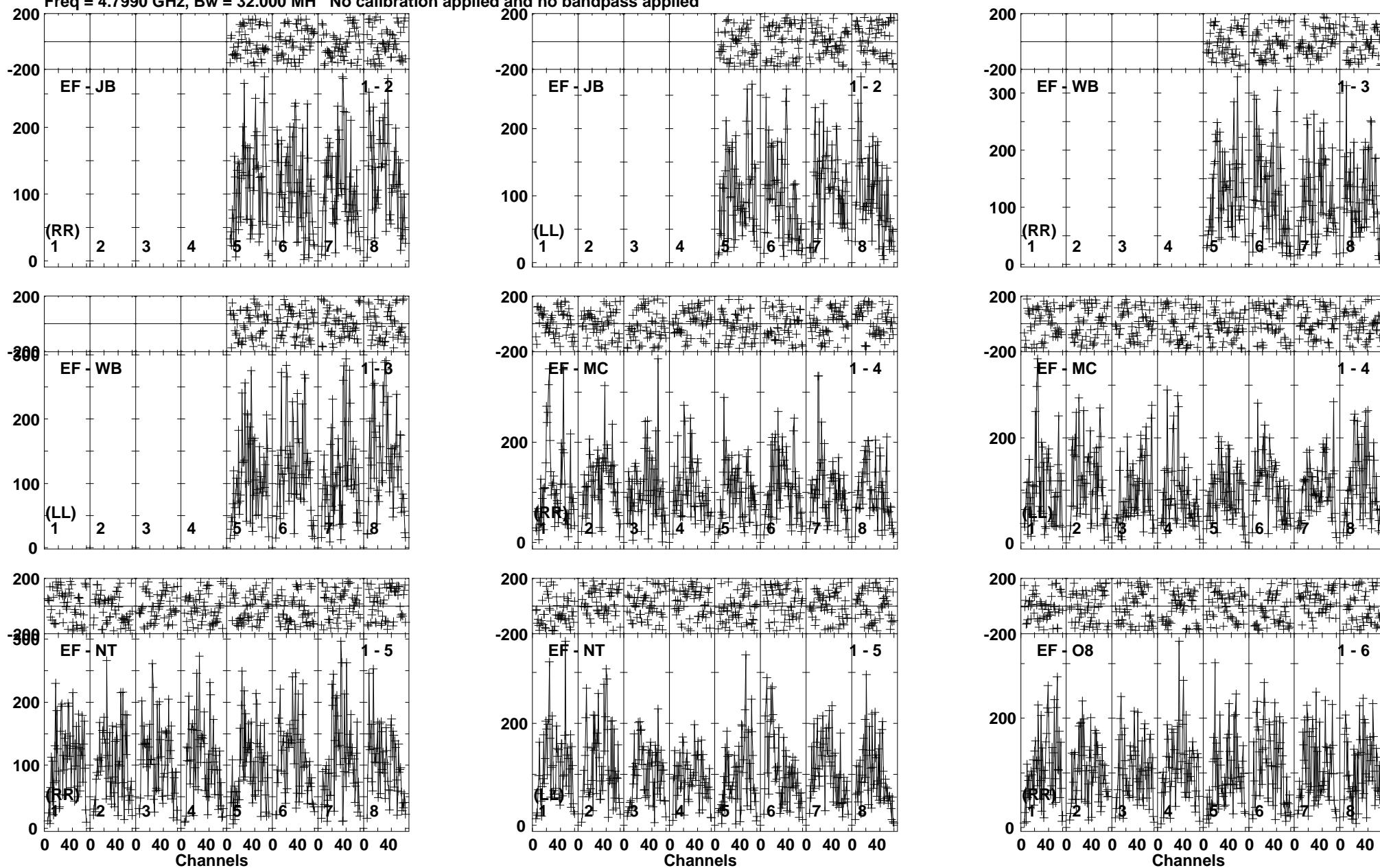
Lower frame: Micro Ampl Jy Top frame: Phas deg Vector averaged cross-power spectrum Baseline: EF (01) - JB (02) Timerange: 00/21:59:01 to 00/22:01:29
