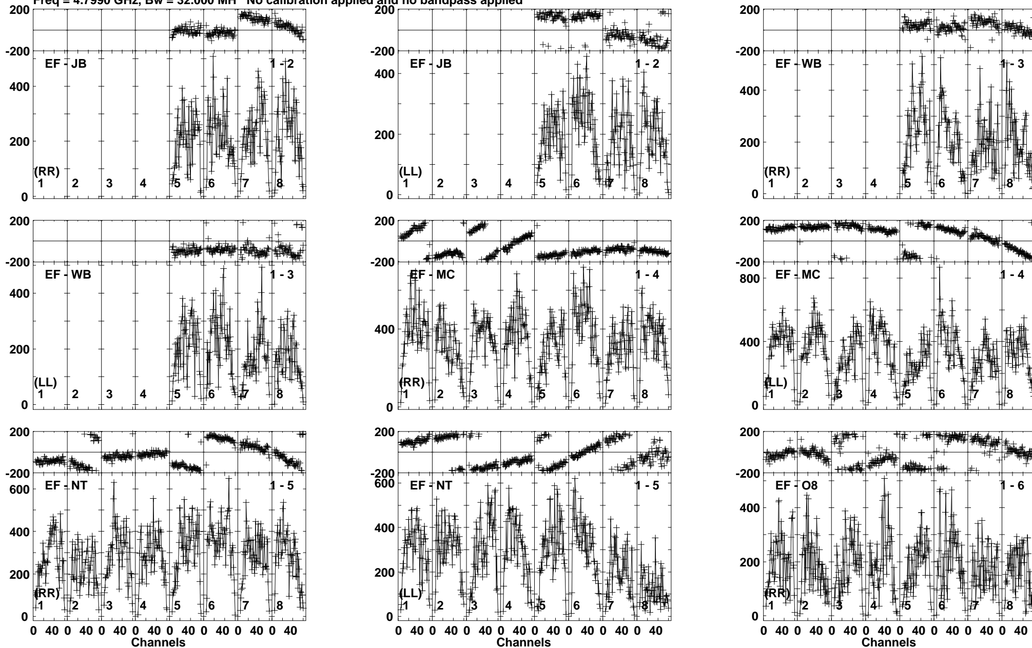
Lower frame: Micro Ampl Jy Top frame: Phas deg Vector averaged cross-power spectrum Baseline: EF (01) - JB (02) Timerange: 00:18:39:01 to 00:18:41:29
