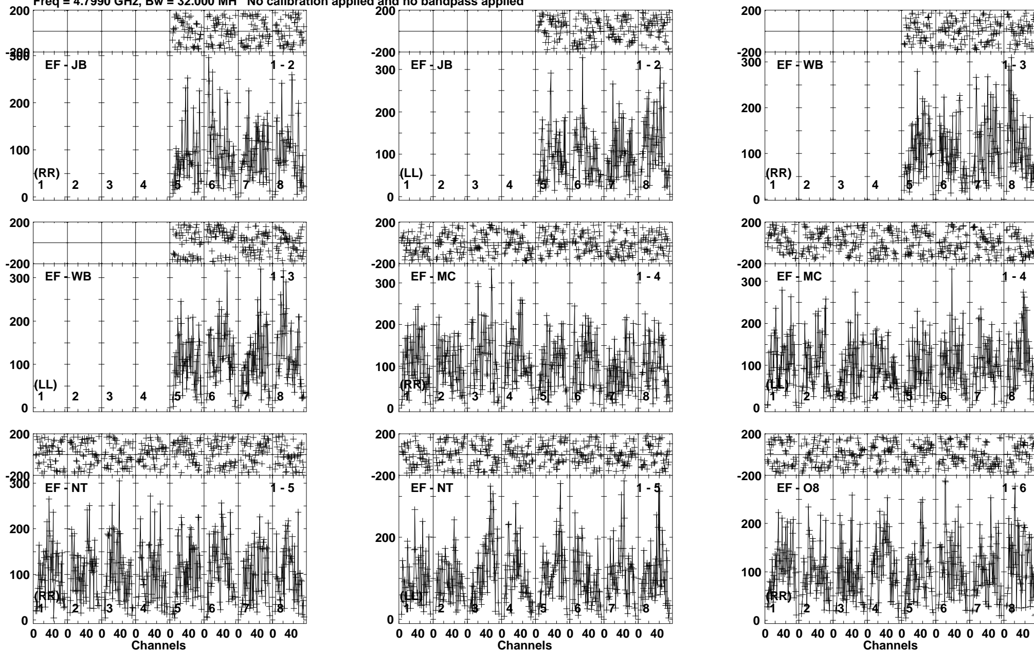
Lower frame: Micro Ampl Jy Top frame: Phas deg Vector averaged cross-power spectrum Baseline: EF (01) - JB (02) Timerange: 00/21:19:01 to 00/21:21:29
