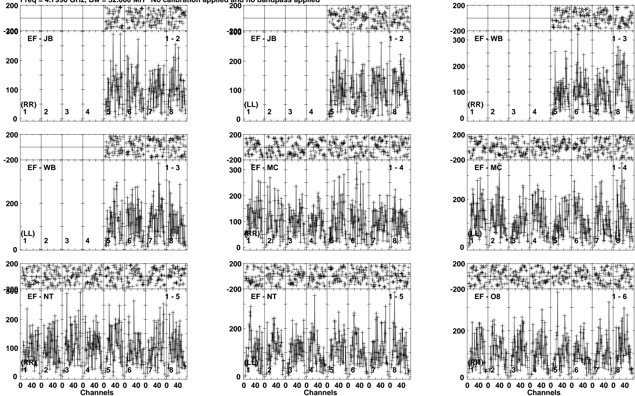
Lower frame: Micro Ampl Jy Top frame: Phas deg Vector averaged cross-power spectrum Baseline: EF (01) - JB (02) Timerange: 00/19:19:01 to 00/19:21:29
