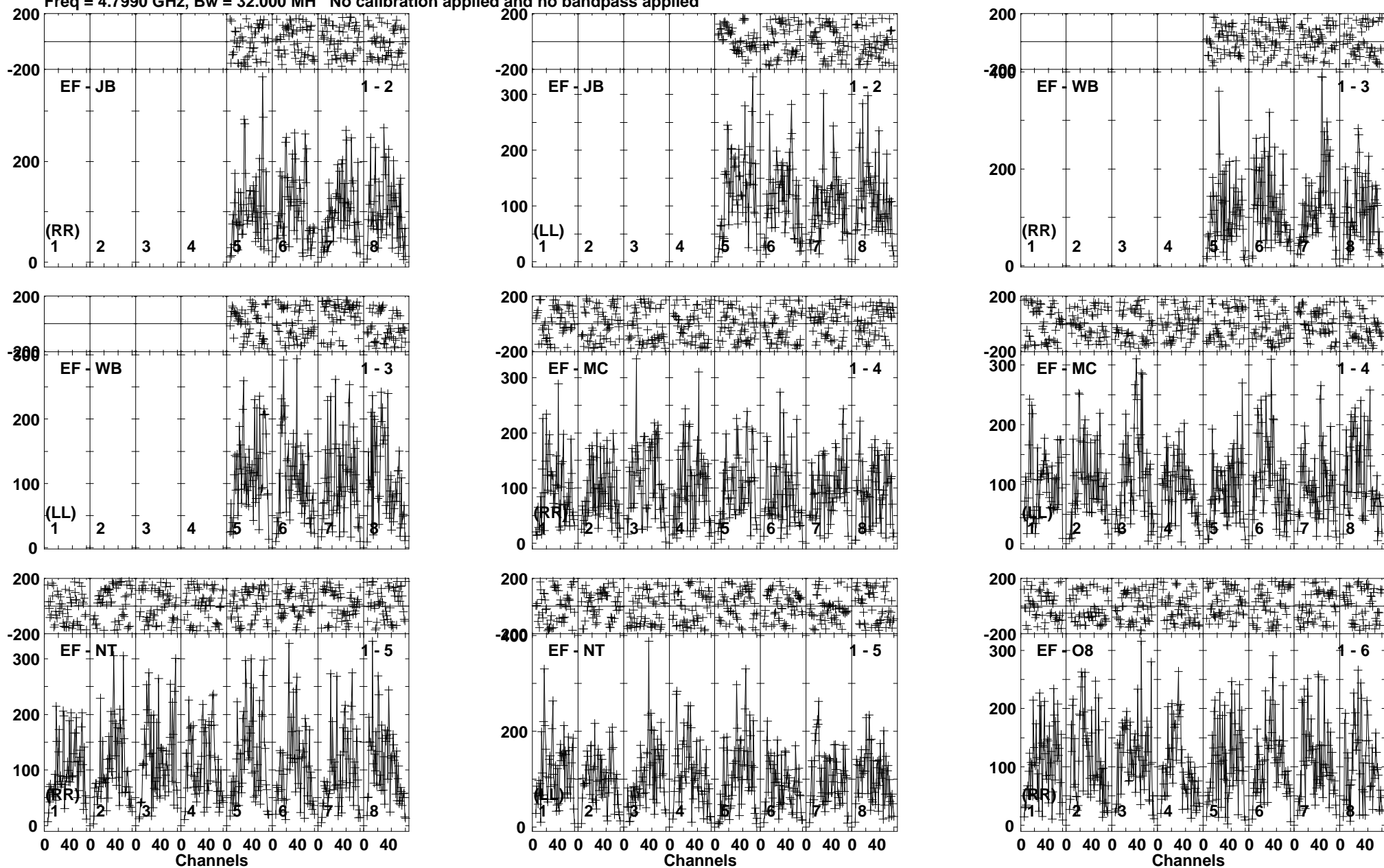
Lower frame: Micro Ampl Jy Top frame: Phas deg Vector averaged cross-power spectrum Baseline: EF (01) - JB (02) Timerange: 00/22:43:01 to 00/22:45:29
