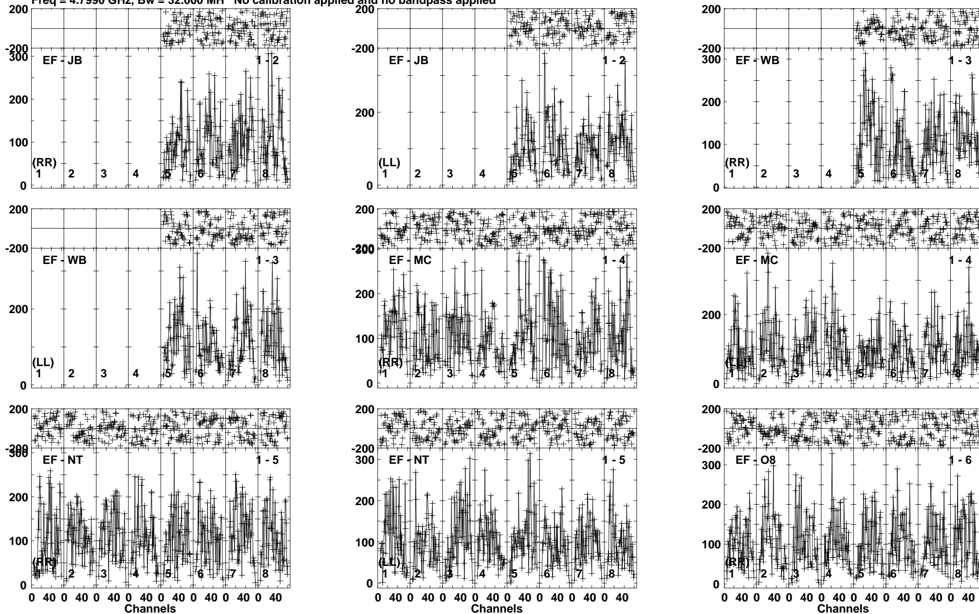
Lower frame: Micro Ampl Jy Top frame: Phas deg Vector averaged cross-power spectrum Baseline: EF (01) - JB (02) Timerange: 00/20:35:01 to 00/20:37:29
