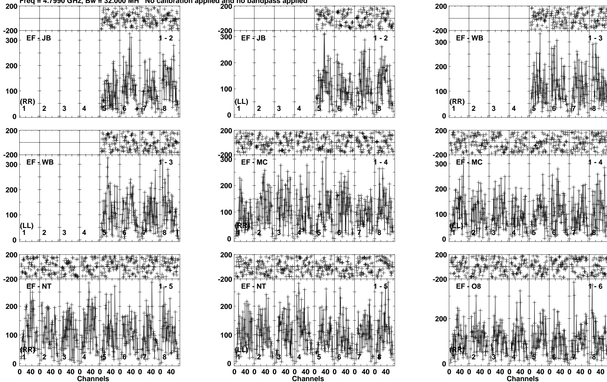
Lower frame: Micro Ampl Jy Top frame: Phas deg Vector averaged cross-power spectrum Baseline: EF (01) - JB (02) Timerange: 00/22:35:01 to 00/22:37:29
