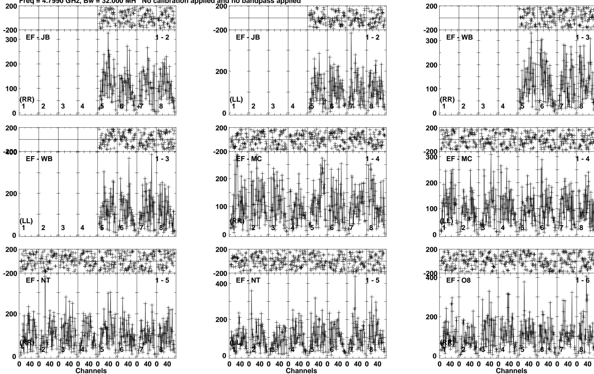
Lower frame: Micro Ampl Jy Top frame: Phas deg Vector averaged cross-power spectrum Baseline: EF (01) - JB (02) Timerange: 00/22:11:01 to 00/22:13:29
