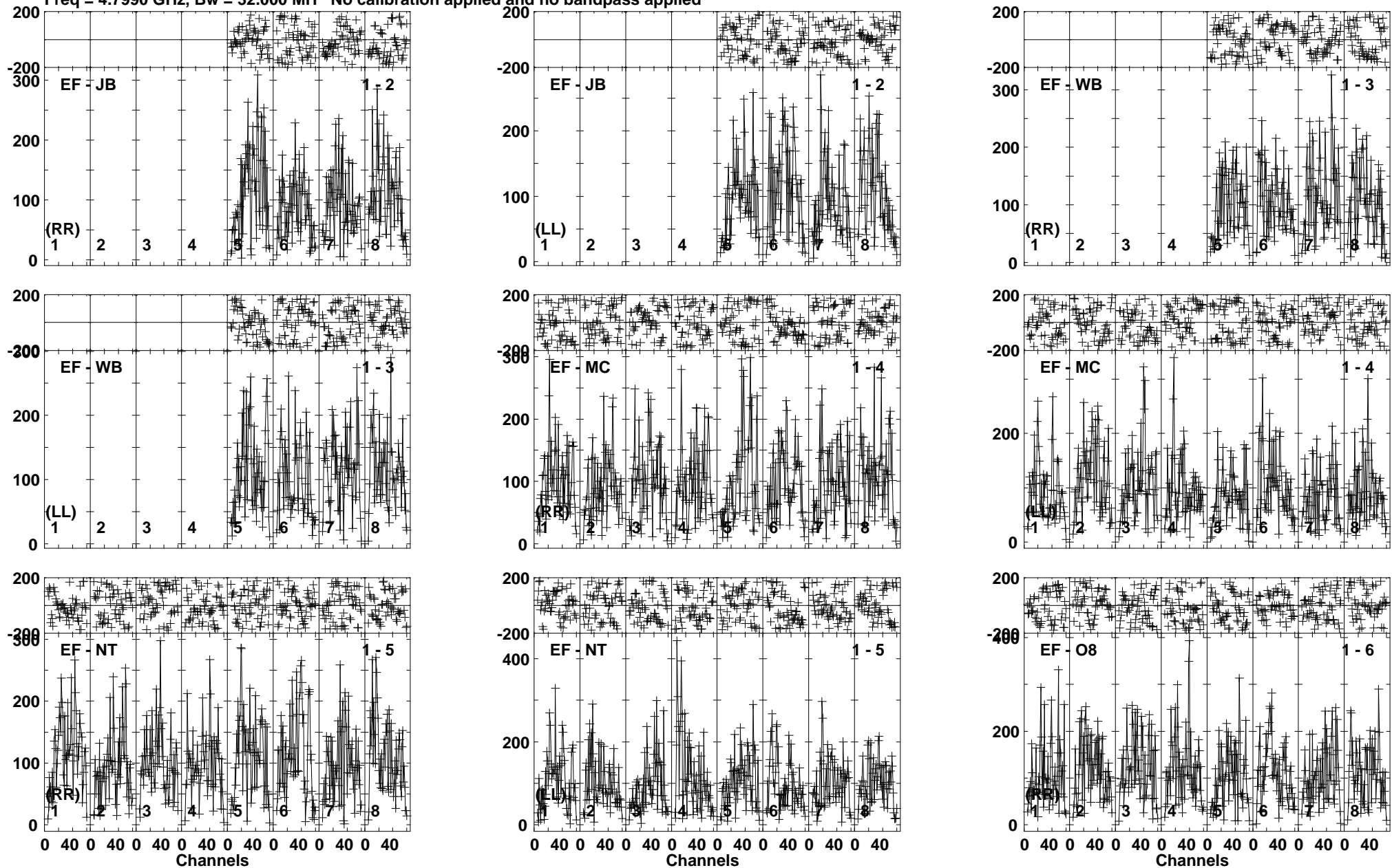
Lower frame: Micro Ampl Jy Top frame: Phas deg Vector averaged cross-power spectrum Baseline: EF (01) - JB (02) Timerange: 00/18:23:01 to 00/18:25:29
