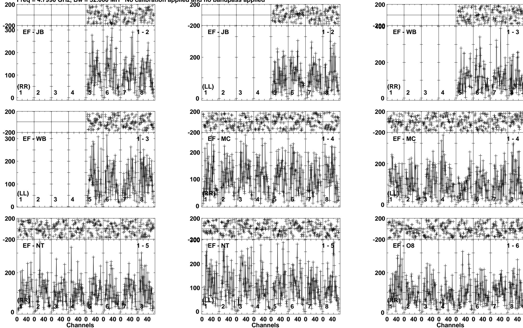
Lower frame: Micro Ampl Jy Top frame: Phas deg Vector averaged cross-power spectrum Baseline: EF (01) - JB (02) Timerange: 00/18:27:01 to 00/18:29:29
