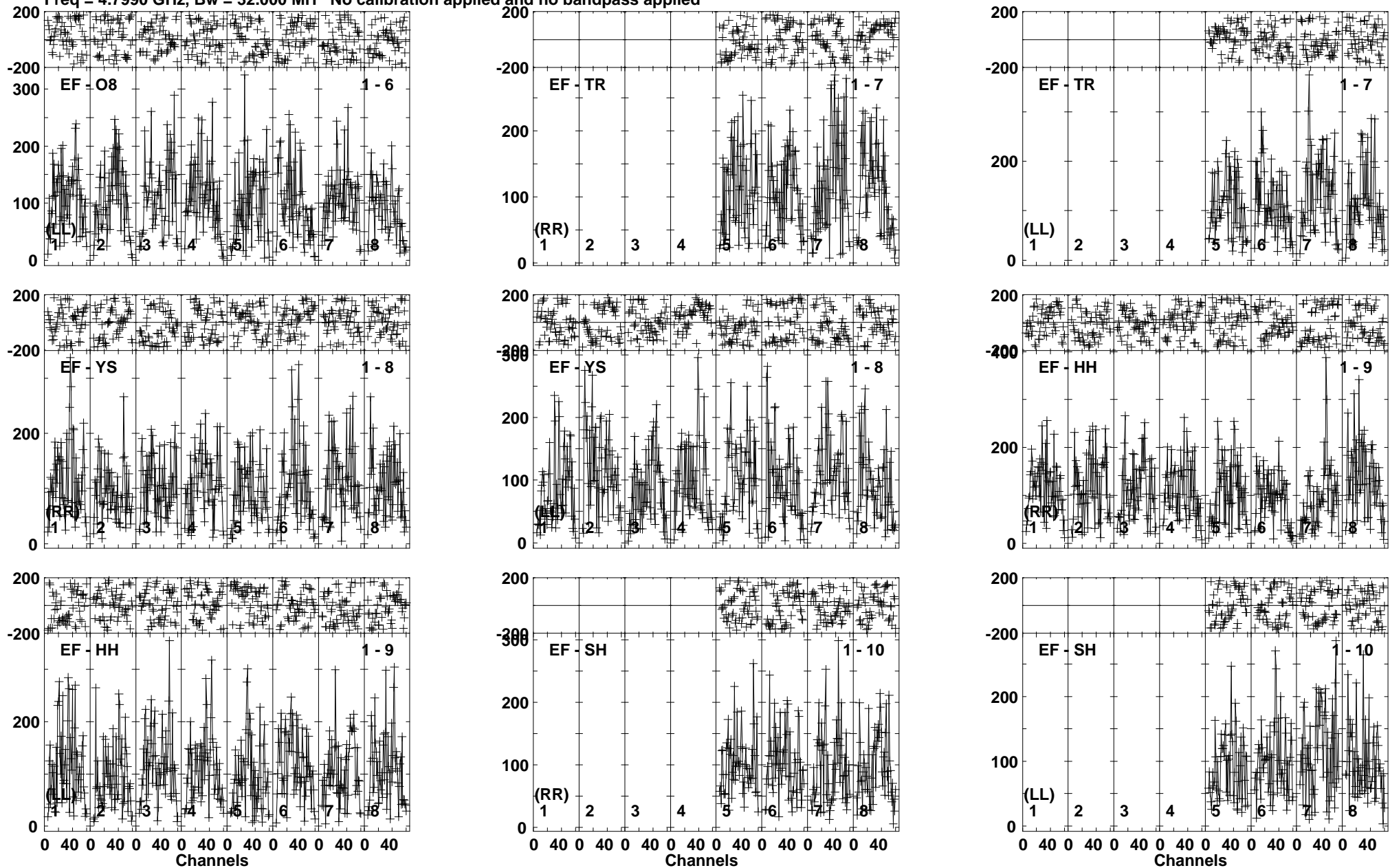
Lower frame: Micro Ampl Jy Top frame: Phas deg Vector averaged cross-power spectrum Baseline: EF (01) - O8 (06) Timerange: 00:18:47:01 to 00:18:49:29
