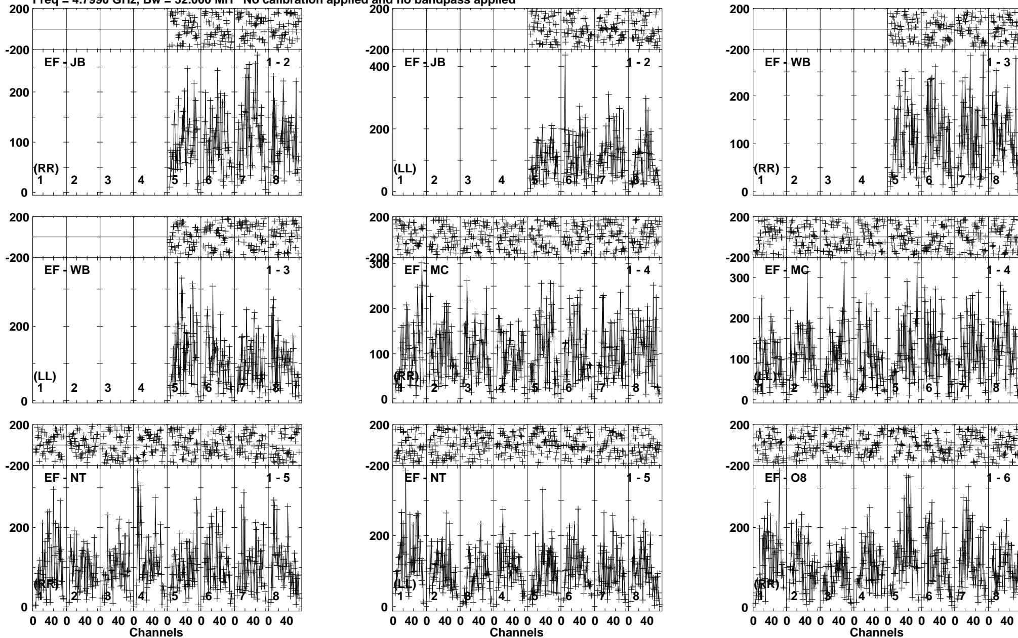
Lower frame: Micro Ampl Jy Top frame: Phas deg Vector averaged cross-power spectrum Baseline: EF (01) - JB (02) Timerange: 00/22:19:01 to 00/22:21:29
