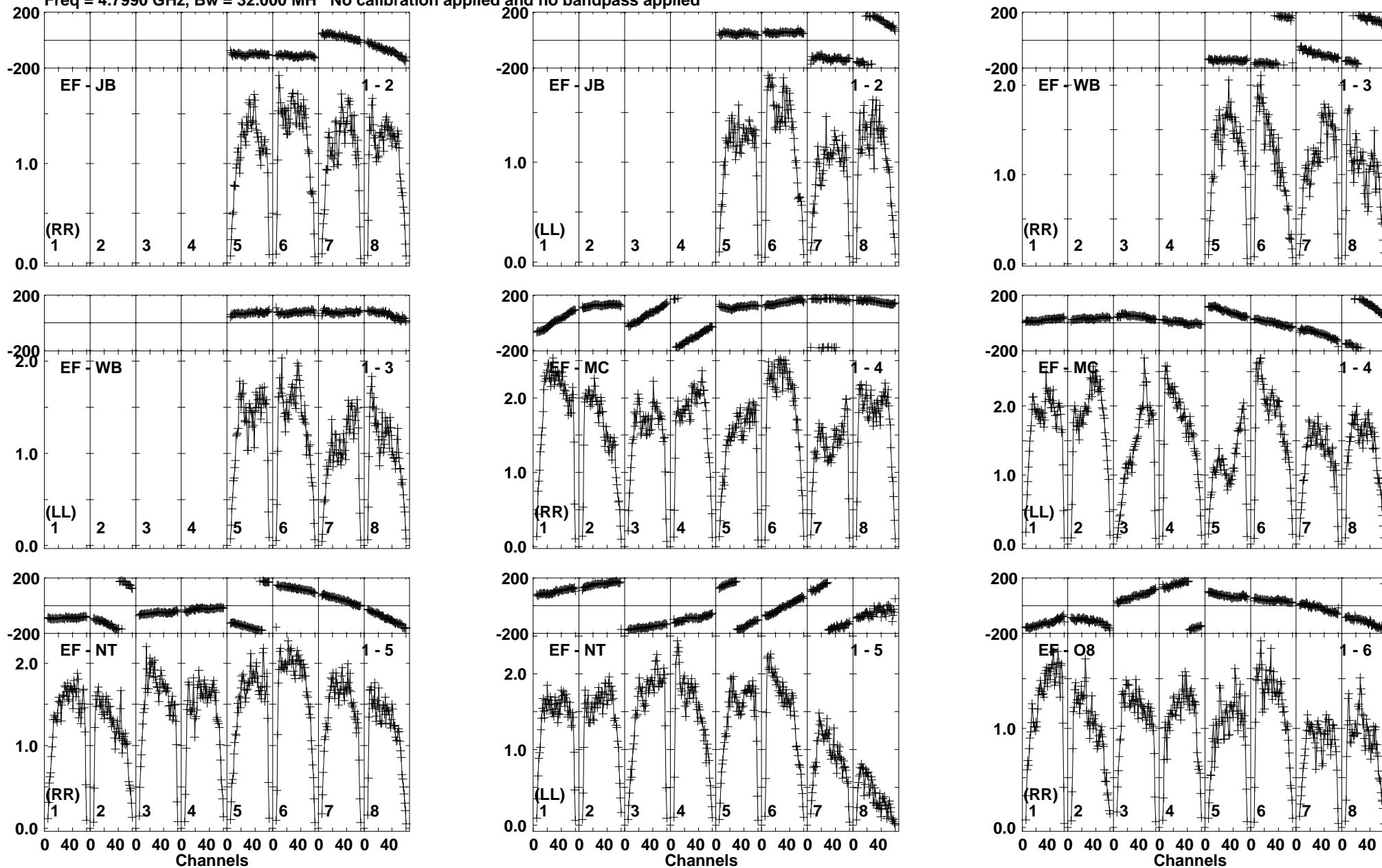
Lower frame: Milli Ampl Jy Top frame: Phas deg Vector averaged cross-power spectrum Baseline: EF (01) - JB (02) Timerange: 00/18:21:31 to 00/18:22:59
