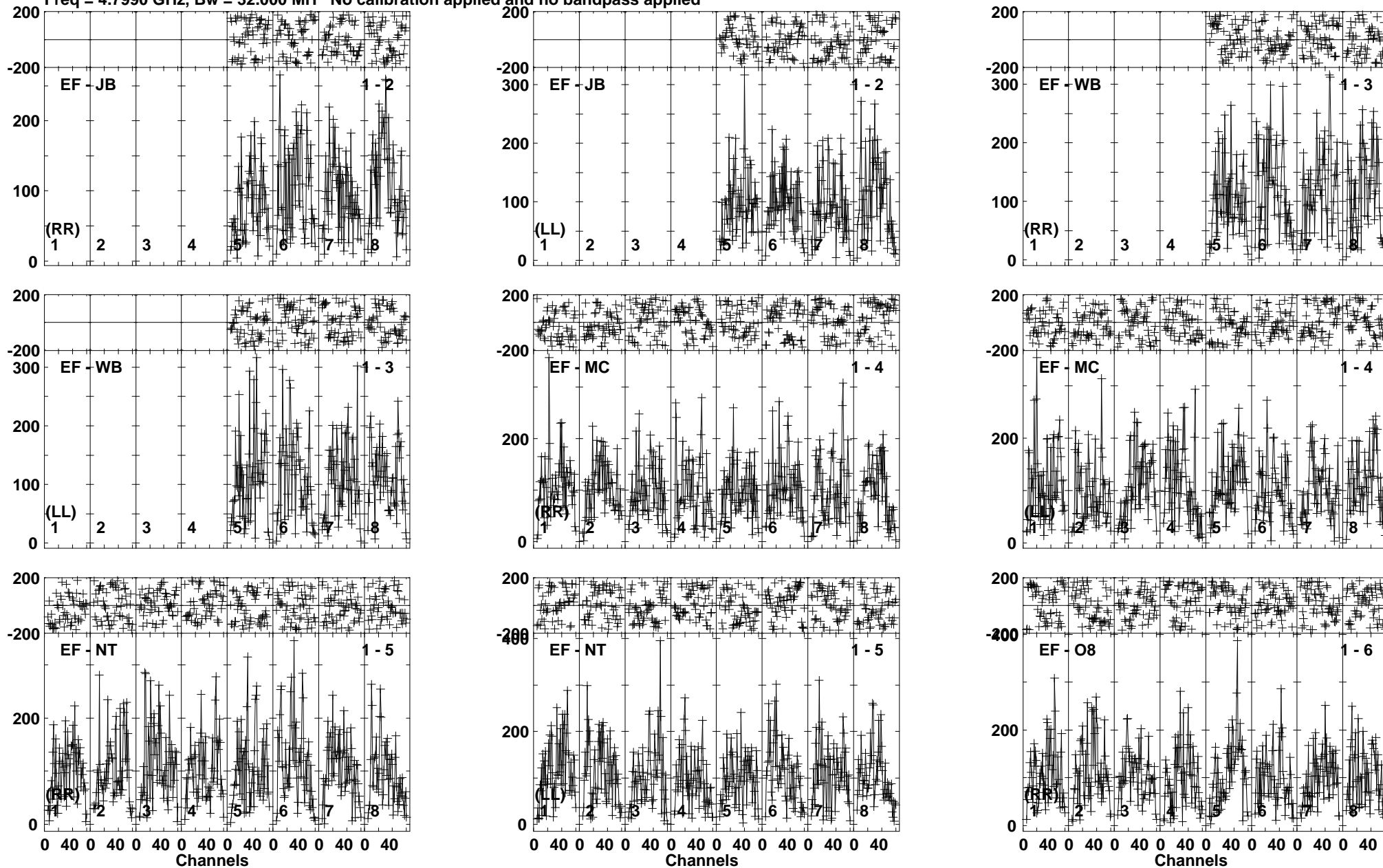
Lower frame: Micro Ampl Jy Top frame: Phas deg Vector averaged cross-power spectrum Baseline: EF (01) - JB (02) Timerange: 00/20:11:01 to 00/20:13:29
