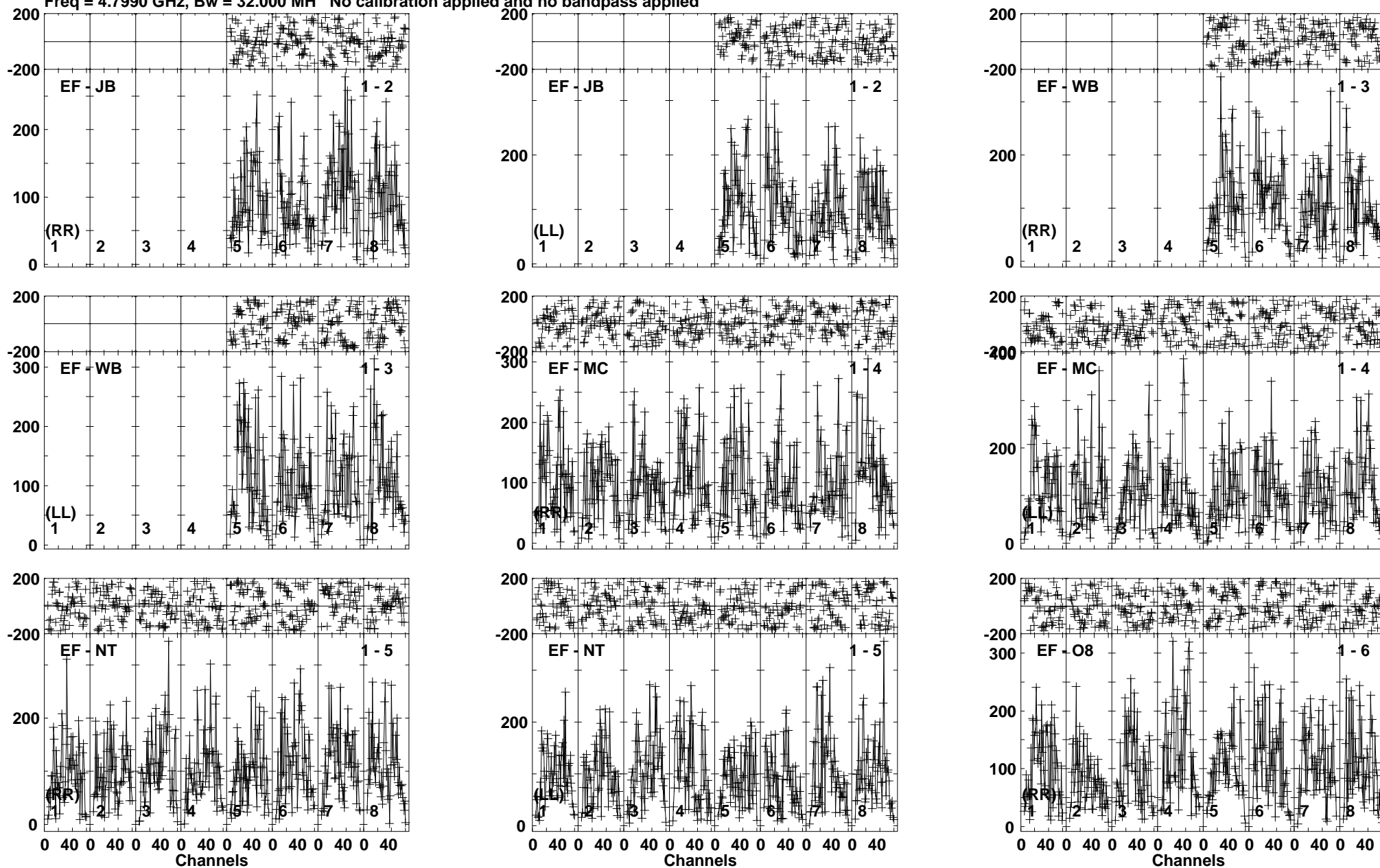
Lower frame: Micro Ampl Jy Top frame: Phas deg Vector averaged cross-power spectrum Baseline: EF (01) - JB (02) Timerange: 00/23:19:01 to 00/23:21:29
