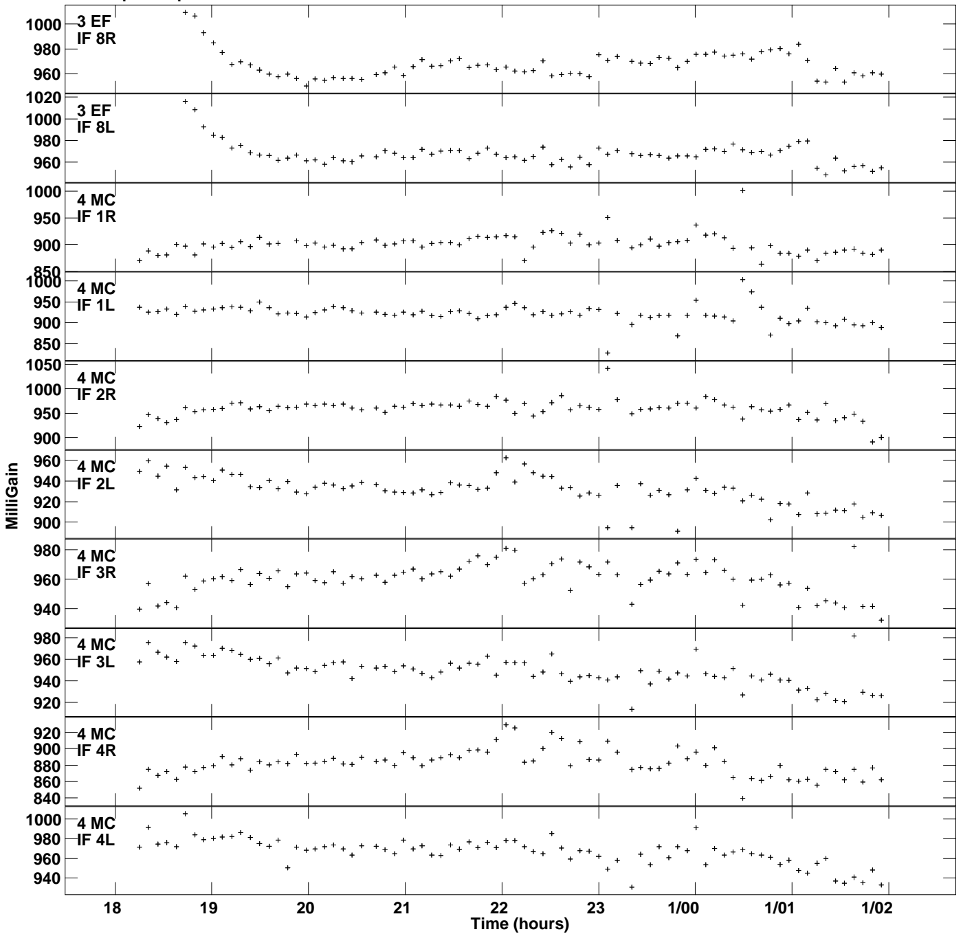
Plot file version 4 created 12-APR-2022 18:13:33 Gain amp vs UTC time for J1329+3154.MULTI.1 SN 2 Rpol & Lpol IF 1 - 8
