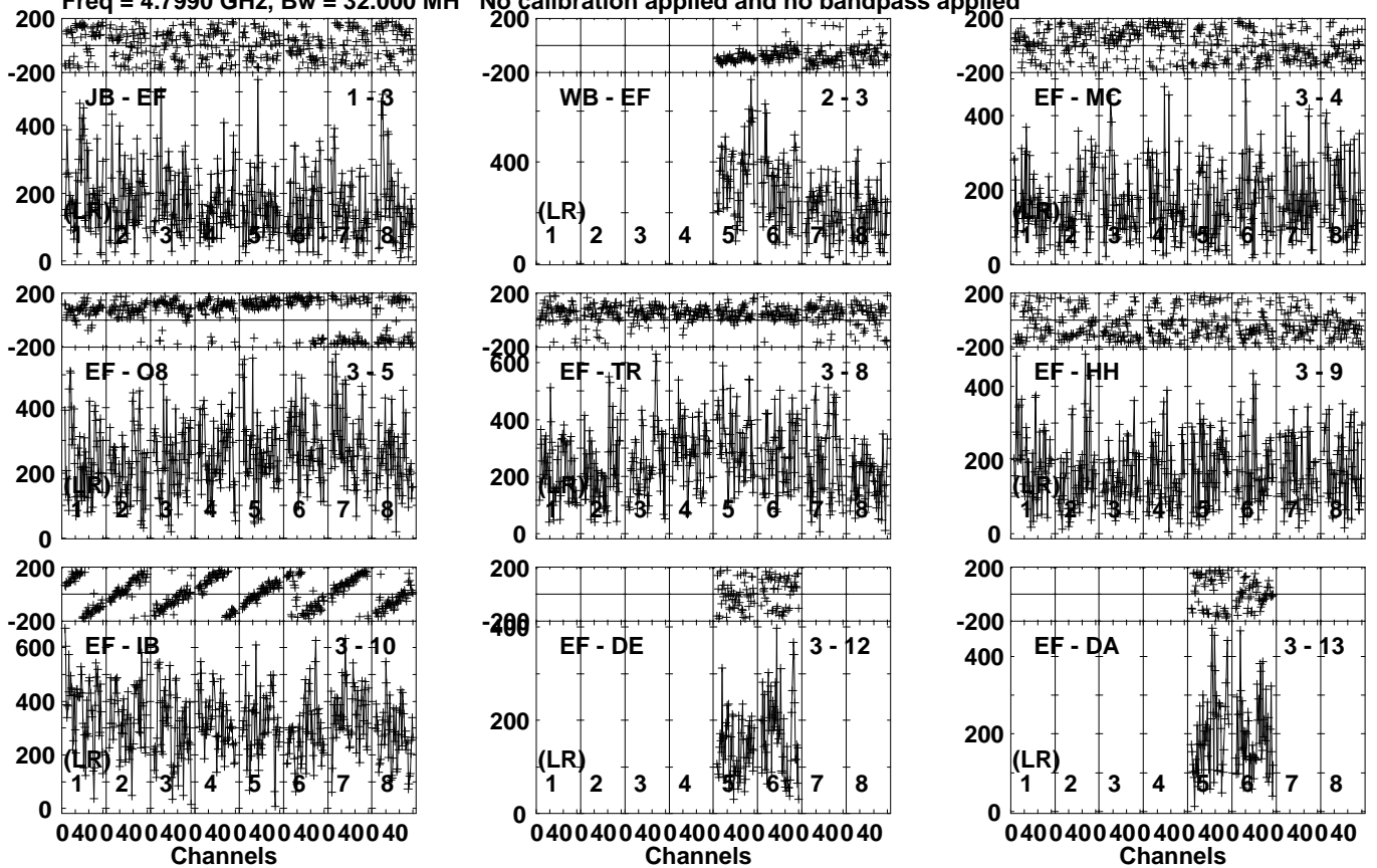
Lower frame: Micro Ampl Jy Top frame: Phas deg Vector averaged cross-power spectrum Several baselines displayed Timerange: 00/16:31:01 to 00/16:31:59
