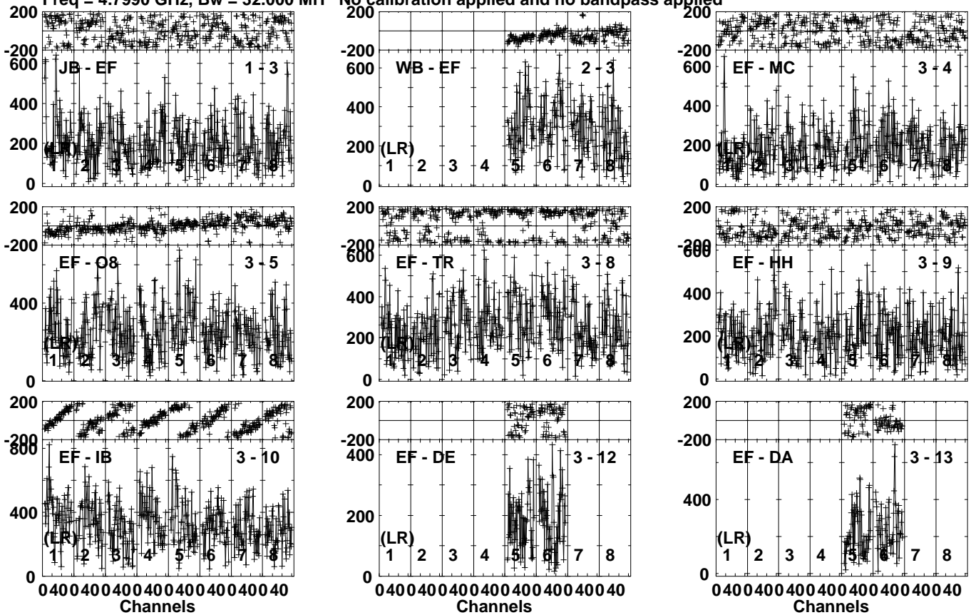
Lower frame: Micro Ampl Jy Top frame: Phas deg Vector averaged cross-power spectrum Several baselines displayed Timerange: 00/17:15:03 to 00/17:16:29
