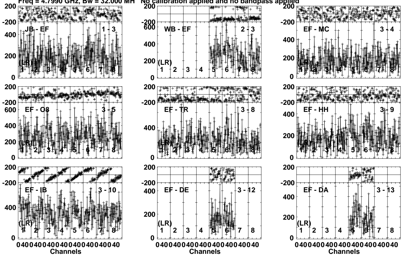
Lower frame: Micro Ampl Jy Top frame: Phas deg Vector averaged cross-power spectrum Several baselines displayed Timerange: 00/15:08:31 to 00/15:09:29
