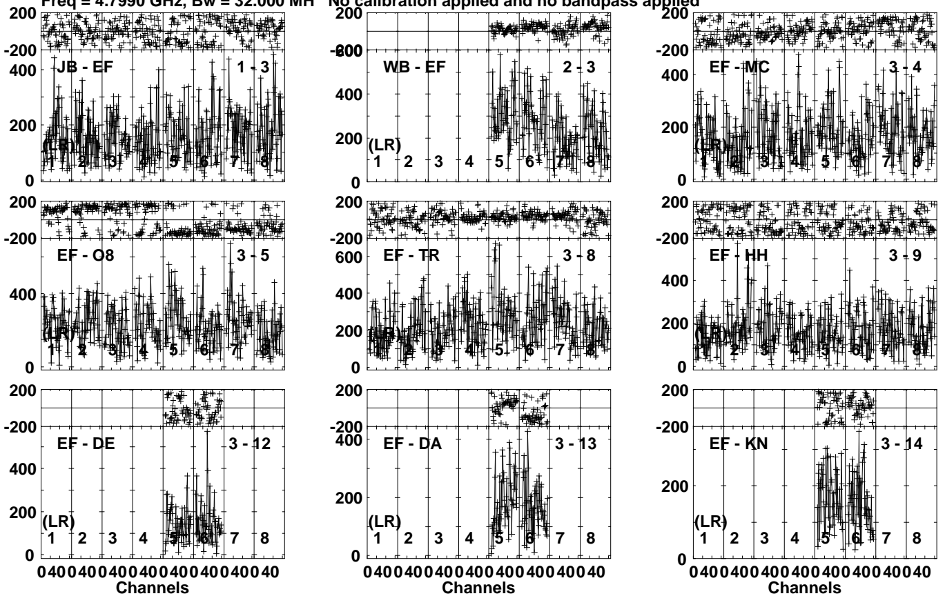
Lower frame: Micro Ampl Jy Top frame: Phas deg Vector averaged cross-power spectrum Several baselines displayed Timerange: 00/18:42:01 to 00/18:42:59
