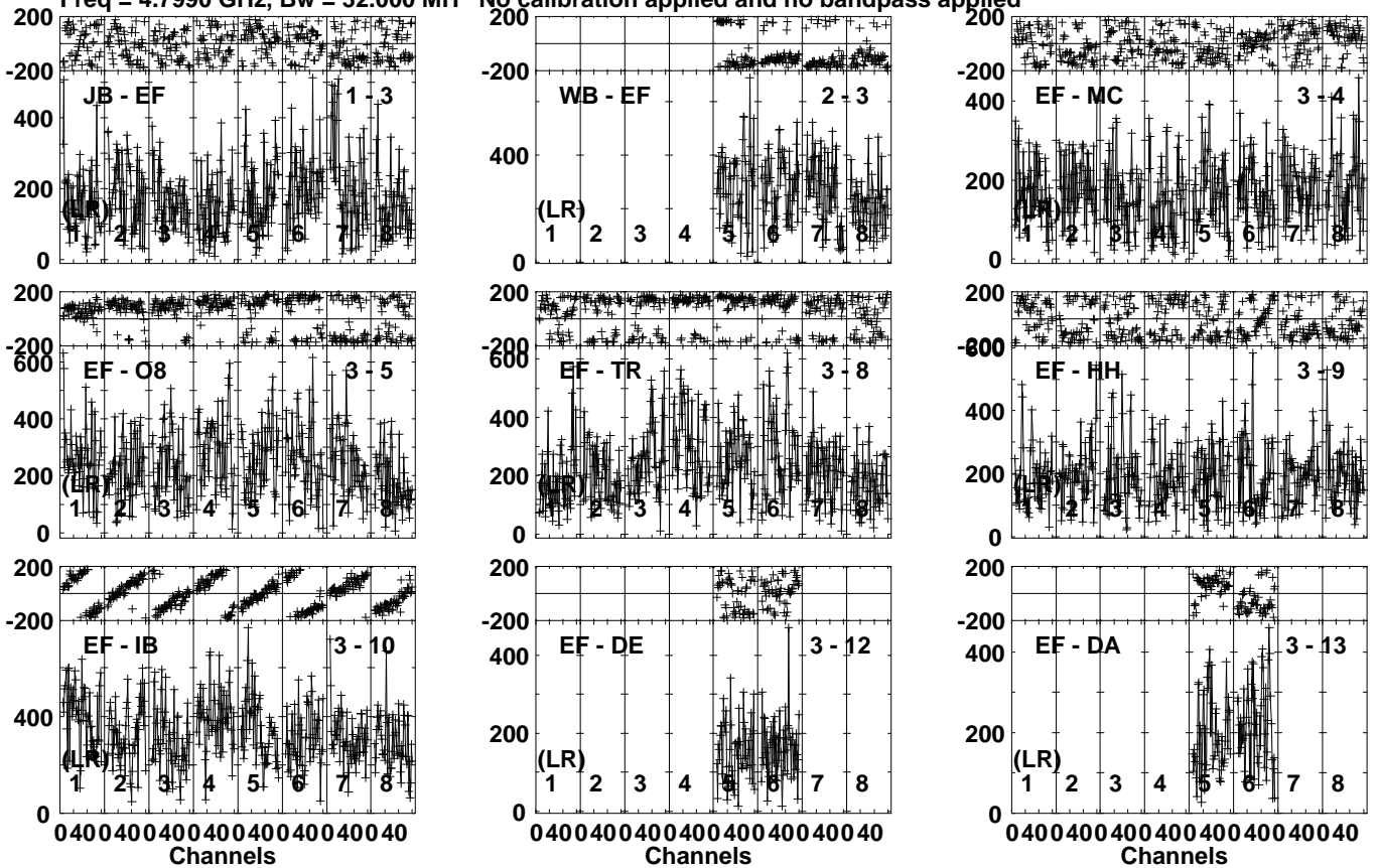
Lower frame: Micro Ampl Jy Top frame: Phas deg Vector averaged cross-power spectrum Several baselines displayed Timerange: 00/16:20:31 to 00/16:21:59
