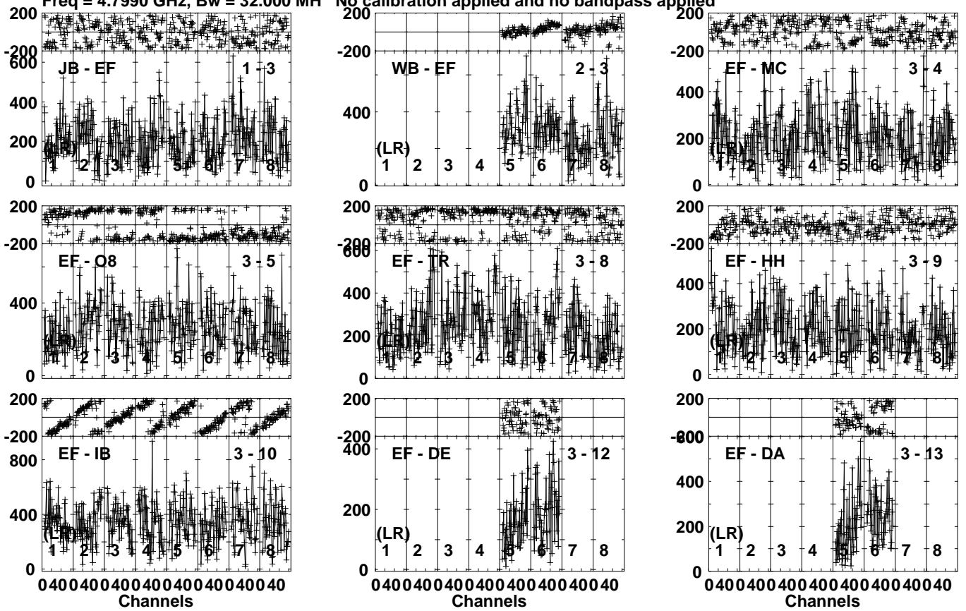
Lower frame: Micro Ampl Jy Top frame: Phas deg Vector averaged cross-power spectrum Several baselines displayed Timerange: 00/16:44:31 to 00/16:45:59
