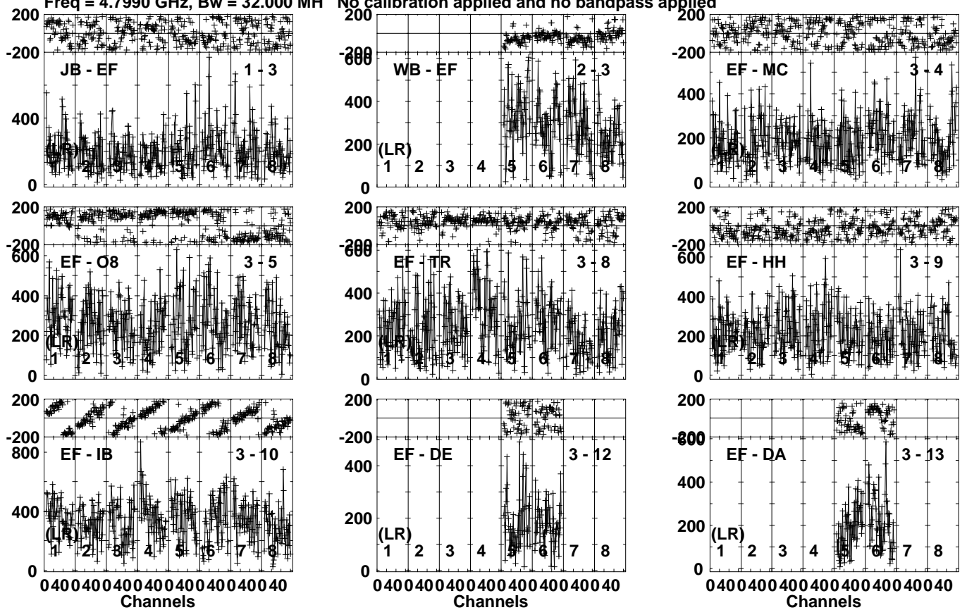
Lower frame: Micro Ampl Jy Top frame: Phas deg Vector averaged cross-power spectrum Several baselines displayed Timerange: 00/16:34:31 to 00/16:35:59
