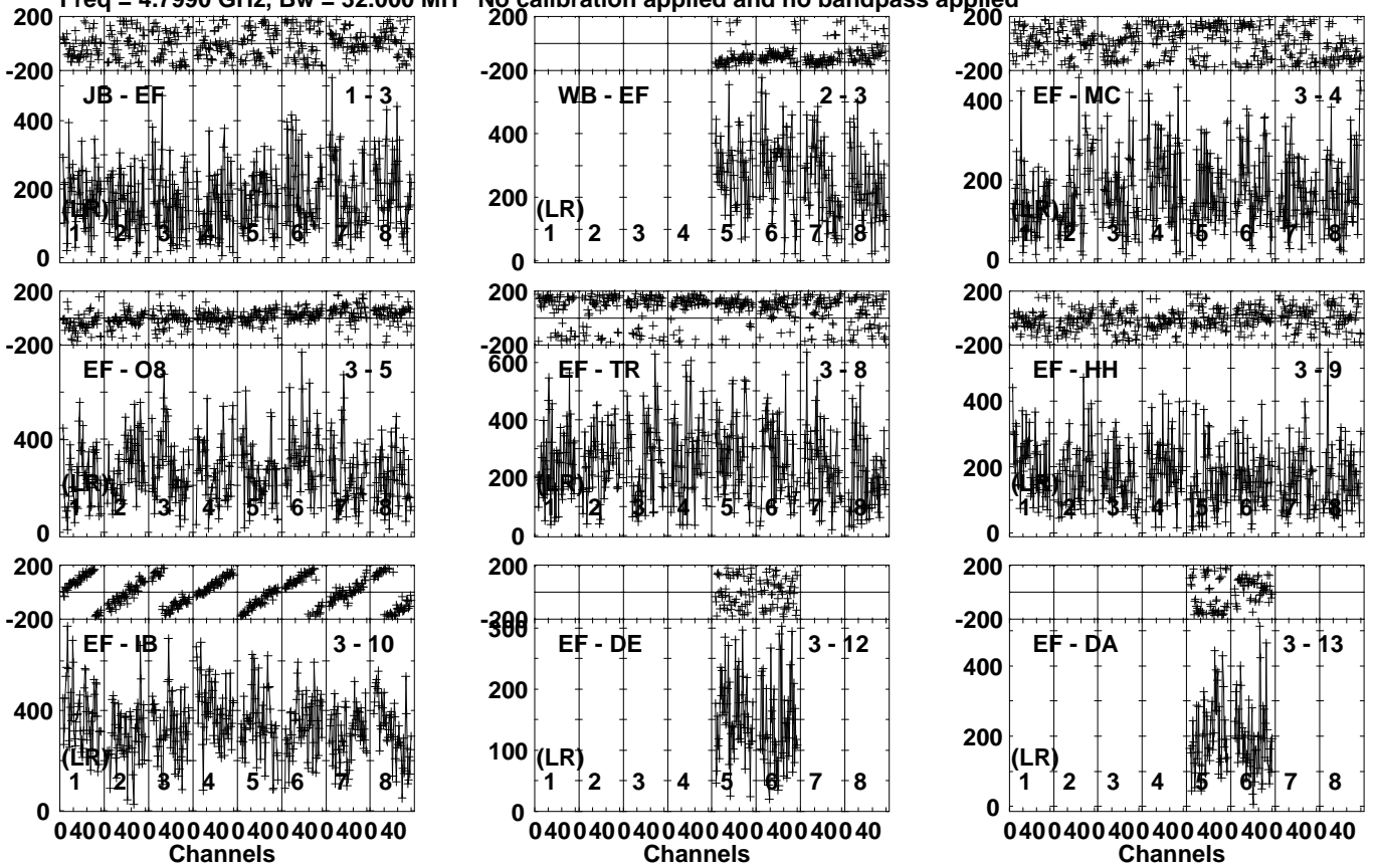
Lower frame: Micro Ampl Jy Top frame: Phas deg Vector averaged cross-power spectrum Several baselines displayed Timerange: 00/15:32:03 to 00/15:33:29
