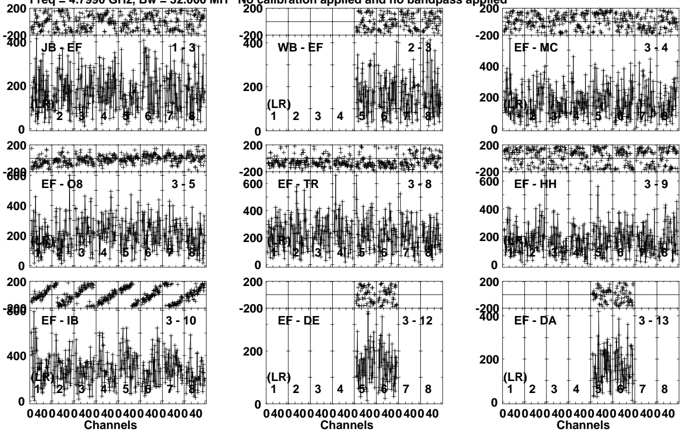
Lower frame: Micro Ampl Jy Top frame: Phas deg Vector averaged cross-power spectrum Several baselines displayed Timerange: 00/14:16:01 to 00/14:17:29
