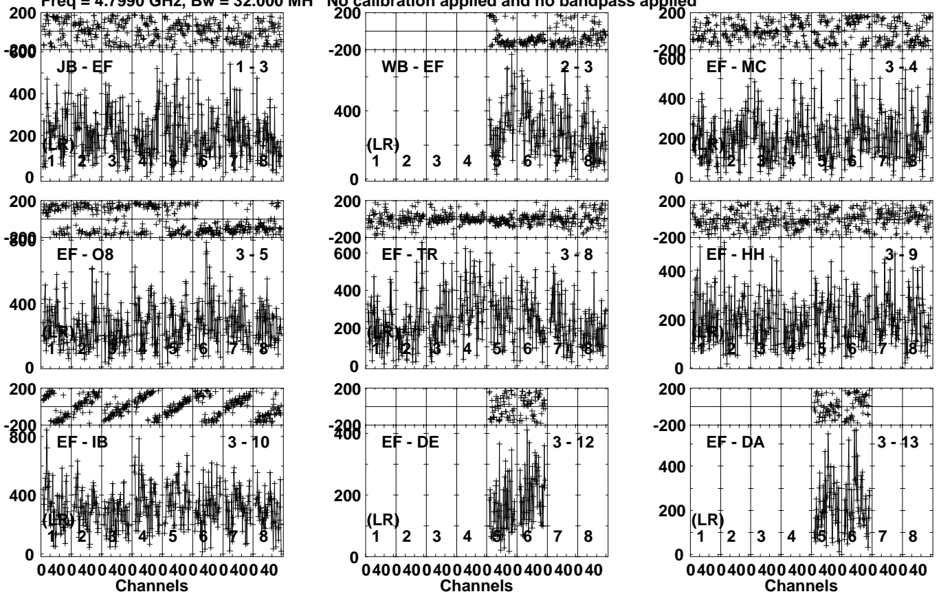
Lower frame: Micro Ampl Jy Top frame: Phas deg Vector averaged cross-power spectrum Several baselines displayed Timerange: 00/17:29:31 to 00/17:30:29
