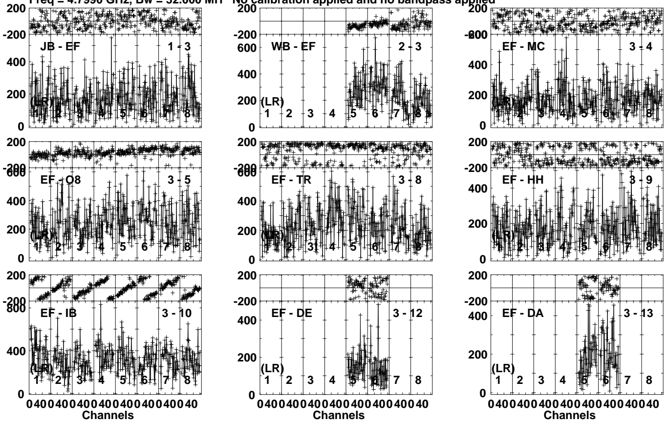
Lower frame: Micro Ampl Jy Top frame: Phas deg Vector averaged cross-power spectrum Several baselines displayed Timerange: 00/15:17:31 to 00/15:18:29
