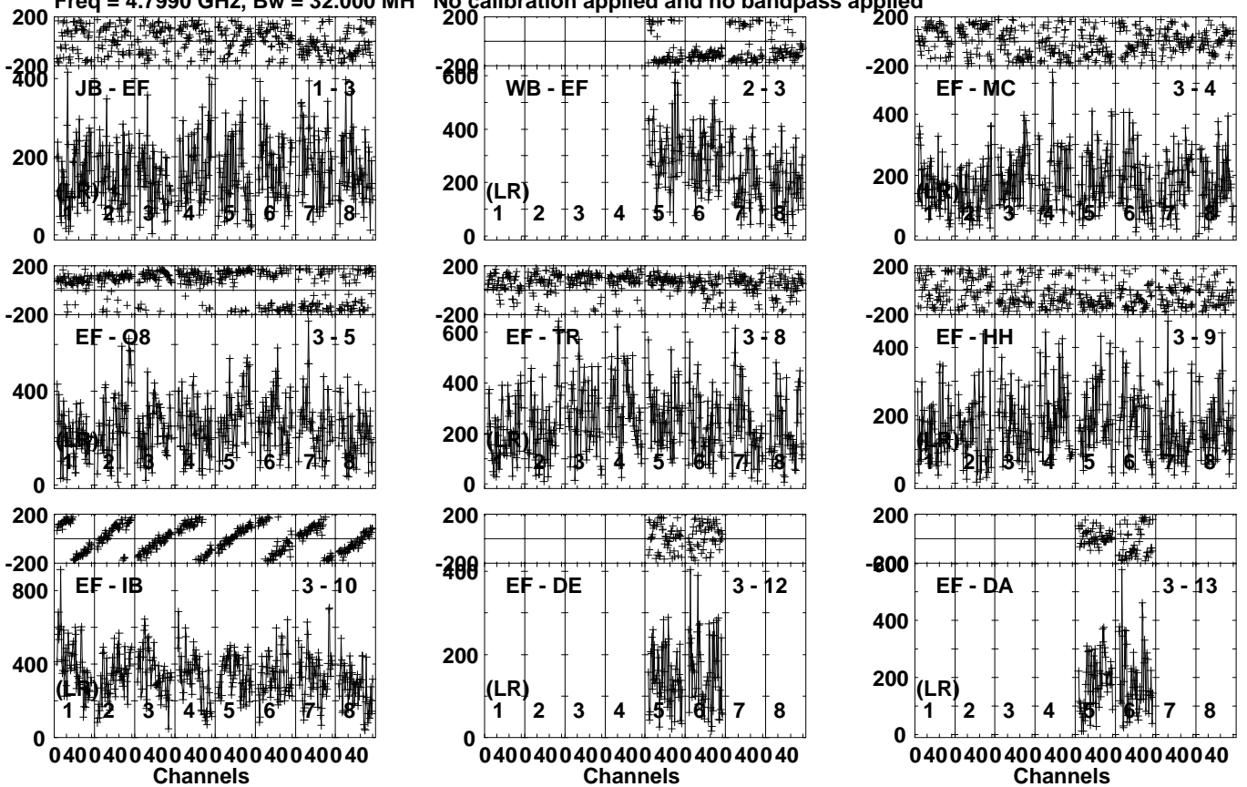
Lower frame: Micro Ampl Jy Top frame: Phas deg Vector averaged cross-power spectrum Several baselines displayed Timerange: 00/16:25:31 to 00/16:26:59
