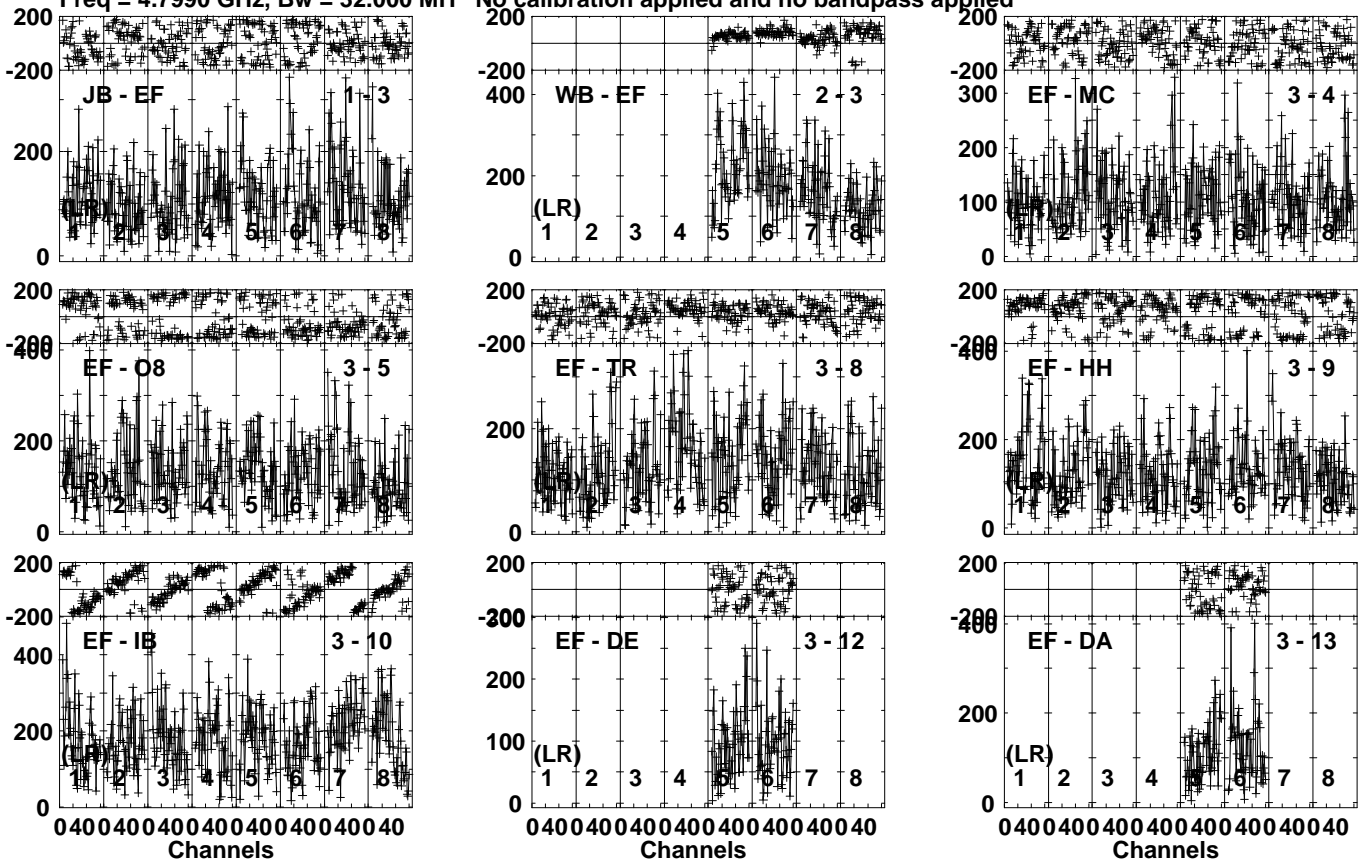
Lower frame: Micro Ampl Jy Top frame: Phas deg Vector averaged cross-power spectrum Several baselines displayed Timerange: 00/15:38:31 to 00/15:40:59
