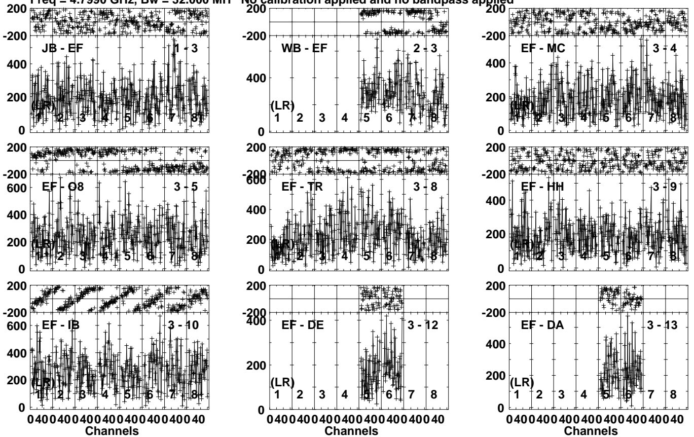
Lower frame: Micro Ampl Jy Top frame: Phas deg Vector averaged cross-power spectrum Several baselines displayed Timerange: 00/18:27:31 to 00/18:28:59
