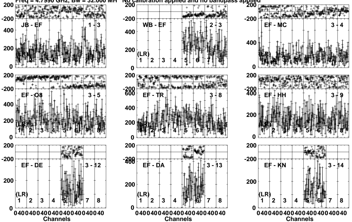
Lower frame: Micro Ampl Jy Top frame: Phas deg Vector averaged cross-power spectrum Several baselines displayed Timerange: 00/18:51:31 to 00/18:52:59
