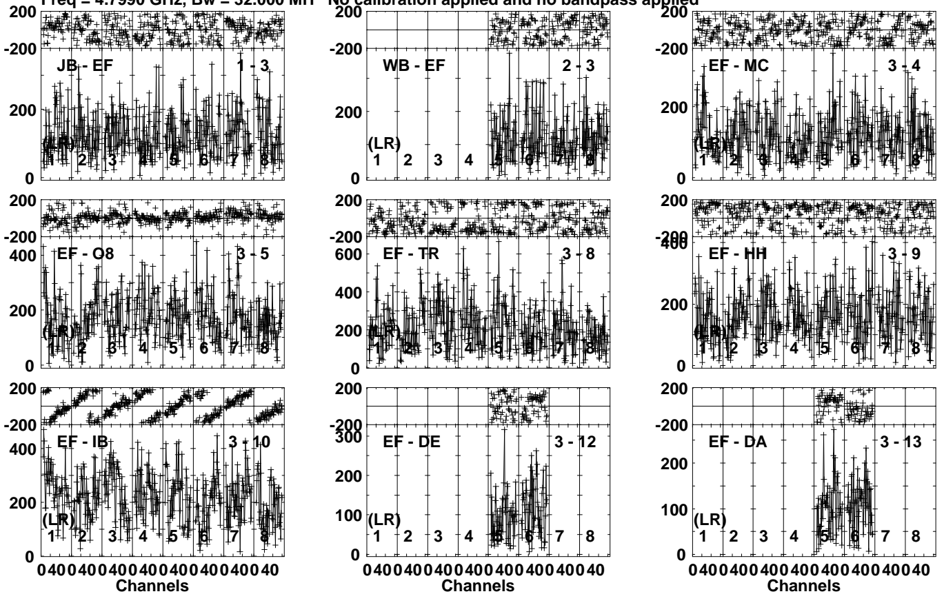
Lower frame: Micro Ampl Jy Top frame: Phas deg Vector averaged cross-power spectrum Several baselines displayed Timerange: 00/13:50:31 to 00/13:51:59
