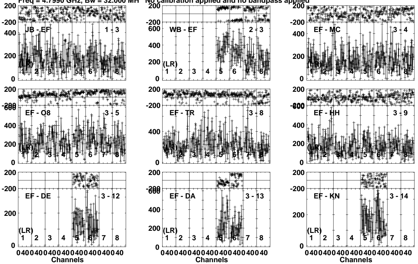
Lower frame: Micro Ampl Jy Top frame: Phas deg Vector averaged cross-power spectrum Several baselines displayed Timerange: 00/15:56:31 to 00/15:57:29
