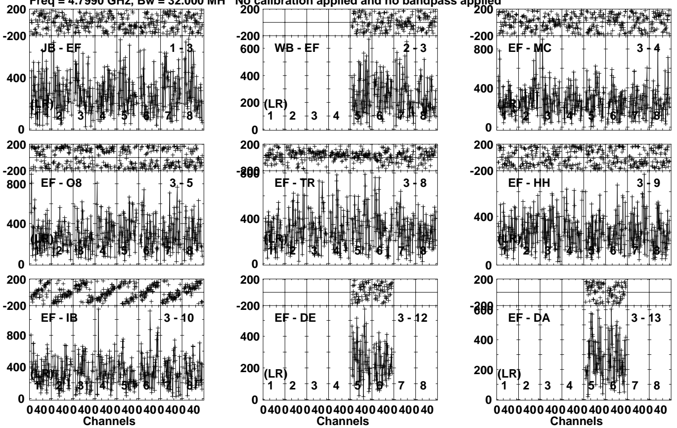
Lower frame: Micro Ampl Jy Top frame: Phas deg Vector averaged cross-power spectrum Several baselines displayed Timerange: 00/14:11:31 to 00/14:12:29
