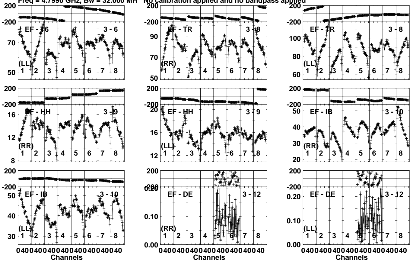
Lower frame: Milli Ampl Jy Top frame: Phas deg Vector averaged cross-power spectrum Several baselines displayed Timerange: 00/17:01:01 to 00/17:06:29
