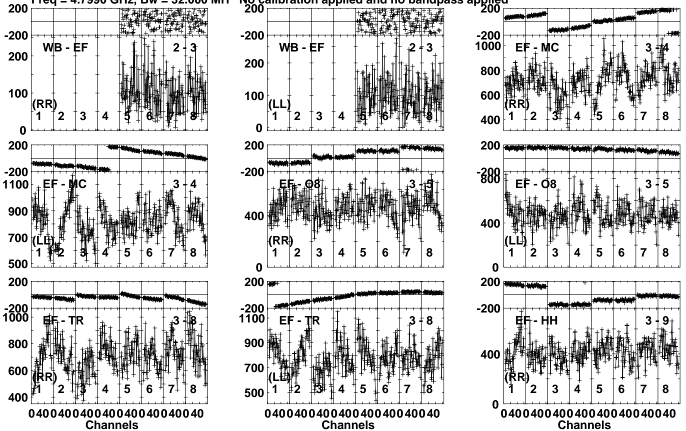
Lower frame: Micro Ampl Jy Top frame: Phas deg Vector averaged cross-power spectrum Several baselines displayed Timerange: 00/13:57:01 to 00/13:59:29
