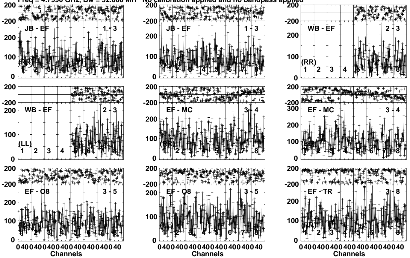
Lower frame: Micro Ampl Jy Top frame: Phas deg Vector averaged cross-power spectrum Several baselines displayed Timerange: 00/14:17:31 to 00/14:20:59
