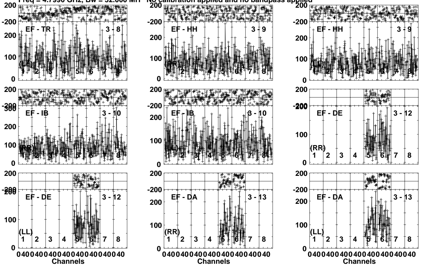
Lower frame: Micro Ampl Jy Top frame: Phas deg Vector averaged cross-power spectrum Several baselines displayed Timerange: 00/15:47:31 to 00/15:50:59
