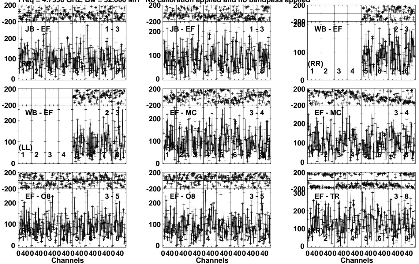
Lower frame: Micro Ampl Jy Top frame: Phas deg Vector averaged cross-power spectrum Several baselines displayed Timerange: 00/17:30:31 to 00/17:33:59
