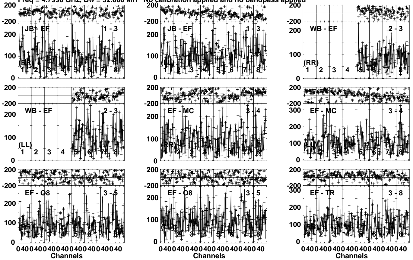
Lower frame: Micro Ampl Jy Top frame: Phas deg Vector averaged cross-power spectrum Several baselines displayed Timerange: 00/14:54:31 to 00/14:57:59
