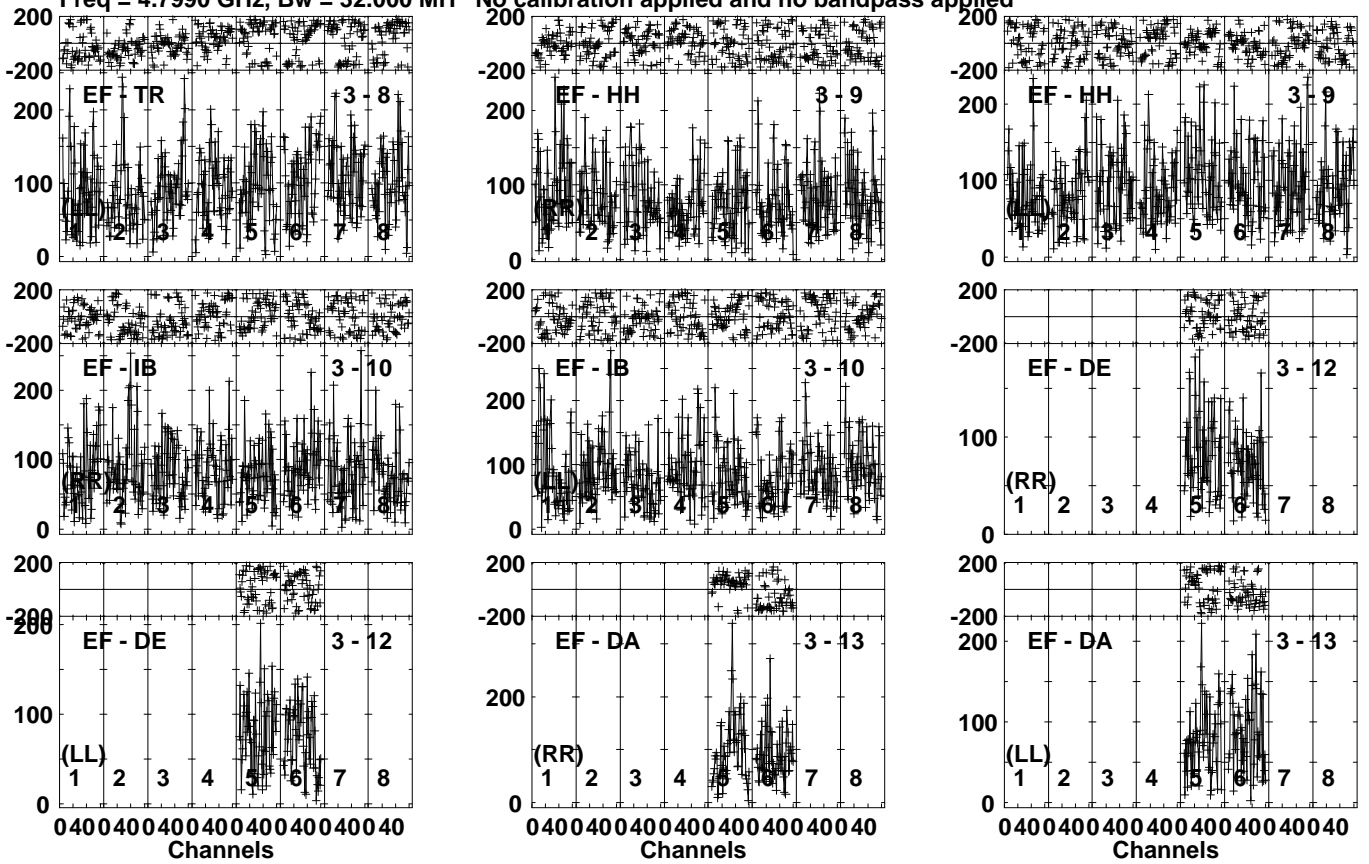
Lower frame: Micro Ampl Jy Top frame: Phas deg Vector averaged cross-power spectrum Several baselines displayed Timerange: 00/14:59:33 to 00/15:02:59
