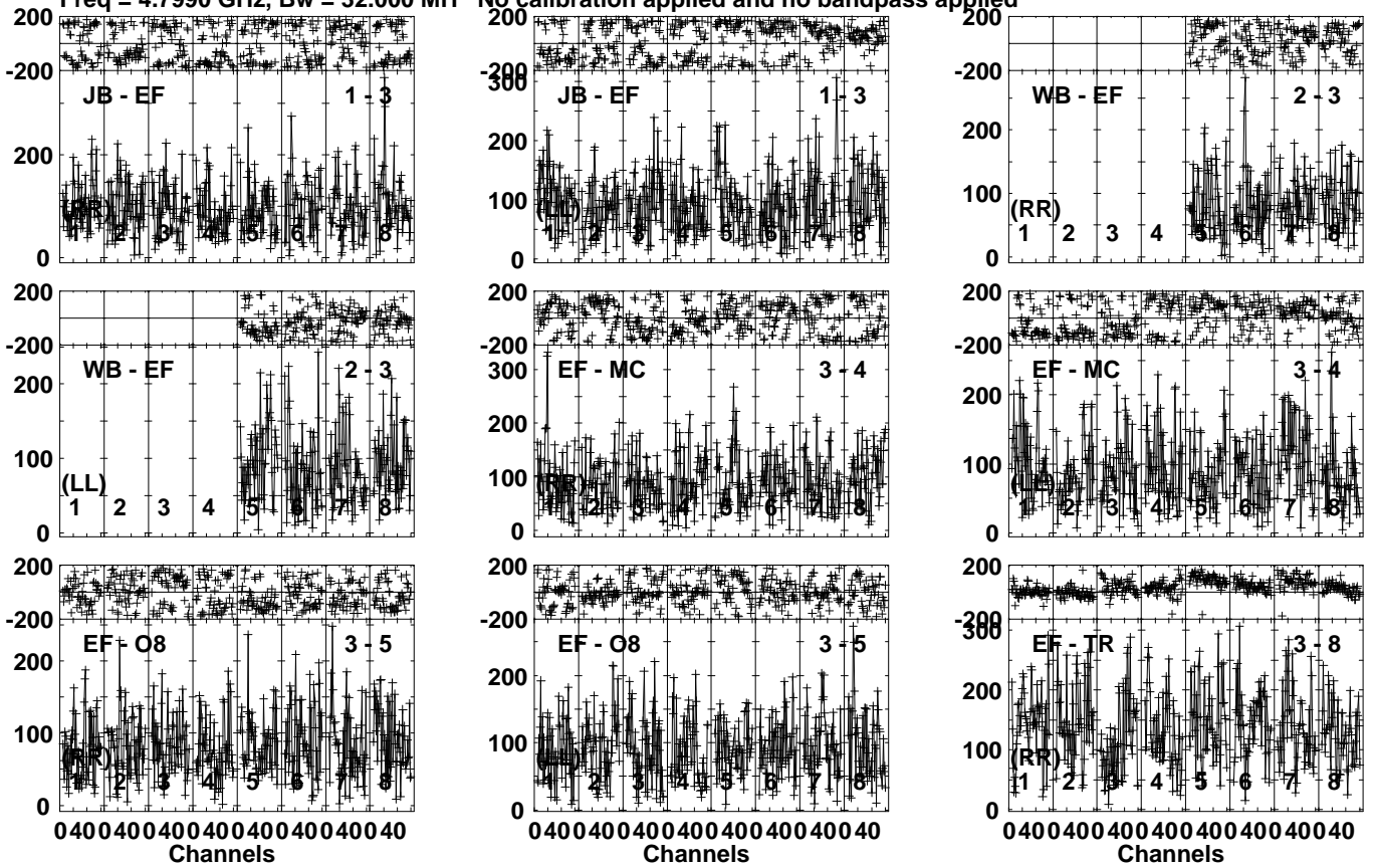
Lower frame: Micro Ampl Jy Top frame: Phas deg Vector averaged cross-power spectrum Several baselines displayed Timerange: 00/18:24:01 to 00/18:27:29
