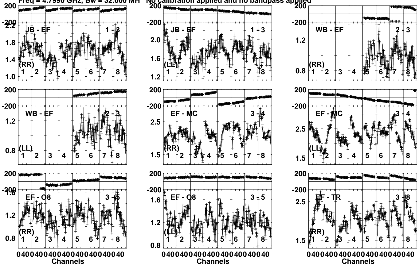
Lower frame: Milli Ampl Jy Top frame: Phas deg Vector averaged cross-power spectrum Several baselines displayed Timerange: 00/17:07:31 to 00/17:11:29
