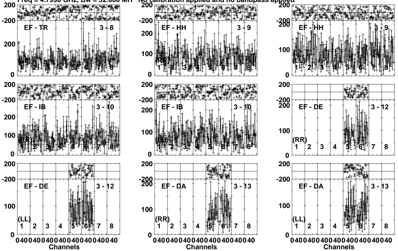
Lower frame: Micro Ampl Jy Top frame: Phas deg Vector averaged cross-power spectrum Several baselines displayed Timerange: 00/15:04:31 to 00/15:07:59
