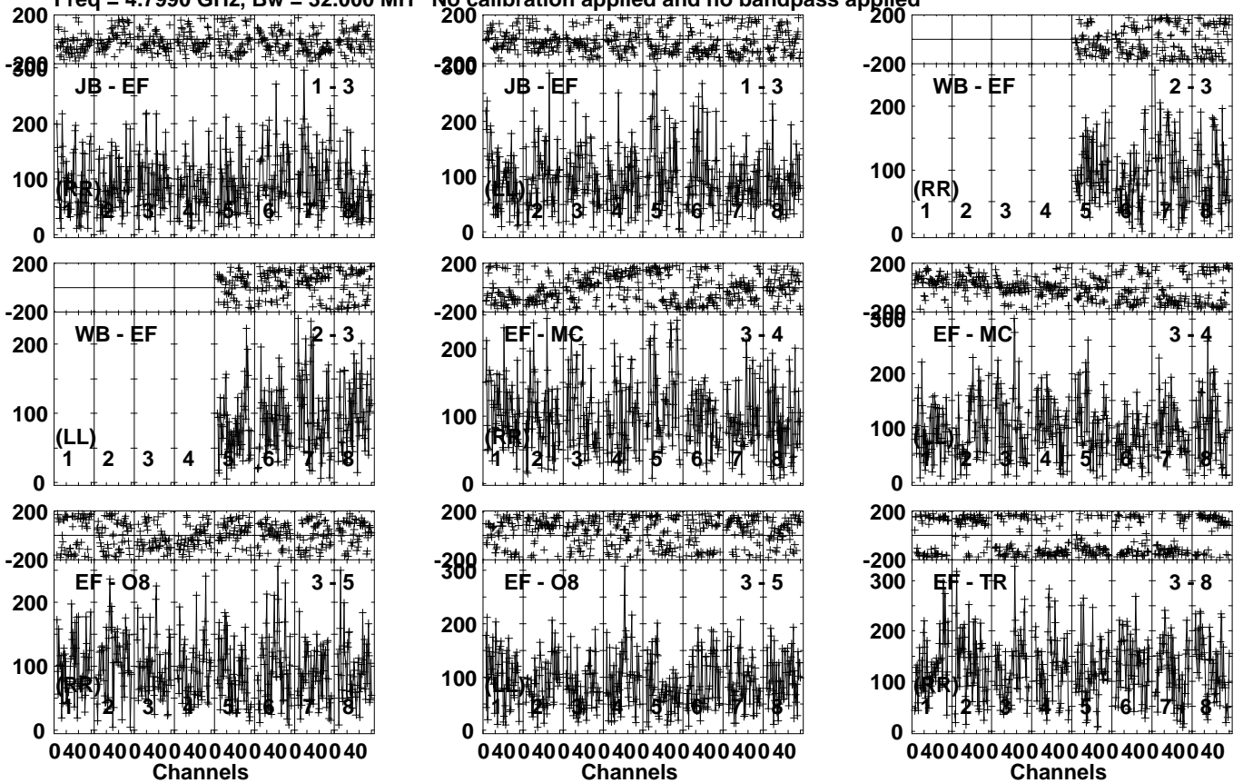
Lower frame: Micro Ampl Jy Top frame: Phas deg Vector averaged cross-power spectrum Several baselines displayed Timerange: 00/17:35:31 to 00/17:38:59
