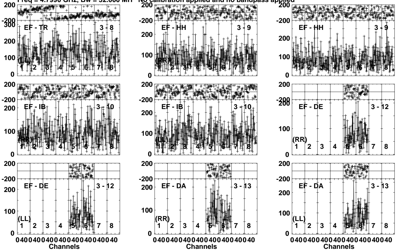
Lower frame: Micro Ampl Jy Top frame: Phas deg Vector averaged cross-power spectrum Several baselines displayed Timerange: 00/17:25:31 to 00/17:28:59
