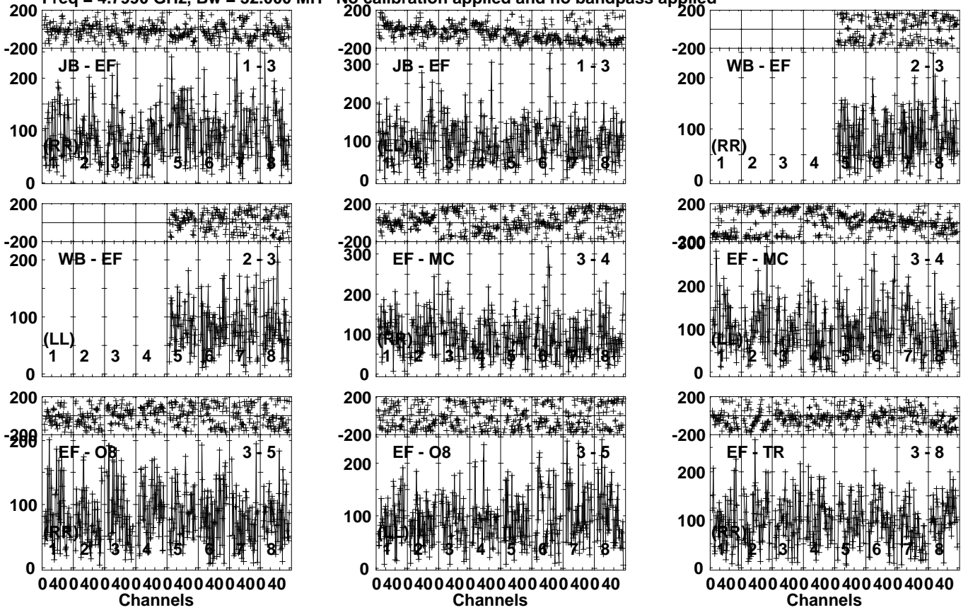
Lower frame: Micro Ampl Jy Top frame: Phas deg Vector averaged cross-power spectrum Several baselines displayed Timerange: 00/15:33:31 to 00/15:36:59
