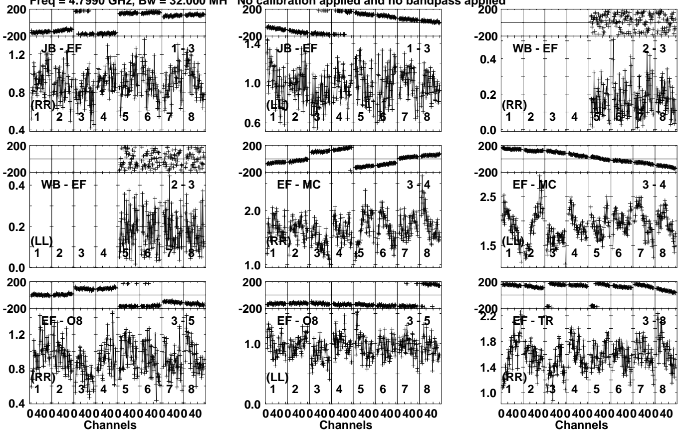
Lower frame: Milli Ampl Jy Top frame: Phas deg Vector averaged cross-power spectrum Several baselines displayed Timerange: 00/13:59:31 to 00/14:00:59
