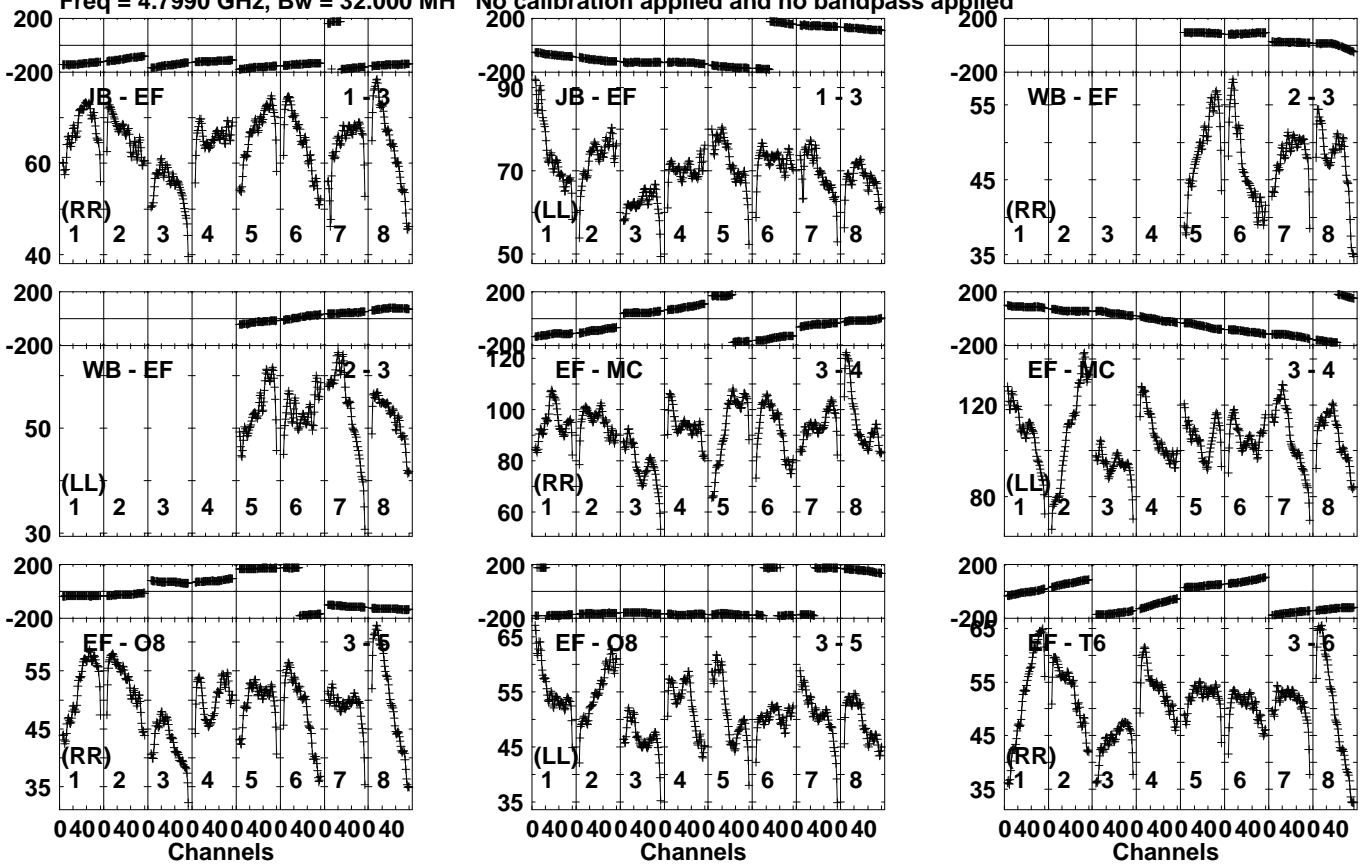
Lower frame: Milli Ampl Jy Top frame: Phas deg Vector averaged cross-power spectrum Several baselines displayed Timerange: 00/17:50:31 to 00/17:55:59
