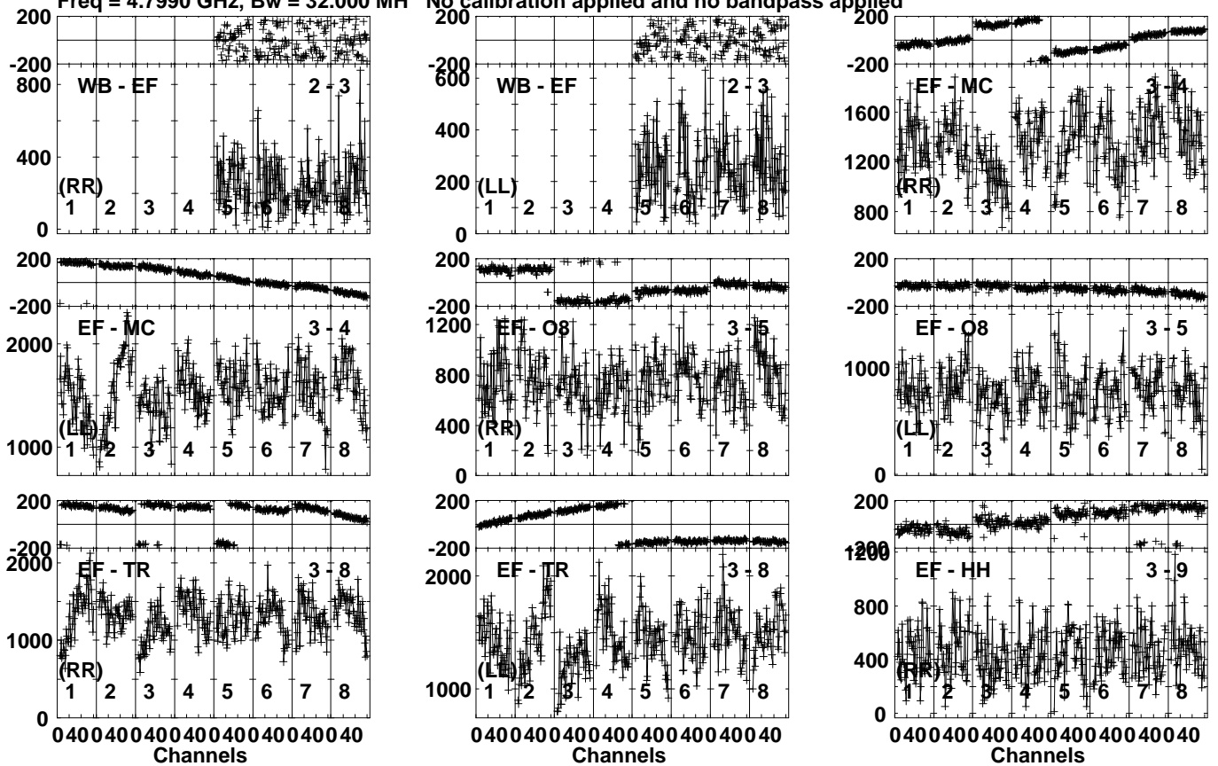
Lower frame: Micro Ampl Jy Top frame: Phas deg Vector averaged cross-power spectrum Several baselines displayed Timerange: 00/13:46:01 to 00/13:46:59
