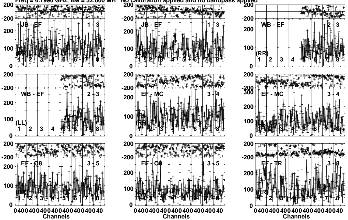
Lower frame: Micro Ampl Jy Top frame: Phas deg Vector averaged cross-power spectrum Several baselines displayed Timerange: 00:18:43:01 to 00:18:46:29
