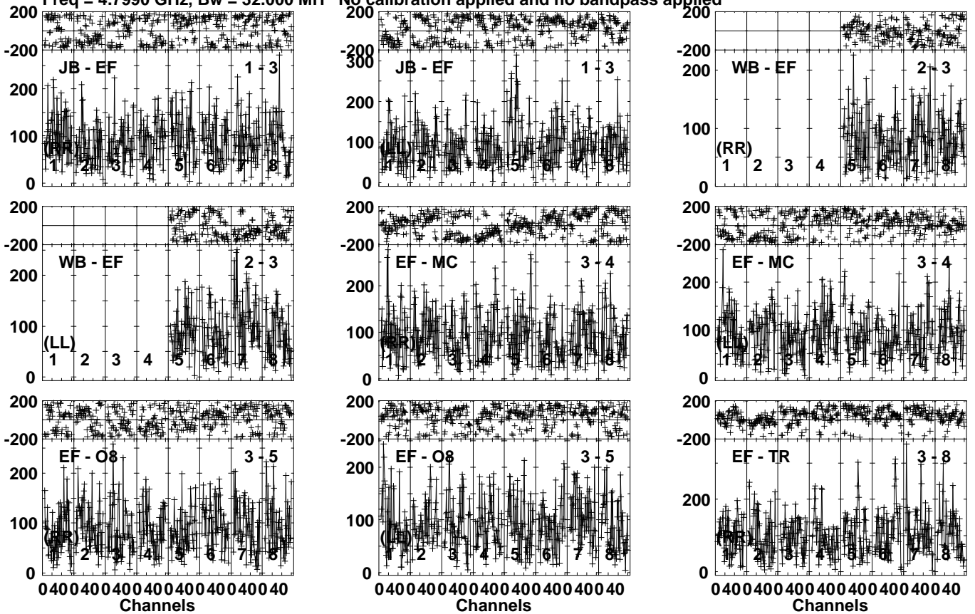
Lower frame: Micro Ampl Jy Top frame: Phas deg Vector averaged cross-power spectrum Several baselines displayed Timerange: 00/16:46:01 to 00/16:49:29
