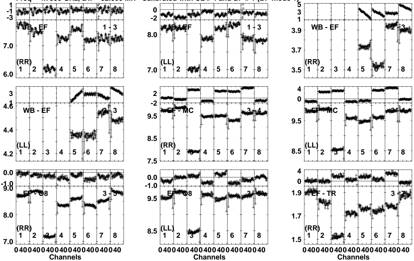
Lower frame: Ampl Jy Top frame: Phas deg Vector averaged cross-power spectrum Several baselines displayed Timerange: 00/18:26:01 to 00/18:29:59
