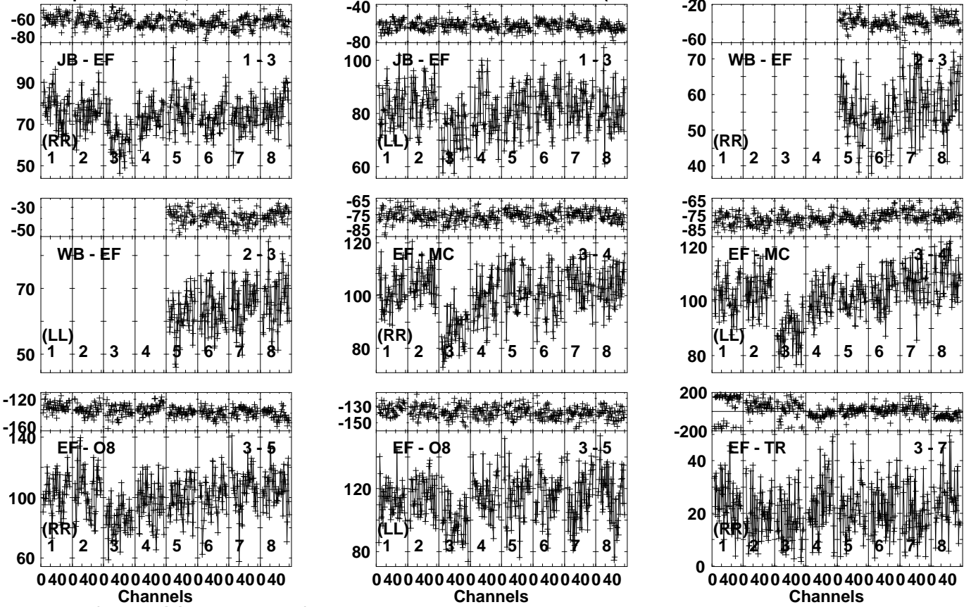
Lower frame: Milli Ampl Jy Top frame: Phas deg Vector averaged cross-power spectrum Several baselines displayed Timerange: 00/16:18:01 to 00/16:20:29
