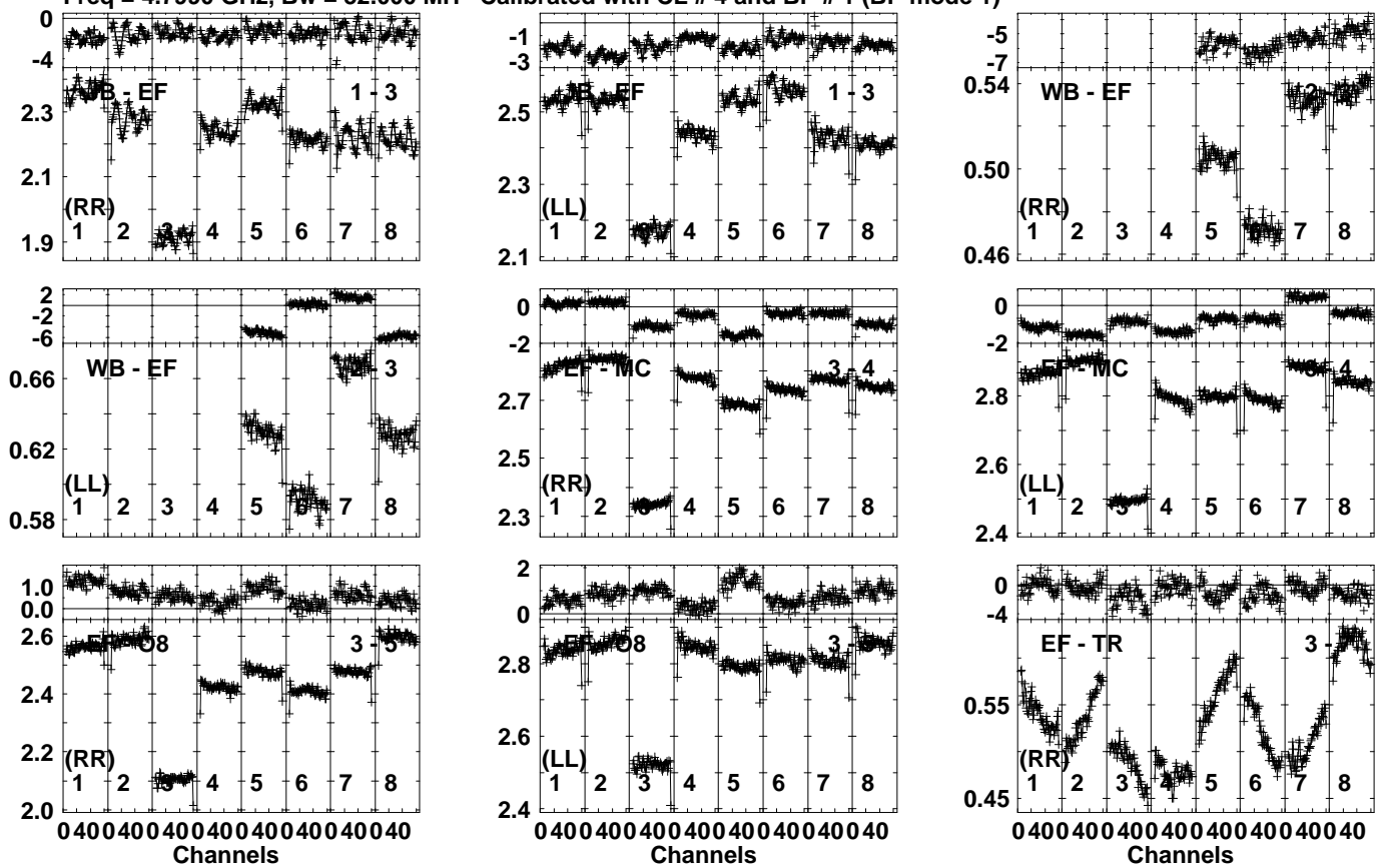
Lower frame: Ampl Jy Top frame: Phas deg Vector averaged cross-power spectrum Several baselines displayed Timerange: 00/15:41:01 to 00/15:46:29
