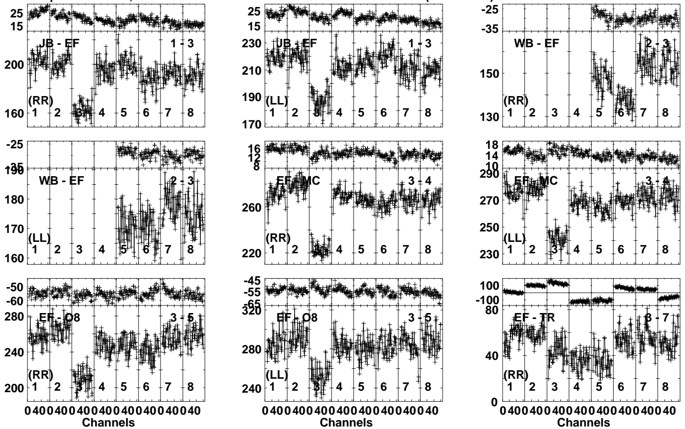
Lower frame: Milli Ampl Jy Top frame: Phas deg Vector averaged cross-power spectrum Several baselines displayed Timerange: 00/15:54:01 to 00/15:57:29
