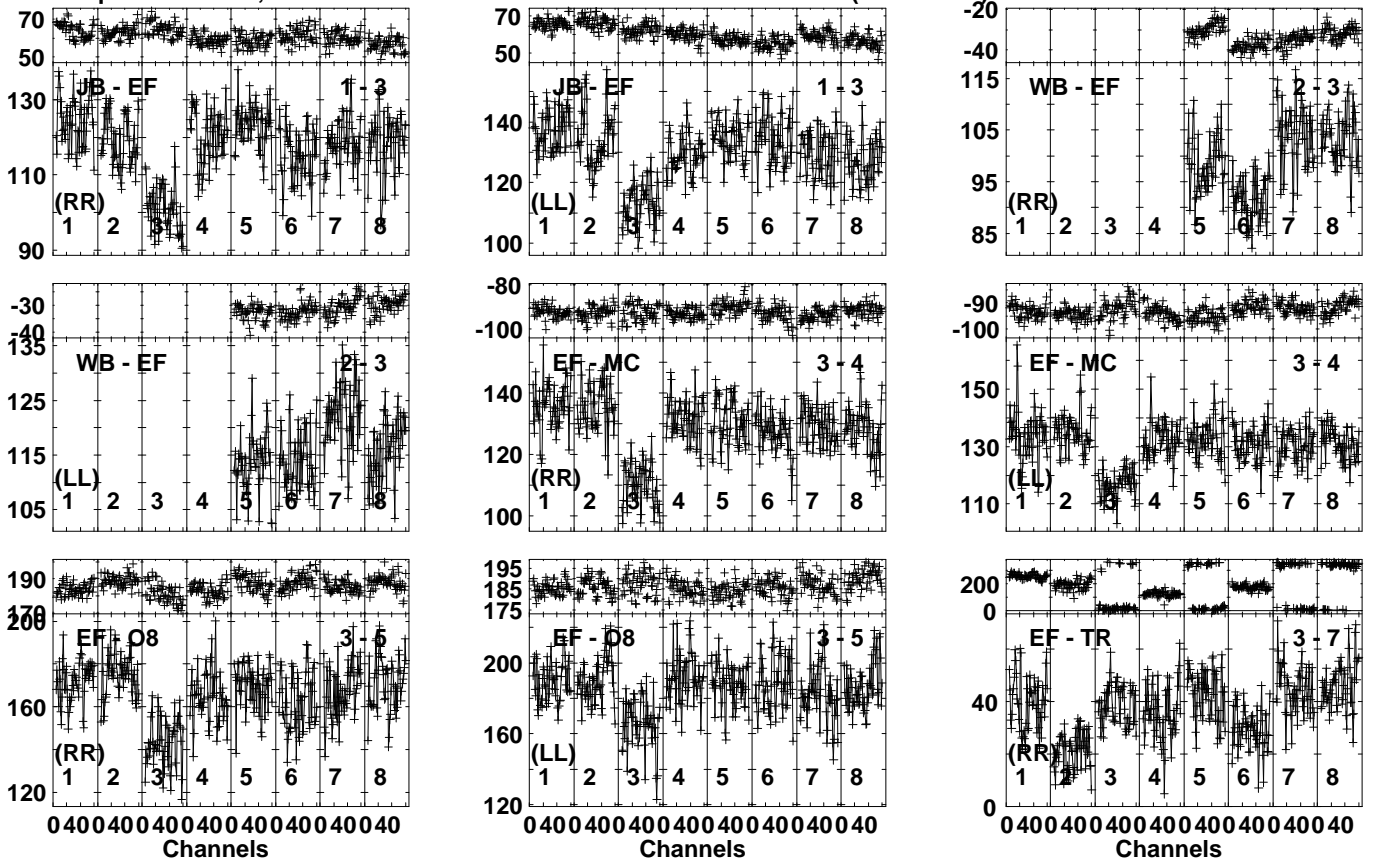
Lower frame: Milli Ampl Jy Top frame: Phas deg Vector averaged cross-power spectrum Several baselines displayed Timerange: 00:18:20:01 to 00:18:23:29
