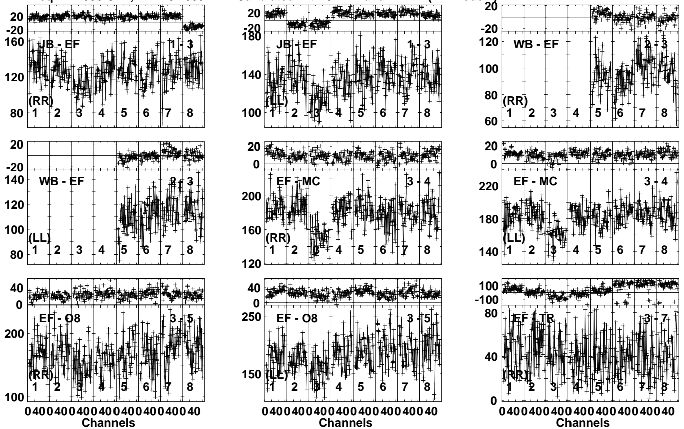
Lower frame: Milli Ampl Jy Top frame: Phas deg Vector averaged cross-power spectrum Several baselines displayed Timerange: 00/13:52:01 to 00/13:53:29
