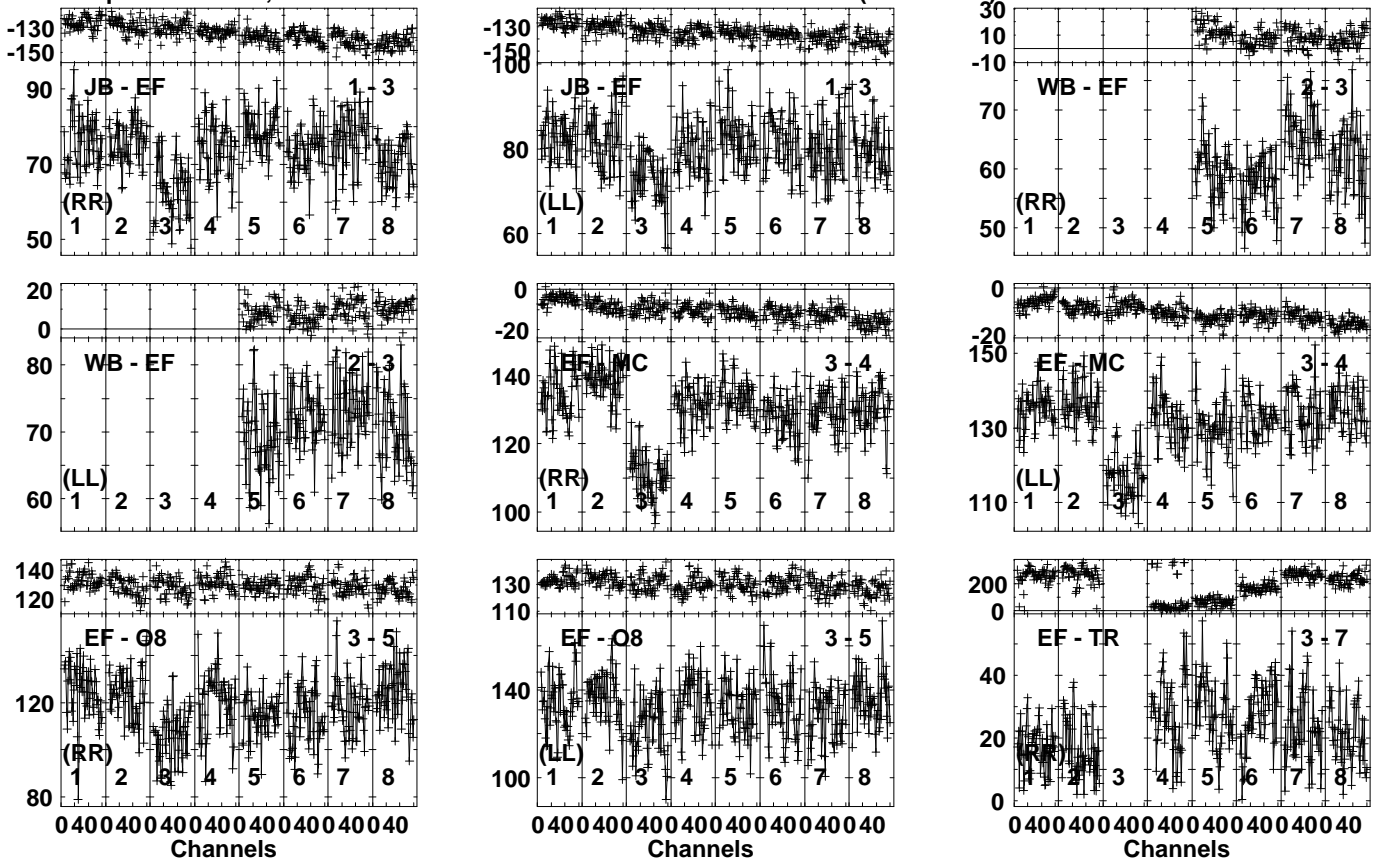
Lower frame: Milli Ampl Jy Top frame: Phas deg Vector averaged cross-power spectrum Several baselines displayed Timerange: 00/13:44:31 to 00/13:47:59
