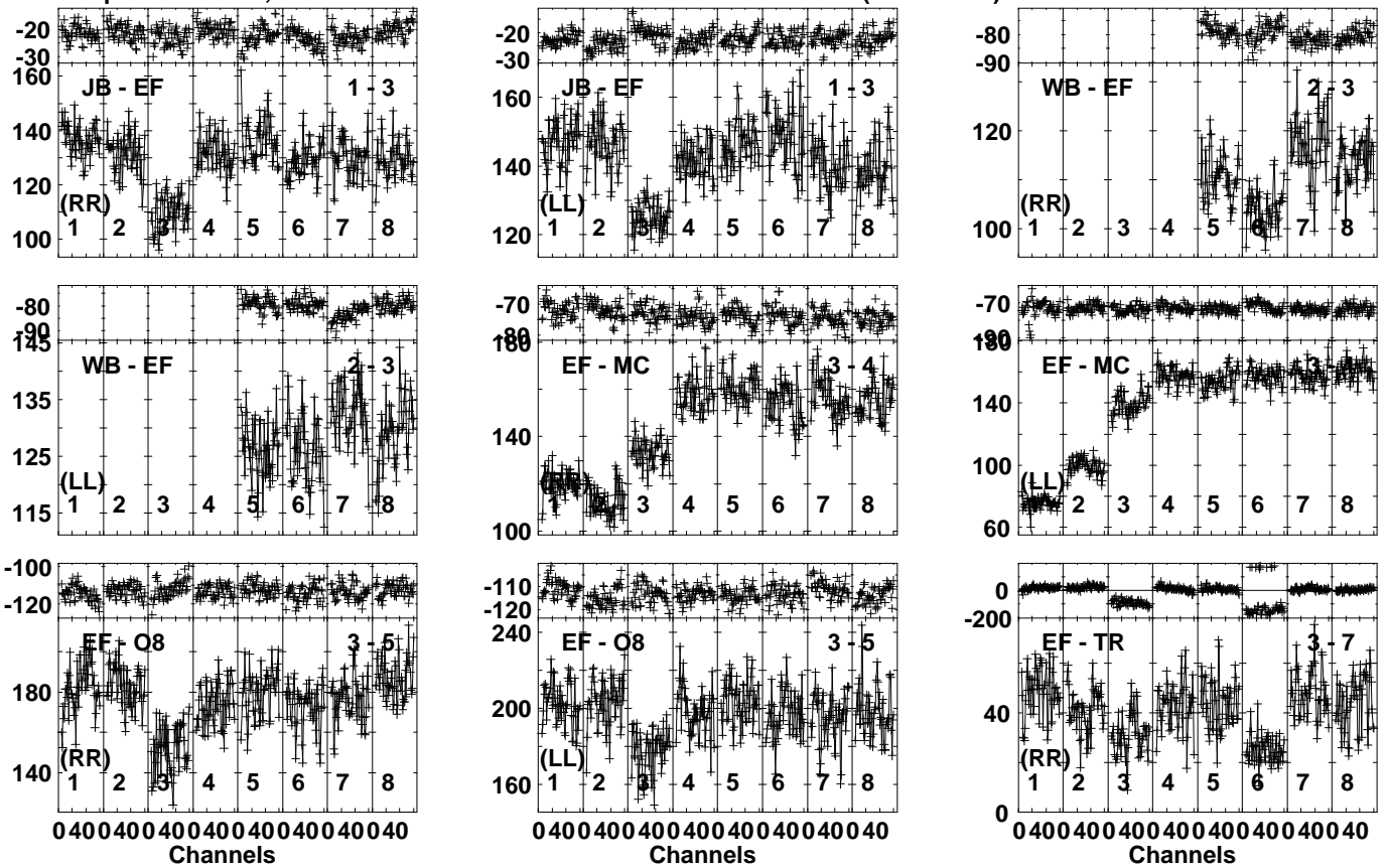
Lower frame: Milli Ampl Jy Top frame: Phas deg Vector averaged cross-power spectrum Several baselines displayed Timerange: 00:18:05:01 to 00:18:08:29
