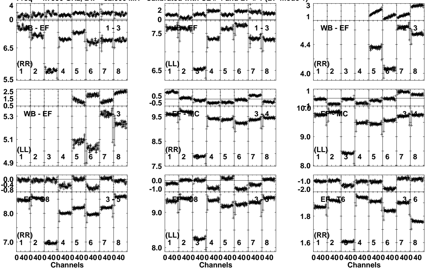
Lower frame: Ampl Jy Top frame: Phas deg Vector averaged cross-power spectrum Several baselines displayed Timerange: 00/17:17:31 to 00/17:22:59
