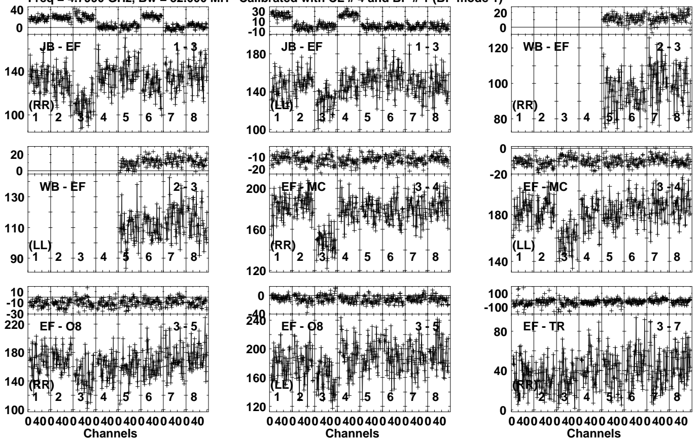
Lower frame: Milli Ampl Jy Top frame: Phas deg Vector averaged cross-power spectrum Several baselines displayed Timerange: 00/15:18:01 to 00/15:19:29
