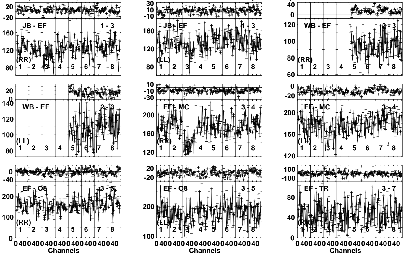
Lower frame: Milli Ampl Jy Top frame: Phas deg Vector averaged cross-power spectrum Several baselines displayed Timerange: 00/14:04:01 to 00/14:04:59
