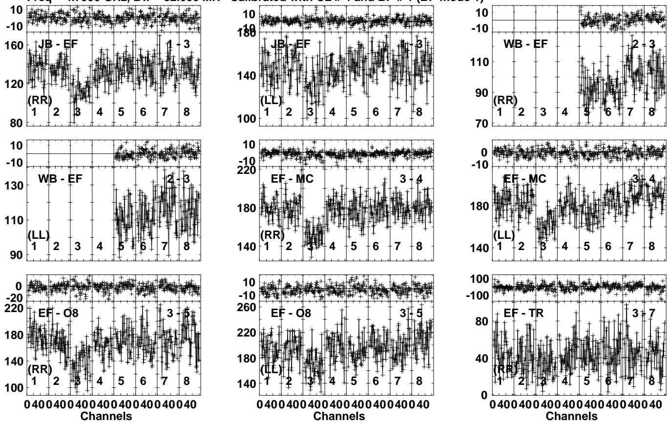
Lower frame: Milli Ampl Jy Top frame: Phas deg Vector averaged cross-power spectrum Several baselines displayed Timerange: 00/15:58:01 to 00/15:58:59
