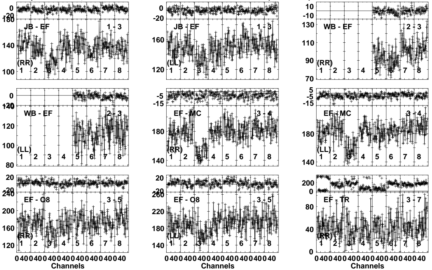
Lower frame: Milli Ampl Jy Top frame: Phas deg Vector averaged cross-power spectrum Several baselines displayed Timerange: 00/17:10:01 to 00/17:11:29
