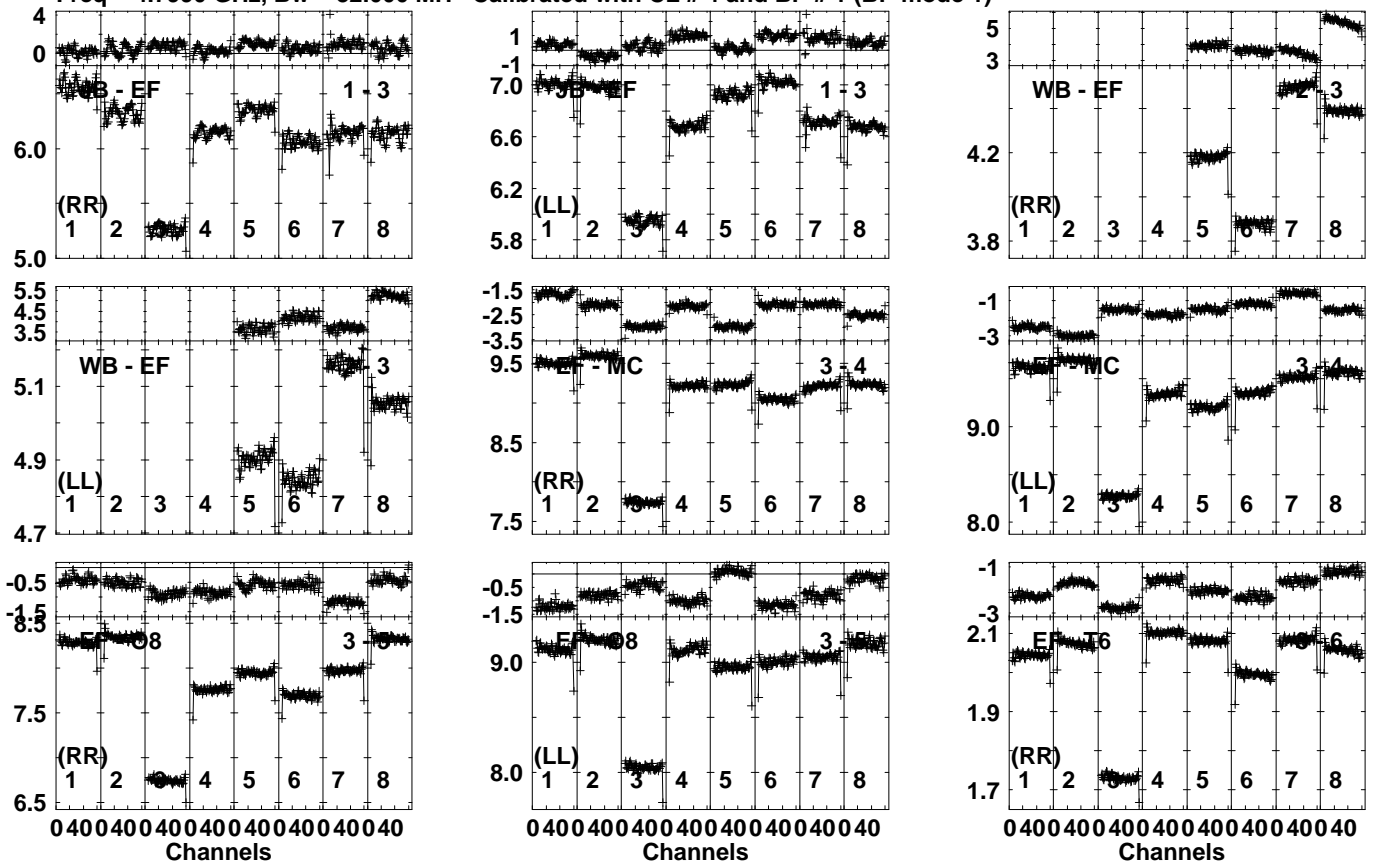
Lower frame: Ampl Jy Top frame: Phas deg Vector averaged cross-power spectrum Several baselines displayed Timerange: 00/16:28:01 to 00/16:33:29
