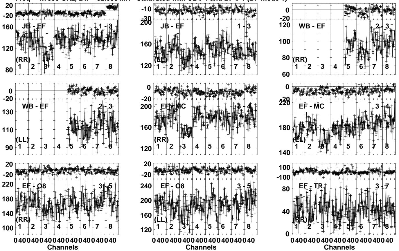
Lower frame: Milli Ampl Jy Top frame: Phas deg Vector averaged cross-power spectrum Several baselines displayed Timerange: 00:16:42:01 to 00:16:43:29
