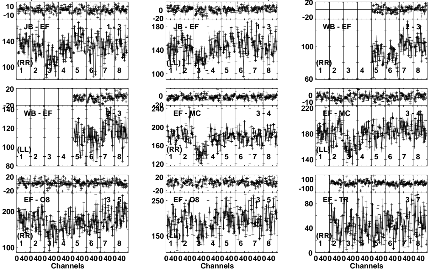
Lower frame: Milli Ampl Jy Top frame: Phas deg Vector averaged cross-power spectrum Several baselines displayed Timerange: 00/16:56:31 to 00/16:57:29
