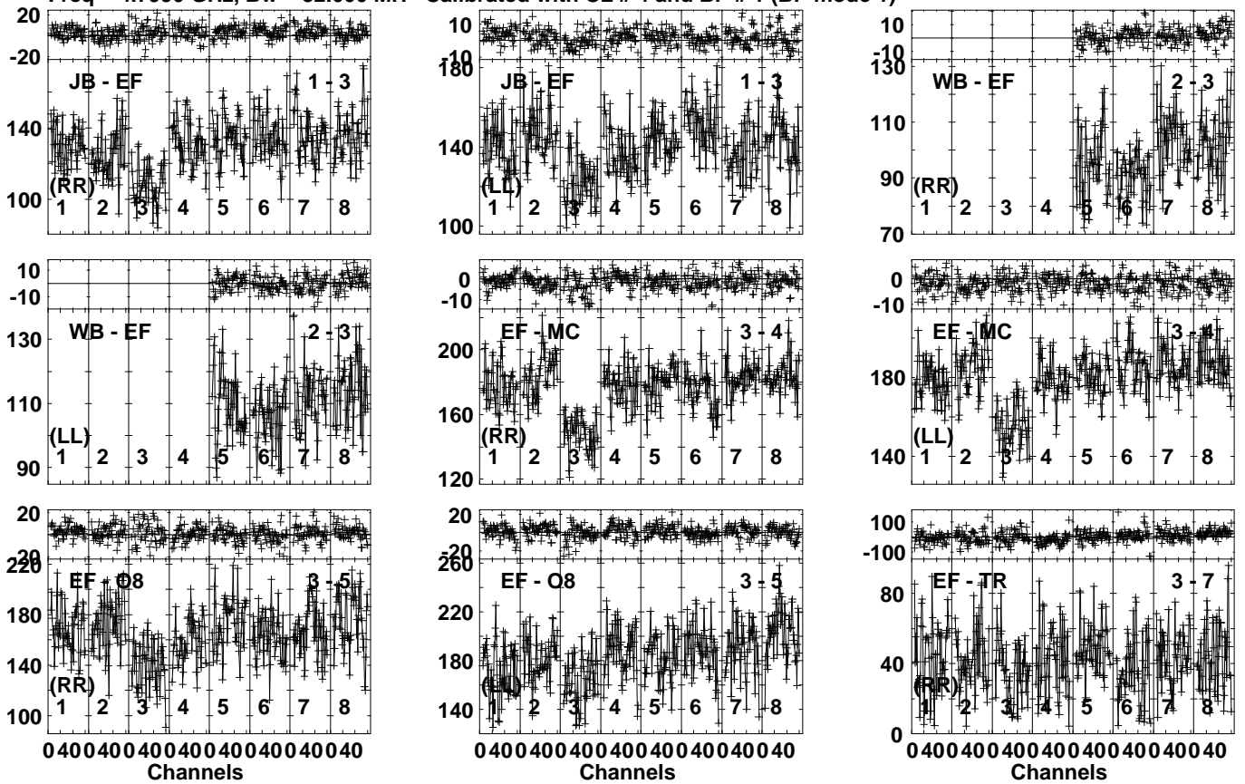
Lower frame: Milli Ampl Jy Top frame: Phas deg Vector averaged cross-power spectrum Several baselines displayed Timerange: 00/14:25:31 to 00/14:26:29
