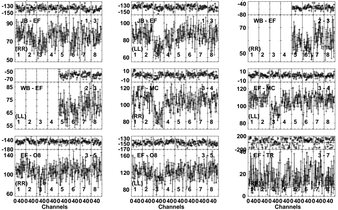
Lower frame: Milli Ampl Jy Top frame: Phas deg Vector averaged cross-power spectrum Several baselines displayed Timerange: 00/15:24:31 to 00/15:26:59
