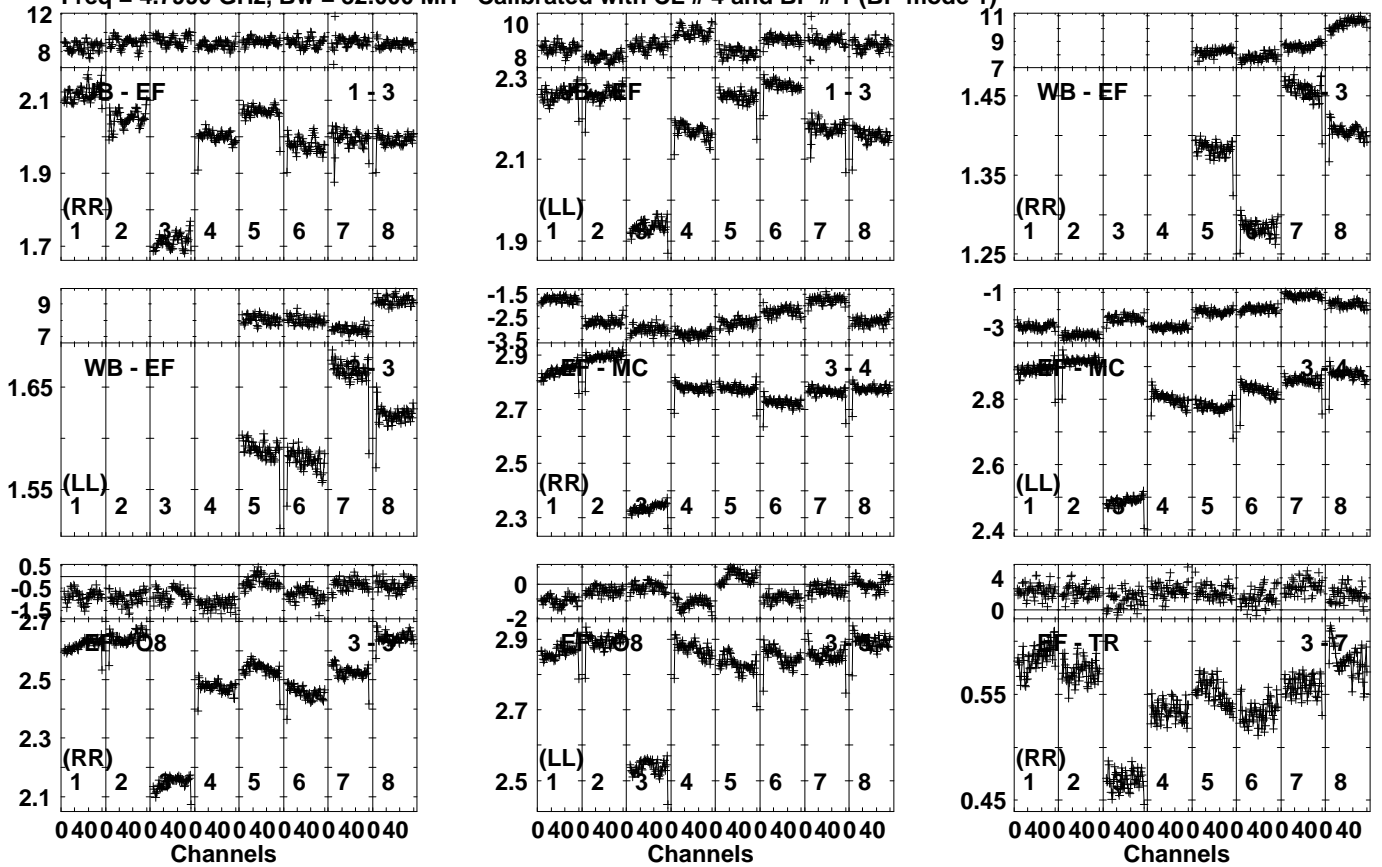
Lower frame: Ampl Jy Top frame: Phas deg Vector averaged cross-power spectrum Several baselines displayed Timerange: 00/13:59:01 to 00/14:02:59
