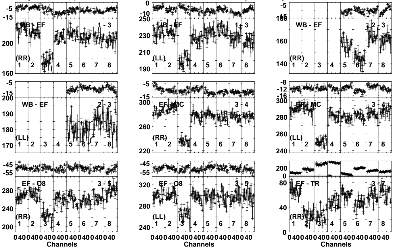
Lower frame: Milli Ampl Jy Top frame: Phas deg Vector averaged cross-power spectrum Several baselines displayed Timerange: 00:16:03:01 to 00:16:06:29
