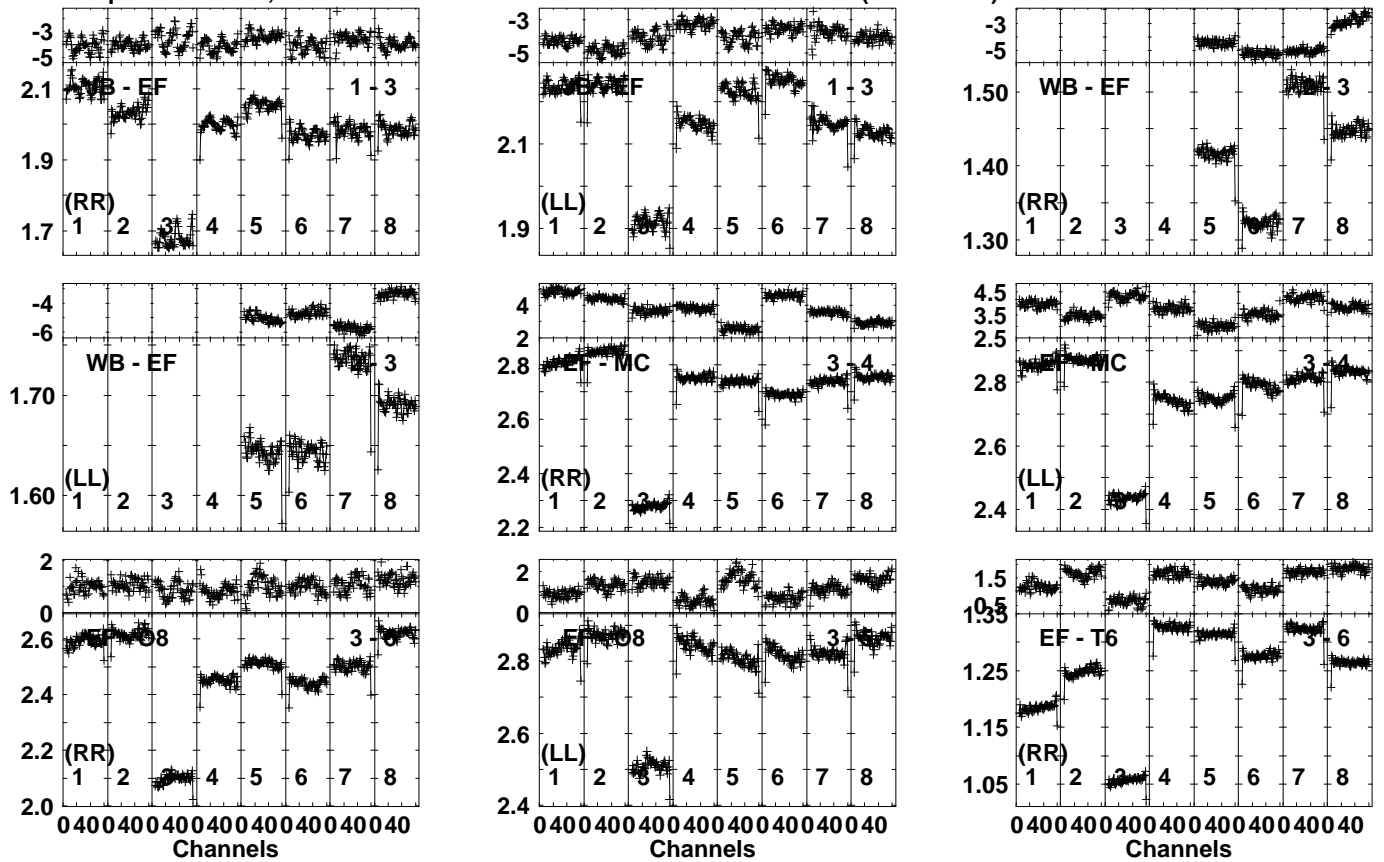
Lower frame: Ampl Jy Top frame: Phas deg Vector averaged cross-power spectrum Several baselines displayed Timerange: 00/13:33:31 to 00/13:37:29
