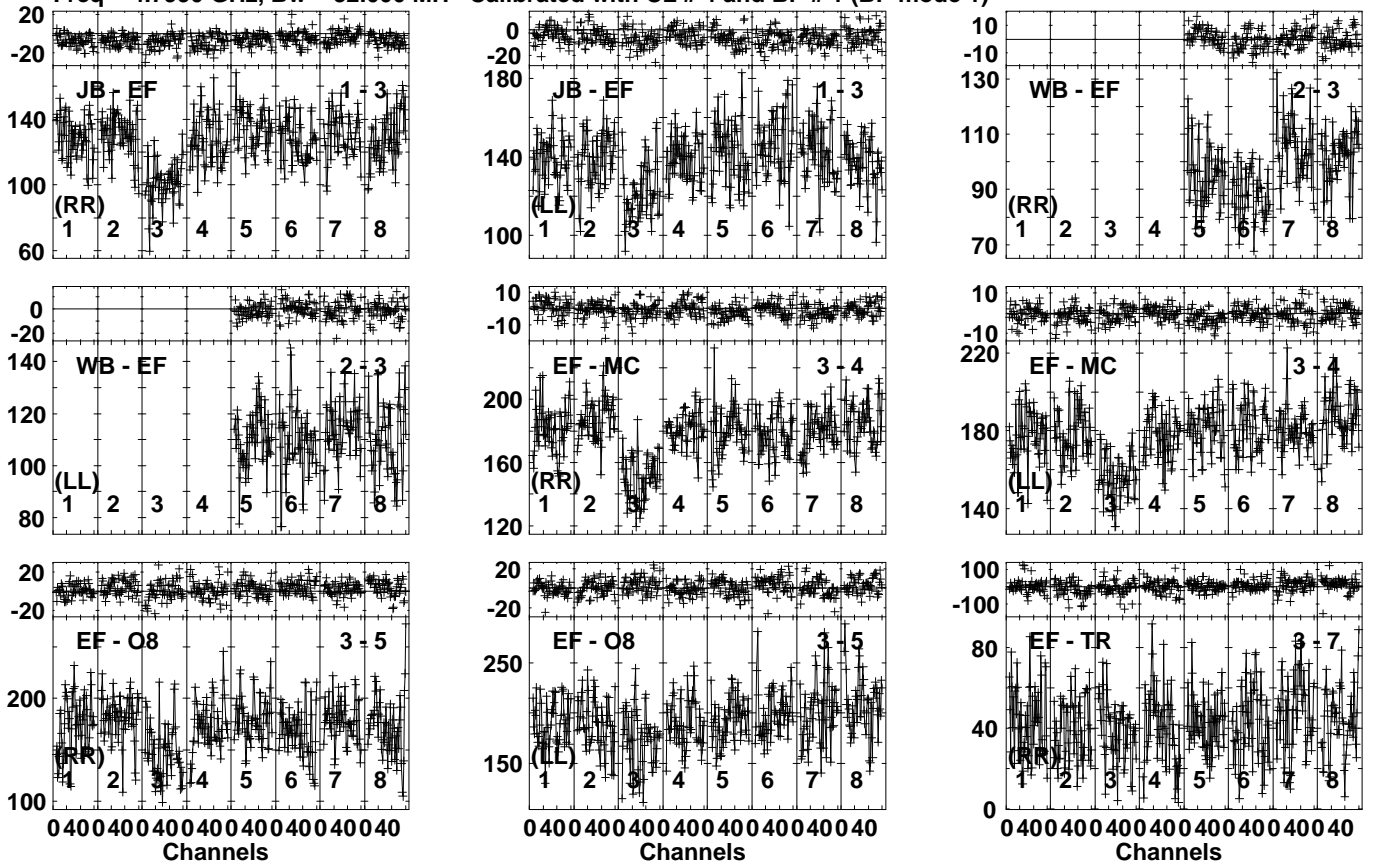
Lower frame: Milli Ampl Jy Top frame: Phas deg Vector averaged cross-power spectrum Several baselines displayed Timerange: 00:17:41:01 to 00:17:41:59
