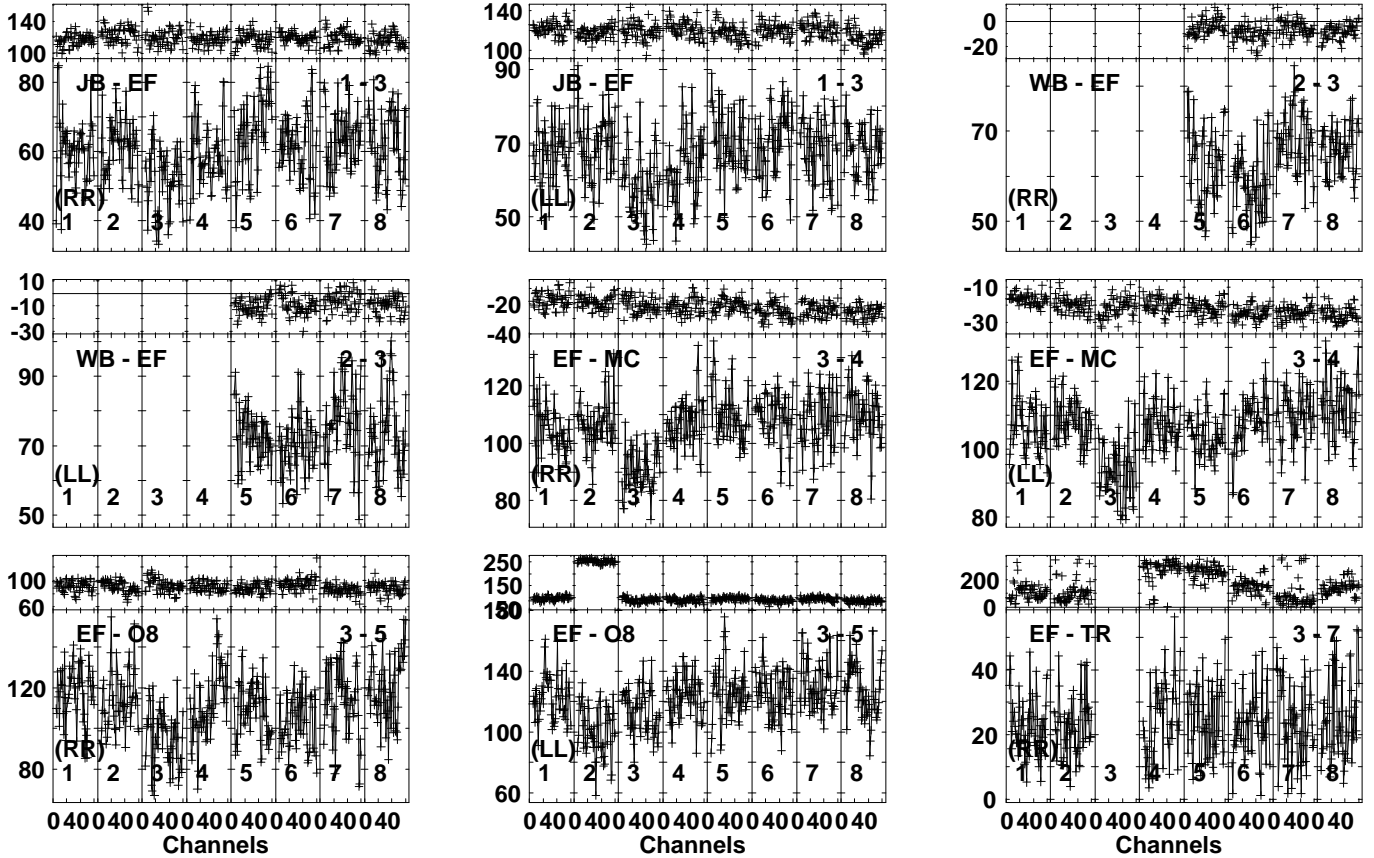
Lower frame: Milli Ampl Jy Top frame: Phas deg Vector averaged cross-power spectrum Several baselines displayed Timerange: 00/13:49:31 to 00/13:51:59
