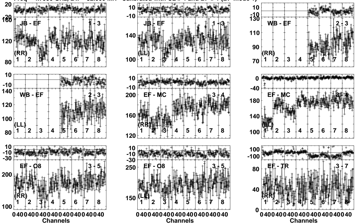
Lower frame: Milli Ampl Jy Top frame: Phas deg Vector averaged cross-power spectrum Several baselines displayed Timerange: 00:18:13:31 to 00:18:14:59
