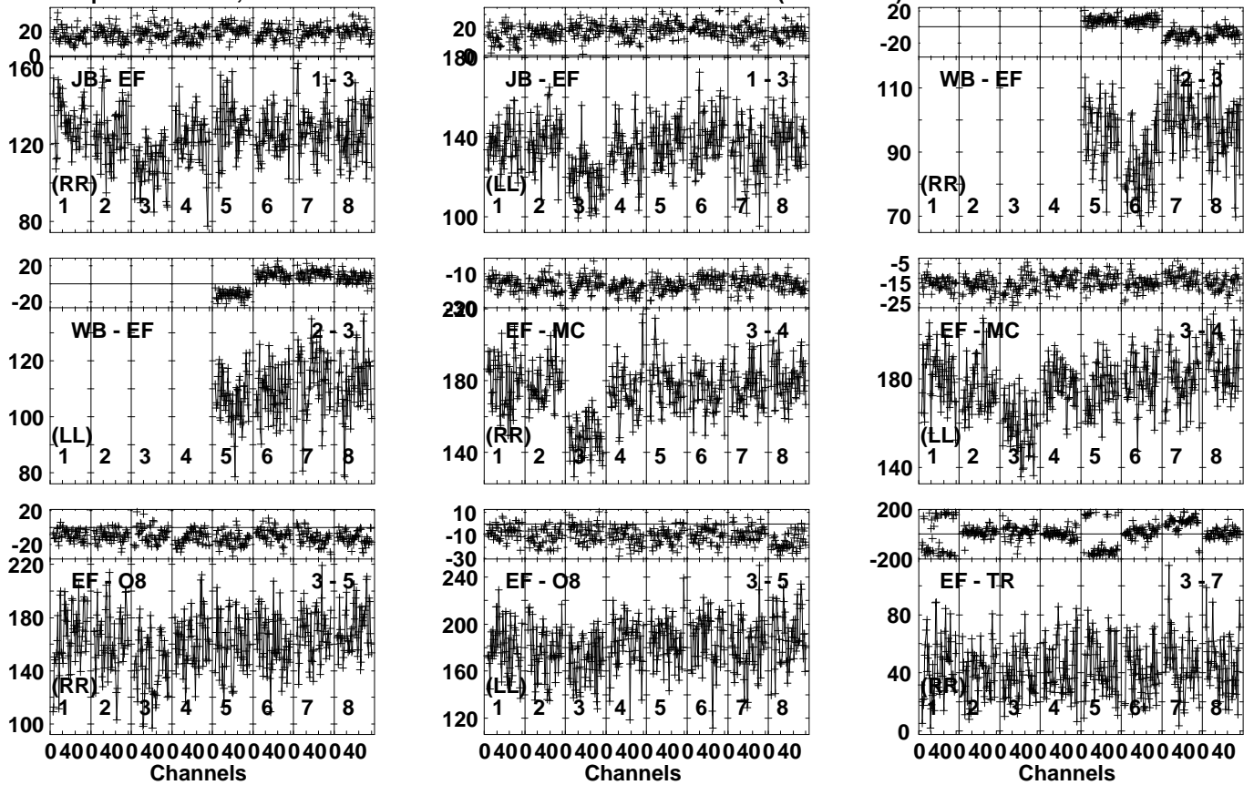
Lower frame: Milli Ampl Jy Top frame: Phas deg Vector averaged cross-power spectrum Several baselines displayed Timerange: 00/14:11:01 to 00/14:12:29
