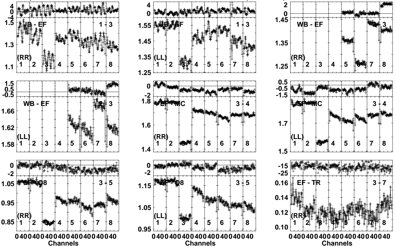
Lower frame: Ampl Jy Top frame: Phas deg Vector averaged cross-power spectrum Several baselines displayed Timerange: 00/12:27:07 to 00/12:31:59
