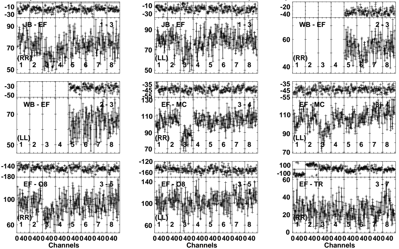
Lower frame: Milli Ampl Jy Top frame: Phas deg Vector averaged cross-power spectrum Several baselines displayed Timerange: 00:17:07:31 to 00:17:09:59
