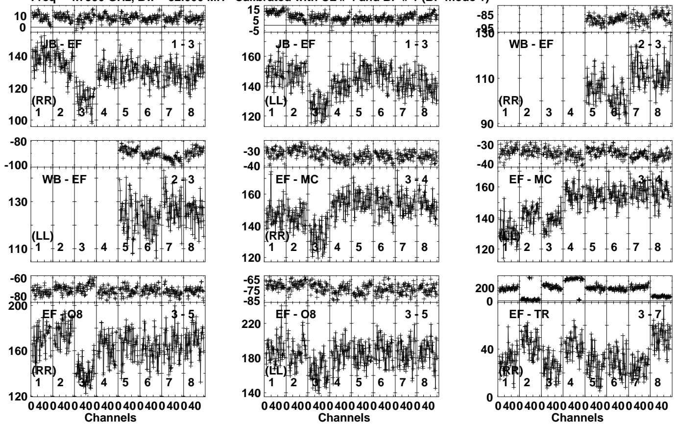
Lower frame: Milli Ampl Jy Top frame: Phas deg Vector averaged cross-power spectrum Several baselines displayed Timerange: 00/17:56:01 to 00/17:59:29
