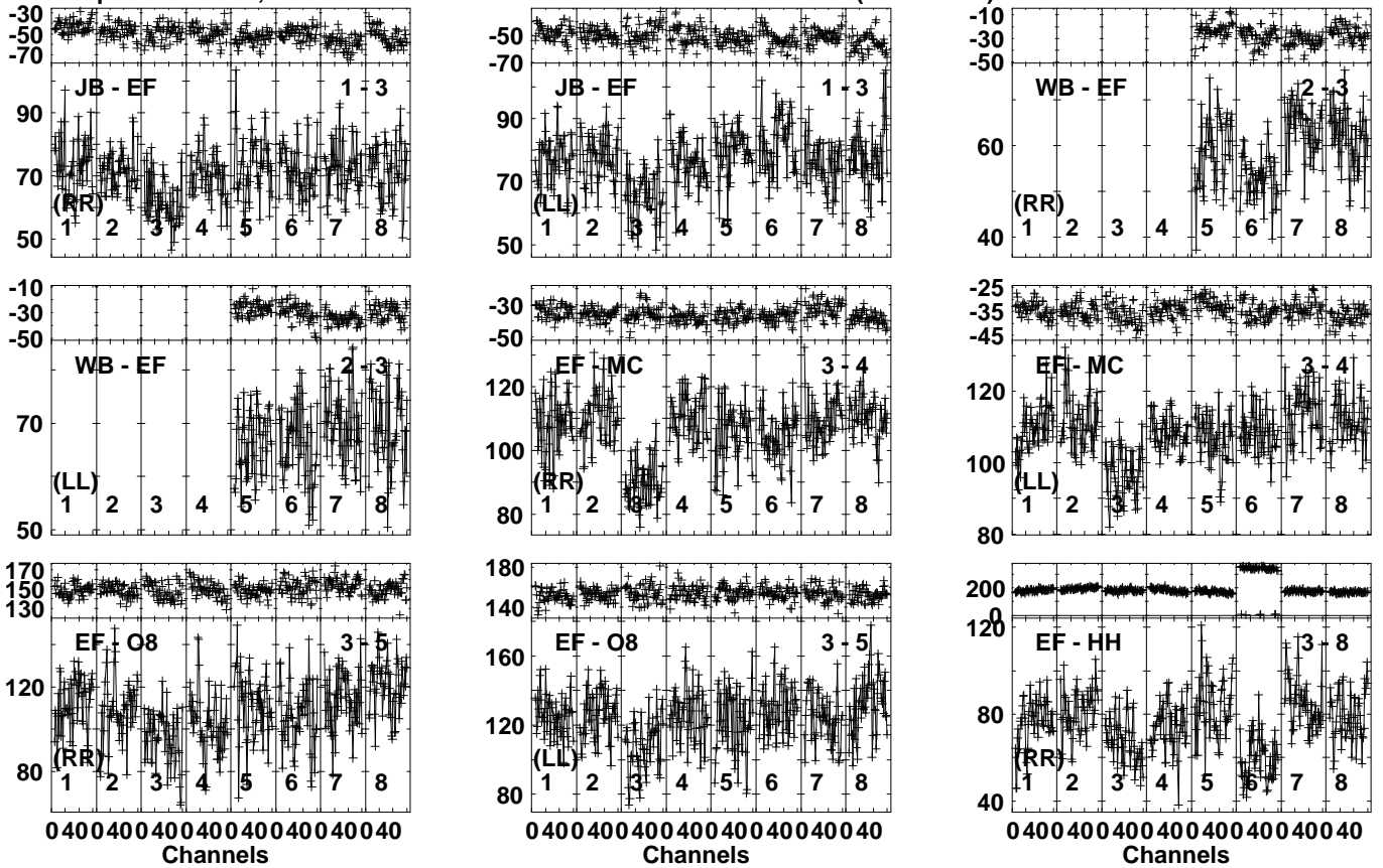
Lower frame: Milli Ampl Jy Top frame: Phas deg Vector averaged cross-power spectrum Several baselines displayed Timerange: 00/14:36:31 to 00/14:38:59
