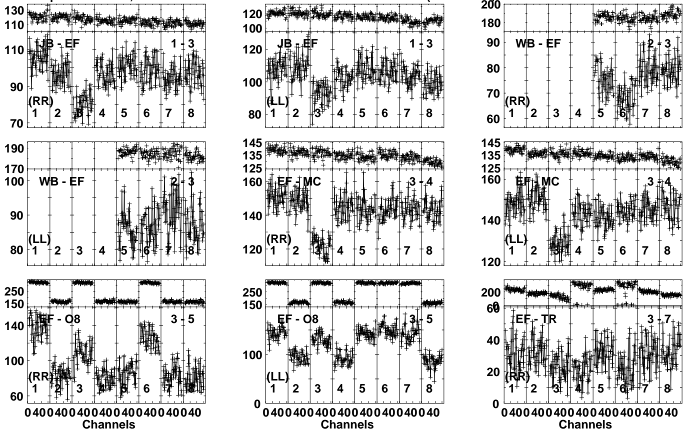
Lower frame: Milli Ampl Jy Top frame: Phas deg Vector averaged cross-power spectrum Several baselines displayed Timerange: 00/14:07:31 to 00/14:10:59
