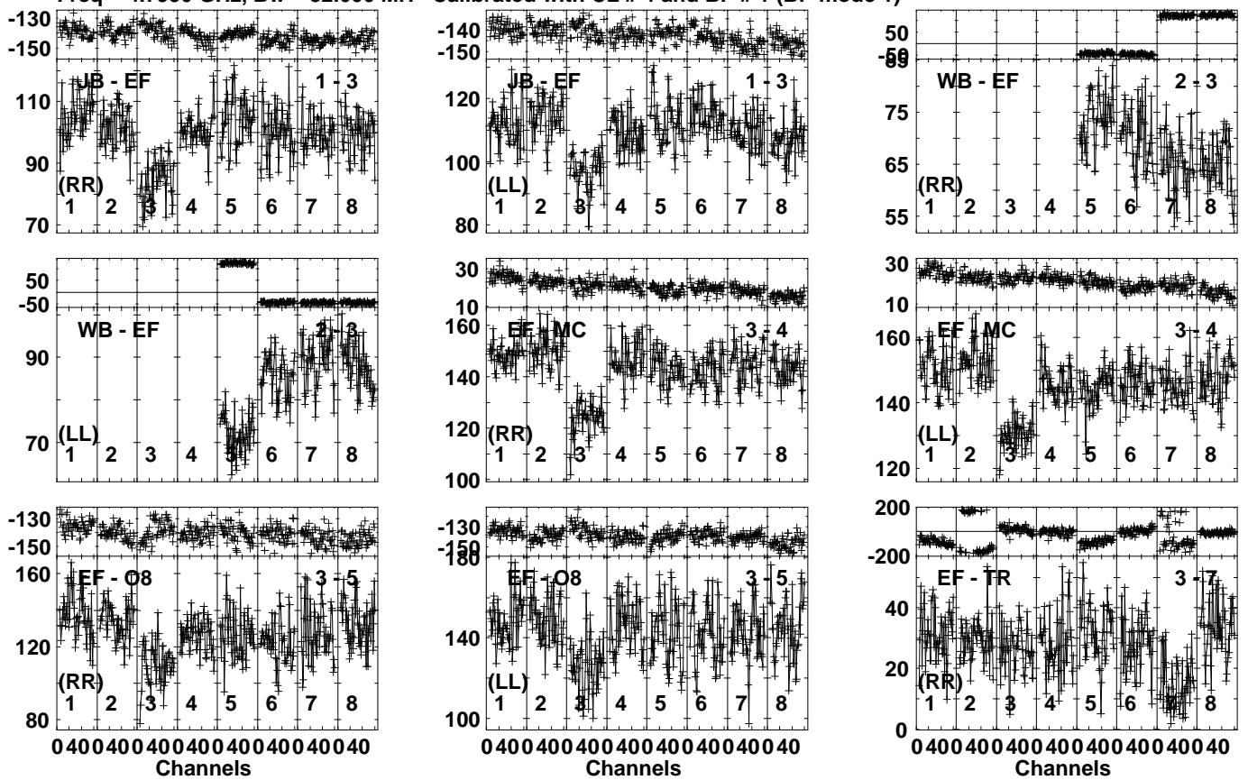
Lower frame: Milli Ampl Jy Top frame: Phas deg Vector averaged cross-power spectrum Several baselines displayed Timerange: 00/14:12:31 to 00/14:15:59
