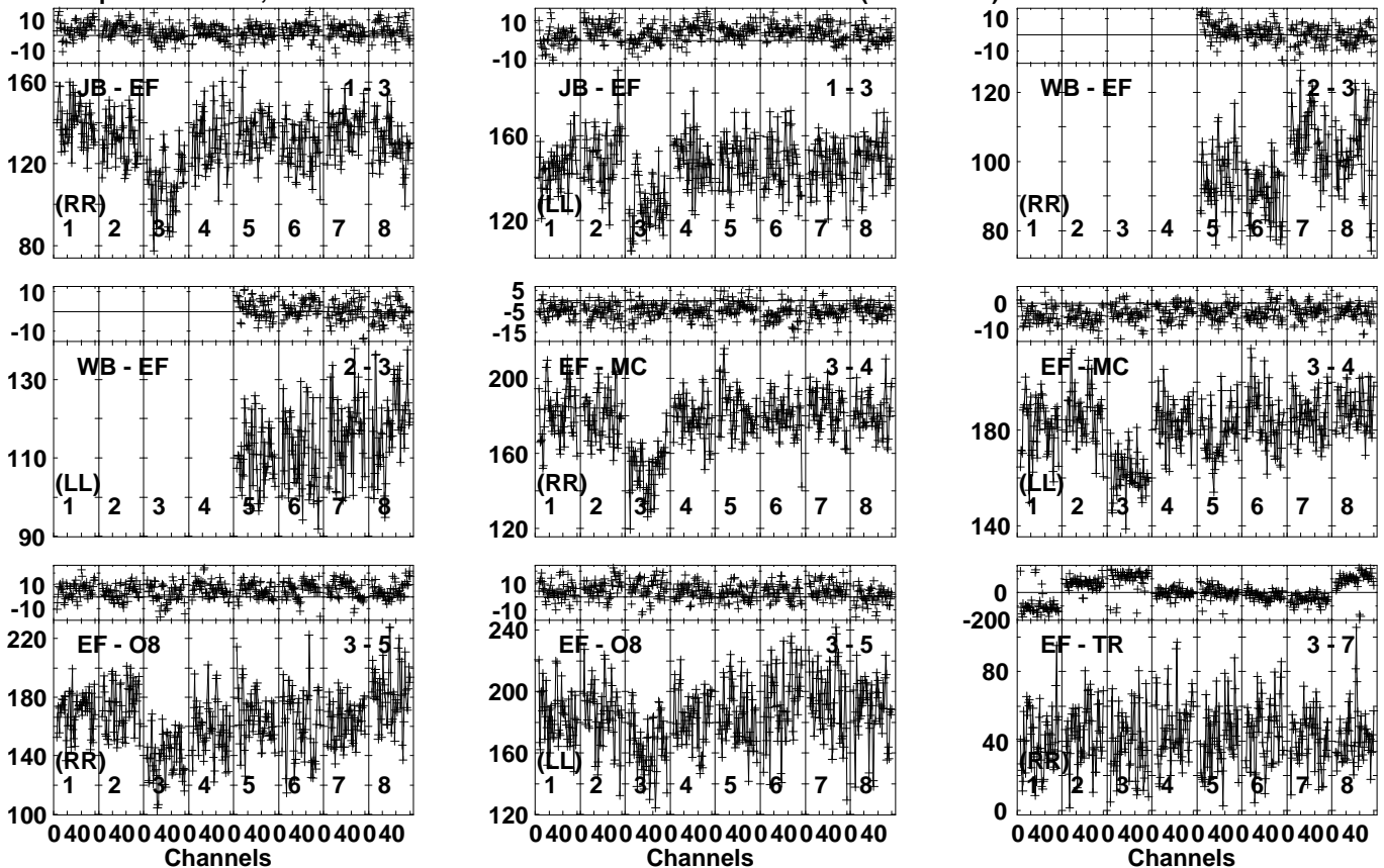
Lower frame: Milli Ampl Jy Top frame: Phas deg Vector averaged cross-power spectrum Several baselines displayed Timerange: 00/15:52:31 to 00/15:53:59
