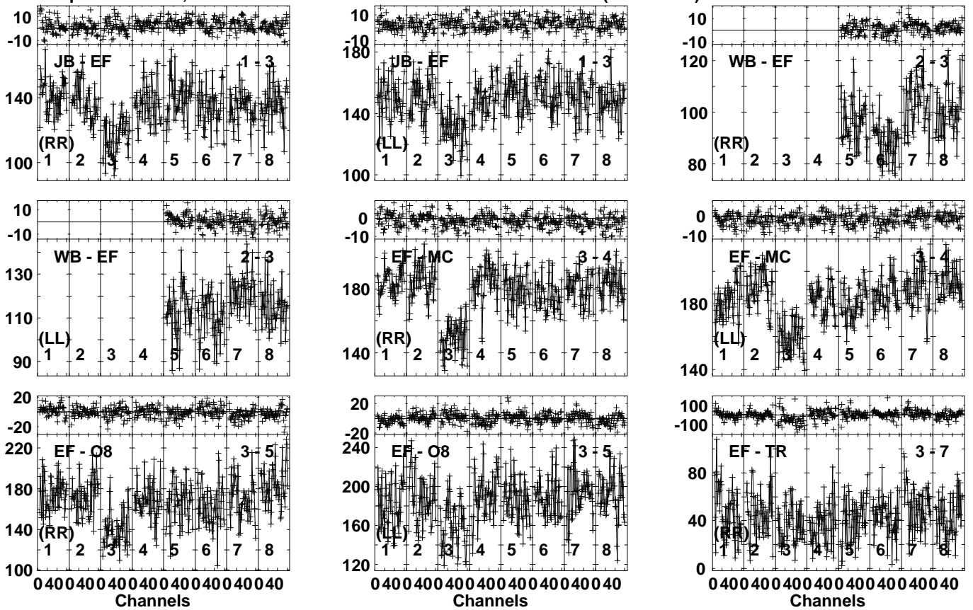
Lower frame: Milli Ampl Jy Top frame: Phas deg Vector averaged cross-power spectrum Several baselines displayed Timerange: 00/15:32:31 to 00/15:33:29
