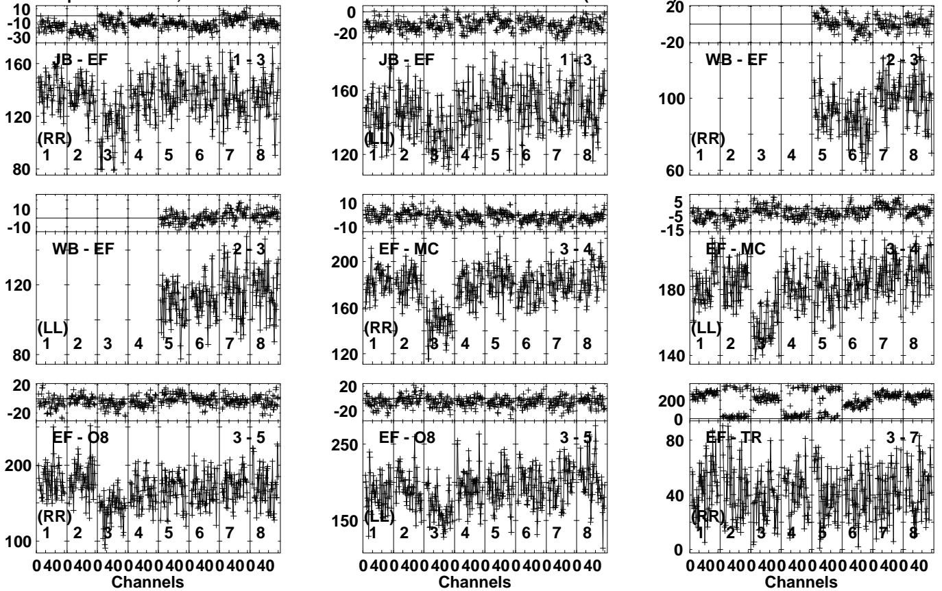
Lower frame: Milli Ampl Jy Top frame: Phas deg Vector averaged cross-power spectrum Several baselines displayed Timerange: 00/17:01:01 to 00/17:02:29
