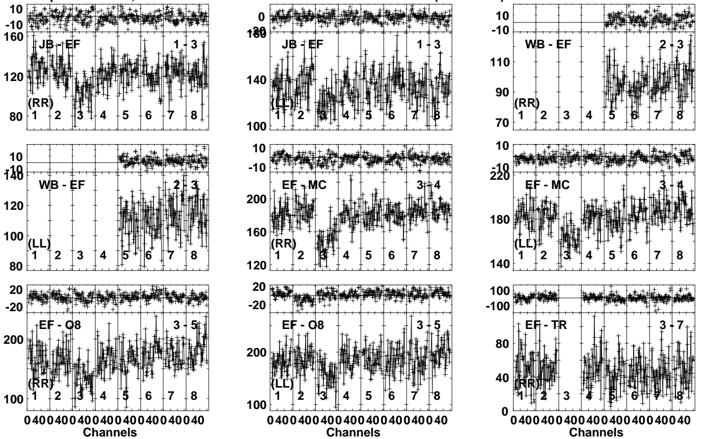
Lower frame: Milli Ampl Jy Top frame: Phas deg Vector averaged cross-power spectrum Several baselines displayed Timerange: 00/13:48:31 to 00/13:49:29
