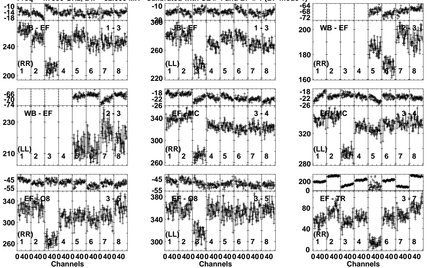
Lower frame: Milli Ampl Jy Top frame: Phas deg Vector averaged cross-power spectrum Several baselines displayed Timerange: 00:16:22:01 to 00:16:25:29
