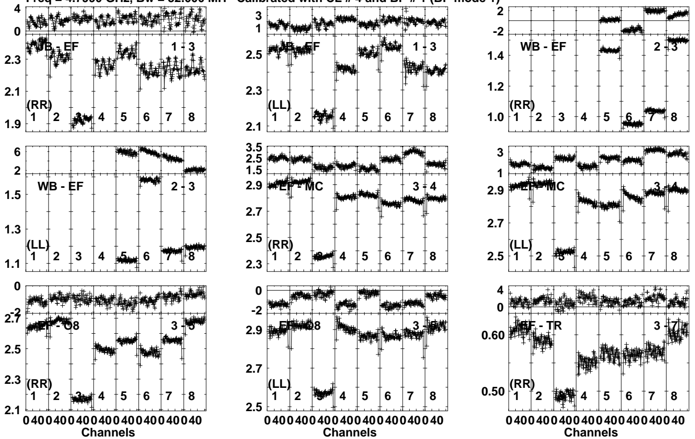
Lower frame: Ampl Jy Top frame: Phas deg Vector averaged cross-power spectrum Several baselines displayed Timerange: 00/17:24:01 to 00/17:29:29
