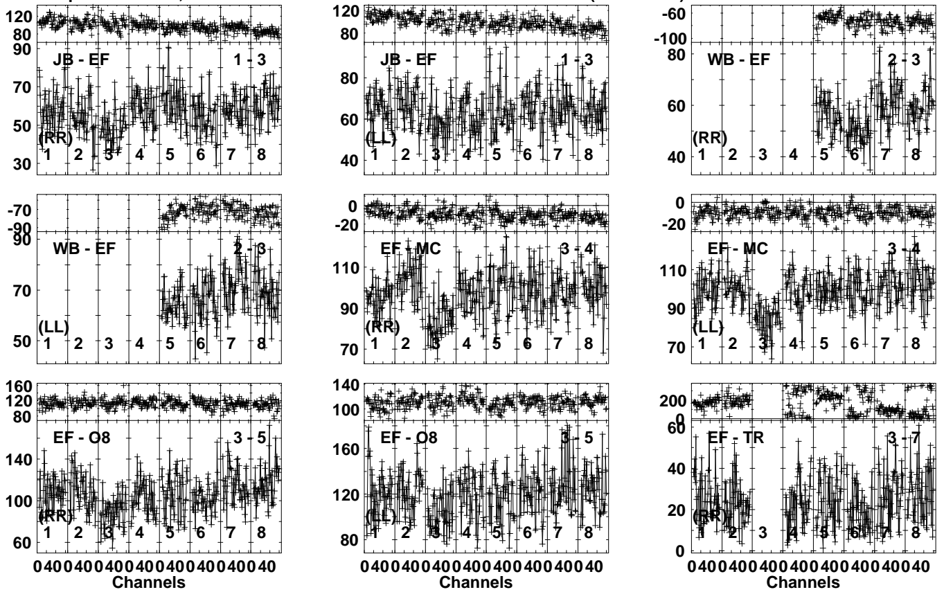
Lower frame: Milli Ampl Jy Top frame: Phas deg Vector averaged cross-power spectrum Several baselines displayed Timerange: 00/13:24:01 to 00/13:26:29
