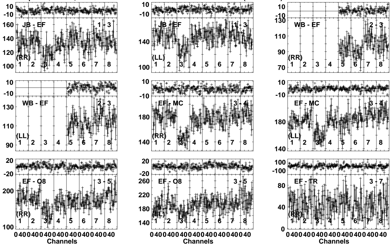
Lower frame: Milli Ampl Jy Top frame: Phas deg Vector averaged cross-power spectrum Several baselines displayed Timerange: 00/16:26:01 to 00/16:26:59
