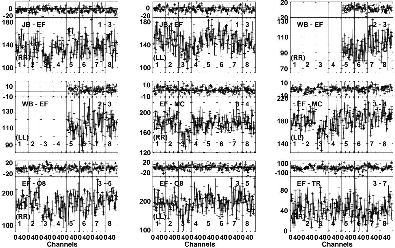
Lower frame: Milli Ampl Jy Top frame: Phas deg Vector averaged cross-power spectrum Several baselines displayed Timerange: 00/16:47:31 to 00/16:48:29
