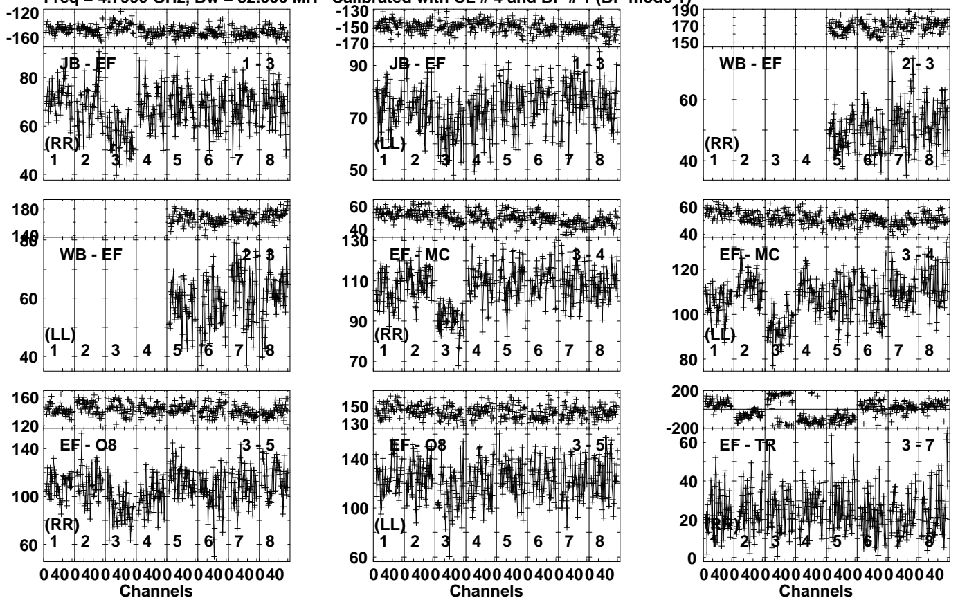
Lower frame: Milli Ampl Jy Top frame: Phas deg Vector averaged cross-power spectrum Several baselines displayed Timerange: 00/14:17:31 to 00/14:19:59
