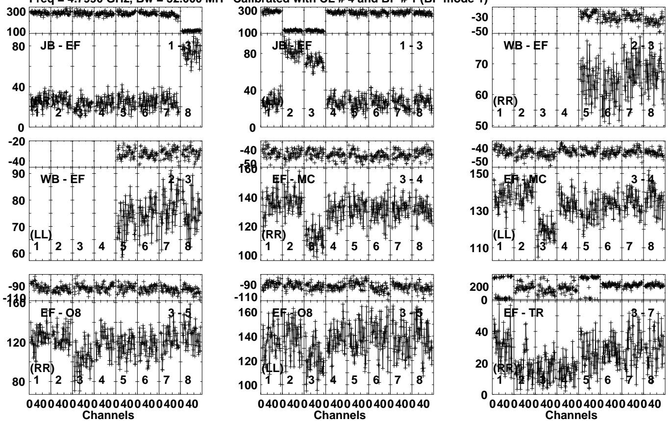
Lower frame: Milli Ampl Jy Top frame: Phas deg Vector averaged cross-power spectrum Several baselines displayed Timerange: 00/13:53:31 to 00/13:56:59
