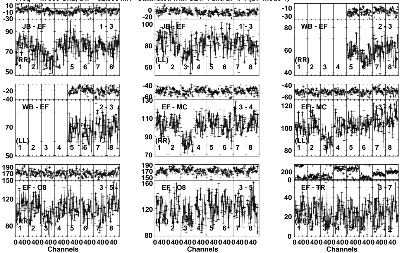
Lower frame: Milli Ampl Jy Top frame: Phas deg Vector averaged cross-power spectrum Several baselines displayed Timerange: 00:15:59:01 to 00:16:01:29
