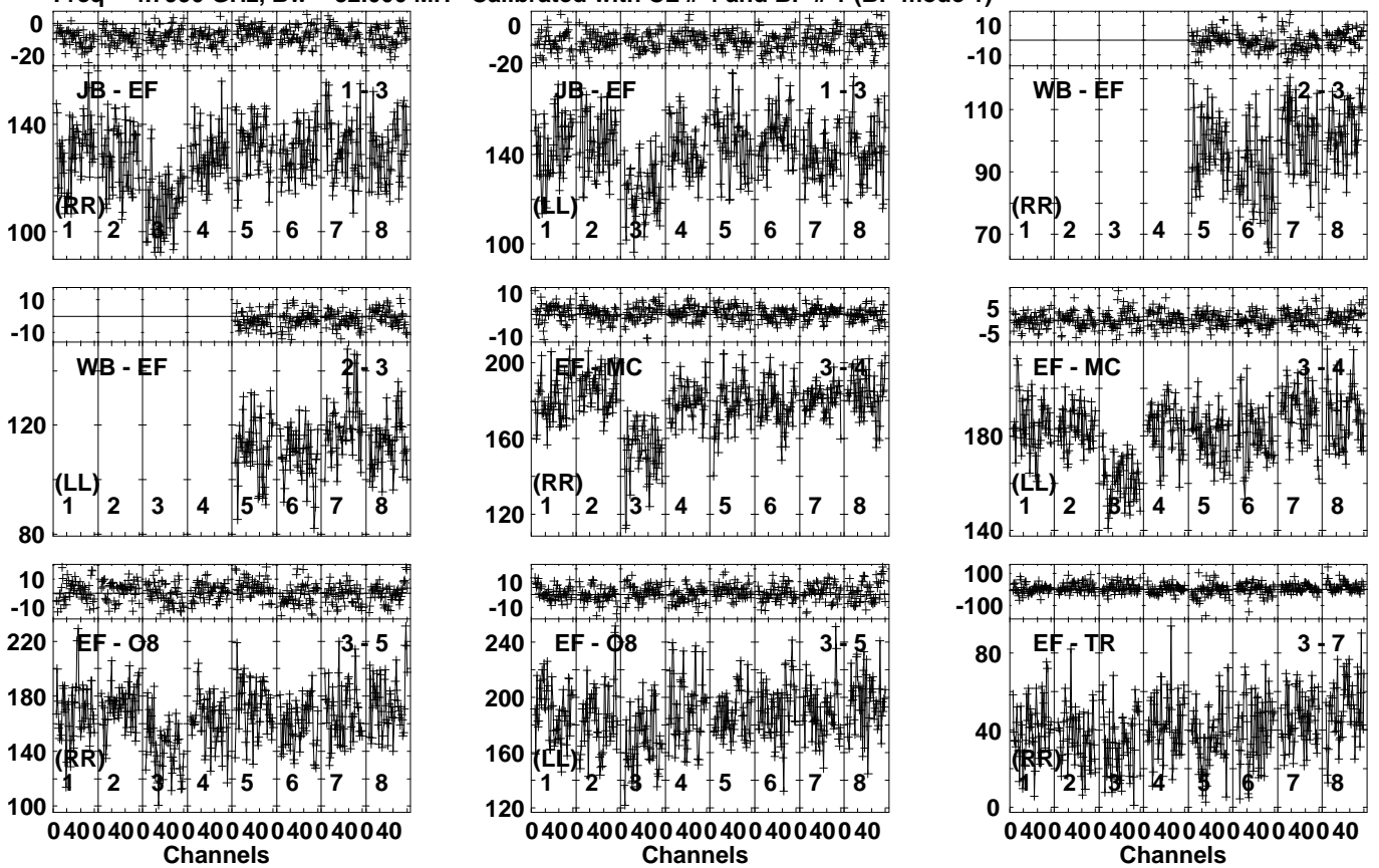
Lower frame: Milli Ampl Jy Top frame: Phas deg Vector averaged cross-power spectrum Several baselines displayed Timerange: 00/15:13:31 to 00/15:14:29
