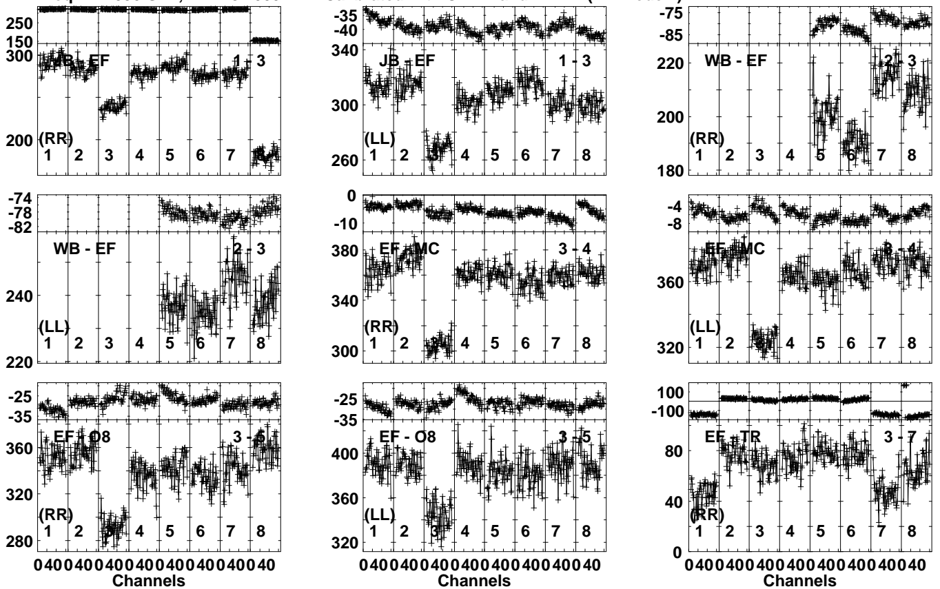
Lower frame: Milli Ampl Jy Top frame: Phas deg Vector averaged cross-power spectrum Several baselines displayed Timerange: 00/16:43:31 to 00/16:46:59
