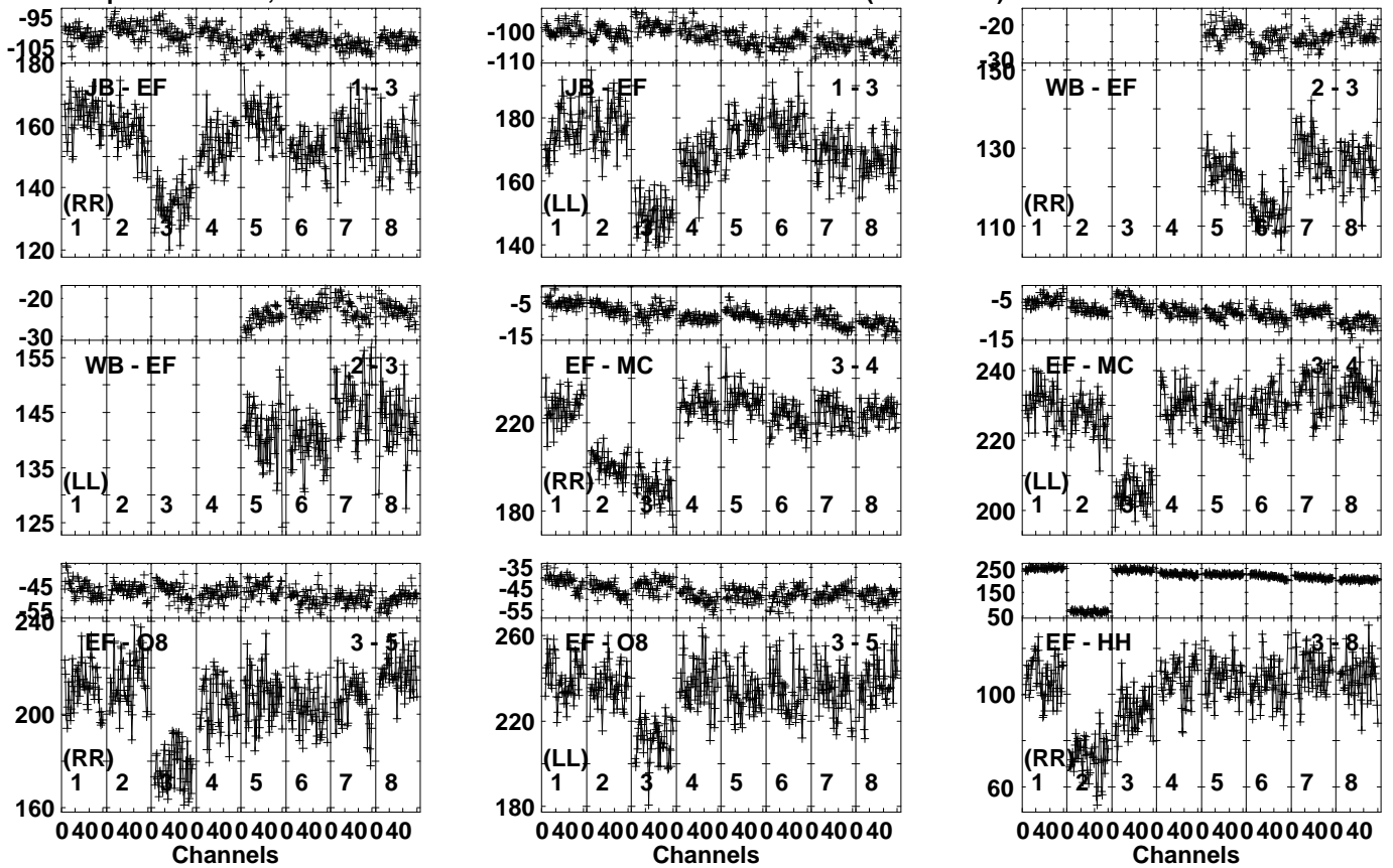
Lower frame: Milli Ampl Jy Top frame: Phas deg Vector averaged cross-power spectrum Several baselines displayed Timerange: 00/15:14:31 to 00/15:17:59
