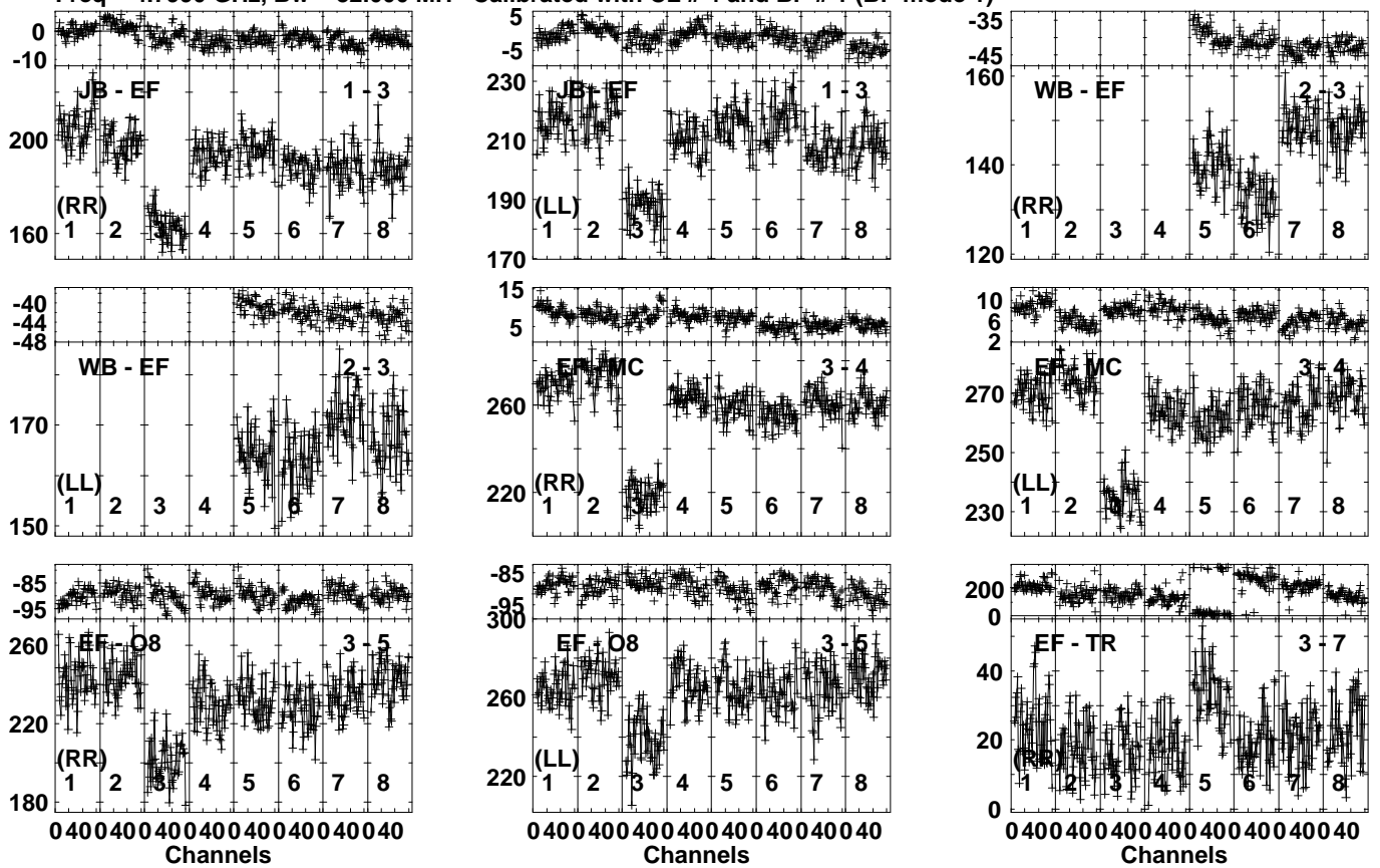
Lower frame: Milli Ampl Jy Top frame: Phas deg Vector averaged cross-power spectrum Several baselines displayed Timerange: 00/15:49:01 to 00/15:52:29
