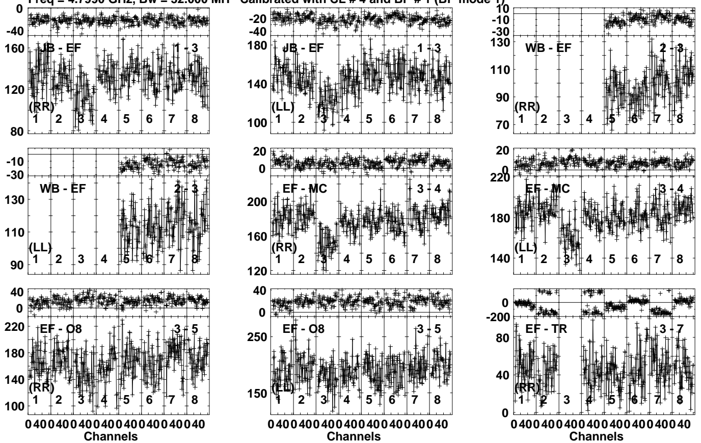
Lower frame: Milli Ampl Jy Top frame: Phas deg Vector averaged cross-power spectrum Several baselines displayed Timerange: 00:15:27:01 to 00:15:28:29
