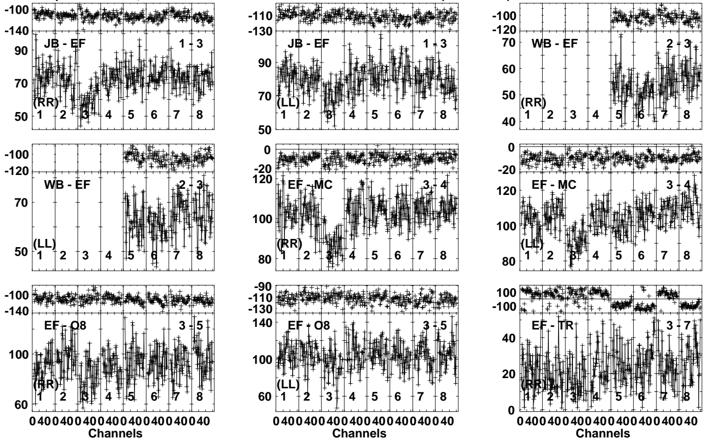
Lower frame: Milli Ampl Jy Top frame: Phas deg Vector averaged cross-power spectrum Several baselines displayed Timerange: 00/16:48:31 to 00/16:50:59
