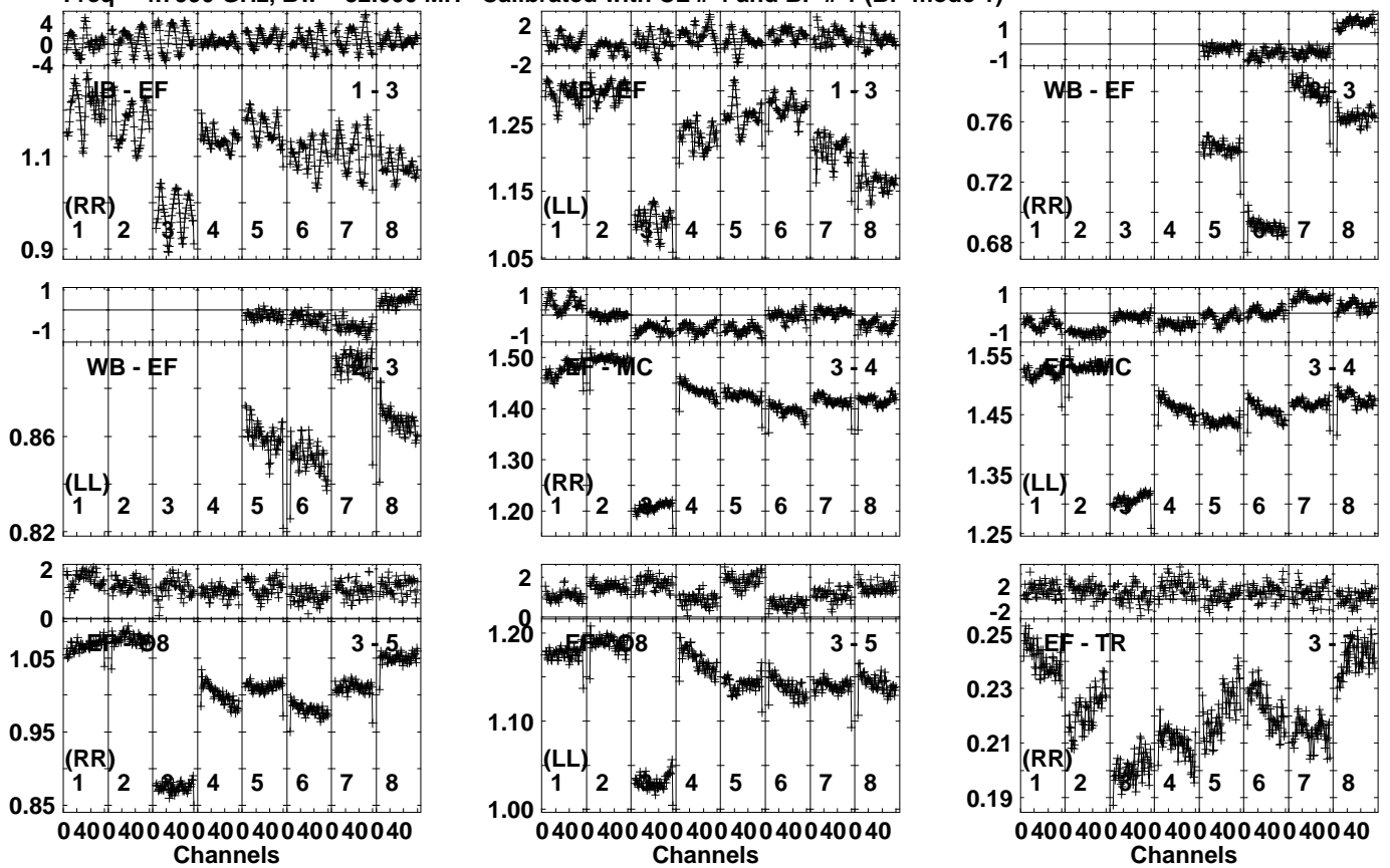
Lower frame: Ampl Jy Top frame: Phas deg Vector averaged cross-power spectrum Several baselines displayed Timerange: 00/12:33:01 to 00/12:41:59
