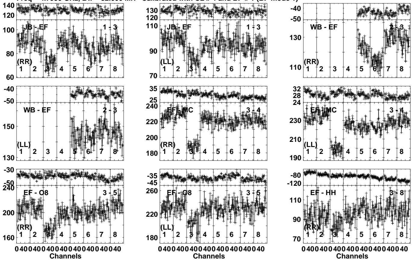
Lower frame: Milli Ampl Jy Top frame: Phas deg Vector averaged cross-power spectrum Several baselines displayed Timerange: 00/15:09:31 to 00/15:12:59
