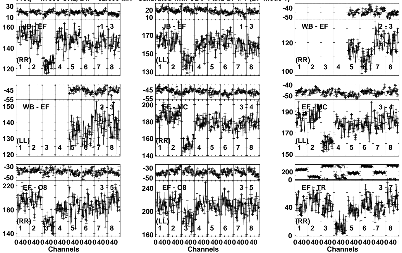
Lower frame: Milli Ampl Jy Top frame: Phas deg Vector averaged cross-power spectrum Several baselines displayed Timerange: 00:17:37:01 to 00:17:40:29
