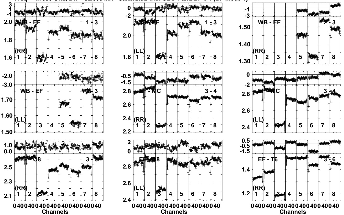
Lower frame: Ampl Jy Top frame: Phas deg Vector averaged cross-power spectrum Several baselines displayed Timerange: 00/13:08:01 to 00/13:11:59
