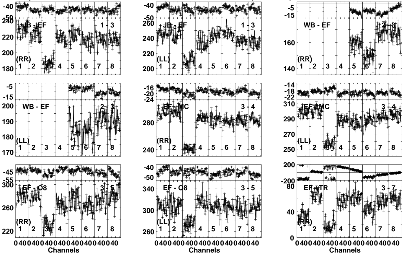
Lower frame: Milli Ampl Jy Top frame: Phas deg Vector averaged cross-power spectrum Several baselines displayed Timerange: 00/16:08:01 to 00/16:11:29
