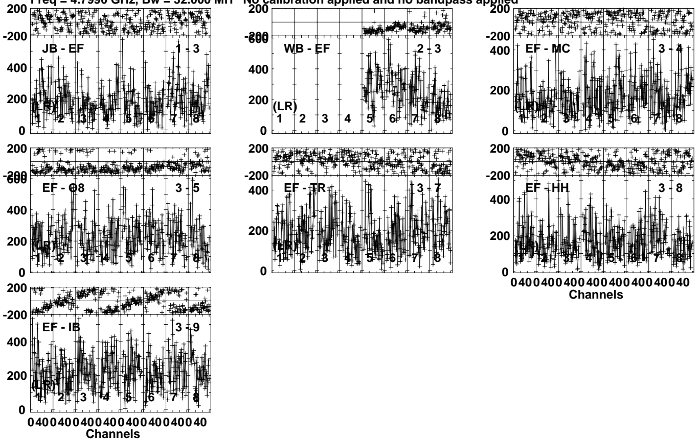
Lower frame: Micro Ampl Jy Top frame: Phas deg Vector averaged cross-power spectrum Several baselines displayed Timerange: 00/16:26:01 to 00/16:26:59
