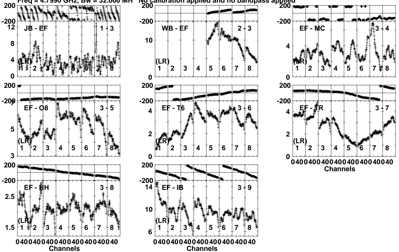
Lower frame: Milli Ampl Jy Top frame: Phas deg Vector averaged cross-power spectrum Several baselines displayed Timerange: 00/17:17:31 to 00/17:22:59
