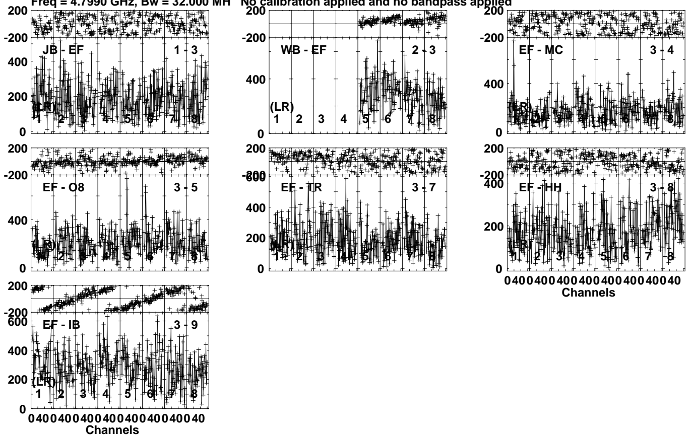
Lower frame: Micro Ampl Jy Top frame: Phas deg Vector averaged cross-power spectrum Several baselines displayed Timerange: 00/15:23:31 to 00/15:24:29
