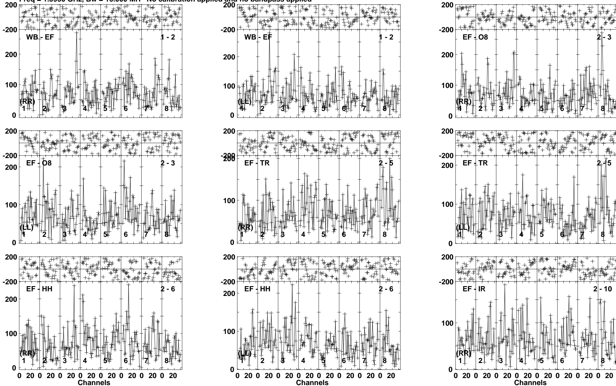
Lower frame: Micro Ampl Jy Top frame: Phas deg Vector averaged cross-power spectrum Baseline: WB (01) - EF (02) Timerange: 01/03:59:11 to 01/04:03:10
