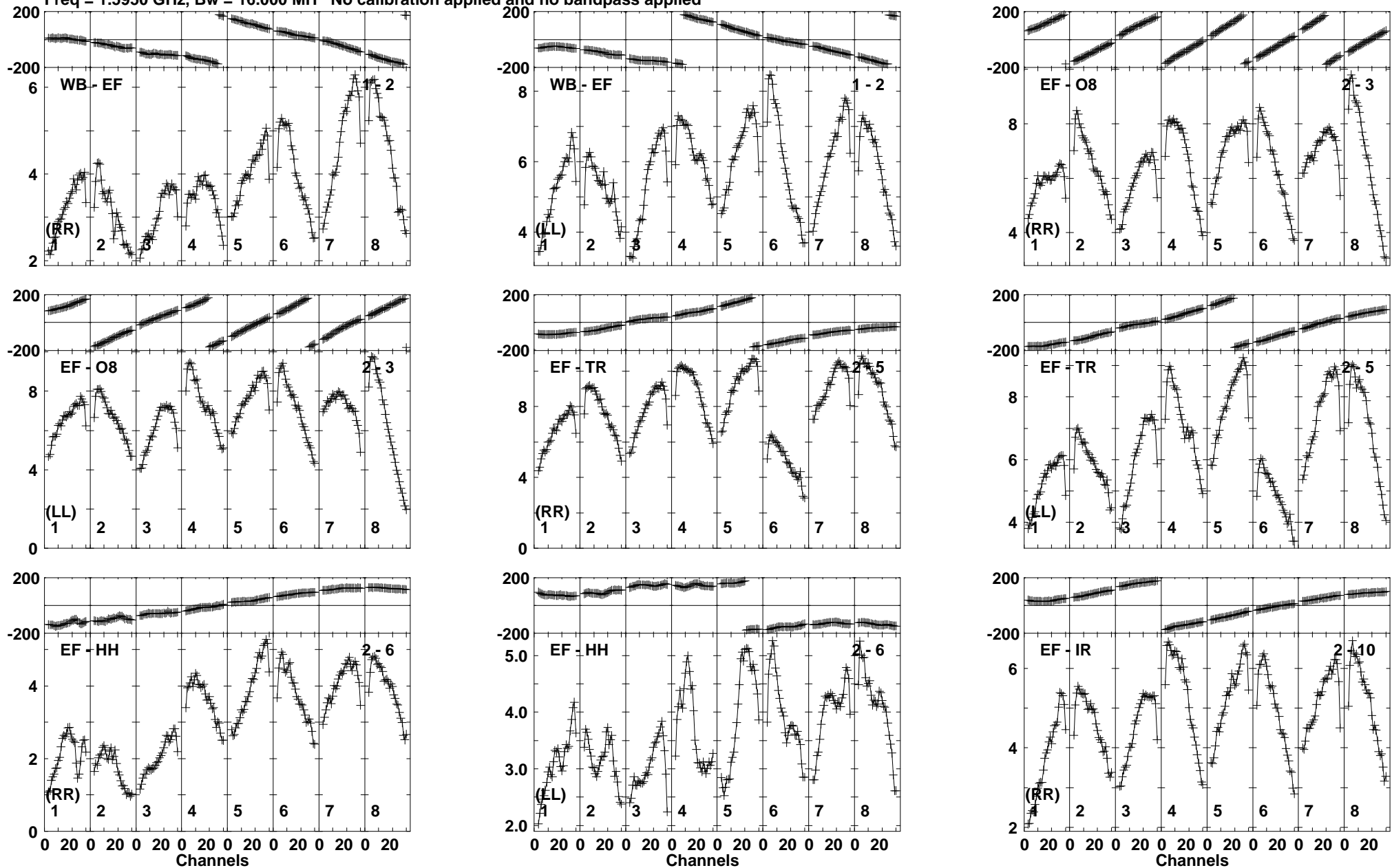
Lower frame: Milli Ampl Jy Top frame: Phas deg Vector averaged cross-power spectrum Baseline: WB (01) - EF (02) Timerange: 01/05:32:01 to 01/05:32:59
