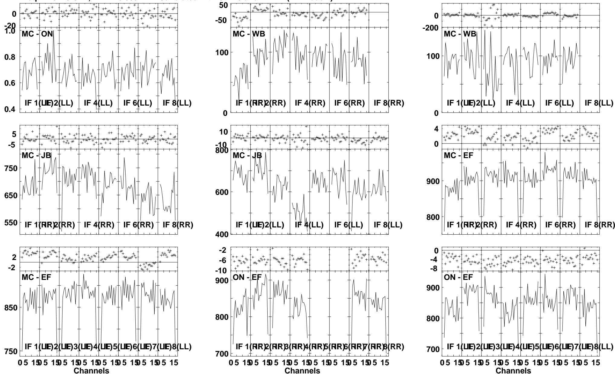
Lower frame: Ampl Jy Top frame: Phas deg Vector averaged cross-power spectrum Several baselines displayed Timerange: 01/03:42:31 to 01/03:44:29
