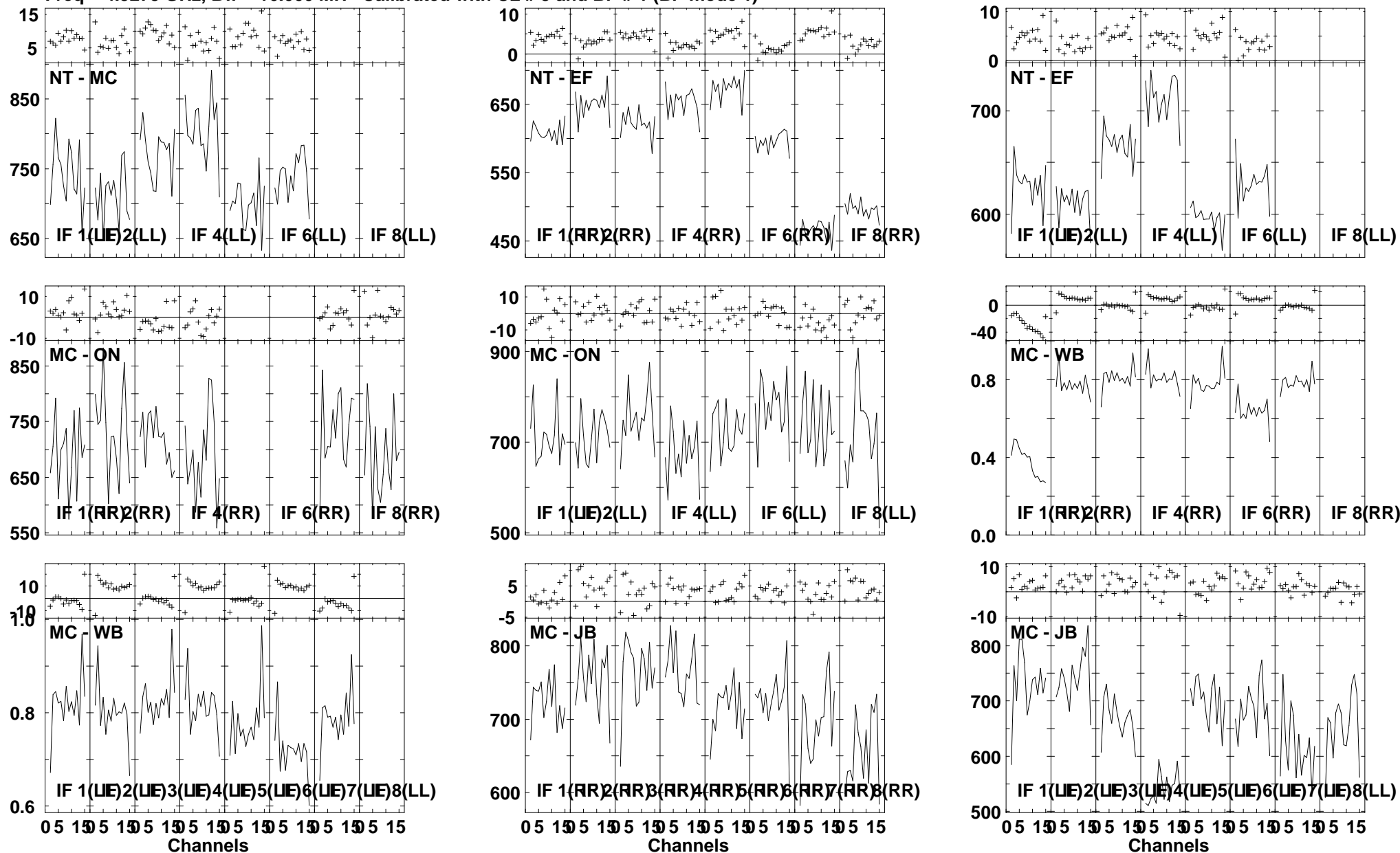
Lower frame: Milli Ampl Jy Top frame: Phas deg Vector averaged cross-power spectrum Several baselines displayed Timerange: 01/00:08:01 to 01/00:09:59
