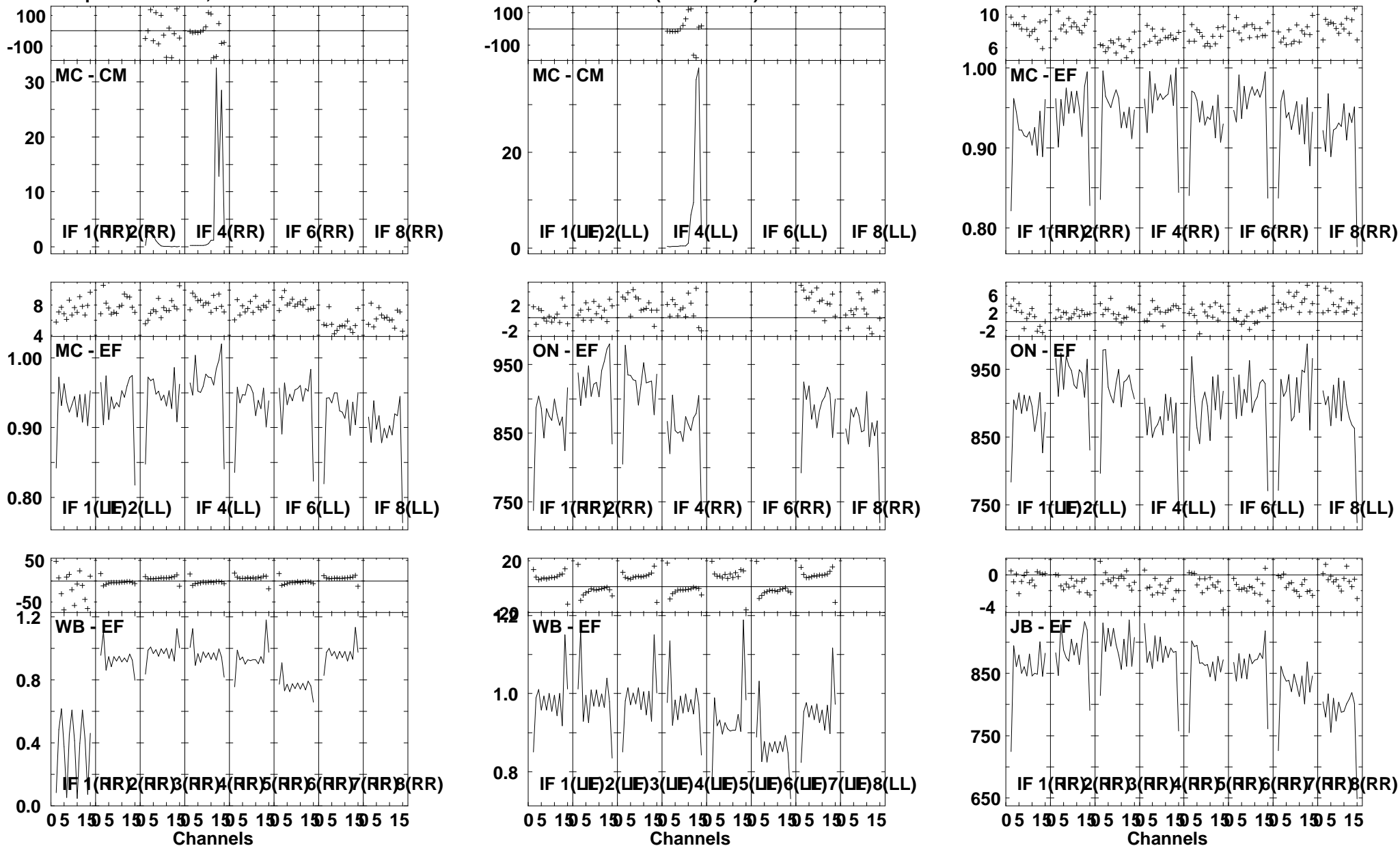
Lower frame: Ampl Jy Top frame: Phas deg Vector averaged cross-power spectrum Several baselines displayed Timerange: 01/00:02:01 to 01/00:03:59
