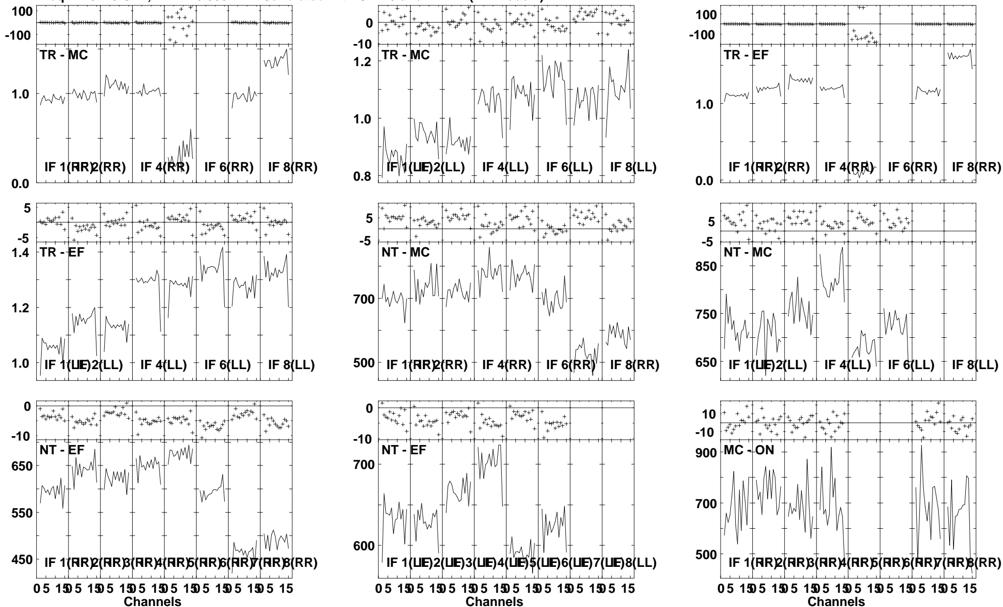
Lower frame: Ampl Jy Top frame: Phas deg Vector averaged cross-power spectrum Several baselines displayed Timerange: 01/01:27:31 to 01/01:29:29
