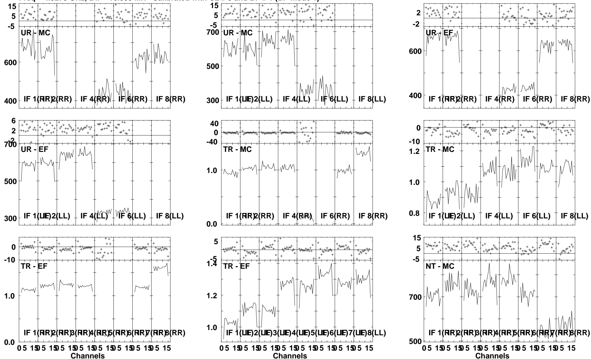
Lower frame: Milli Ampl Jy Top frame: Phas deg Vector averaged cross-power spectrum Several baselines displayed Timerange: 01/00:59:01 to 01/01:00:59
