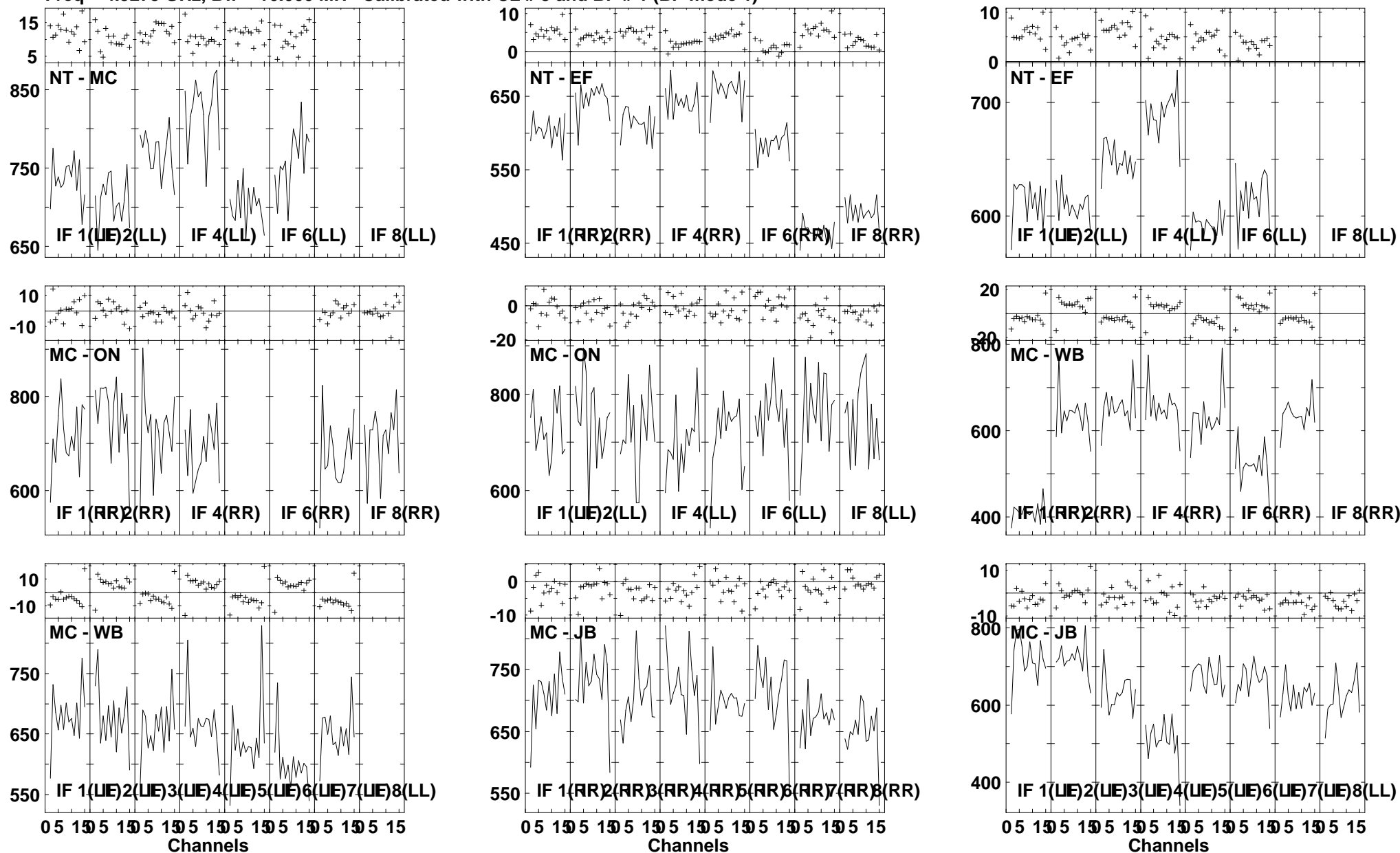
Lower frame: Milli Ampl Jy Top frame: Phas deg Vector averaged cross-power spectrum Several baselines displayed Timerange: 00/23:06:31 to 00/23:08:29
