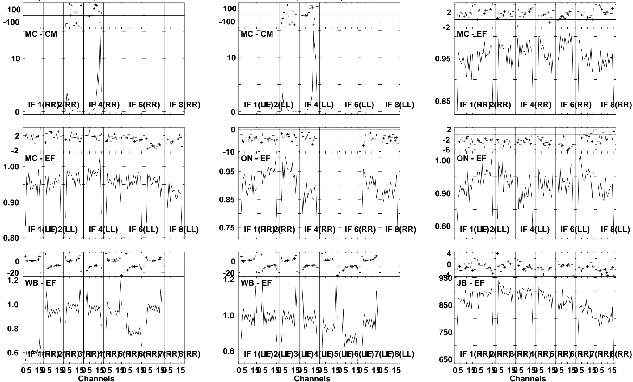
Lower frame: Ampl Jy Top frame: Phas deg Vector averaged cross-power spectrum Several baselines displayed Timerange: 00/23:35:01 to 00/23:36:59
