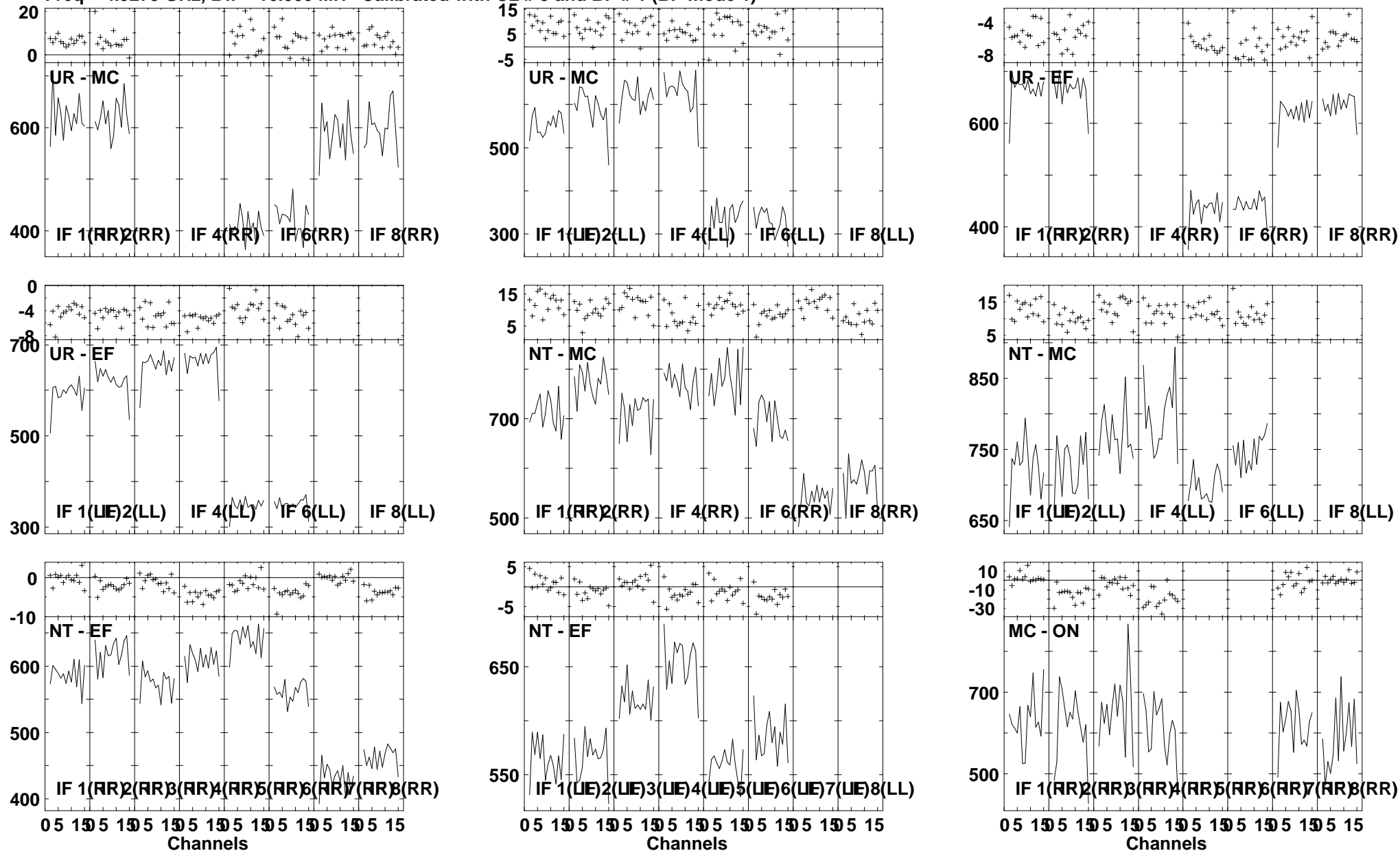
Lower frame: Milli Ampl Jy Top frame: Phas deg Vector averaged cross-power spectrum Several baselines displayed Timerange: 00/22:15:31 to 00/22:17:29
