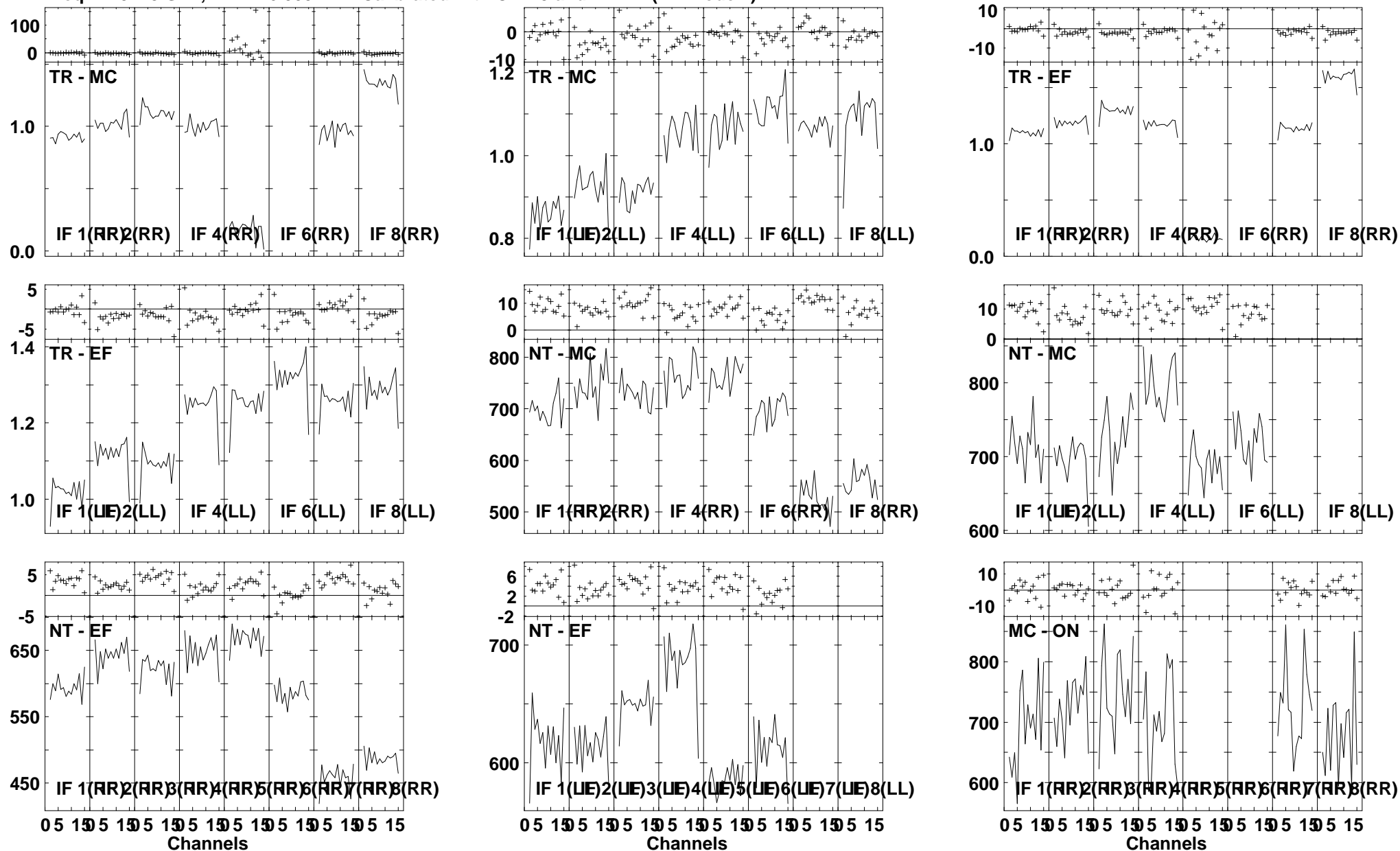
Lower frame: Ampl Jy Top frame: Phas deg Vector averaged cross-power spectrum Several baselines displayed Timerange: 01/01:38:01 to 01/01:39:59
