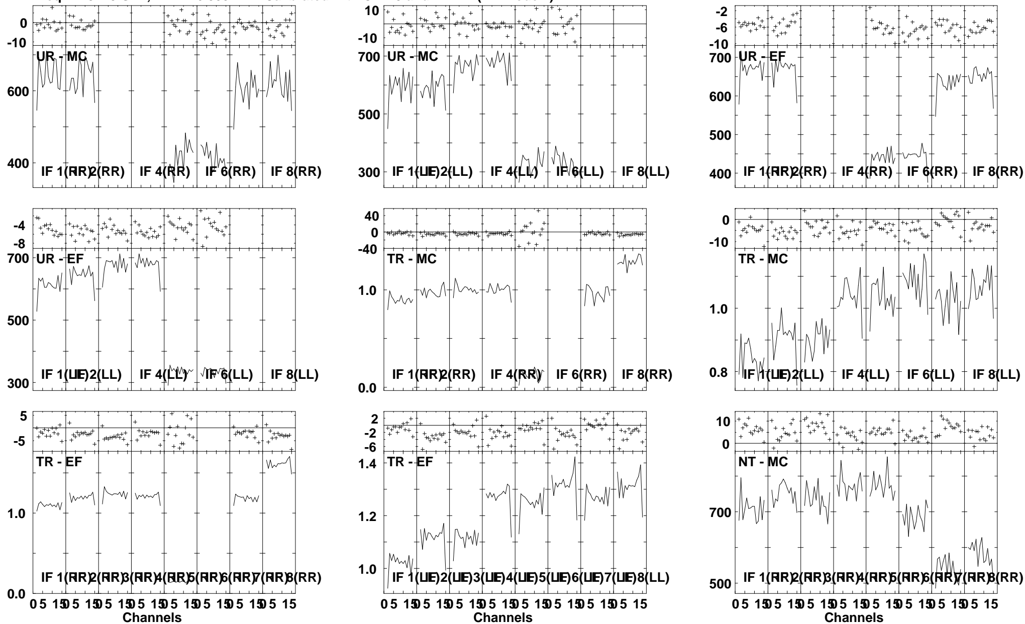
Lower frame: Milli Ampl Jy Top frame: Phas deg Vector averaged cross-power spectrum Several baselines displayed Timerange: 00/23:57:54 to 00/23:59:29
