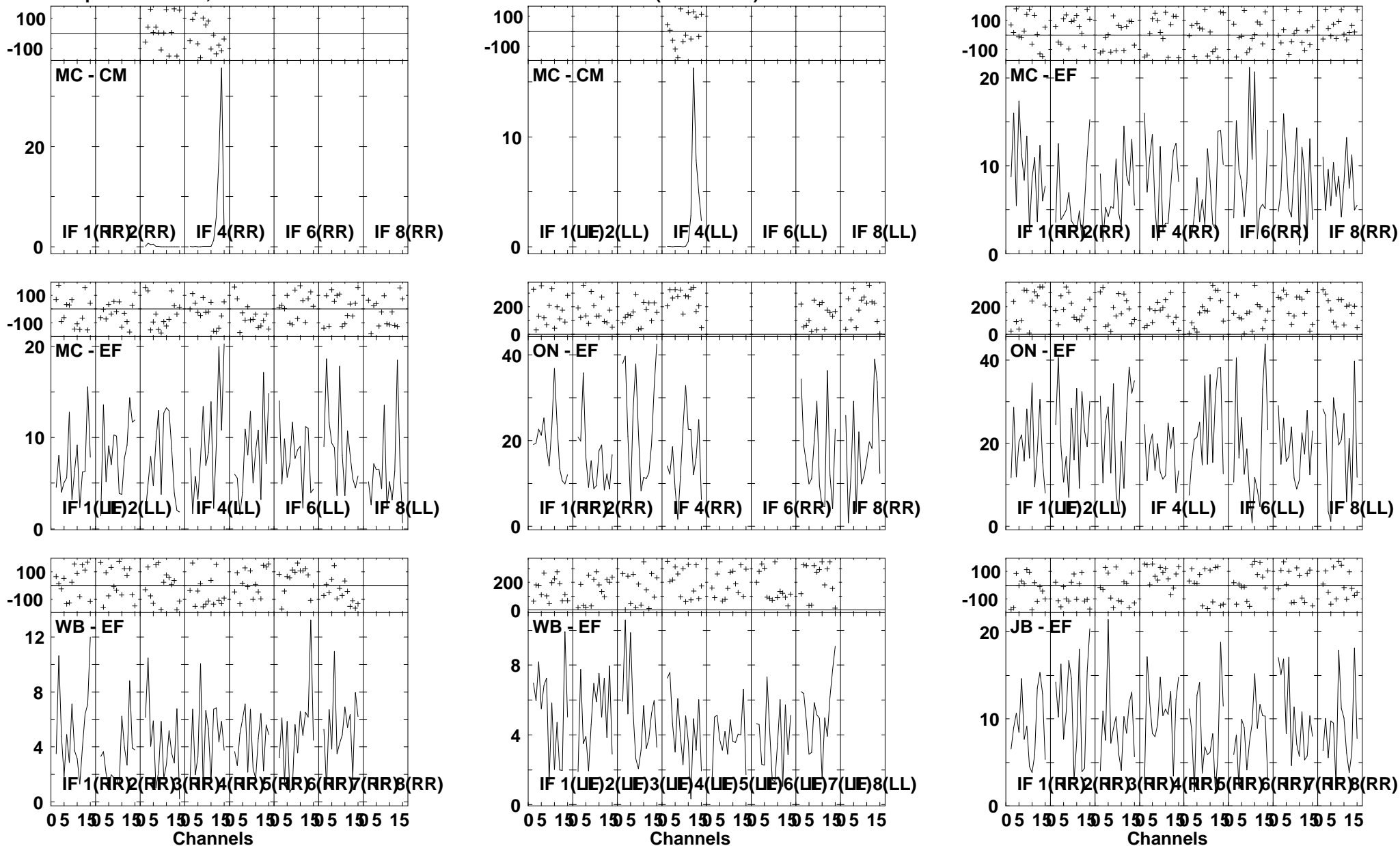
Lower frame: Ampl Jy Top frame: Phas deg Vector averaged cross-power spectrum Several baselines displayed Timerange: 00/23:53:31 to 00/23:57:29
