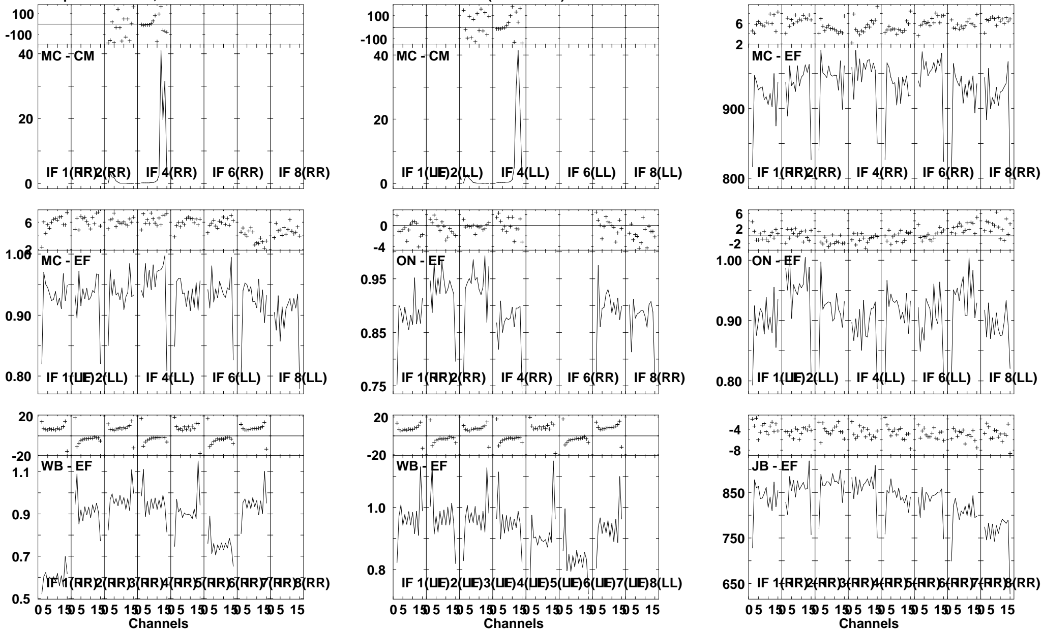
Lower frame: Ampl Jy Top frame: Phas deg Vector averaged cross-power spectrum Several baselines displayed Timerange: 00/23:12:31 to 00/23:14:29
