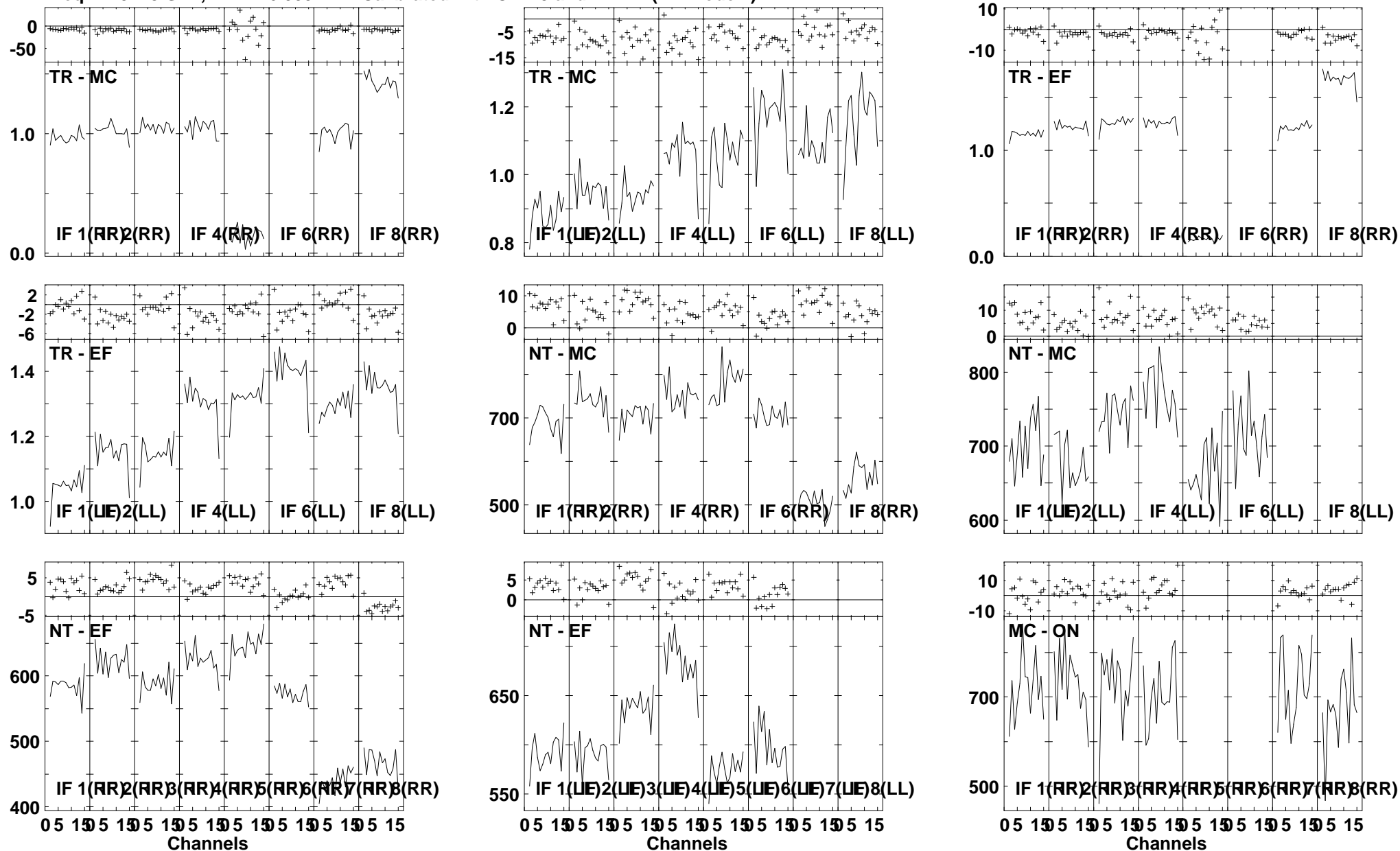
Lower frame: Ampl Jy Top frame: Phas deg Vector averaged cross-power spectrum Several baselines displayed Timerange: 01/04:32:01 to 01/04:33:59
