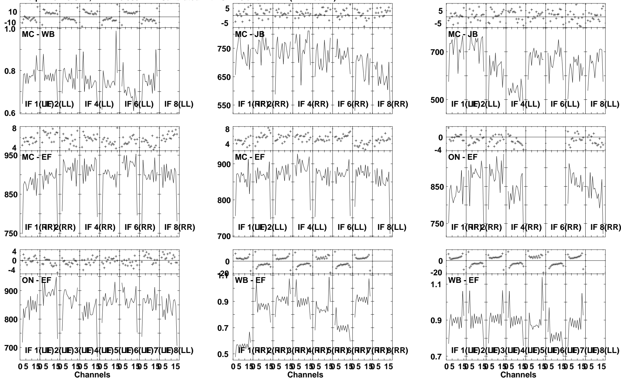
Lower frame: Ampl Jy Top frame: Phas deg Vector averaged cross-power spectrum Several baselines displayed Timerange: 01/03:30:31 to 01/03:32:29
