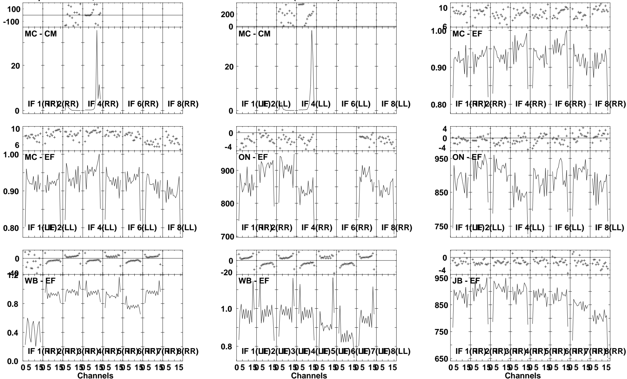
Lower frame: Ampl Jy Top frame: Phas deg Vector averaged cross-power spectrum Several baselines displayed Timerange: 01/00:36:31 to 01/00:38:29
