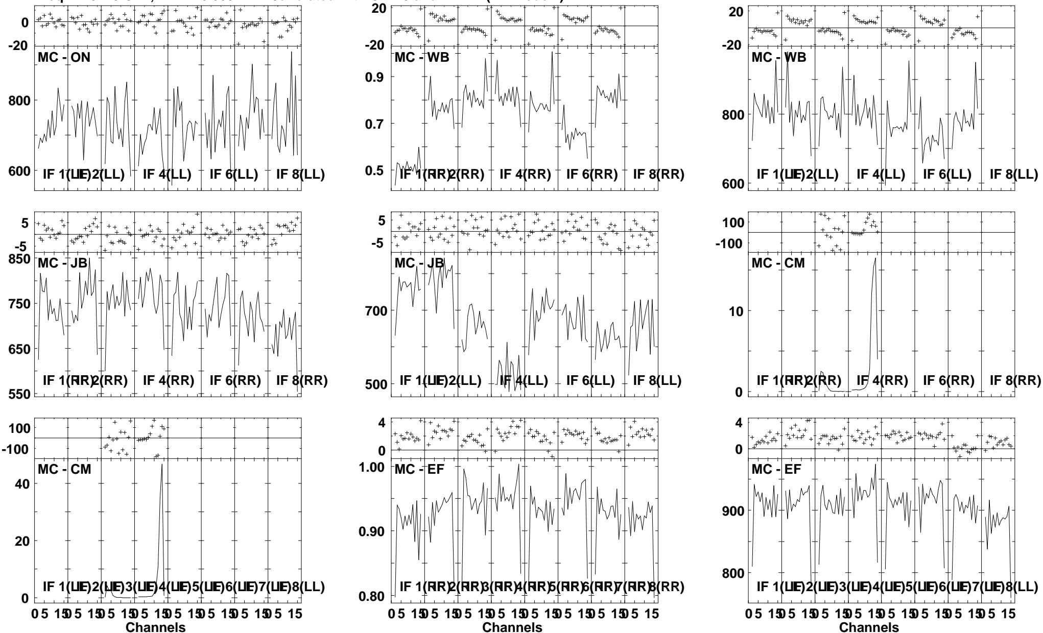
Lower frame: Milli Ampl Jy Top frame: Phas deg Vector averaged cross-power spectrum Several baselines displayed Timerange: 01/01:38:01 to 01/01:39:59
