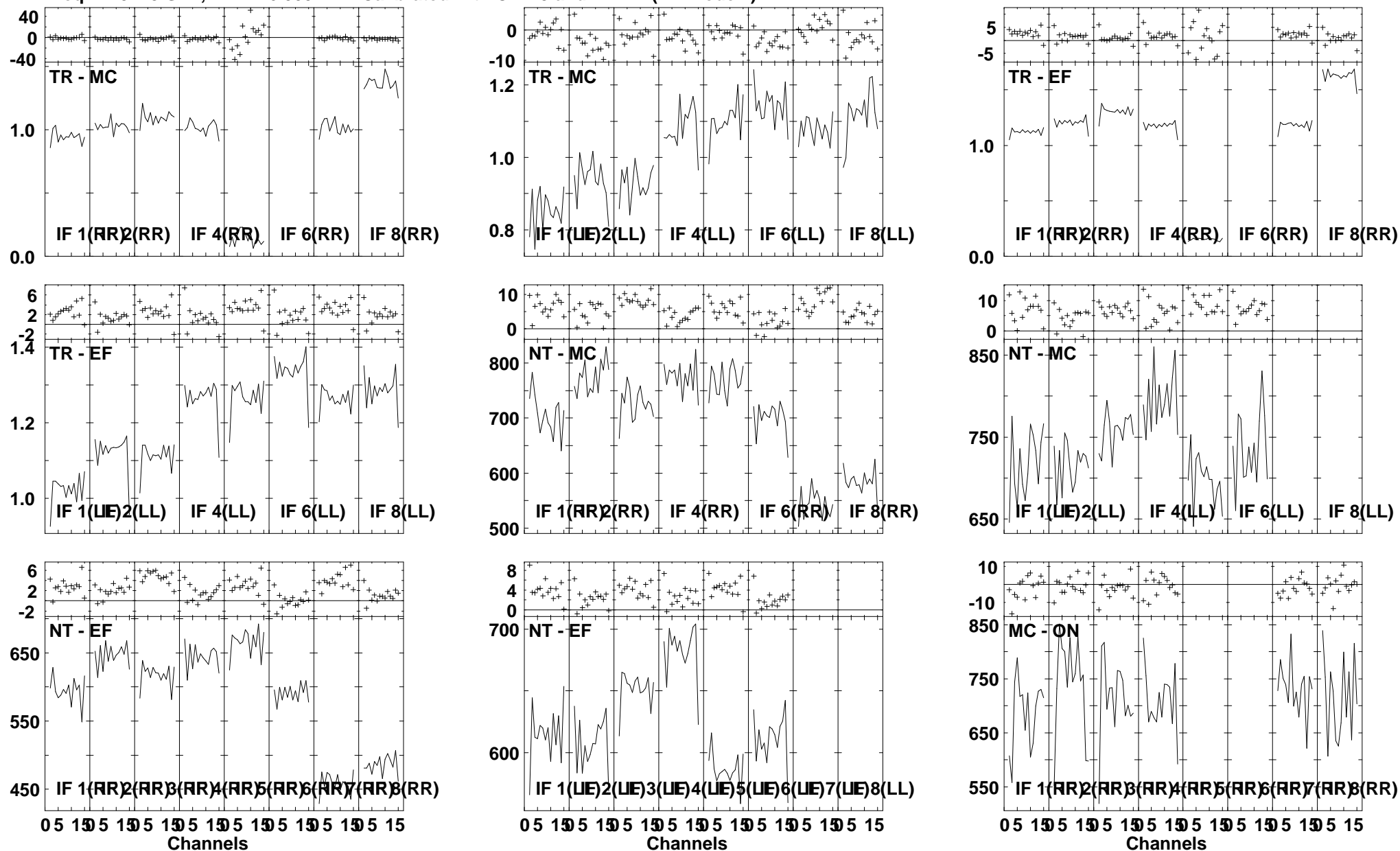
Lower frame: Ampl Jy Top frame: Phas deg Vector averaged cross-power spectrum Several baselines displayed Timerange: 01/01:50:01 to 01/01:51:59
