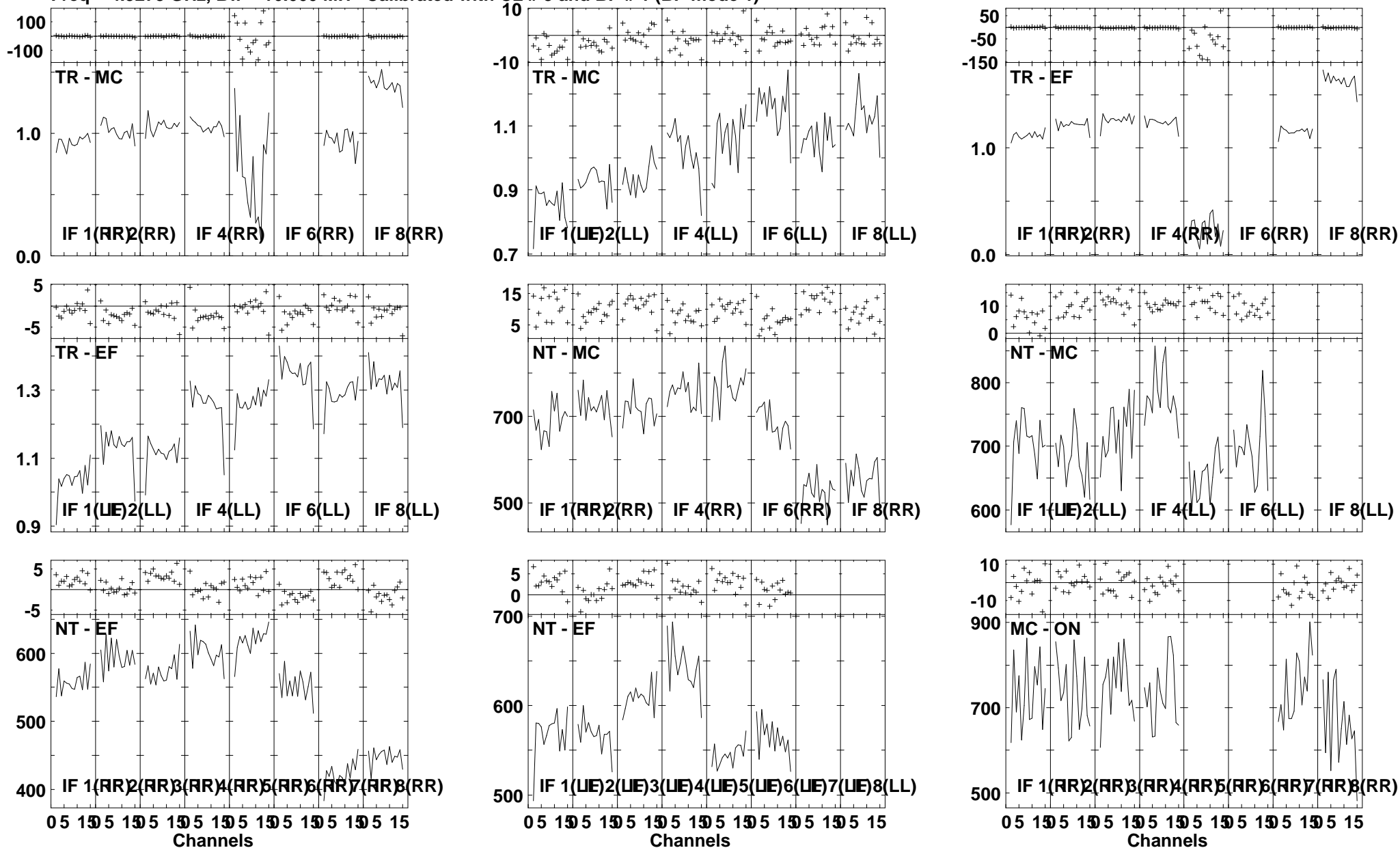
Lower frame: Ampl Jy Top frame: Phas deg Vector averaged cross-power spectrum Several baselines displayed Timerange: 01/05:06:48 to 01/05:08:29
