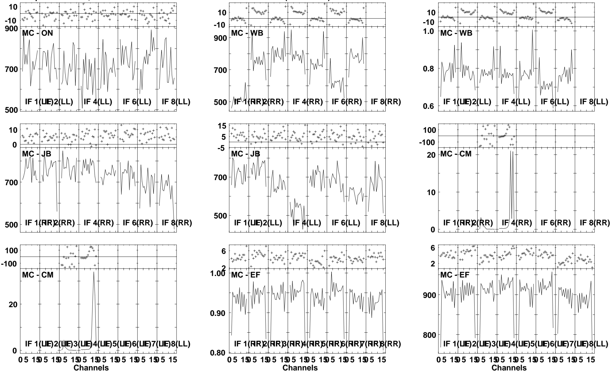
Lower frame: Milli Ampl Jy Top frame: Phas deg Vector averaged cross-power spectrum Several baselines displayed Timerange: 01/02:35:01 to 01/02:36:59
