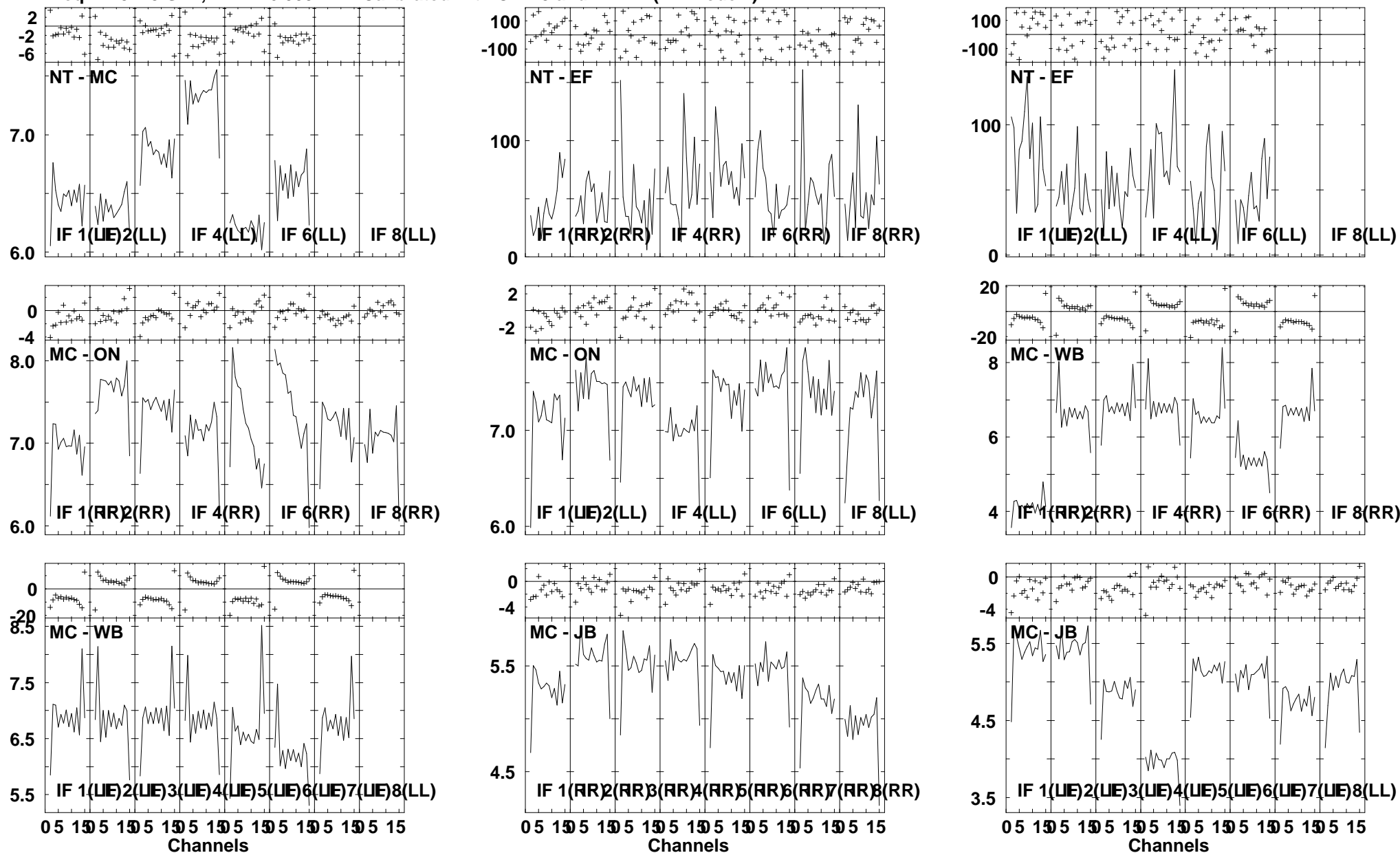
Lower frame: Ampl Jy Top frame: Phas deg Vector averaged cross-power spectrum Several baselines displayed Timerange: 00/21:45:54 to 00/21:46:59
