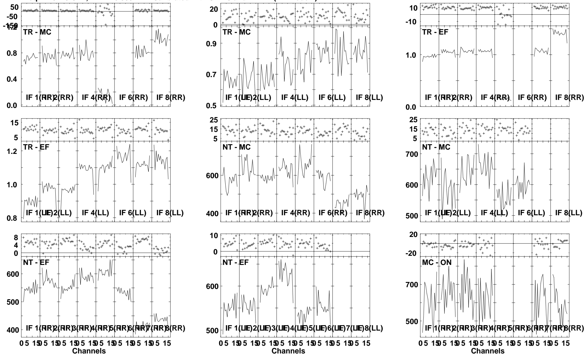
Lower frame: Ampl Jy Top frame: Phas deg Vector averaged cross-power spectrum Several baselines displayed Timerange: 01/05:29:01 to 01/05:30:59
