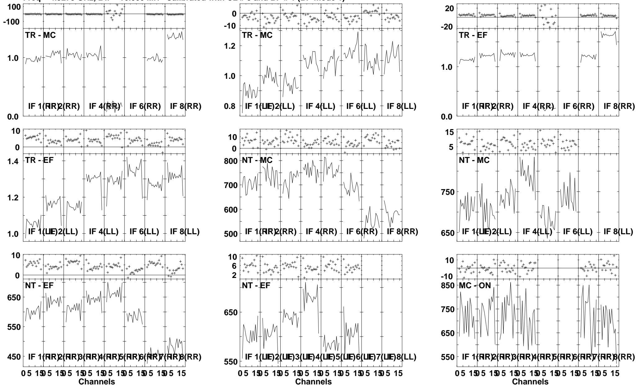
Lower frame: Ampl Jy Top frame: Phas deg Vector averaged cross-power spectrum Several baselines displayed Timerange: 01/02:39:31 to 01/02:41:29
