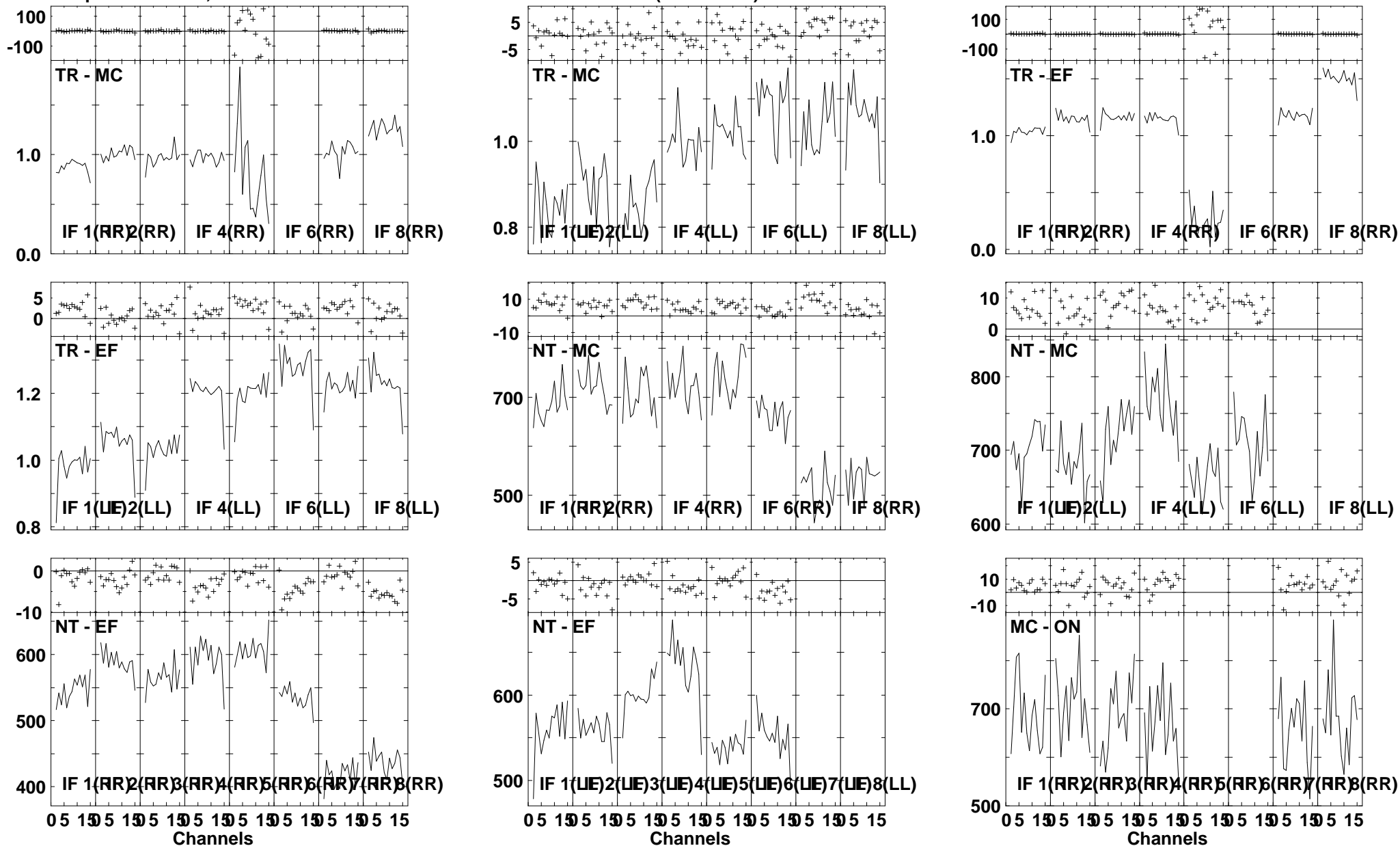
Lower frame: Ampl Jy Top frame: Phas deg Vector averaged cross-power spectrum Several baselines displayed Timerange: 01/05:35:01 to 01/05:36:59
