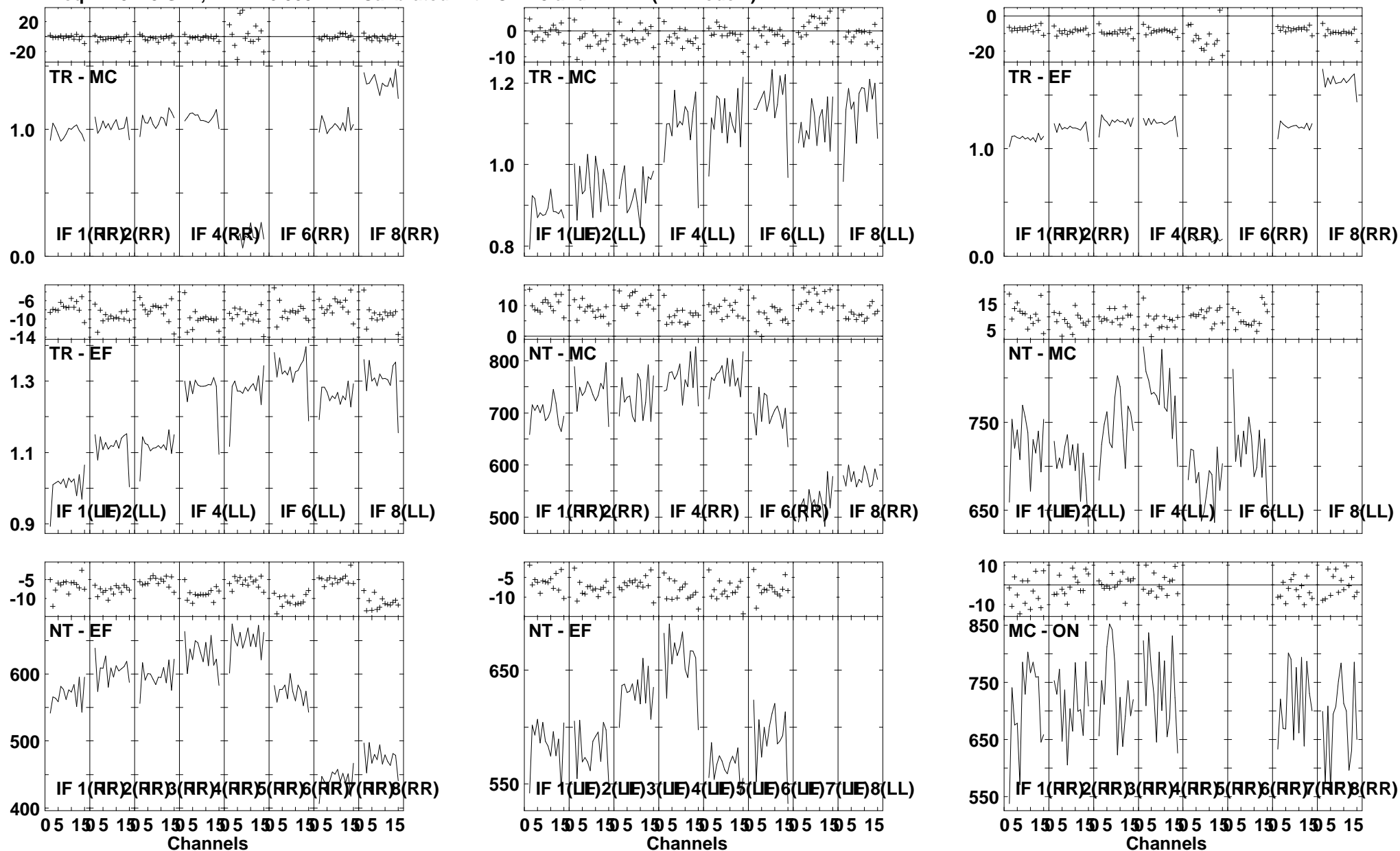
Lower frame: Ampl Jy Top frame: Phas deg Vector averaged cross-power spectrum Several baselines displayed Timerange: 01/03:24:31 to 01/03:26:29
