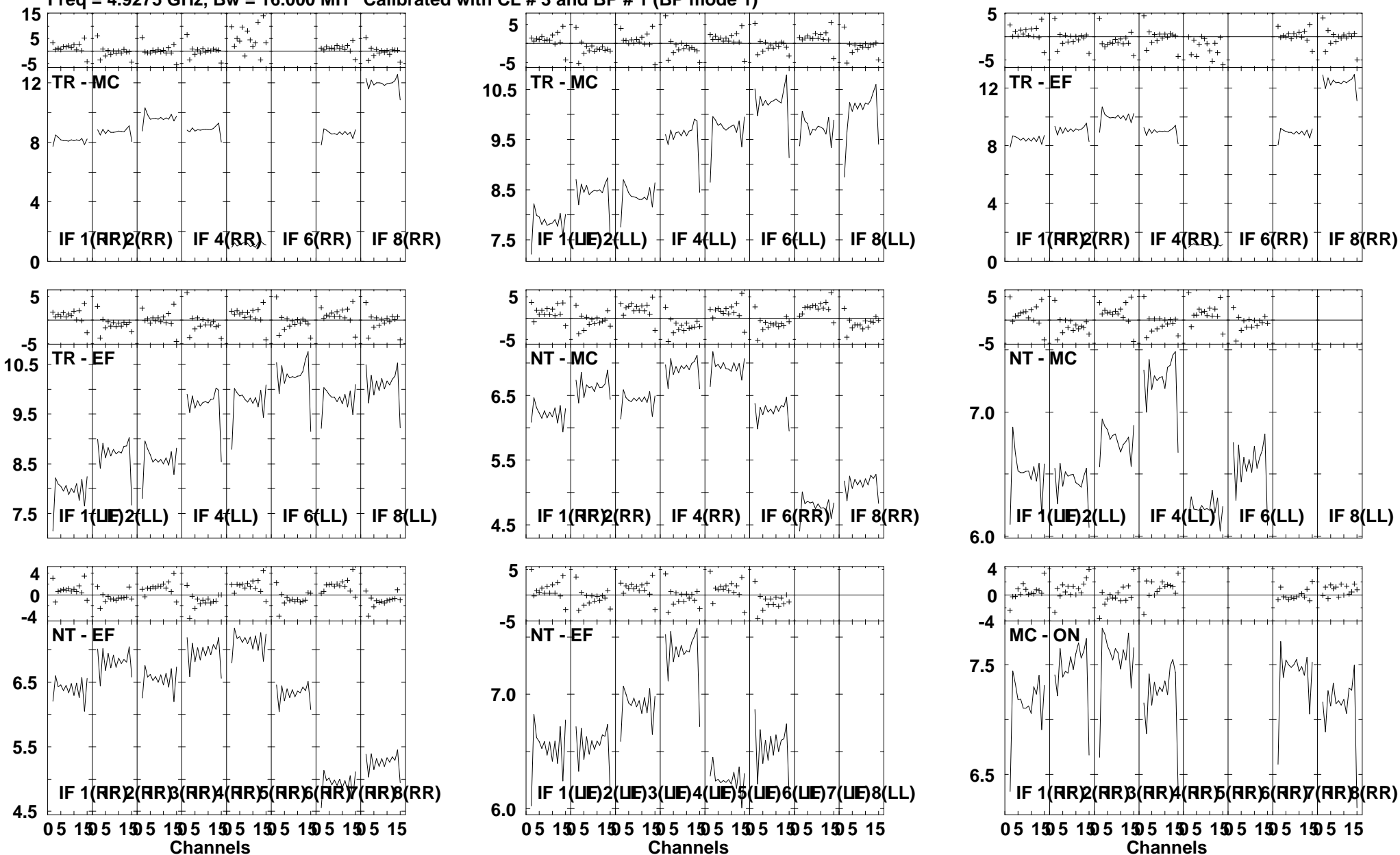
Lower frame: Ampl Jy Top frame: Phas deg Vector averaged cross-power spectrum Several baselines displayed Timerange: 01/01:30:54 to 01/01:31:59
