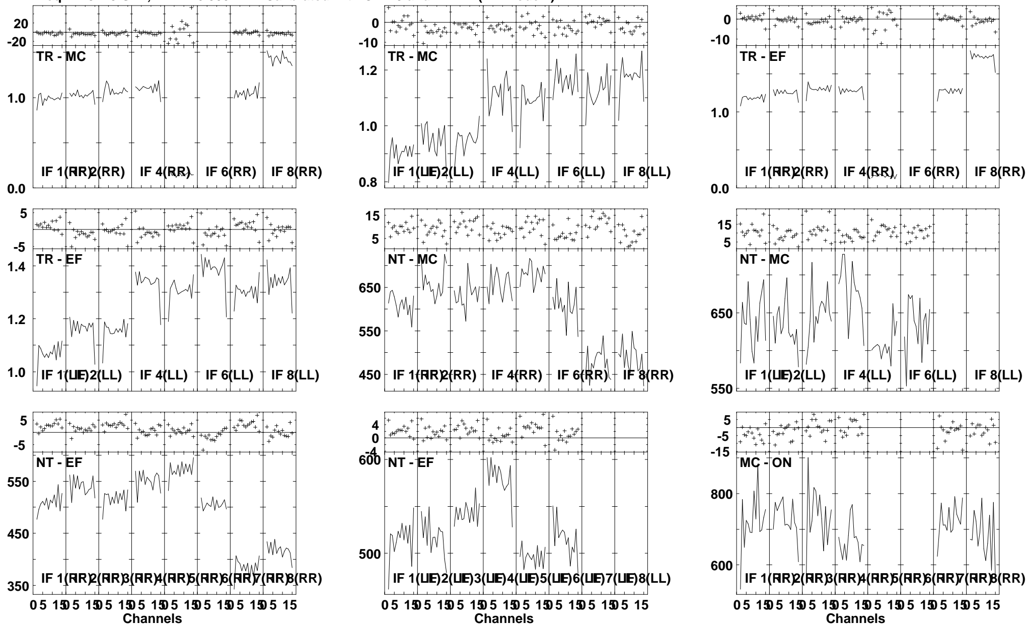
Lower frame: Ampl Jy Top frame: Phas deg Vector averaged cross-power spectrum Several baselines displayed Timerange: 01/03:59:01 to 01/04:00:59
