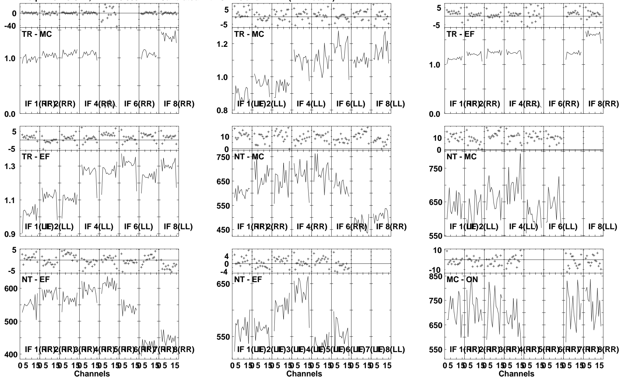
Lower frame: Ampl Jy Top frame: Phas deg Vector averaged cross-power spectrum Several baselines displayed Timerange: 01/03:53:01 to 01/03:54:59
