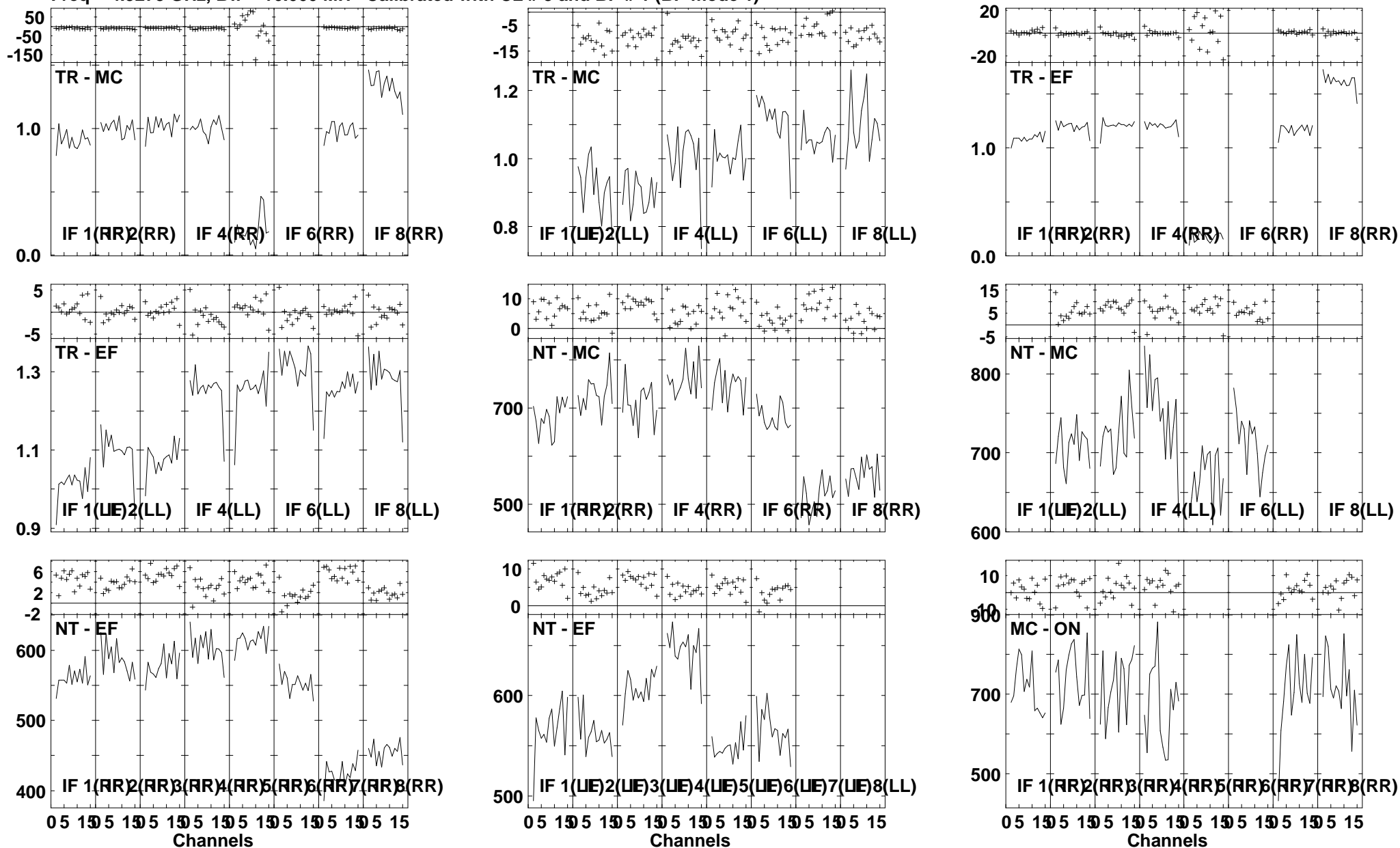
Lower frame: Ampl Jy Top frame: Phas deg Vector averaged cross-power spectrum Several baselines displayed Timerange: 01/05:12:31 to 01/05:14:29
