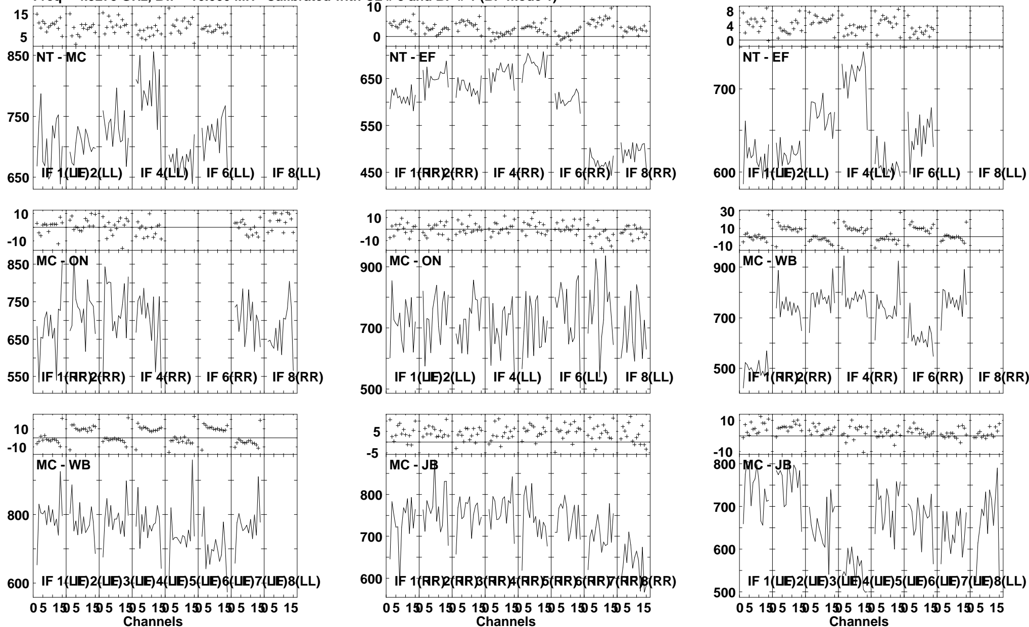
Lower frame: Milli Ampl Jy Top frame: Phas deg Vector averaged cross-power spectrum Several baselines displayed Timerange: 01/00:24:31 to 01/00:26:29
