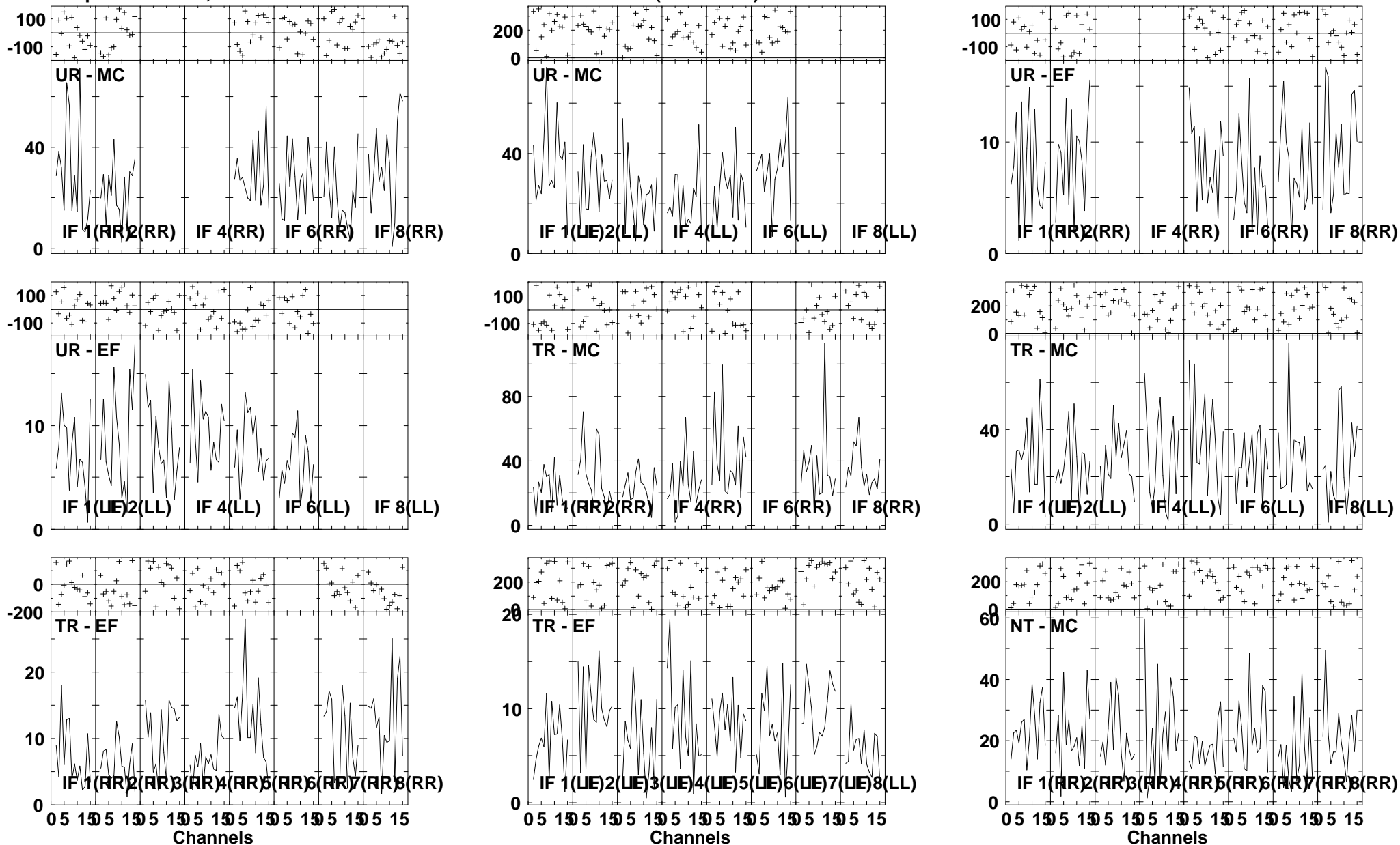
Lower frame: Milli Ampl Jy Top frame: Phas deg Vector averaged cross-power spectrum Several baselines displayed Timerange: 00/23:53:31 to 00/23:57:29
