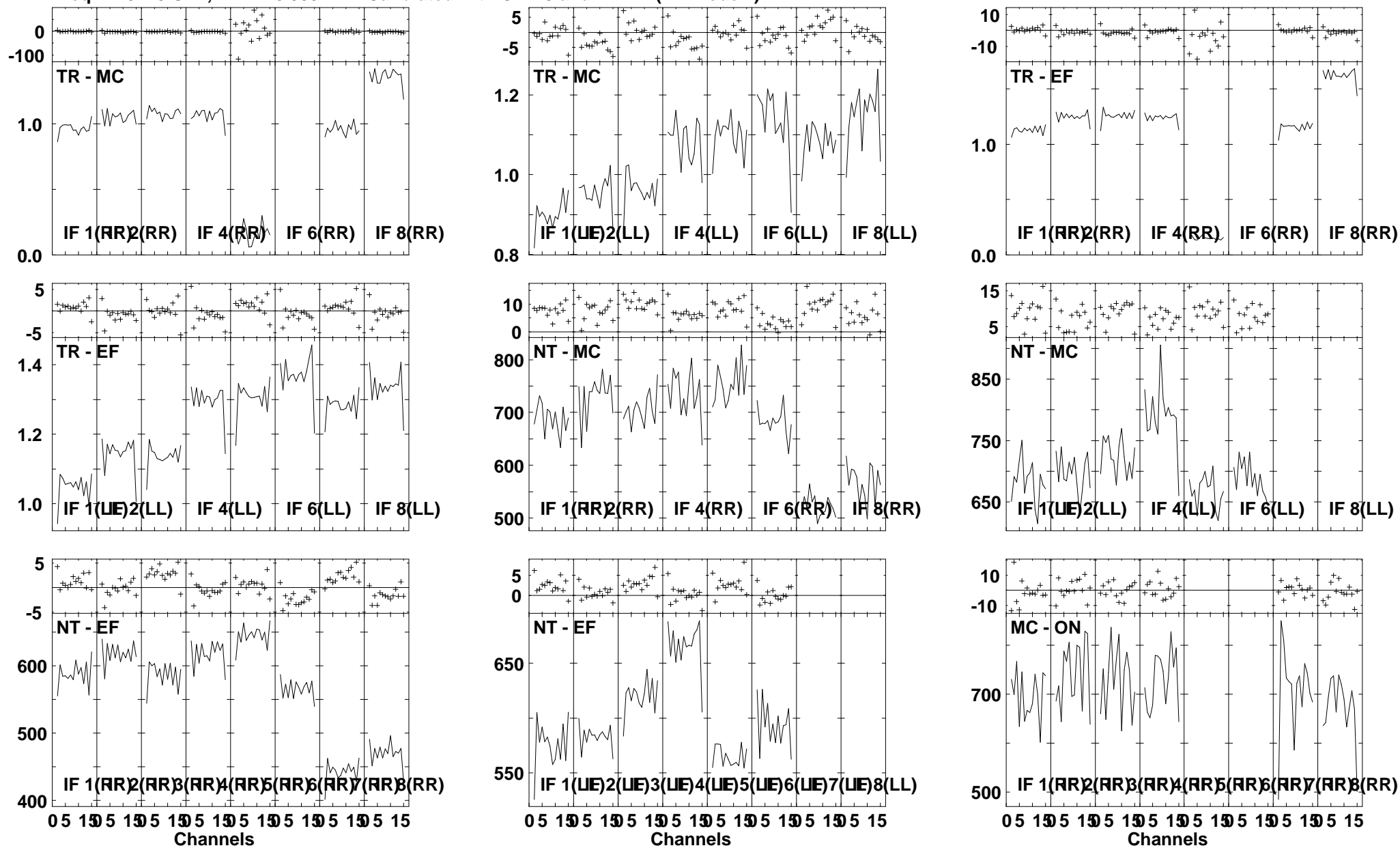
Lower frame: Ampl Jy Top frame: Phas deg Vector averaged cross-power spectrum Several baselines displayed Timerange: 01/02:29:01 to 01/02:30:59
