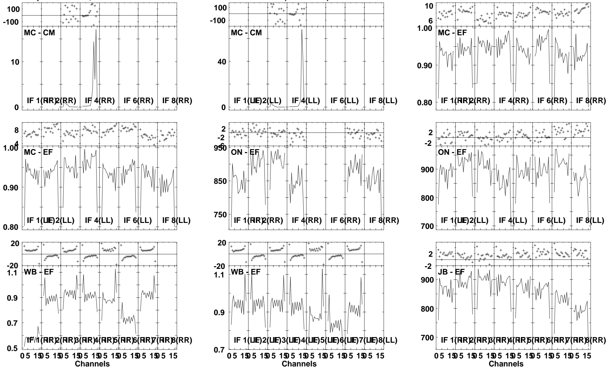
Lower frame: Ampl Jy Top frame: Phas deg Vector averaged cross-power spectrum Several baselines displayed Timerange: 01/00:20:01 to 01/00:21:59
