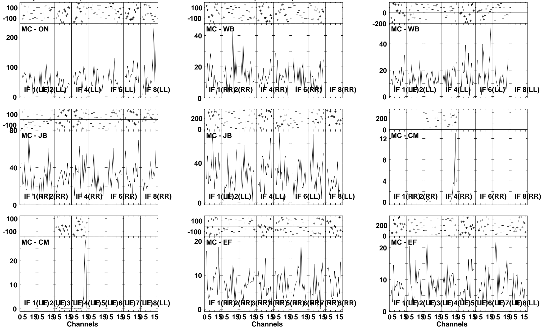
Lower frame: Milli Ampl Jy Top frame: Phas deg Vector averaged cross-power spectrum Several baselines displayed Timerange: 01/02:08:31 to 01/02:12:29
