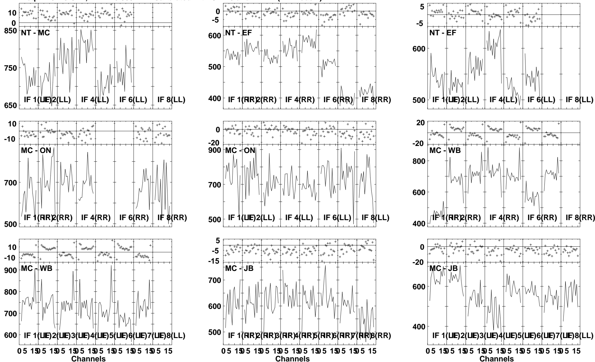
Lower frame: Milli Ampl Jy Top frame: Phas deg Vector averaged cross-power spectrum Several baselines displayed Timerange: 00/22:05:01 to 00/22:06:59
