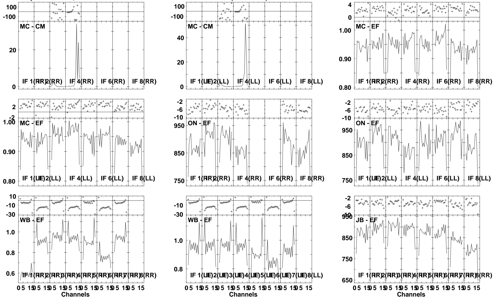
Lower frame: Ampl Jy Top frame: Phas deg Vector averaged cross-power spectrum Several baselines displayed Timerange: 01/00:24:31 to 01/00:26:29
