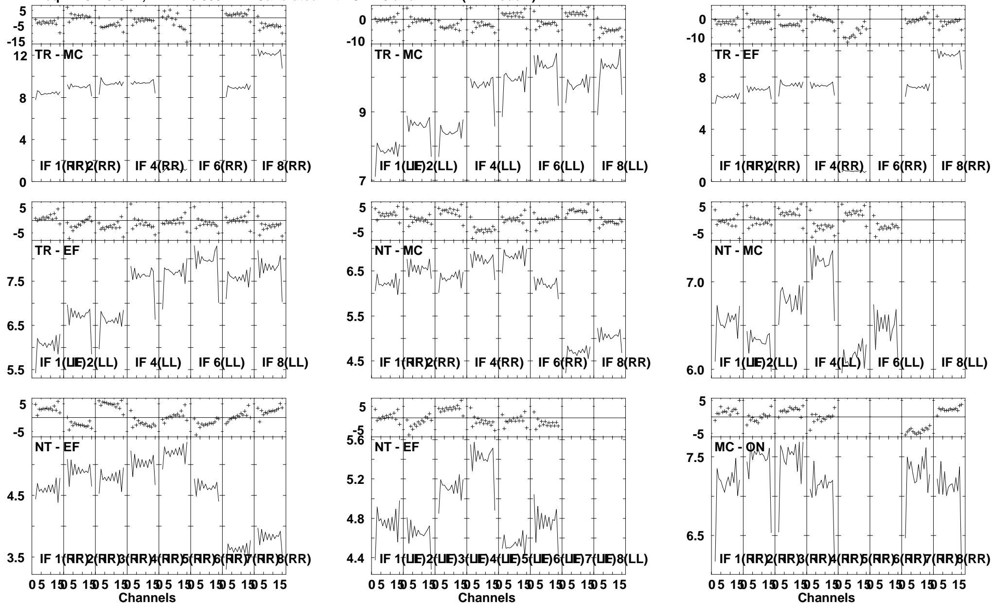
Lower frame: Ampl Jy Top frame: Phas deg Vector averaged cross-power spectrum Several baselines displayed Timerange: 01/03:23:02 to 01/03:24:29
