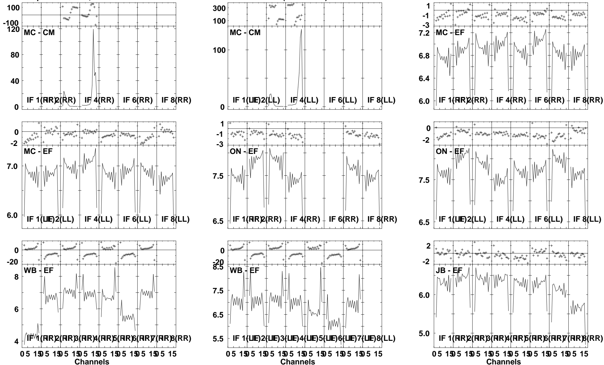
Lower frame: Ampl Jy Top frame: Phas deg Vector averaged cross-power spectrum Several baselines displayed Timerange: 00/23:38:02 to 00/23:39:29
