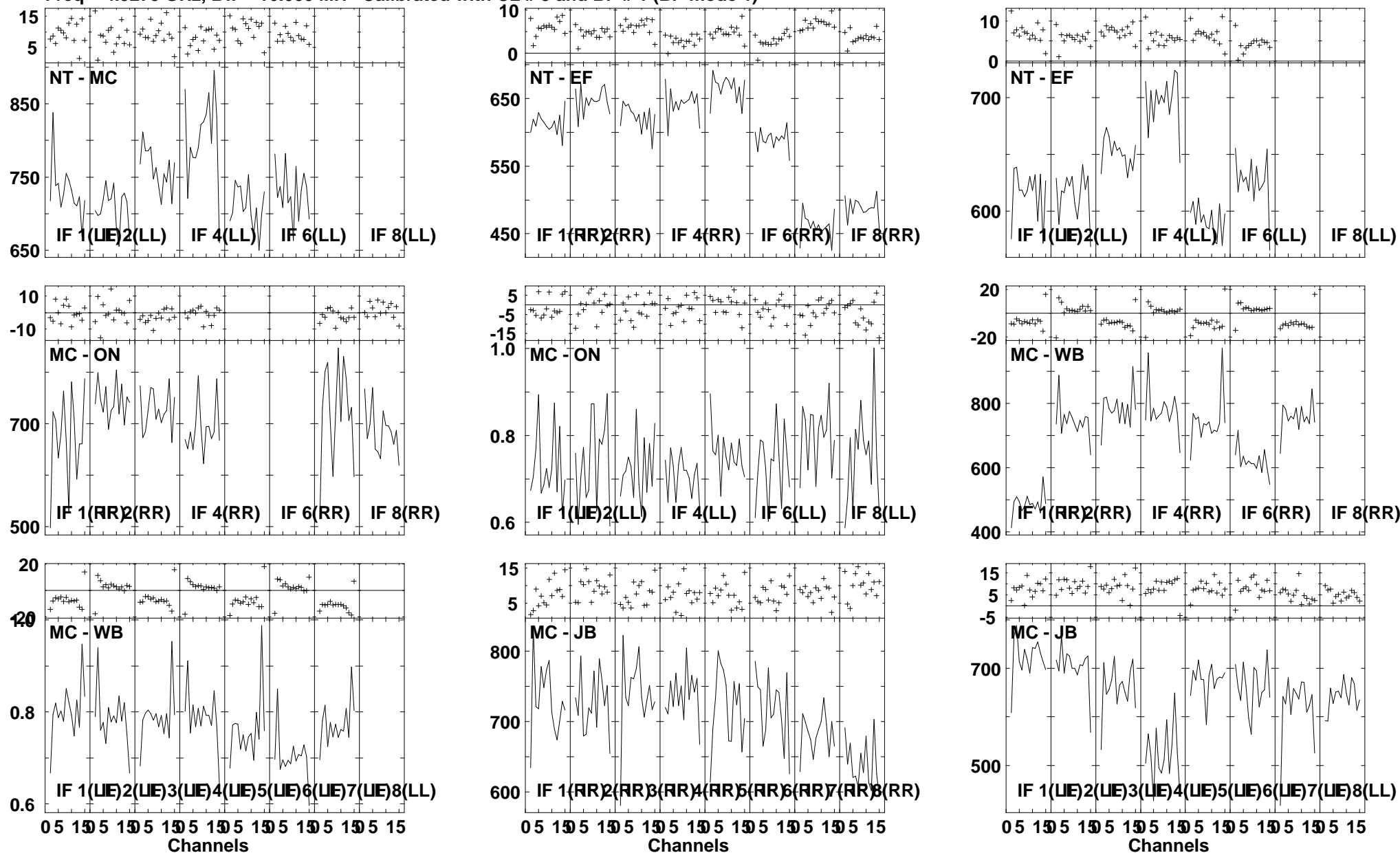
Lower frame: Milli Ampl Jy Top frame: Phas deg Vector averaged cross-power spectrum Several baselines displayed Timerange: 00/23:12:31 to 00/23:14:29
