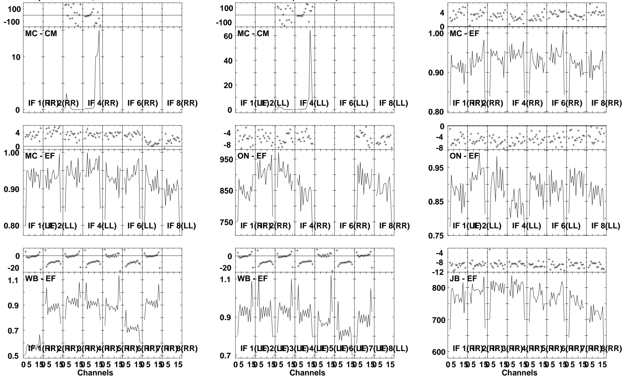
Lower frame: Ampl Jy Top frame: Phas deg Vector averaged cross-power spectrum Several baselines displayed Timerange: 00/22:50:01 to 00/22:51:59
