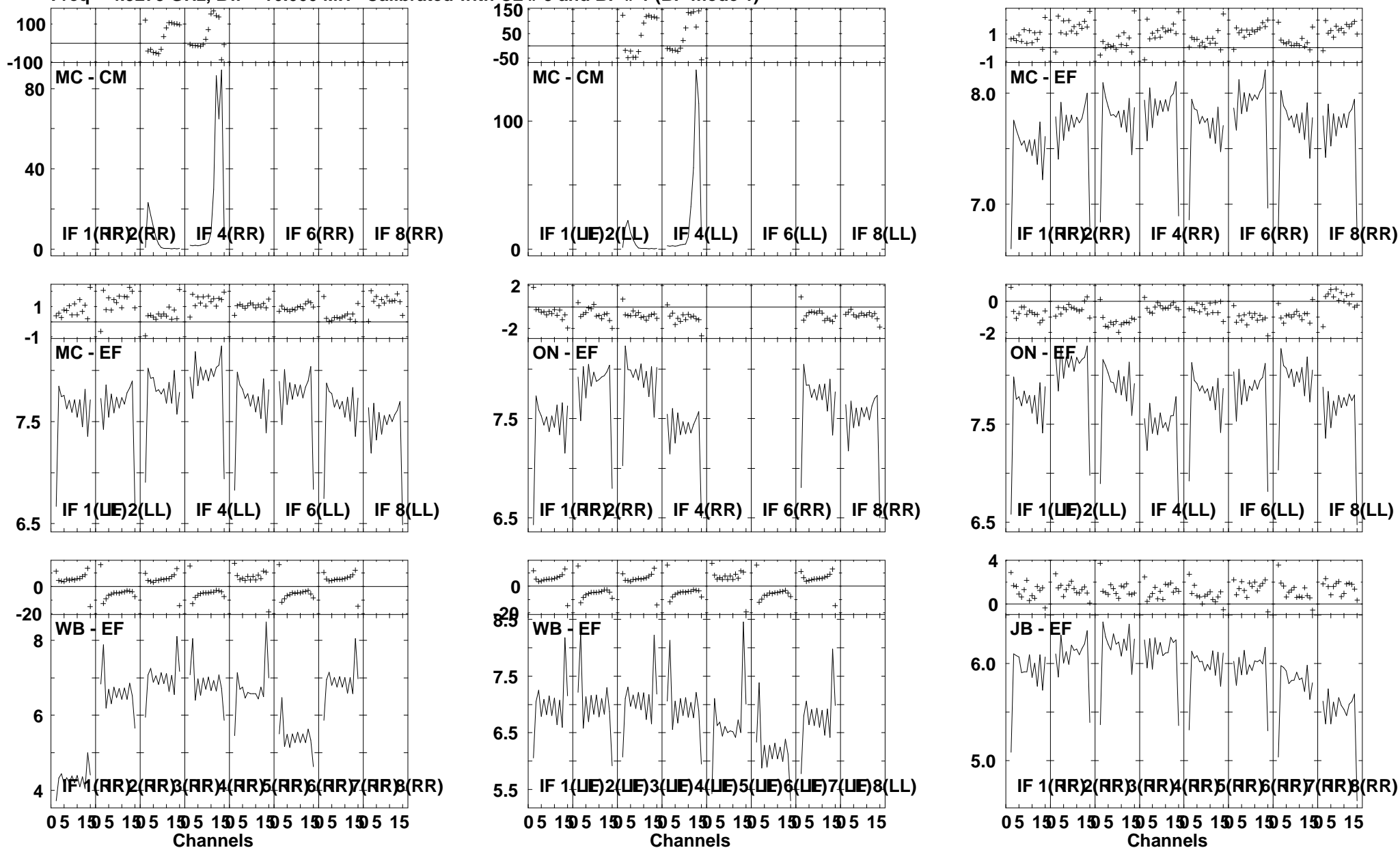
Lower frame: Ampl Jy Top frame: Phas deg Vector averaged cross-power spectrum Several baselines displayed Timerange: 00/22:30:54 to 00/22:31:59
