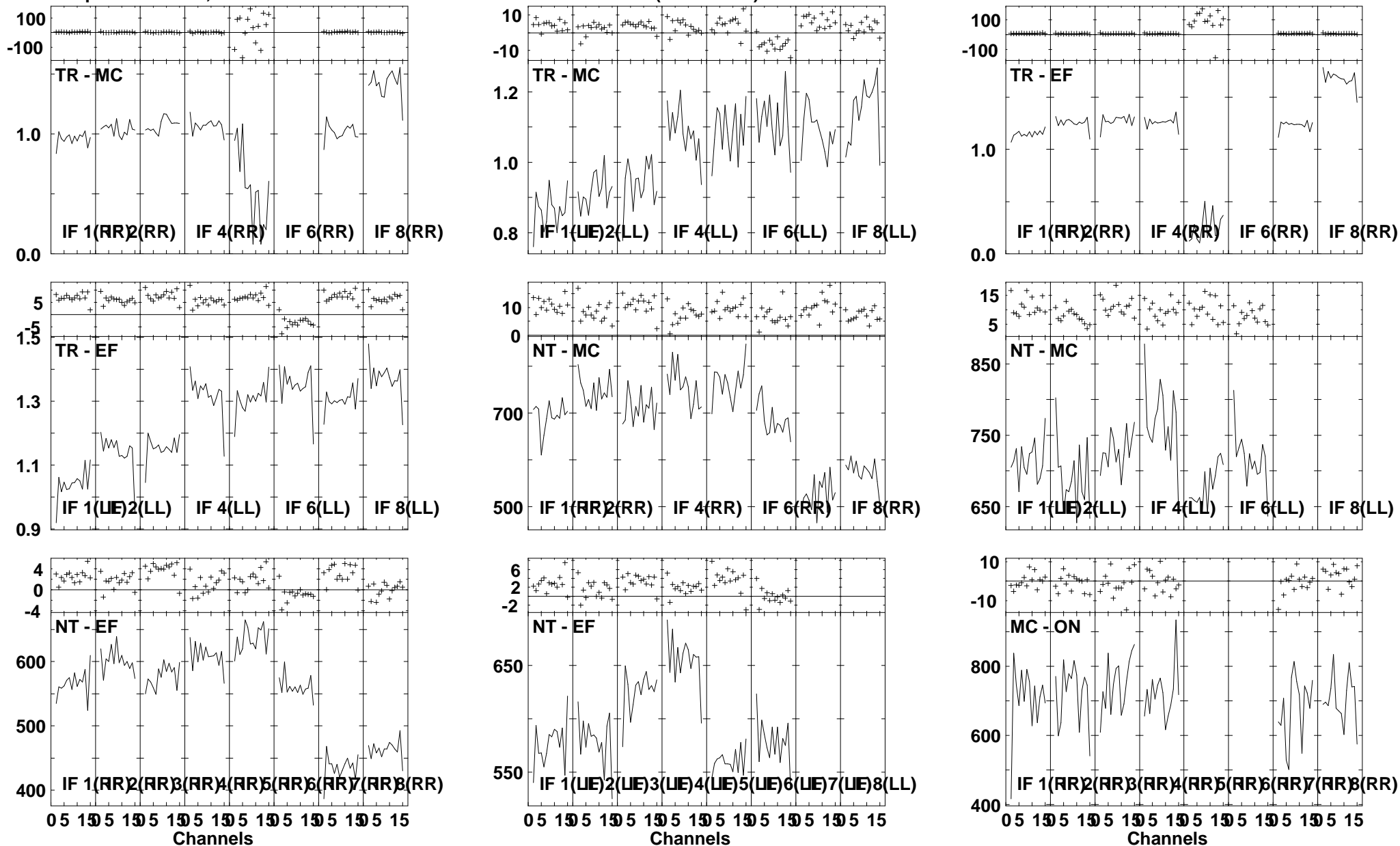
Lower frame: Ampl Jy Top frame: Phas deg Vector averaged cross-power spectrum Several baselines displayed Timerange: 01/04:50:01 to 01/04:51:59
