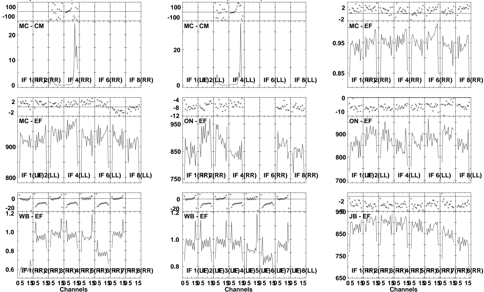
Lower frame: Ampl Jy Top frame: Phas deg Vector averaged cross-power spectrum Several baselines displayed Timerange: 01/00:47:01 to 01/00:48:59
