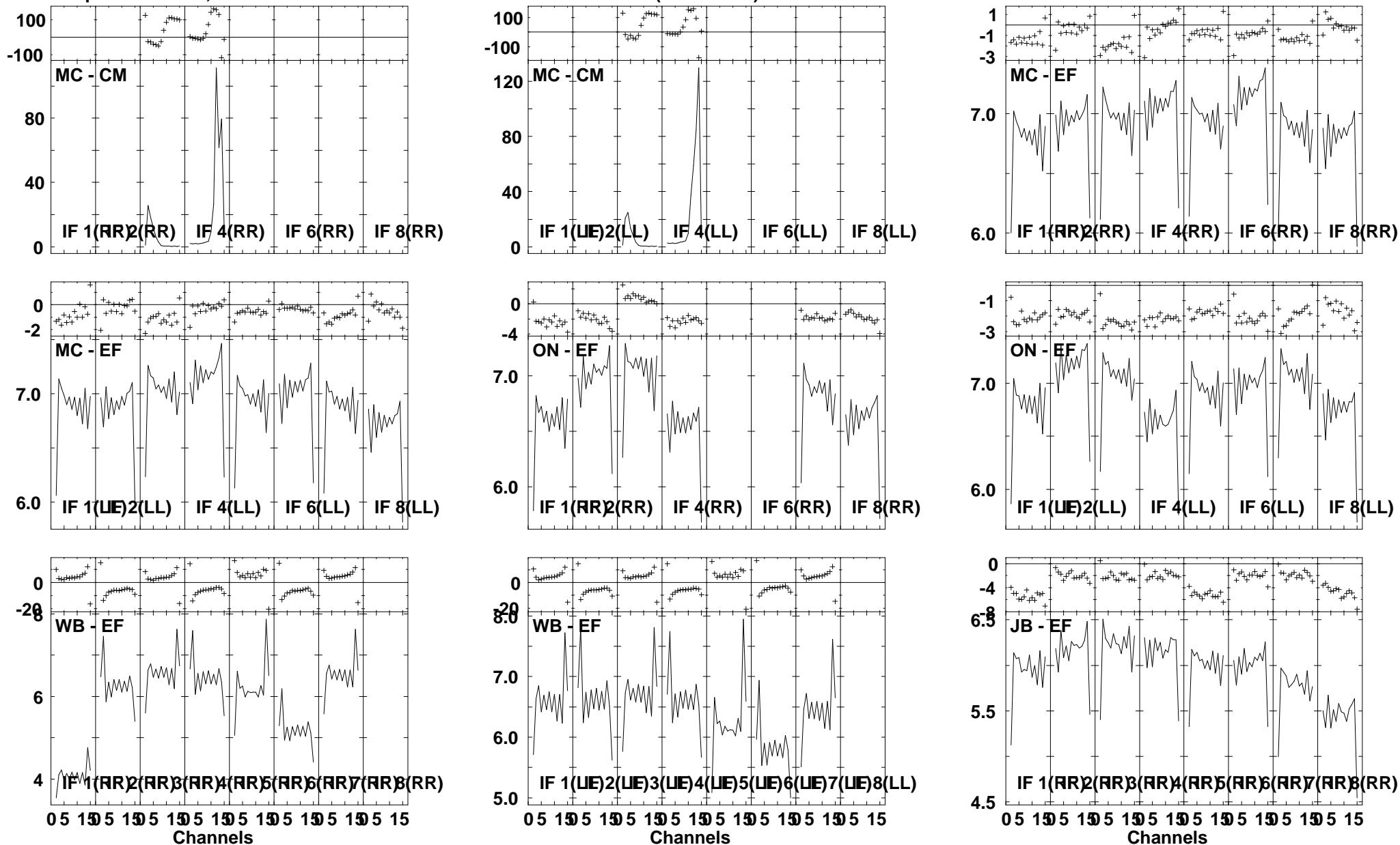
Lower frame: Ampl Jy Top frame: Phas deg Vector averaged cross-power spectrum Several baselines displayed Timerange: 01/00:23:02 to 01/00:24:29
