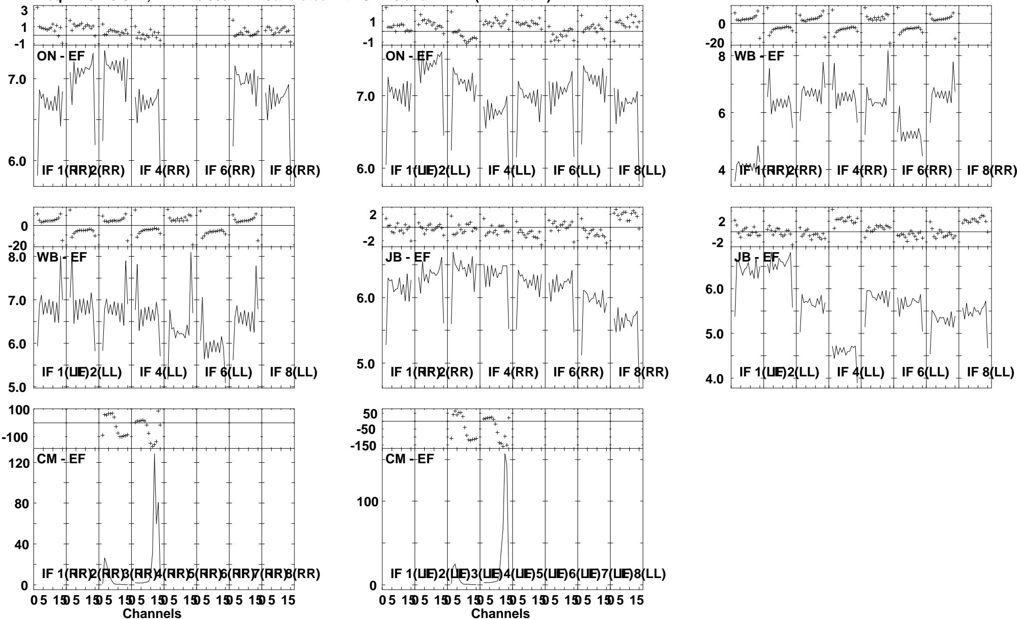
Lower frame: Ampl Jy Top frame: Phas deg Vector averaged cross-power spectrum Several baselines displayed Timerange: 01/01:08:02 to 01/01:09:29
