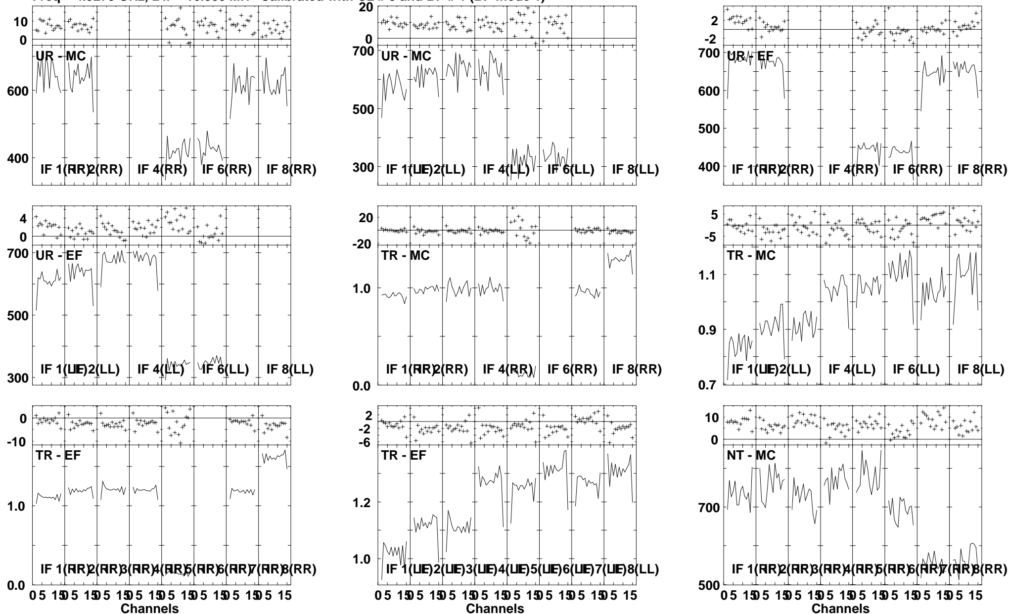
Lower frame: Milli Ampl Jy Top frame: Phas deg Vector averaged cross-power spectrum Several baselines displayed Timerange: 00/23:51:31 to 00/23:53:29
