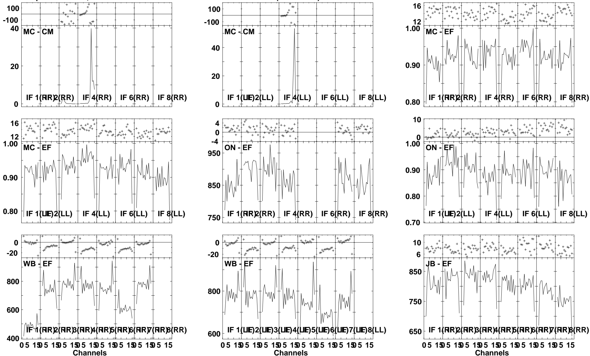
Lower frame: Ampl Jy Top frame: Phas deg Vector averaged cross-power spectrum Several baselines displayed Timerange: 00/22:32:01 to 00/22:33:59
