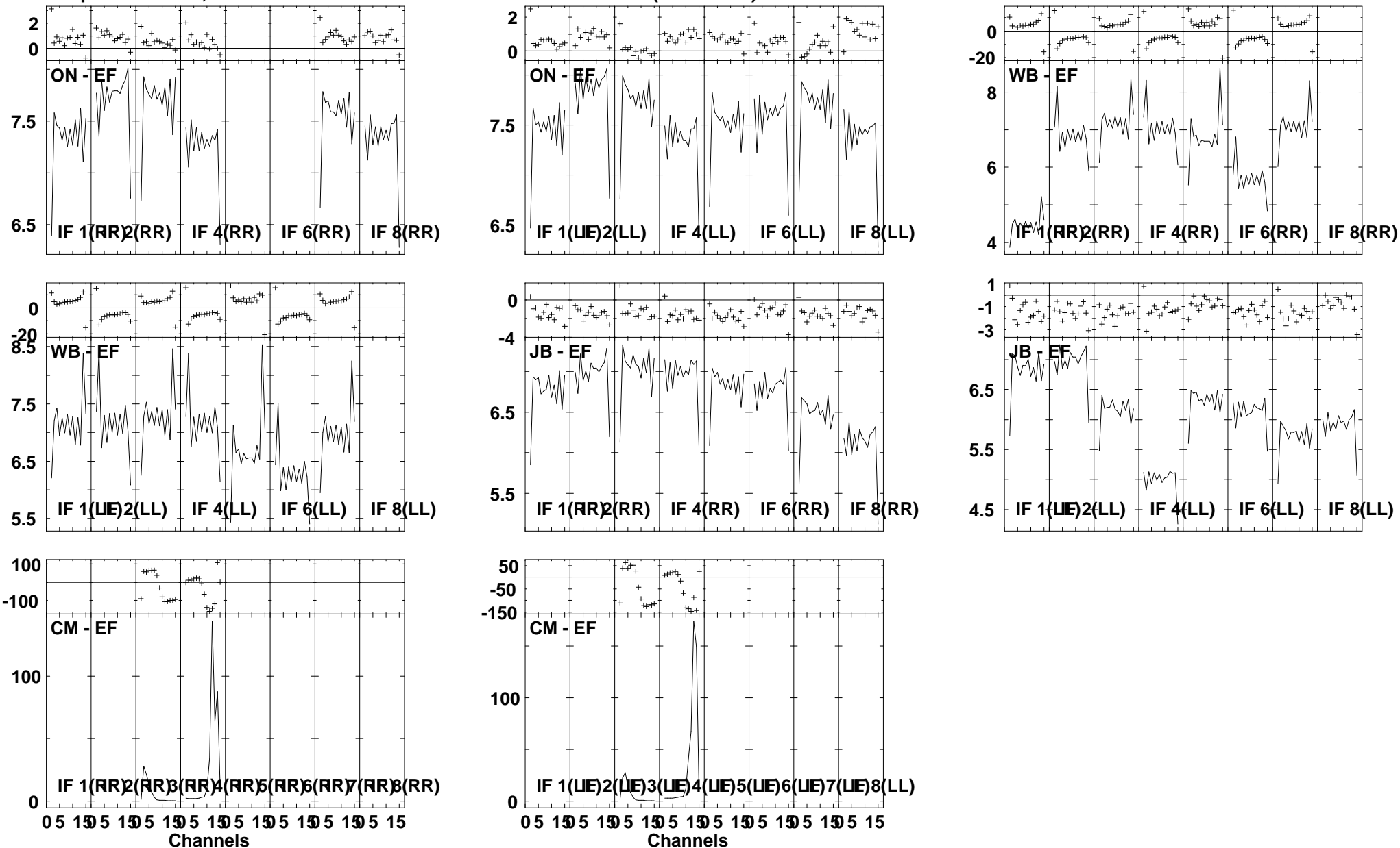
Lower frame: Ampl Jy Top frame: Phas deg Vector averaged cross-power spectrum Several baselines displayed Timerange: 01/01:53:24 to 01/01:54:29
