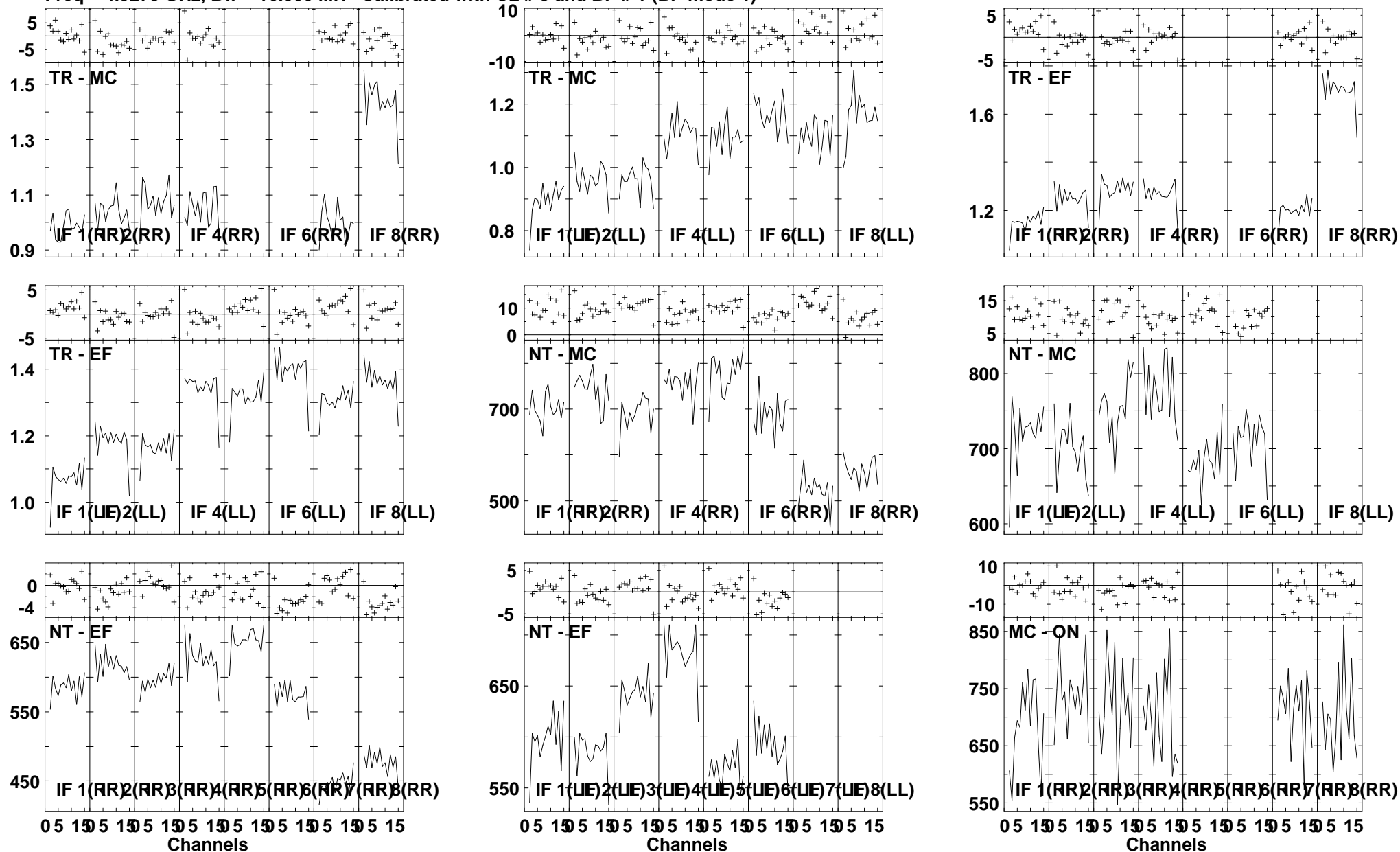
Lower frame: Ampl Jy Top frame: Phas deg Vector averaged cross-power spectrum Several baselines displayed Timerange: 01/04:21:31 to 01/04:23:29
