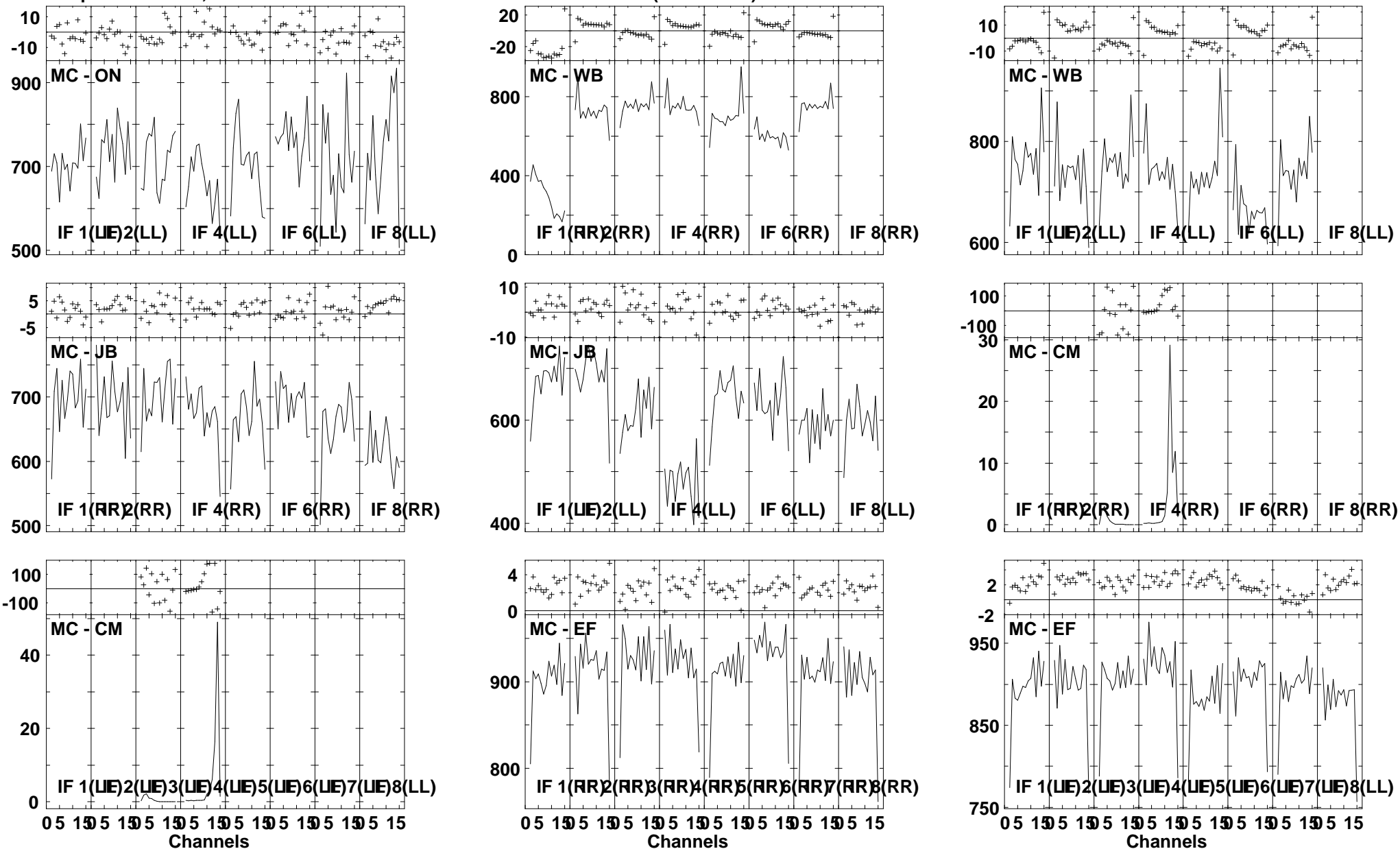
Lower frame: Milli Ampl Jy Top frame: Phas deg Vector averaged cross-power spectrum Several baselines displayed Timerange: 01/04:27:31 to 01/04:29:29
