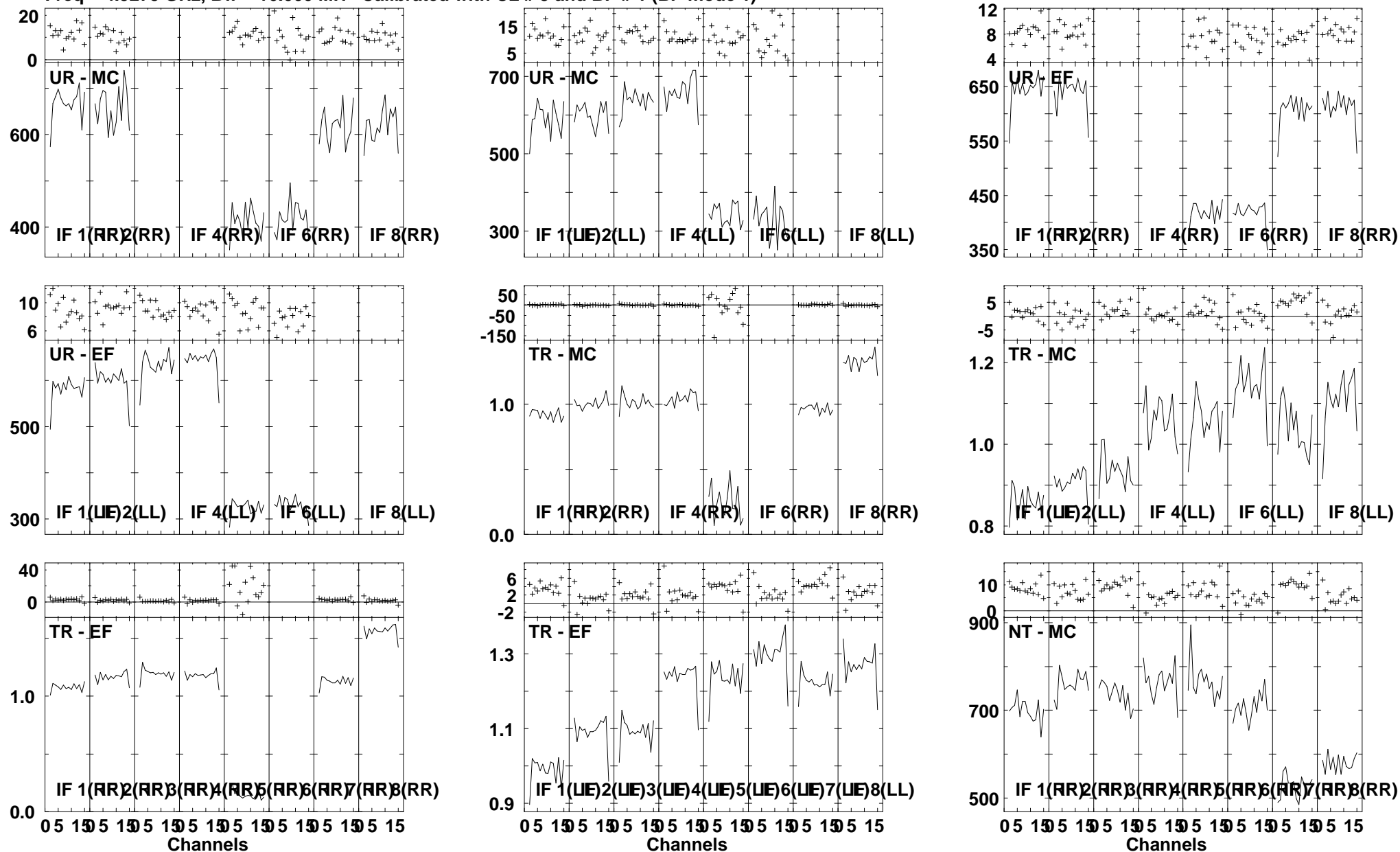
Lower frame: Milli Ampl Jy Top frame: Phas deg Vector averaged cross-power spectrum Several baselines displayed Timerange: 01/00:30:31 to 01/00:32:29
