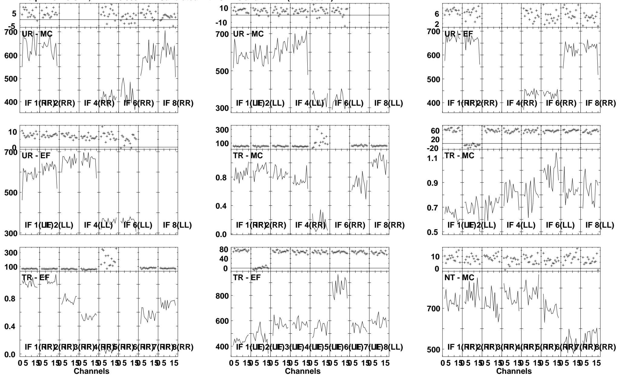
Lower frame: Milli Ampl Jy Top frame: Phas deg Vector averaged cross-power spectrum Several baselines displayed Timerange: 00/22:09:31 to 00/22:11:29
