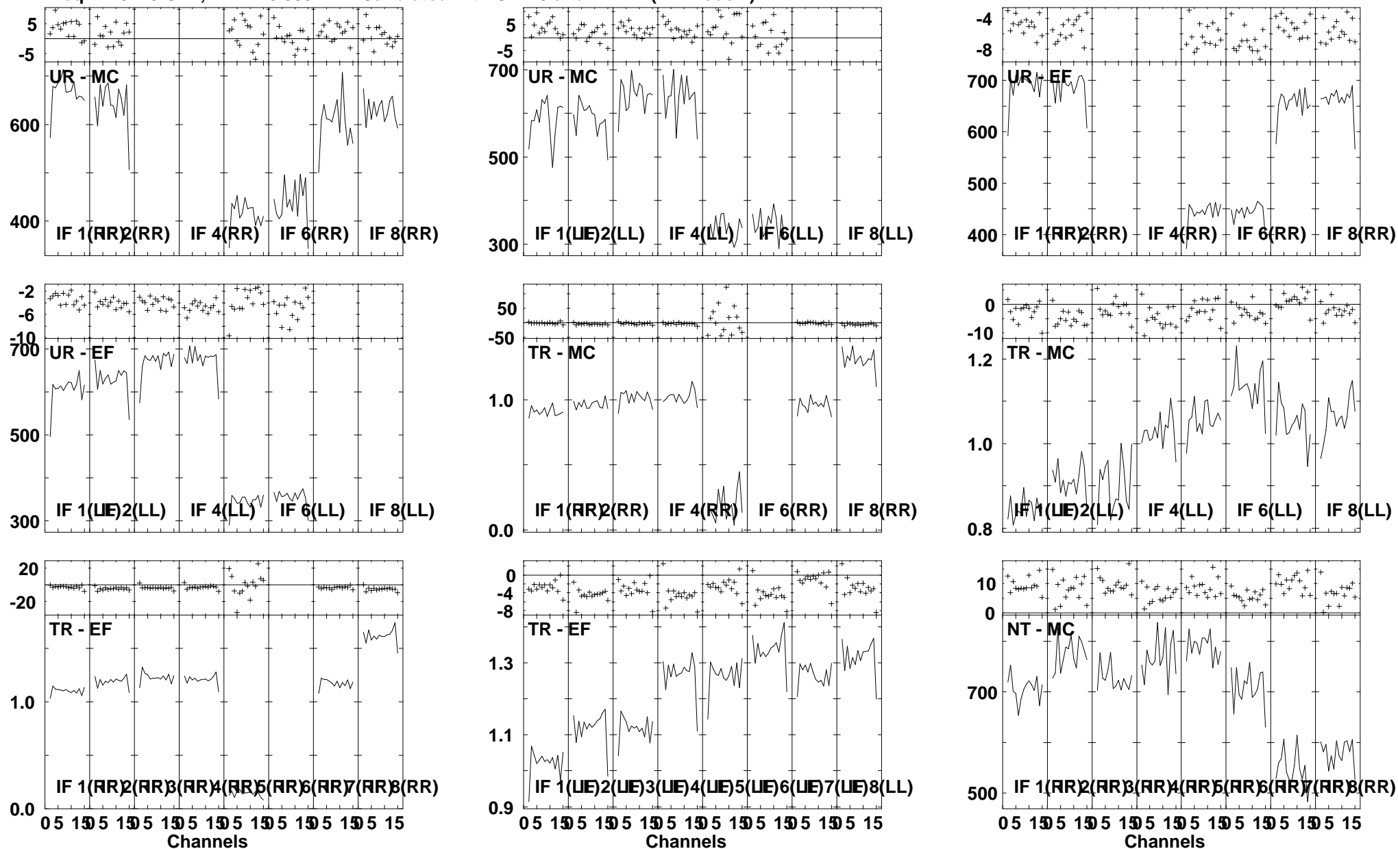
Lower frame: Milli Ampl Jy Top frame: Phas deg Vector averaged cross-power spectrum Several baselines displayed Timerange: 00/23:35:01 to 00/23:36:59
