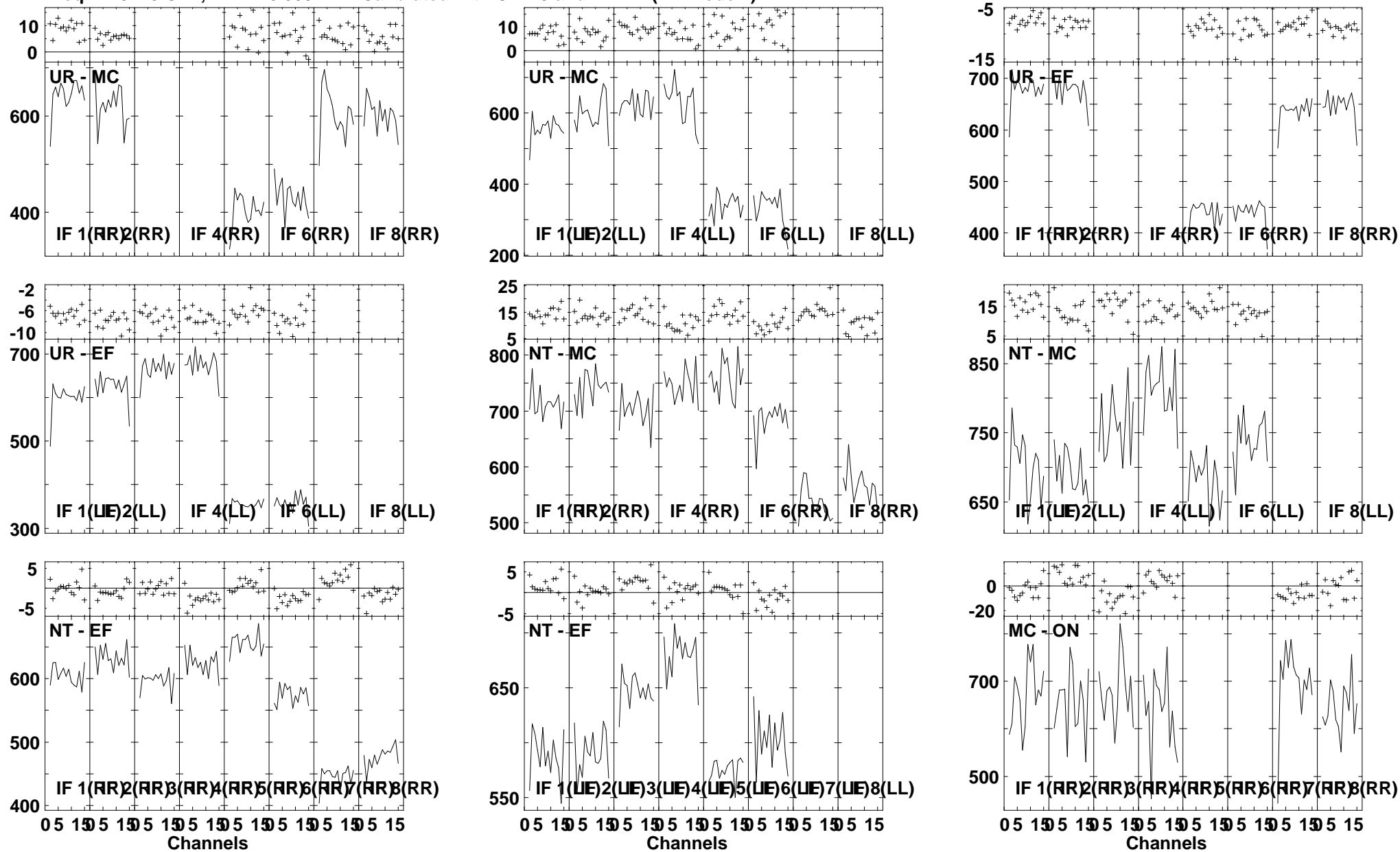
Lower frame: Milli Ampl Jy Top frame: Phas deg Vector averaged cross-power spectrum Several baselines displayed Timerange: 00/22:21:31 to 00/22:23:29
