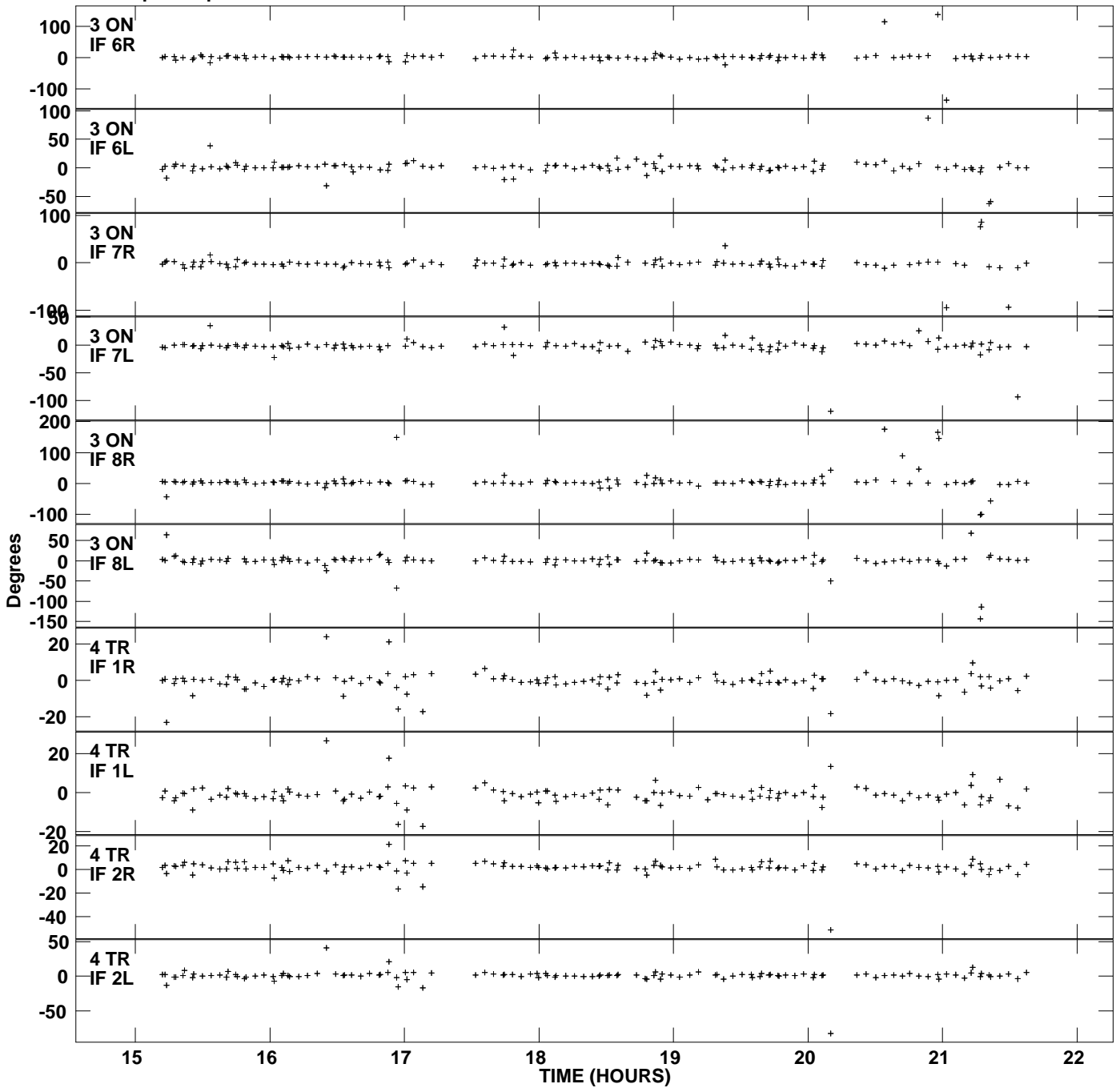
Plot file version 5 created 12-FEB-2010 15:59:05 Gain phs vs UTC time for 0448-095.MULTI.1 SN 1 Rpol & Lpol IF 1 - 8
