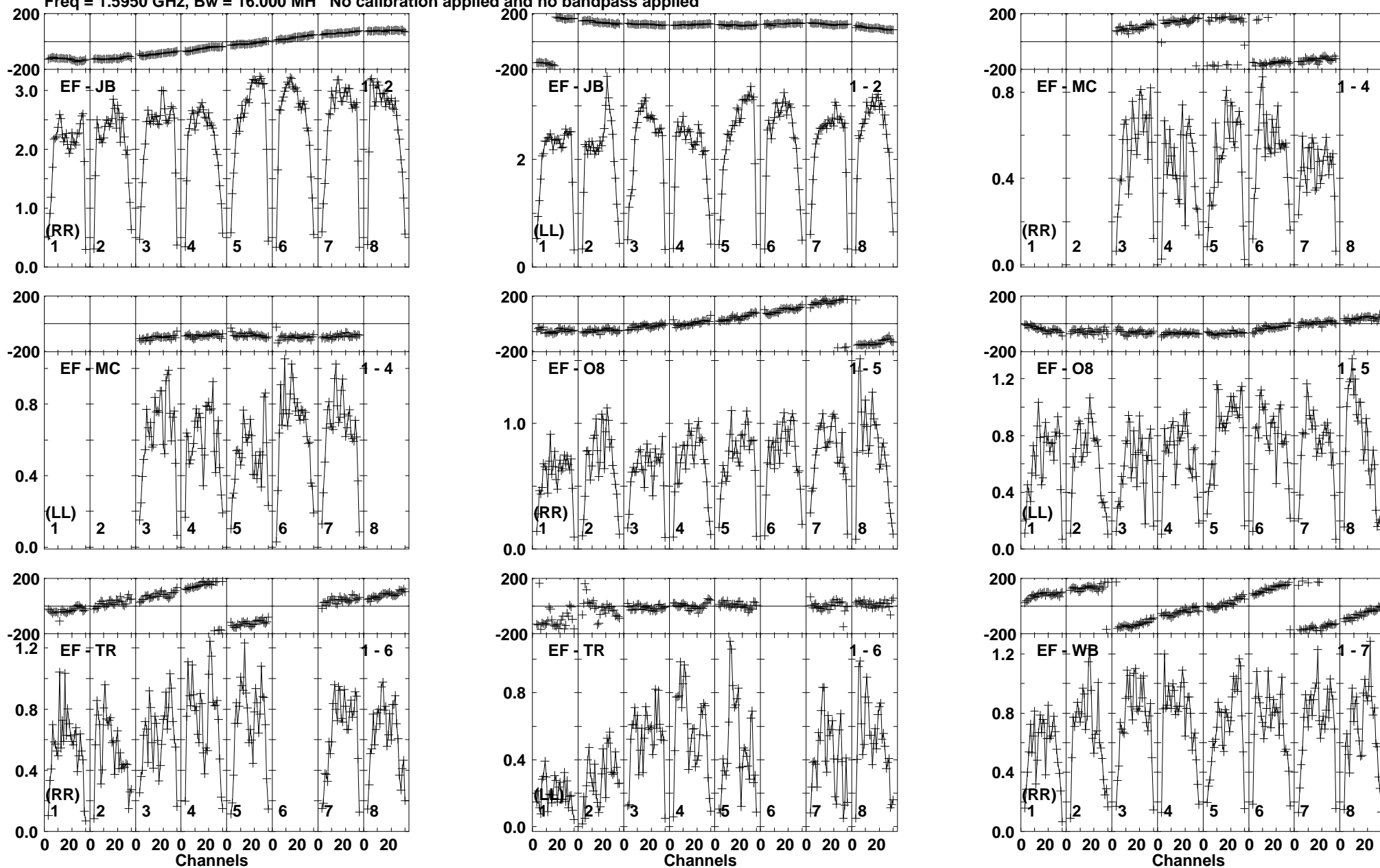
Lower frame: Milli Ampl Jy Top frame: Phas deg Vector averaged cross-power spectrum Baseline: EF (01) - JB (02) Timerange: 00:18:33:43 to 00:18:34:39
