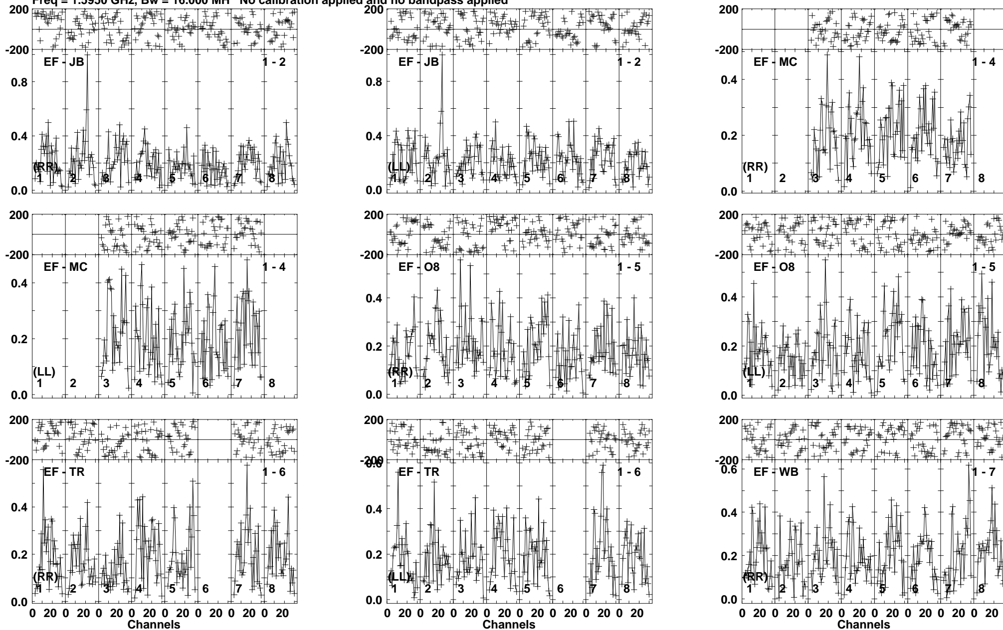
Lower frame: Milli Ampl Jy Top frame: Phas deg Vector averaged cross-power spectrum Baseline: EF (01) - JB (02) Timerange: 00/18:50:53 to 00/18:51:29
