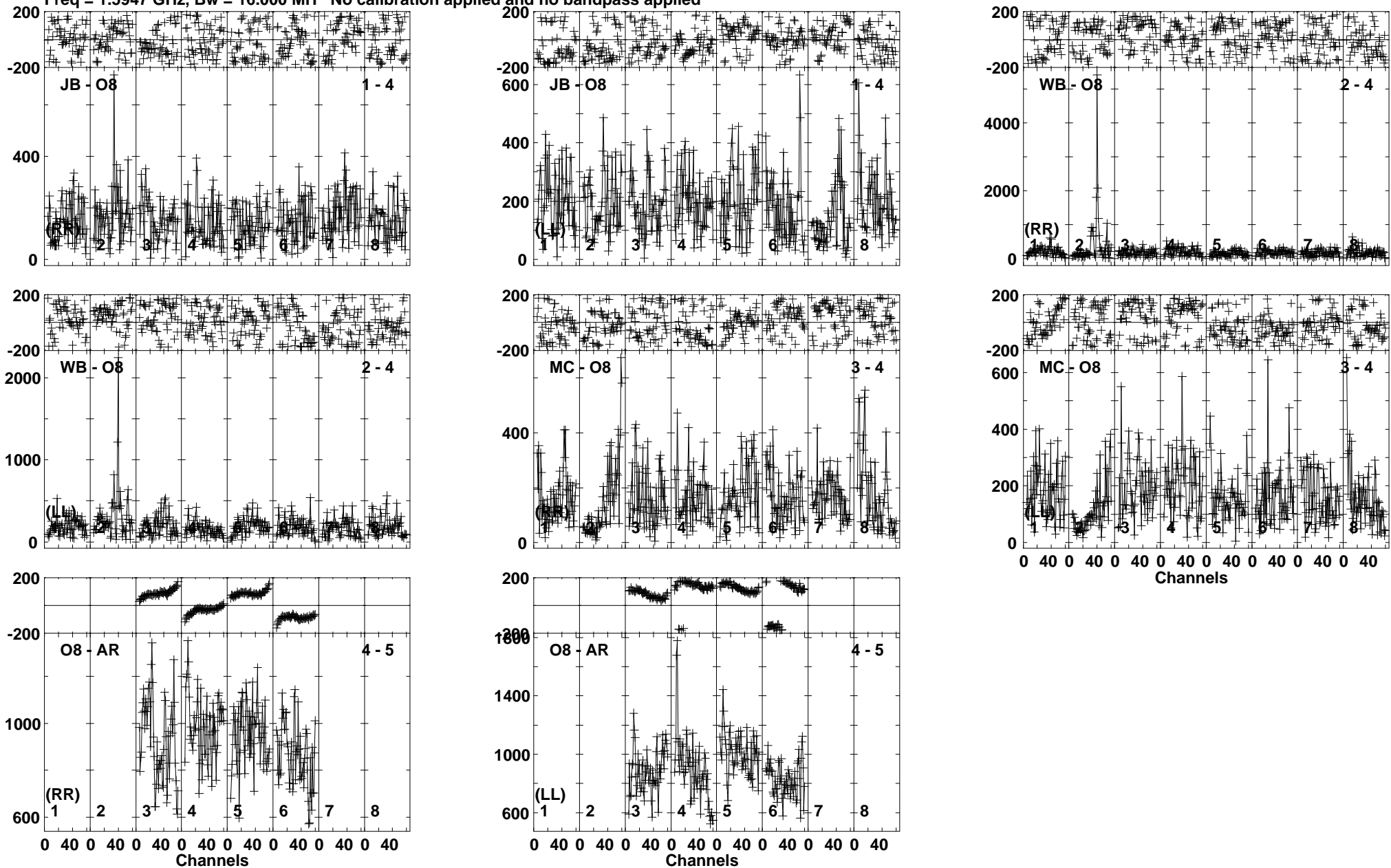
Lower frame: Micro Ampl Jy Top frame: Phas deg Vector averaged cross-power spectrum Baseline: JB (01) - O8 (04) Timerange: 00/10:20:51 to 00/10:22:09
