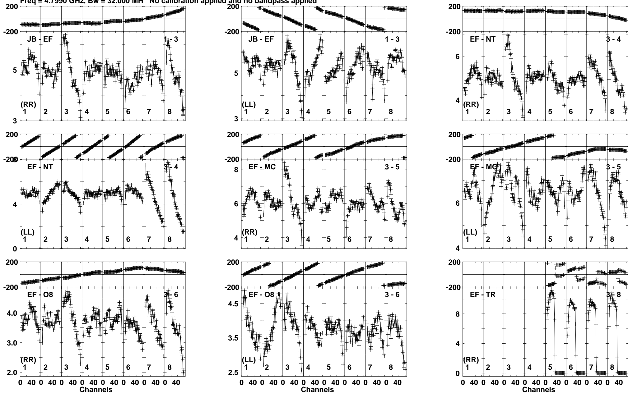
Lower frame: Milli Ampl Jy Top frame: Phas deg Vector averaged cross-power spectrum Baseline: JB (01) - EF (03) Timerange: 00/11:44:58 to 00/11:46:27
