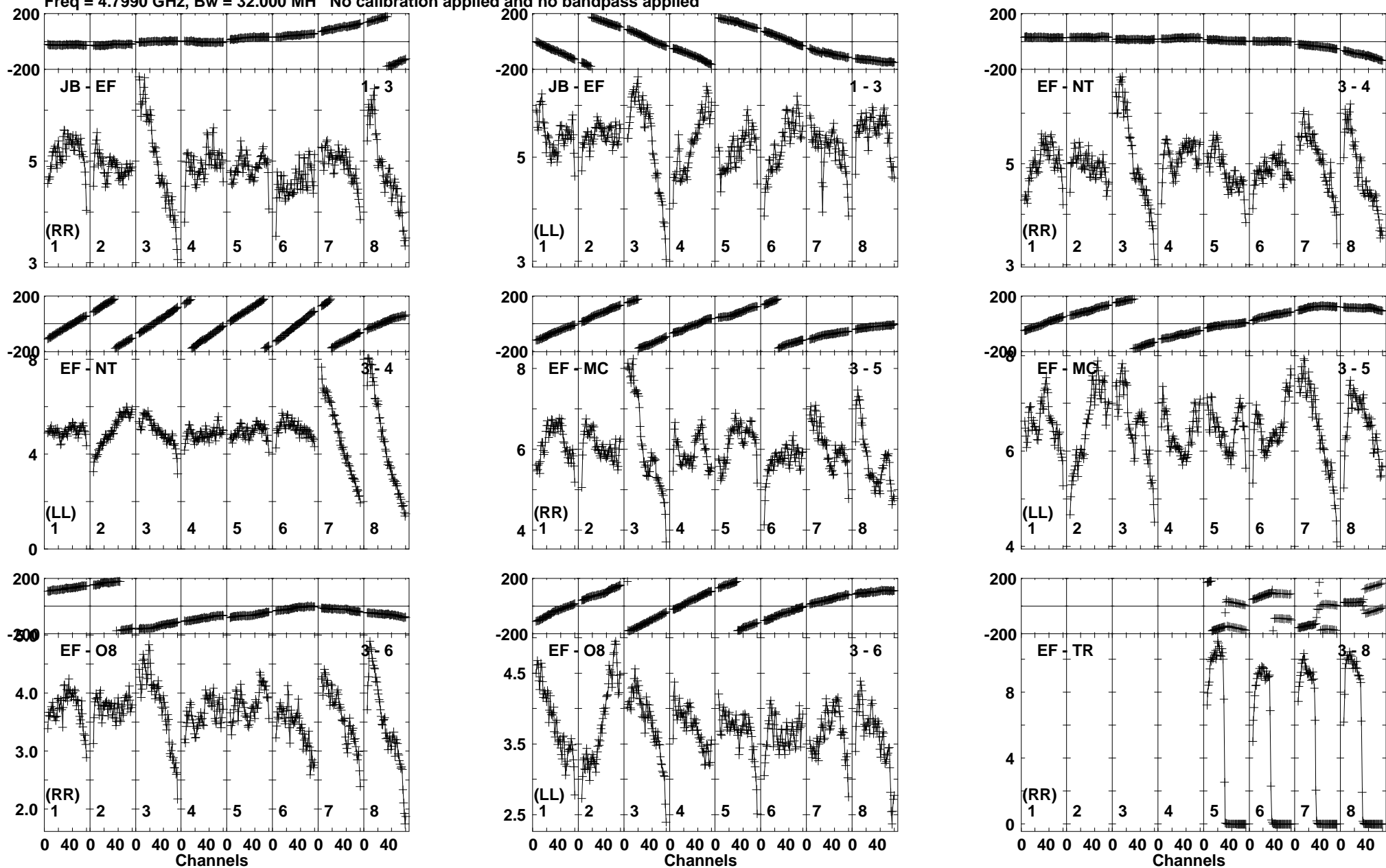
Lower frame: Milli Ampl Jy Top frame: Phas deg Vector averaged cross-power spectrum Baseline: JB (01) - EF (03) Timerange: 00/11:22:47 to 00/11:24:15
