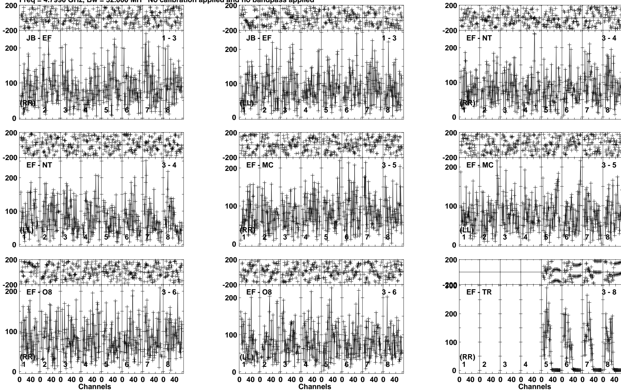
Lower frame: Micro Ampl Jy Top frame: Phas deg Vector averaged cross-power spectrum Baseline: JB (01) - EF (03) Timerange: 00/09:39:07 to 00/09:42:49
