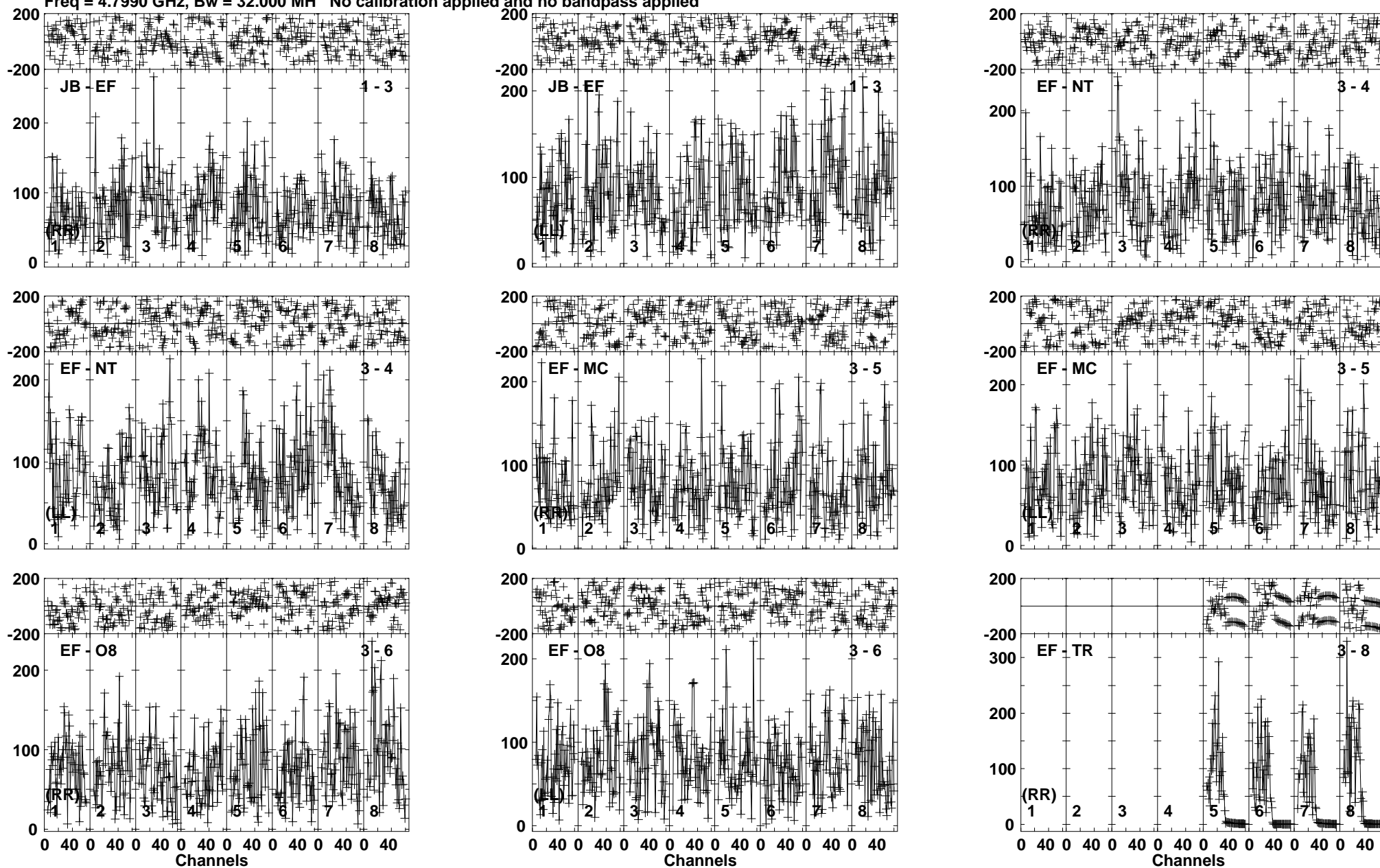
Lower frame: Micro Ampl Jy Top frame: Phas deg Vector averaged cross-power spectrum Baseline: JB (01) - EF (03) Timerange: 00/09:49:41 to 00/09:53:23
