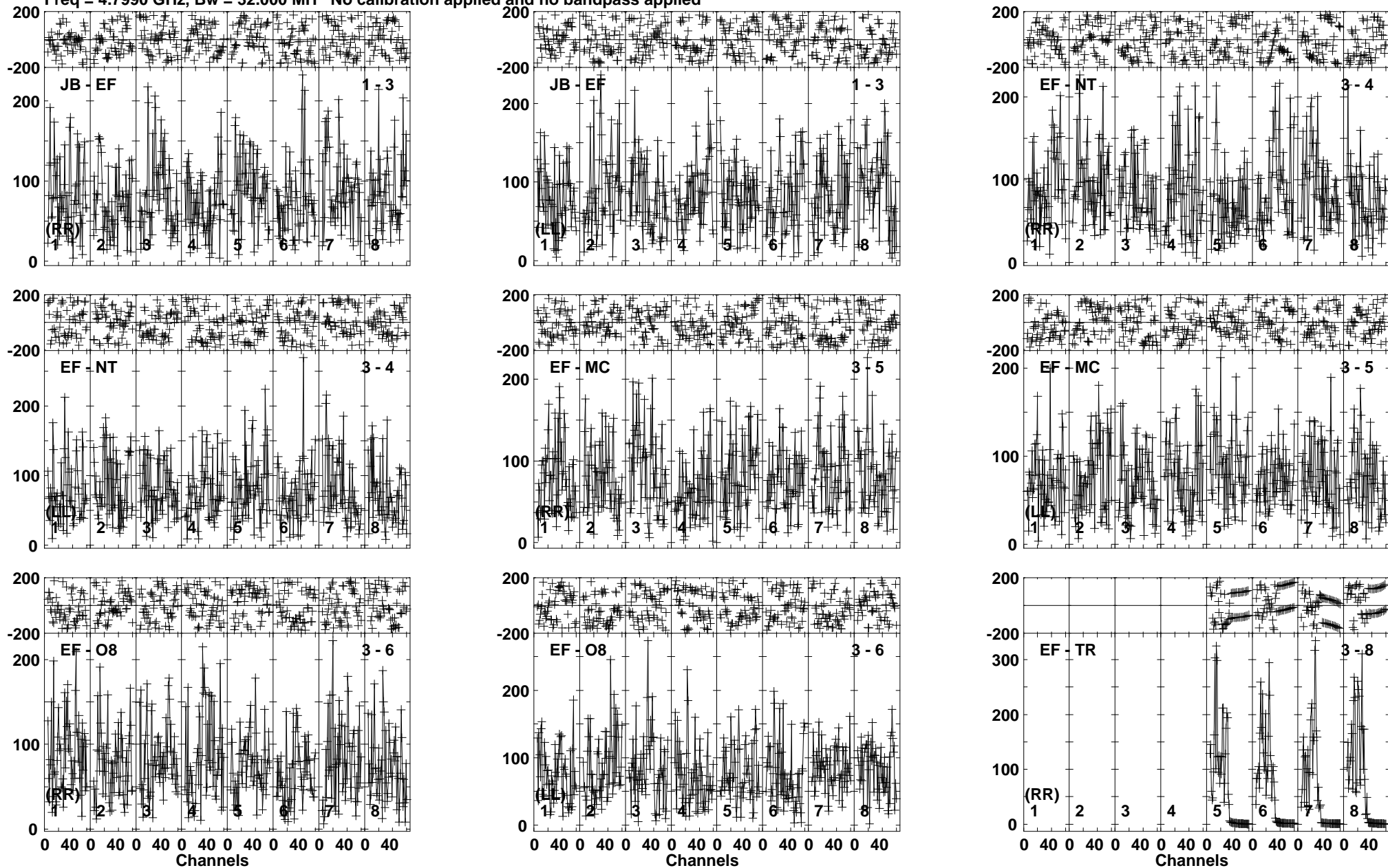
Lower frame: Micro Ampl Jy Top frame: Phas deg Vector averaged cross-power spectrum Baseline: JB (01) - EF (03) Timerange: 00/10:26:35 to 00/10:30:14
