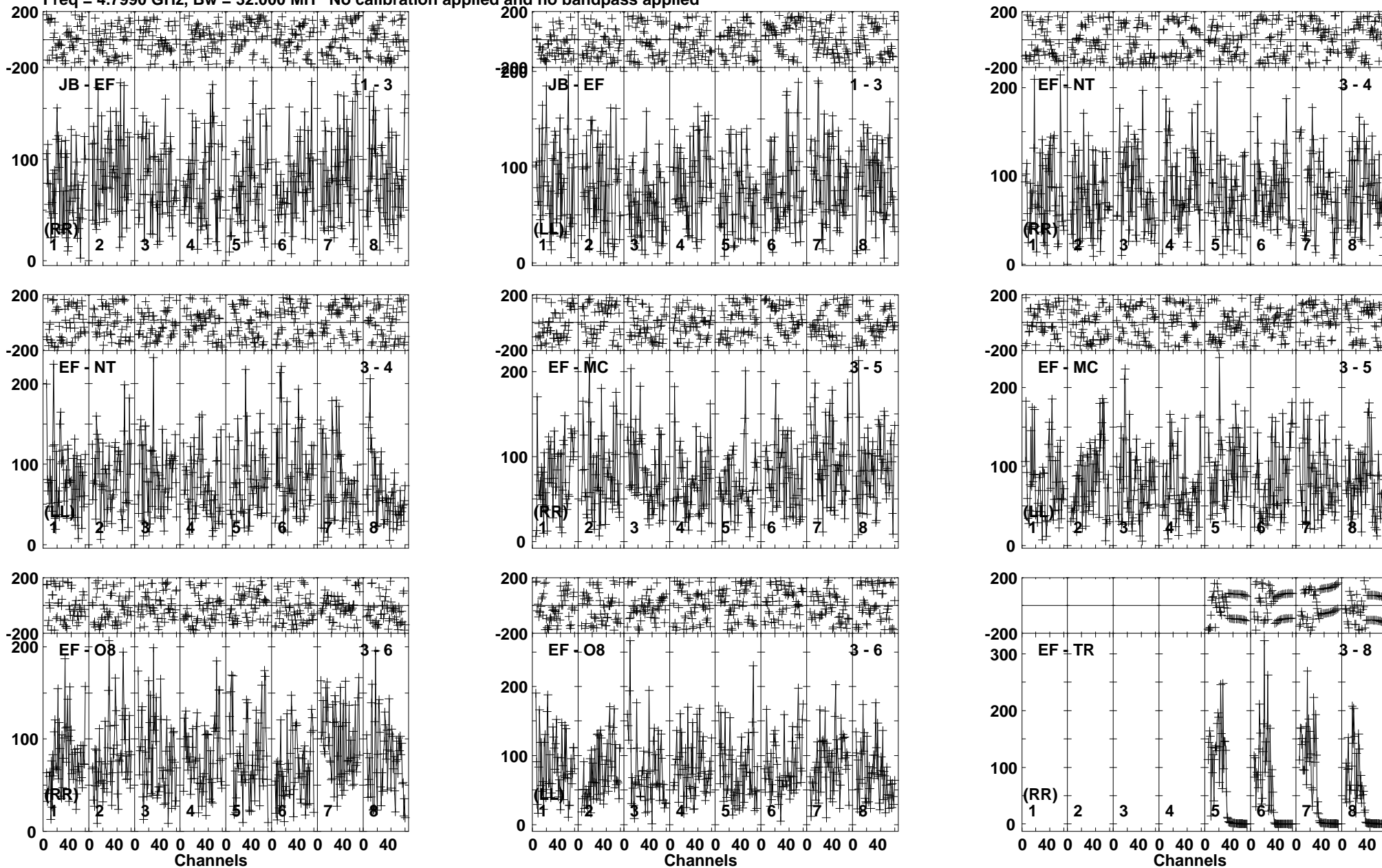
Lower frame: Micro Ampl Jy Top frame: Phas deg Vector averaged cross-power spectrum Baseline: JB (01) - EF (03) Timerange: 00/09:28:39 to 00/09:32:22
