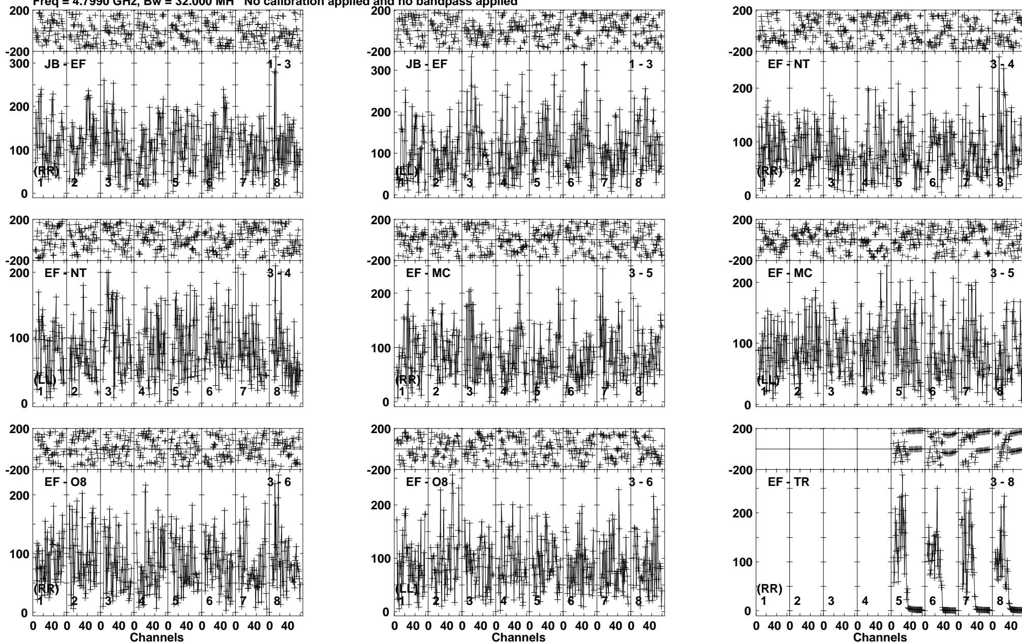
Lower frame: Micro Ampl Jy Top frame: Phas deg Vector averaged cross-power spectrum Baseline: JB (01) - EF (03) Timerange: 00/12:03:30 to 00/12:07:10
