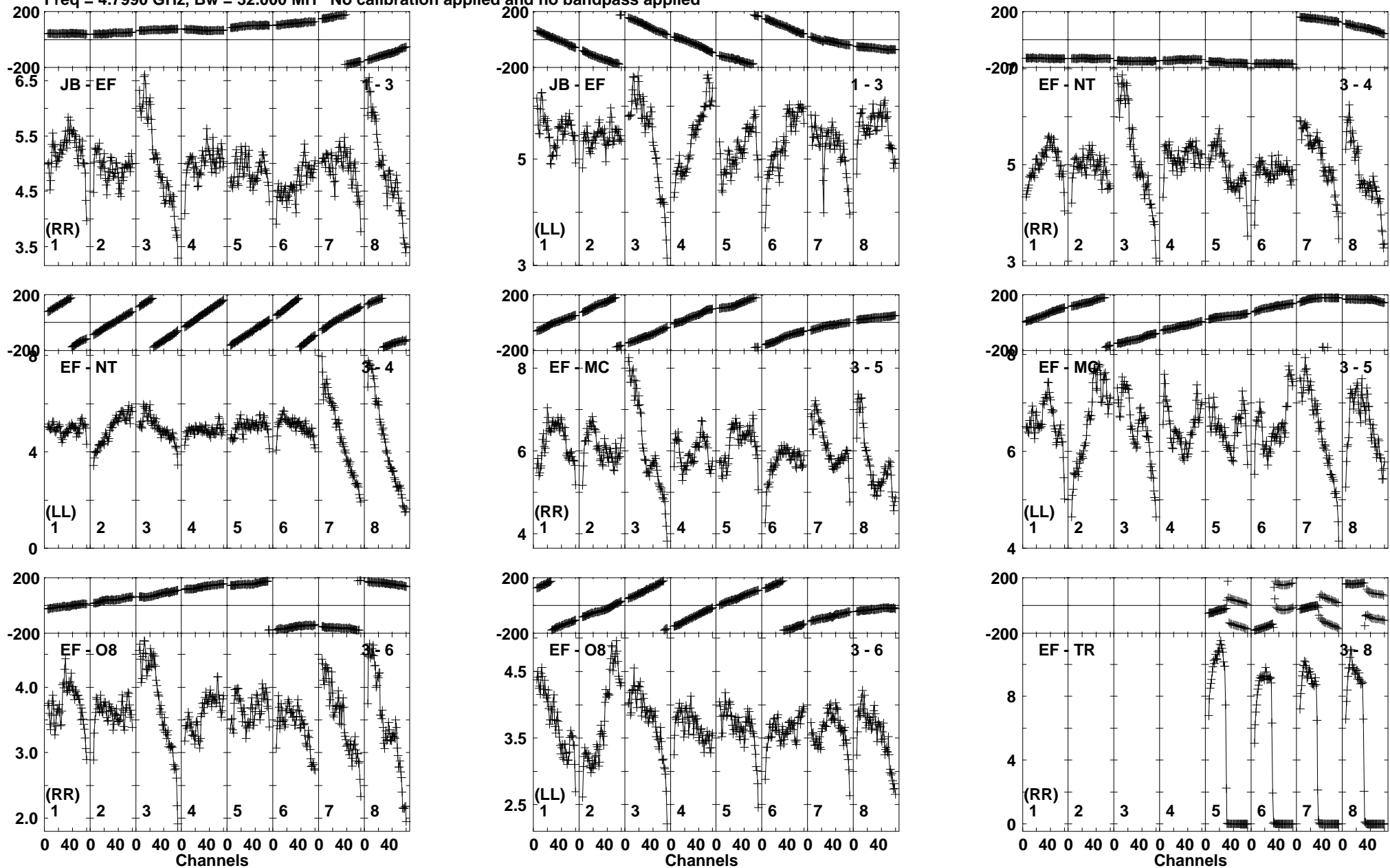
Lower frame: Milli Ampl Jy Top frame: Phas deg Vector averaged cross-power spectrum Baseline: JB (01) - EF (03) Timerange: 00/10:57:10 to 00/10:58:00
