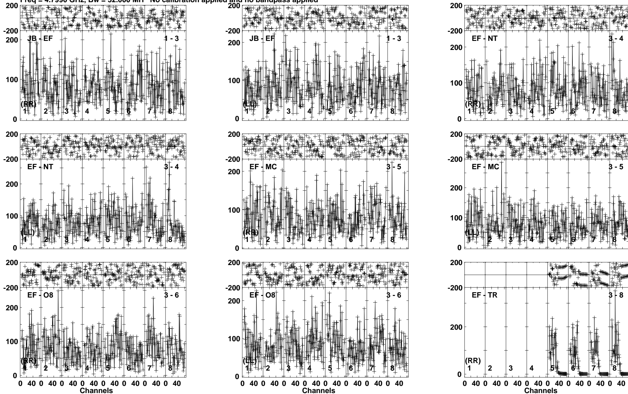
Lower frame: Micro Ampl Jy Top frame: Phas deg Vector averaged cross-power spectrum Baseline: JB (01) - EF (03) Timerange: 00/08:51:48 to 00/08:55:31
