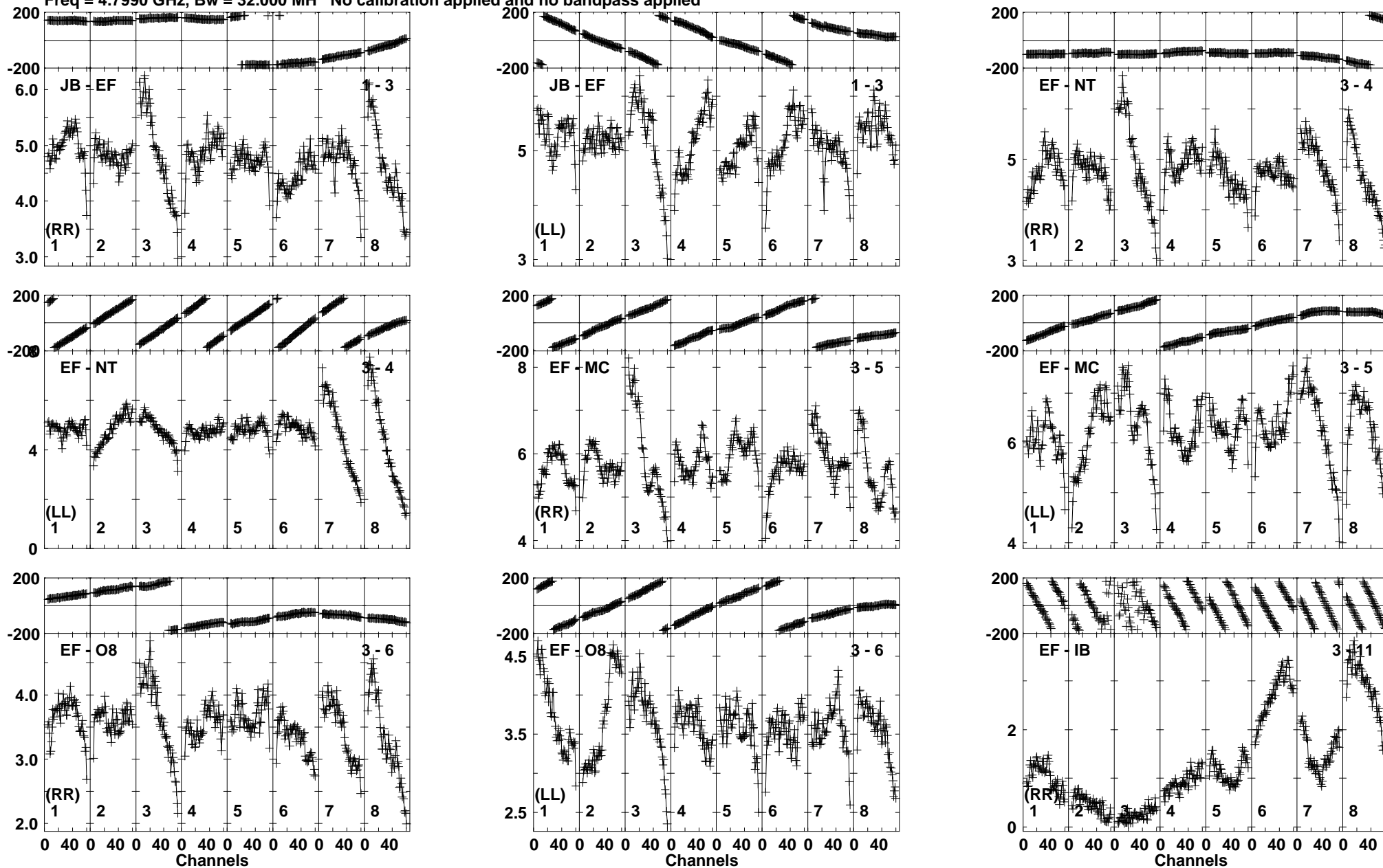
Lower frame: Milli Ampl Jy Top frame: Phas deg Vector averaged cross-power spectrum Baseline: JB (01) - EF (03) Timerange: 00/12:58:00 to 00/13:00:00
