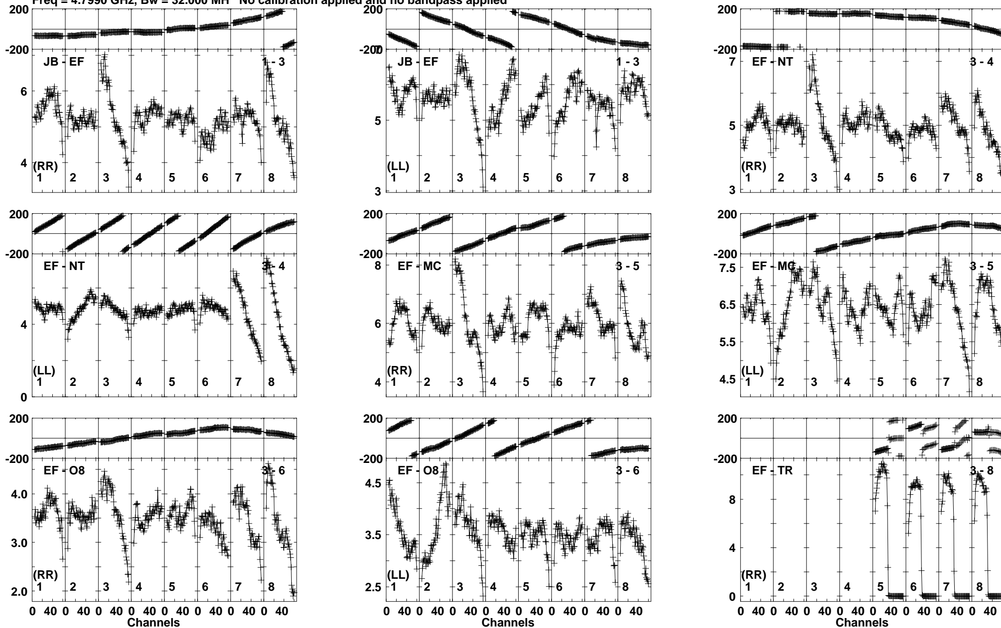
Lower frame: Milli Ampl Jy Top frame: Phas deg Vector averaged cross-power spectrum Baseline: JB (01) - EF (03) Timerange: 00/08:45:04 to 00/08:46:34
