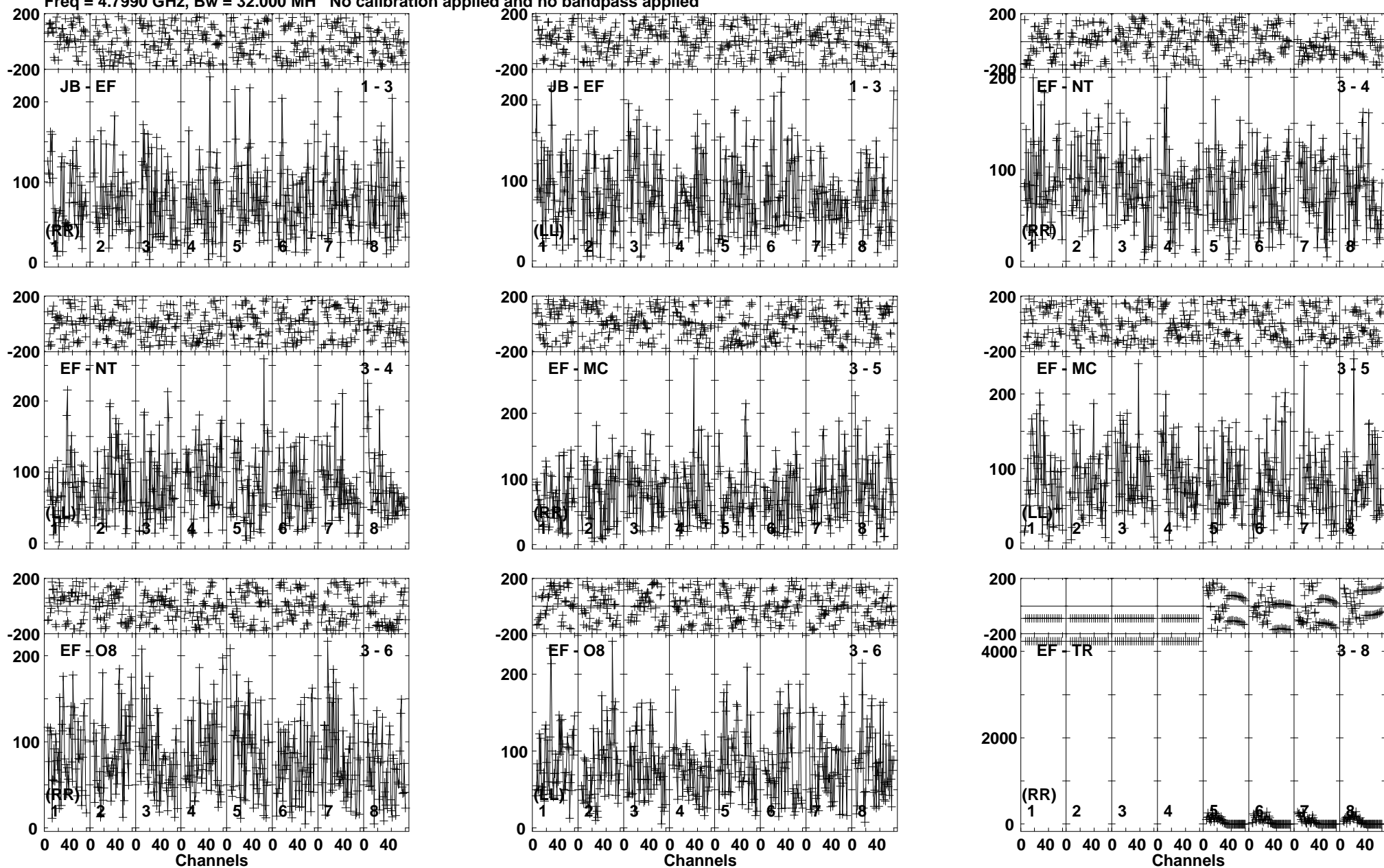
Lower frame: Micro Ampl Jy Top frame: Phas deg Vector averaged cross-power spectrum Baseline: JB (01) - EF (03) Timerange: 00/09:07:37 to 00/09:11:20
