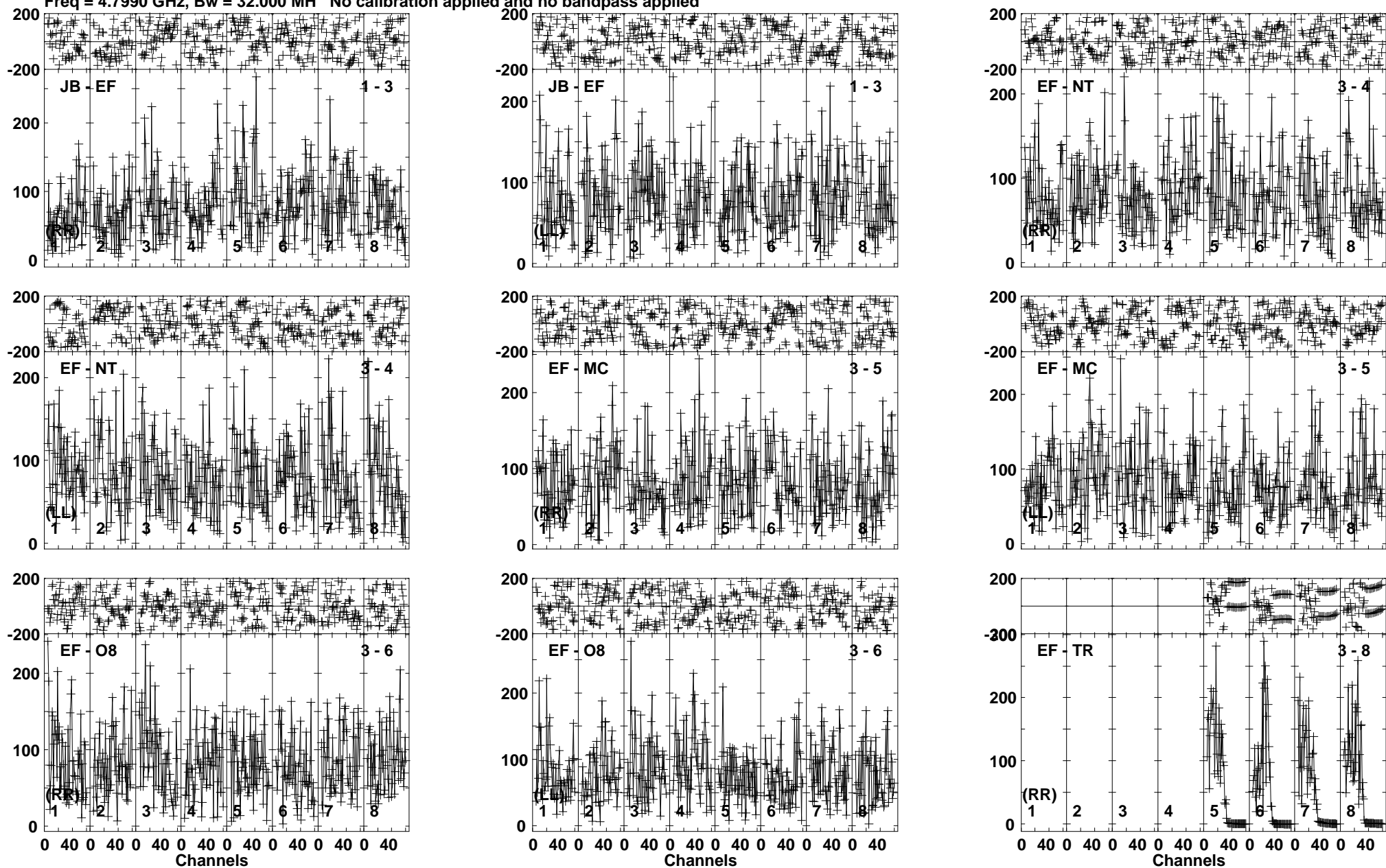
Lower frame: Micro Ampl Jy Top frame: Phas deg Vector averaged cross-power spectrum Baseline: JB (01) - EF (03) Timerange: 00/11:13:48 to 00/11:17:31
