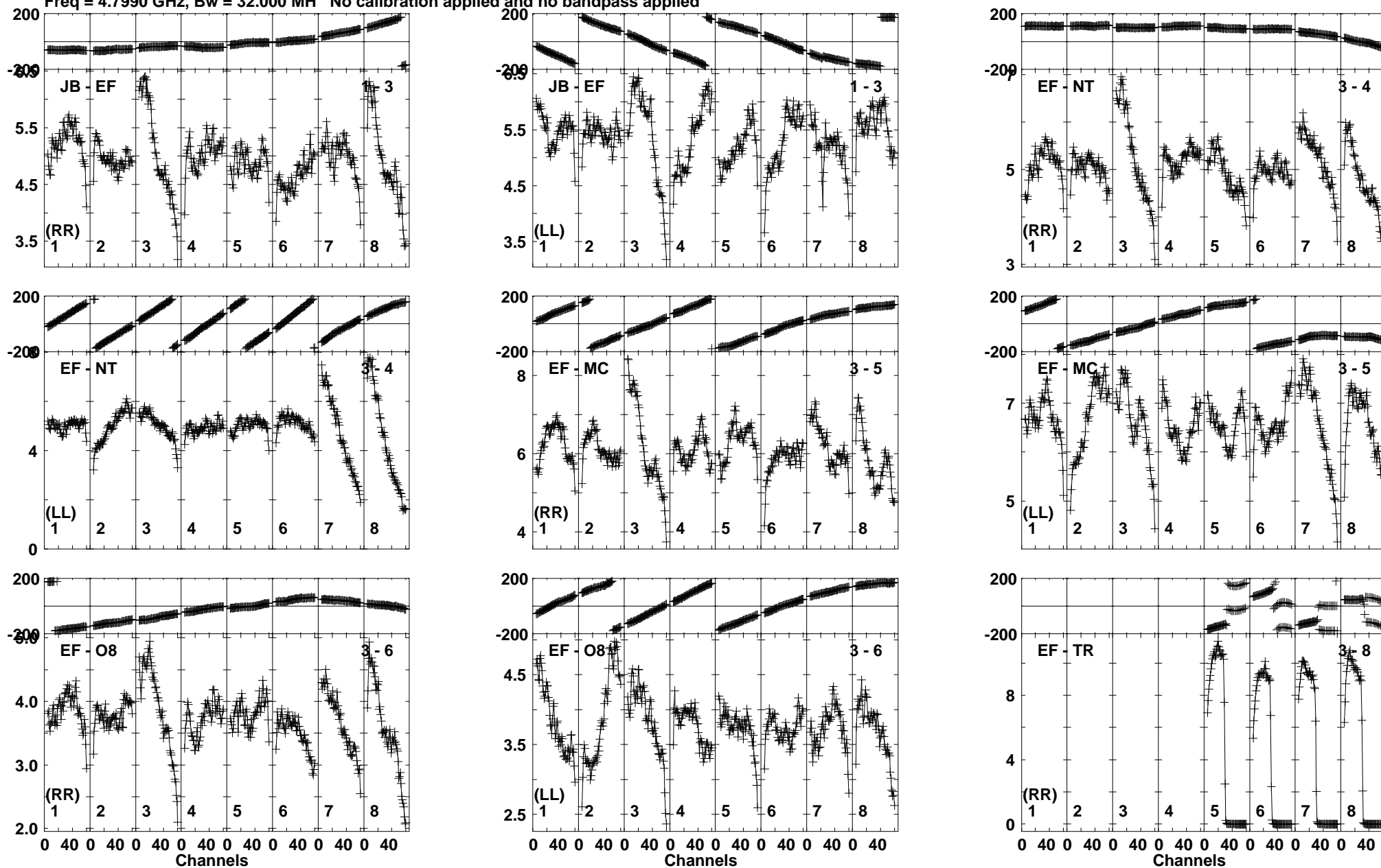
Lower frame: Milli Ampl Jy Top frame: Phas deg Vector averaged cross-power spectrum Baseline: JB (01) - EF (03) Timerange: 00/11:39:54 to 00/11:41:13
