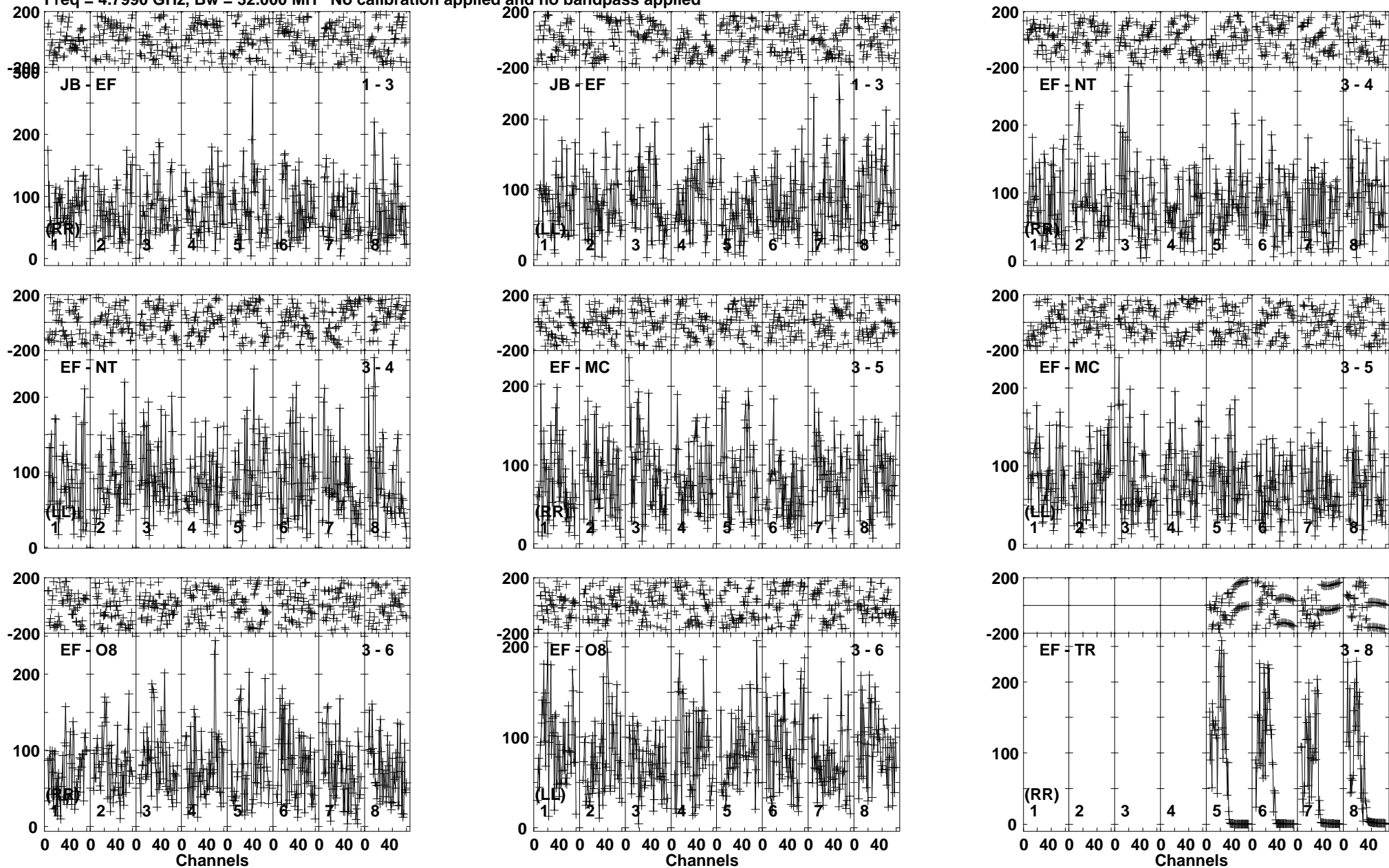
Lower frame: Micro Ampl Jy Top frame: Phas deg Vector averaged cross-power spectrum Baseline: JB (01) - EF (03) Timerange: 00/10:36:59 to 00/10:40:41
