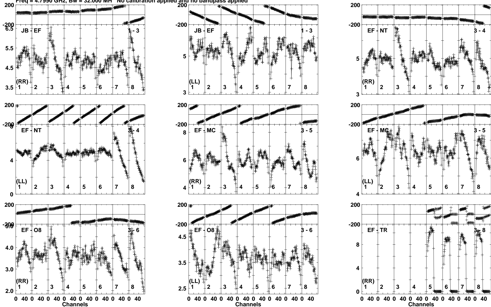
Lower frame: Milli Ampl Jy Top frame: Phas deg Vector averaged cross-power spectrum Baseline: JB (01) - EF (03) Timerange: 00/11:12:19 to 00/11:13:48
