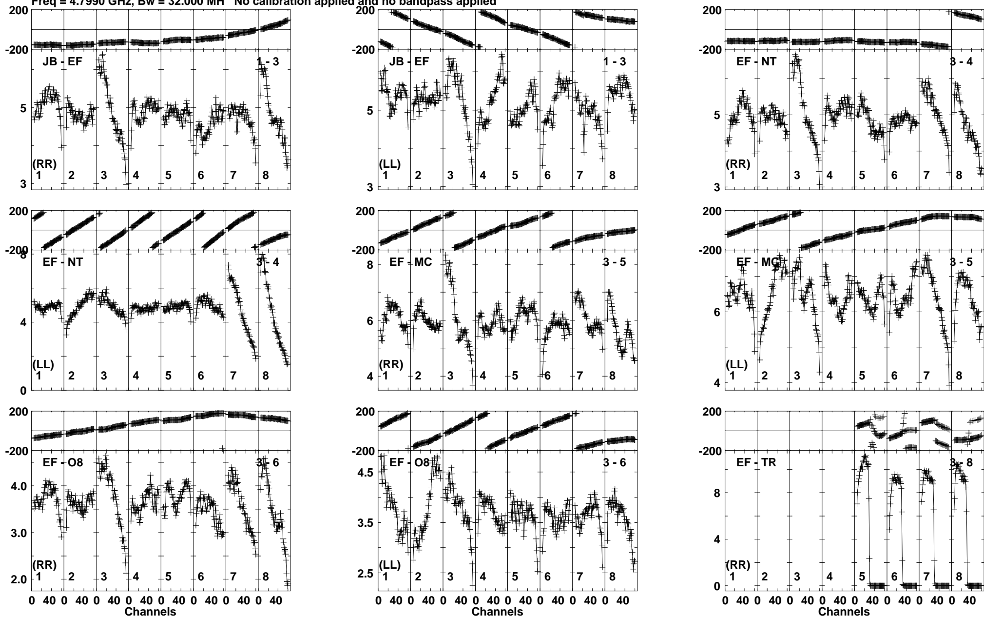
Lower frame: Milli Ampl Jy Top frame: Phas deg Vector averaged cross-power spectrum Baseline: JB (01) - EF (03) Timerange: 00:12:07:10 to 00:12:09:06
