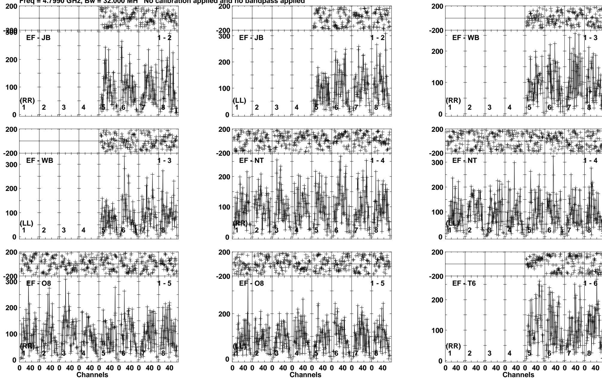
Lower frame: Micro Ampl Jy Top frame: Phas deg Vector averaged cross-power spectrum Baseline: EF (01) - JB (02) Timerange: 00/22:00:37 to 00/22:04:16
