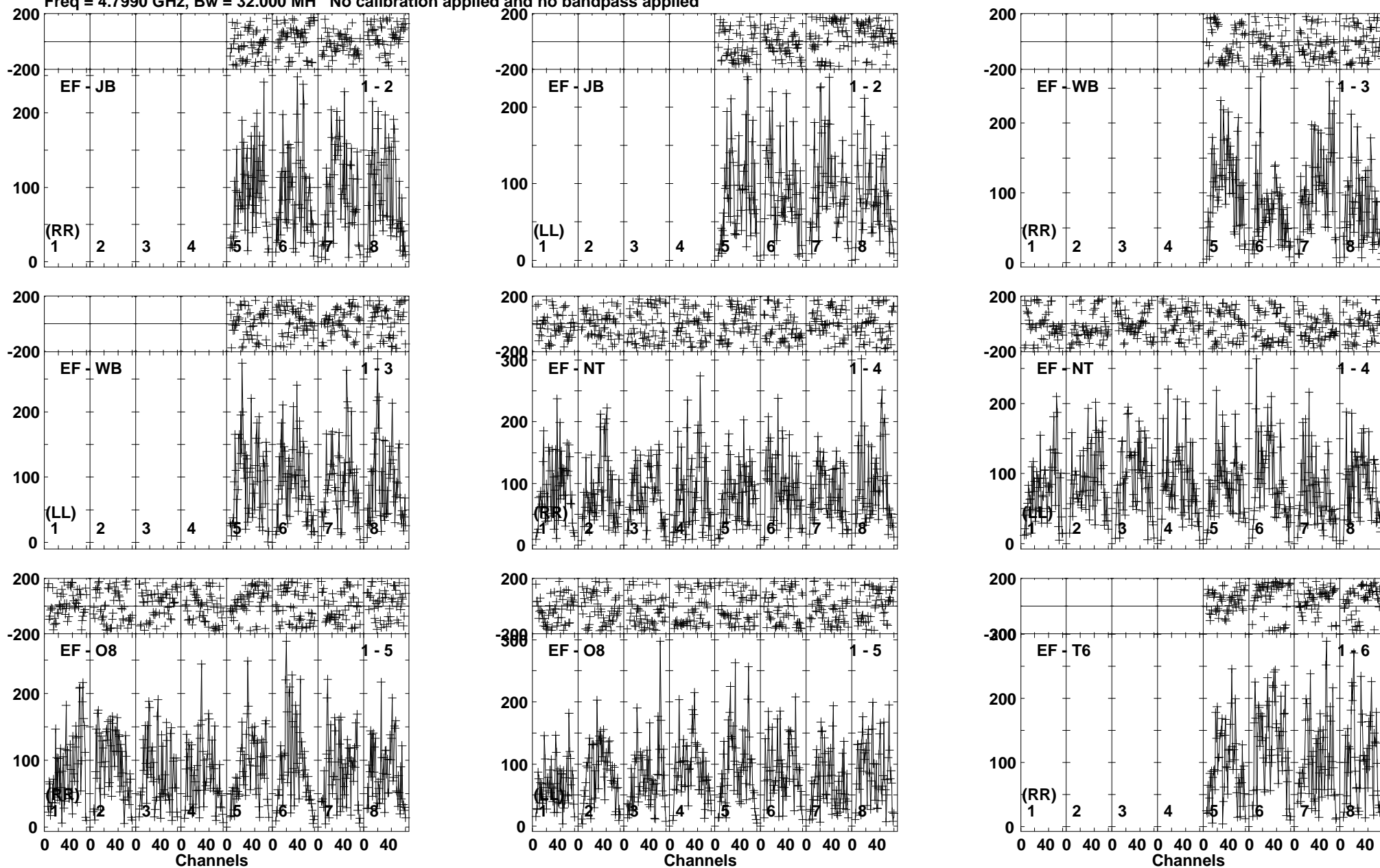
Lower frame: Micro Ampl Jy Top frame: Phas deg Vector averaged cross-power spectrum Baseline: EF (01) - JB (02) Timerange: 00/20:30:15 to 00/20:33:58
