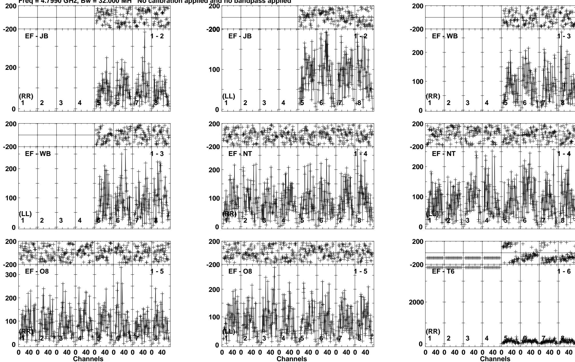
Lower frame: Micro Ampl Jy Top frame: Phas deg Vector averaged cross-power spectrum Baseline: EF (01) - JB (02) Timerange: 00:18:50:28 to 00:18:54:08
