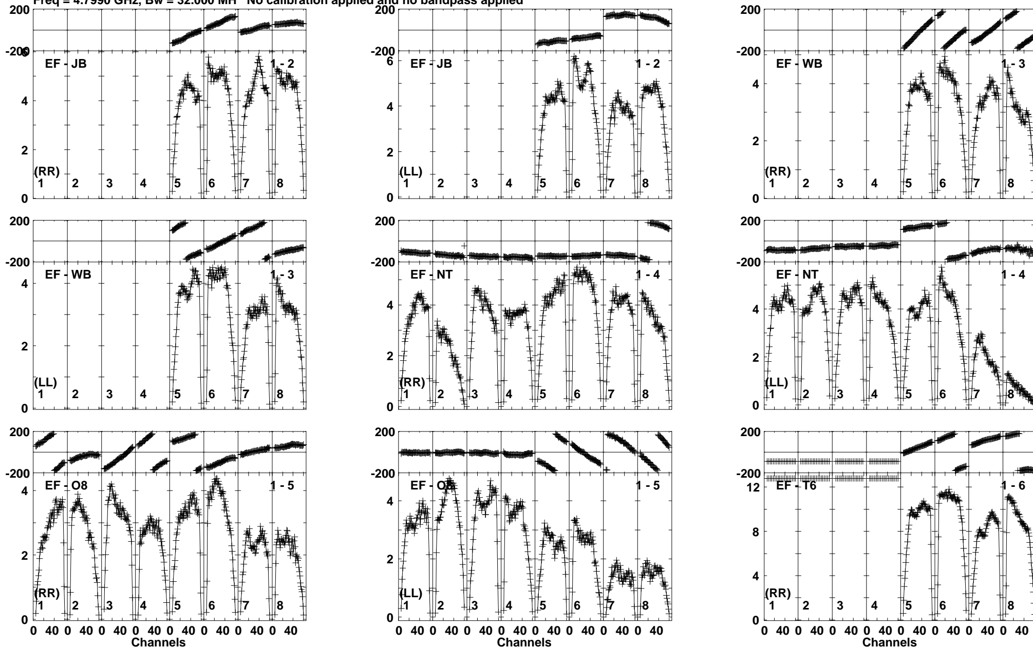
Lower frame: Milli Ampl Jy Top frame: Phas deg Vector averaged cross-power spectrum Baseline: EF (01) - JB (02) Timerange: 00/21:06:14 to 00/21:07:04
