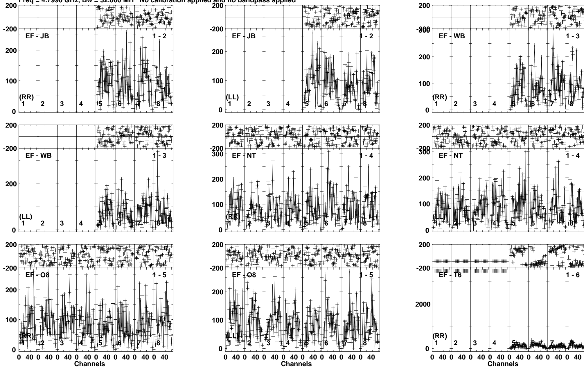
Lower frame: Micro Ampl Jy Top frame: Phas deg Vector averaged cross-power spectrum Baseline: EF (01) - JB (02) Timerange: 00/19:06:07 to 00/19:09:49
