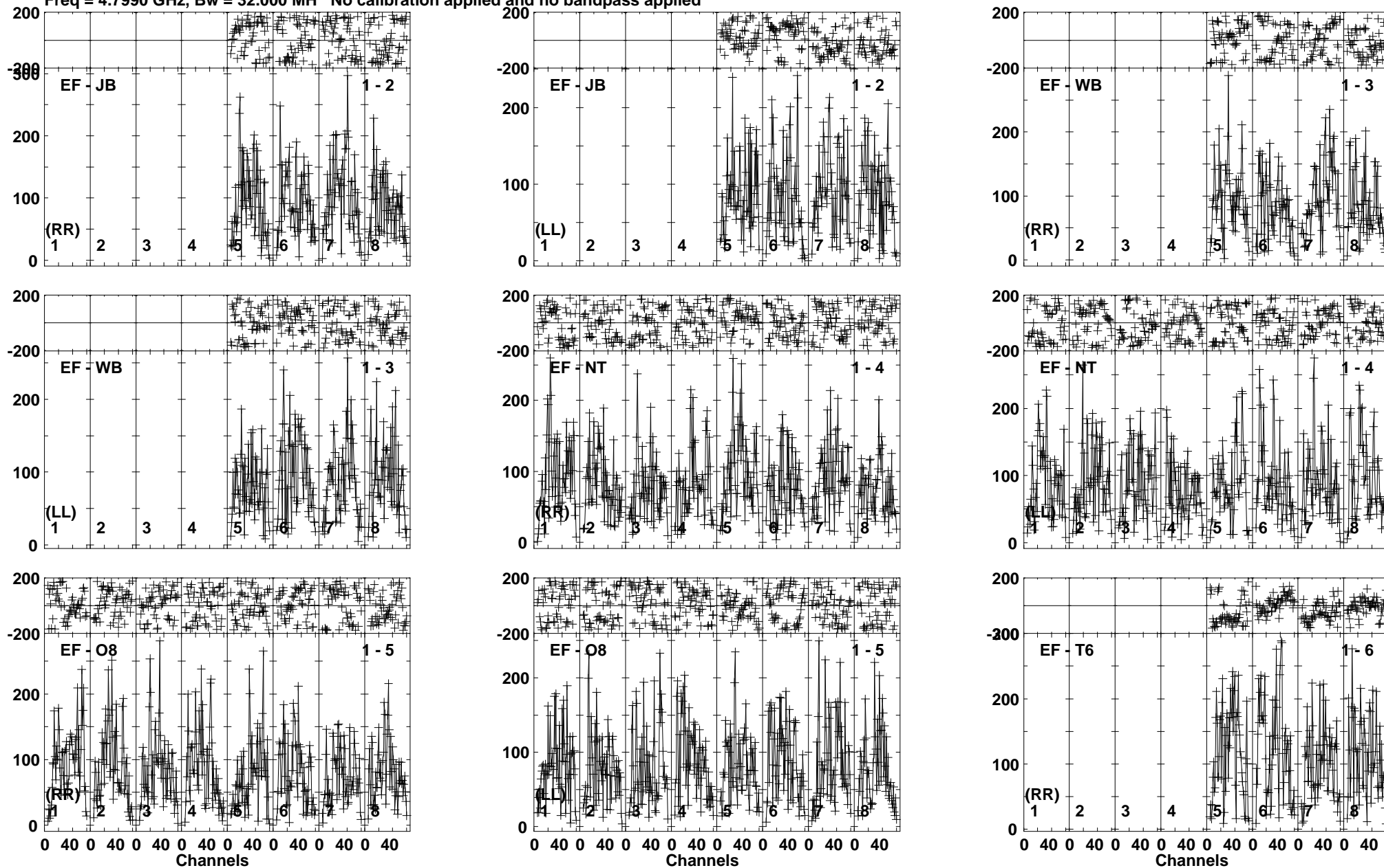
Lower frame: Micro Ampl Jy Top frame: Phas deg Vector averaged cross-power spectrum Baseline: EF (01) - JB (02) Timerange: 00/20:09:13 to 00/20:12:55
