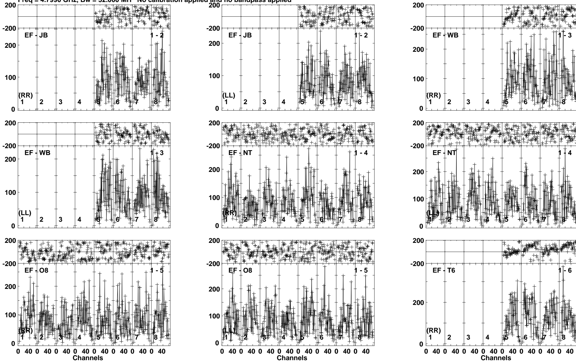
Lower frame: Micro Ampl Jy Top frame: Phas deg Vector averaged cross-power spectrum Baseline: EF (01) - JB (02) Timerange: 00/19:16:40 to 00/19:20:24
