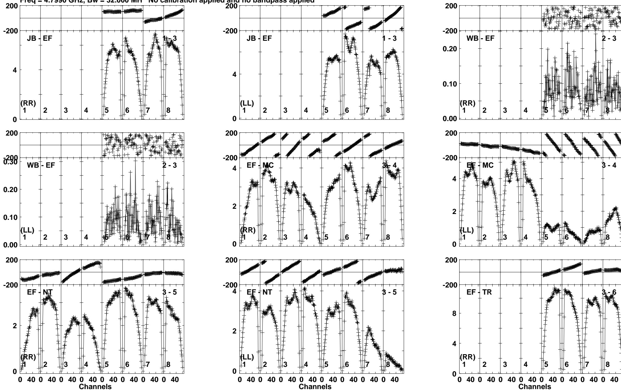
Lower frame: Milli Ampl Jy Top frame: Phas deg Vector averaged cross-power spectrum Baseline: JB (01) - EF (03) Timerange: 00/16:12:01 to 00/16:14:59
