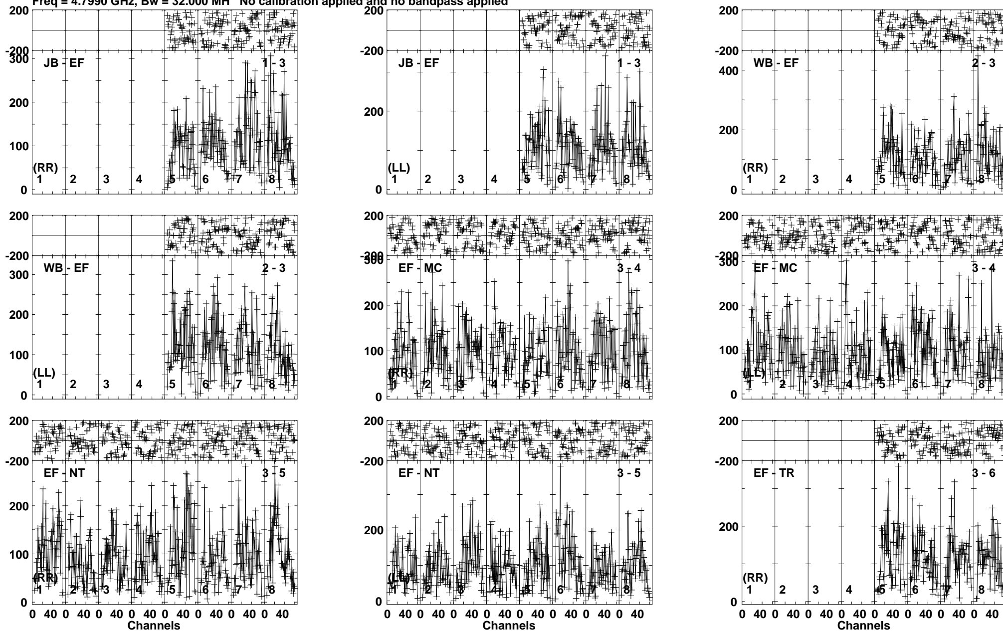
Lower frame: Micro Ampl Jy Top frame: Phas deg Vector averaged cross-power spectrum Baseline: JB (01) - EF (03) Timerange: 00/15:42:31 to 00/15:44:59
