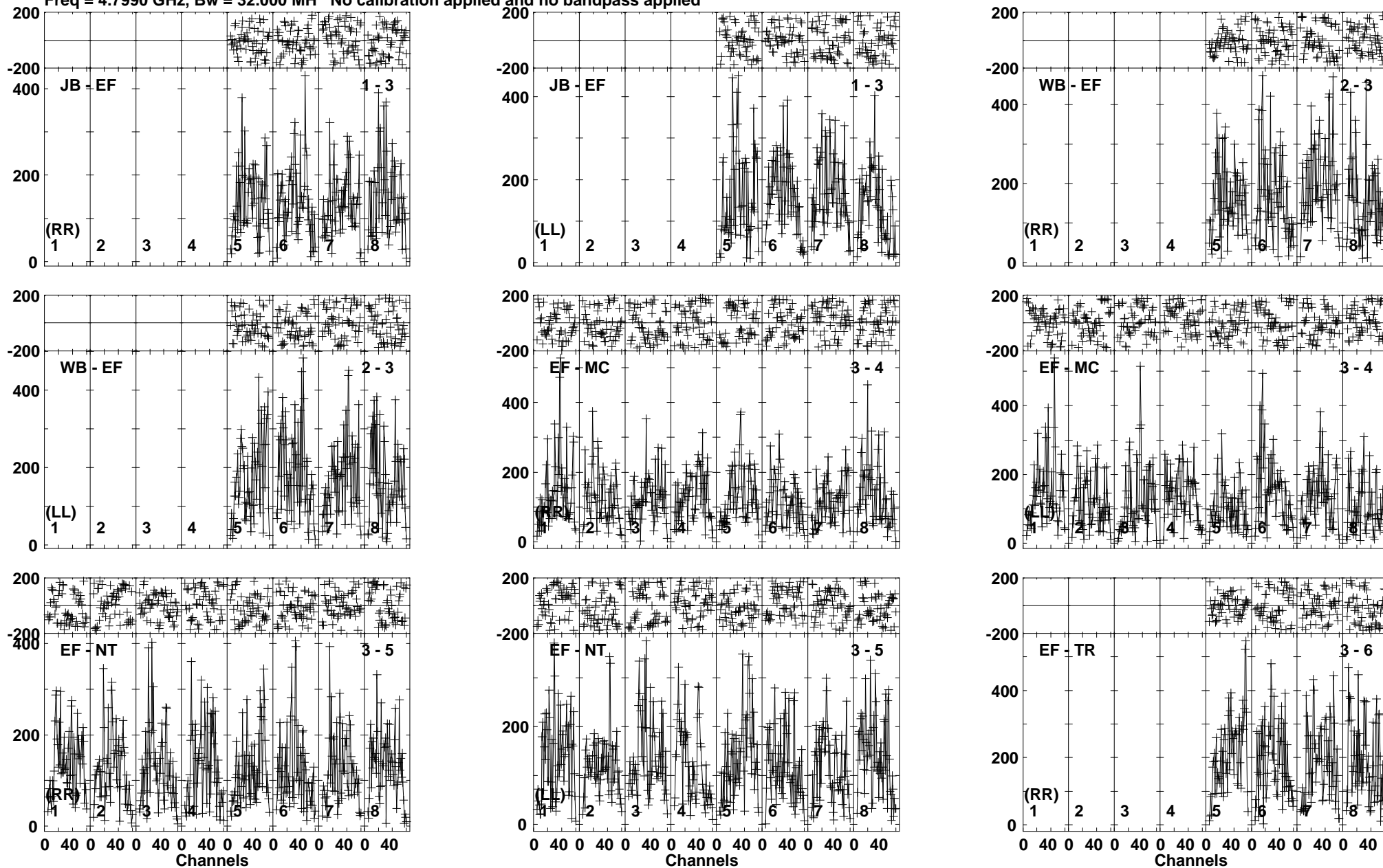
Lower frame: Micro Ampl Jy Top frame: Phas deg Vector averaged cross-power spectrum Baseline: JB (01) - EF (03) Timerange: 00/12:27:01 to 00/12:28:29
