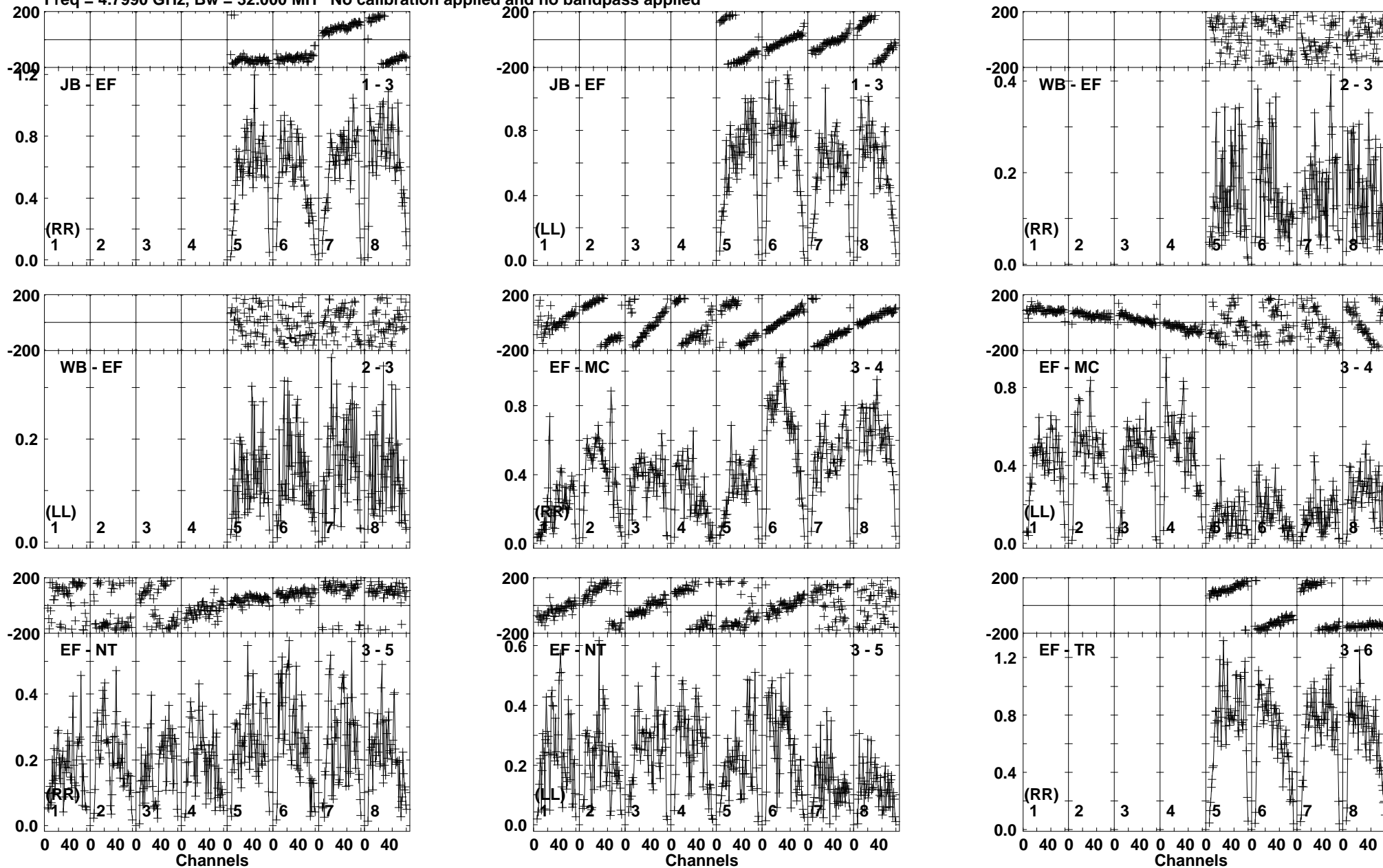
Lower frame: Milli Ampl Jy Top frame: Phas deg Vector averaged cross-power spectrum Baseline: JB (01) - EF (03) Timerange: 00/16:05:01 to 00/16:06:29
