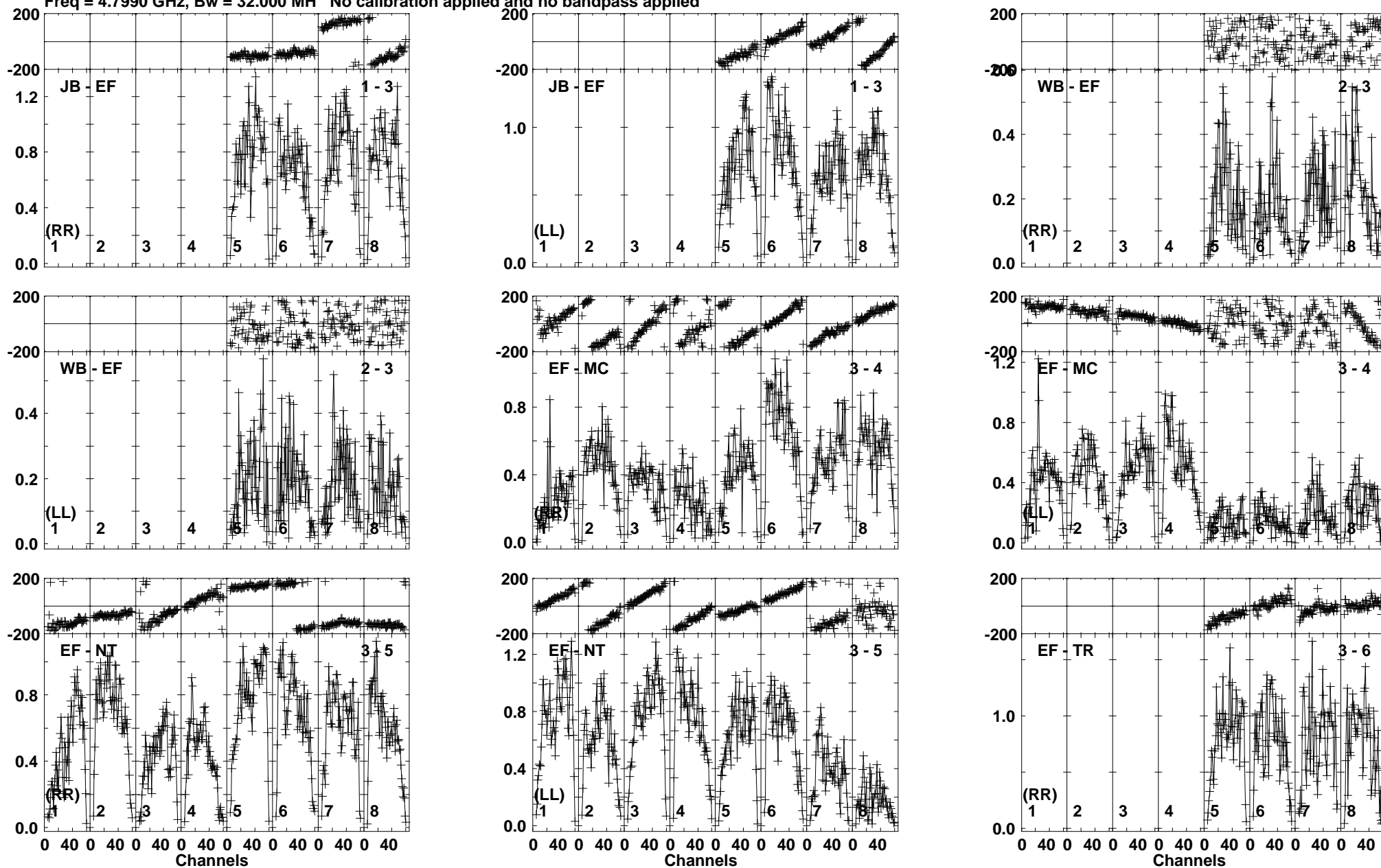
Lower frame: Milli Ampl Jy Top frame: Phas deg Vector averaged cross-power spectrum Baseline: JB (01) - EF (03) Timerange: 00/16:01:01 to 00/16:02:29
