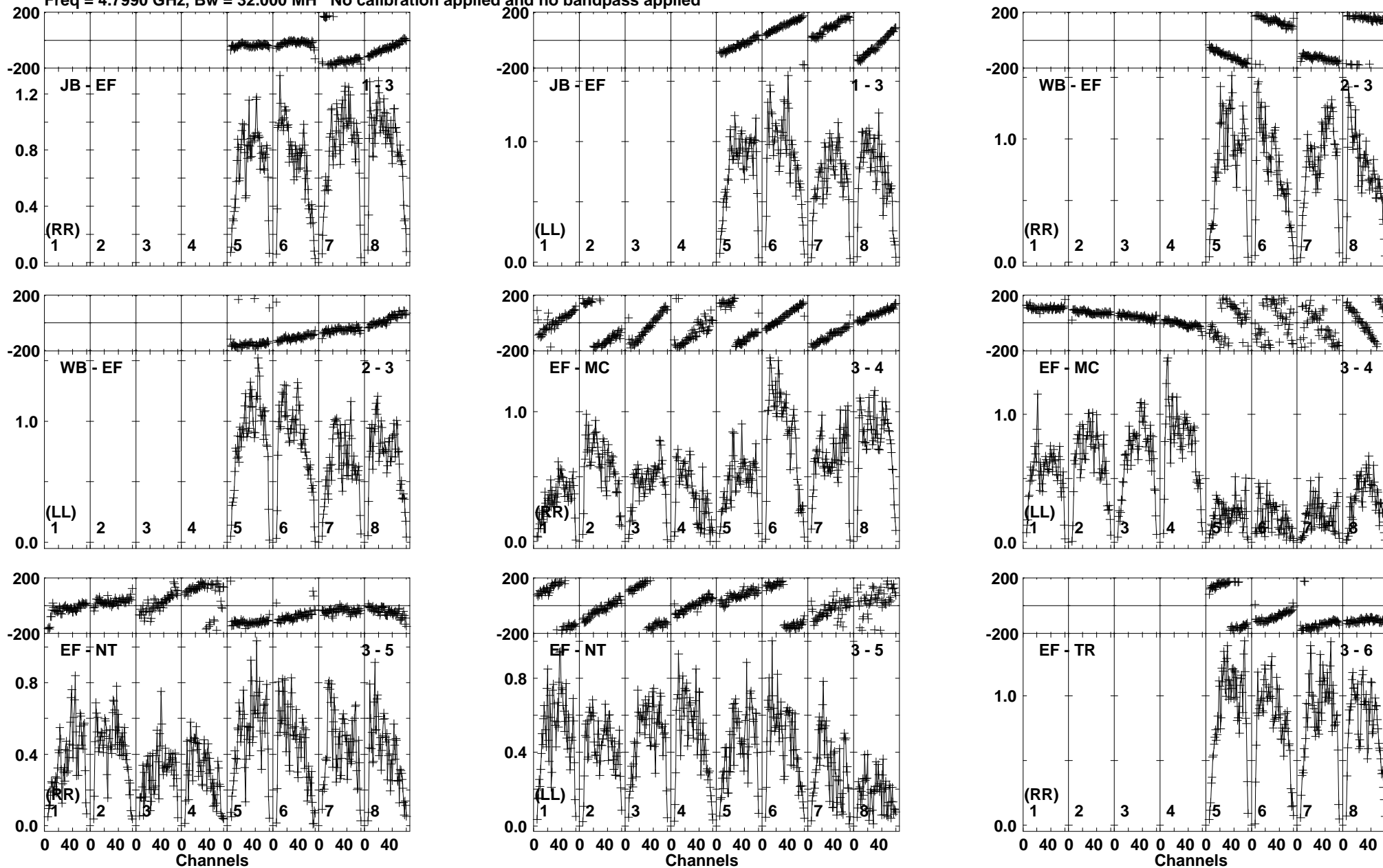
Lower frame: Milli Ampl Jy Top frame: Phas deg Vector averaged cross-power spectrum Baseline: JB (01) - EF (03) Timerange: 00/15:57:31 to 00/15:58:29
