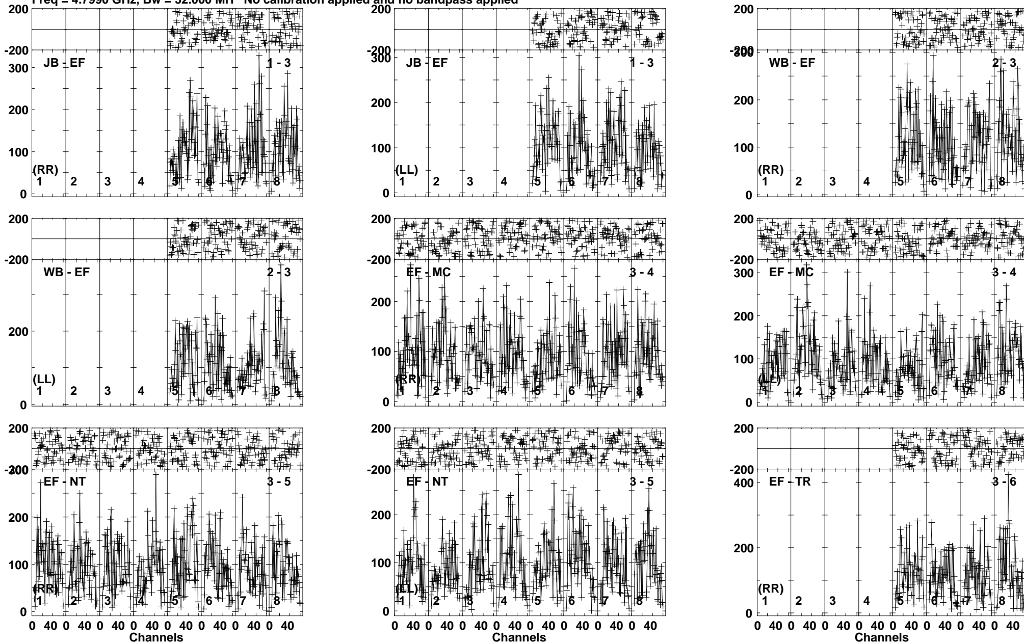
Lower frame: Micro Ampl Jy Top frame: Phas deg Vector averaged cross-power spectrum Baseline: JB (01) - EF (03) Timerange: 00/12:48:41 to 00/12:51:09
