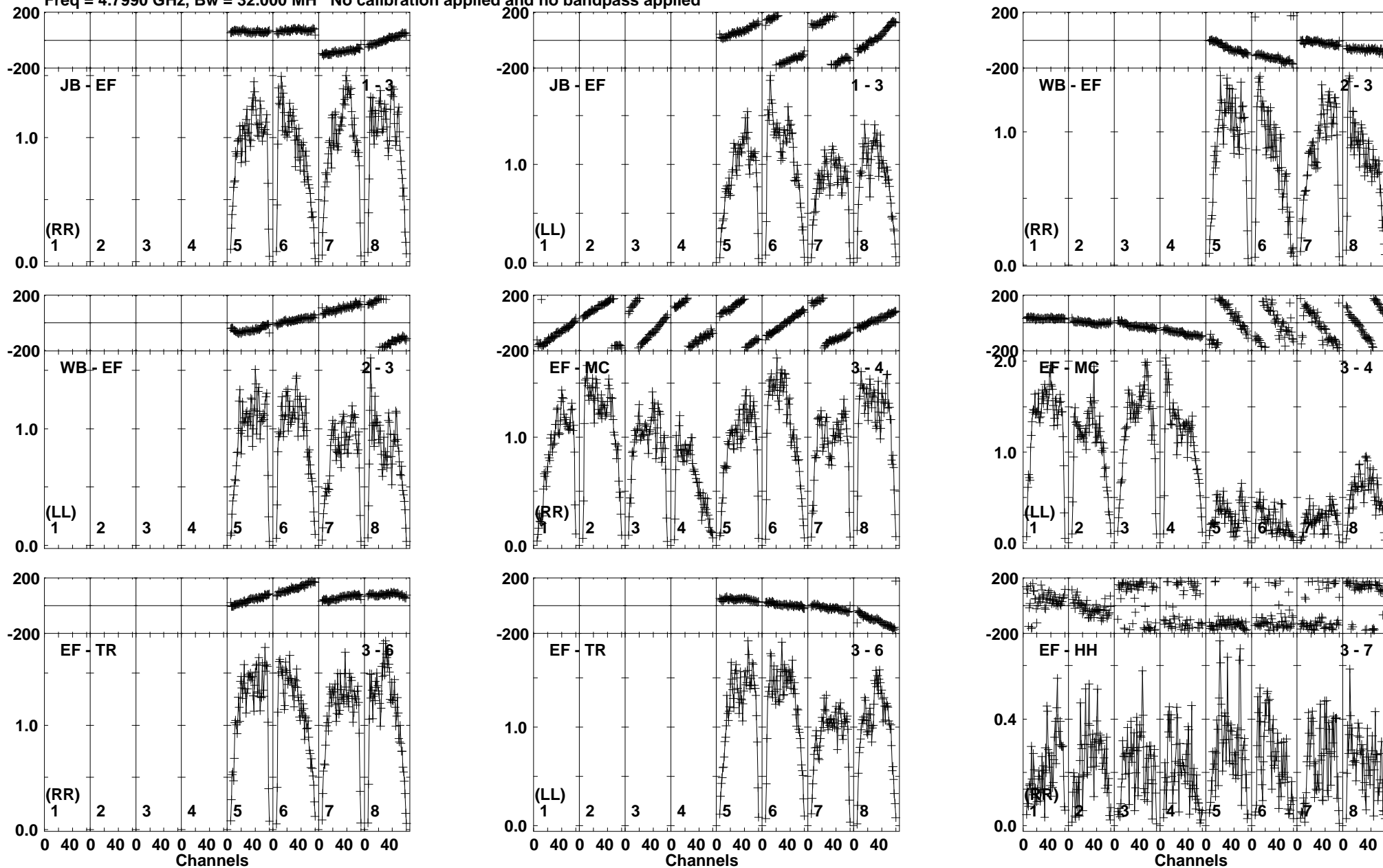
Lower frame: Milli Ampl Jy Top frame: Phas deg Vector averaged cross-power spectrum Baseline: JB (01) - EF (03) Timerange: 00/13:48:21 to 00/13:49:19
