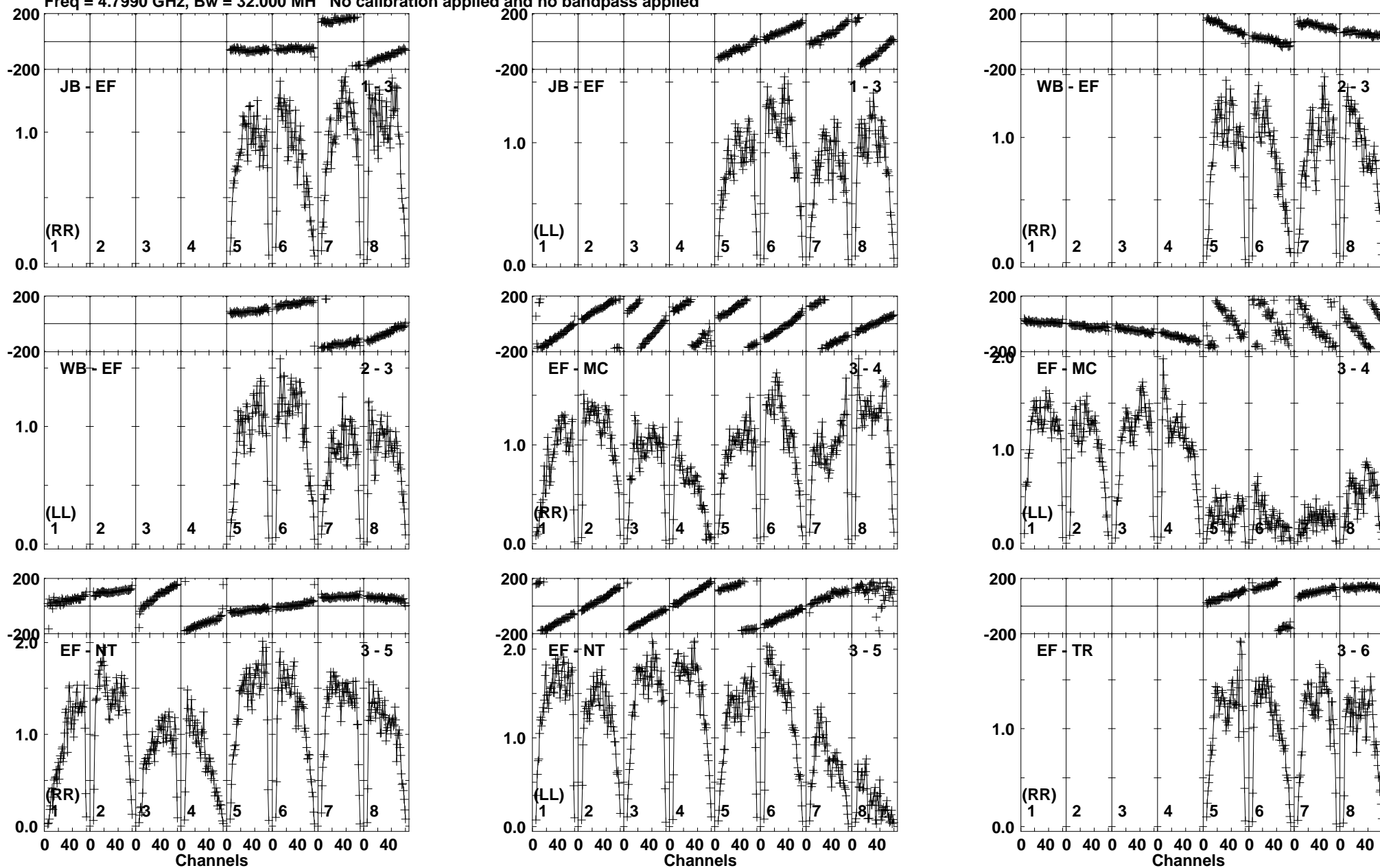
Lower frame: Milli Ampl Jy Top frame: Phas deg Vector averaged cross-power spectrum Baseline: JB (01) - EF (03) Timerange: 00/14:53:01 to 00/14:53:59
