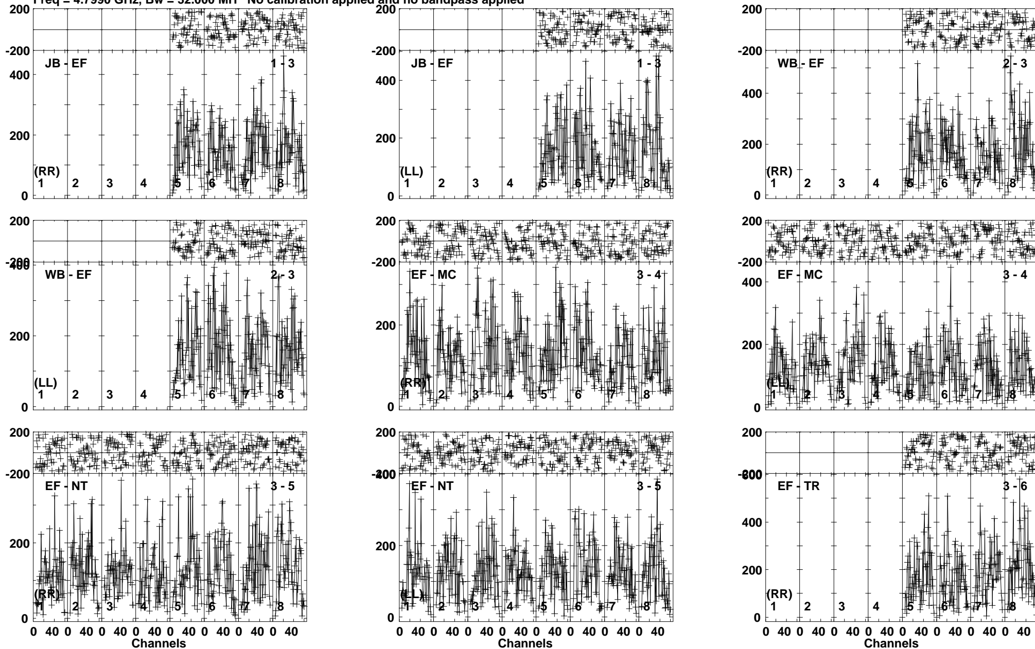
Lower frame: Micro Ampl Jy Top frame: Phas deg Vector averaged cross-power spectrum Baseline: JB (01) - EF (03) Timerange: 00:12:39:01 to 00:12:40:29
