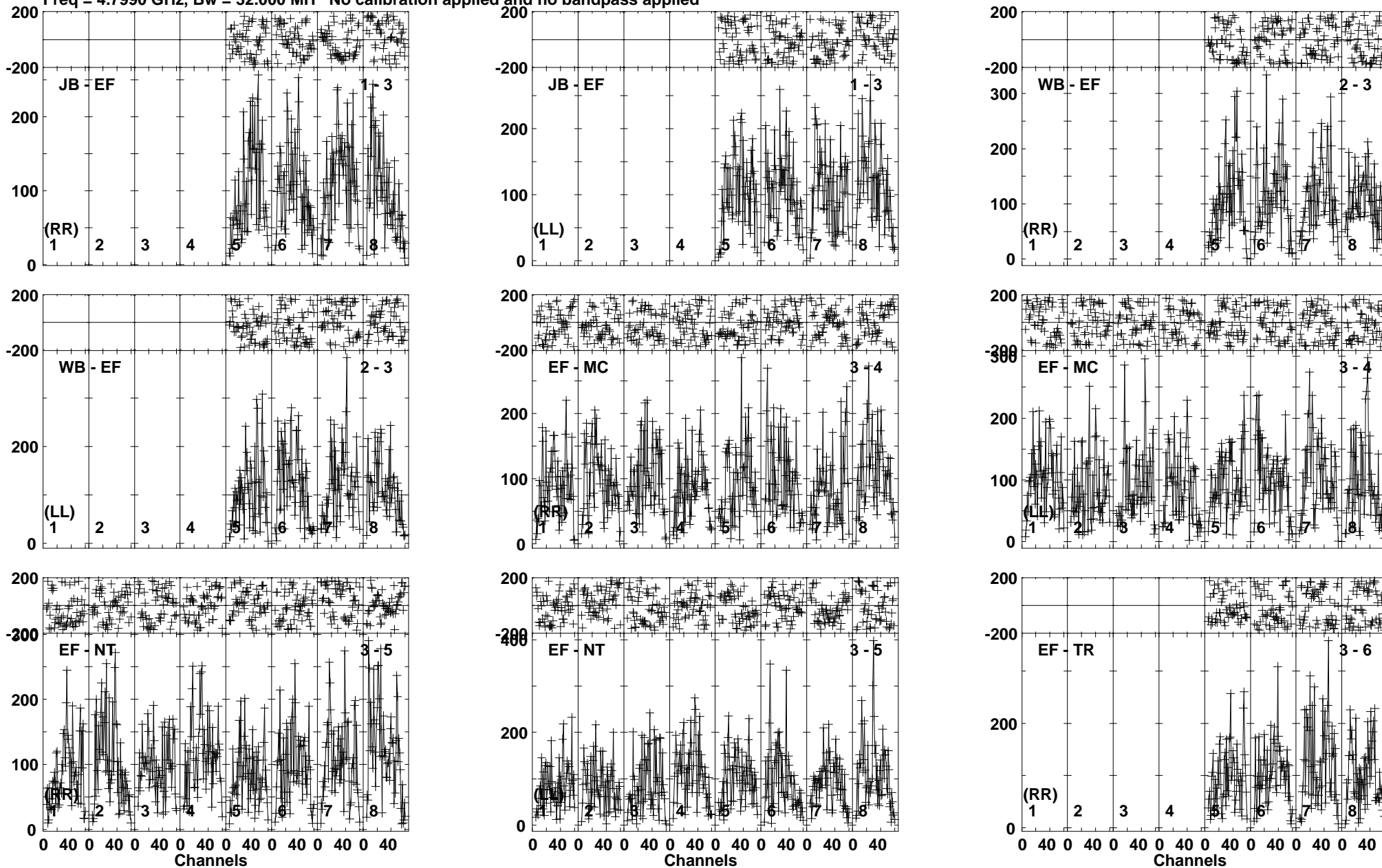
Lower frame: Micro Ampl Jy Top frame: Phas deg Vector averaged cross-power spectrum Baseline: JB (01) - EF (03) Timerange: 00/13:57:21 to 00/13:59:49
