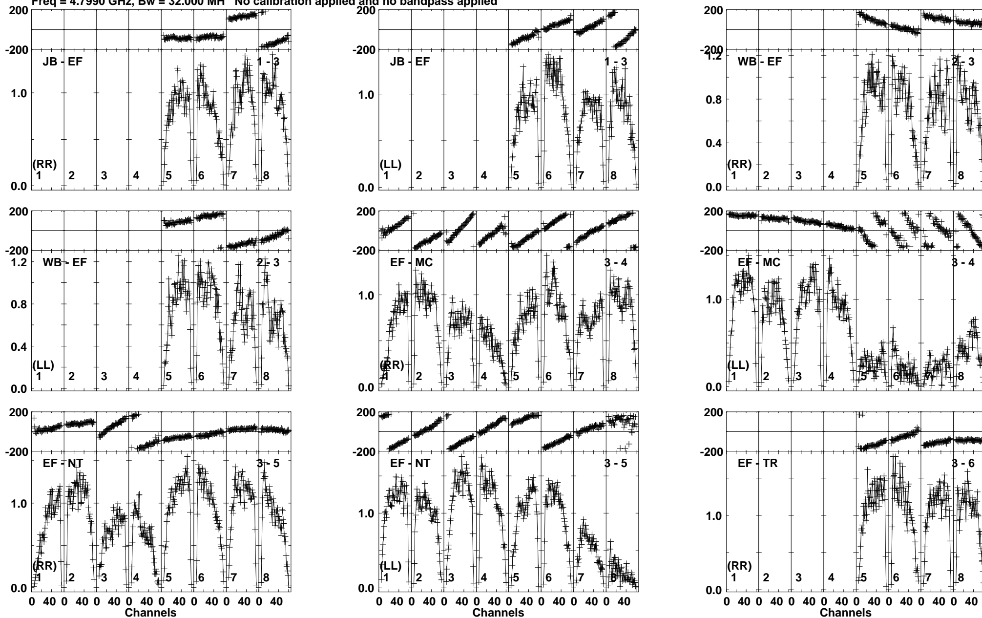
Lower frame: Milli Ampl Jy Top frame: Phas deg Vector averaged cross-power spectrum Baseline: JB (01) - EF (03) Timerange: 00/14:32:11 to 00/14:33:39
