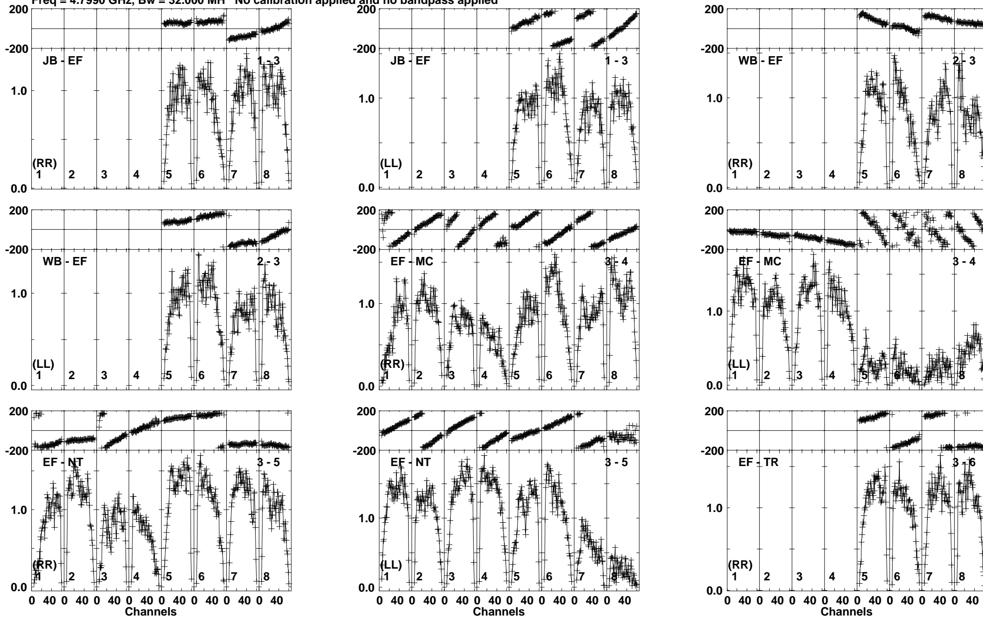
Lower frame: Milli Ampl Jy Top frame: Phas deg Vector averaged cross-power spectrum Baseline: JB (01) - EF (03) Timerange: 00:14:36:51 to 00:14:37:49
