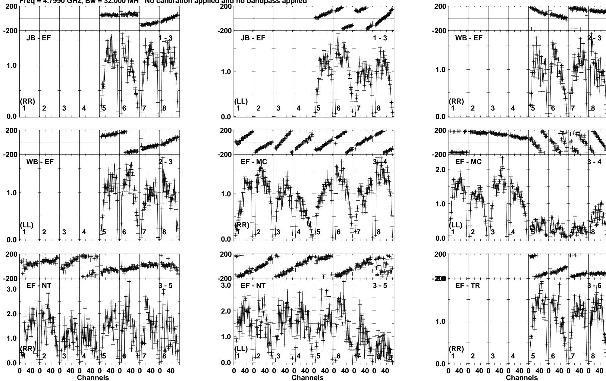
Lower frame: Milli Ampl Jy Top frame: Phas deg Vector averaged cross-power spectrum Baseline: JB (01) - EF (03) Timerange: 00/13:40:11 to 00/13:41:09
