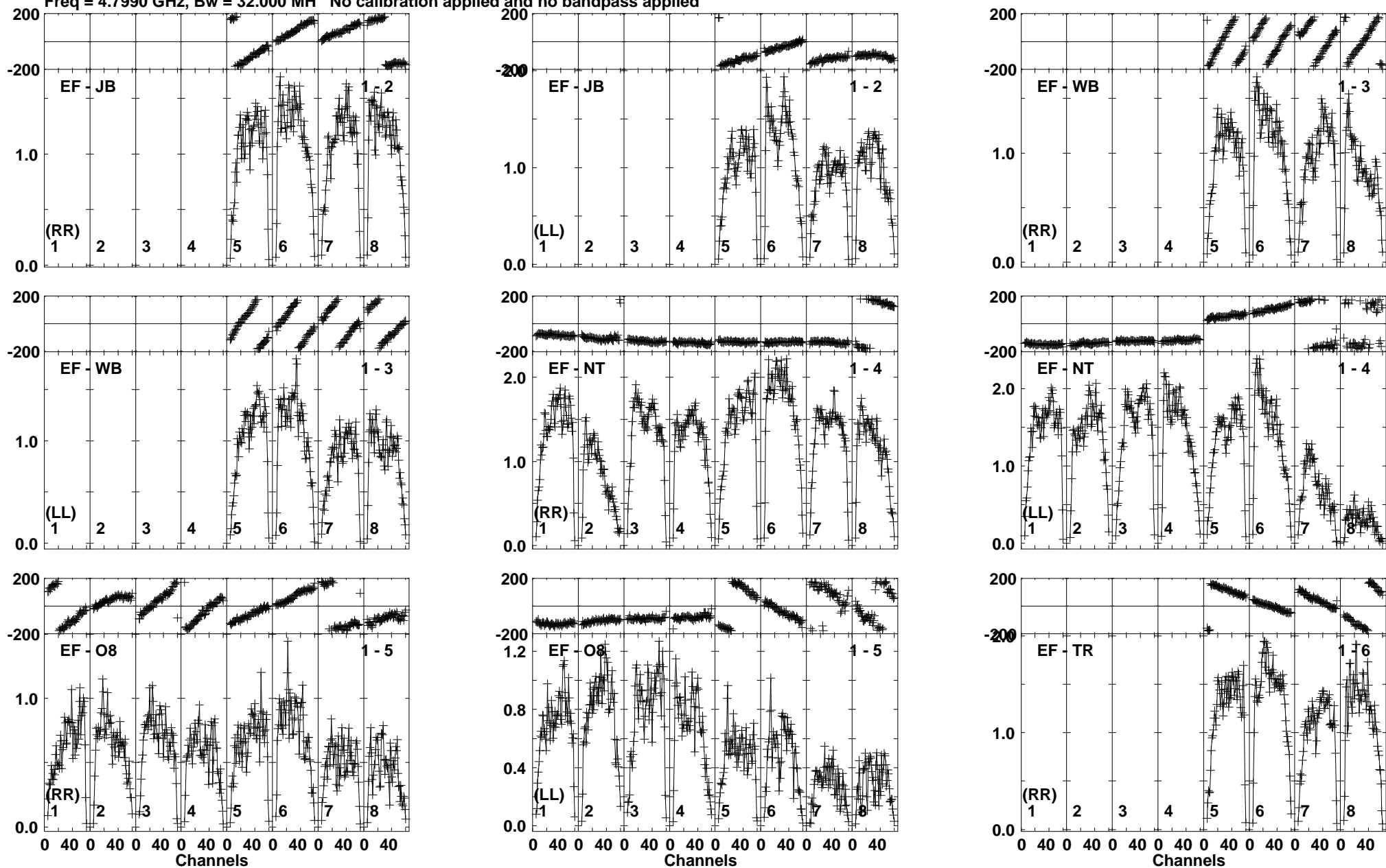
Lower frame: Milli Ampl Jy Top frame: Phas deg Vector averaged cross-power spectrum Baseline: EF (01) - JB (02) Timerange: 00:12:41:10 to 00:12:42:08
