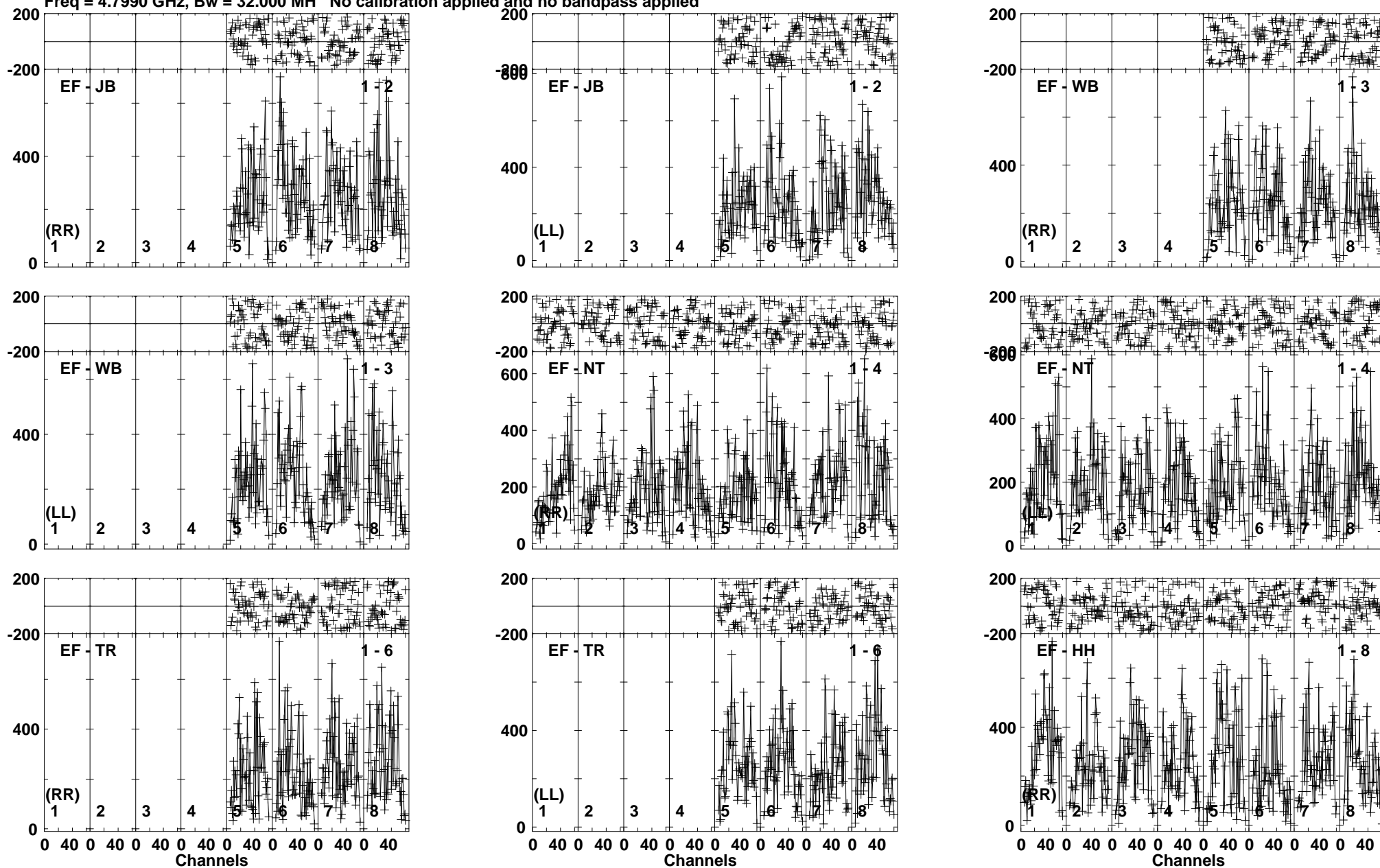
Lower frame: Micro Ampl Jy Top frame: Phas deg Vector averaged cross-power spectrum Baseline: EF (01) - JB (02) Timerange: 00/10:25:40 to 00/10:28:09
