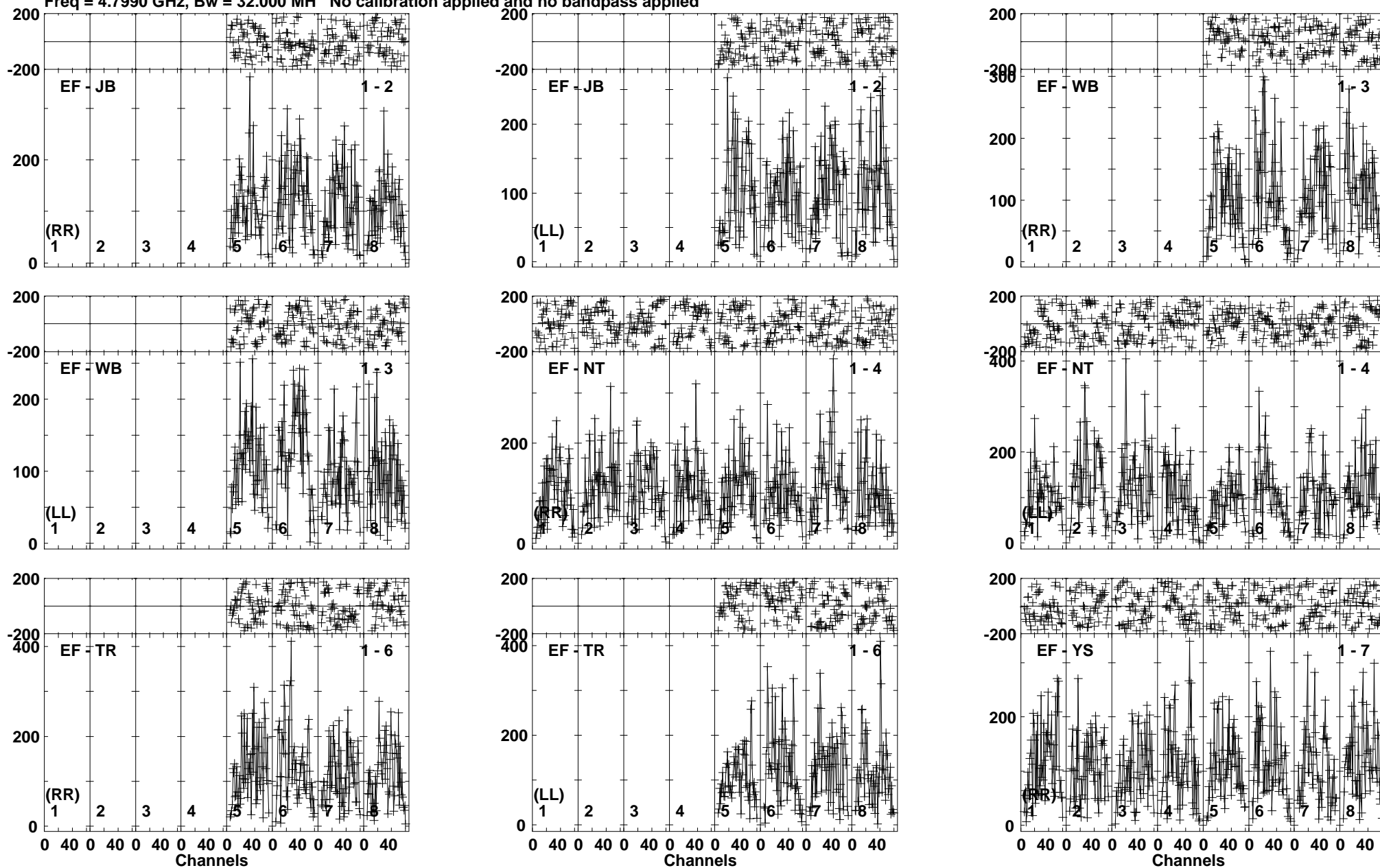
Lower frame: Micro Ampl Jy Top frame: Phas deg Vector averaged cross-power spectrum Baseline: EF (01) - JB (02) Timerange: 00/13:54:49 to 00/13:57:18
