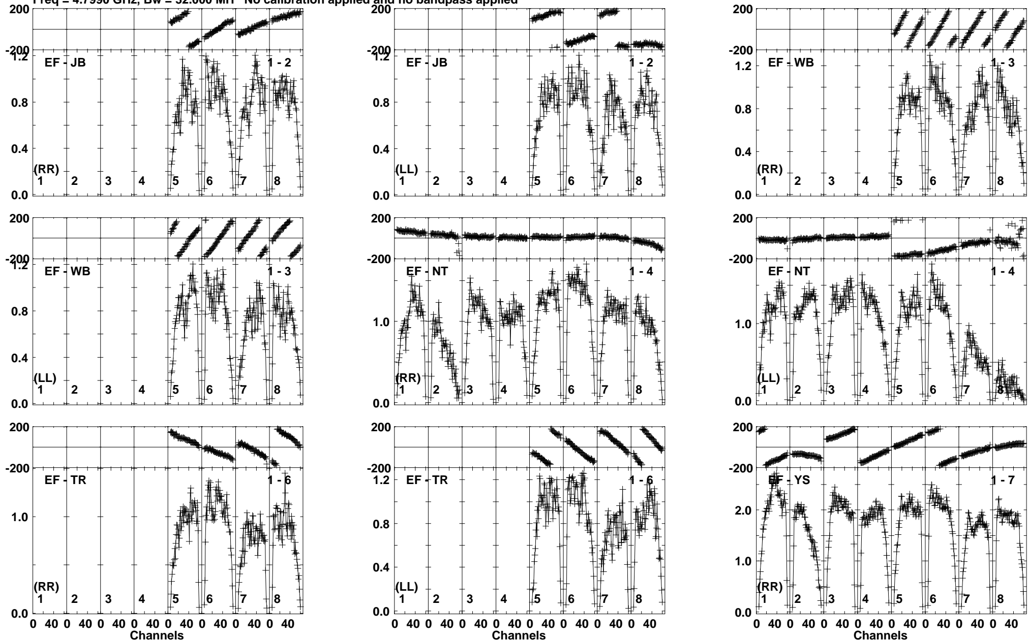
Lower frame: Milli Ampl Jy Top frame: Phas deg Vector averaged cross-power spectrum Baseline: EF (01) - JB (02) Timerange: 00/14:21:39 to 00/14:23:38
