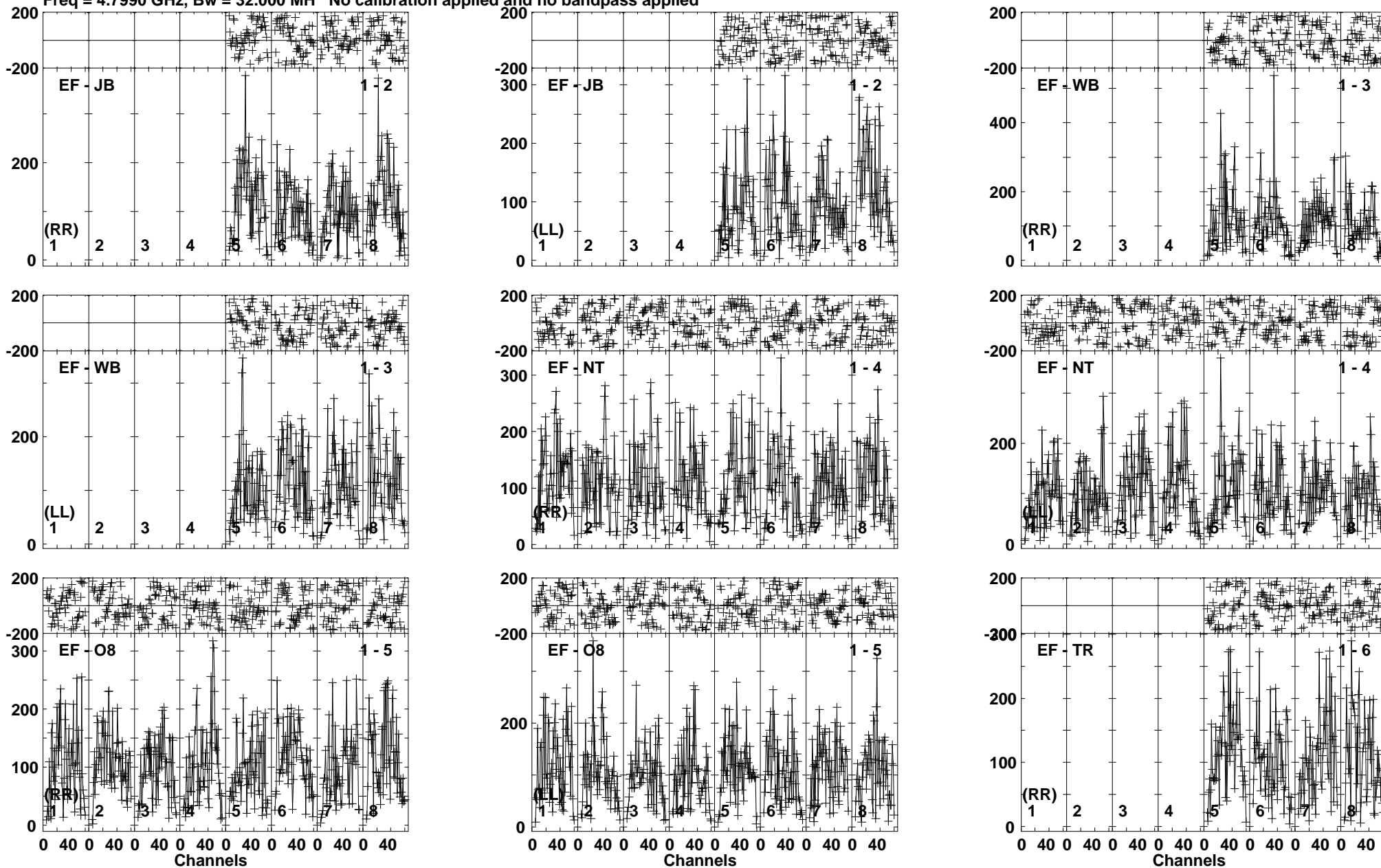
Lower frame: Micro Ampl Jy Top frame: Phas deg Vector averaged cross-power spectrum Baseline: EF (01) - JB (02) Timerange: 00/10:58:00 to 00/11:00:28
