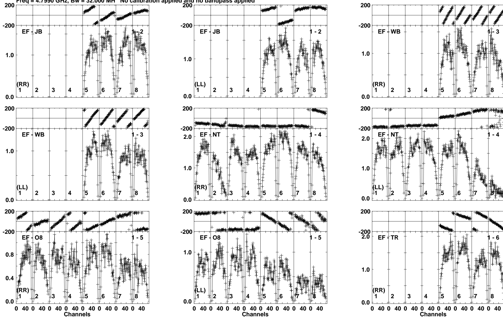
Lower frame: Milli Ampl Jy Top frame: Phas deg Vector averaged cross-power spectrum Baseline: EF (01) - JB (02) Timerange: 00/12:28:30 to 00/12:29:58
