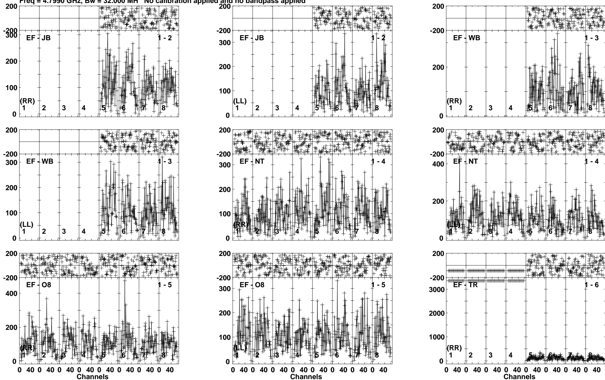
Lower frame: Micro Ampl Jy Top frame: Phas deg Vector averaged cross-power spectrum Baseline: EF (01) - JB (02) Timerange: 00:12:46:10 to 00:12:48:38
