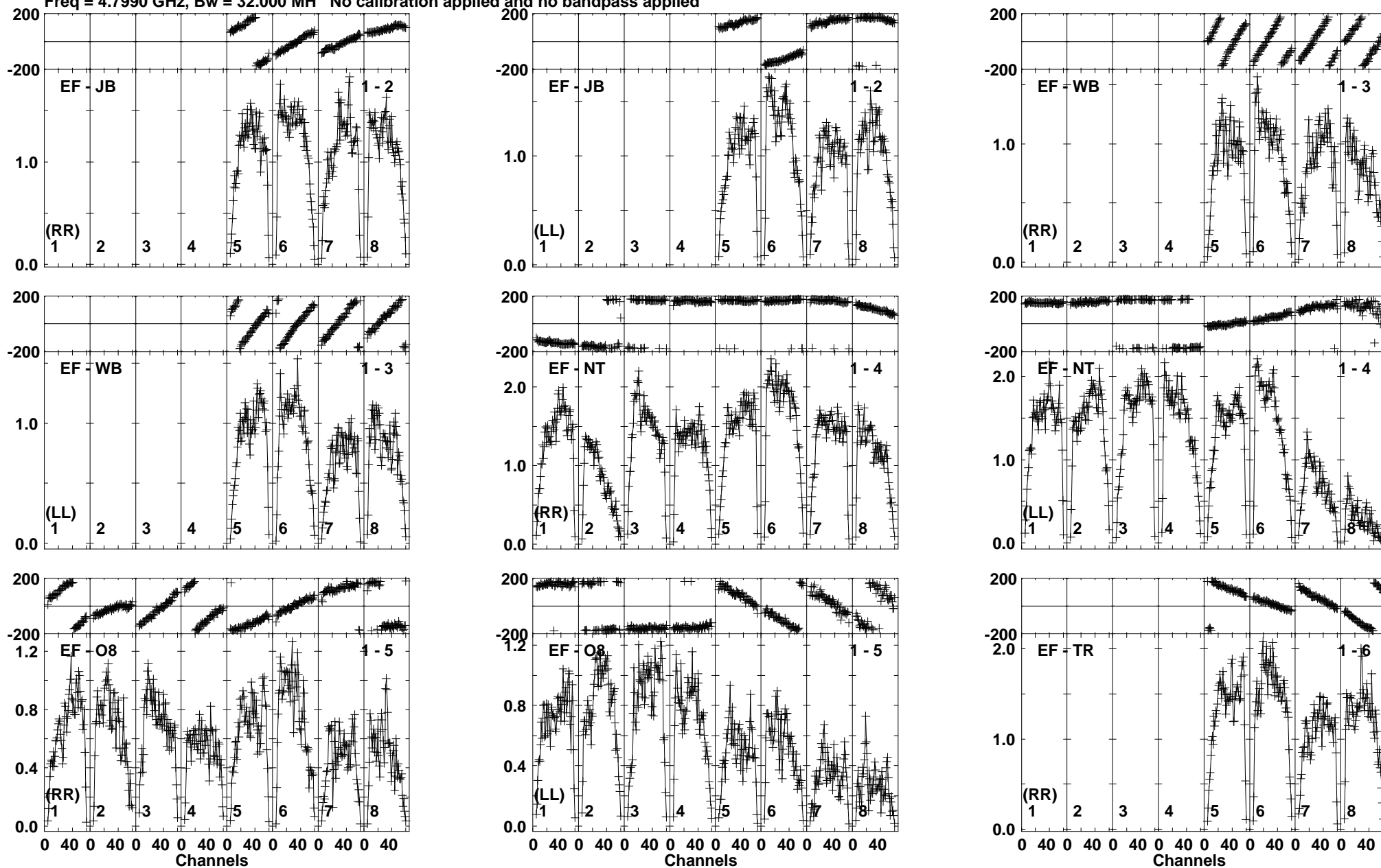
Lower frame: Milli Ampl Jy Top frame: Phas deg Vector averaged cross-power spectrum Baseline: EF (01) - JB (02) Timerange: 00/12:36:29 to 00/12:37:59
