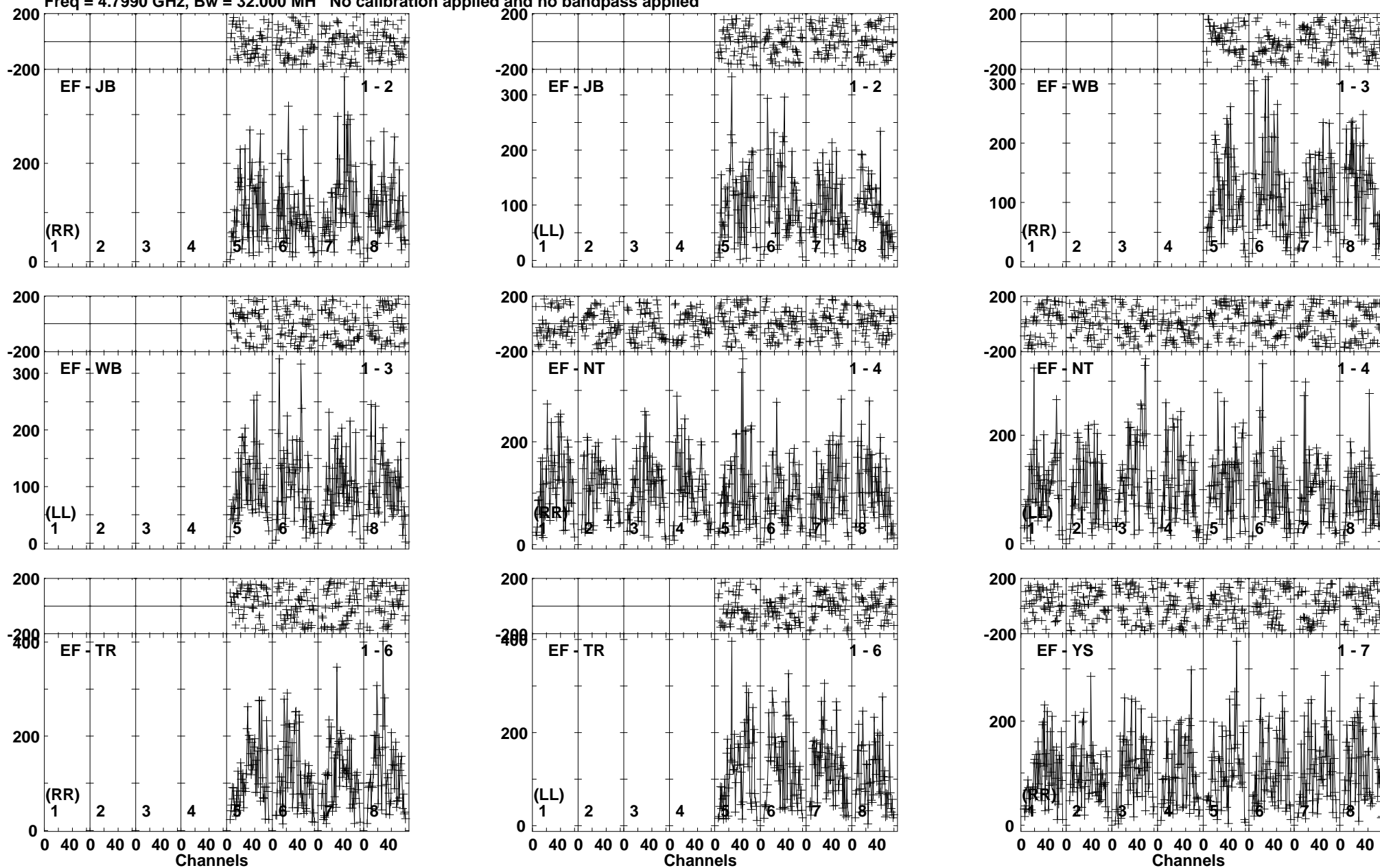
Lower frame: Micro Ampl Jy Top frame: Phas deg Vector averaged cross-power spectrum Baseline: EF (01) - JB (02) Timerange: 00/14:19:09 to 00/14:21:38
