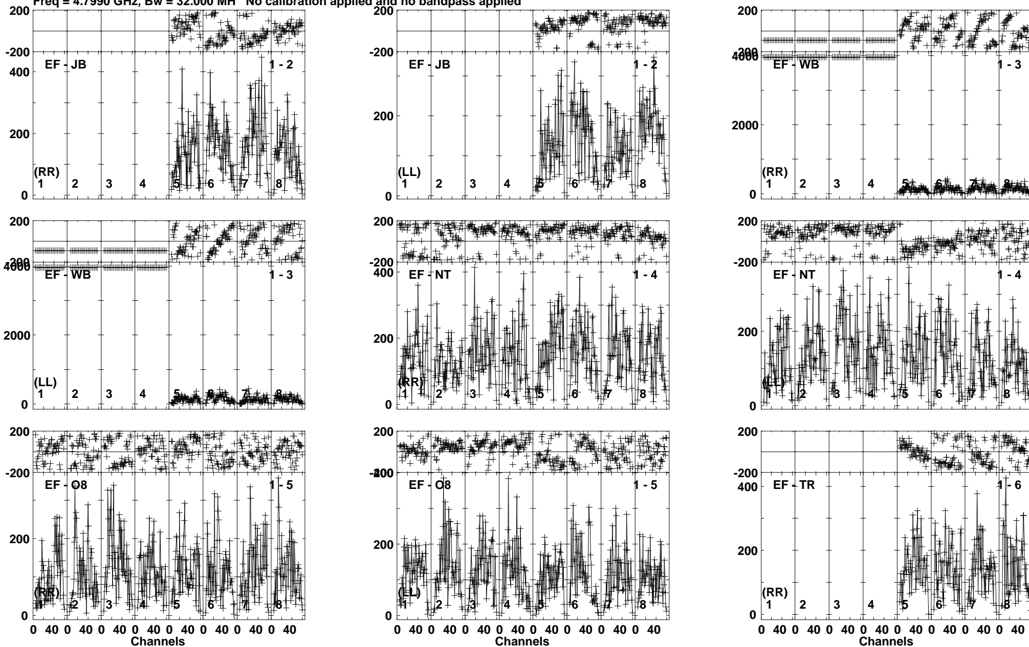
Lower frame: Micro Ampl Jy Top frame: Phas deg Vector averaged cross-power spectrum Baseline: EF (01) - JB (02) Timerange: 00/13:42:39 to 00/13:45:08
