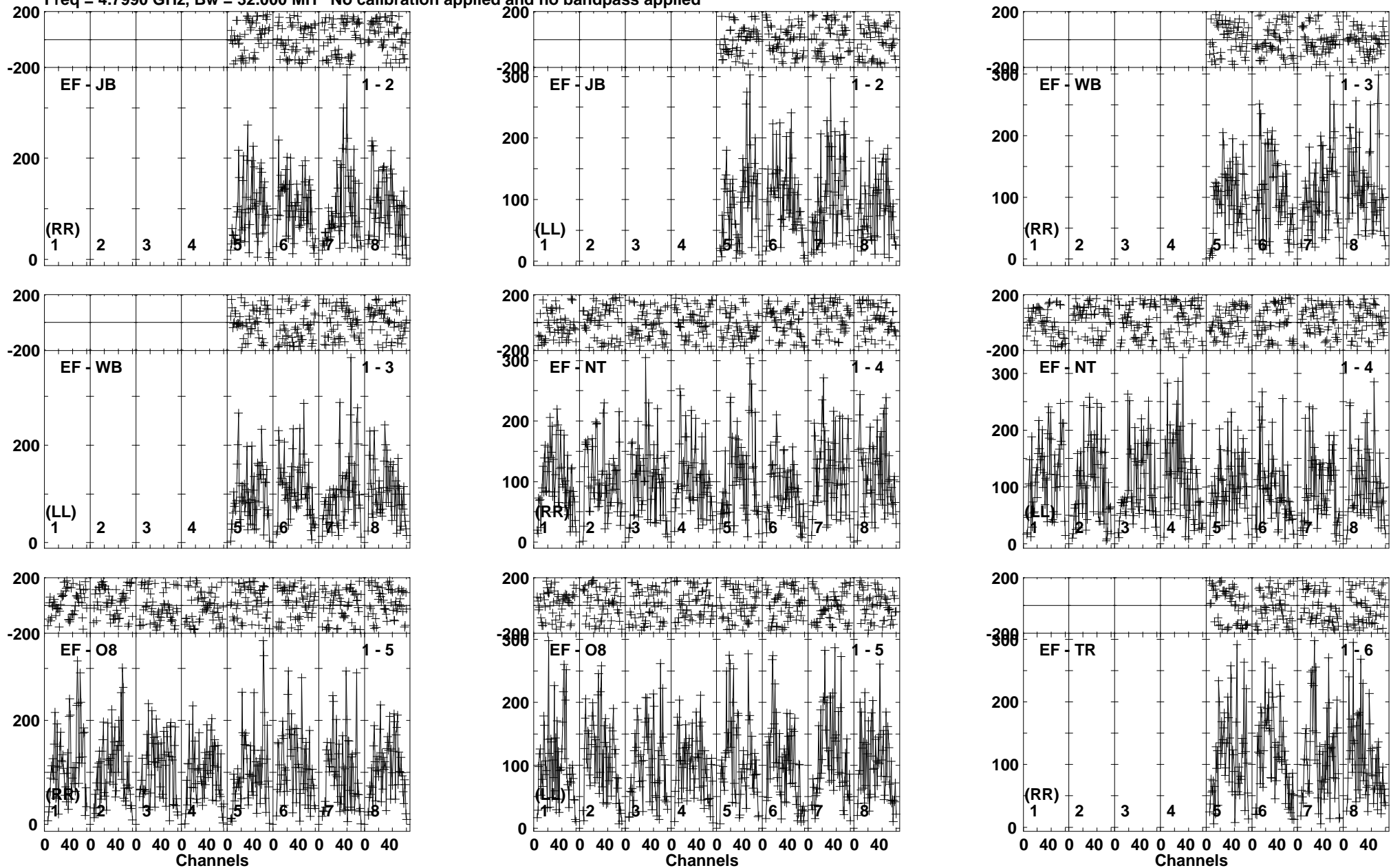
Lower frame: Micro Ampl Jy Top frame: Phas deg Vector averaged cross-power spectrum Baseline: EF (01) - JB (02) Timerange: 00/13:34:40 to 00/13:37:08
