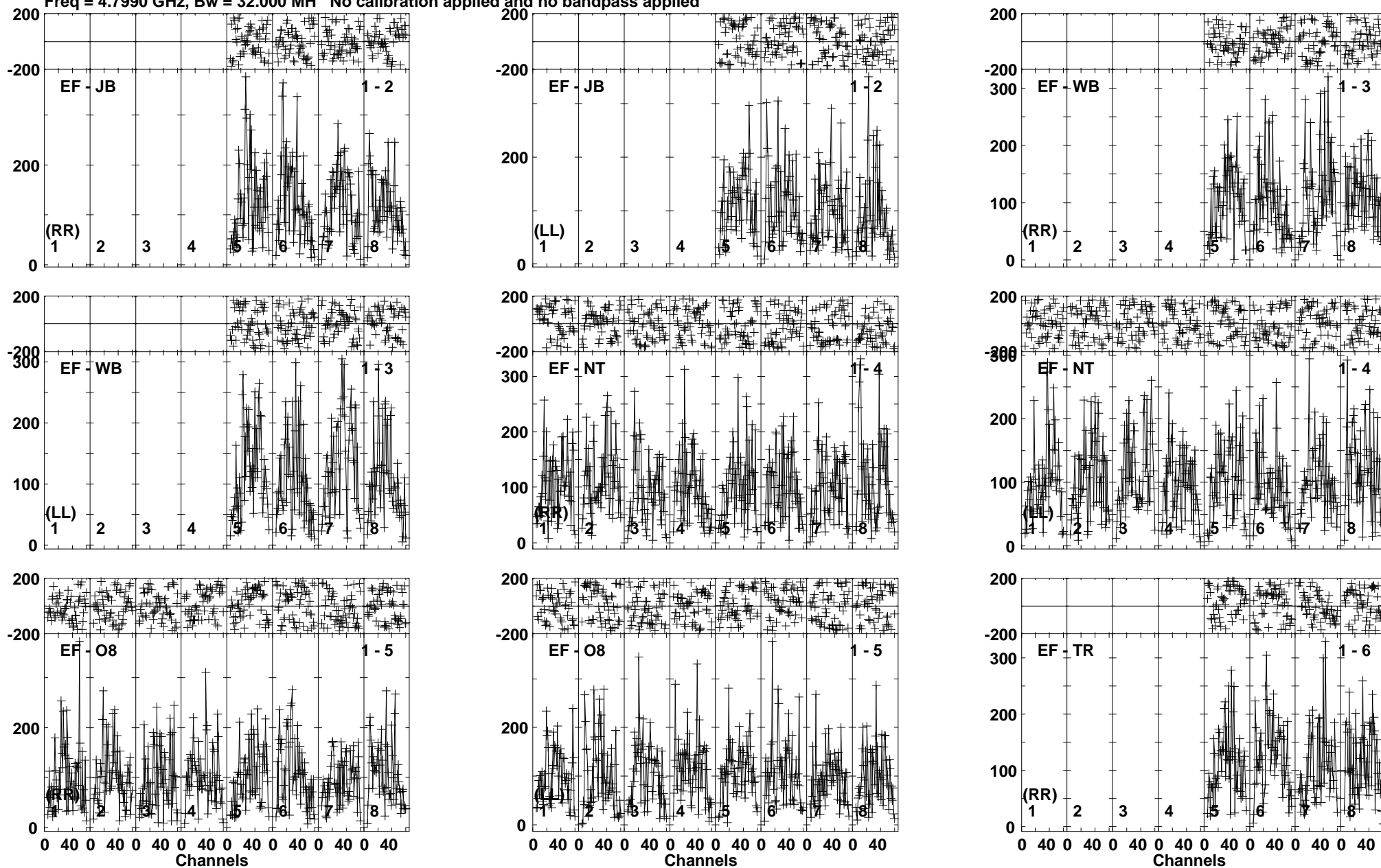
Lower frame: Micro Ampl Jy Top frame: Phas deg Vector averaged cross-power spectrum Baseline: EF (01) - JB (02) Timerange: 00/13:14:30 to 00/13:16:59
