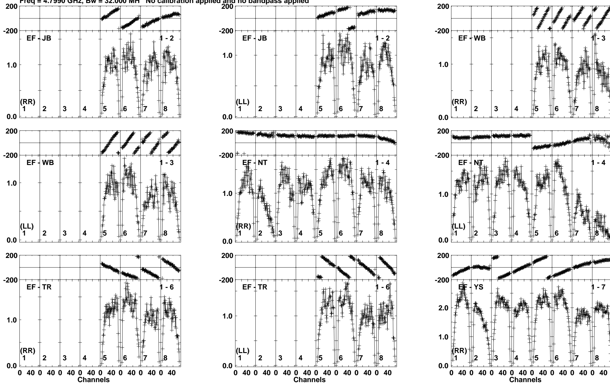
Lower frame: Milli Ampl Jy Top frame: Phas deg Vector averaged cross-power spectrum Baseline: EF (01) - JB (02) Timerange: 00/14:10:00 to 00/14:10:58
