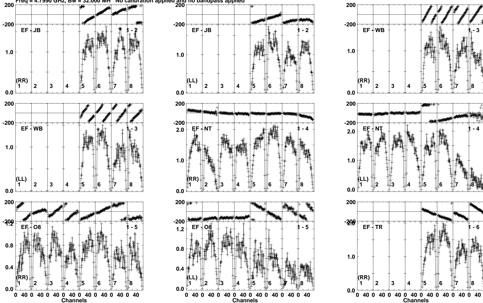
Lower frame: Milli Ampl Jy Top frame: Phas deg Vector averaged cross-power spectrum Baseline: EF (01) - JB (02) Timerange: 00:12:44:39 to 00:12:46:08
