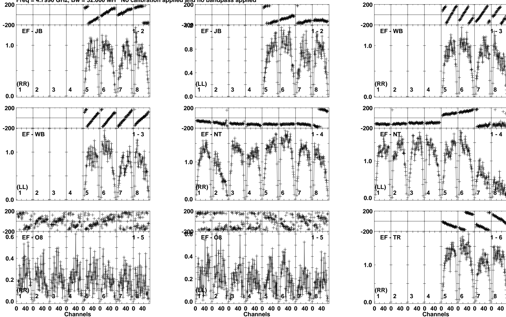
Lower frame: Milli Ampl Jy Top frame: Phas deg Vector averaged cross-power spectrum Baseline: EF (01) - JB (02) Timerange: 00/10:52:20 to 00/10:53:48
