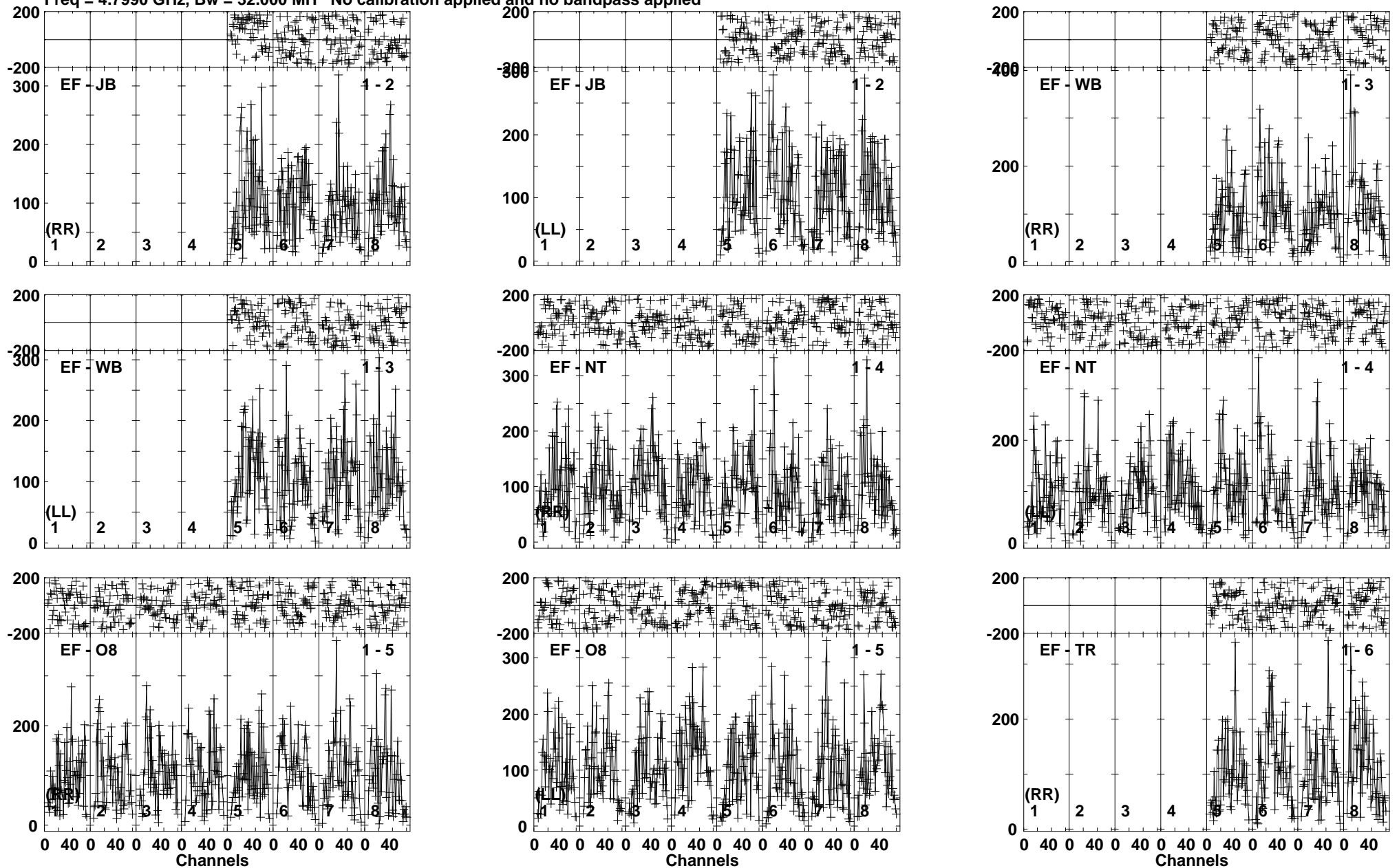
Lower frame: Micro Ampl Jy Top frame: Phas deg Vector averaged cross-power spectrum Baseline: EF (01) - JB (02) Timerange: 00/10:41:49 to 00/10:44:18
