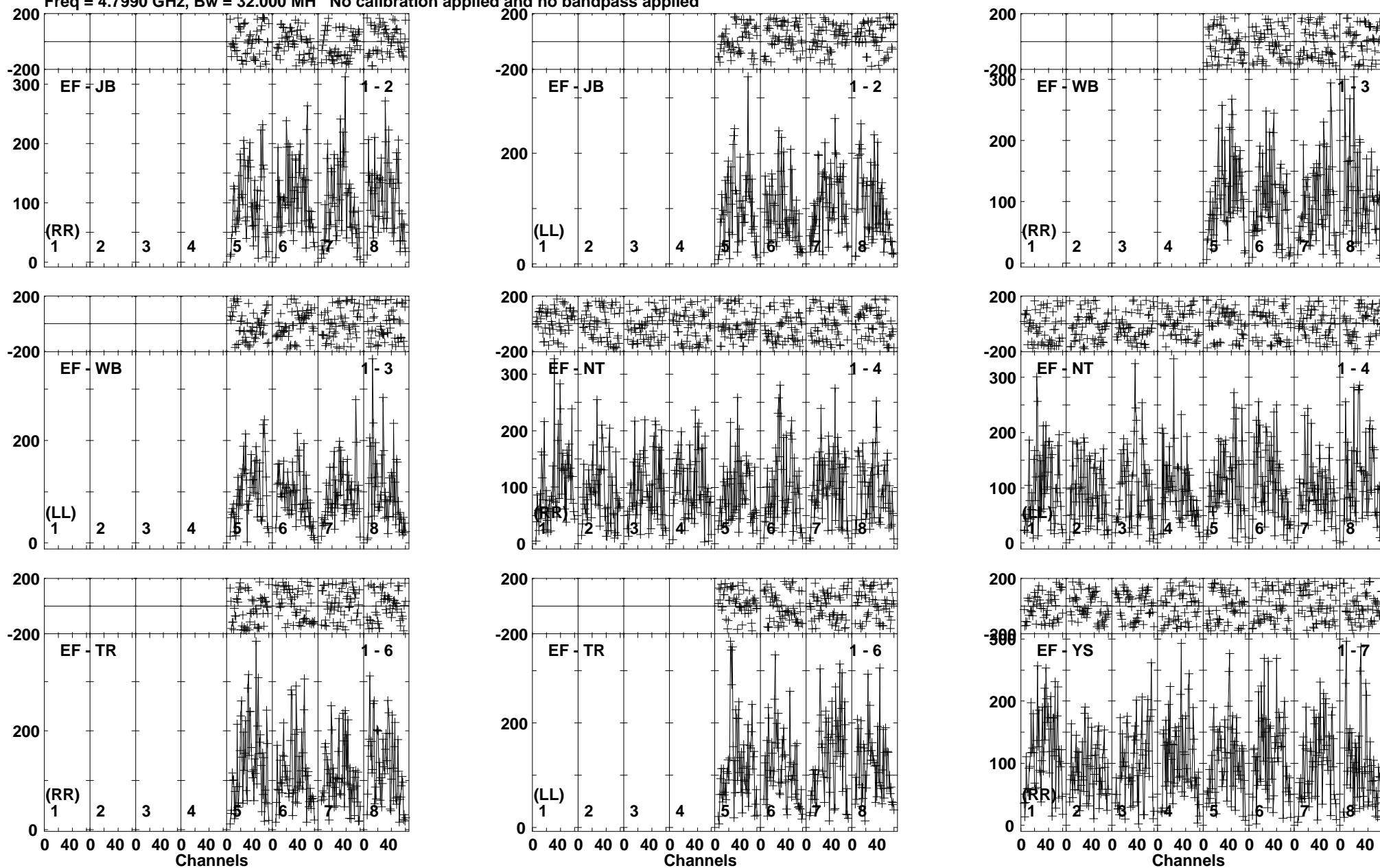
Lower frame: Micro Ampl Jy Top frame: Phas deg Vector averaged cross-power spectrum Baseline: EF (01) - JB (02) Timerange: 00/14:11:00 to 00/14:13:28
