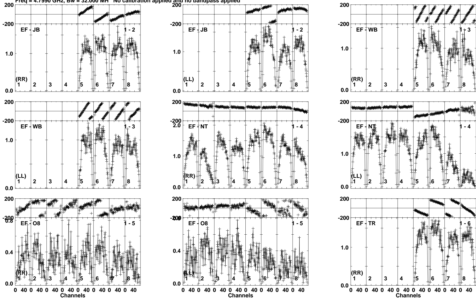
Lower frame: Milli Ampl Jy Top frame: Phas deg Vector averaged cross-power spectrum Baseline: EF (01) - JB (02) Timerange: 00/13:45:50 to 00/13:46:48
