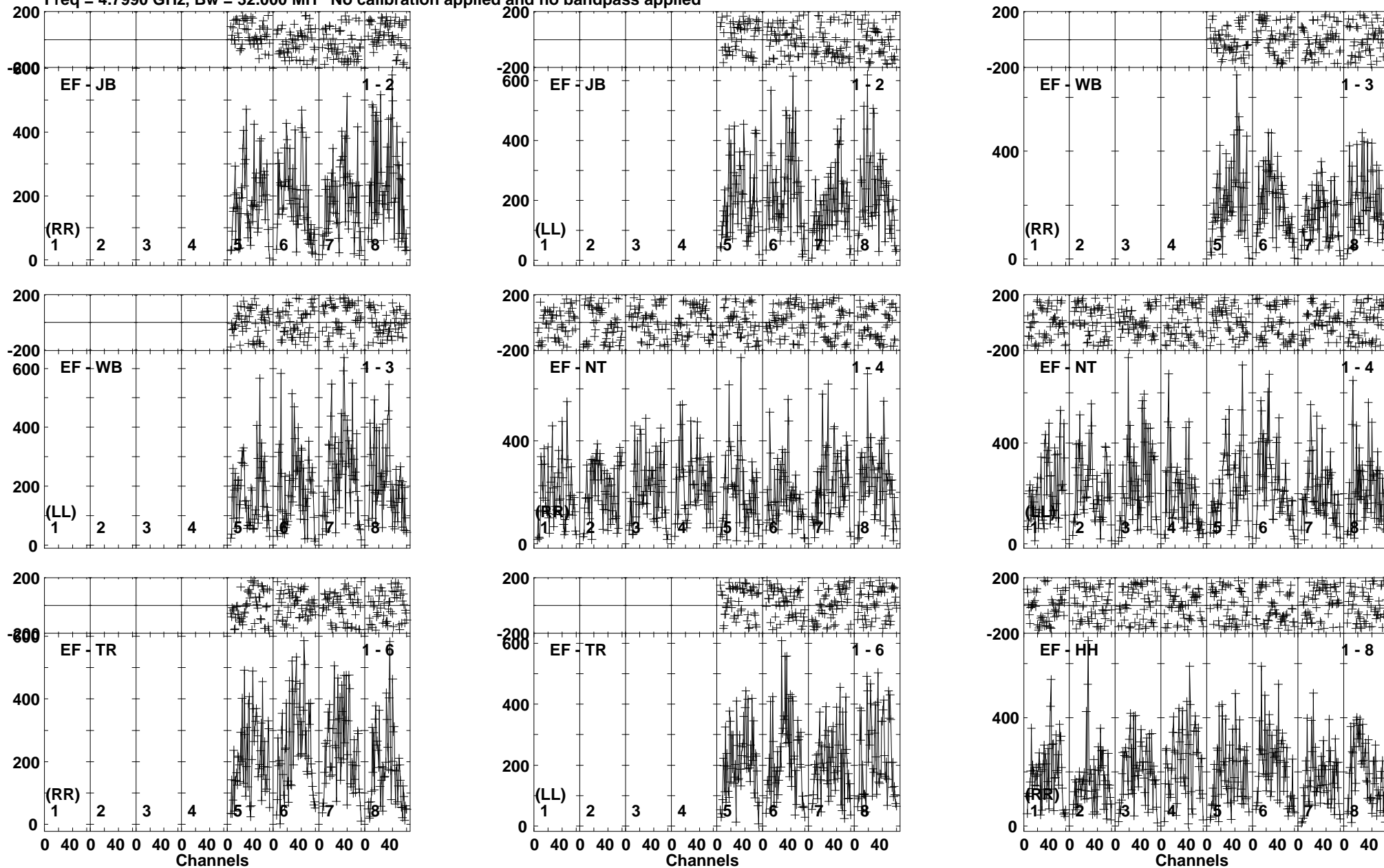
Lower frame: Micro Ampl Jy Top frame: Phas deg Vector averaged cross-power spectrum Baseline: EF (01) - JB (02) Timerange: 00/10:24:40 to 00/10:25:38
