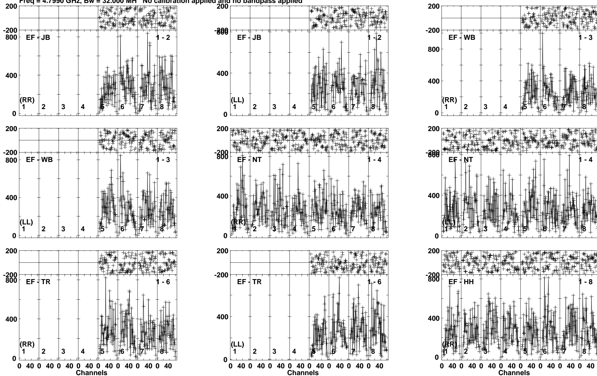
Lower frame: Micro Ampl Jy Top frame: Phas deg Vector averaged cross-power spectrum Baseline: EF (01) - JB (02) Timerange: 00/10:17:29 to 00/10:19:59
