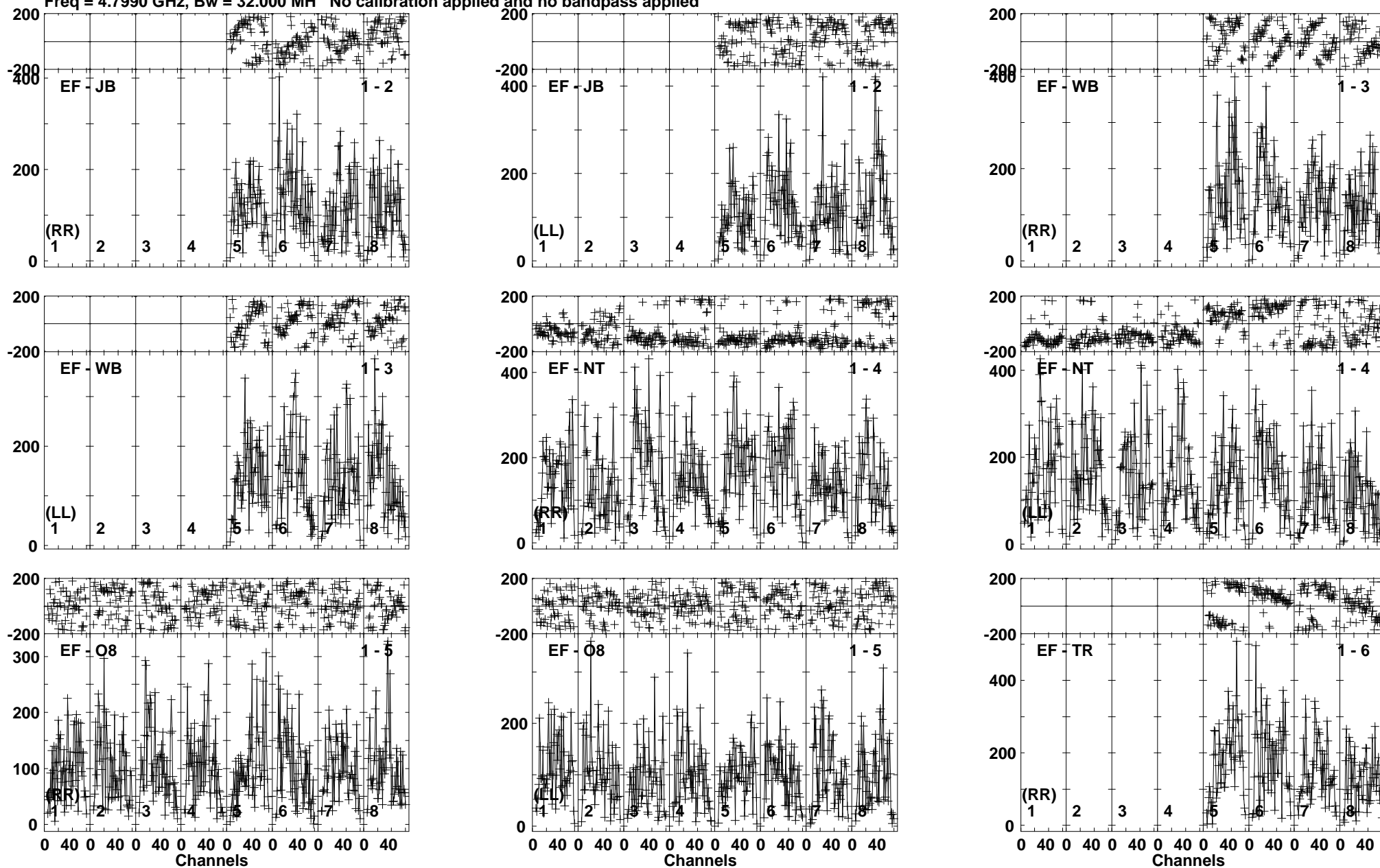
Lower frame: Micro Ampl Jy Top frame: Phas deg Vector averaged cross-power spectrum Baseline: EF (01) - JB (02) Timerange: 00/10:53:49 to 00/10:56:19
