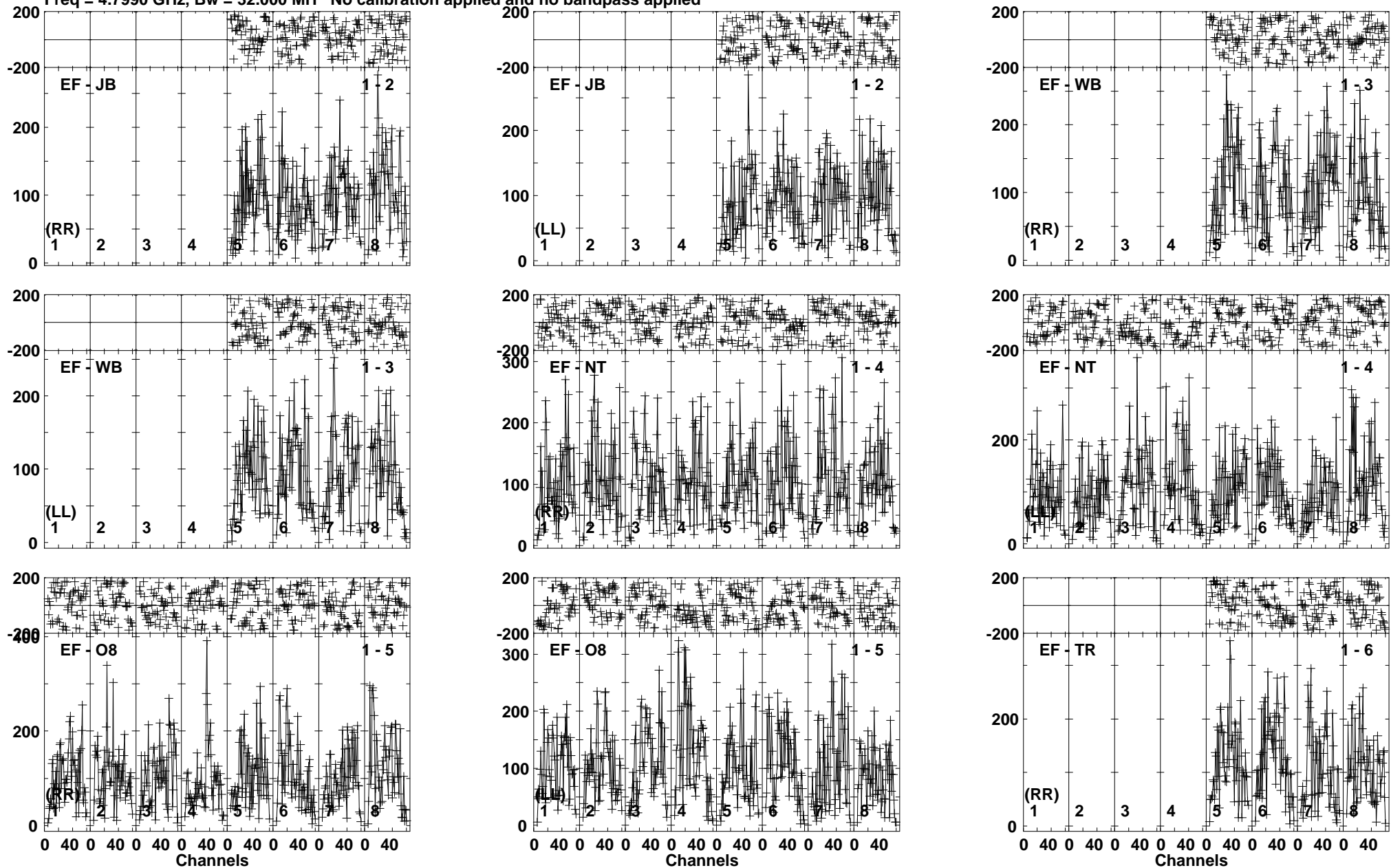
Lower frame: Micro Ampl Jy Top frame: Phas deg Vector averaged cross-power spectrum Baseline: EF (01) - JB (02) Timerange: 00/11:18:10 to 00/11:20:38
