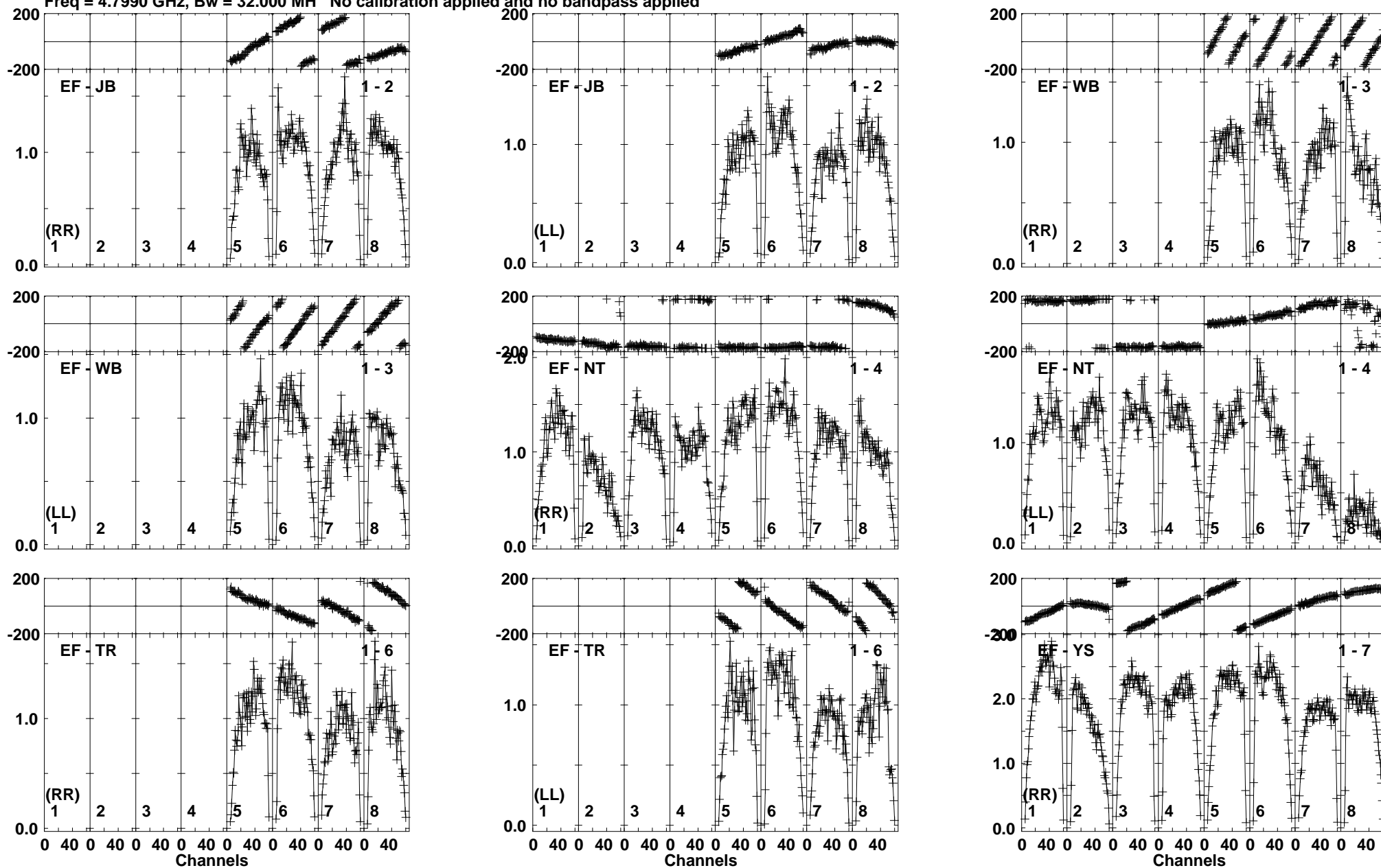
Lower frame: Milli Ampl Jy Top frame: Phas deg Vector averaged cross-power spectrum Baseline: EF (01) - JB (02) Timerange: 00/14:05:30 to 00/14:06:59
