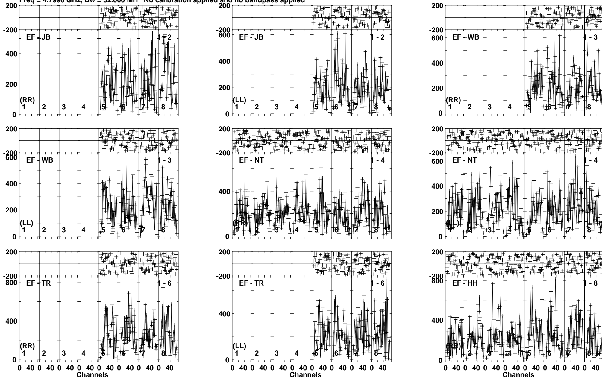
Lower frame: Micro Ampl Jy Top frame: Phas deg Vector averaged cross-power spectrum Baseline: EF (01) - JB (02) Timerange: 00/10:16:30 to 00/10:17:29
