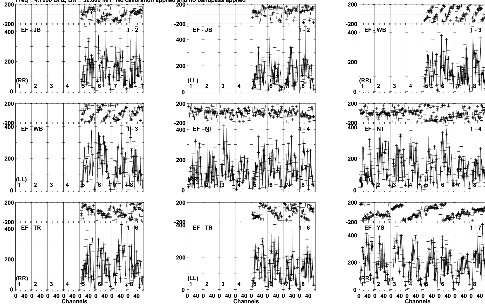
Lower frame: Micro Ampl Jy Top frame: Phas deg Vector averaged cross-power spectrum Baseline: EF (01) - JB (02) Timerange: 00/13:58:50 to 00/14:01:18
