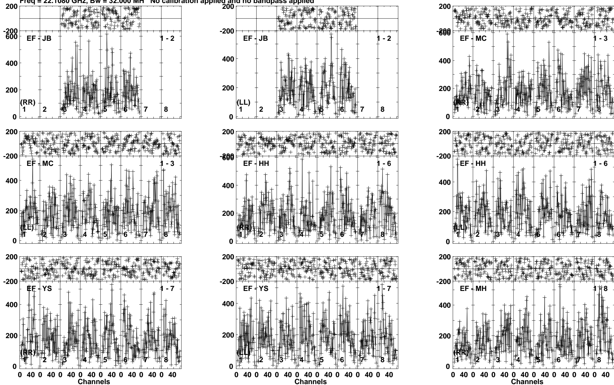
Lower frame: Micro Ampl Jy Top frame: Phas deg Vector averaged cross-power spectrum Baseline: EF (01) - JB (02) Timerange: 00/23:34:01 to 00/23:34:39
