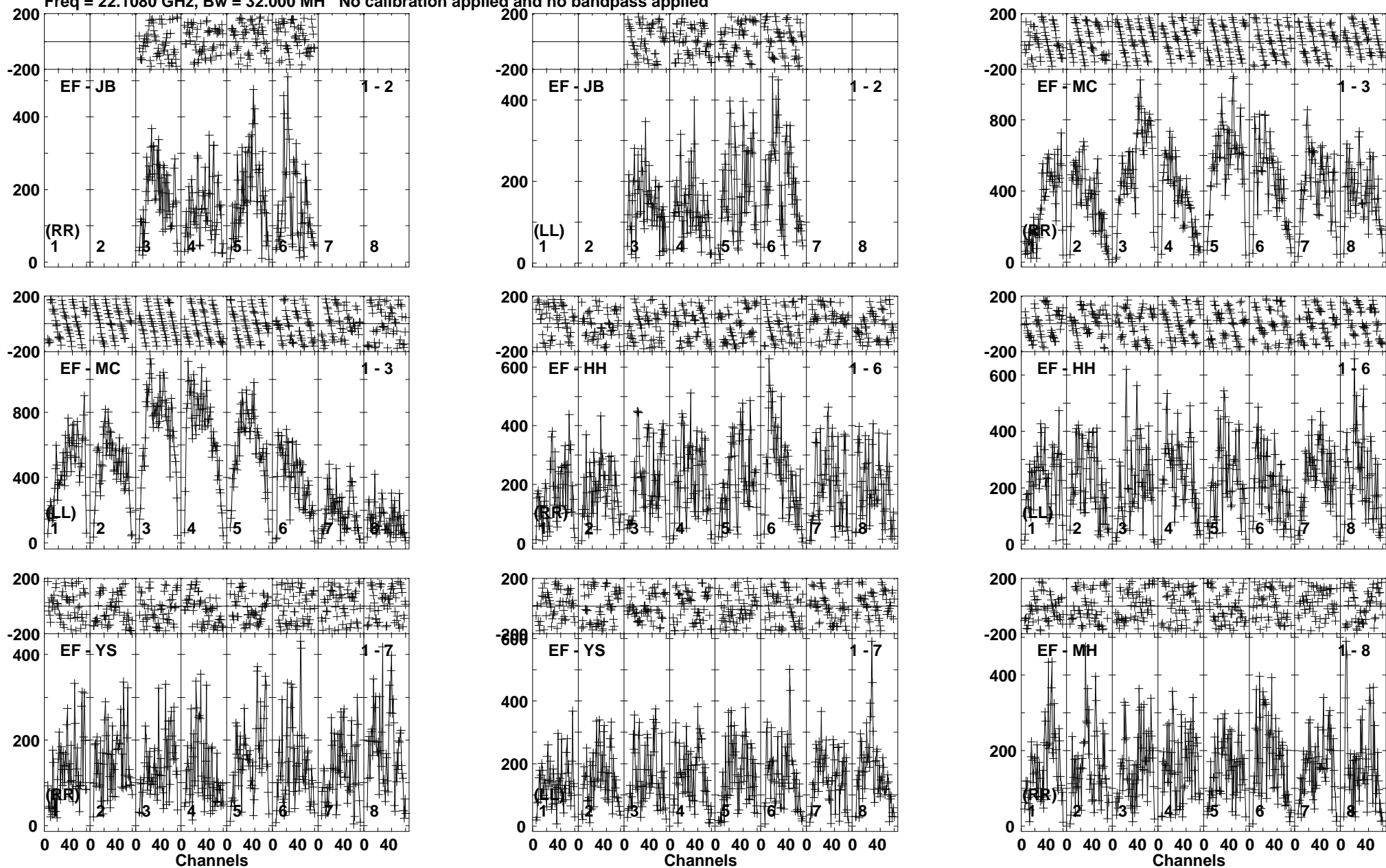
Lower frame: Micro Ampl Jy Top frame: Phas deg Vector averaged cross-power spectrum Baseline: EF (01) - JB (02) Timerange: 01/01:46:41 to 01/01:47:39
