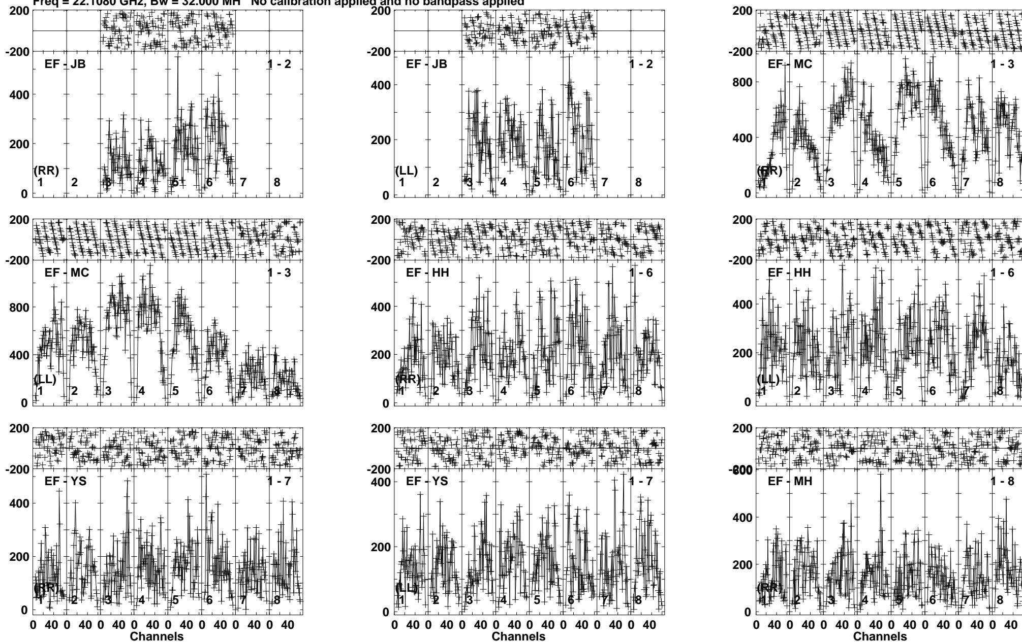
Lower frame: Micro Ampl Jy Top frame: Phas deg Vector averaged cross-power spectrum Baseline: EF (01) - JB (02) Timerange: 01/01:42:41 to 01/01:43:40
