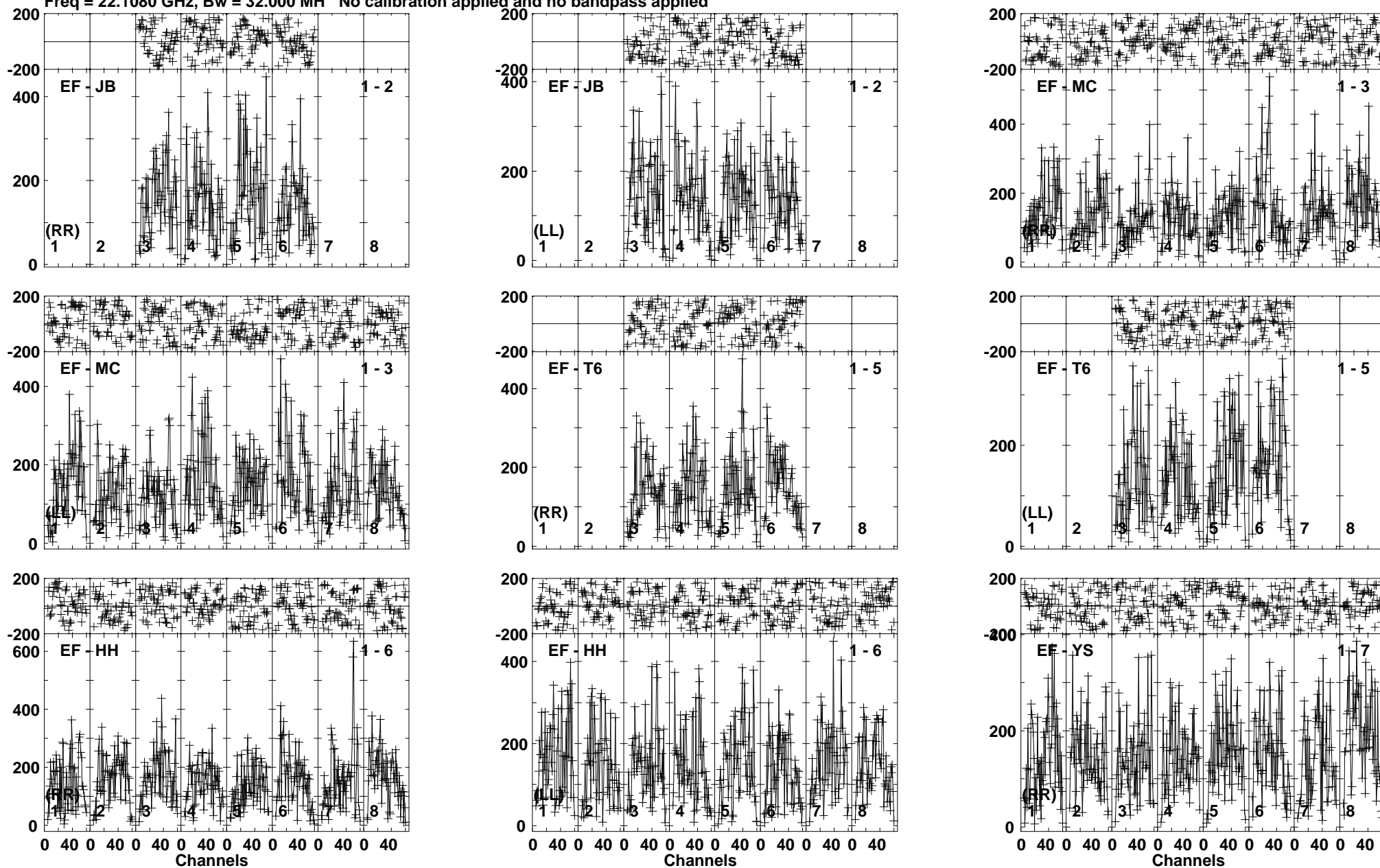
Lower frame: Micro Ampl Jy Top frame: Phas deg Vector averaged cross-power spectrum Baseline: EF (01) - JB (02) Timerange: 00/22:25:41 to 00/22:26:39
