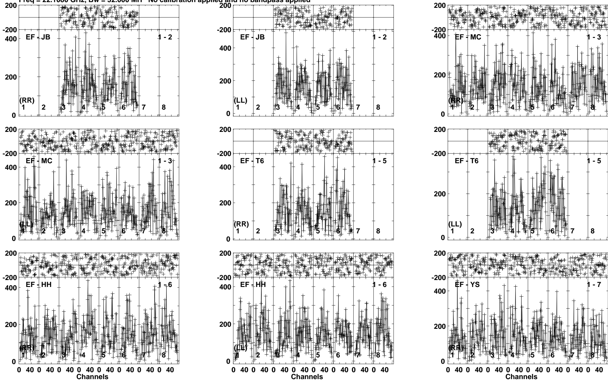
Lower frame: Micro Ampl Jy Top frame: Phas deg Vector averaged cross-power spectrum Baseline: EF (01) - JB (02) Timerange: 00/22:20:41 to 00/22:21:39
