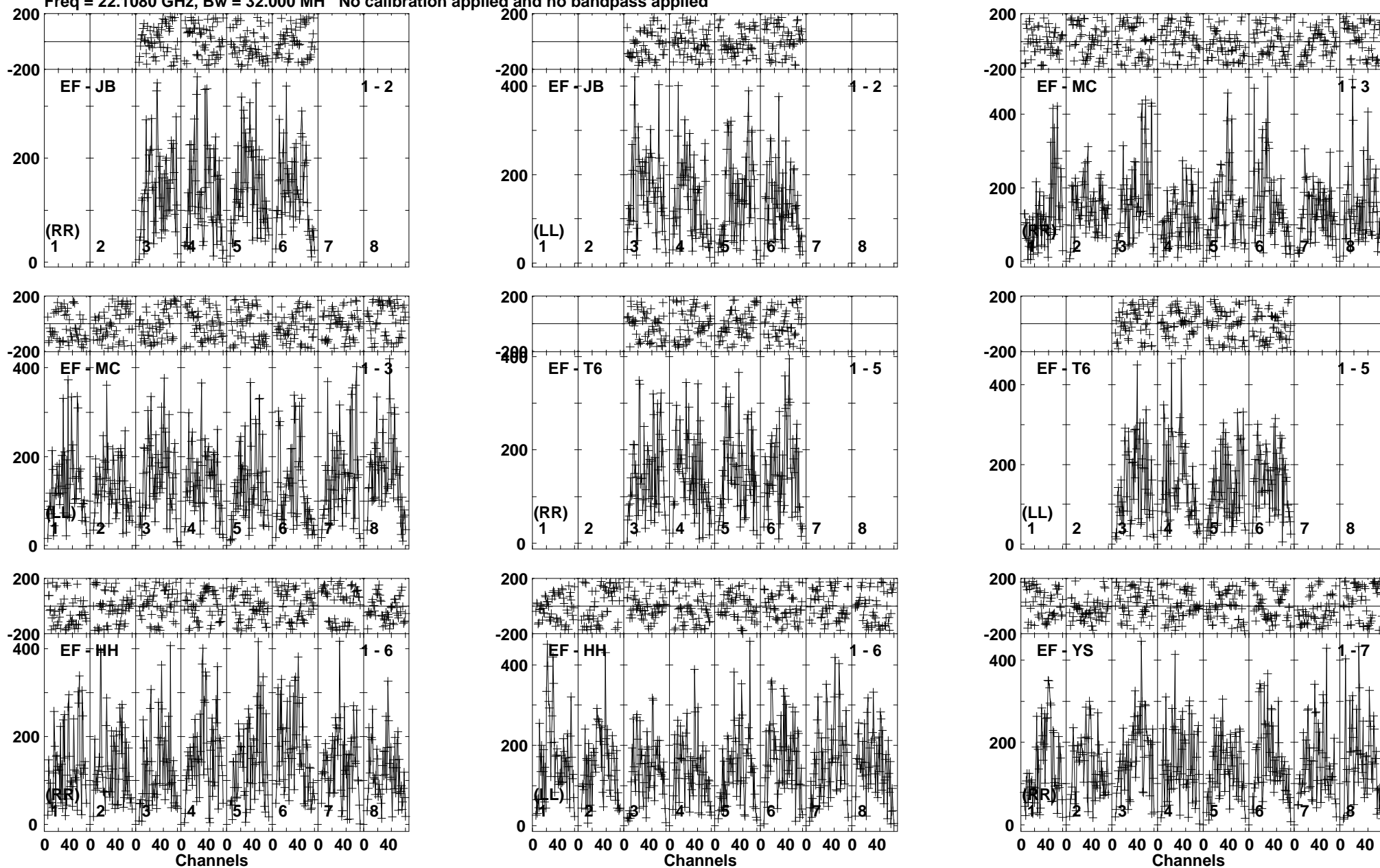
Lower frame: Micro Ampl Jy Top frame: Phas deg Vector averaged cross-power spectrum Baseline: EF (01) - JB (02) Timerange: 00/22:15:21 to 00/22:16:19
