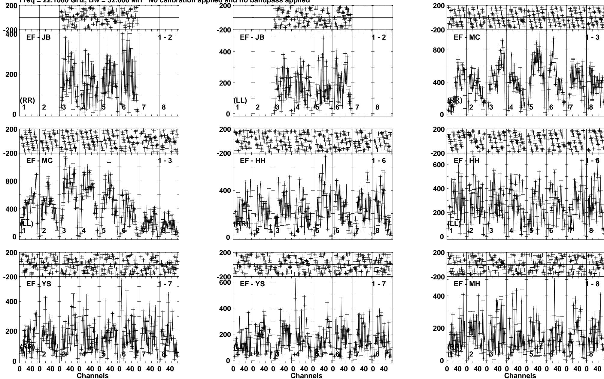
Lower frame: Micro Ampl Jy Top frame: Phas deg Vector averaged cross-power spectrum Baseline: EF (01) - JB (02) Timerange: 01/00:20:41 to 01/00:21:40
