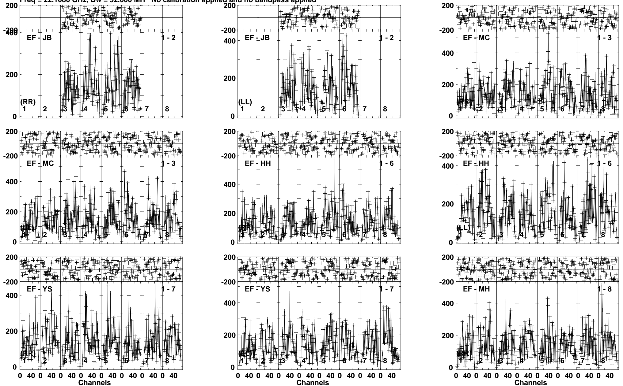
Lower frame: Micro Ampl Jy Top frame: Phas deg Vector averaged cross-power spectrum Baseline: EF (01) - JB (02) Timerange: 01/01:45:41 to 01/01:46:40
