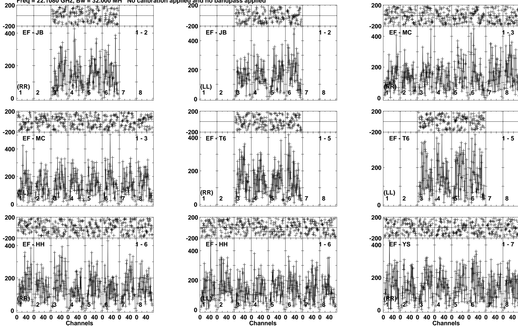
Lower frame: Micro Ampl Jy Top frame: Phas deg Vector averaged cross-power spectrum Baseline: EF (01) - JB (02) Timerange: 00/22:21:40 to 00/22:22:39
