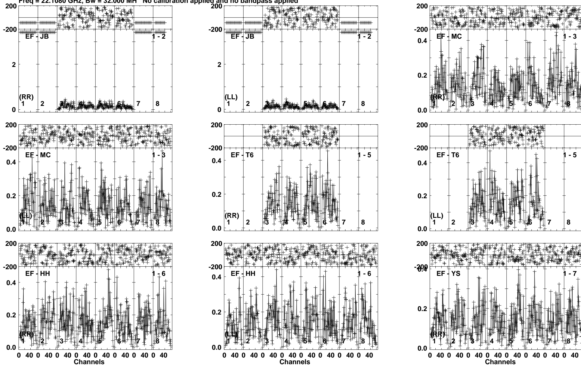
Lower frame: Milli Ampl Jy Top frame: Phas deg Vector averaged cross-power spectrum Baseline: EF (01) - JB (02) Timerange: 00/22:50:20 to 00/22:51:19
