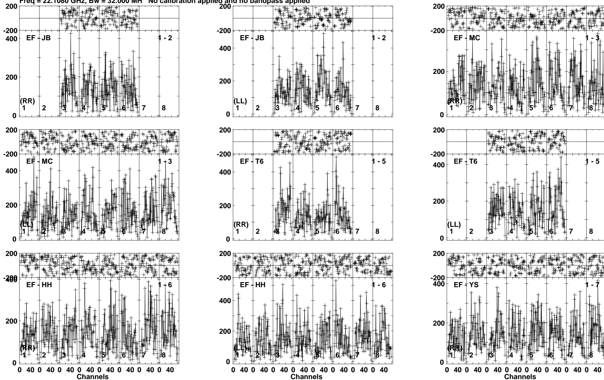
Lower frame: Micro Ampl Jy Top frame: Phas deg Vector averaged cross-power spectrum Baseline: EF (01) - JB (02) Timerange: 00:22:41:00 to 00:22:41:59
