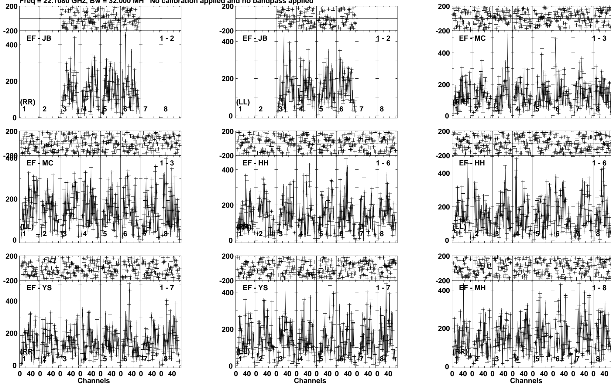
Lower frame: Micro Ampl Jy Top frame: Phas deg Vector averaged cross-power spectrum Baseline: EF (01) - JB (02) Timerange: 01/02:14:21 to 01/02:15:19
