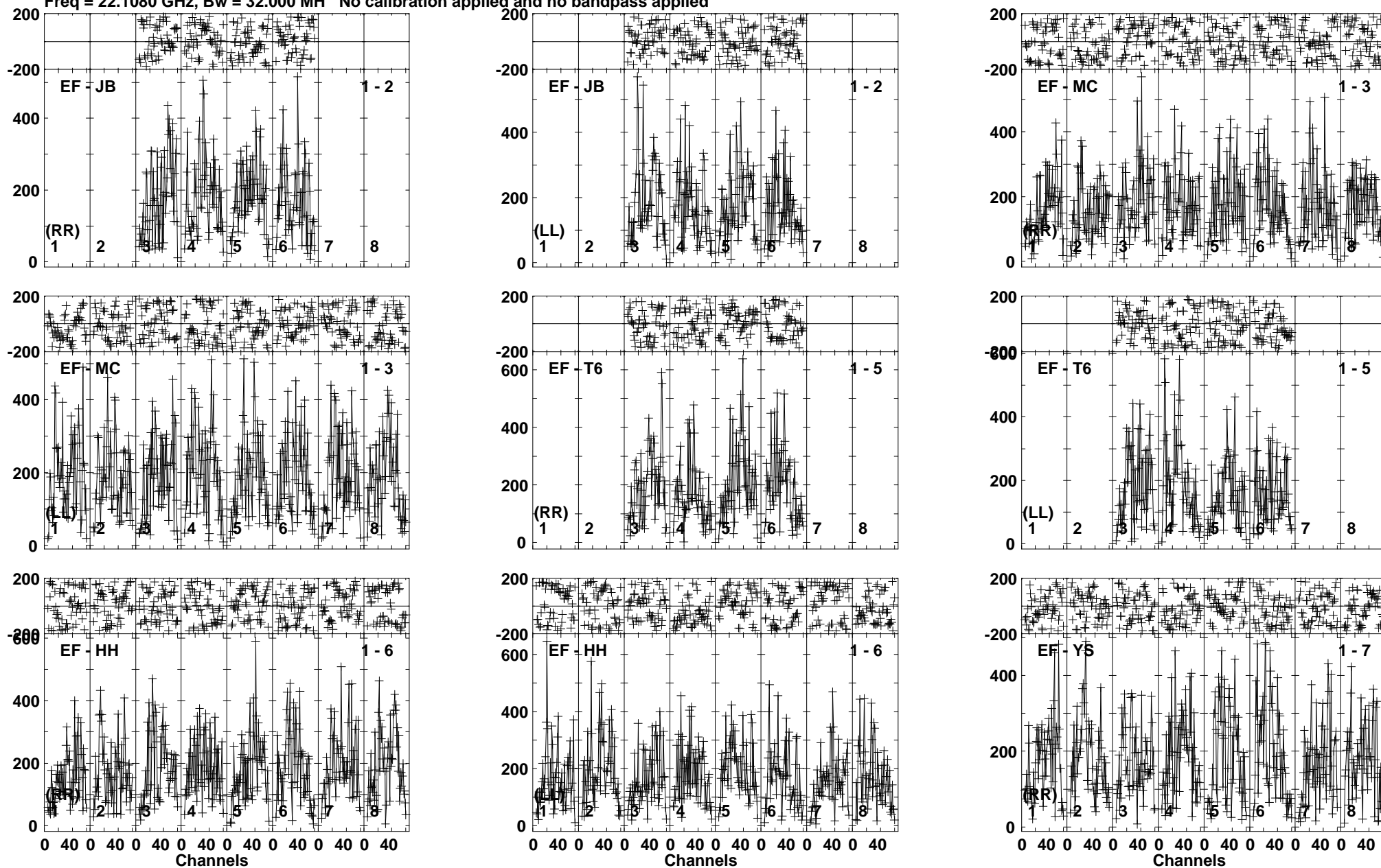
Lower frame: Micro Ampl Jy Top frame: Phas deg Vector averaged cross-power spectrum Baseline: EF (01) - JB (02) Timerange: 00/22:32:21 to 00/22:32:59
