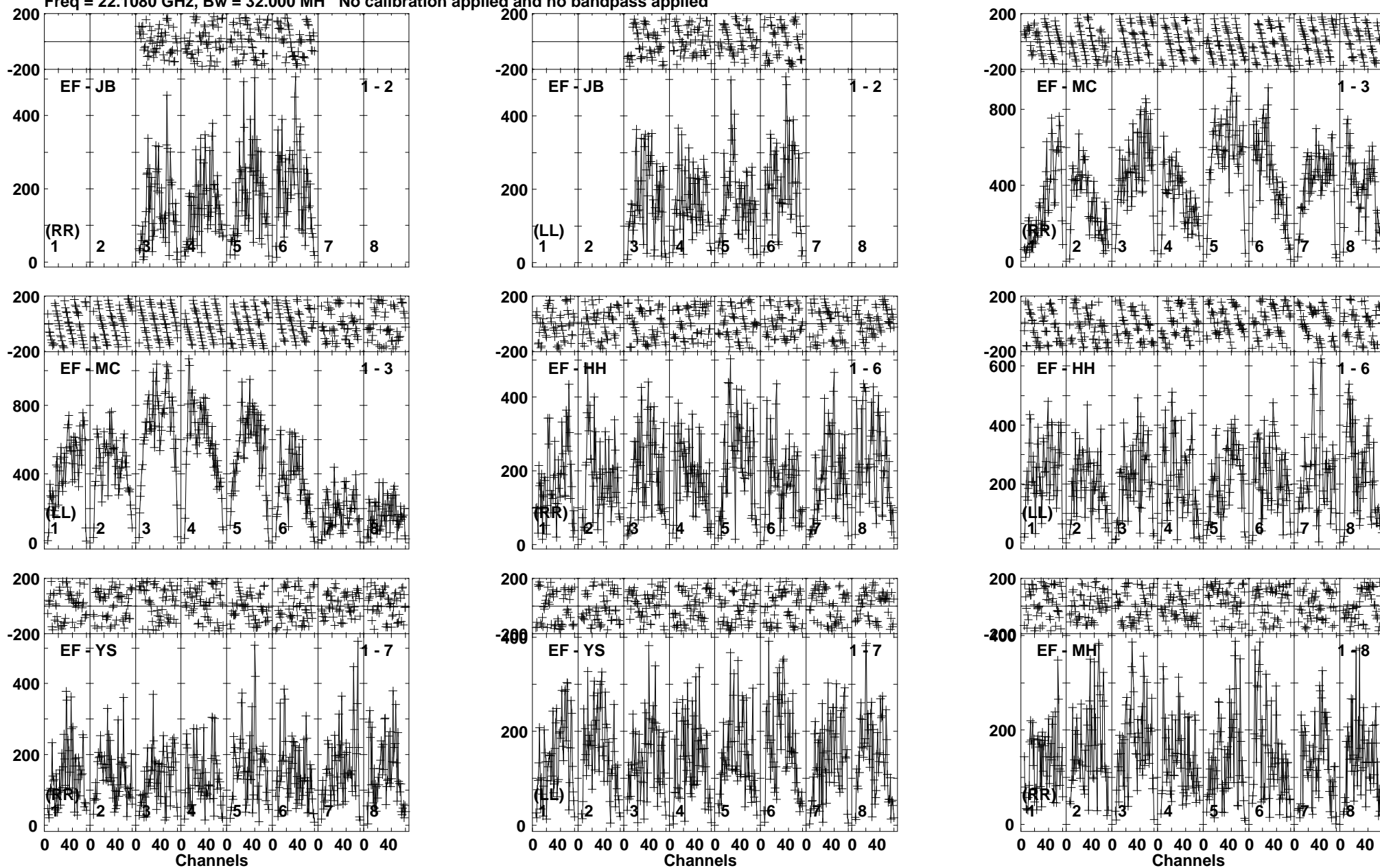
Lower frame: Micro Ampl Jy Top frame: Phas deg Vector averaged cross-power spectrum Baseline: EF (01) - JB (02) Timerange: 01/02:21:41 to 01/02:22:39
