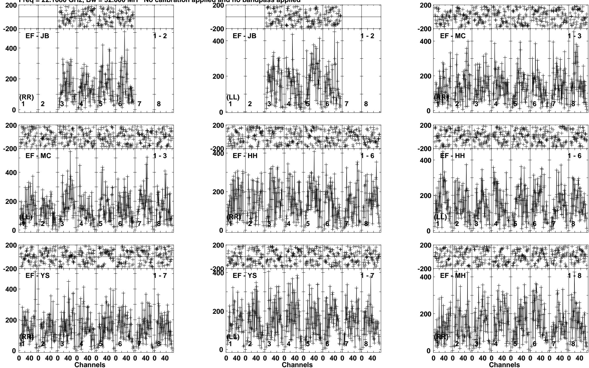
Lower frame: Micro Ampl Jy Top frame: Phas deg Vector averaged cross-power spectrum Baseline: EF (01) - JB (02) Timerange: 01/00:13:41 to 01/00:14:40
