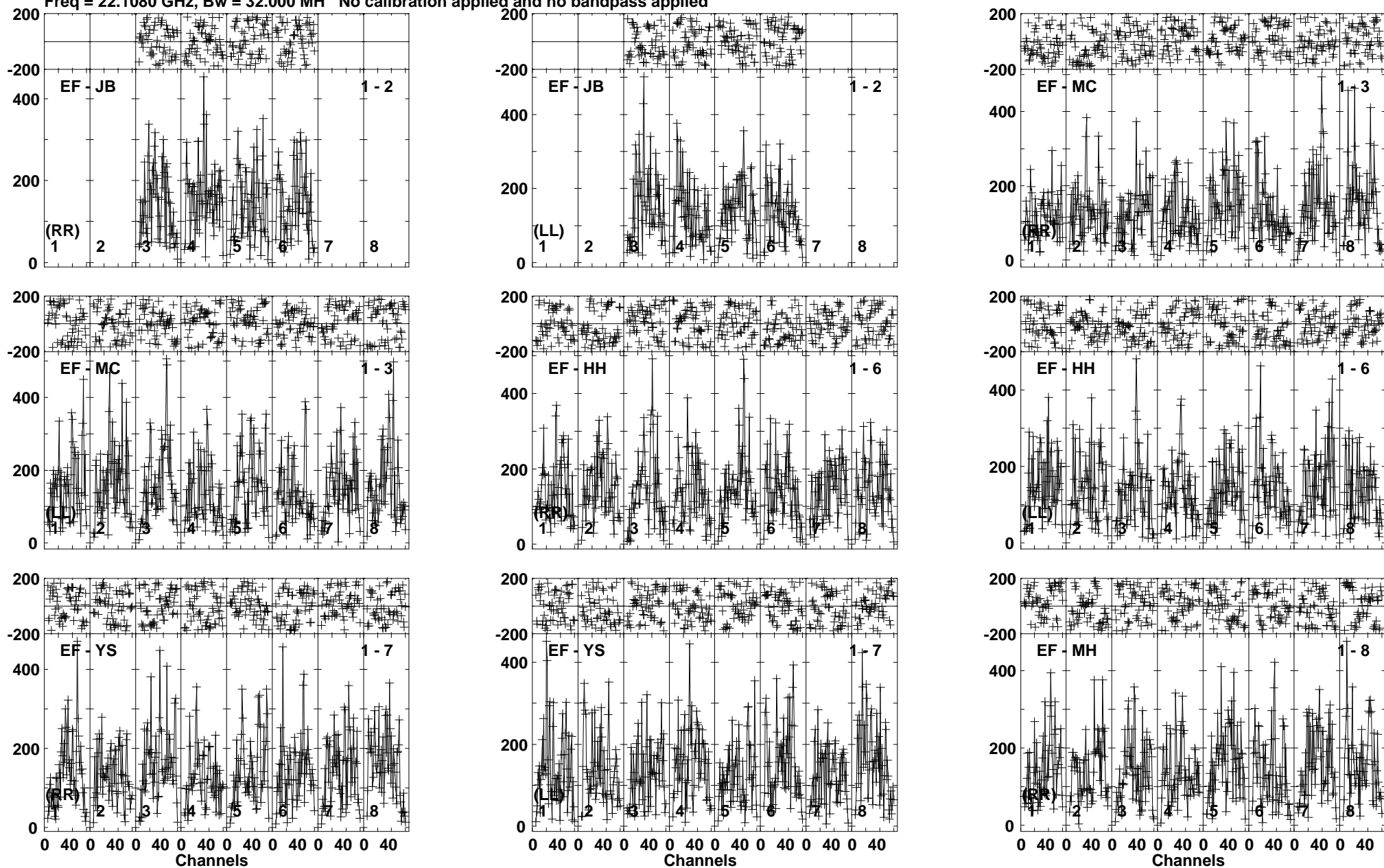
Lower frame: Micro Ampl Jy Top frame: Phas deg Vector averaged cross-power spectrum Baseline: EF (01) - JB (02) Timerange: 01/01:23:20 to 01/01:24:19
