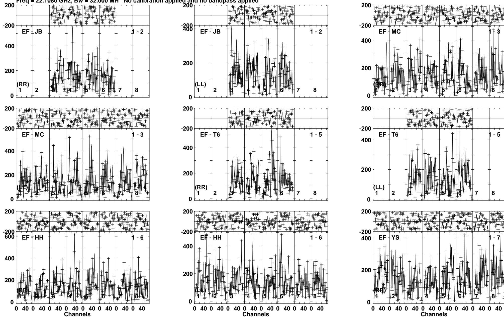
Lower frame: Micro Ampl Jy Top frame: Phas deg Vector averaged cross-power spectrum Baseline: EF (01) - JB (02) Timerange: 00/23:04:41 to 00/23:05:40
