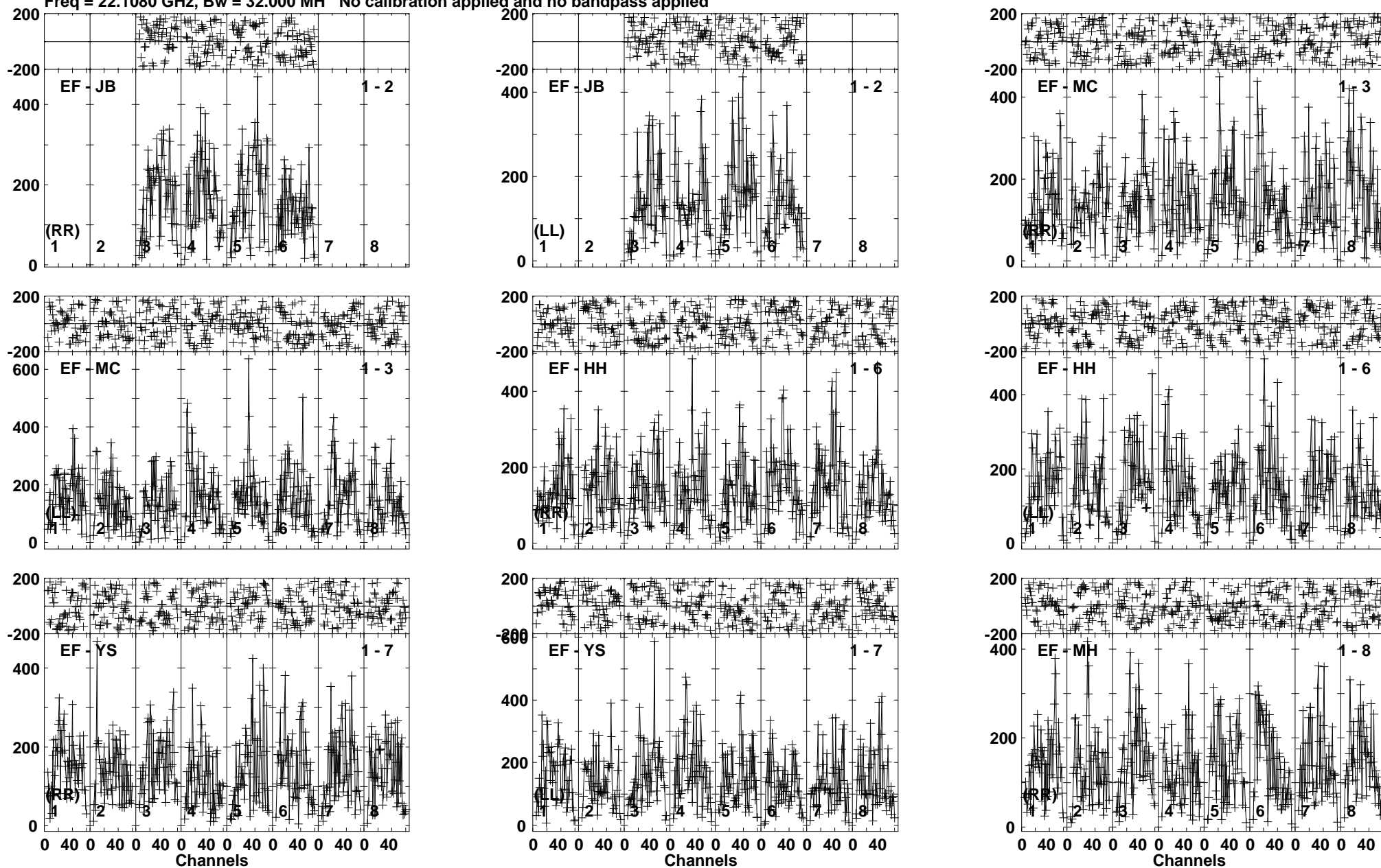
Lower frame: Micro Ampl Jy Top frame: Phas deg Vector averaged cross-power spectrum Baseline: EF (01) - JB (02) Timerange: 00/23:34:40 to 00/23:35:39
