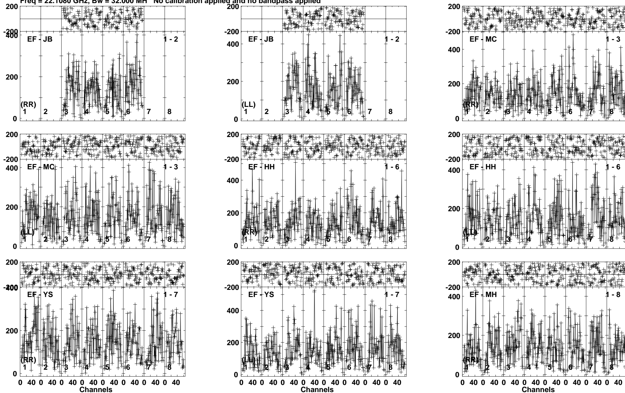
Lower frame: Micro Ampl Jy Top frame: Phas deg Vector averaged cross-power spectrum Baseline: EF (01) - JB (02) Timerange: 01/02:02:00 to 01/02:02:59
