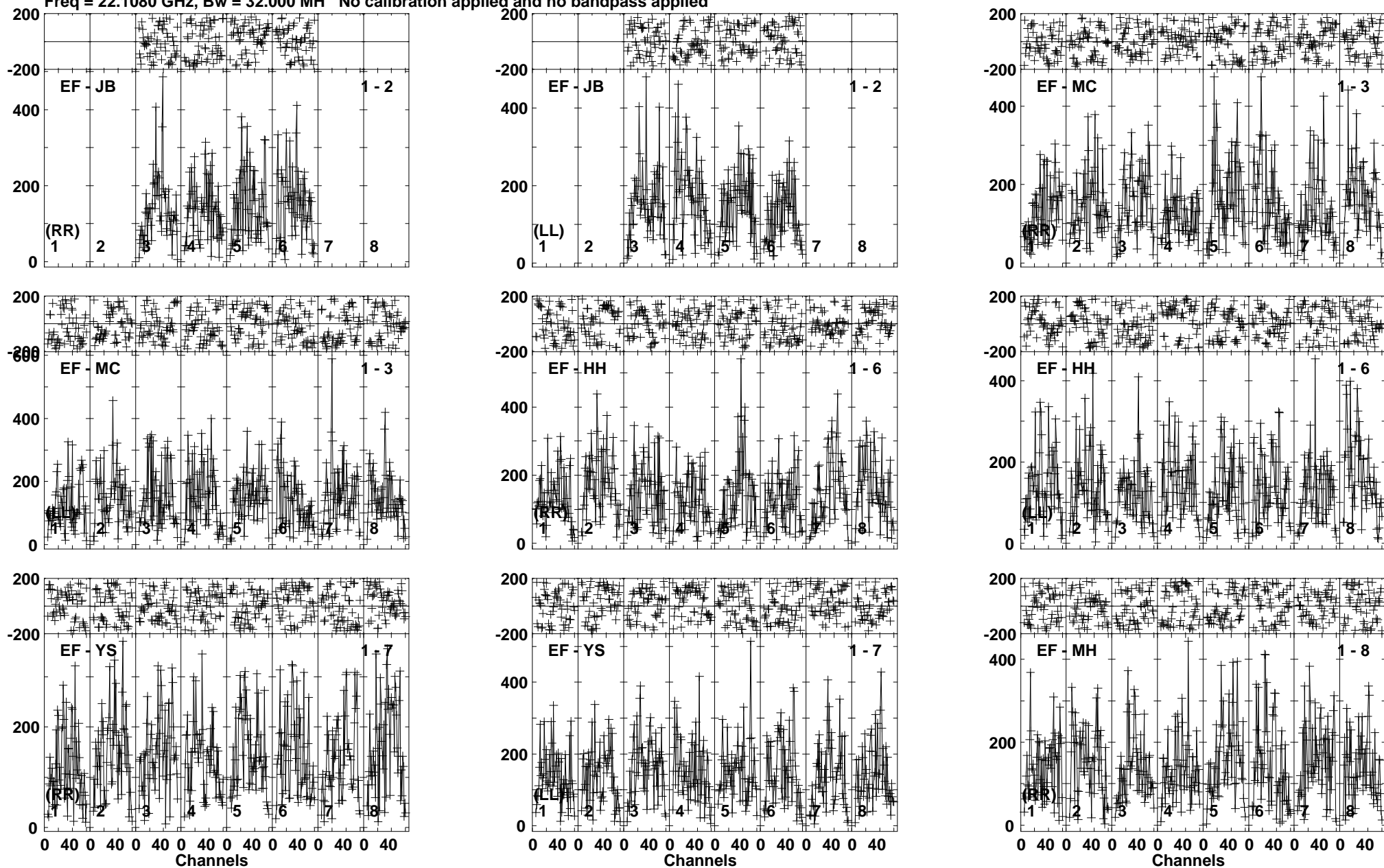
Lower frame: Micro Ampl Jy Top frame: Phas deg Vector averaged cross-power spectrum Baseline: EF (01) - JB (02) Timerange: 00/23:31:21 to 00/23:32:19
