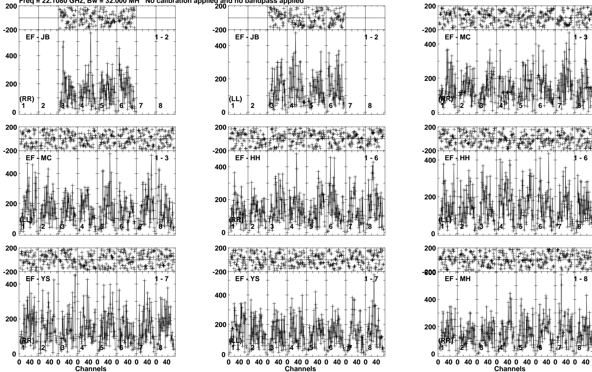
Lower frame: Micro Ampl Jy Top frame: Phas deg Vector averaged cross-power spectrum Baseline: EF (01) - JB (02) Timerange: 01/03:05:41 to 01/03:06:40
