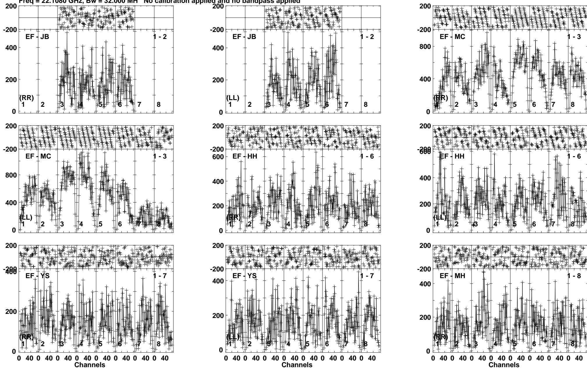
Lower frame: Micro Ampl Jy Top frame: Phas deg Vector averaged cross-power spectrum Baseline: EF (01) - JB (02) Timerange: 01/01:48:41 to 01/01:49:39
