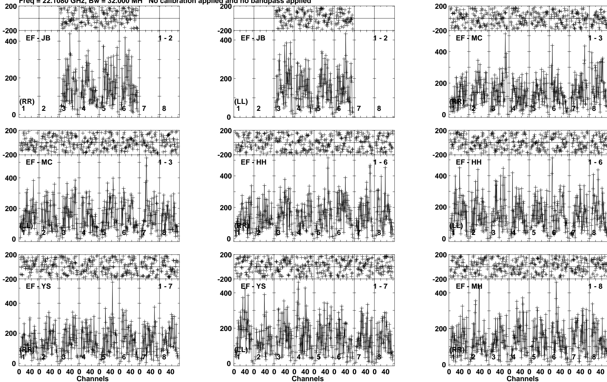
Lower frame: Micro Ampl Jy Top frame: Phas deg Vector averaged cross-power spectrum Baseline: EF (01) - JB (02) Timerange: 01/02:22:40 to 01/02:23:39
