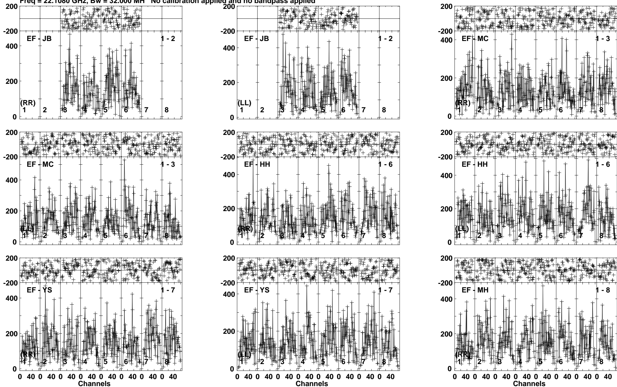
Lower frame: Micro Ampl Jy Top frame: Phas deg Vector averaged cross-power spectrum Baseline: EF (01) - JB (02) Timerange: 01/02:18:40 to 01/02:19:39
