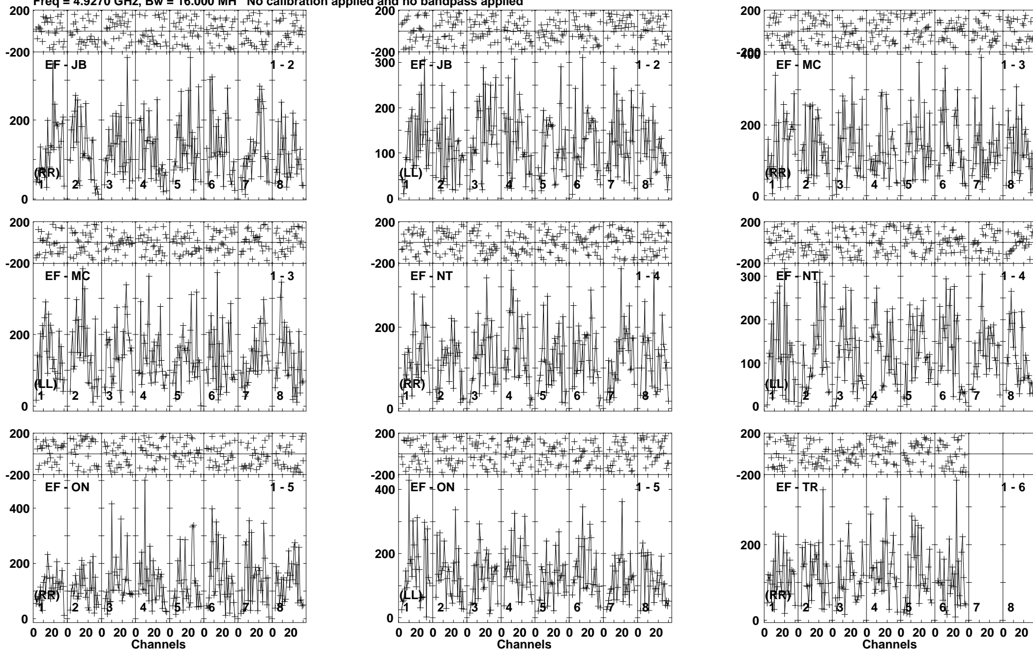
Lower frame: Micro Ampl Jy Top frame: Phas deg Vector averaged cross-power spectrum Baseline: EF (01) - JB (02) Timerange: 00/05:55:42 to 00/05:58:58
