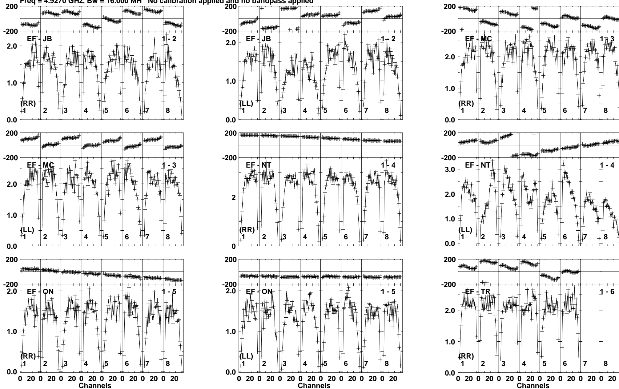
Lower frame: Milli Ampl Jy Top frame: Phas deg Vector averaged cross-power spectrum Baseline: EF (01) - JB (02) Timerange: 00/05:14:42 to 00/05:15:38
