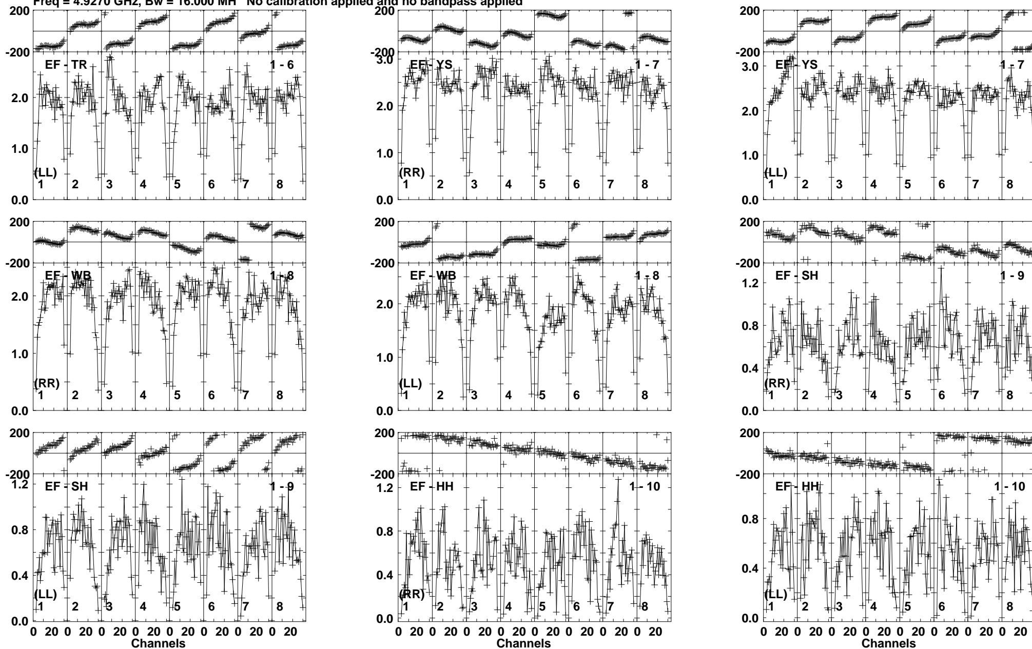
Lower frame: Milli Ampl Jy Top frame: Phas deg Vector averaged cross-power spectrum Baseline: EF (01) - TR (06) Timerange: 00/04:12:22 to 00/04:13:18
