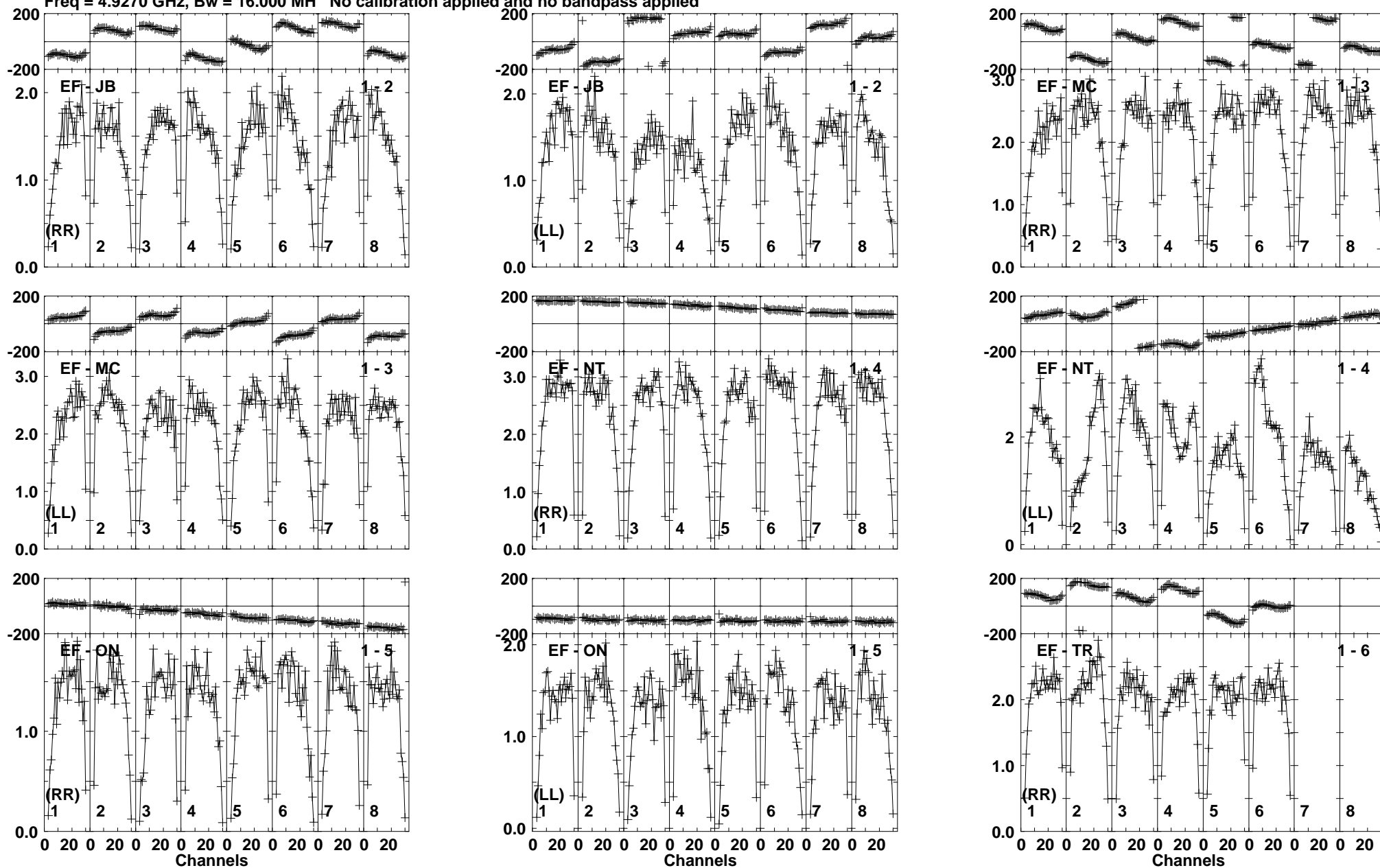
Lower frame: Milli Ampl Jy Top frame: Phas deg Vector averaged cross-power spectrum Baseline: EF (01) - JB (02) Timerange: 00/05:19:02 to 00/05:20:28
