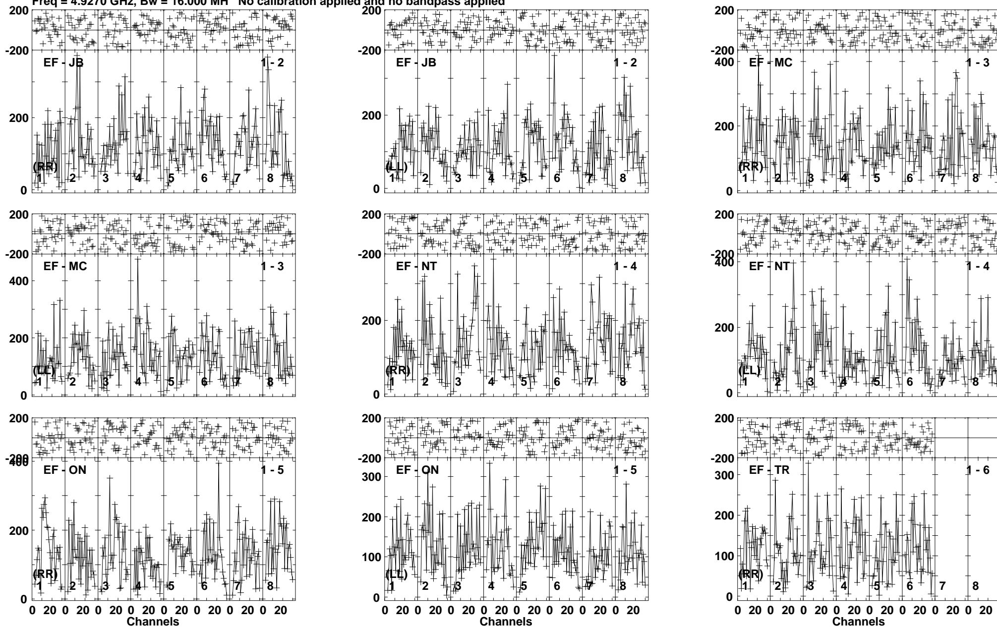
Lower frame: Micro Ampl Jy Top frame: Phas deg Vector averaged cross-power spectrum Baseline: EF (01) - JB (02) Timerange: 00/08:14:12 to 00/08:17:28
