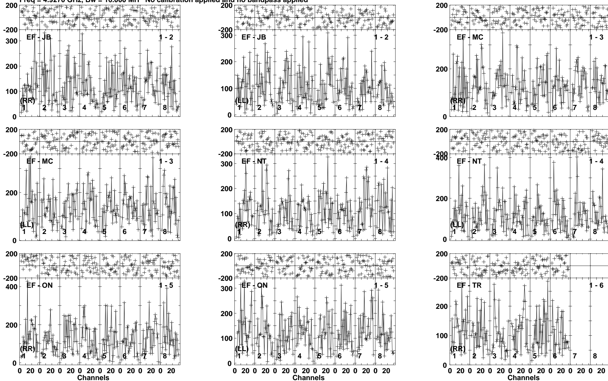
Lower frame: Micro Ampl Jy Top frame: Phas deg Vector averaged cross-power spectrum Baseline: EF (01) - JB (02) Timerange: 00/09:27:32 to 00/09:30:58
