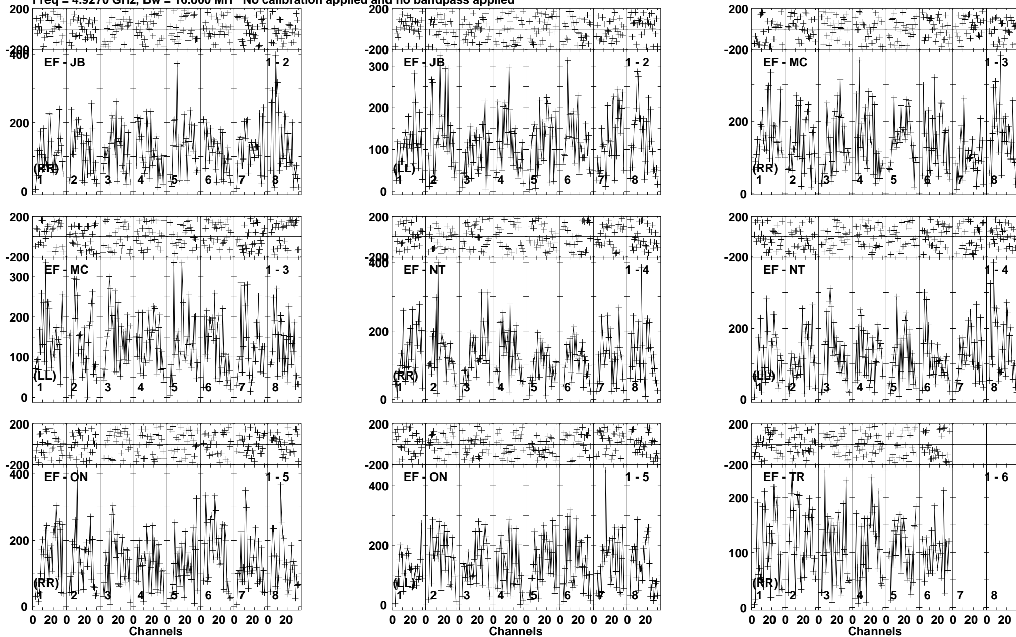
Lower frame: Micro Ampl Jy Top frame: Phas deg Vector averaged cross-power spectrum Baseline: EF (01) - JB (02) Timerange: 00/07:29:02 to 00/07:32:28
