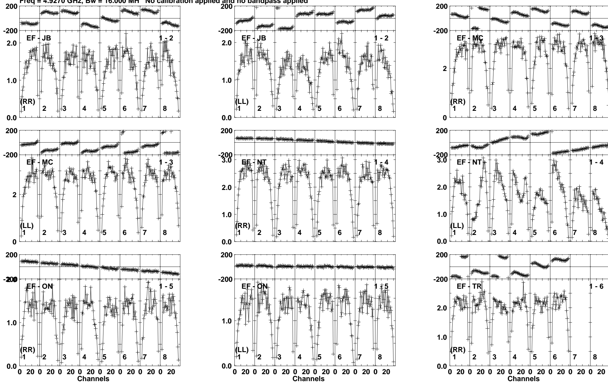
Lower frame: Milli Ampl Jy Top frame: Phas deg Vector averaged cross-power spectrum Baseline: EF (01) - JB (02) Timerange: 00/06:57:32 to 00/06:58:58
