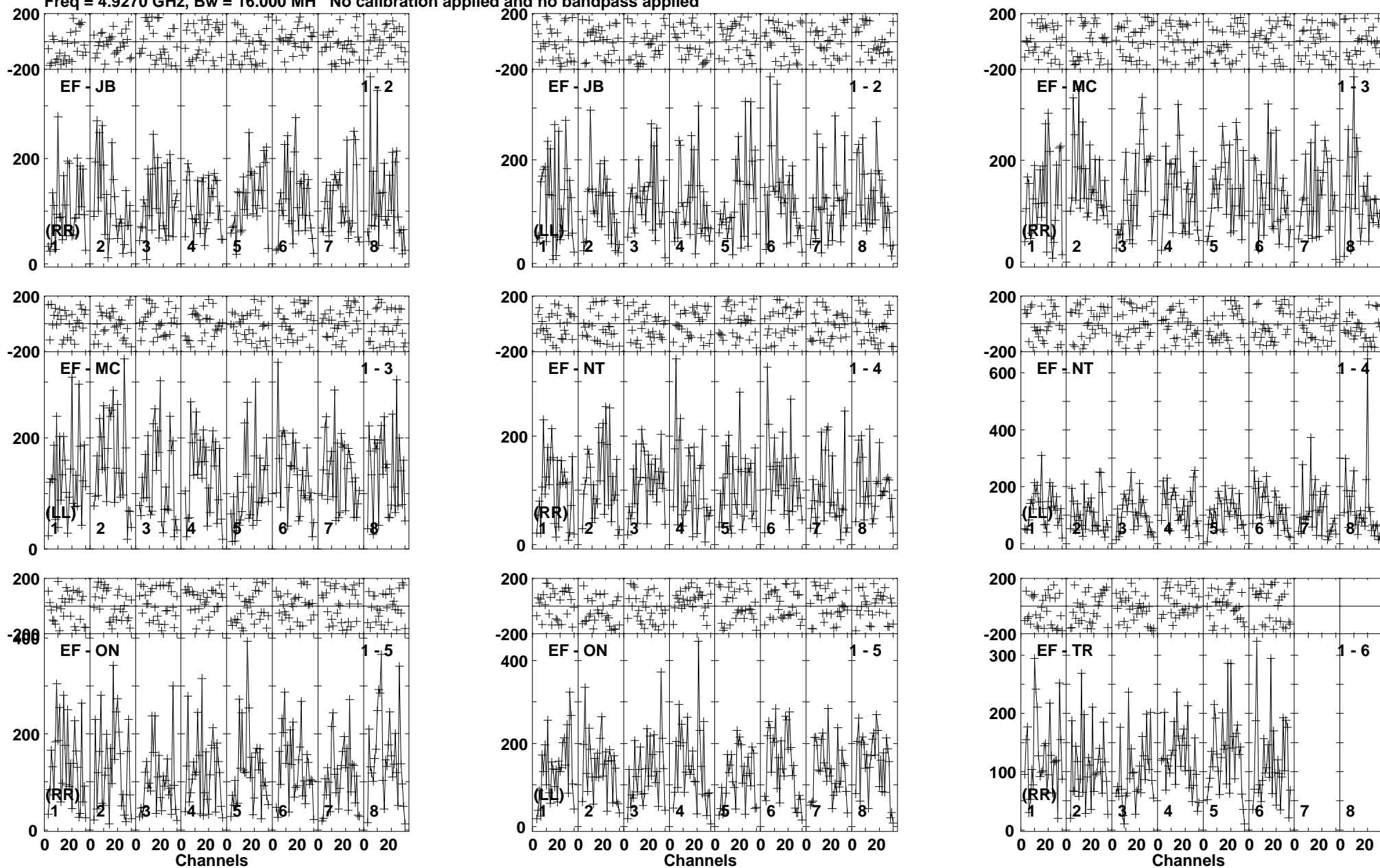
Lower frame: Micro Ampl Jy Top frame: Phas deg Vector averaged cross-power spectrum Baseline: EF (01) - JB (02) Timerange: 00/02:33:32 to 00/02:36:58
