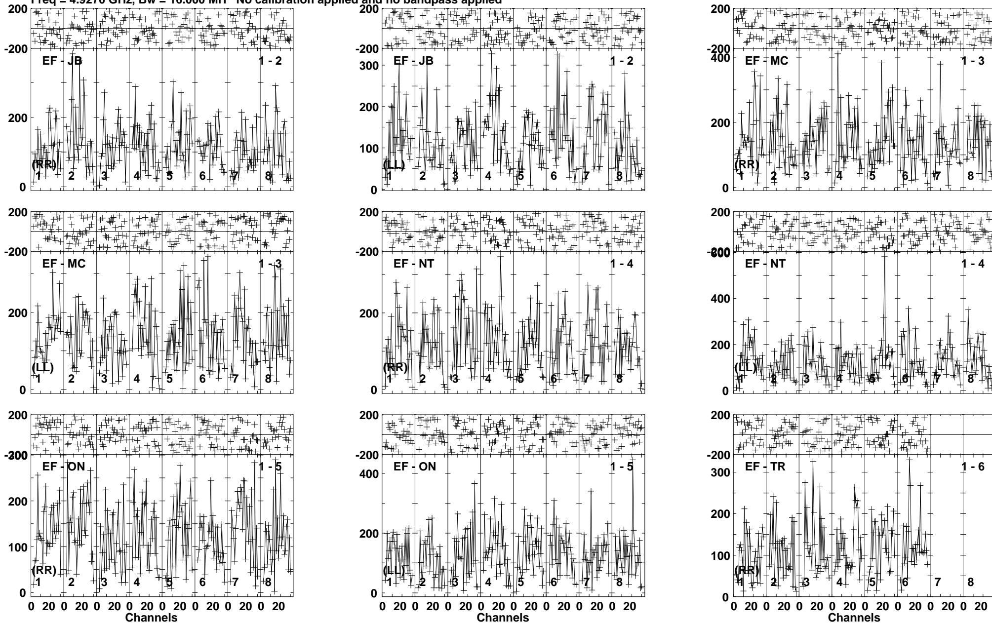
Lower frame: Micro Ampl Jy Top frame: Phas deg Vector averaged cross-power spectrum Baseline: EF (01) - JB (02) Timerange: 00/06:25:42 to 00/06:28:58
