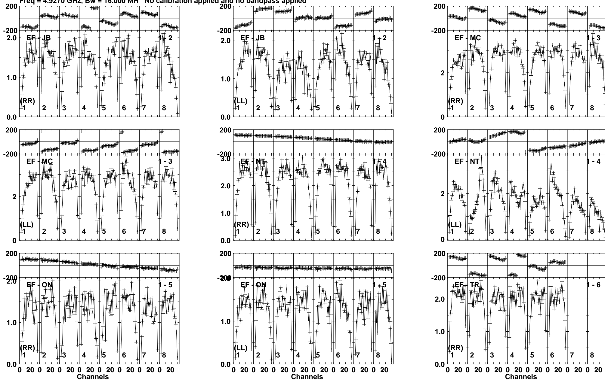
Lower frame: Milli Ampl Jy Top frame: Phas deg Vector averaged cross-power spectrum Baseline: EF (01) - JB (02) Timerange: 00/04:18:32 to 00/04:19:28
