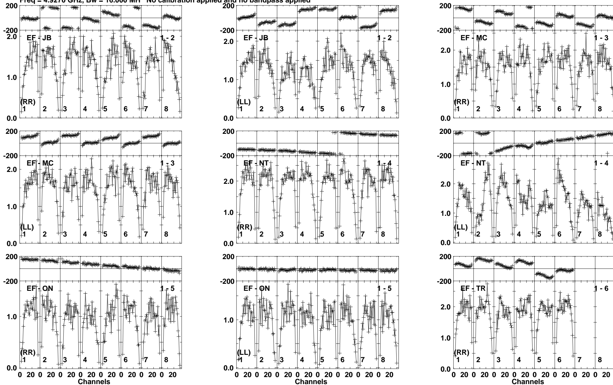
Lower frame: Milli Ampl Jy Top frame: Phas deg Vector averaged cross-power spectrum Baseline: EF (01) - JB (02) Timerange: 00/02:37:42 to 00/02:38:38
