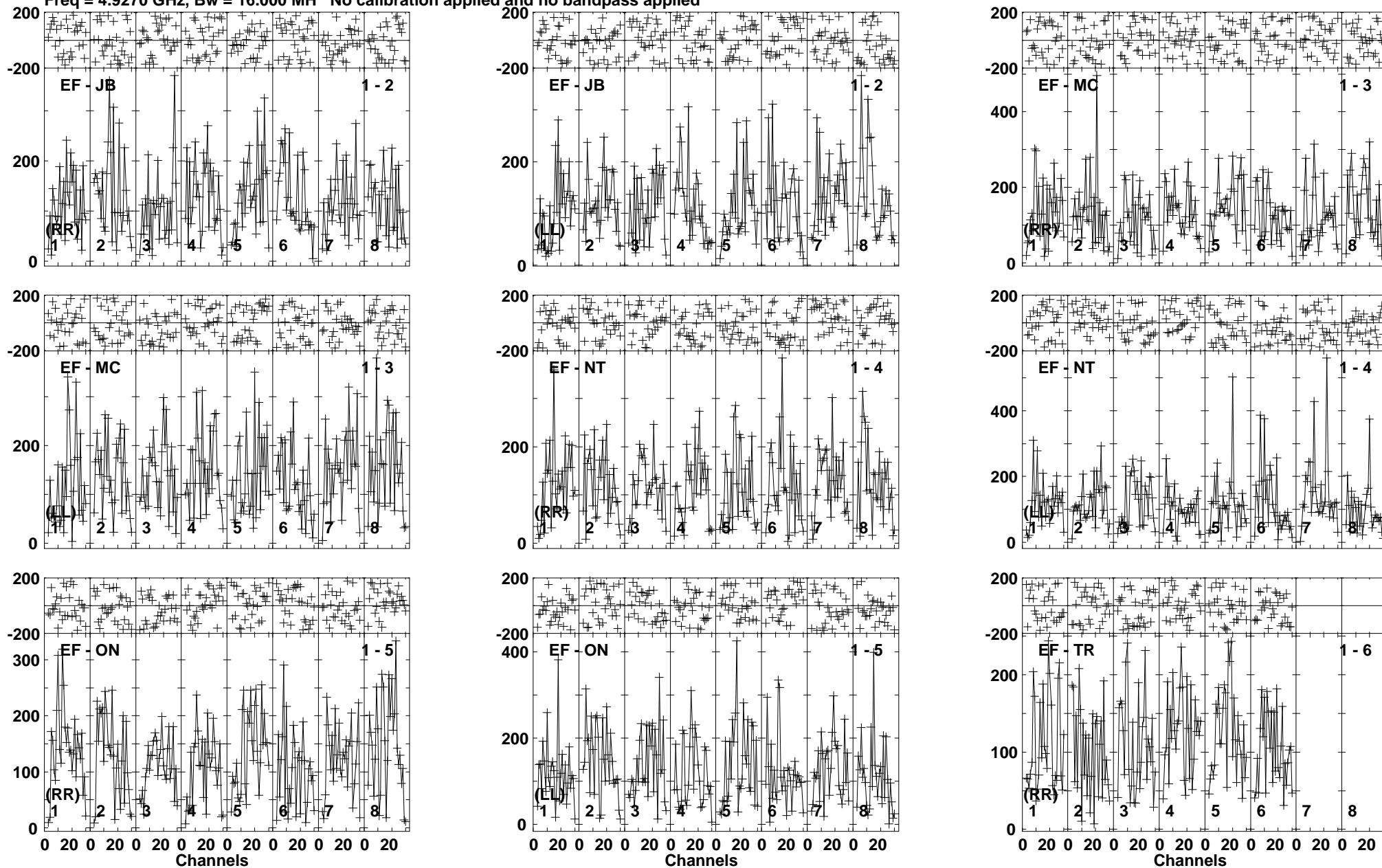
Lower frame: Micro Ampl Jy Top frame: Phas deg Vector averaged cross-power spectrum Baseline: EF (01) - JB (02) Timerange: 00/02:28:42 to 00/02:31:58
