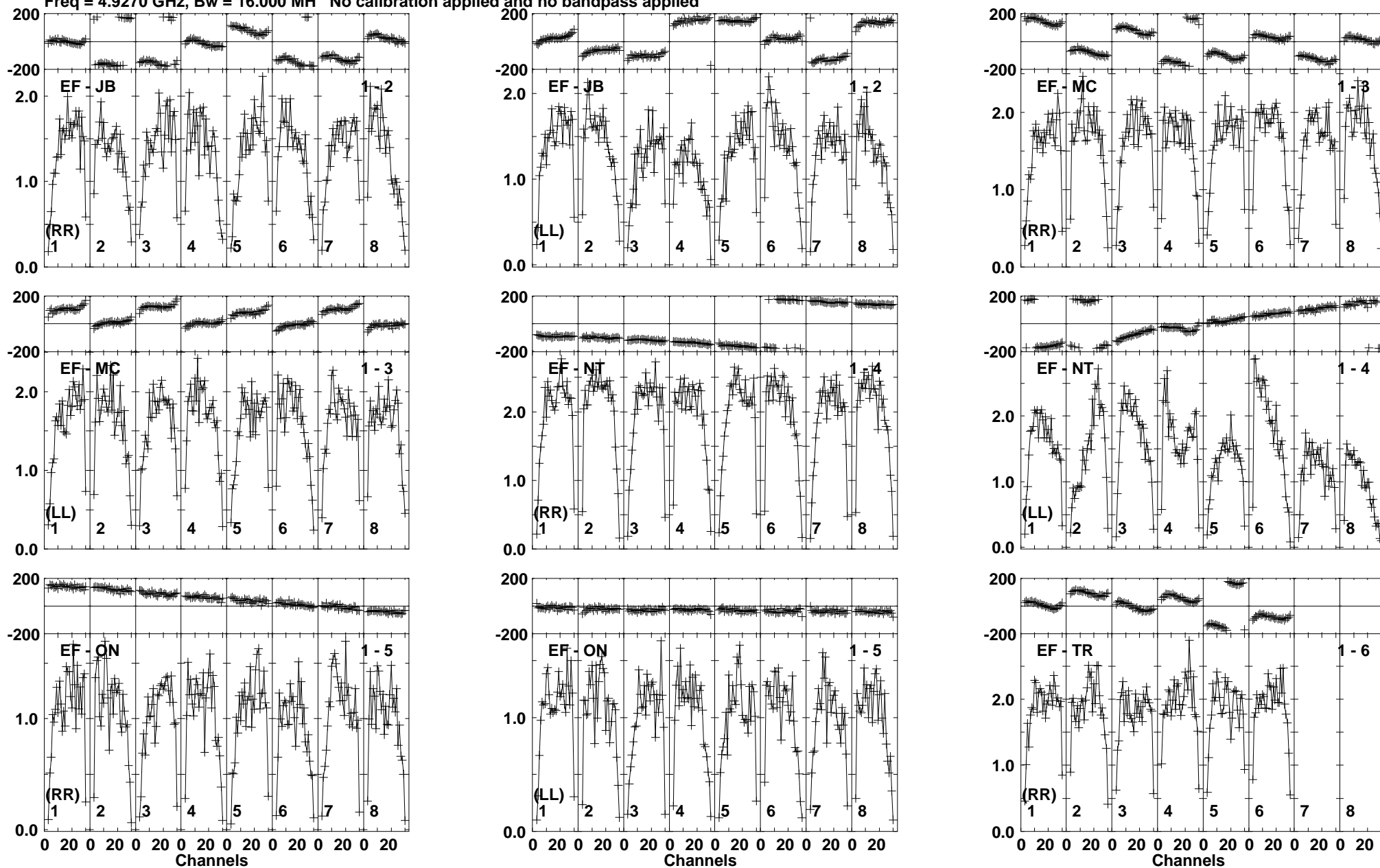
Lower frame: Milli Ampl Jy Top frame: Phas deg Vector averaged cross-power spectrum Baseline: EF (01) - JB (02) Timerange: 00/02:40:12 to 00/02:41:38
