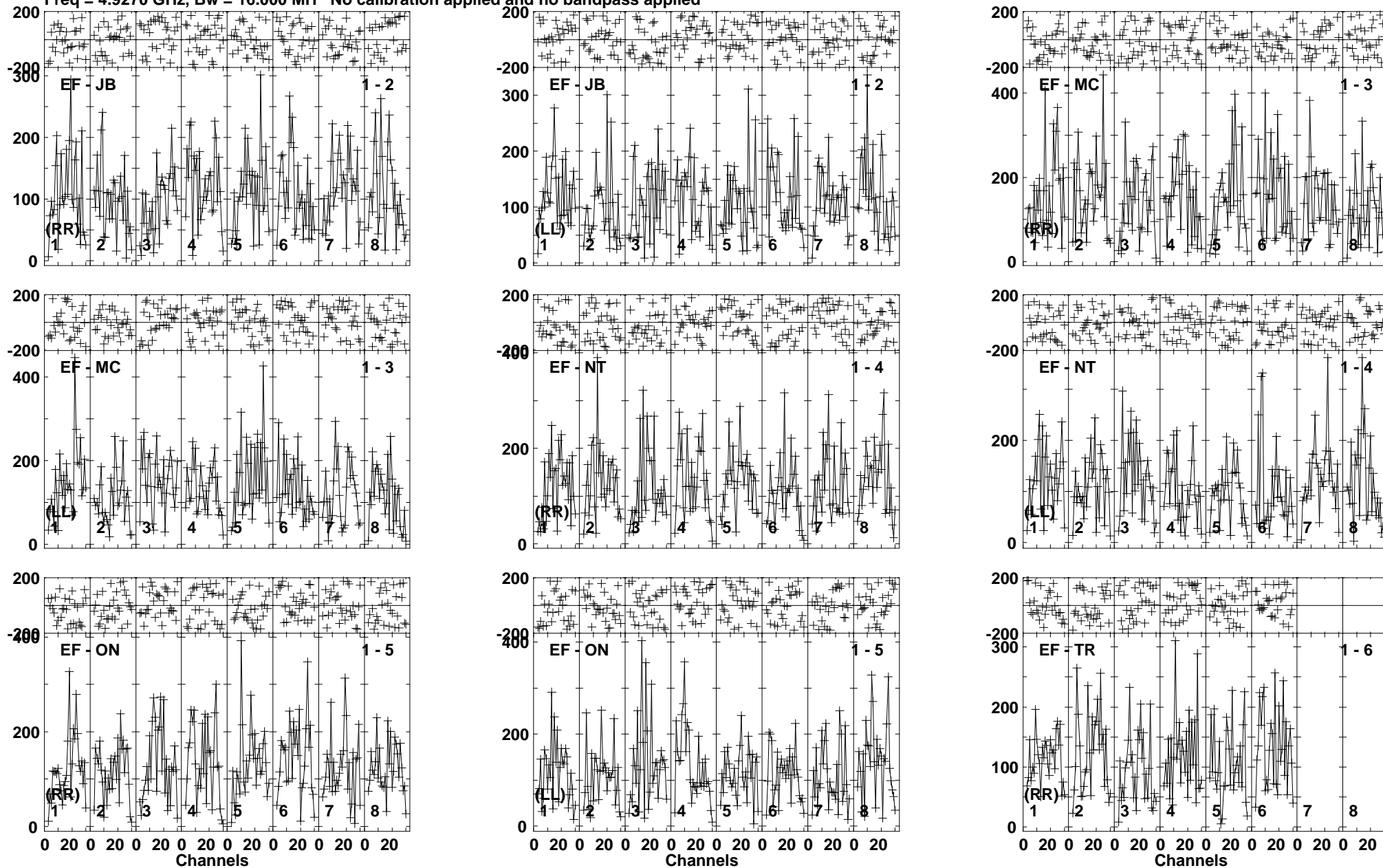
Lower frame: Micro Ampl Jy Top frame: Phas deg Vector averaged cross-power spectrum Baseline: EF (01) - JB (02) Timerange: 00/07:09:02 to 00/07:12:28
