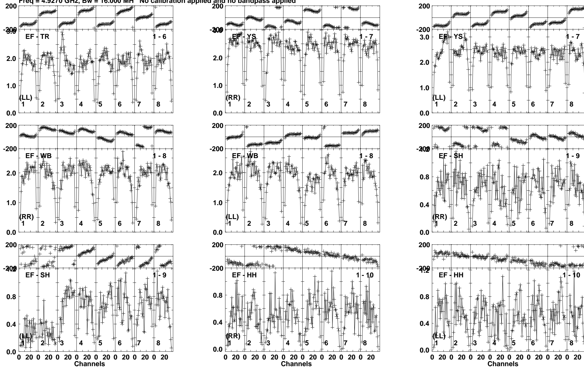
Lower frame: Milli Ampl Jy Top frame: Phas deg Vector averaged cross-power spectrum Baseline: EF (01) - TR (06) Timerange: 00/04:08:42 to 00/04:10:08
