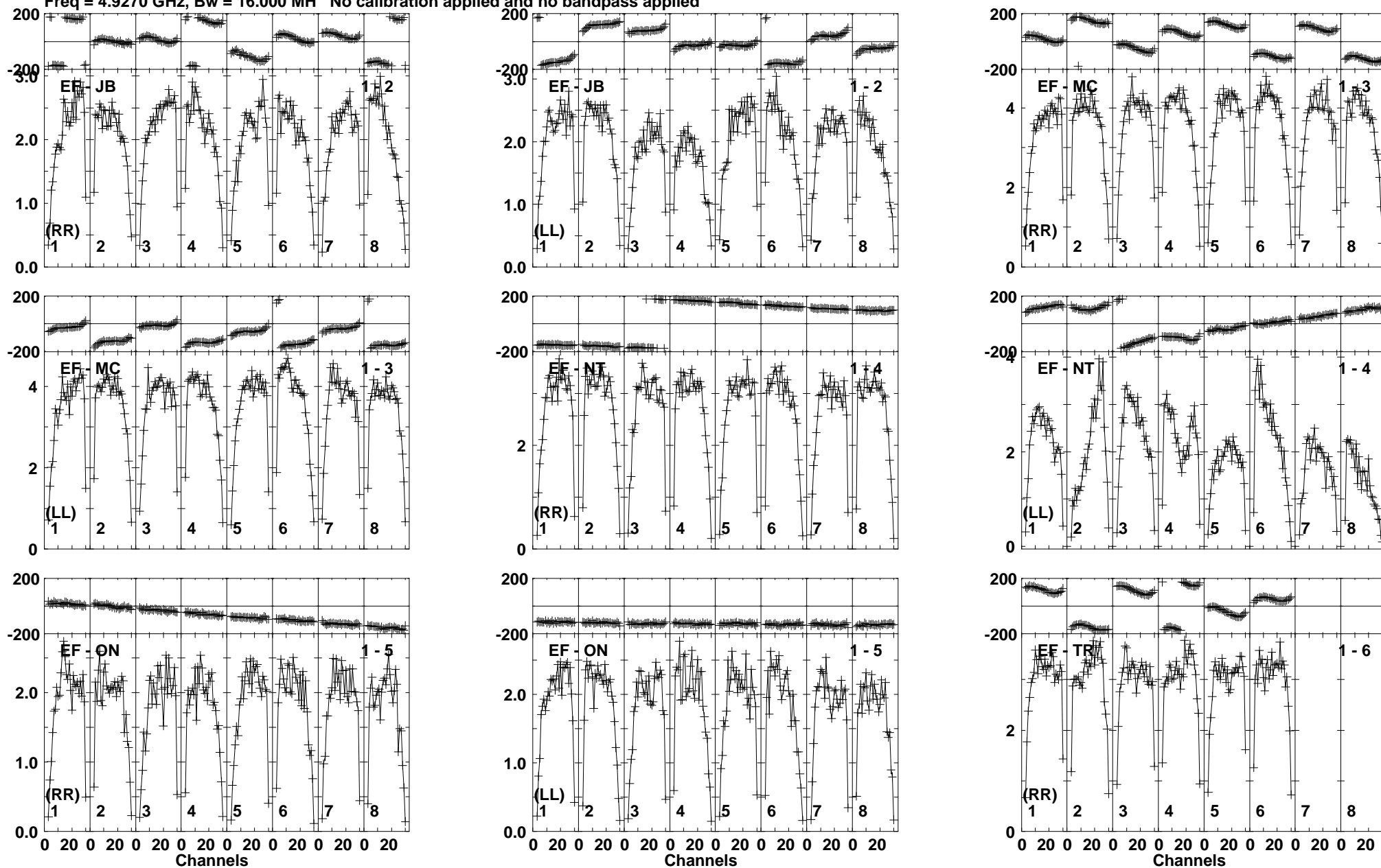
Lower frame: Milli Ampl Jy Top frame: Phas deg Vector averaged cross-power spectrum Baseline: EF (01) - JB (02) Timerange: 00/04:22:32 to 00/04:23:58
