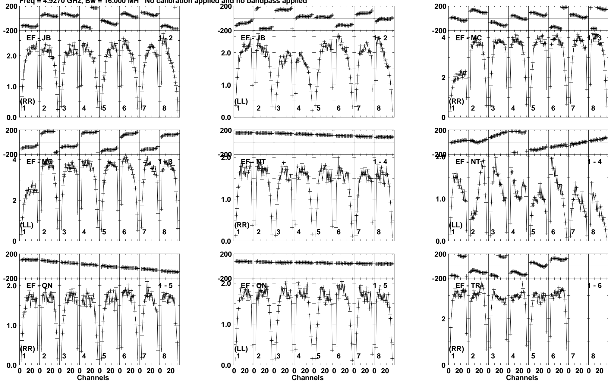
Lower frame: Milli Ampl Jy Top frame: Phas deg Vector averaged cross-power spectrum Baseline: EF (01) - JB (02) Timerange: 00/07:55:12 to 00/07:58:08
