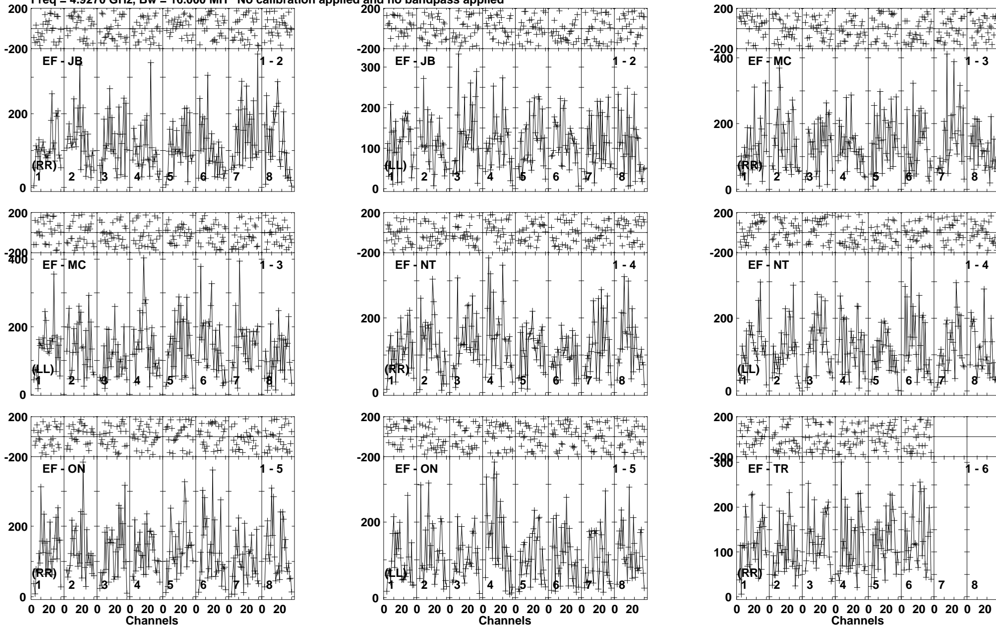
Lower frame: Micro Ampl Jy Top frame: Phas deg Vector averaged cross-power spectrum Baseline: EF (01) - JB (02) Timerange: 00/06:30:32 to 00/06:33:58
