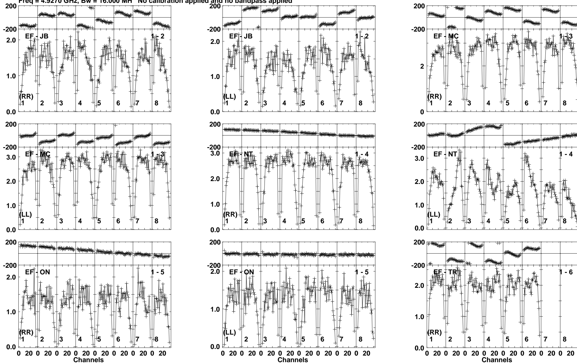
Lower frame: Milli Ampl Jy Top frame: Phas deg Vector averaged cross-power spectrum Baseline: EF (01) - JB (02) Timerange: 00/04:14:52 to 00/04:16:18
