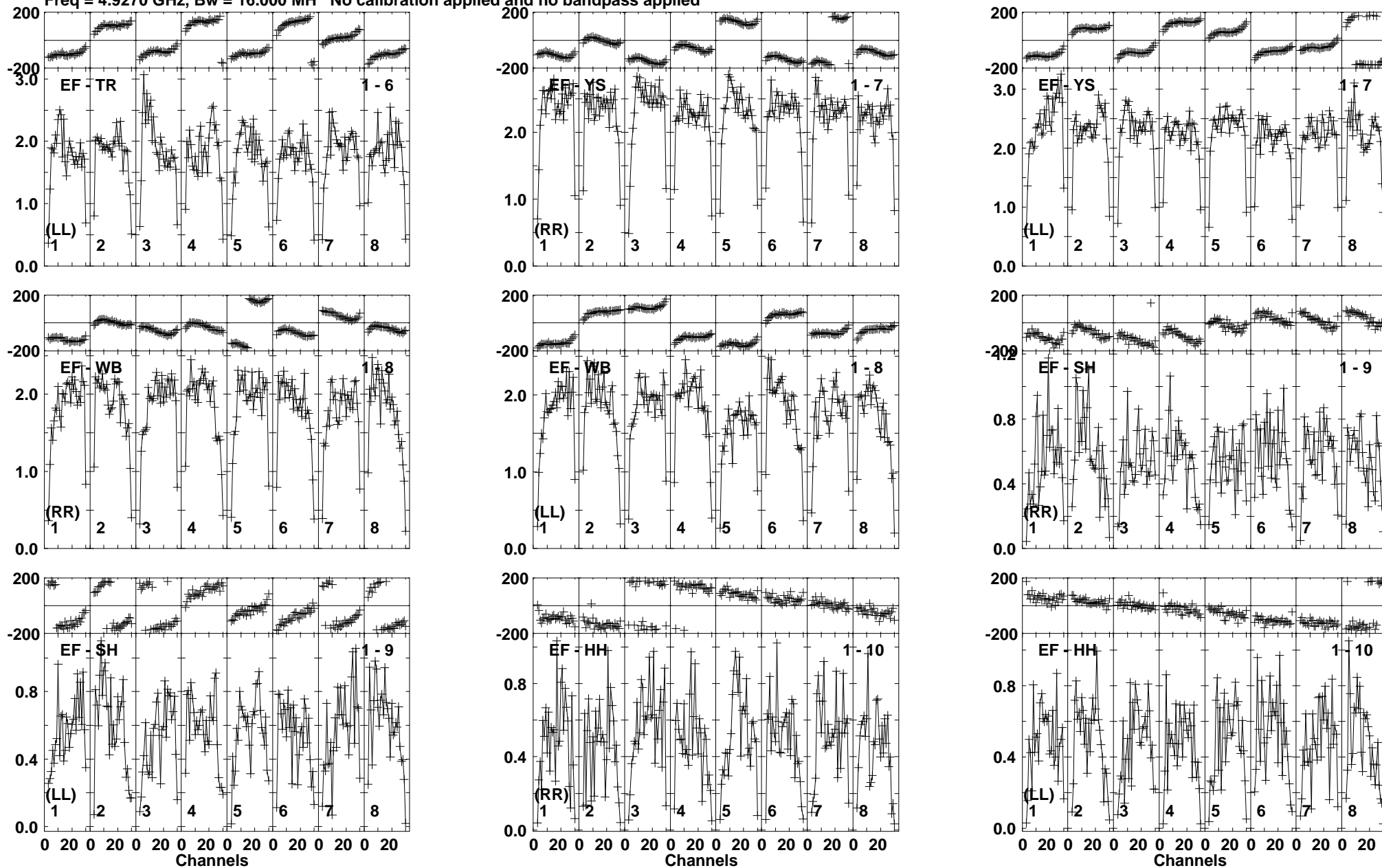
Lower frame: Milli Ampl Jy Top frame: Phas deg Vector averaged cross-power spectrum Baseline: EF (01) - TR (06) Timerange: 00/03:26:12 to 00/03:27:08
