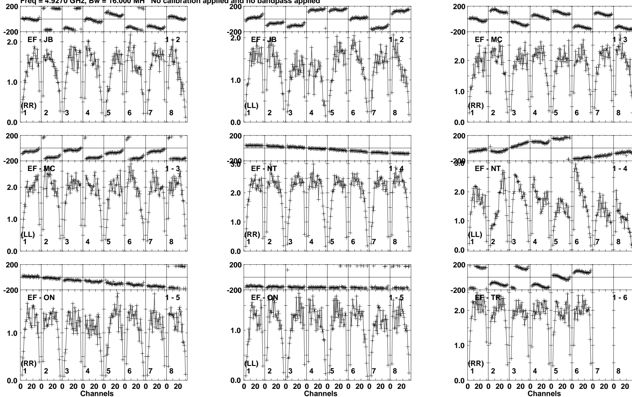
Lower frame: Milli Ampl Jy Top frame: Phas deg Vector averaged cross-power spectrum Baseline: EF (01) - JB (02) Timerange: 00/02:56:12 to 00/02:57:08
