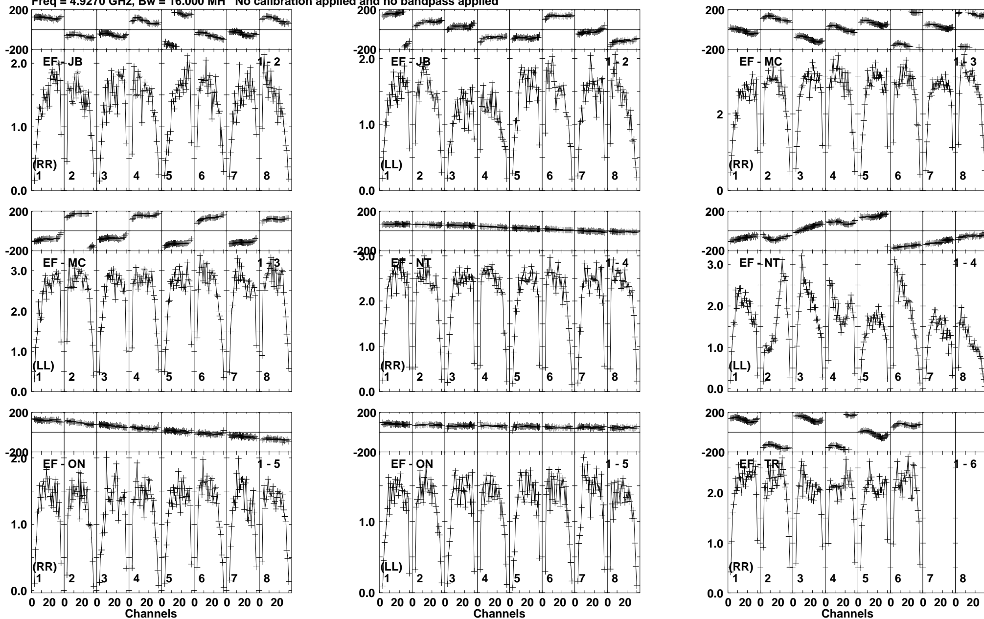
Lower frame: Milli Ampl Jy Top frame: Phas deg Vector averaged cross-power spectrum Baseline: EF (01) - JB (02) Timerange: 00/07:47:32 to 00/07:48:58
