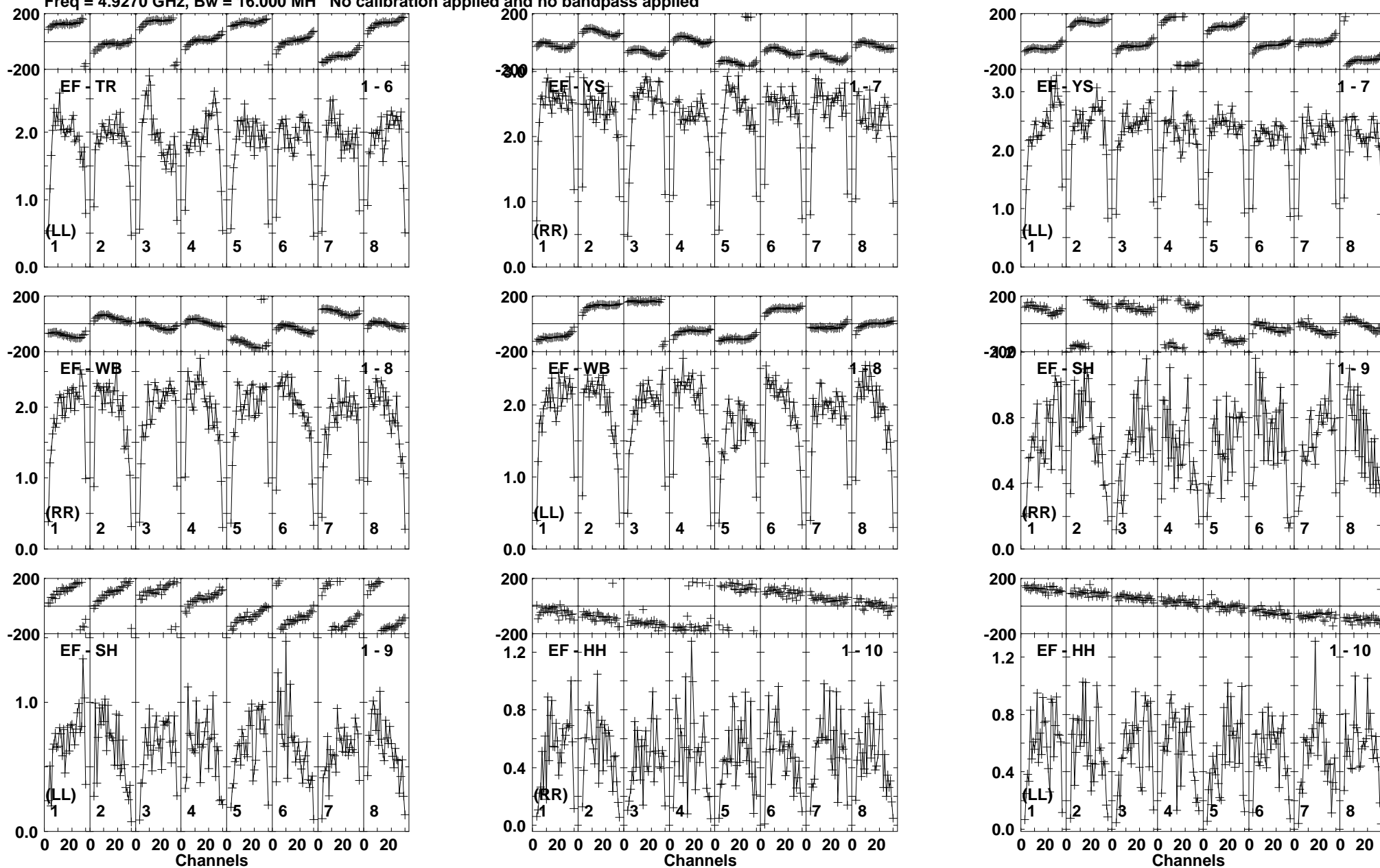
Lower frame: Milli Ampl Jy Top frame: Phas deg Vector averaged cross-power spectrum Baseline: EF (01) - TR (06) Timerange: 00/04:21:02 to 00/04:22:28
