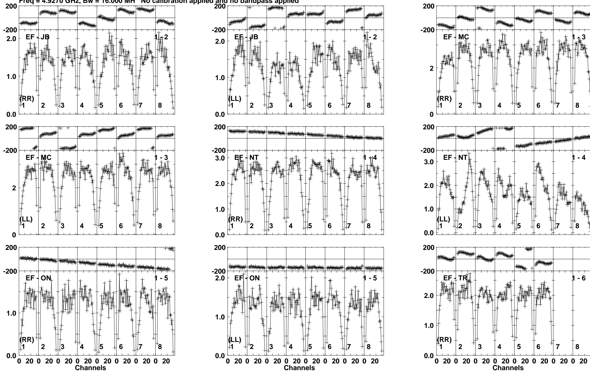
Lower frame: Milli Ampl Jy Top frame: Phas deg Vector averaged cross-power spectrum Baseline: EF (01) - JB (02) Timerange: 00/03:56:12 to 00/03:57:08
