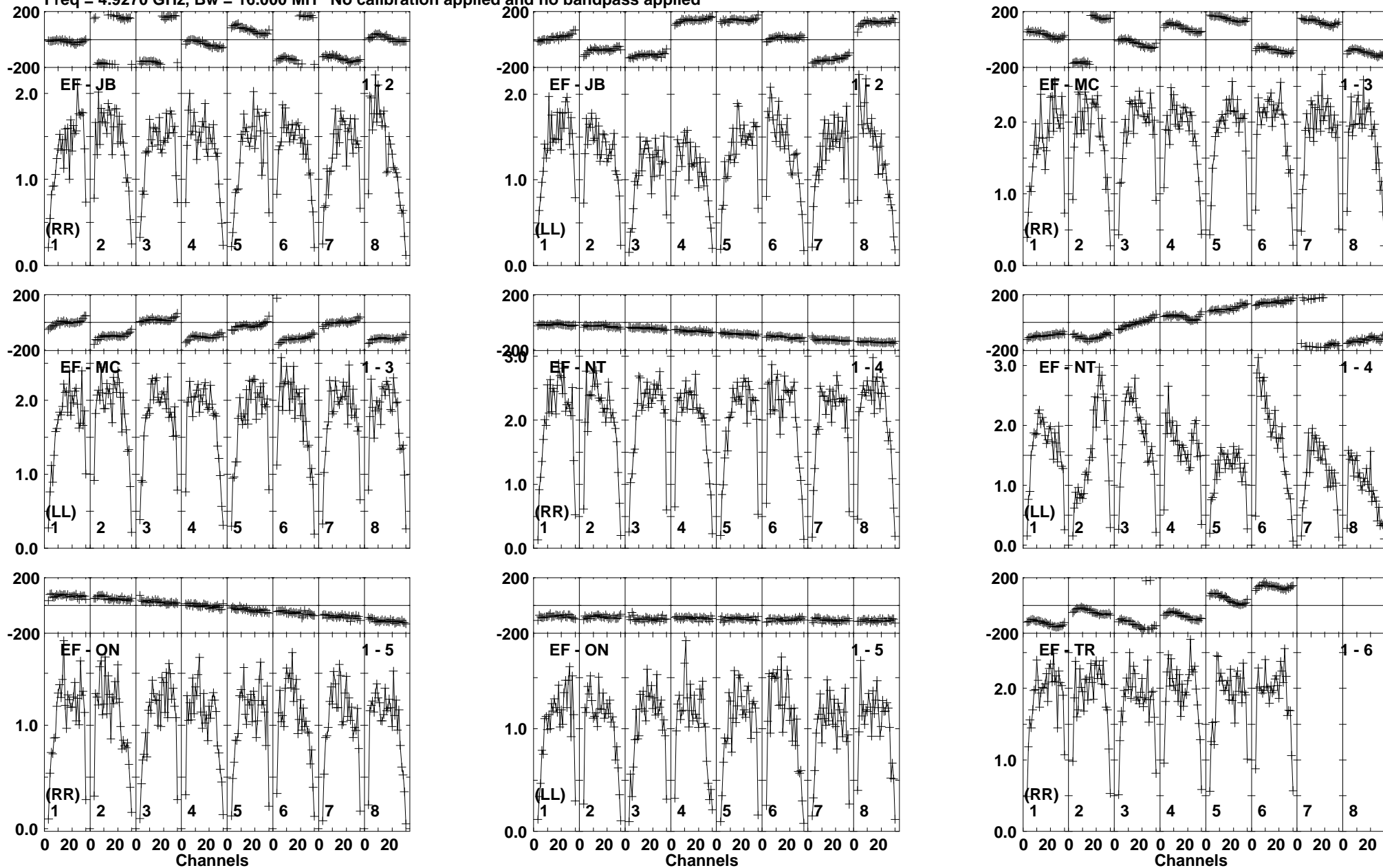
Lower frame: Milli Ampl Jy Top frame: Phas deg Vector averaged cross-power spectrum Baseline: EF (01) - JB (02) Timerange: 00/02:50:02 to 00/02:50:58
