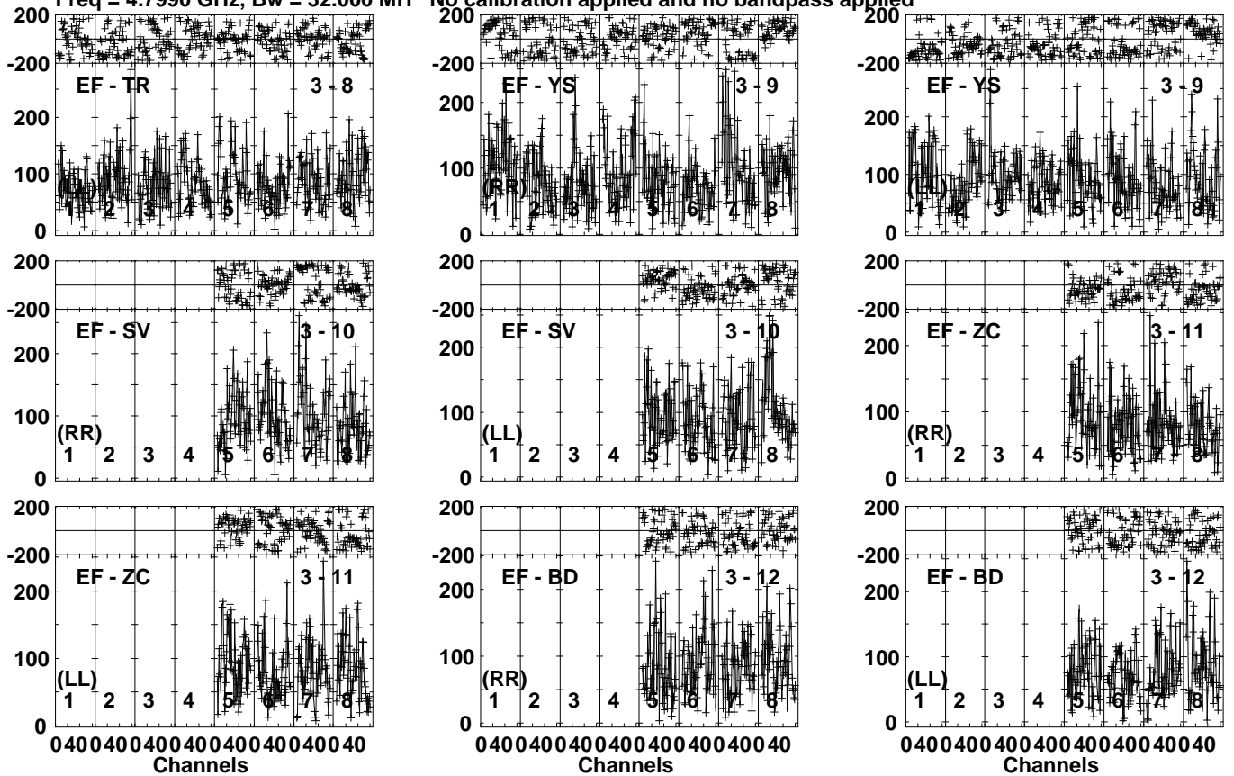
Lower frame: Micro Ampl Jy Top frame: Phas deg Vector averaged cross-power spectrum Several baselines displayed Timerange: 00/17:47:51 to 00/17:51:19
