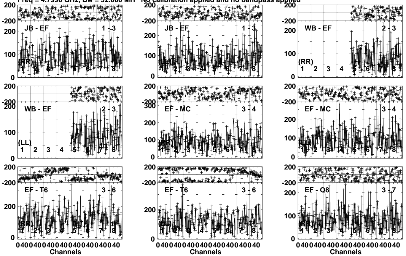
Lower frame: Micro Ampl Jy Top frame: Phas deg Vector averaged cross-power spectrum Several baselines displayed Timerange: 00/21:57:21 to 00/22:00:49
