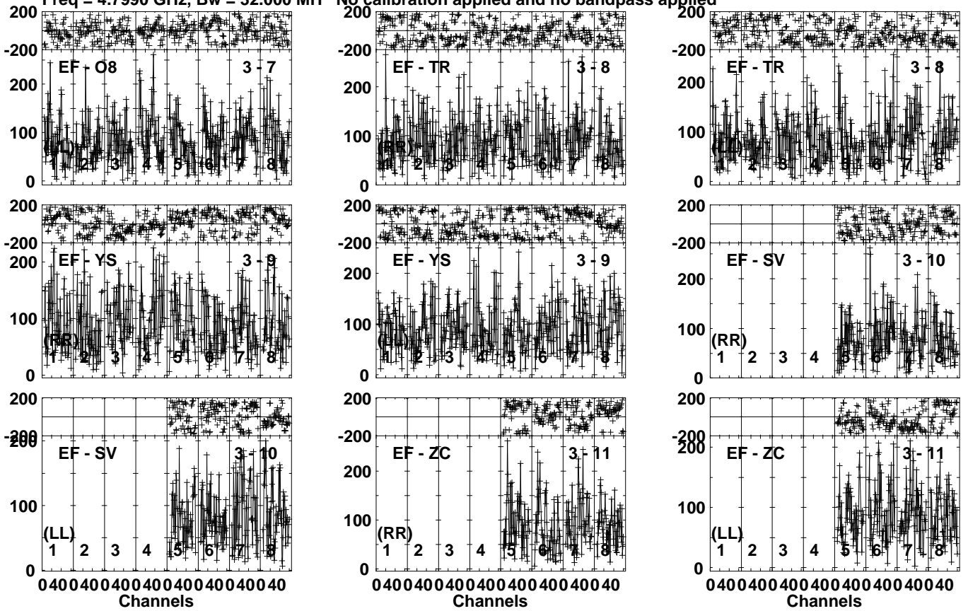
Lower frame: Micro Ampl Jy Top frame: Phas deg Vector averaged cross-power spectrum Several baselines displayed Timerange: 00/22:30:21 to 00/22:33:49
