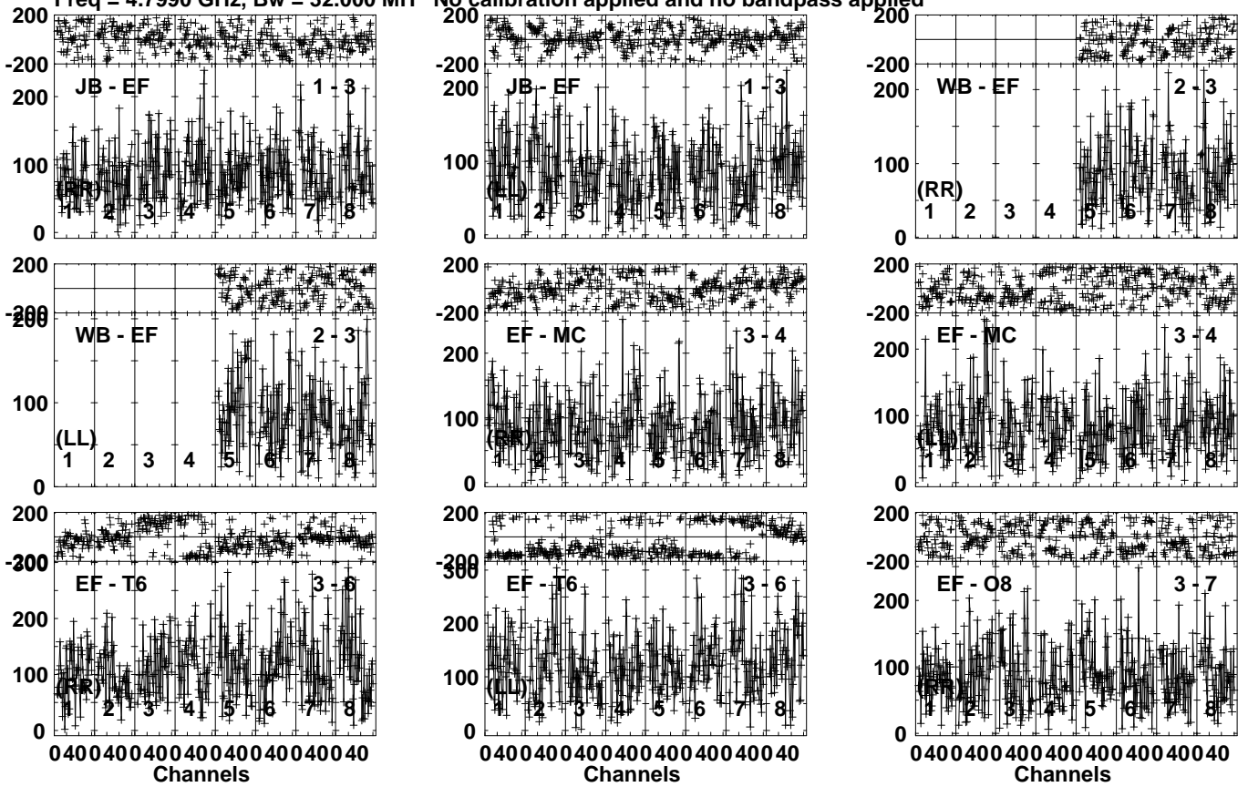
Lower frame: Micro Ampl Jy Top frame: Phas deg Vector averaged cross-power spectrum Several baselines displayed Timerange: 00/21:29:51 to 00/21:33:19
