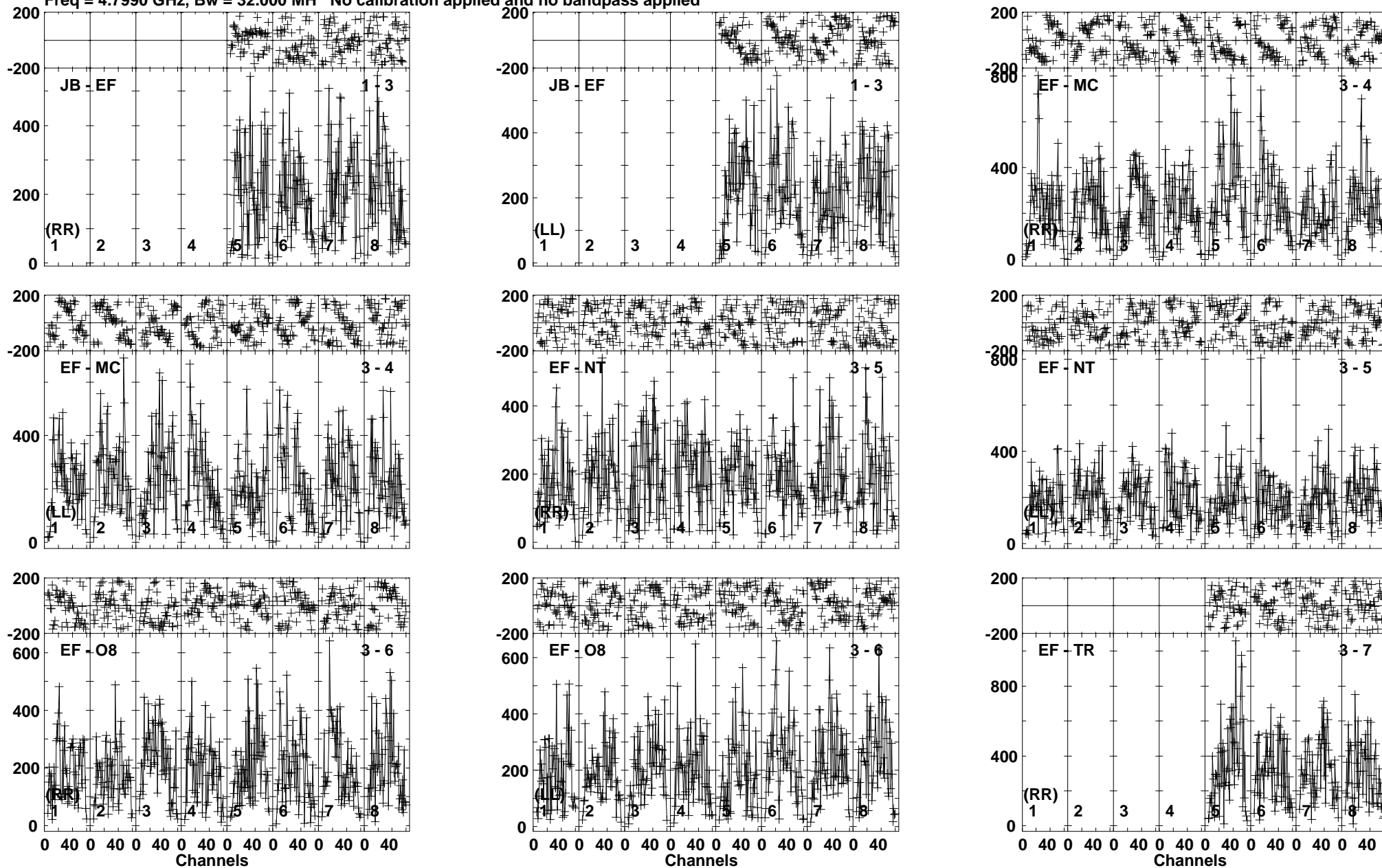
Lower frame: Micro Ampl Jy Top frame: Phas deg Vector averaged cross-power spectrum Baseline: JB (01) - EF (03) Timerange: 00/15:49:01 to 00/15:49:59
