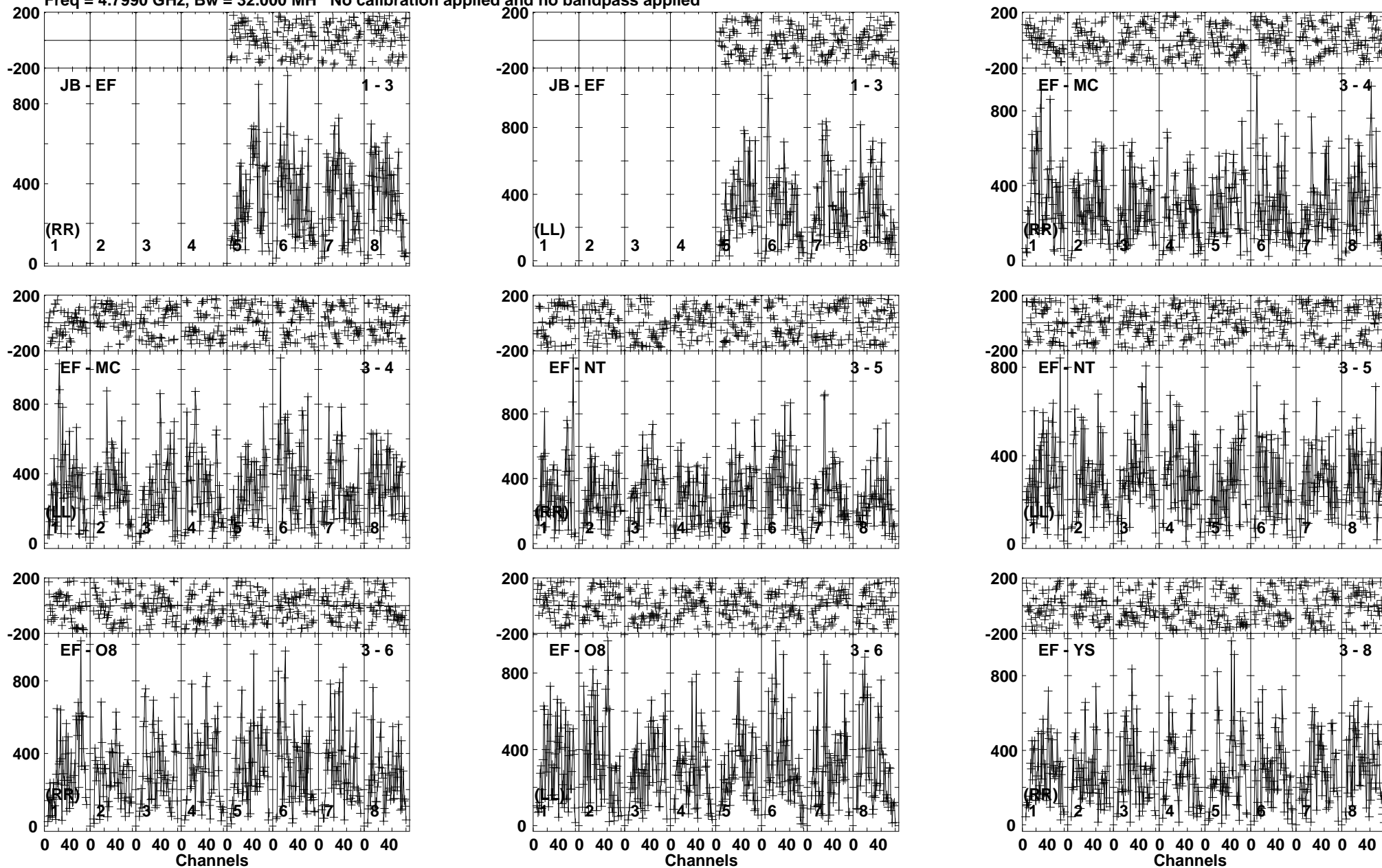
Lower frame: Micro Ampl Jy Top frame: Phas deg Vector averaged cross-power spectrum Baseline: JB (01) - EF (03) Timerange: 00/15:51:31 to 00/15:52:29
