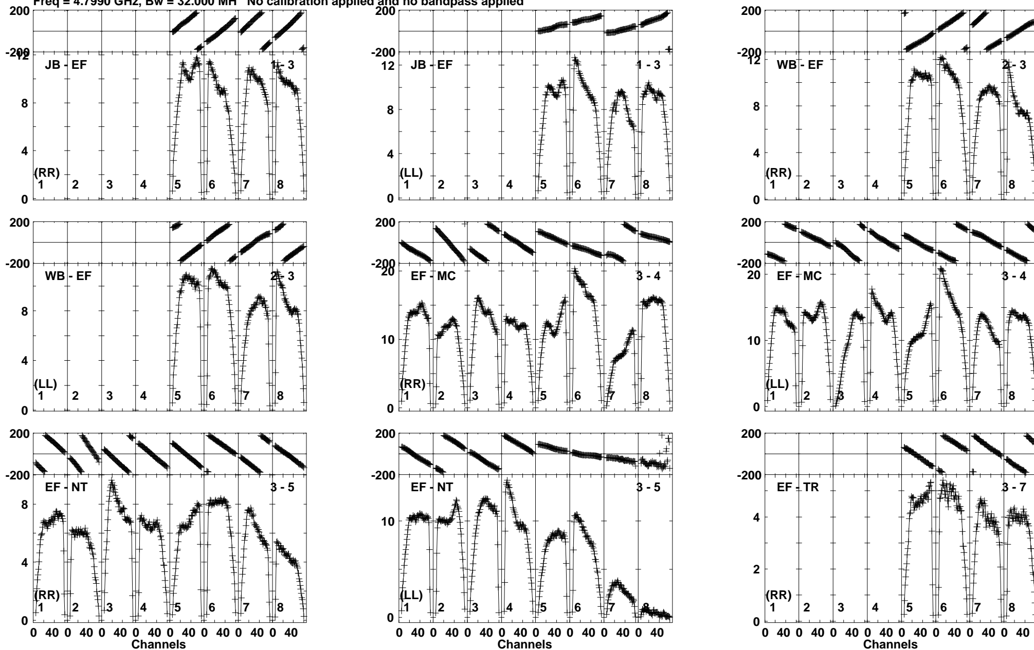
Lower frame: Milli Ampl Jy Top frame: Phas deg Vector averaged cross-power spectrum Baseline: JB (01) - EF (03) Timerange: 00/16:11:31 to 00/16:12:29
