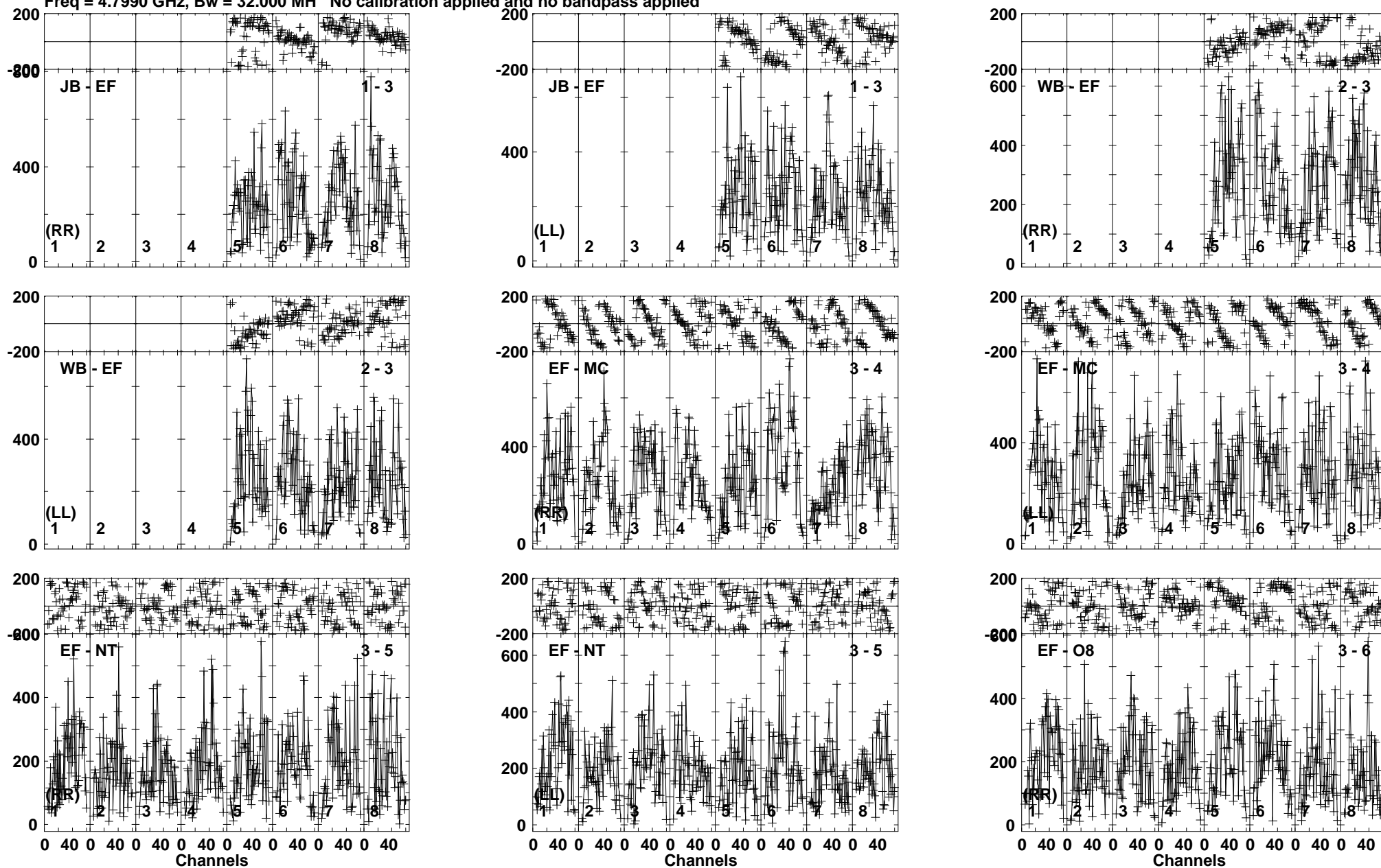
Lower frame: Micro Ampl Jy Top frame: Phas deg Vector averaged cross-power spectrum Baseline: JB (01) - EF (03) Timerange: 00/16:55:31 to 00/16:56:29
