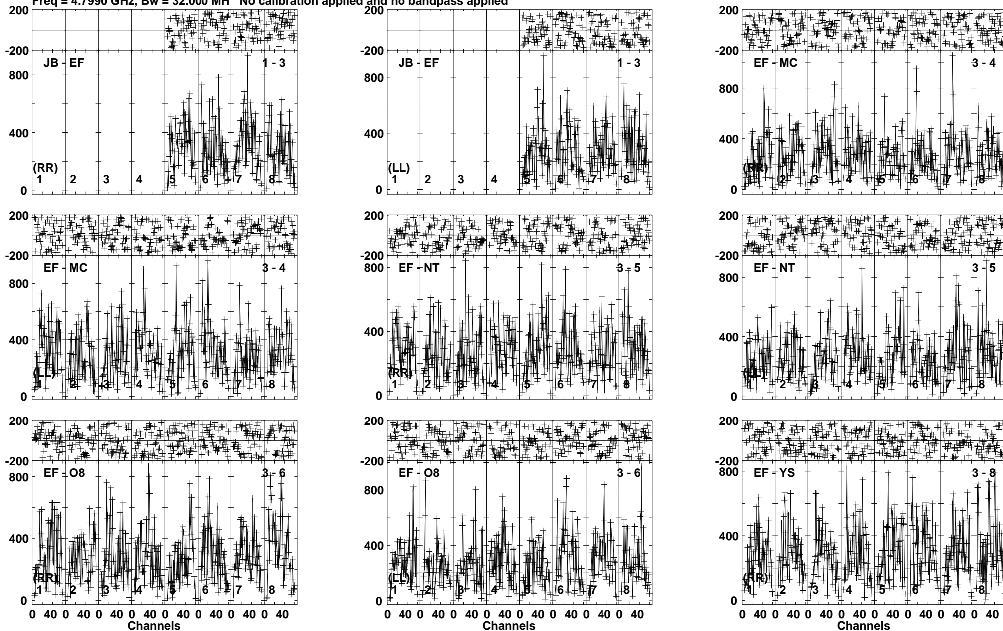
Lower frame: Micro Ampl Jy Top frame: Phas deg Vector averaged cross-power spectrum Baseline: JB (01) - EF (03) Timerange: 00/15:41:01 to 00/15:41:59
