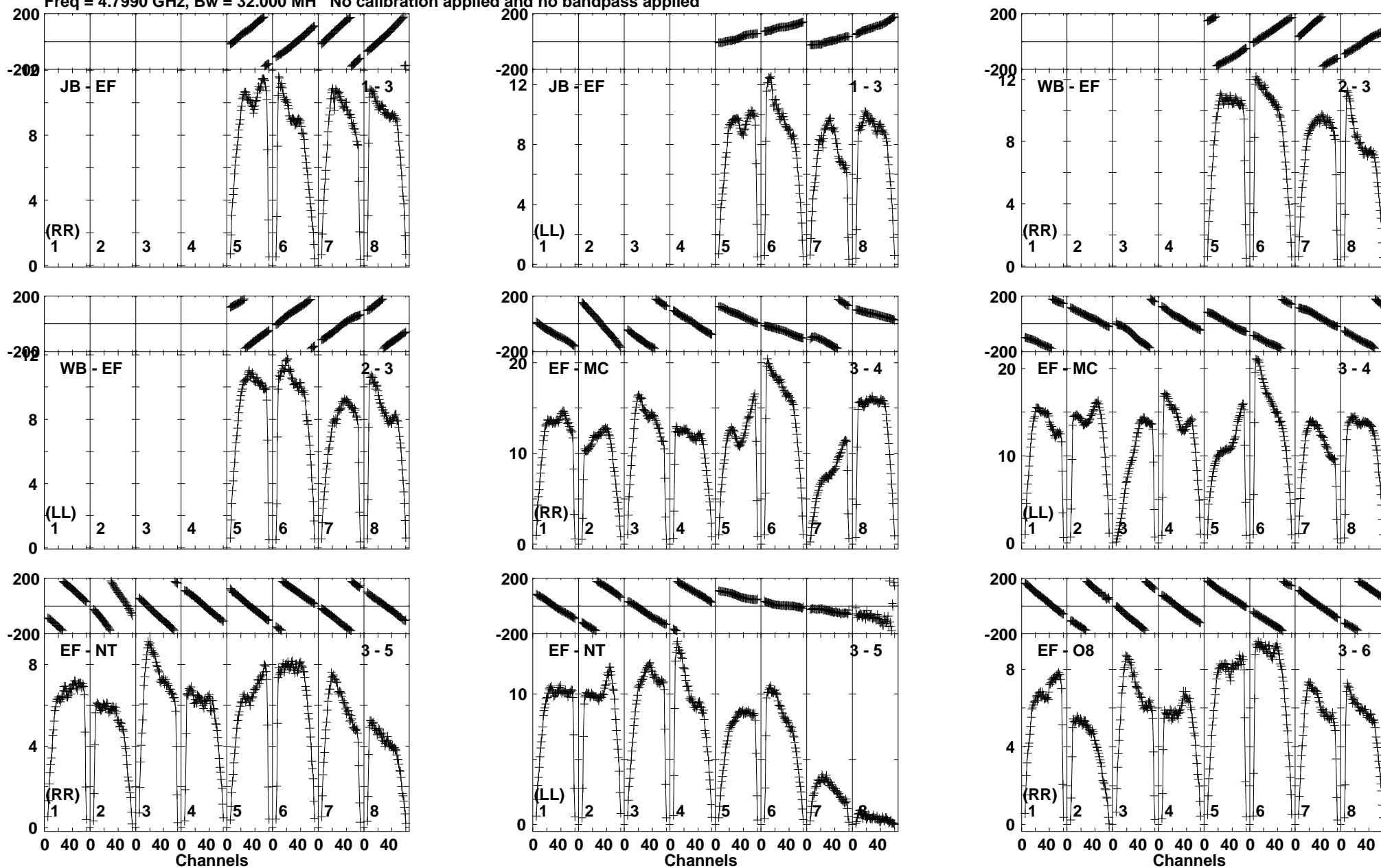
Lower frame: Milli Ampl Jy Top frame: Phas deg Vector averaged cross-power spectrum Baseline: JB (01) - EF (03) Timerange: 00/16:08:01 to 00/16:08:59
