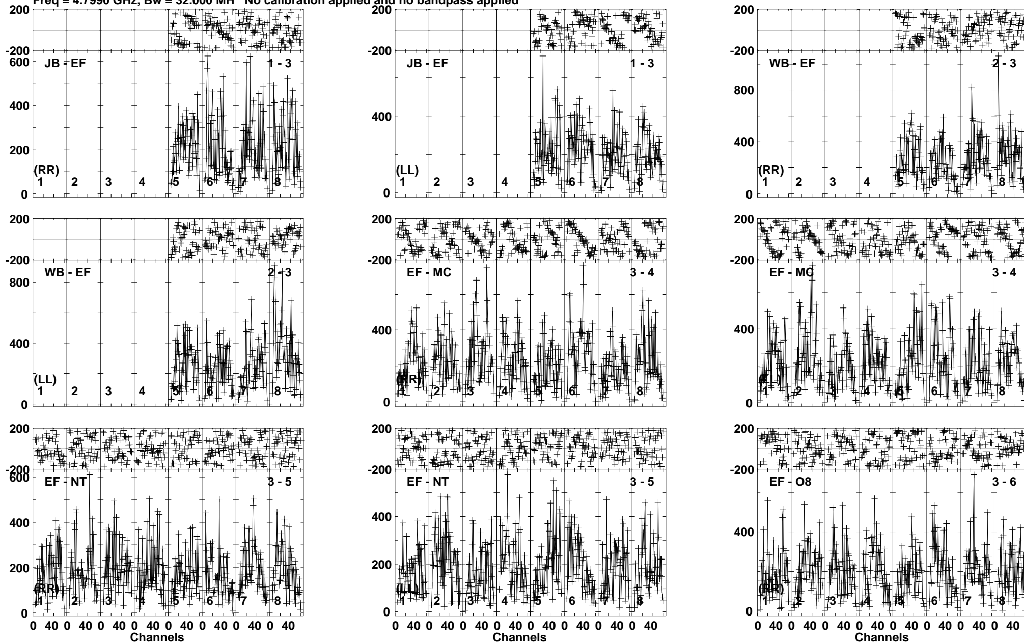
Lower frame: Micro Ampl Jy Top frame: Phas deg Vector averaged cross-power spectrum Baseline: JB (01) - EF (03) Timerange: 00/16:38:01 to 00/16:38:59
