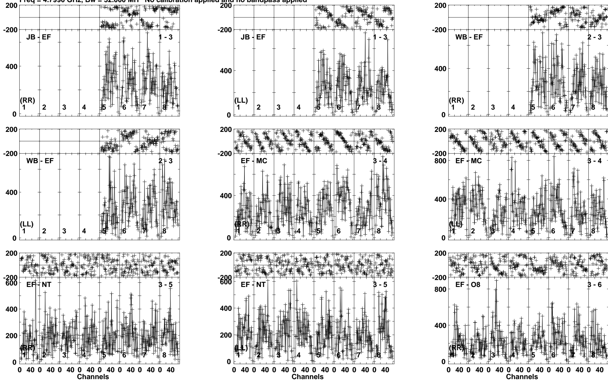
Lower frame: Micro Ampl Jy Top frame: Phas deg Vector averaged cross-power spectrum Baseline: JB (01) - EF (03) Timerange: 00/16:27:31 to 00/16:28:29
