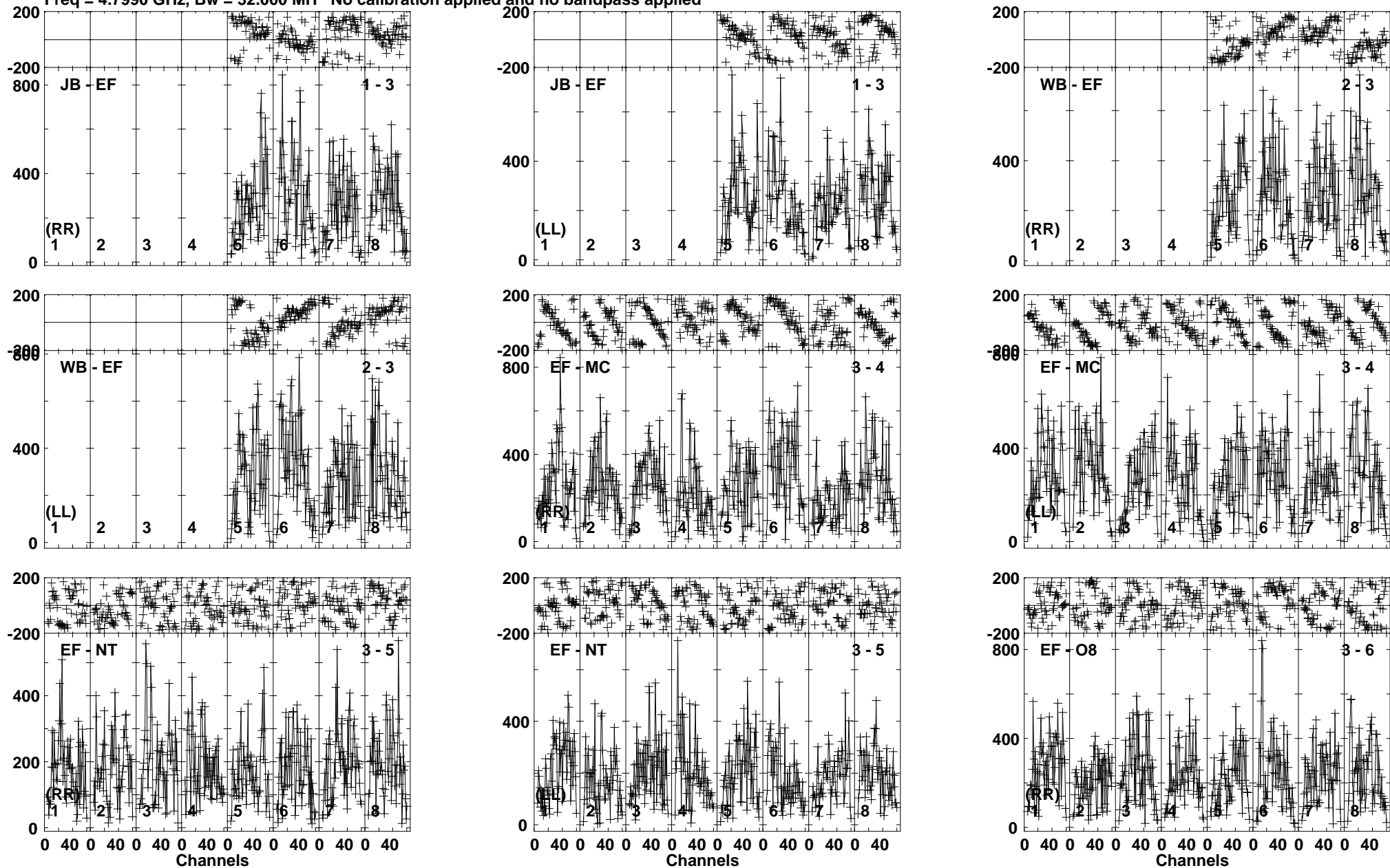
Lower frame: Micro Ampl Jy Top frame: Phas deg Vector averaged cross-power spectrum Baseline: JB (01) - EF (03) Timerange: 00/16:13:31 to 00/16:14:29
