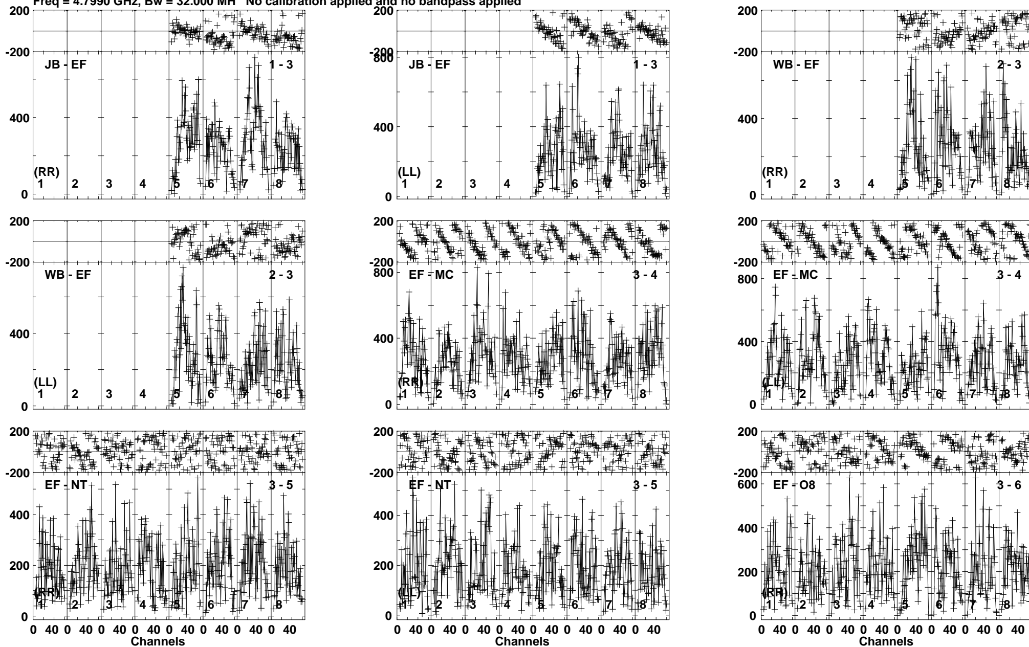
Lower frame: Micro Ampl Jy Top frame: Phas deg Vector averaged cross-power spectrum Baseline: JB (01) - EF (03) Timerange: 00/16:41:31 to 00/16:42:29
