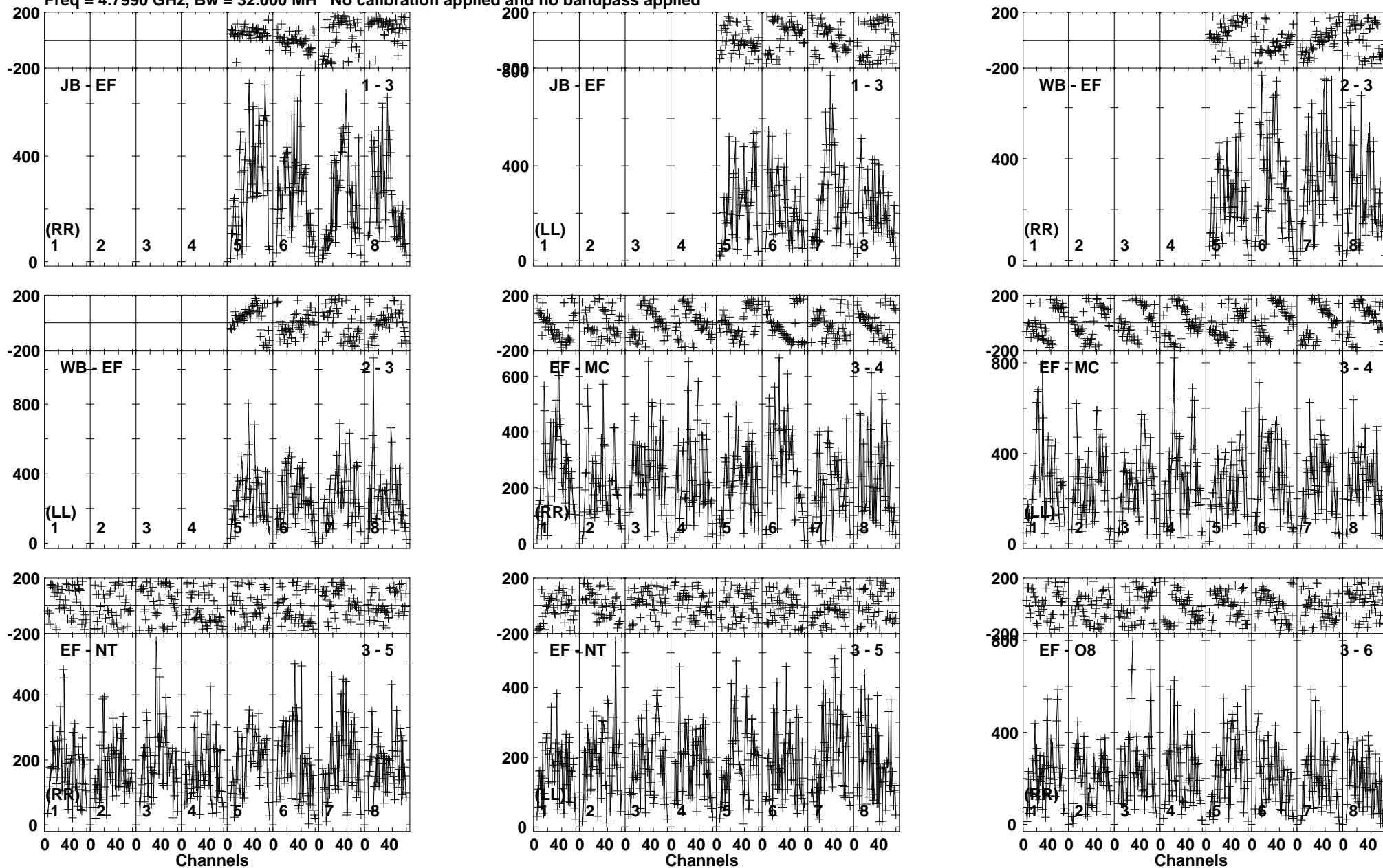
Lower frame: Micro Ampl Jy Top frame: Phas deg Vector averaged cross-power spectrum Baseline: JB (01) - EF (03) Timerange: 00/15:31:31 to 00/15:32:29
