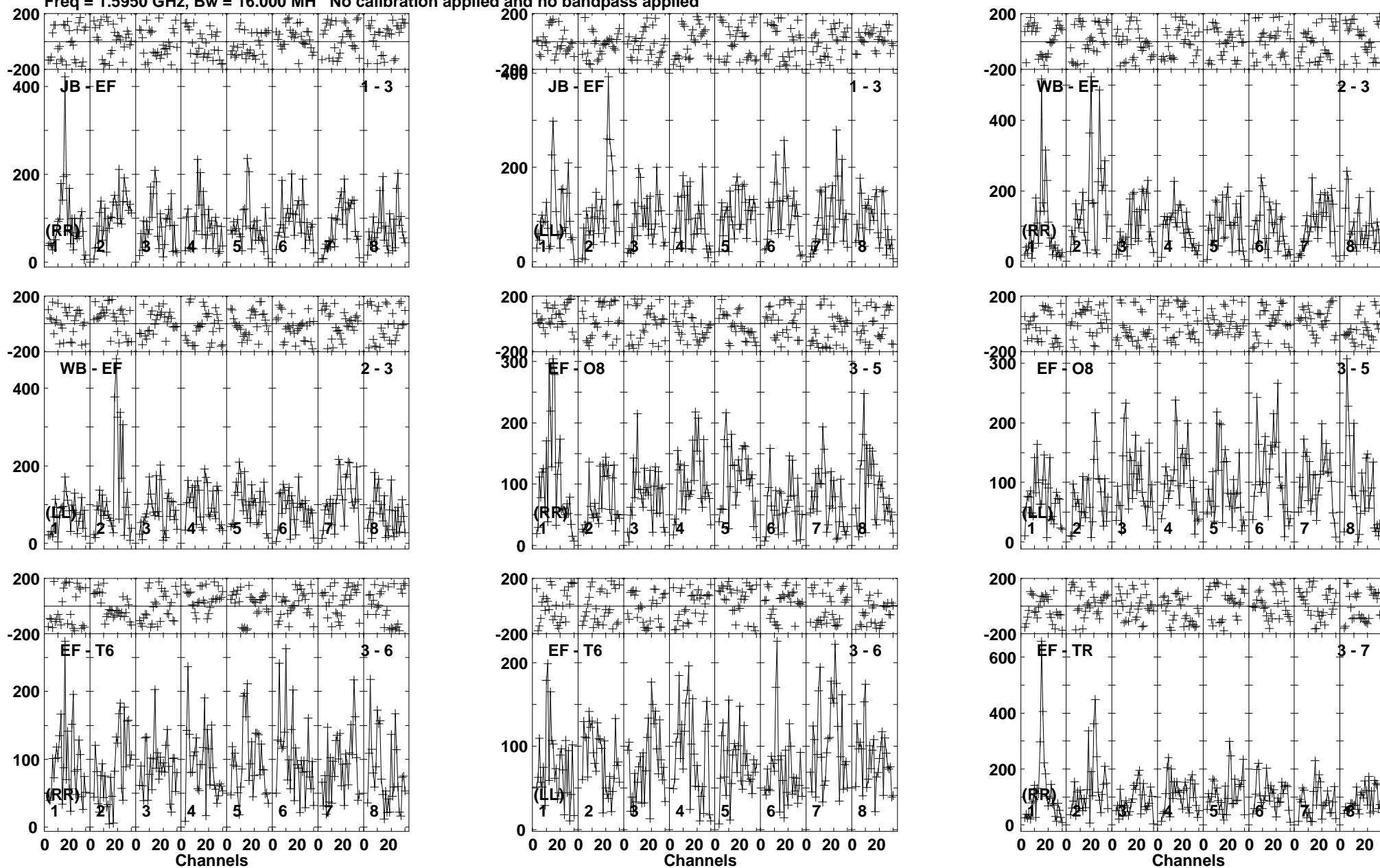
Lower frame: Micro Ampl Jy Top frame: Phas deg Vector averaged cross-power spectrum Baseline: JB (01) - EF (03) Timerange: 00/11:48:11 to 00/11:51:39
