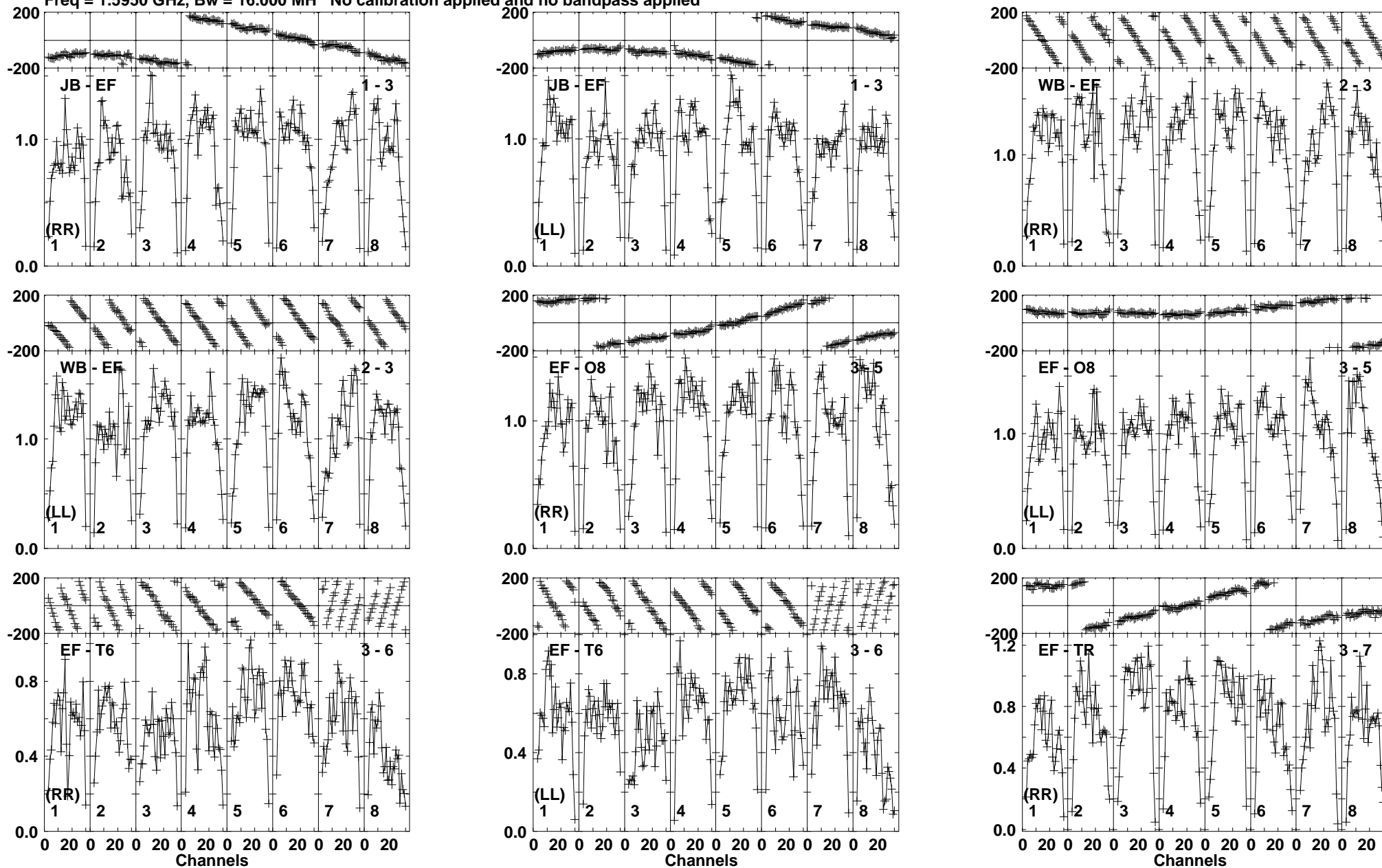
Lower frame: Milli Ampl Jy Top frame: Phas deg Vector averaged cross-power spectrum Baseline: JB (01) - EF (03) Timerange: 00:12:58:31 to 00:12:59:59
