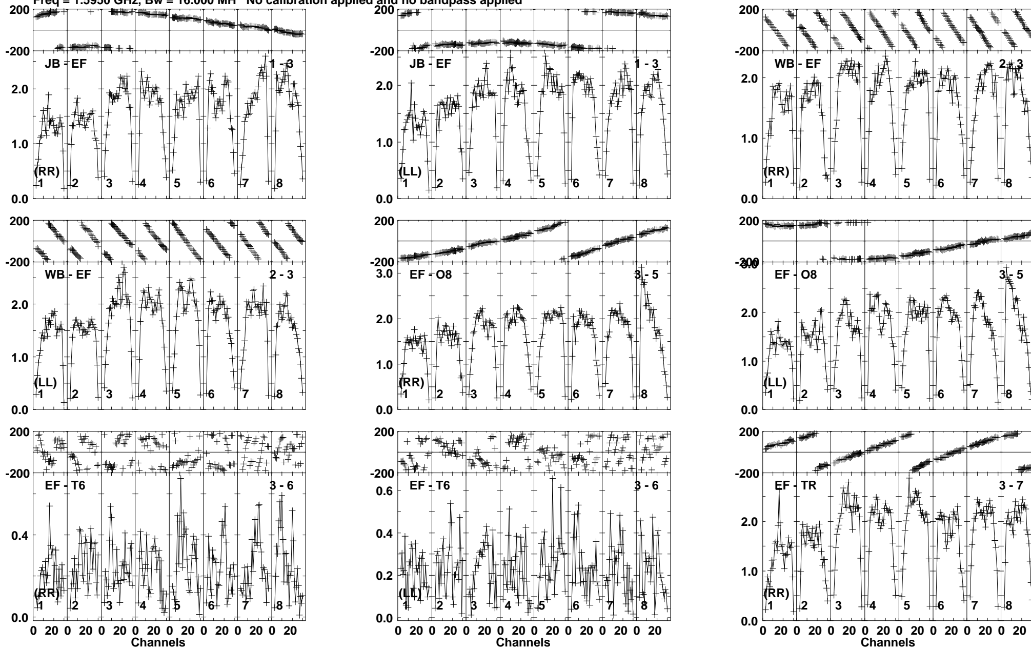
Lower frame: Milli Ampl Jy Top frame: Phas deg Vector averaged cross-power spectrum Baseline: JB (01) - EF (03) Timerange: 00/11:40:41 to 00/11:42:09
