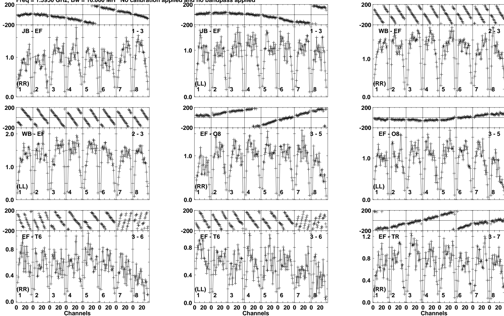
Lower frame: Milli Ampl Jy Top frame: Phas deg Vector averaged cross-power spectrum Baseline: JB (01) - EF (03) Timerange: 00:12:42:51 to 00:12:44:19
