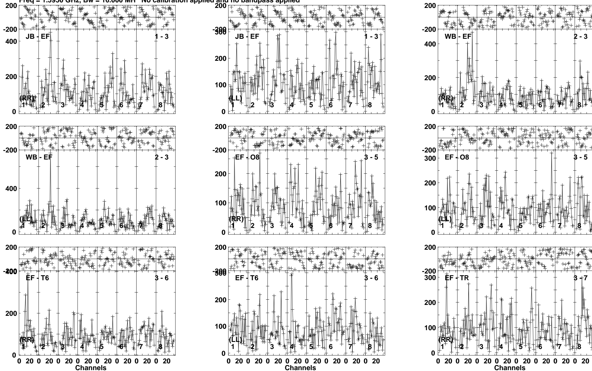
Lower frame: Micro Ampl Jy Top frame: Phas deg Vector averaged cross-power spectrum Baseline: JB (01) - EF (03) Timerange: 00/12:50:01 to 00/12:53:29
