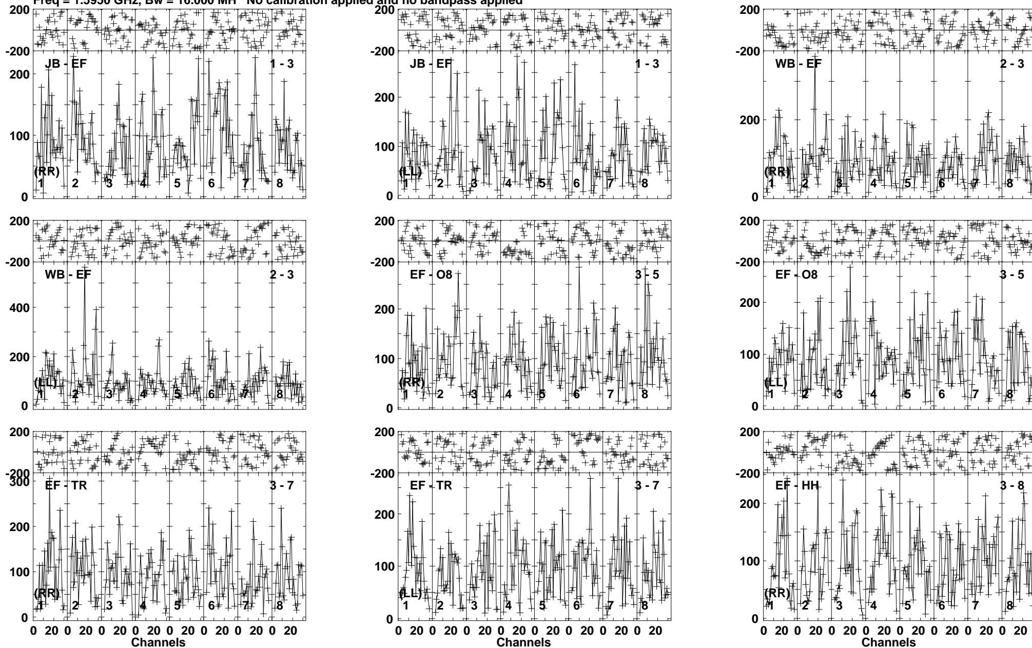
Lower frame: Micro Ampl Jy Top frame: Phas deg Vector averaged cross-power spectrum Baseline: JB (01) - EF (03) Timerange: 00/11:18:11 to 00/11:21:39
