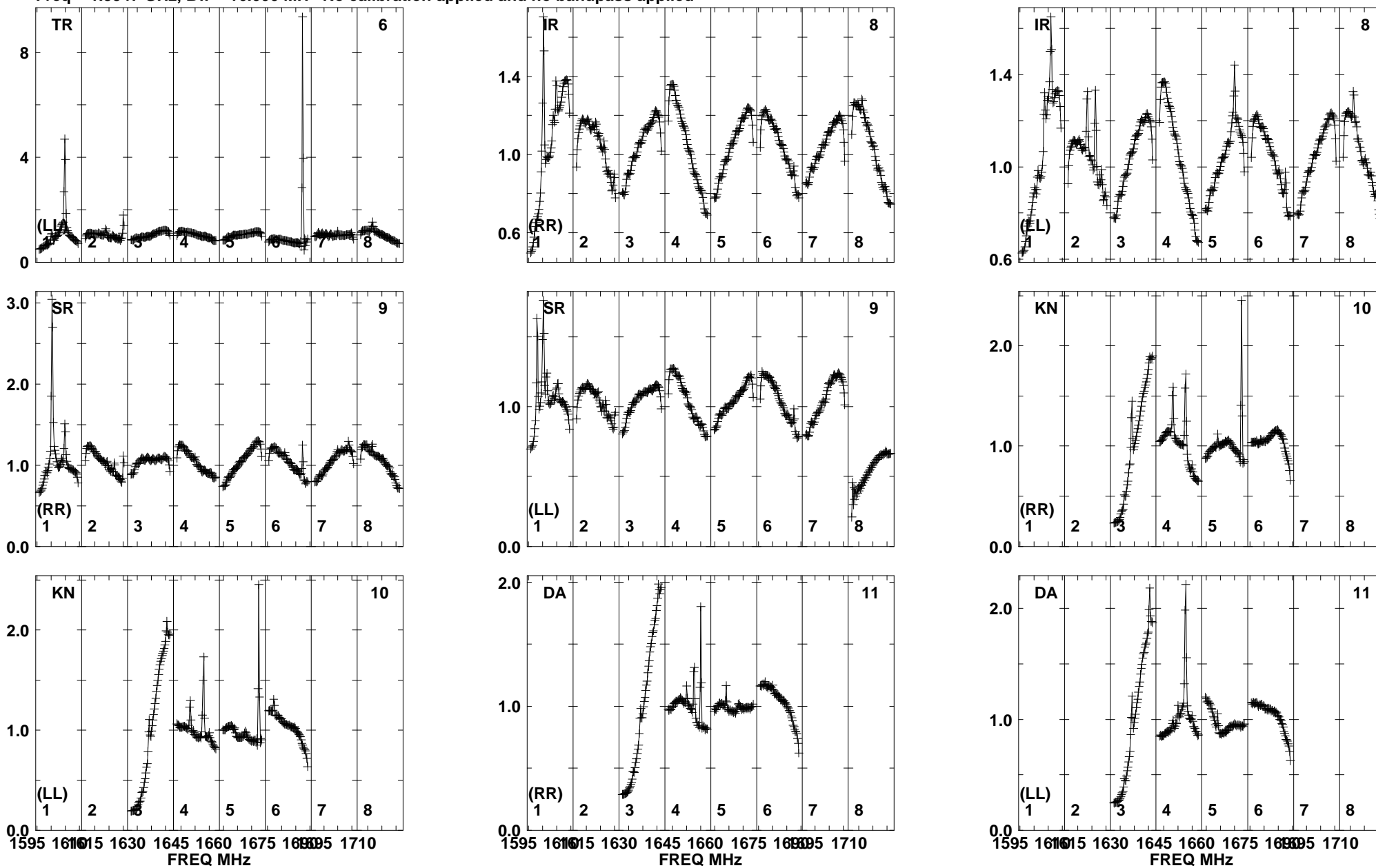
Lower frame: Real Jy Total-power spectrum Antenna: TR (06) Timerange: 00/22:27:41 to 00/22:29:10
