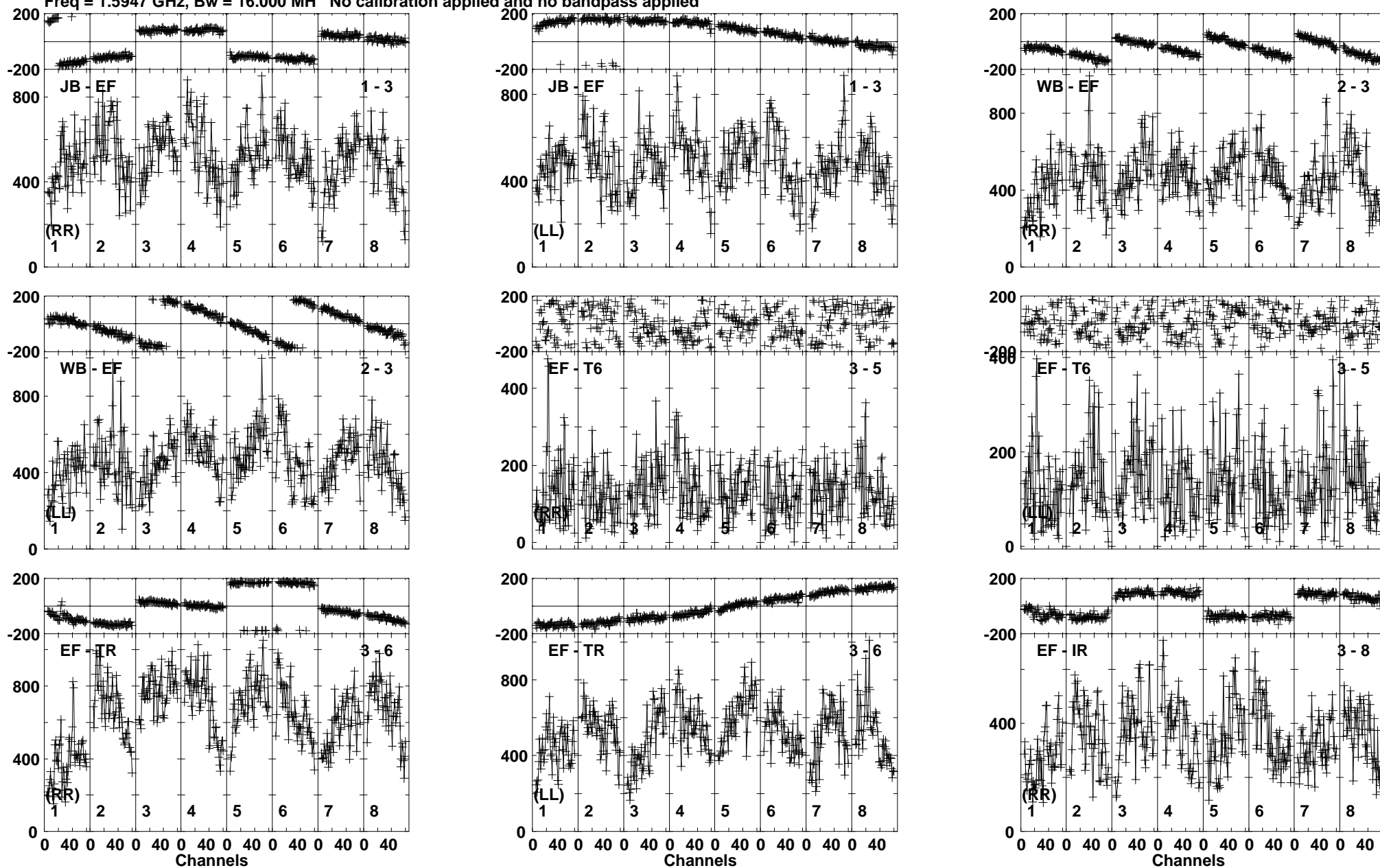
Lower frame: Micro Ampl Jy Top frame: Phas deg Vector averaged cross-power spectrum Baseline: JB (01) - EF (03) Timerange: 00:22:44:10 to 00:22:47:10
