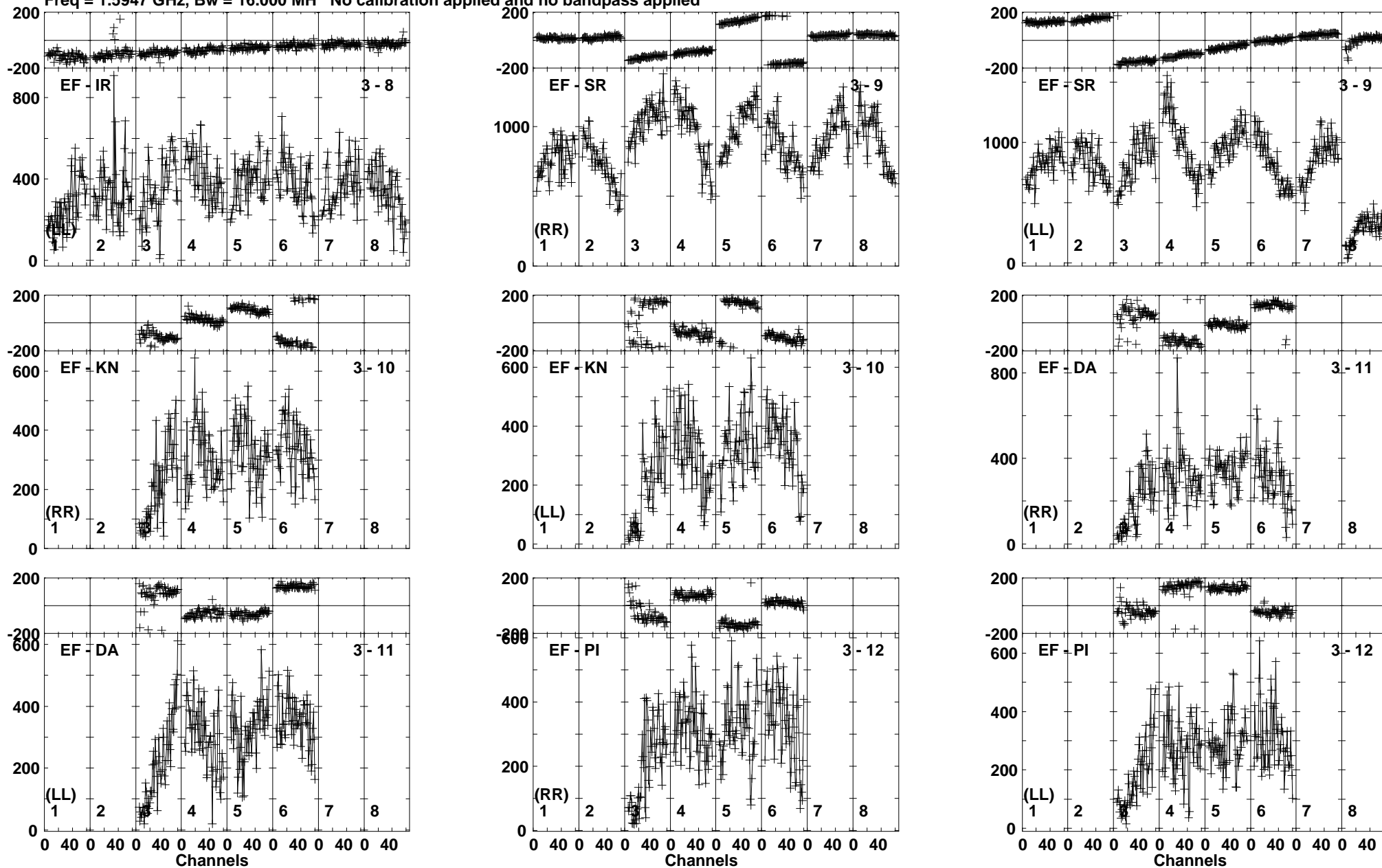
Lower frame: Micro Ampl Jy Top frame: Phas deg Vector averaged cross-power spectrum Baseline: EF (03) - IR (08) Timerange: 00/21:09:10 to 00/21:12:10
