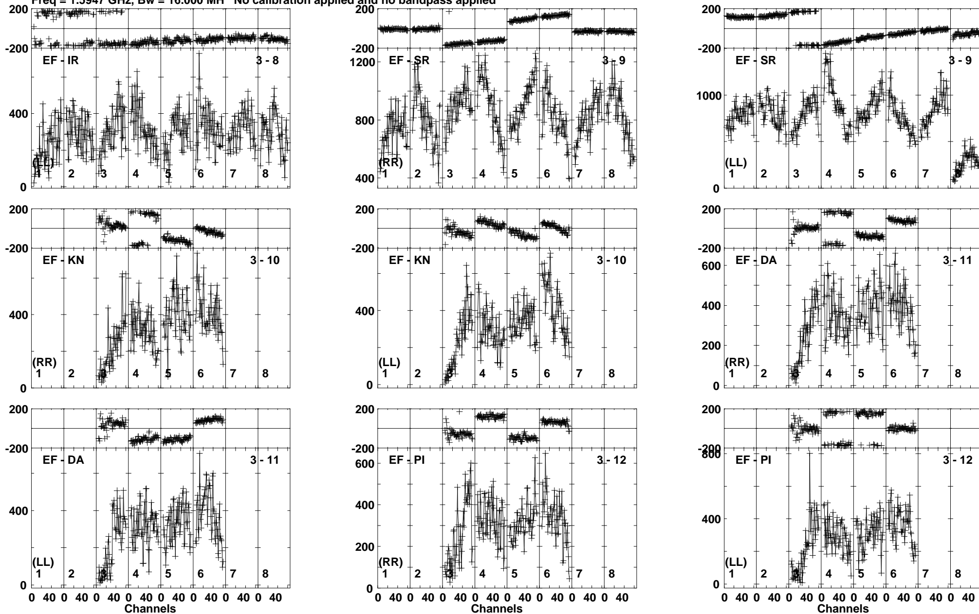
Lower frame: Micro Ampl Jy Top frame: Phas deg Vector averaged cross-power spectrum Baseline: EF (03) - IR (08) Timerange: 00:22:14:10 to 00:22:17:10
