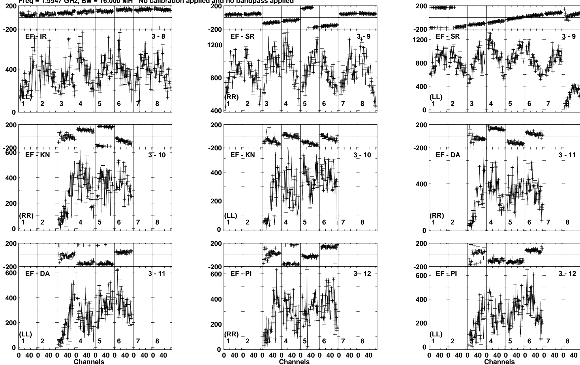
Lower frame: Micro Ampl Jy Top frame: Phas deg Vector averaged cross-power spectrum Baseline: EF (03) - IR (08) Timerange: 00/21:24:10 to 00/21:27:10
