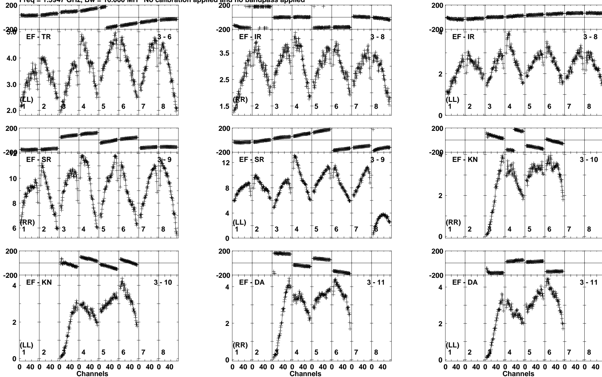
Lower frame: Milli Ampl Jy Top frame: Phas deg Vector averaged cross-power spectrum Baseline: EF (03) - TR (06) Timerange: 00/21:42:10 to 00/21:44:10
