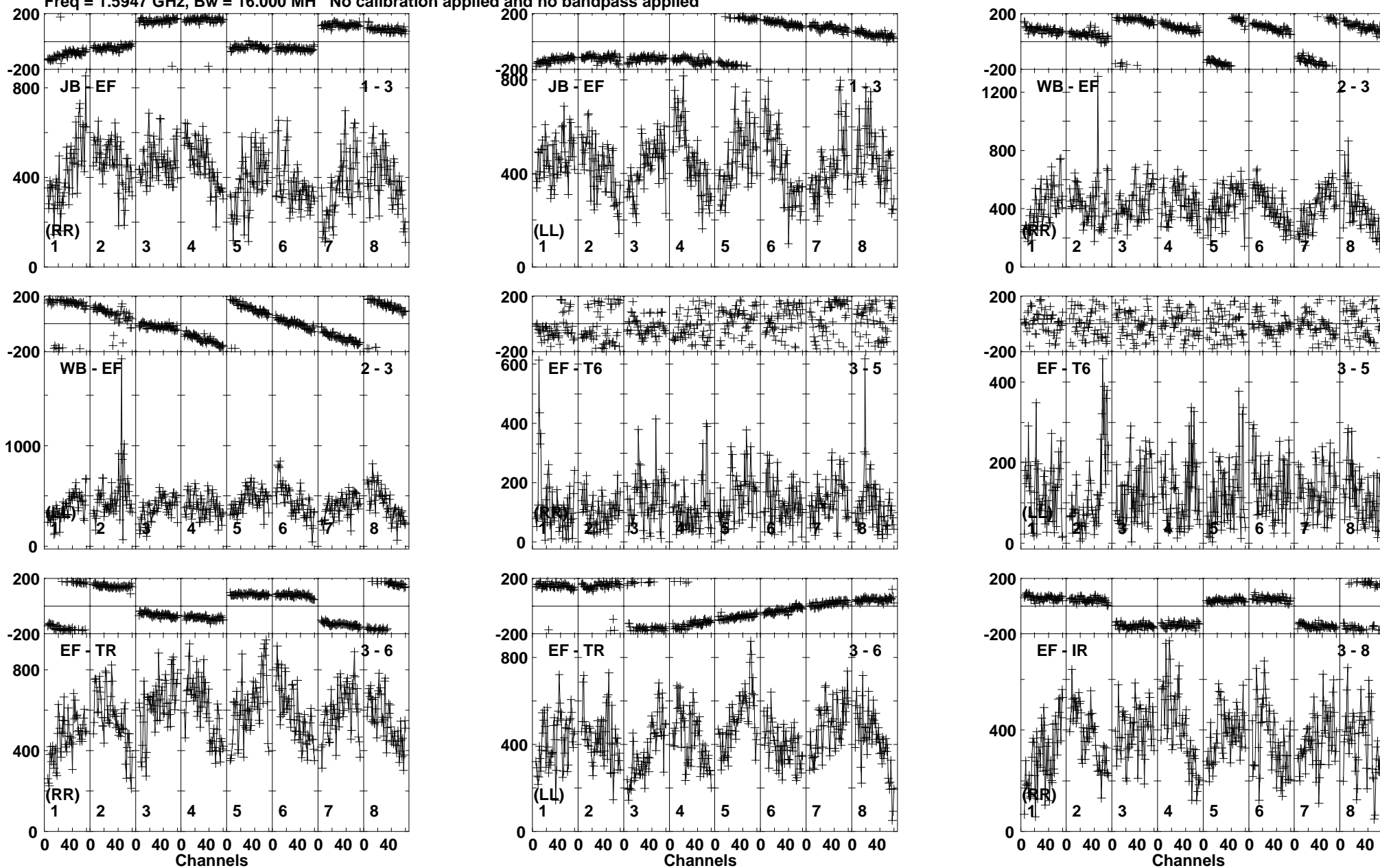
Lower frame: Micro Ampl Jy Top frame: Phas deg Vector averaged cross-power spectrum Baseline: JB (01) - EF (03) Timerange: 00/22:09:10 to 00/22:12:10
