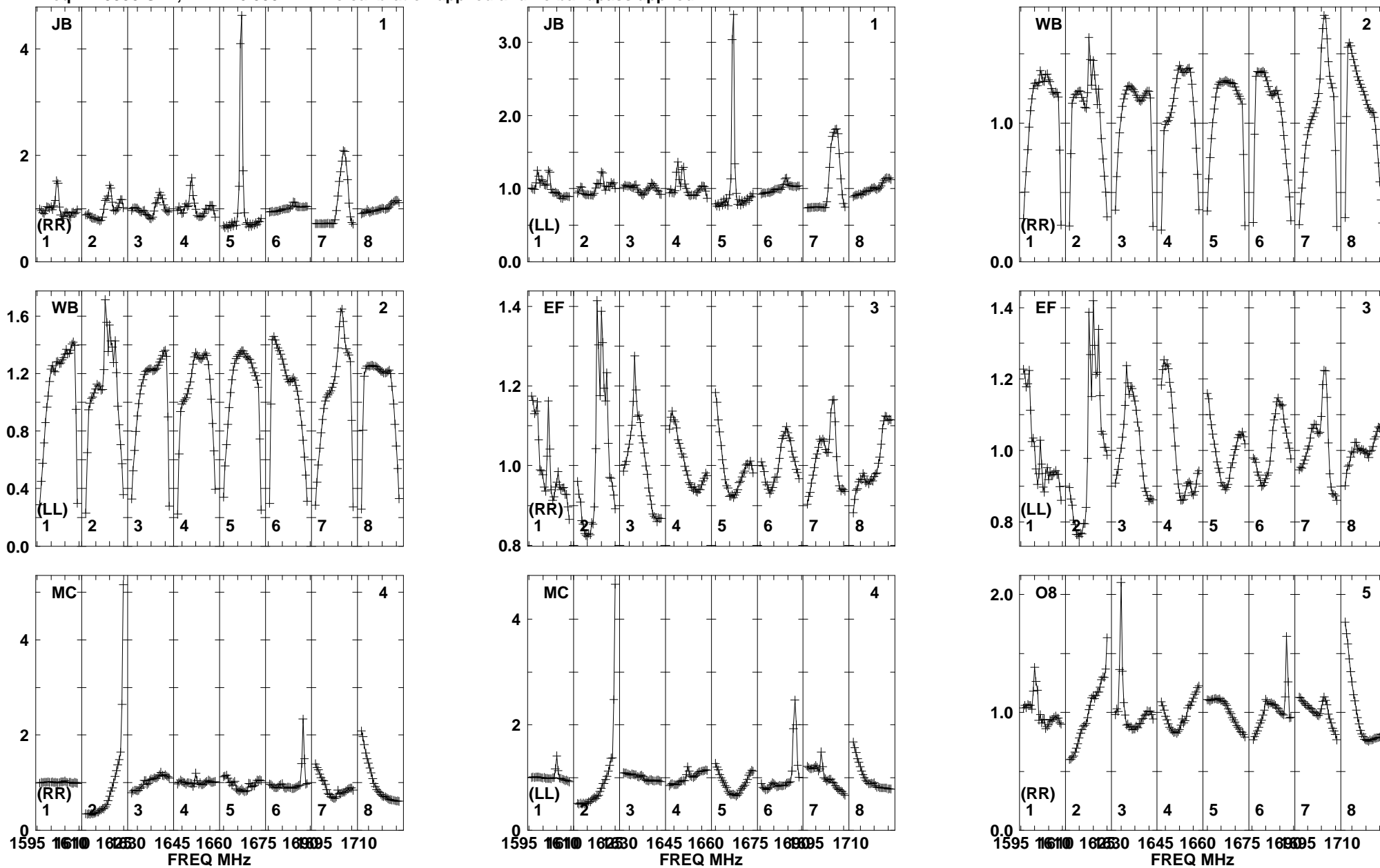
Lower frame: Real Jy Total-power spectrum Antenna: JB (01) Timerange: 00/09:59:21 to 00/10:03:19
