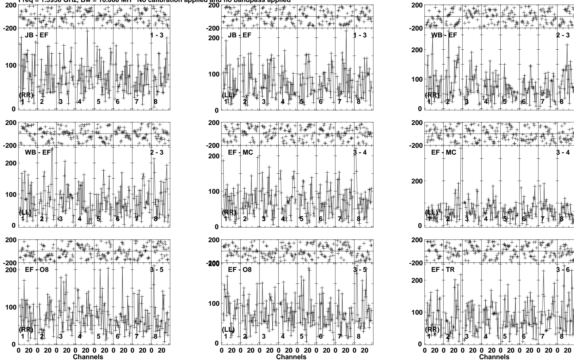
Lower frame: Micro Ampl Jy Top frame: Phas deg Vector averaged cross-power spectrum Baseline: JB (01) - EF (03) Timerange: 00/10:43:41 to 00/10:47:39
