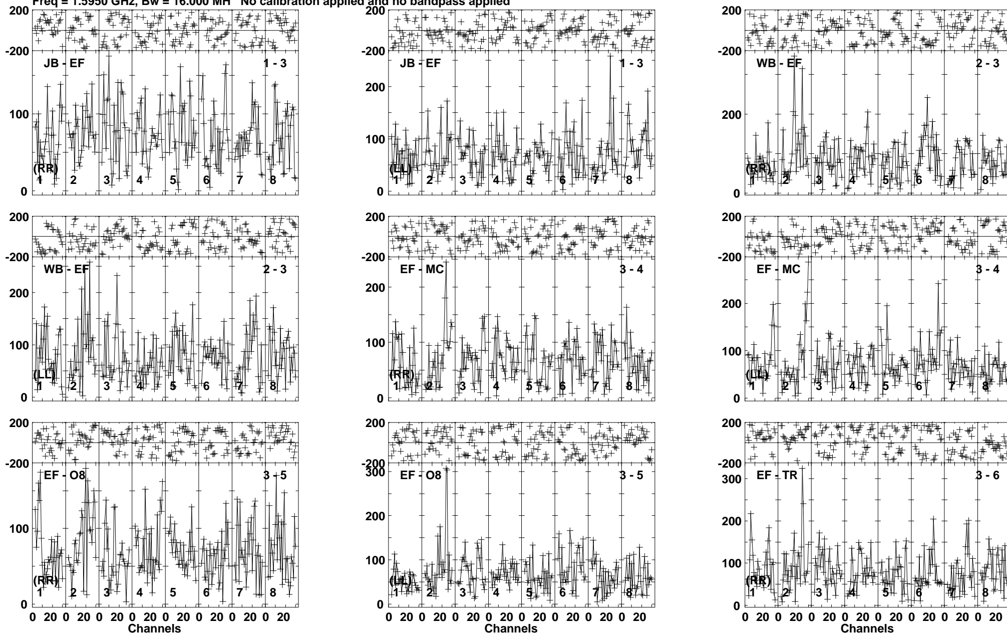
Lower frame: Micro Ampl Jy Top frame: Phas deg Vector averaged cross-power spectrum Baseline: JB (01) - EF (03) Timerange: 00/09:06:01 to 00/09:09:59
