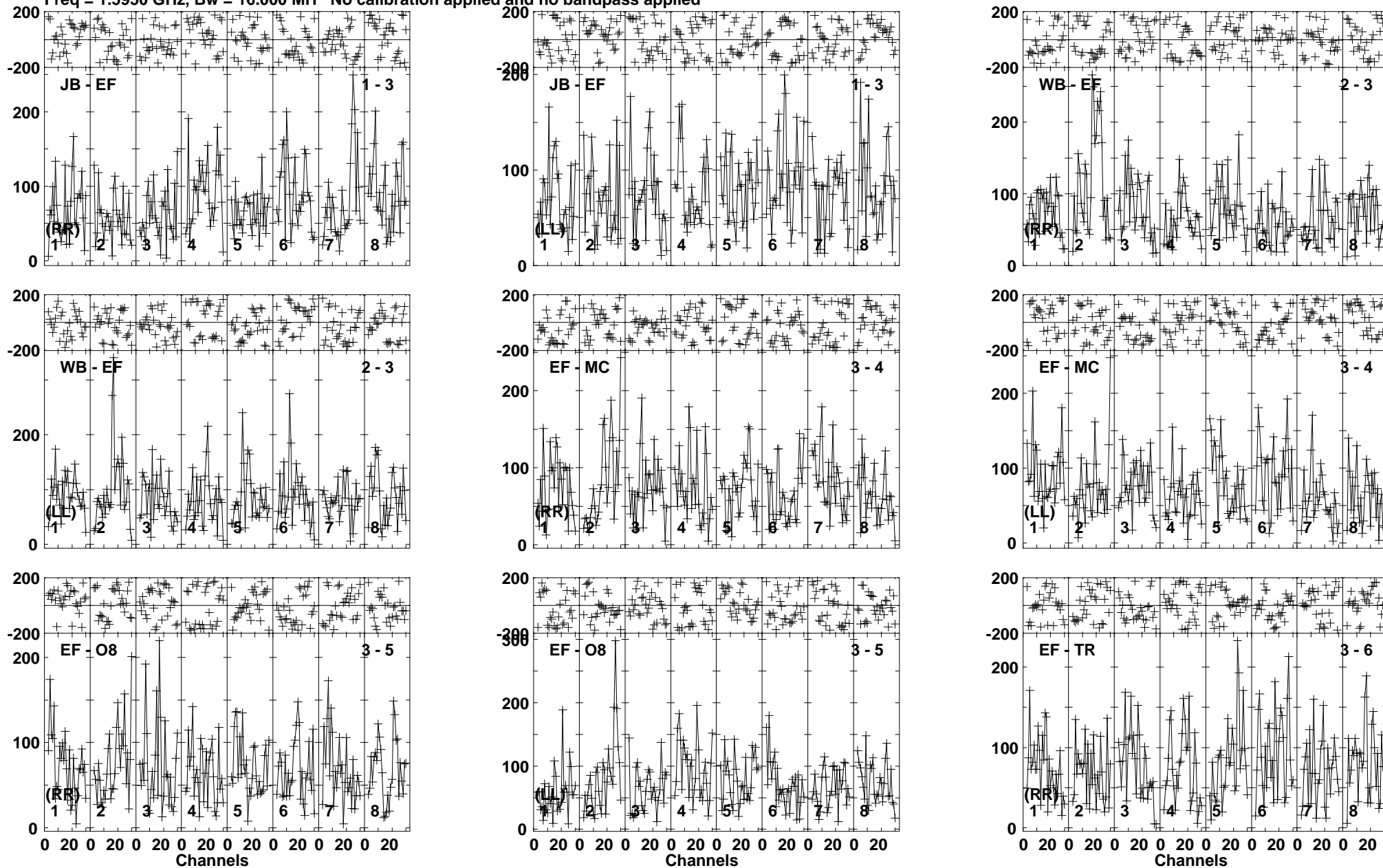
Lower frame: Micro Ampl Jy Top frame: Phas deg Vector averaged cross-power spectrum Baseline: JB (01) - EF (03) Timerange: 00/11:20:41 to 00/11:24:39
