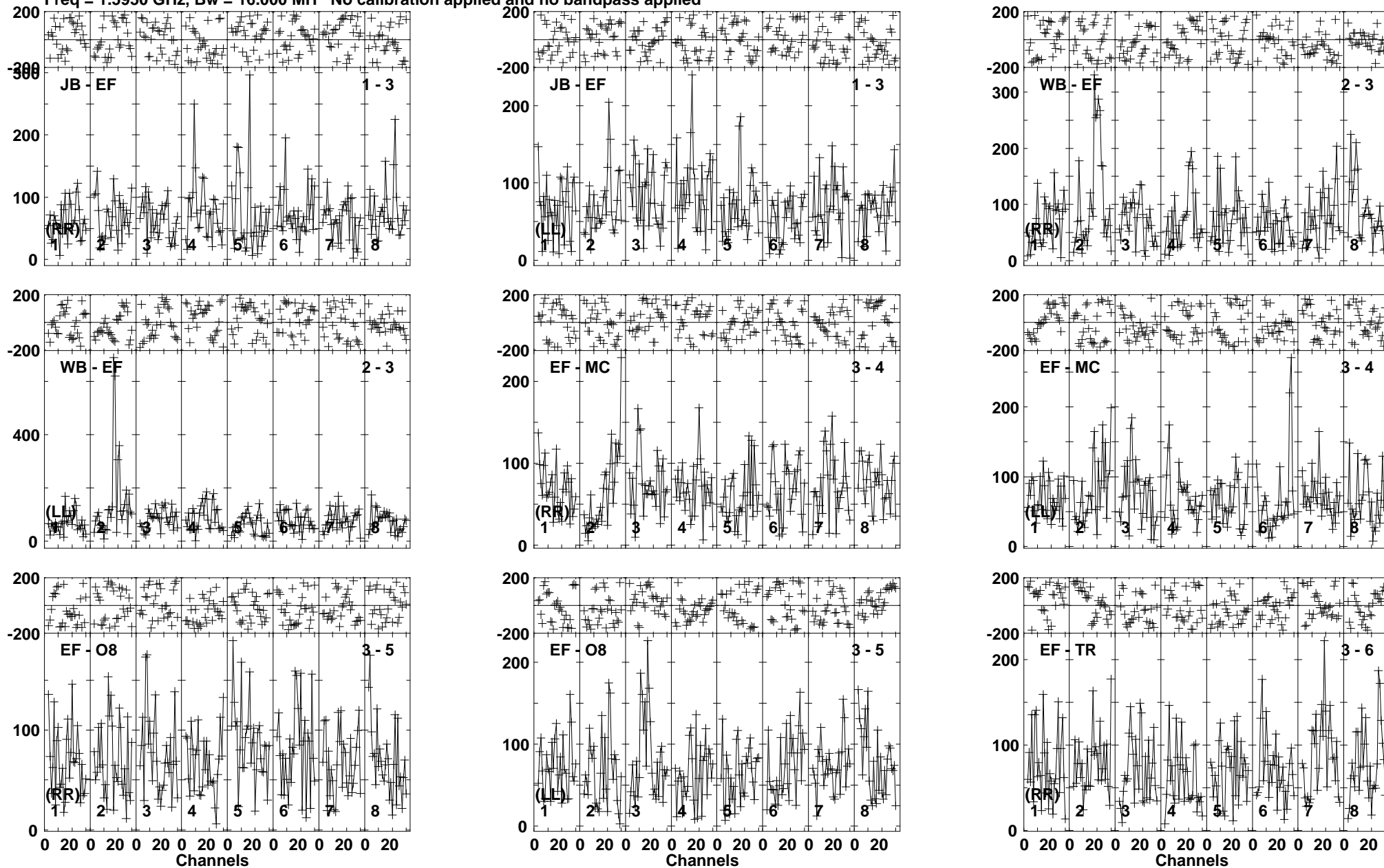
Lower frame: Micro Ampl Jy Top frame: Phas deg Vector averaged cross-power spectrum Baseline: JB (01) - EF (03) Timerange: 00/10:27:21 to 00/10:31:19
