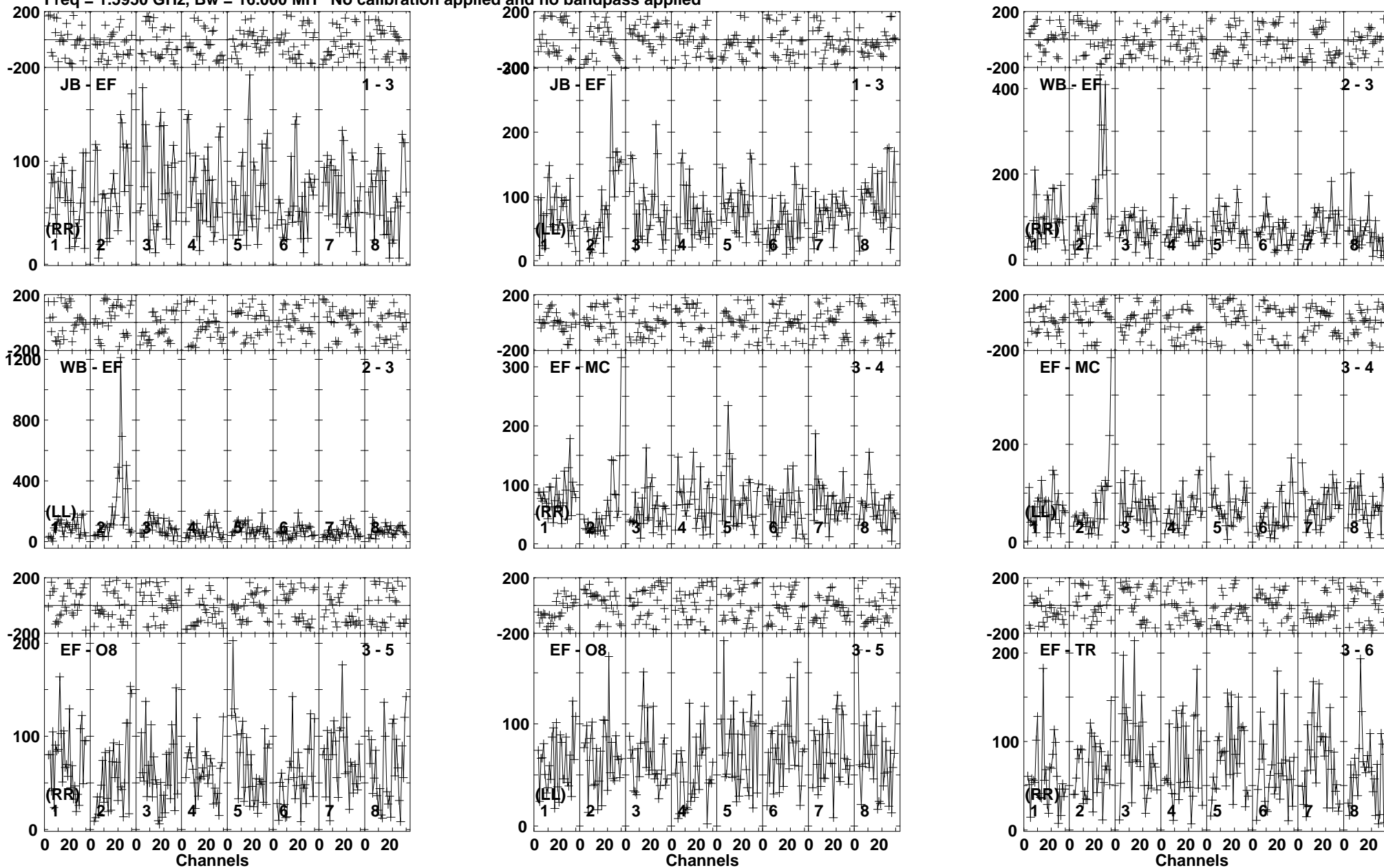
Lower frame: Micro Ampl Jy Top frame: Phas deg Vector averaged cross-power spectrum Baseline: JB (01) - EF (03) Timerange: 00/09:48:41 to 00/09:52:39
