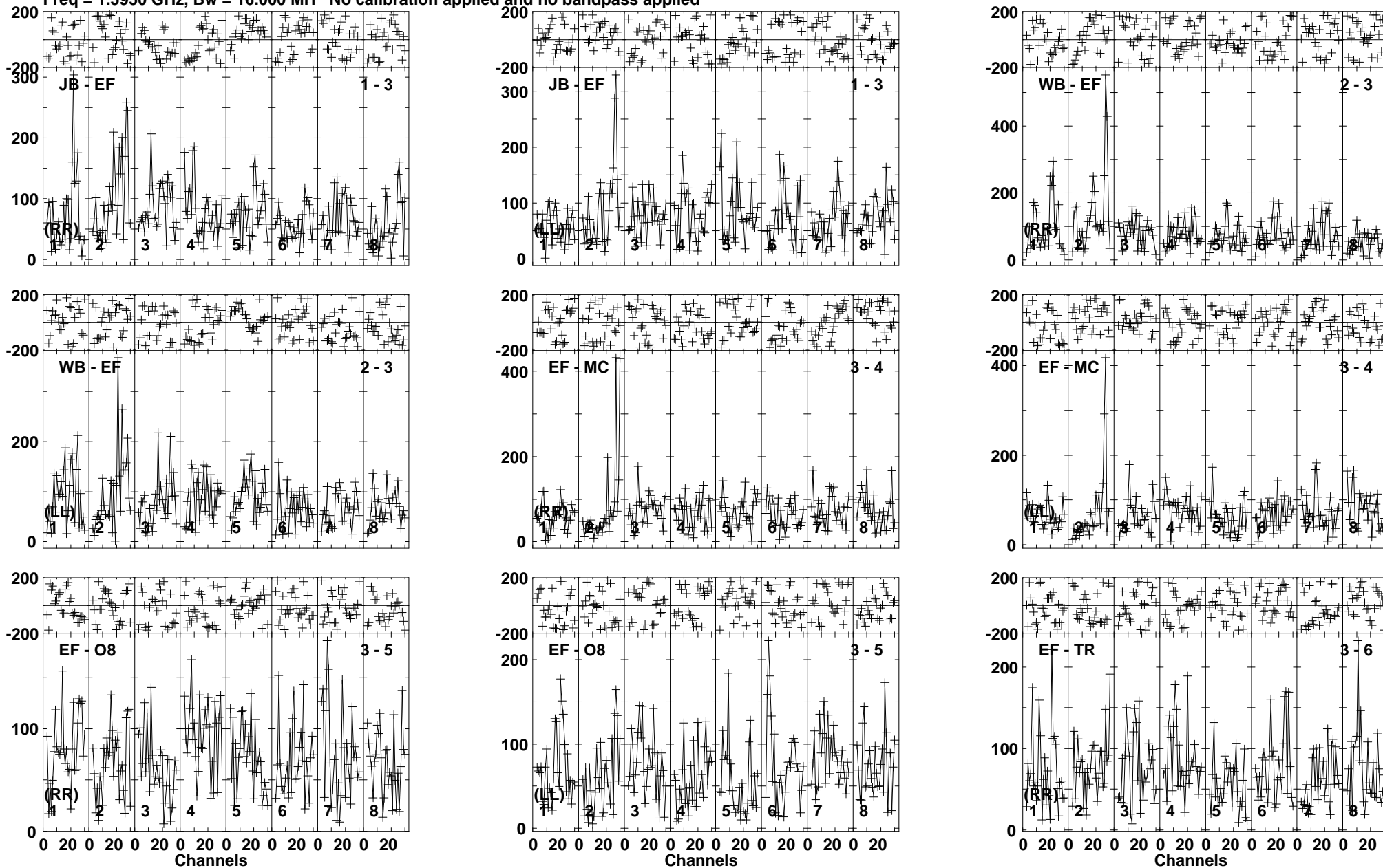
Lower frame: Micro Ampl Jy Top frame: Phas deg Vector averaged cross-power spectrum Baseline: JB (01) - EF (03) Timerange: 00/09:27:21 to 00/09:31:19
