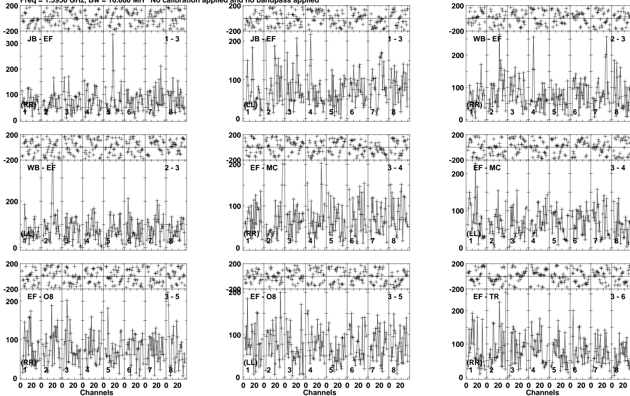
Lower frame: Micro Ampl Jy Top frame: Phas deg Vector averaged cross-power spectrum Baseline: JB (01) - EF (03) Timerange: 00/10:15:41 to 00/10:19:39
