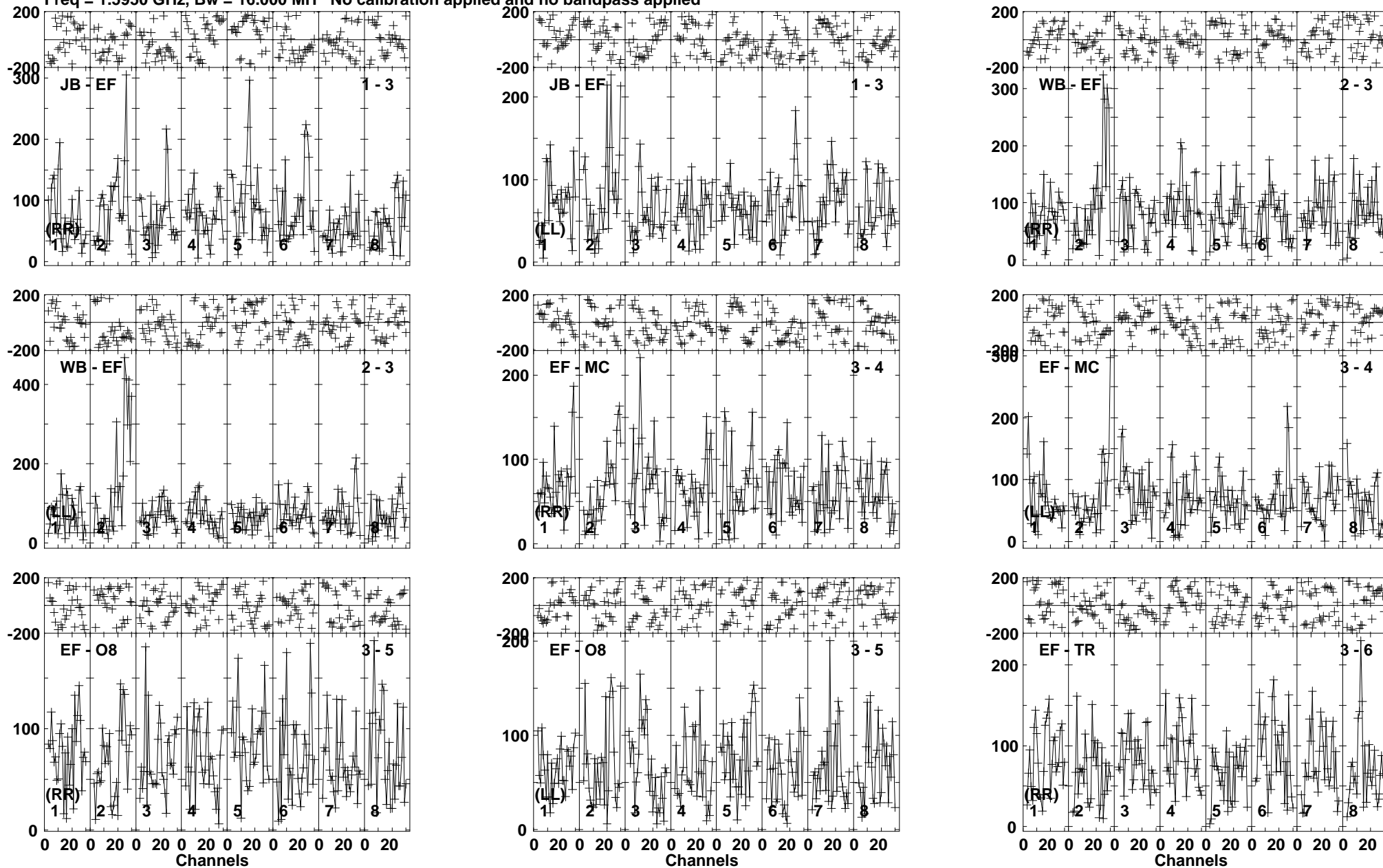
Lower frame: Micro Ampl Jy Top frame: Phas deg Vector averaged cross-power spectrum Baseline: JB (01) - EF (03) Timerange: 00/10:05:01 to 00/10:08:59
