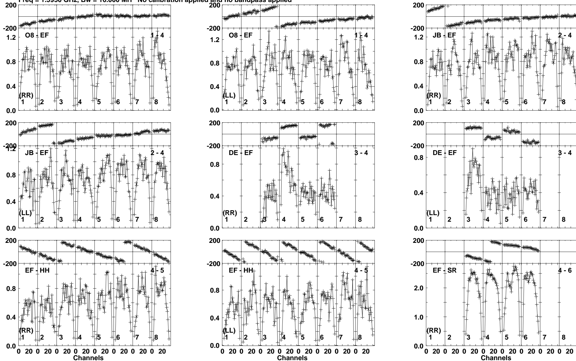
Lower frame: Milli Ampl Jy Top frame: Phas deg Vector averaged cross-power spectrum Baseline: O8 (01) - EF (04) Timerange: 00/01:04:01 to 00/01:05:00
