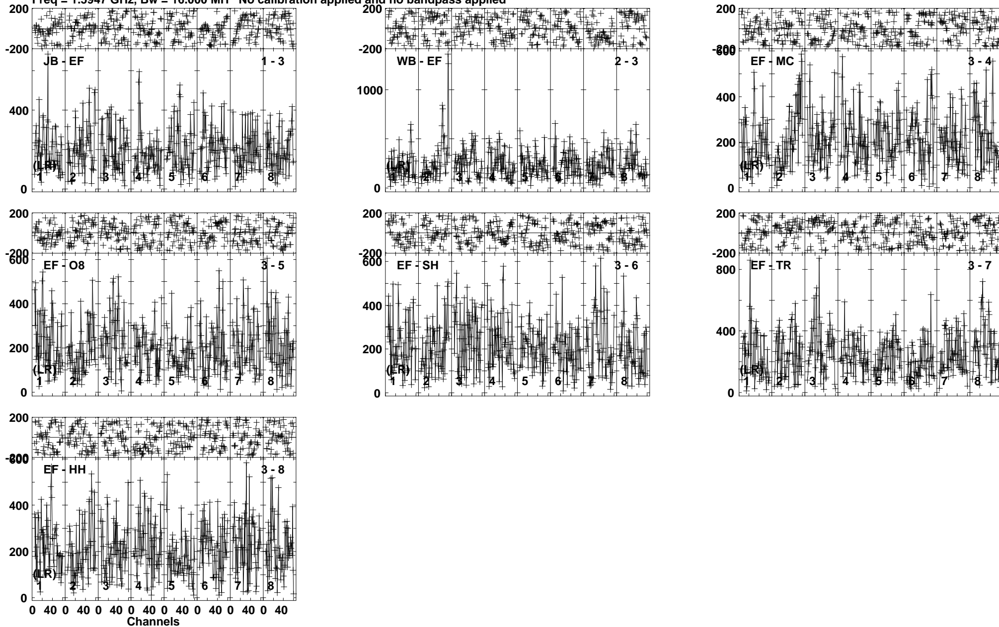
Lower frame: Micro Ampl Jy Top frame: Phas deg Vector averaged cross-power spectrum Baseline: JB (01) - EF (03) Timerange: 00/16:19:51 to 00/16:21:19
