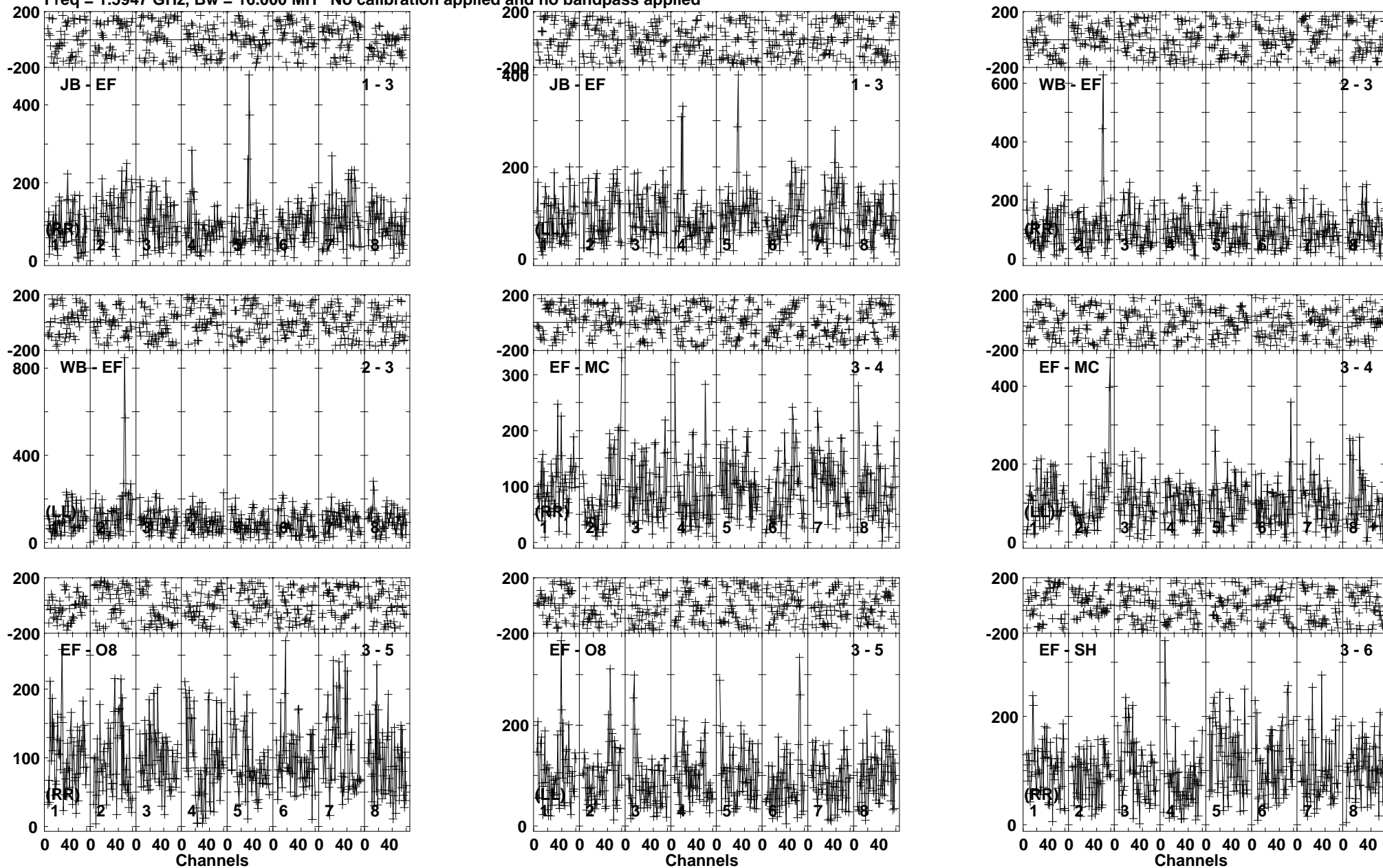
Lower frame: Micro Ampl Jy Top frame: Phas deg Vector averaged cross-power spectrum Baseline: JB (01) - EF (03) Timerange: 00/16:39:41 to 00/16:44:09
