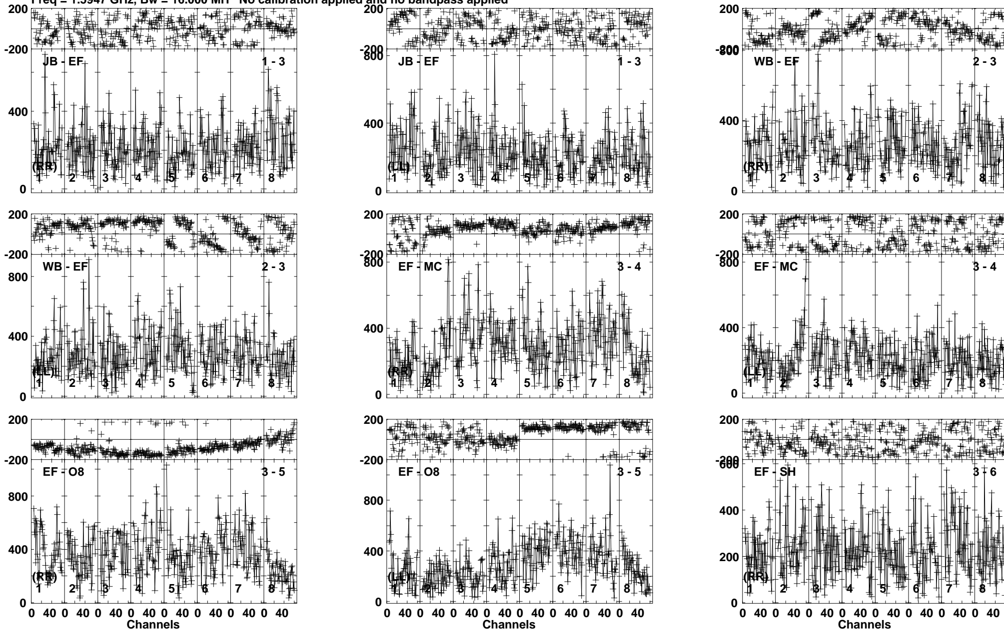
Lower frame: Micro Ampl Jy Top frame: Phas deg Vector averaged cross-power spectrum Baseline: JB (01) - EF (03) Timerange: 00/17:27:21 to 00/17:28:19
