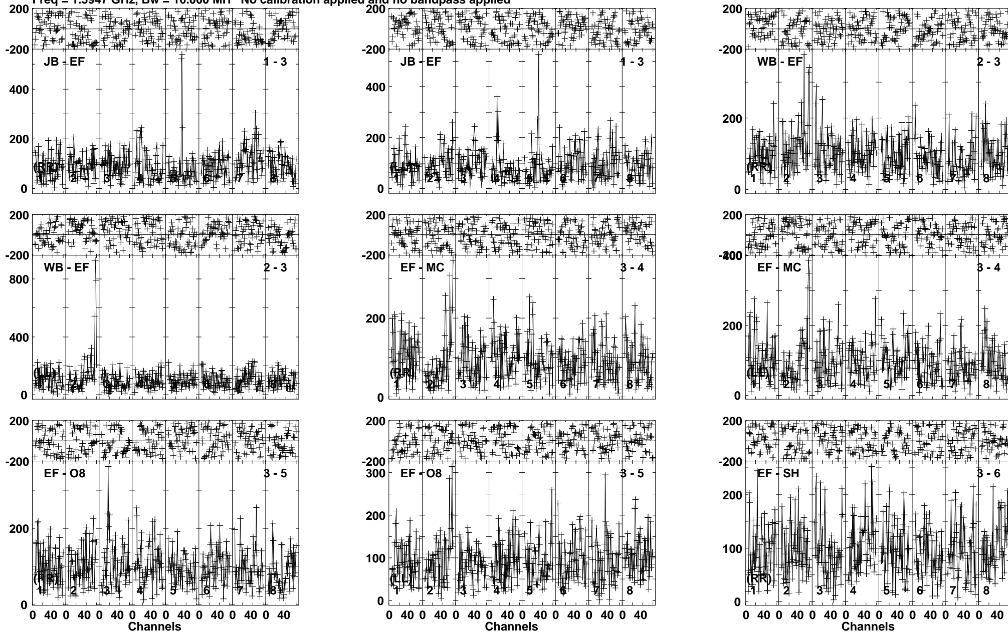
Lower frame: Micro Ampl Jy Top frame: Phas deg Vector averaged cross-power spectrum Baseline: JB (01) - EF (03) Timerange: 00/16:33:31 to 00/16:37:59
