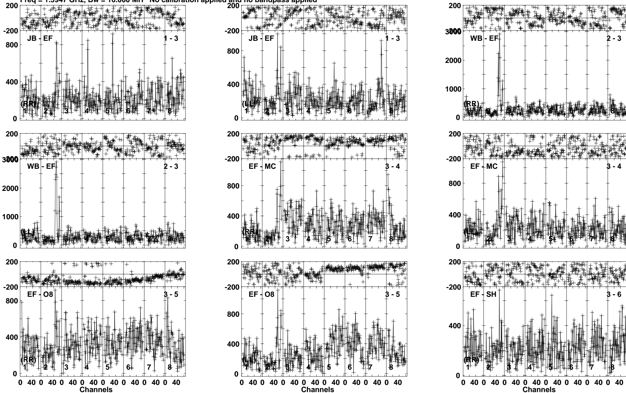
Lower frame: Micro Ampl Jy Top frame: Phas deg Vector averaged cross-power spectrum Baseline: JB (01) - EF (03) Timerange: 00/15:43:21 to 00/15:44:49
