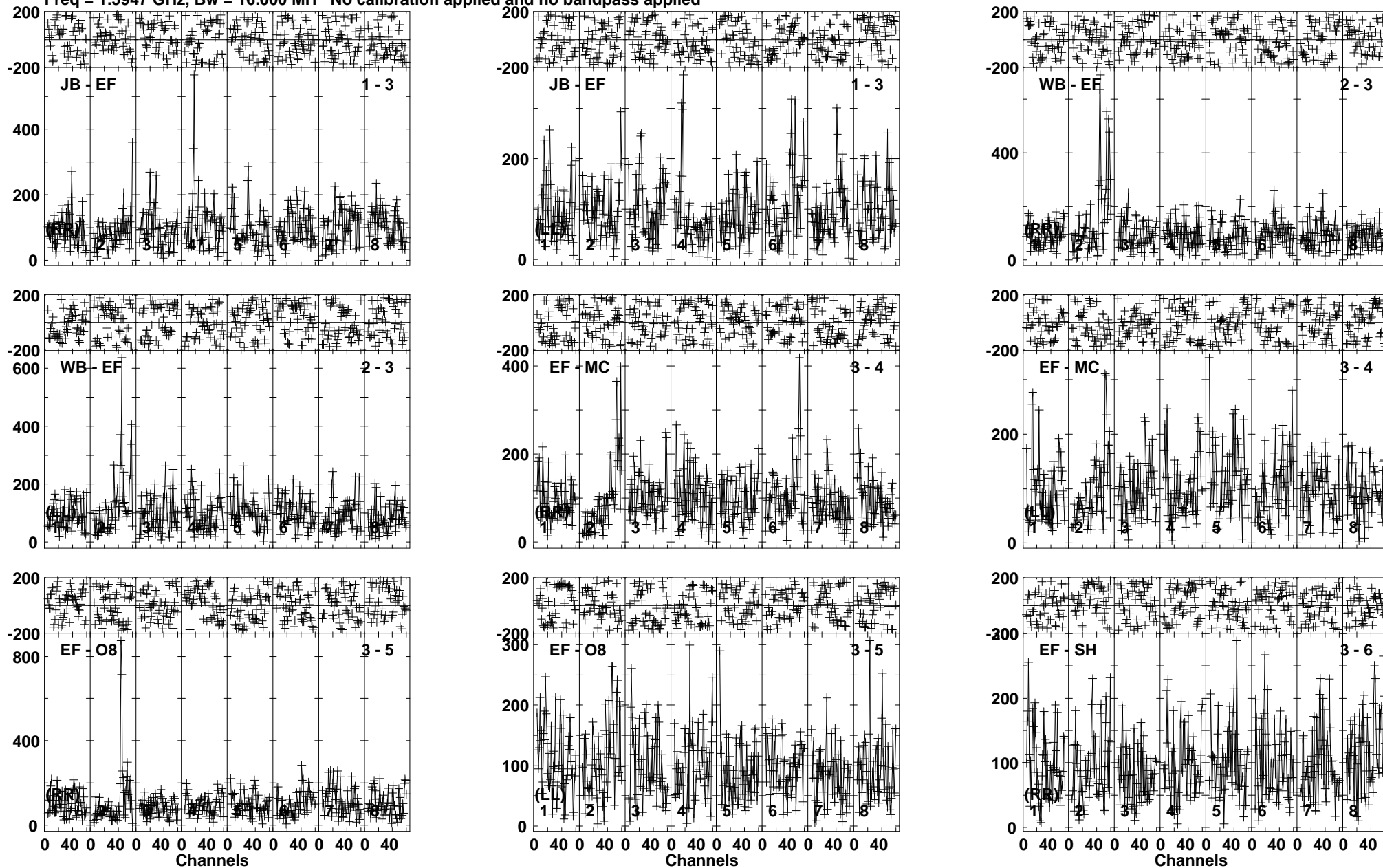
Lower frame: Micro Ampl Jy Top frame: Phas deg Vector averaged cross-power spectrum Baseline: JB (01) - EF (03) Timerange: 00/15:02:21 to 00/15:06:49
