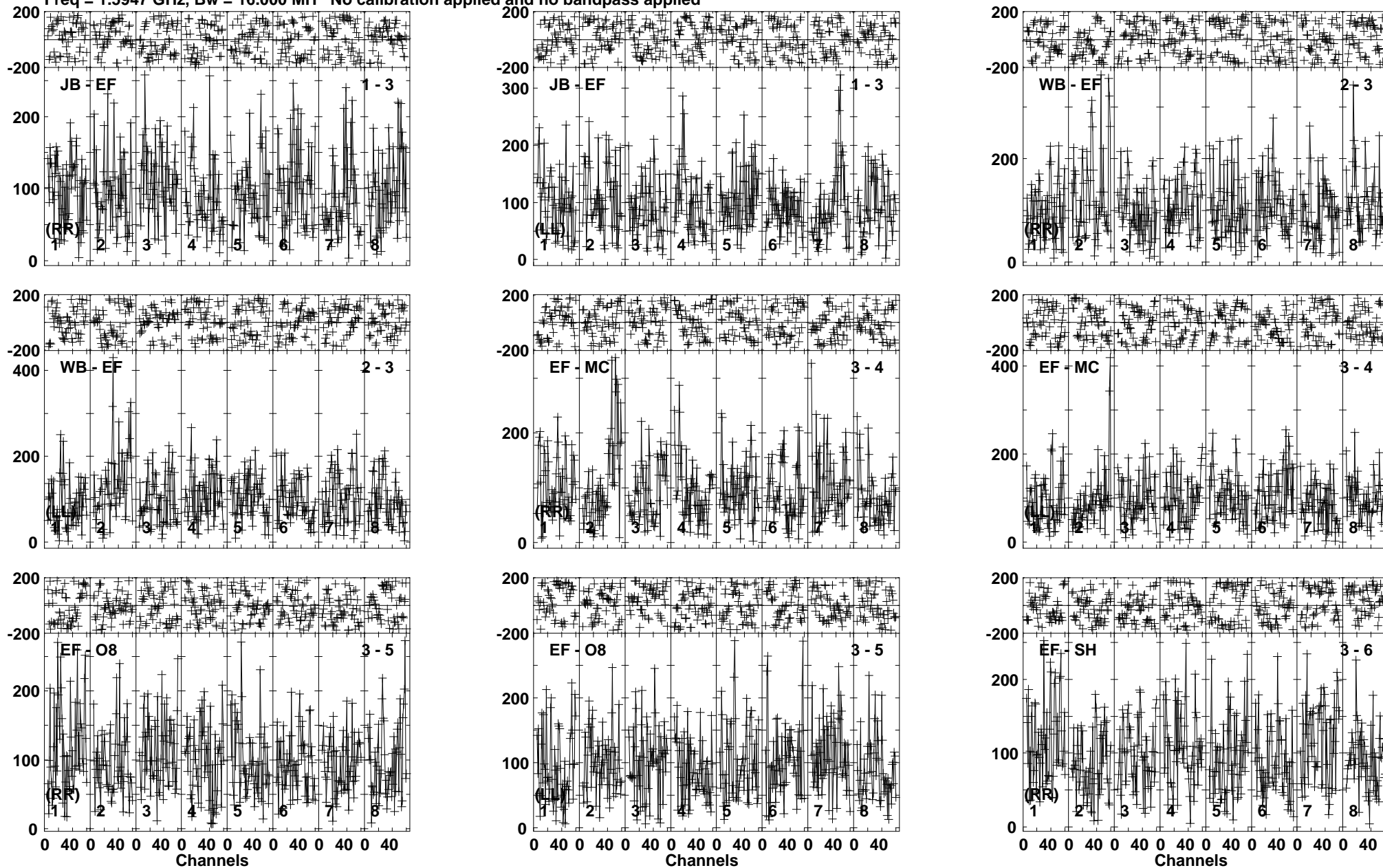
Lower frame: Micro Ampl Jy Top frame: Phas deg Vector averaged cross-power spectrum Baseline: JB (01) - EF (03) Timerange: 00/15:57:01 to 00/16:01:29
