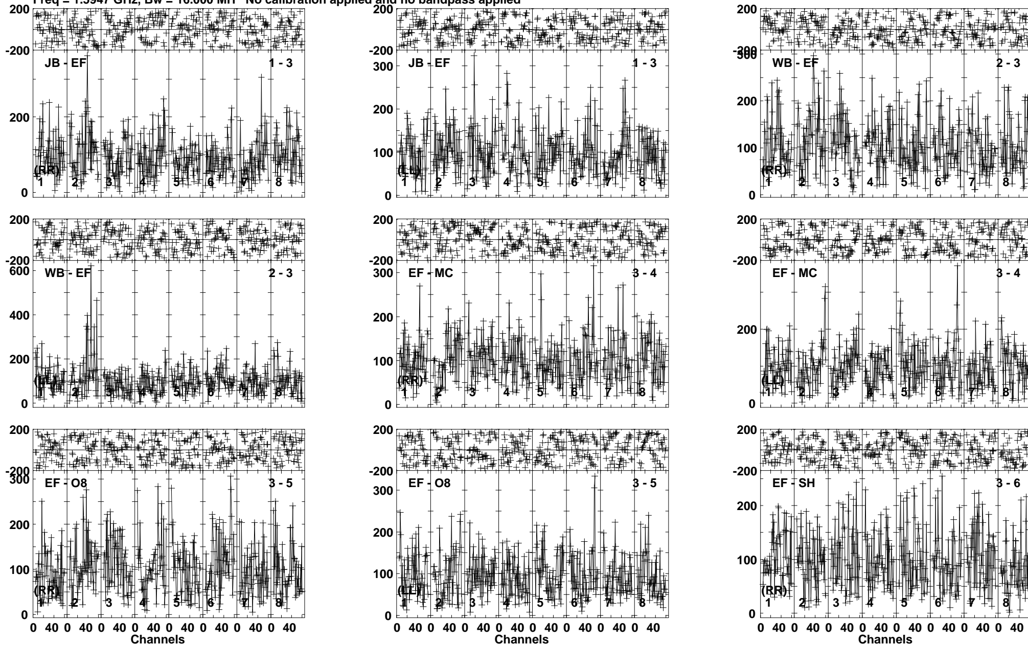
Lower frame: Micro Ampl Jy Top frame: Phas deg Vector averaged cross-power spectrum Baseline: JB (01) - EF (03) Timerange: 00:17:16:11 to 00:17:20:39
