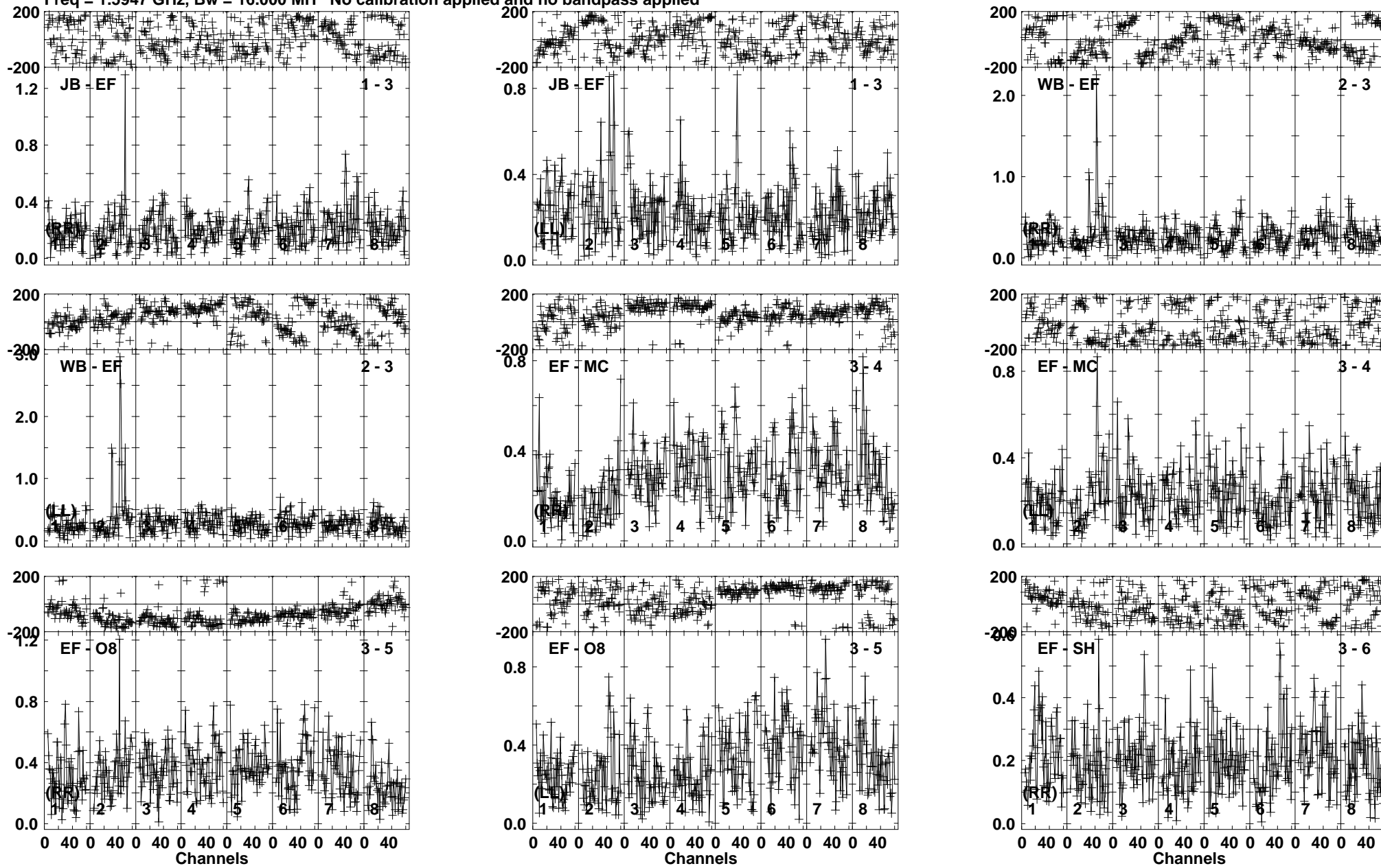
Lower frame: Milli Ampl Jy Top frame: Phas deg Vector averaged cross-power spectrum Baseline: JB (01) - EF (03) Timerange: 00/16:02:11 to 00/16:03:09
