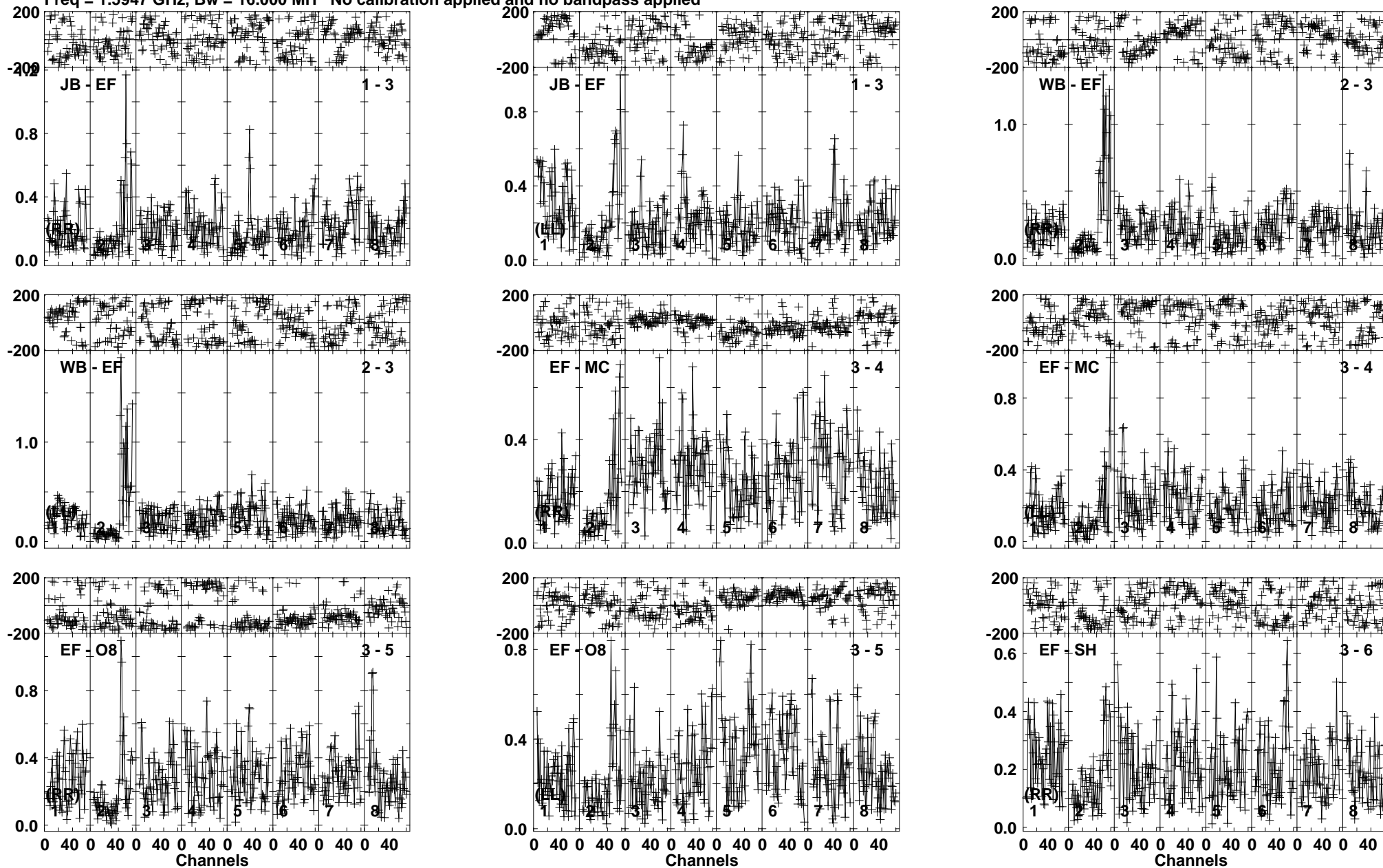
Lower frame: Milli Ampl Jy Top frame: Phas deg Vector averaged cross-power spectrum Baseline: JB (01) - EF (03) Timerange: 00/15:25:41 to 00/15:26:39
