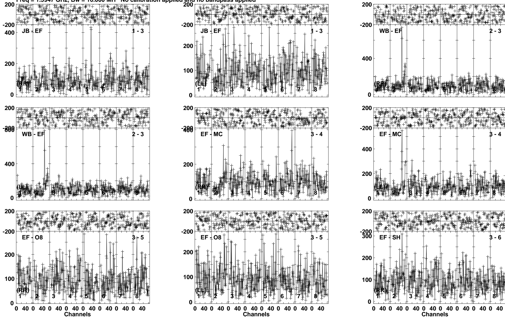
Lower frame: Micro Ampl Jy Top frame: Phas deg Vector averaged cross-power spectrum Baseline: JB (01) - EF (03) Timerange: 00/16:15:21 to 00/16:19:49
