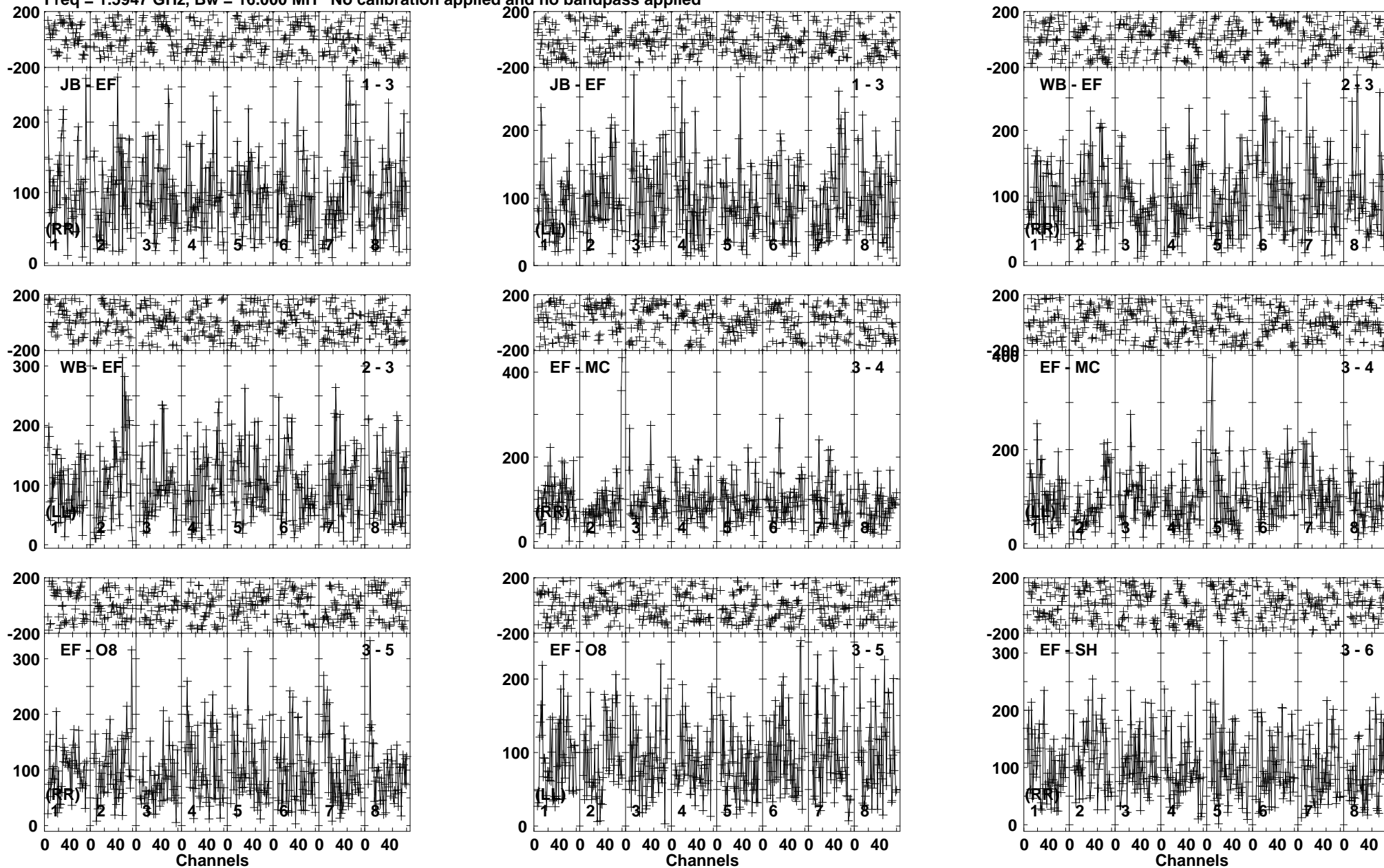
Lower frame: Micro Ampl Jy Top frame: Phas deg Vector averaged cross-power spectrum Baseline: JB (01) - EF (03) Timerange: 00/17:22:11 to 00/17:26:39
