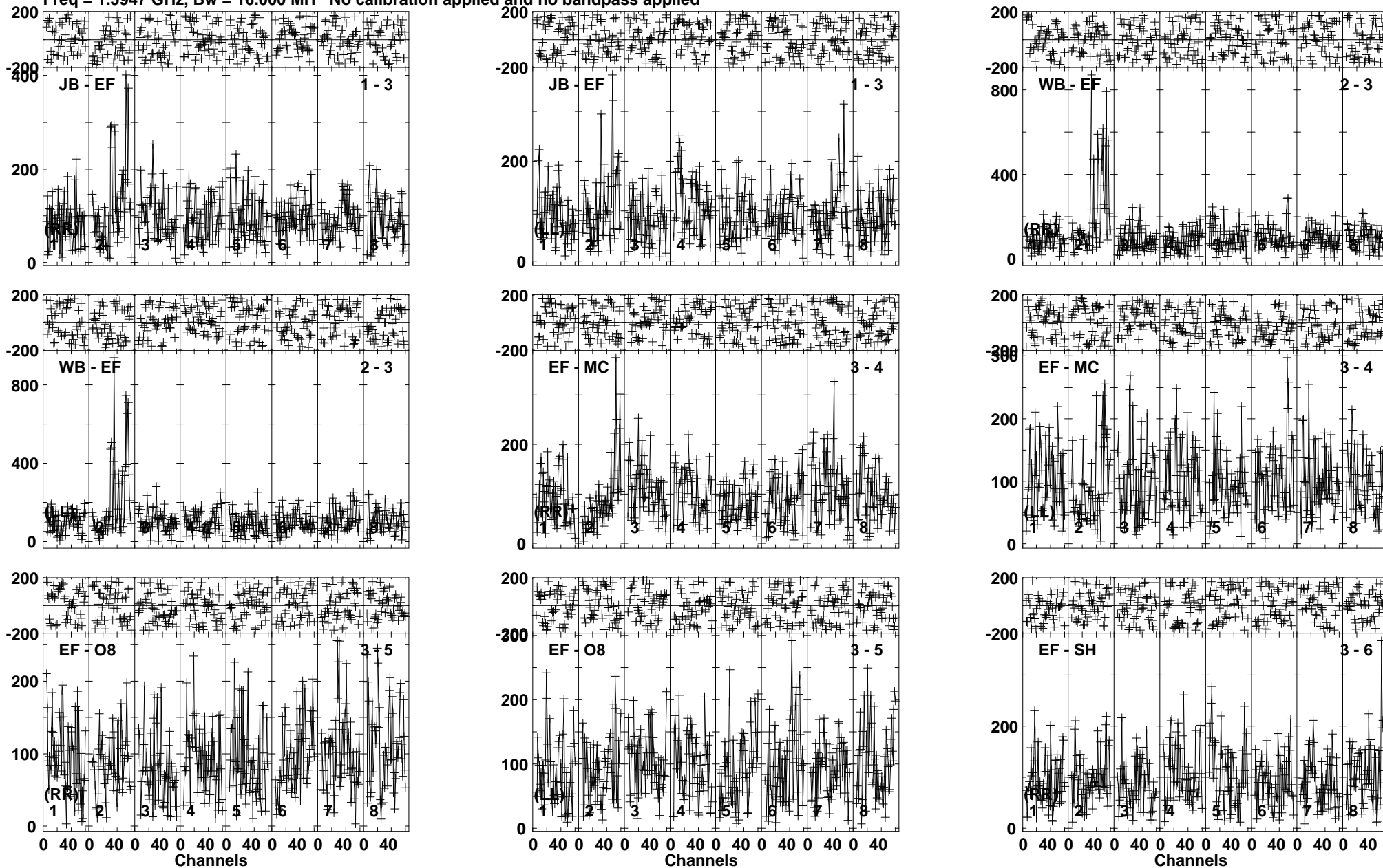
Lower frame: Micro Ampl Jy Top frame: Phas deg Vector averaged cross-power spectrum Baseline: JB (01) - EF (03) Timerange: 00/15:51:01 to 00/15:55:29
