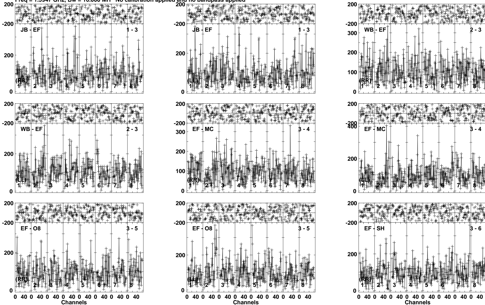
Lower frame: Micro Ampl Jy Top frame: Phas deg Vector averaged cross-power spectrum Baseline: JB (01) - EF (03) Timerange: 00/16:57:51 to 00/17:02:19
