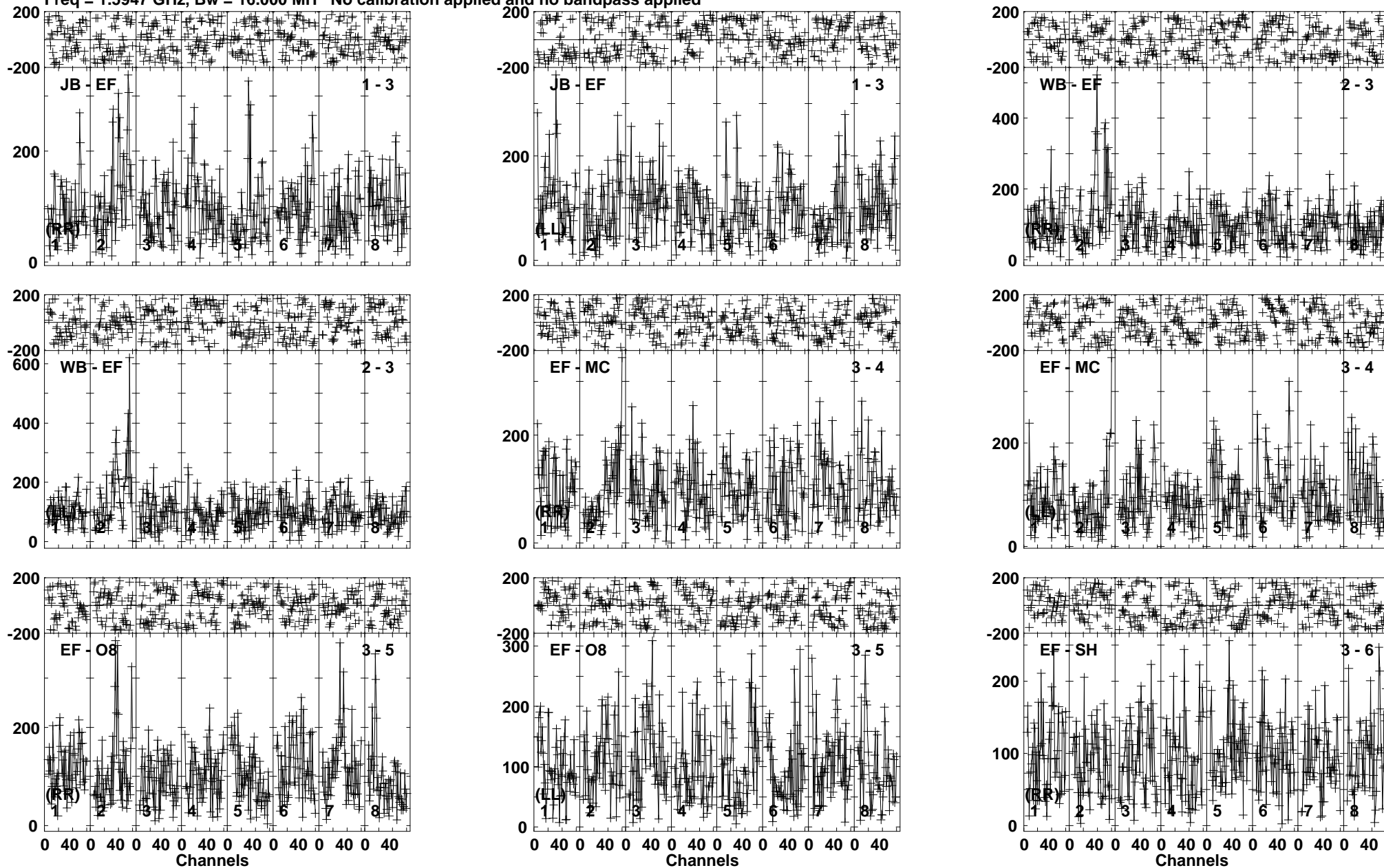
Lower frame: Micro Ampl Jy Top frame: Phas deg Vector averaged cross-power spectrum Baseline: JB (01) - EF (03) Timerange: 00:16:09:11 to 00:16:13:39
