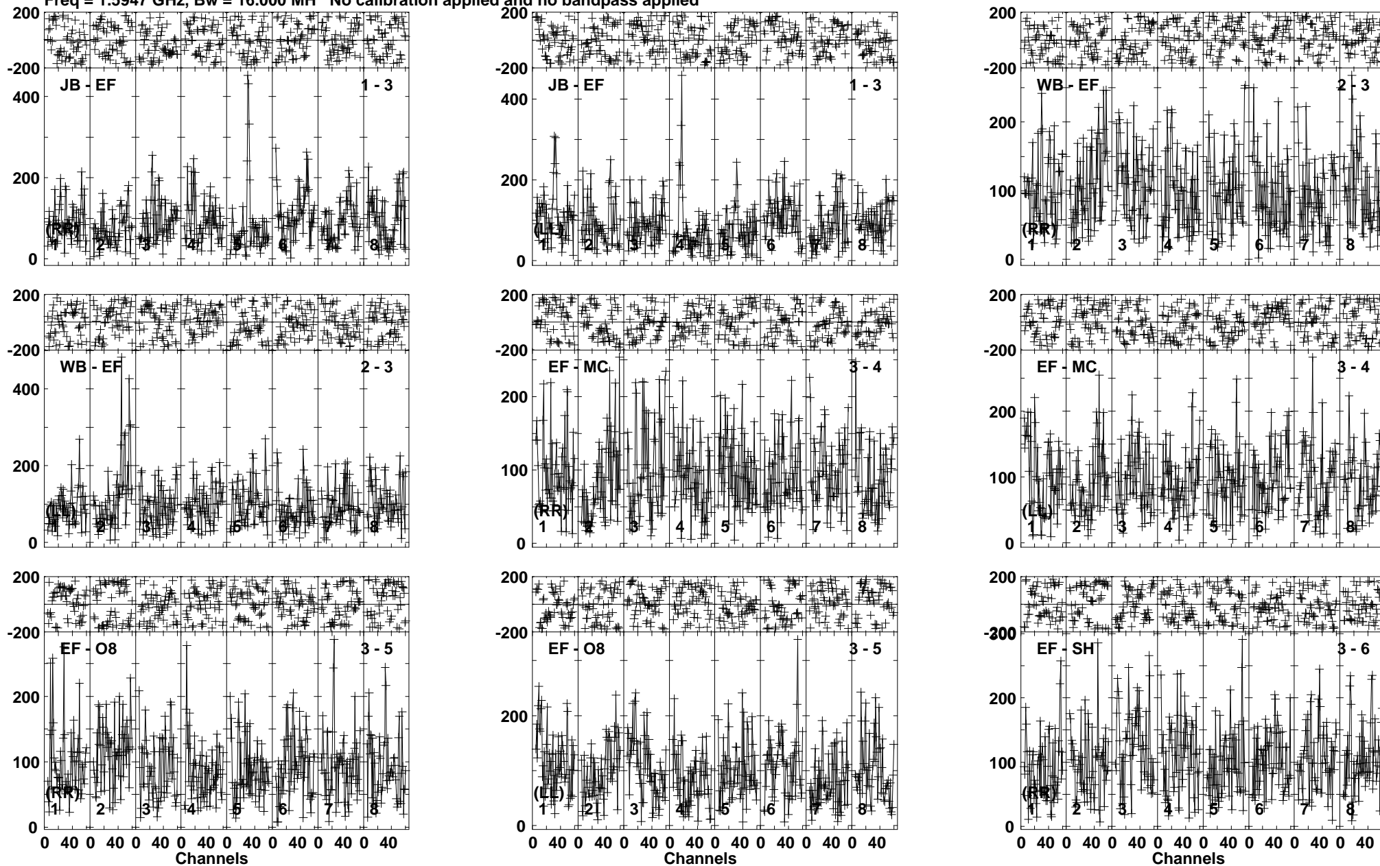
Lower frame: Micro Ampl Jy Top frame: Phas deg Vector averaged cross-power spectrum Baseline: JB (01) - EF (03) Timerange: 00/16:27:31 to 00/16:31:59
