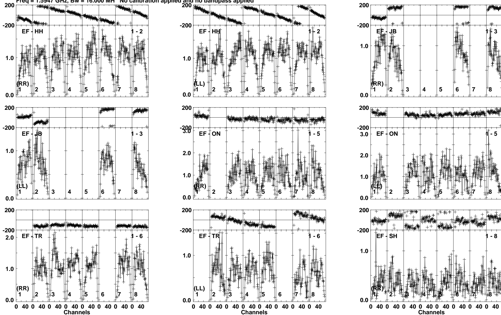
Lower frame: Milli Ampl Jy Top frame: Phas deg Vector averaged cross-power spectrum Baseline: EF (01) - HH (02) Timerange: 00/17:24:12 to 00/17:24:58
