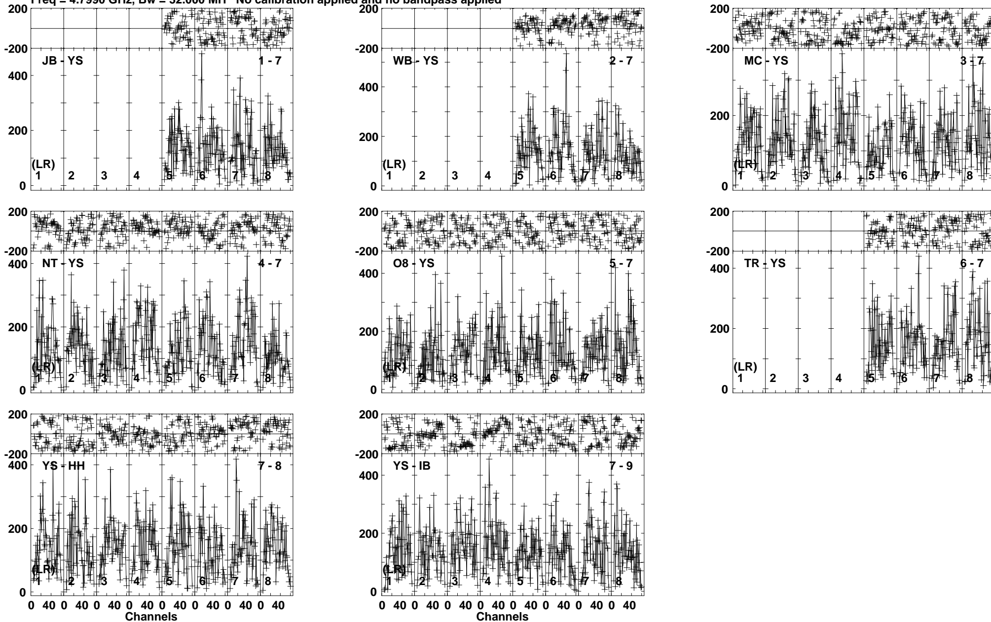
Lower frame: Micro Ampl Jy Top frame: Phas deg Vector averaged cross-power spectrum Baseline: JB (01) - YS (07) Timerange: 00/23:12:10 to 00/23:13:30
