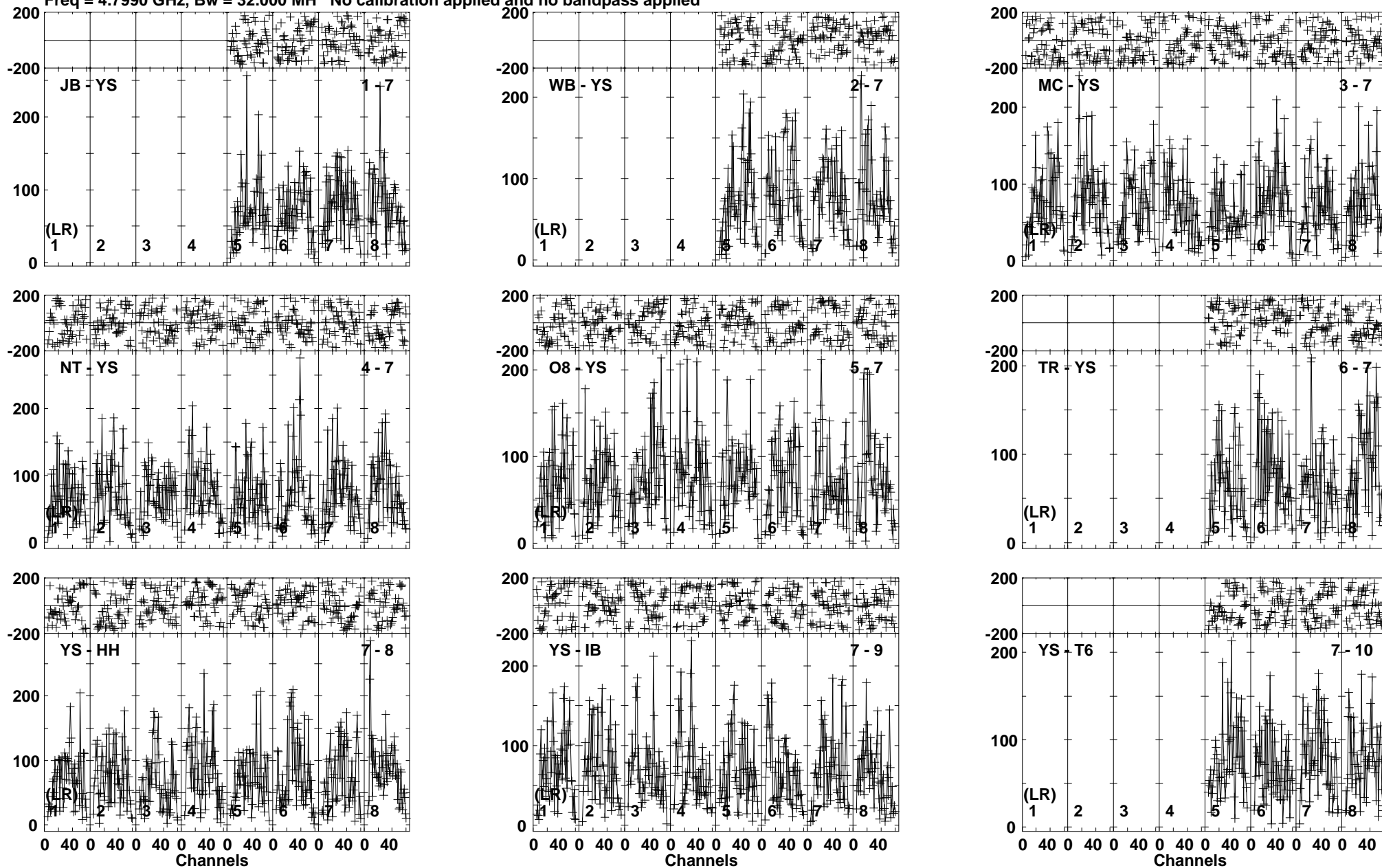
Lower frame: Micro Ampl Jy Top frame: Phas deg Vector averaged cross-power spectrum Baseline: JB (01) - YS (07) Timerange: 00/21:54:30 to 00/21:59:00
