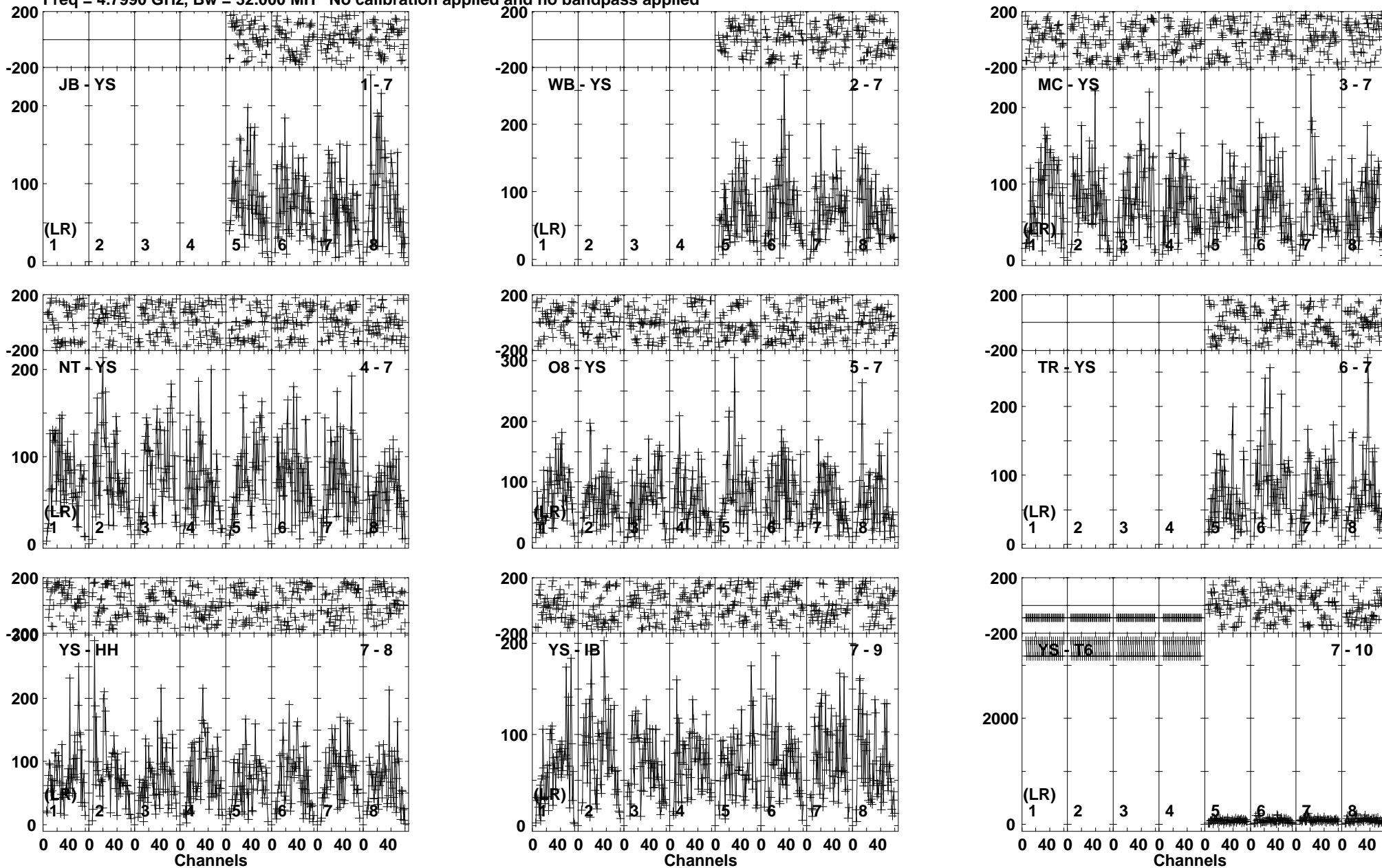
Lower frame: Micro Ampl Jy Top frame: Phas deg Vector averaged cross-power spectrum Baseline: JB (01) - YS (07) Timerange: 00:22:00:30 to 00:22:05:00
