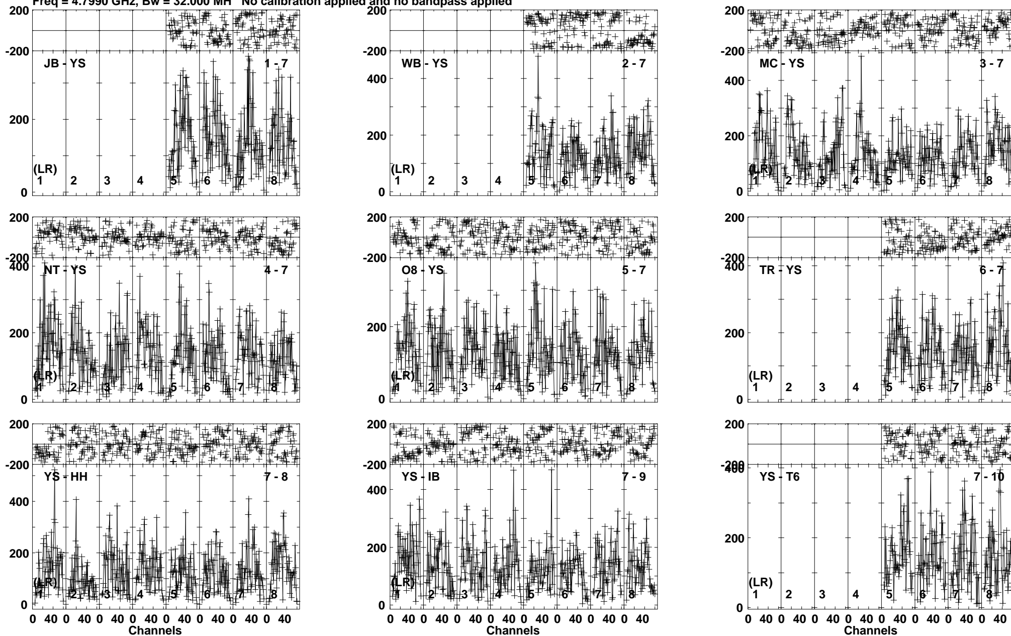
Lower frame: Micro Ampl Jy Top frame: Phas deg Vector averaged cross-power spectrum Baseline: JB (01) - YS (07) Timerange: 00/21:40:41 to 00/21:41:59
