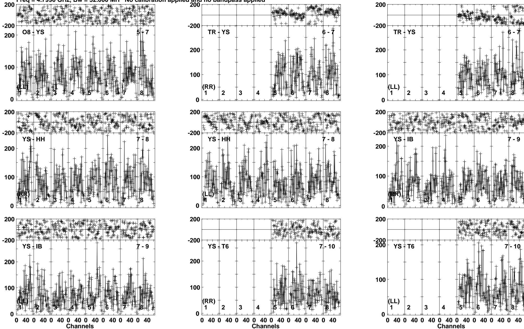
Lower frame: Micro Ampl Jy Top frame: Phas deg Vector averaged cross-power spectrum Baseline: O8 (05) - YS (07) Timerange: 00/21:29:30 to 00/21:34:00
