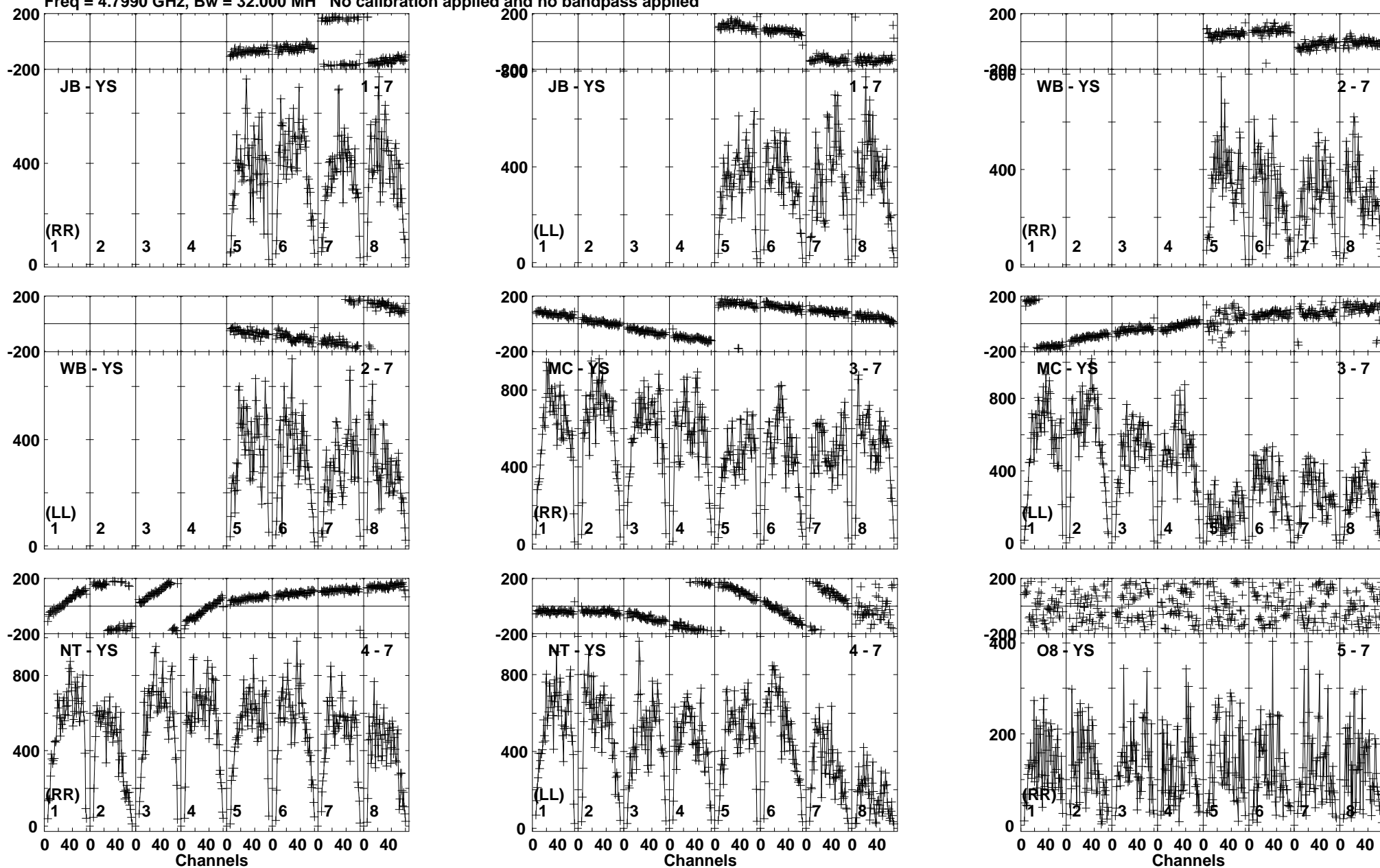
Lower frame: Micro Ampl Jy Top frame: Phas deg Vector averaged cross-power spectrum Baseline: JB (01) - YS (07) Timerange: 00/22:34:41 to 00/22:36:00
