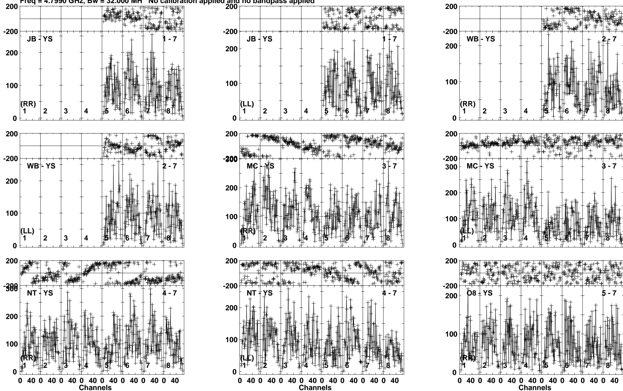
Lower frame: Micro Ampl Jy Top frame: Phas deg Vector averaged cross-power spectrum Baseline: JB (01) - YS (07) Timerange: 00/23:44:30 to 00/23:49:00
