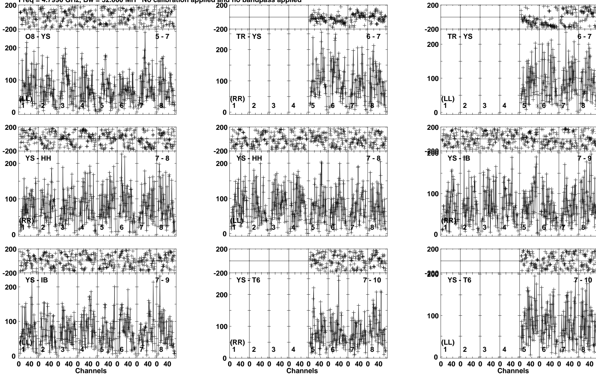
Lower frame: Micro Ampl Jy Top frame: Phas deg Vector averaged cross-power spectrum Baseline: O8 (05) - YS (07) Timerange: 00/21:17:00 to 00/21:21:29
