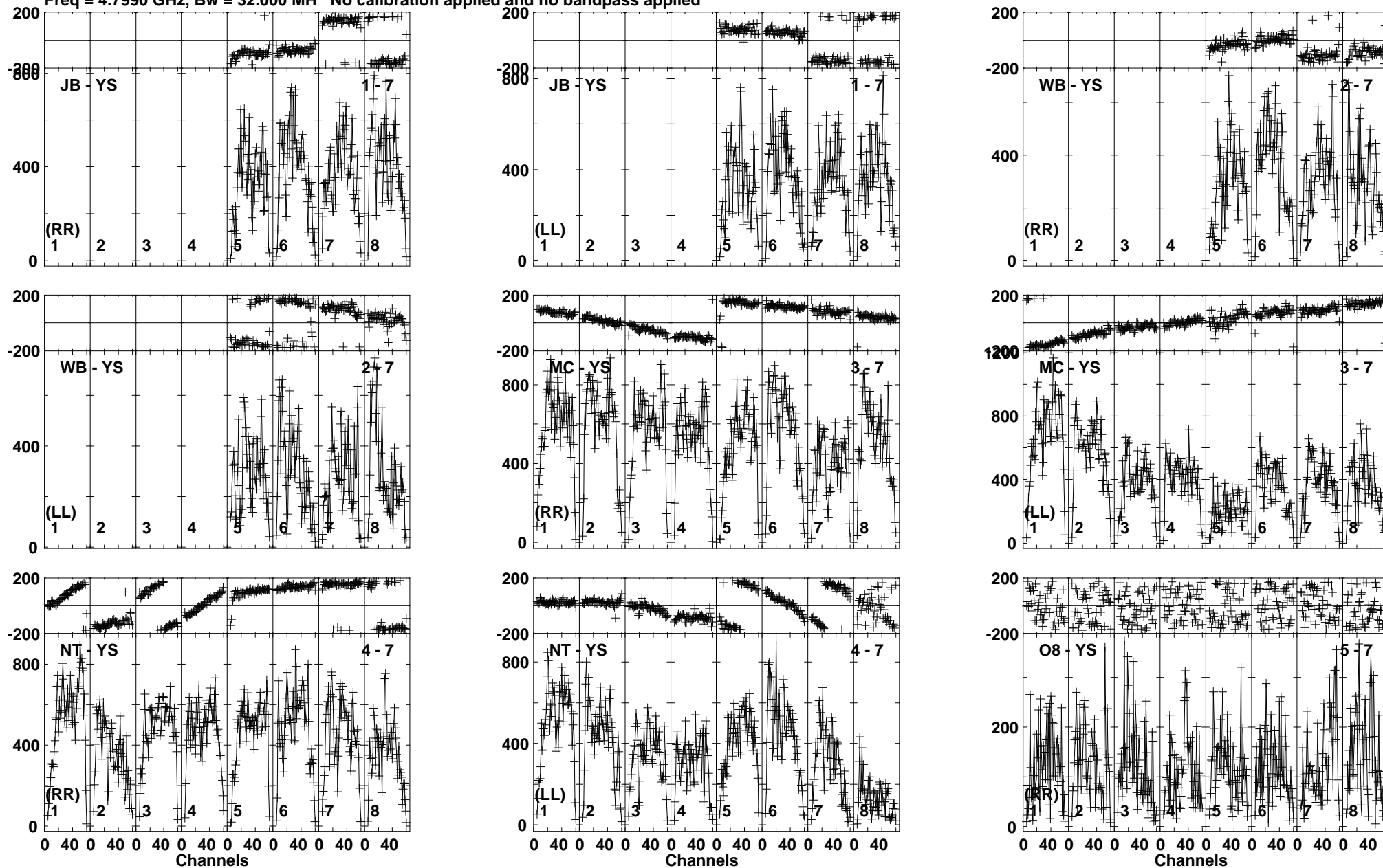
Lower frame: Micro Ampl Jy Top frame: Phas deg Vector averaged cross-power spectrum Baseline: JB (01) - YS (07) Timerange: 00/22:53:01 to 00/22:54:30
