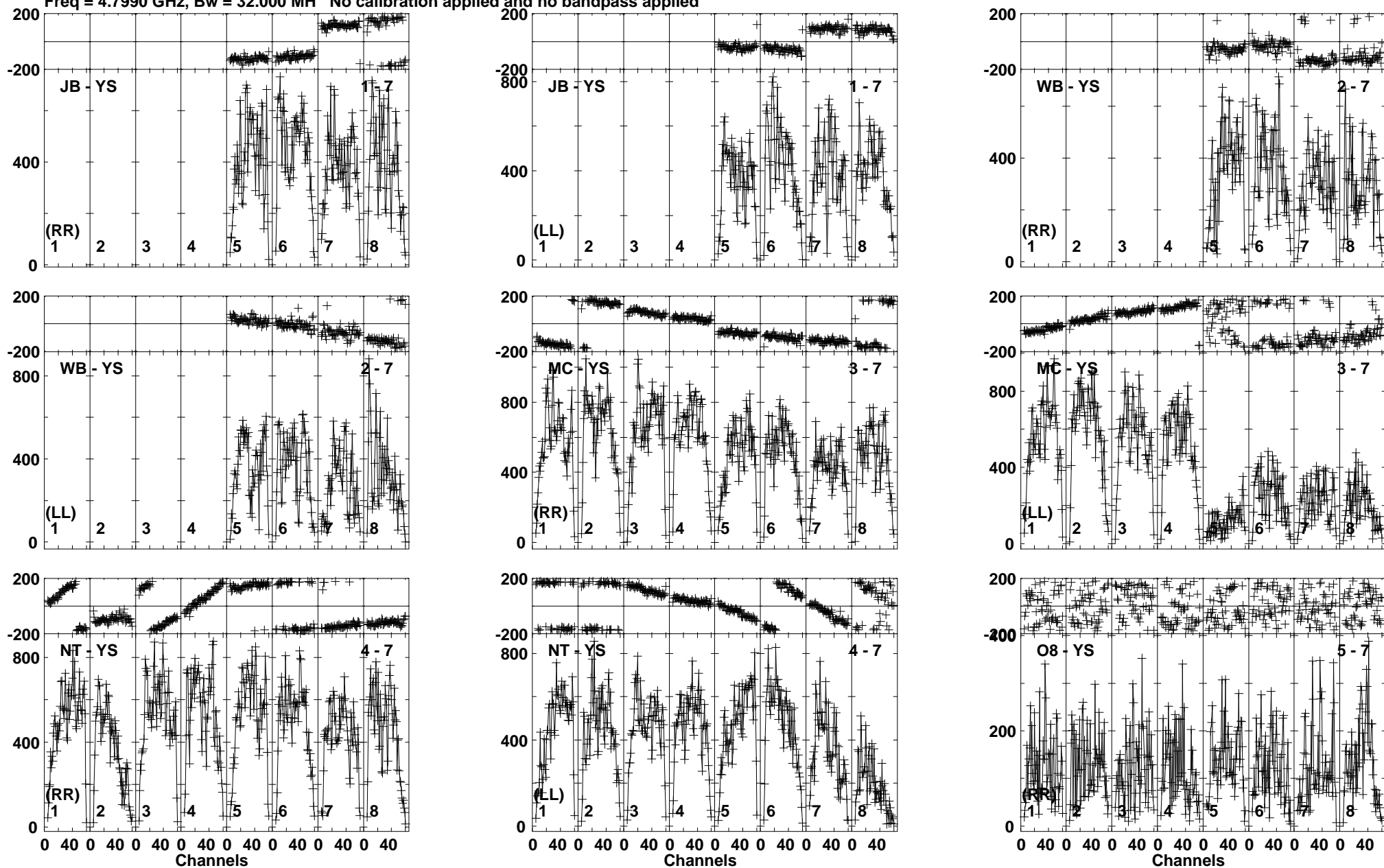
Lower frame: Micro Ampl Jy Top frame: Phas deg Vector averaged cross-power spectrum Baseline: JB (01) - YS (07) Timerange: 01/00:27:11 to 01/00:28:39
