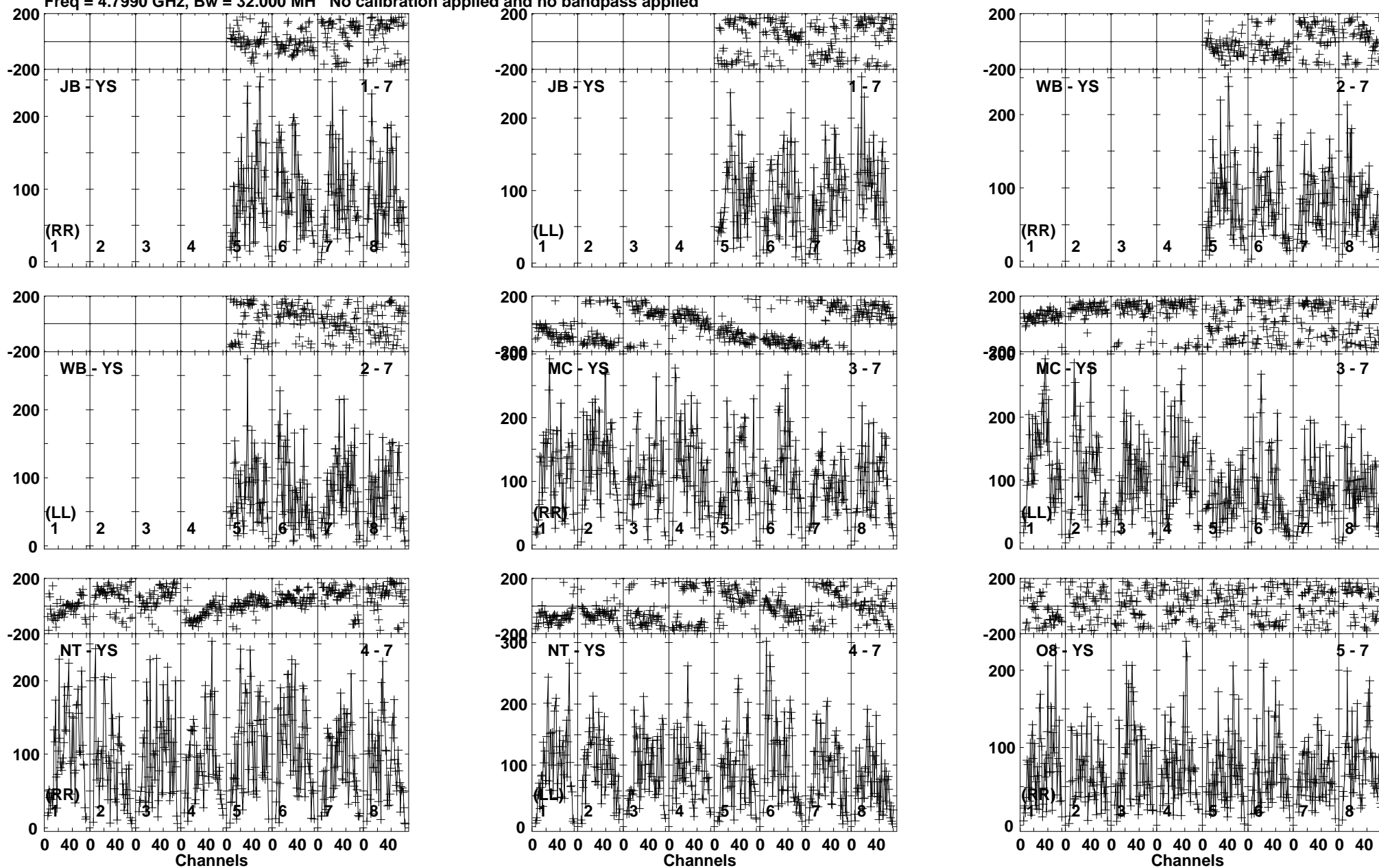
Lower frame: Micro Ampl Jy Top frame: Phas deg Vector averaged cross-power spectrum Baseline: JB (01) - YS (07) Timerange: 00:22:42:00 to 00:22:46:29
