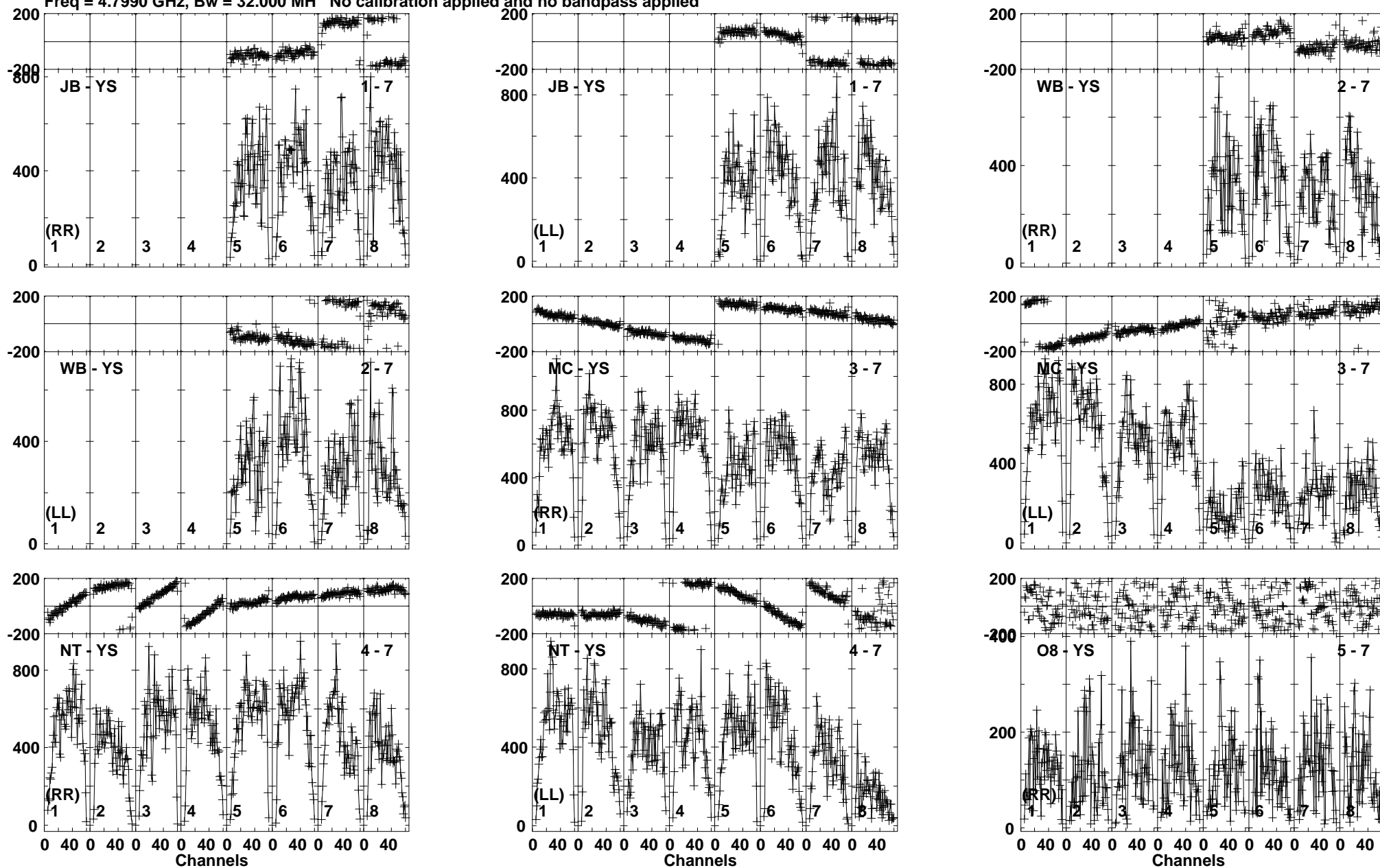
Lower frame: Micro Ampl Jy Top frame: Phas deg Vector averaged cross-power spectrum Baseline: JB (01) - YS (07) Timerange: 00/22:40:30 to 00/22:42:00
