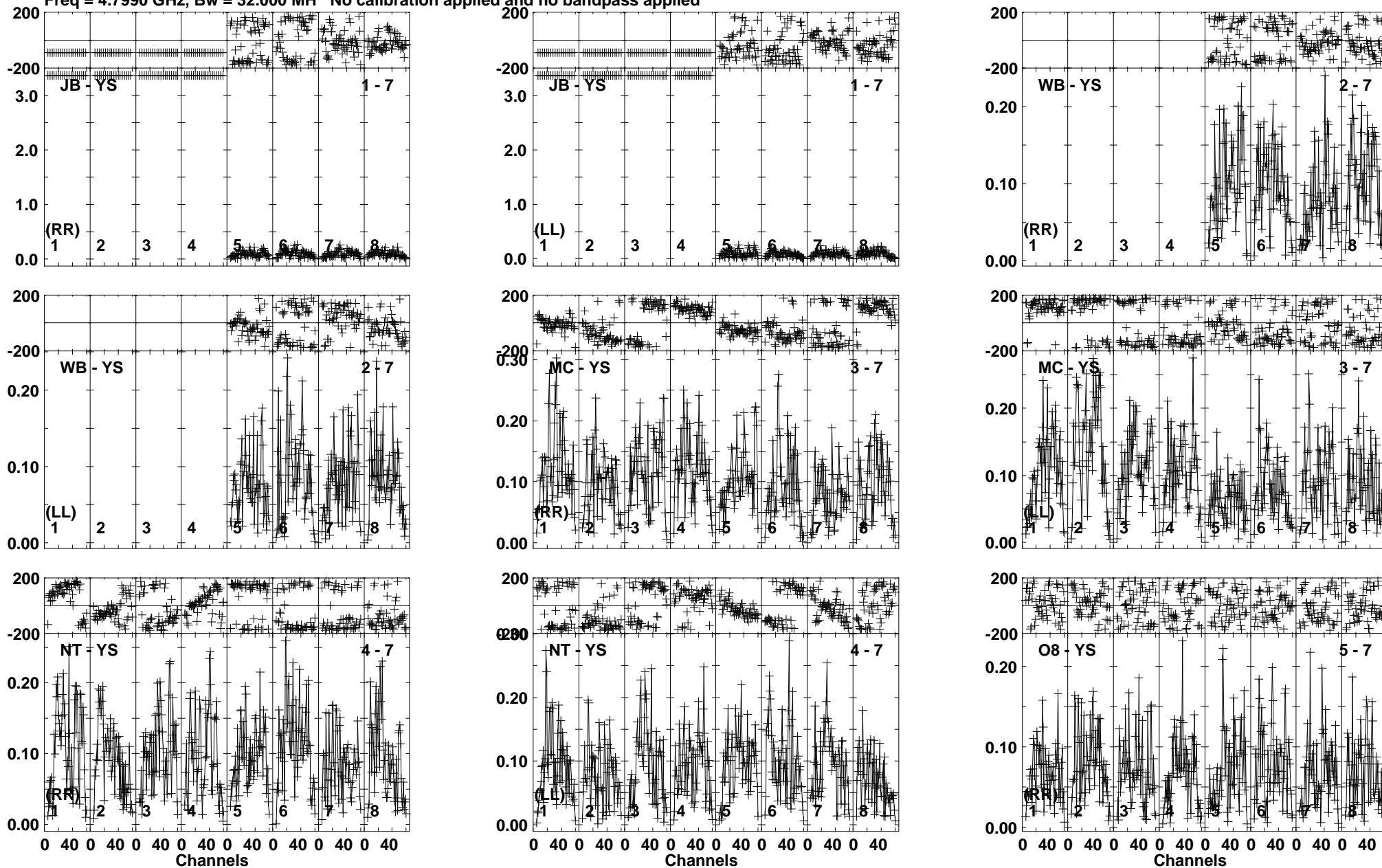
Lower frame: Milli Ampl Jy Top frame: Phas deg Vector averaged cross-power spectrum Baseline: JB (01) - YS (07) Timerange: 01/00:03:31 to 01/00:07:59
