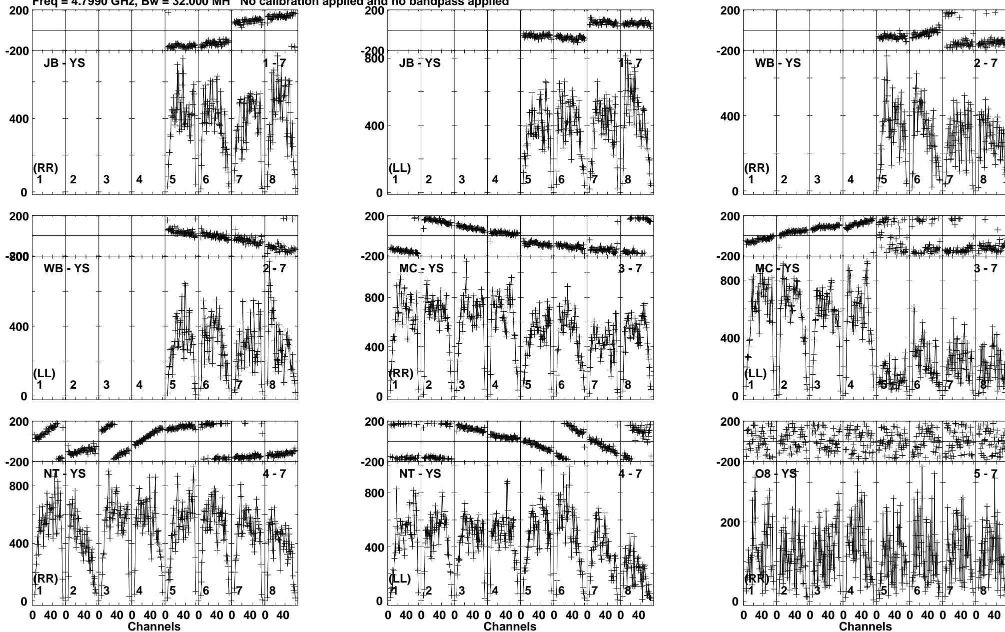
Lower frame: Micro Ampl Jy Top frame: Phas deg Vector averaged cross-power spectrum Baseline: JB (01) - YS (07) Timerange: 01/00:21:11 to 01/00:22:39
