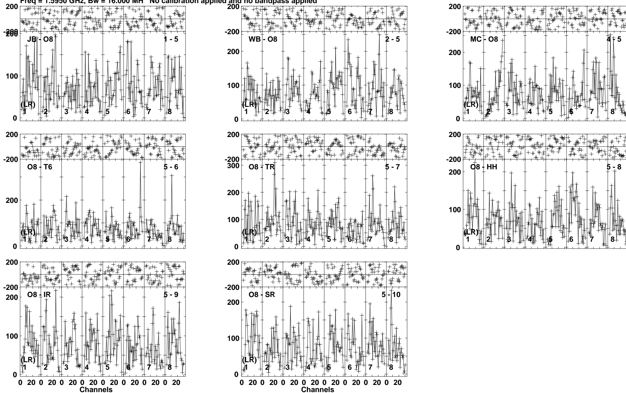
Lower frame: Micro Ampl Jy Top frame: Phas deg Vector averaged cross-power spectrum Baseline: JB (01) - O8 (05) Timerange: 00/21:08:21 to 00/21:13:19
