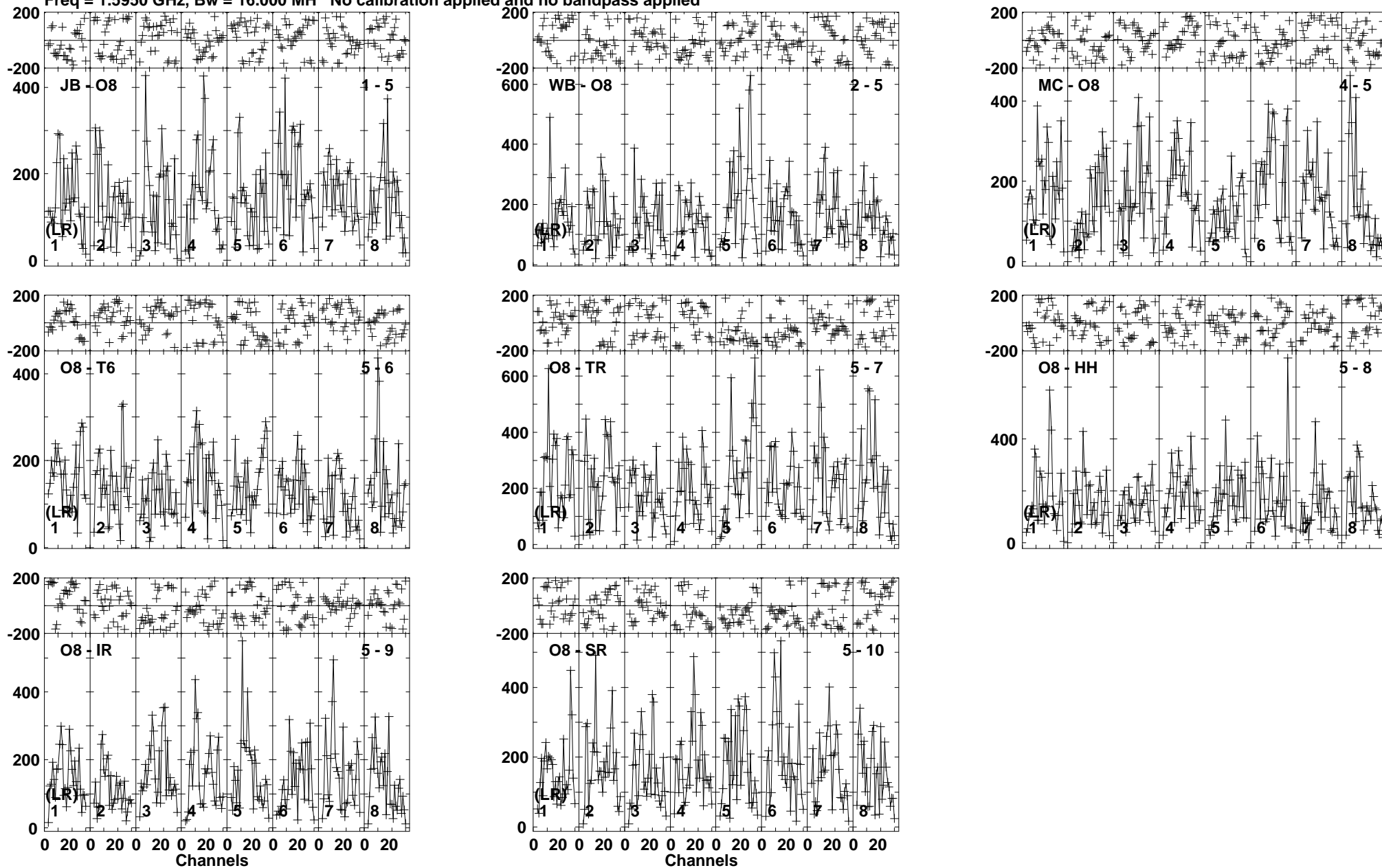
Lower frame: Micro Ampl Jy Top frame: Phas deg Vector averaged cross-power spectrum Baseline: JB (01) - O8 (05) Timerange: 00/21:21:01 to 00/21:22:29
