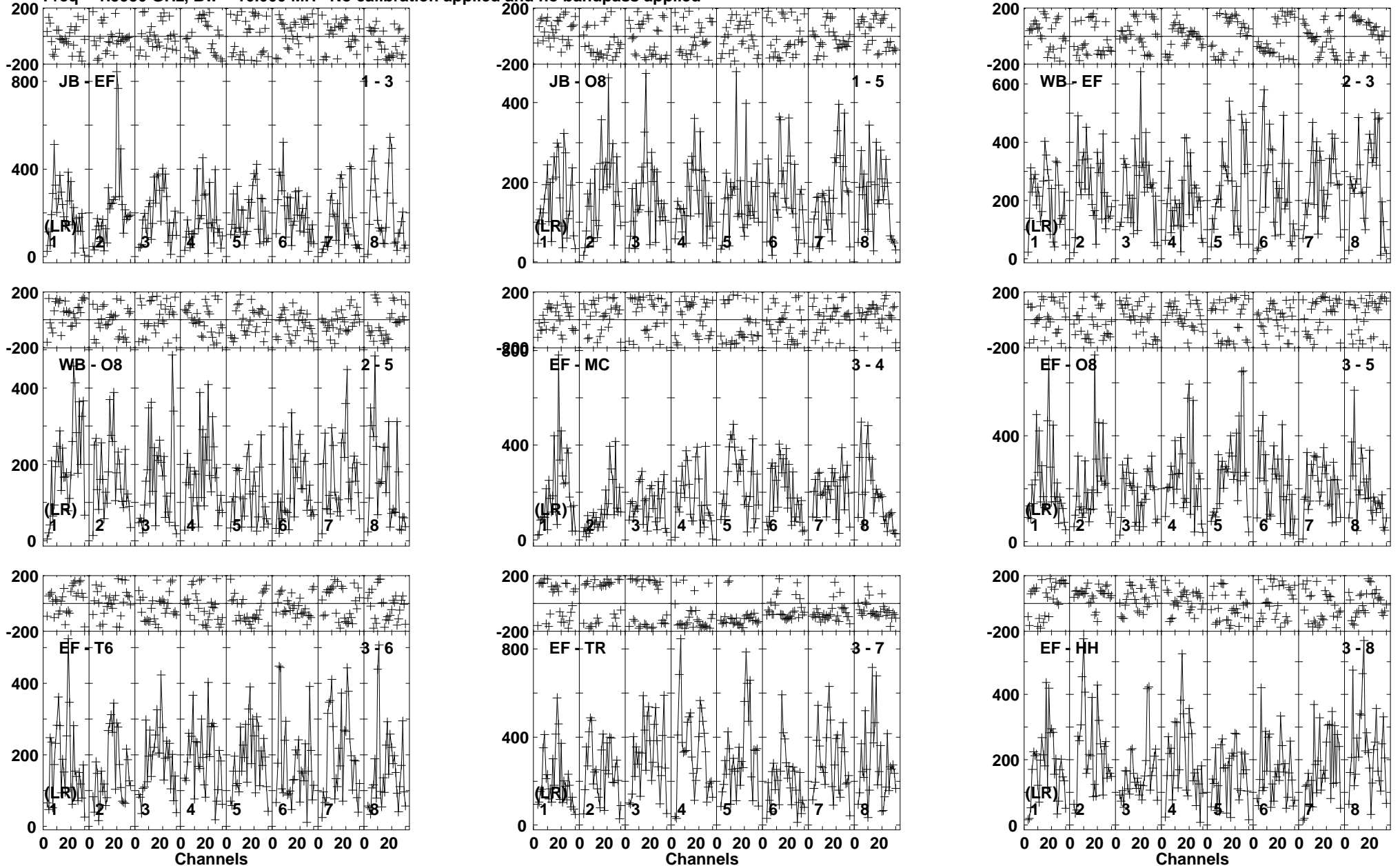
Lower frame: Micro Ampl Jy Top frame: Phas deg Vector averaged cross-power spectrum Baseline: JB (01) - EF (03) Timerange: 00/20:27:21 to 00/20:28:49
