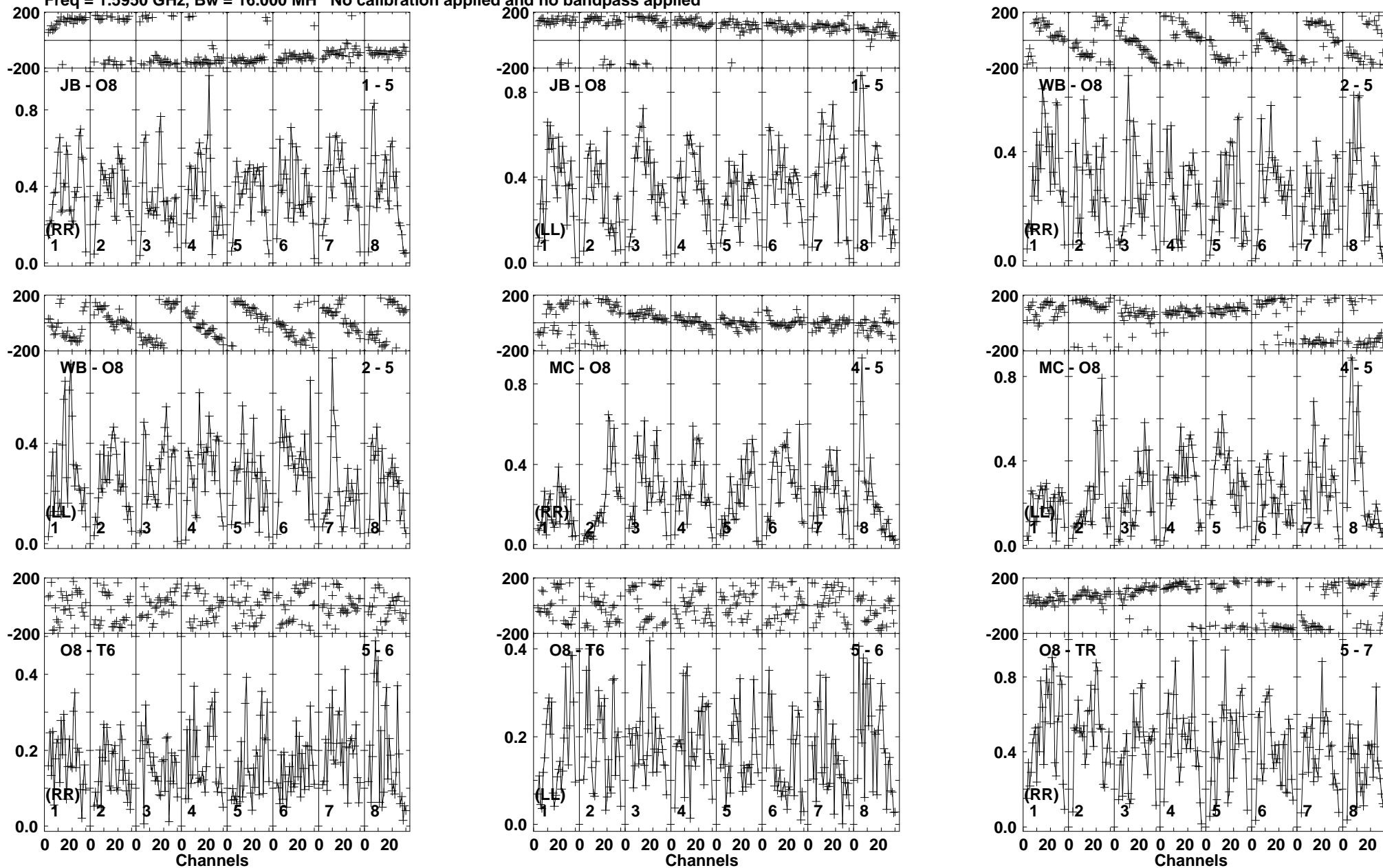
Lower frame: Milli Ampl Jy Top frame: Phas deg Vector averaged cross-power spectrum Baseline: JB (01) - O8 (05) Timerange: 00/20:40:01 to 00/20:41:29
