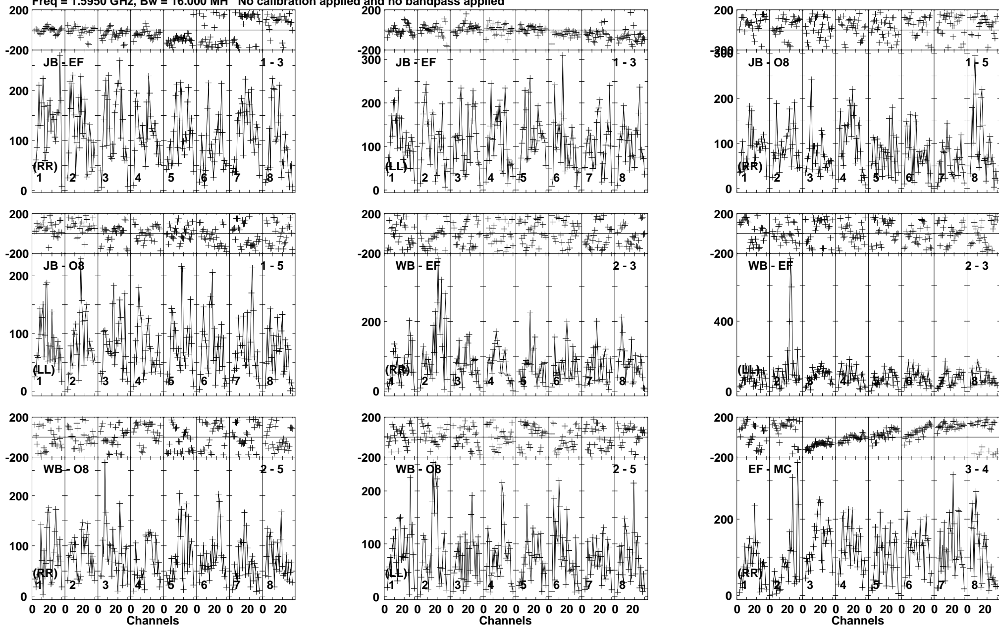
Lower frame: Micro Ampl Jy Top frame: Phas deg Vector averaged cross-power spectrum Baseline: JB (01) - EF (03) Timerange: 00/20:14:41 to 00/20:19:39
