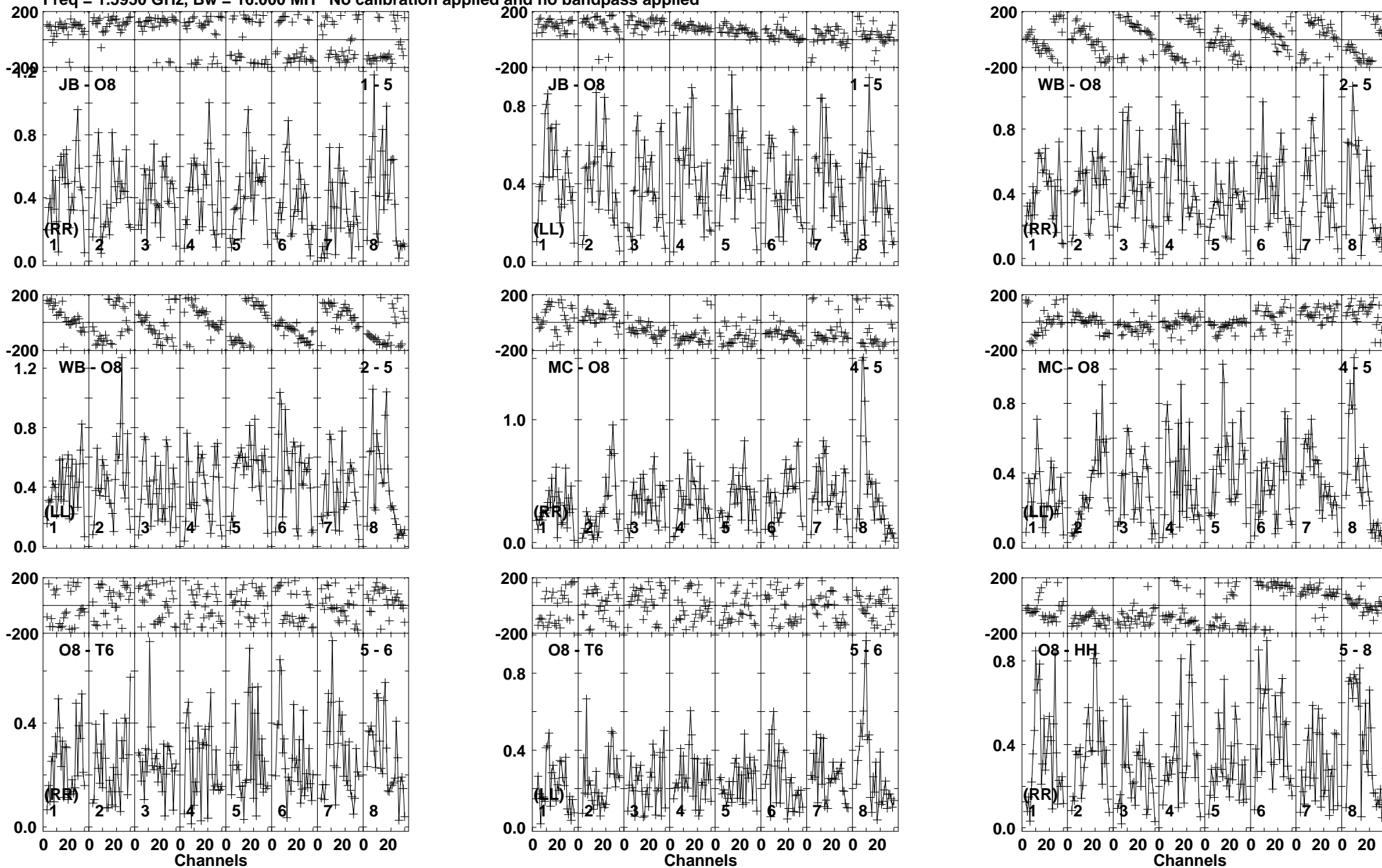
Lower frame: Milli Ampl Jy Top frame: Phas deg Vector averaged cross-power spectrum Baseline: JB (01) - O8 (05) Timerange: 00/20:54:11 to 00/20:55:39
