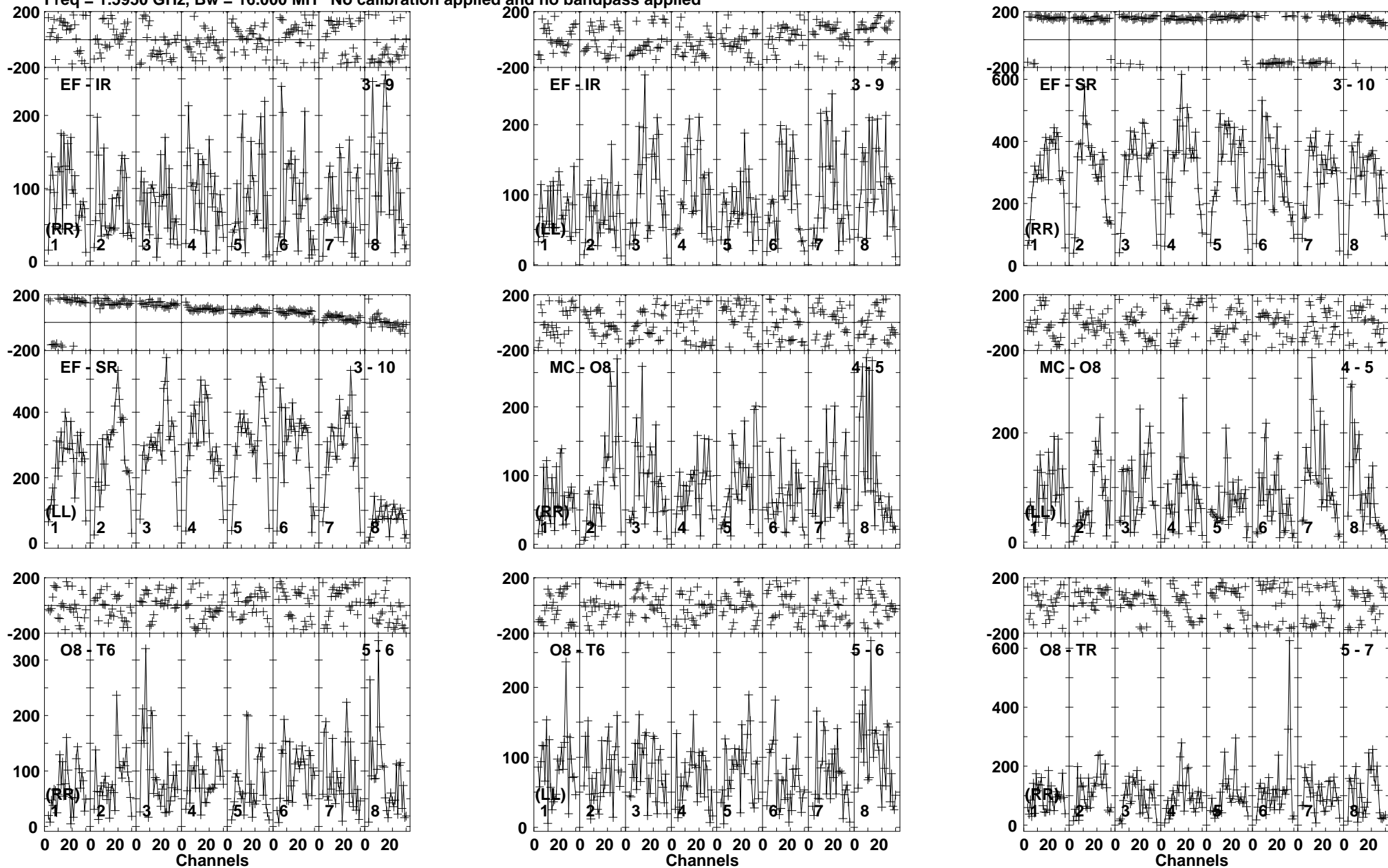
Lower frame: Micro Ampl Jy Top frame: Phas deg Vector averaged cross-power spectrum Baseline: EF (03) - IR (09) Timerange: 00/20:23:51 to 00/20:27:19
