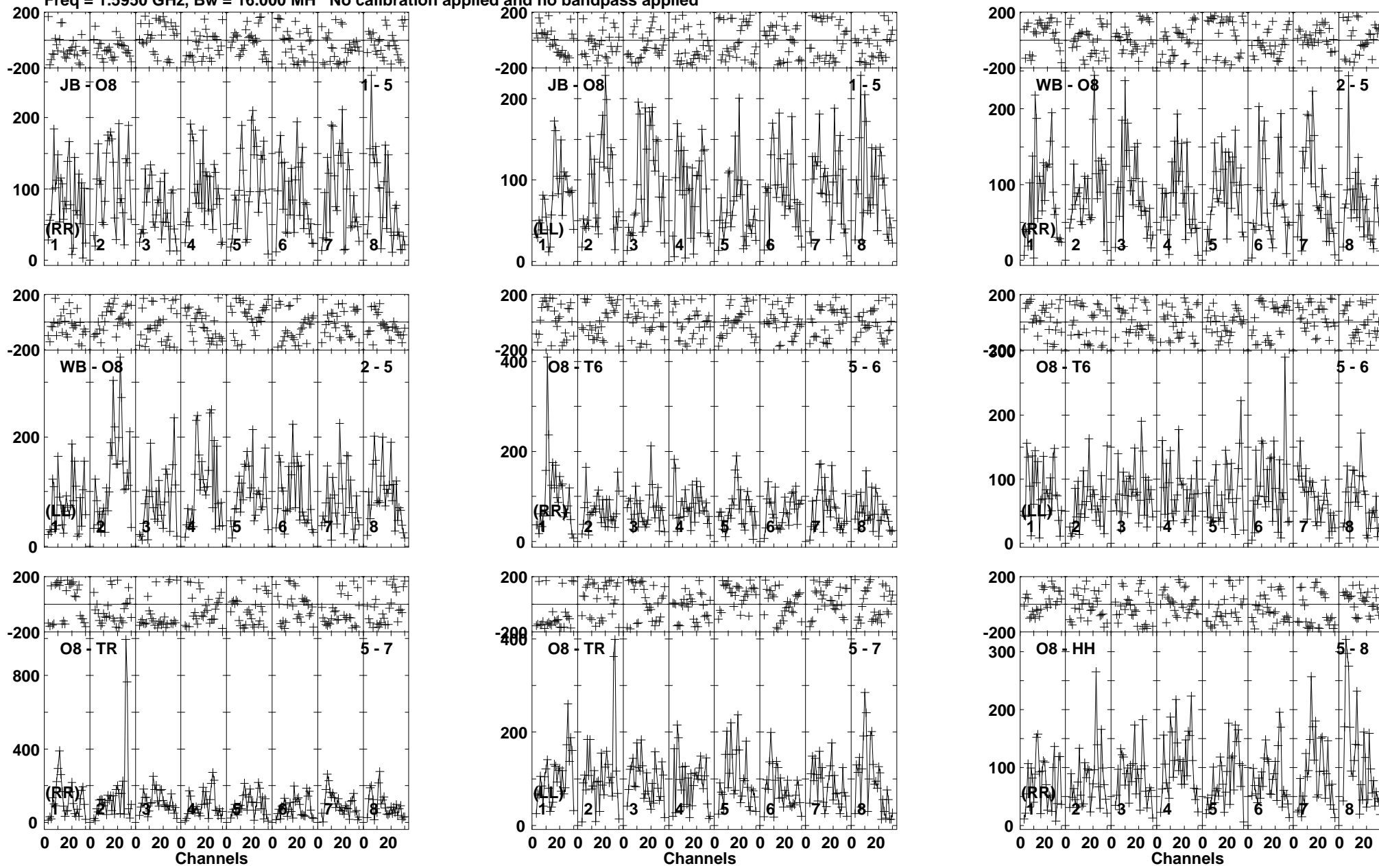
Lower frame: Micro Ampl Jy Top frame: Phas deg Vector averaged cross-power spectrum Baseline: JB (01) - O8 (05) Timerange: 00/21:44:21 to 00/21:47:49
