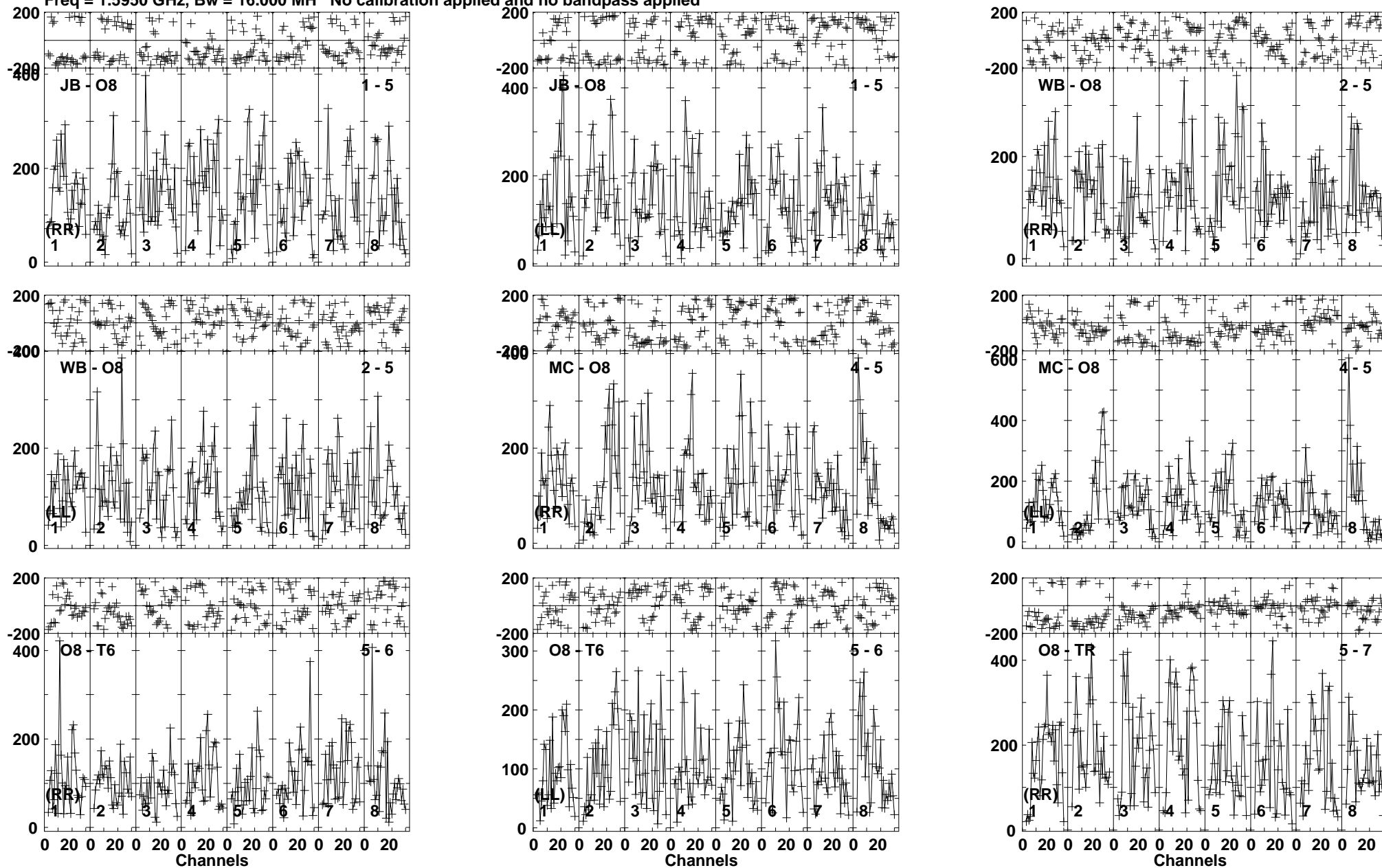
Lower frame: Micro Ampl Jy Top frame: Phas deg Vector averaged cross-power spectrum Baseline: JB (01) - O8 (05) Timerange: 00/20:48:41 to 00/20:50:39
