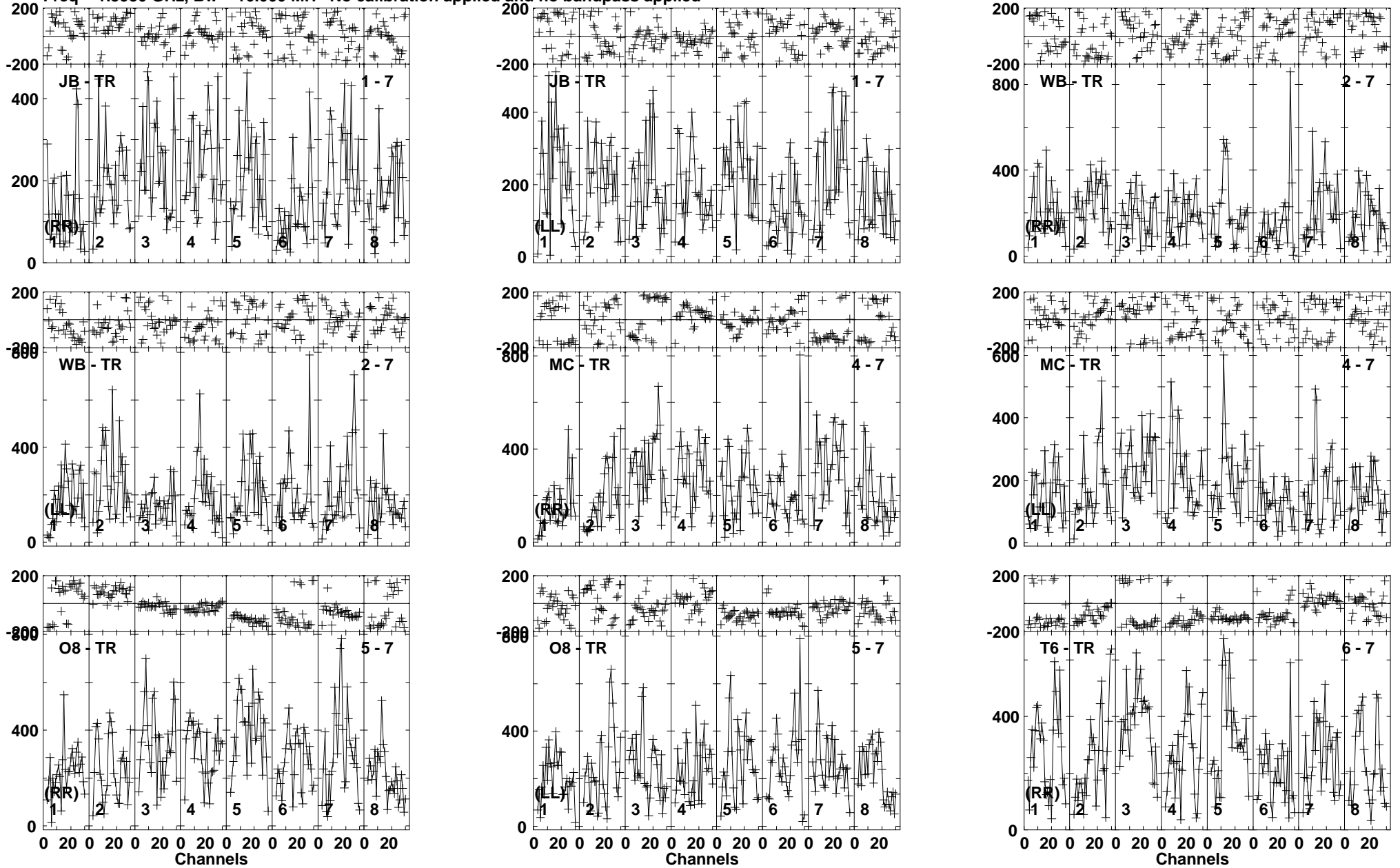
Lower frame: Micro Ampl Jy Top frame: Phas deg Vector averaged cross-power spectrum Baseline: JB (01) - TR (07) Timerange: 00/20:23:21 to 00/20:24:49
