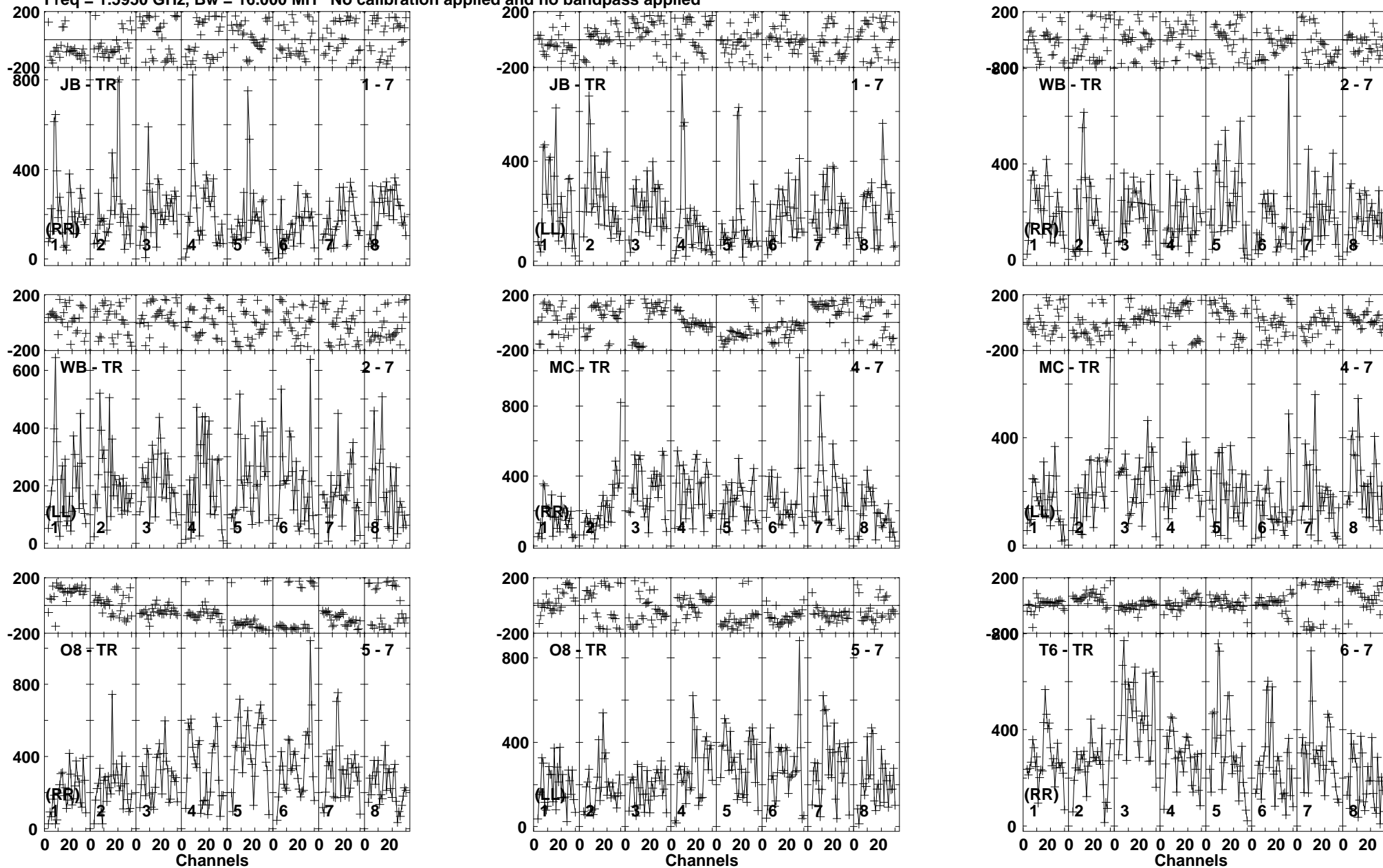
Lower frame: Micro Ampl Jy Top frame: Phas deg Vector averaged cross-power spectrum Baseline: JB (01) - TR (07) Timerange: 00/19:43:51 to 00/19:45:19
