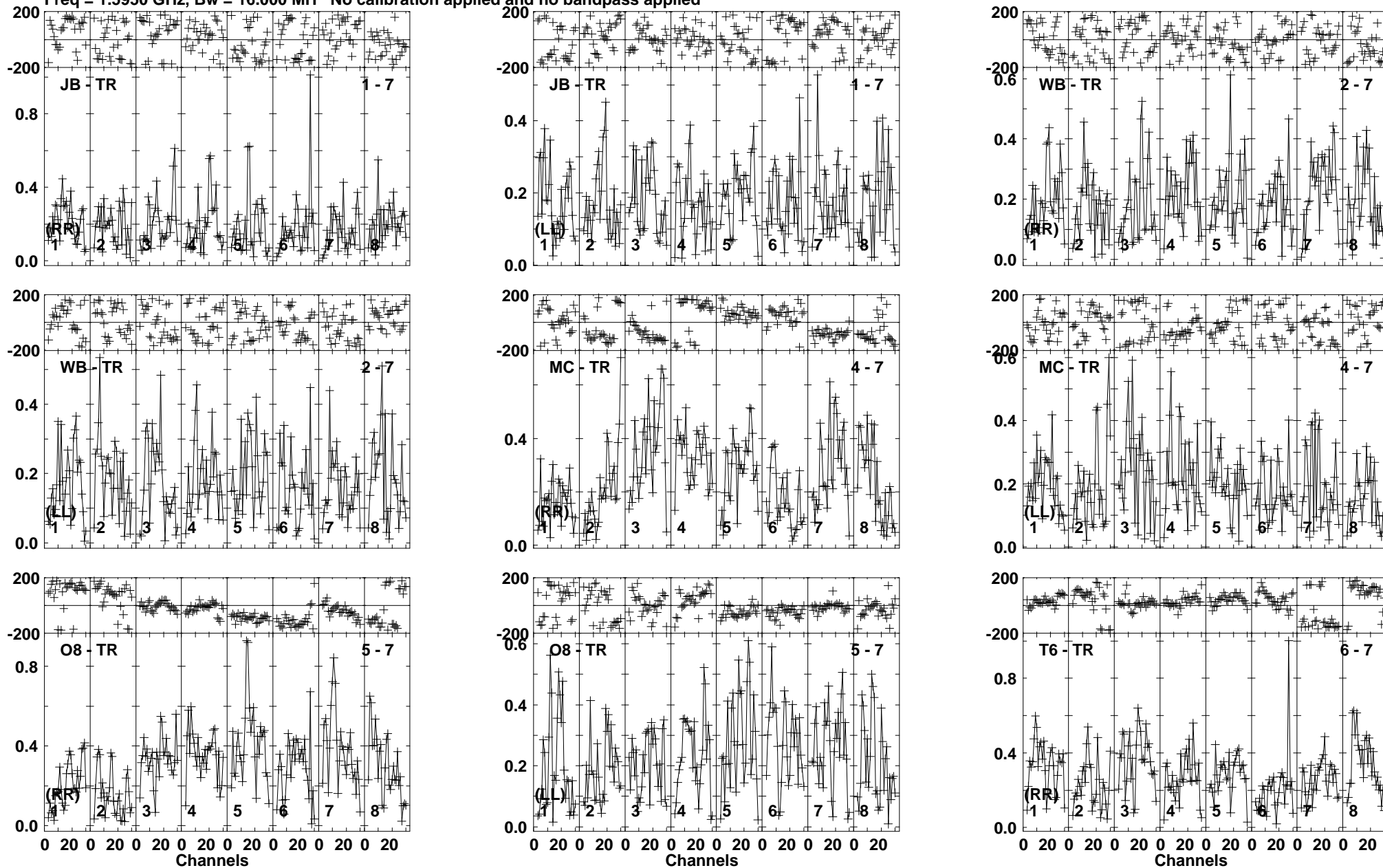
Lower frame: Milli Ampl Jy Top frame: Phas deg Vector averaged cross-power spectrum Baseline: JB (01) - TR (07) Timerange: 00/20:10:41 to 00/20:12:09
