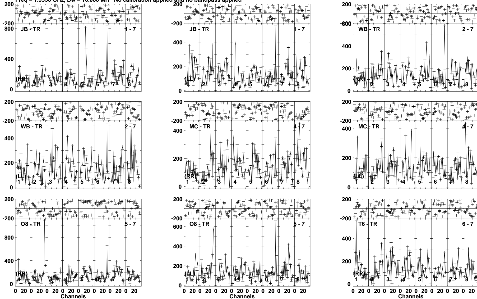
Lower frame: Micro Ampl Jy Top frame: Phas deg Vector averaged cross-power spectrum Baseline: JB (01) - TR (07) Timerange: 00:19:38:21 to 00:19:40:19
