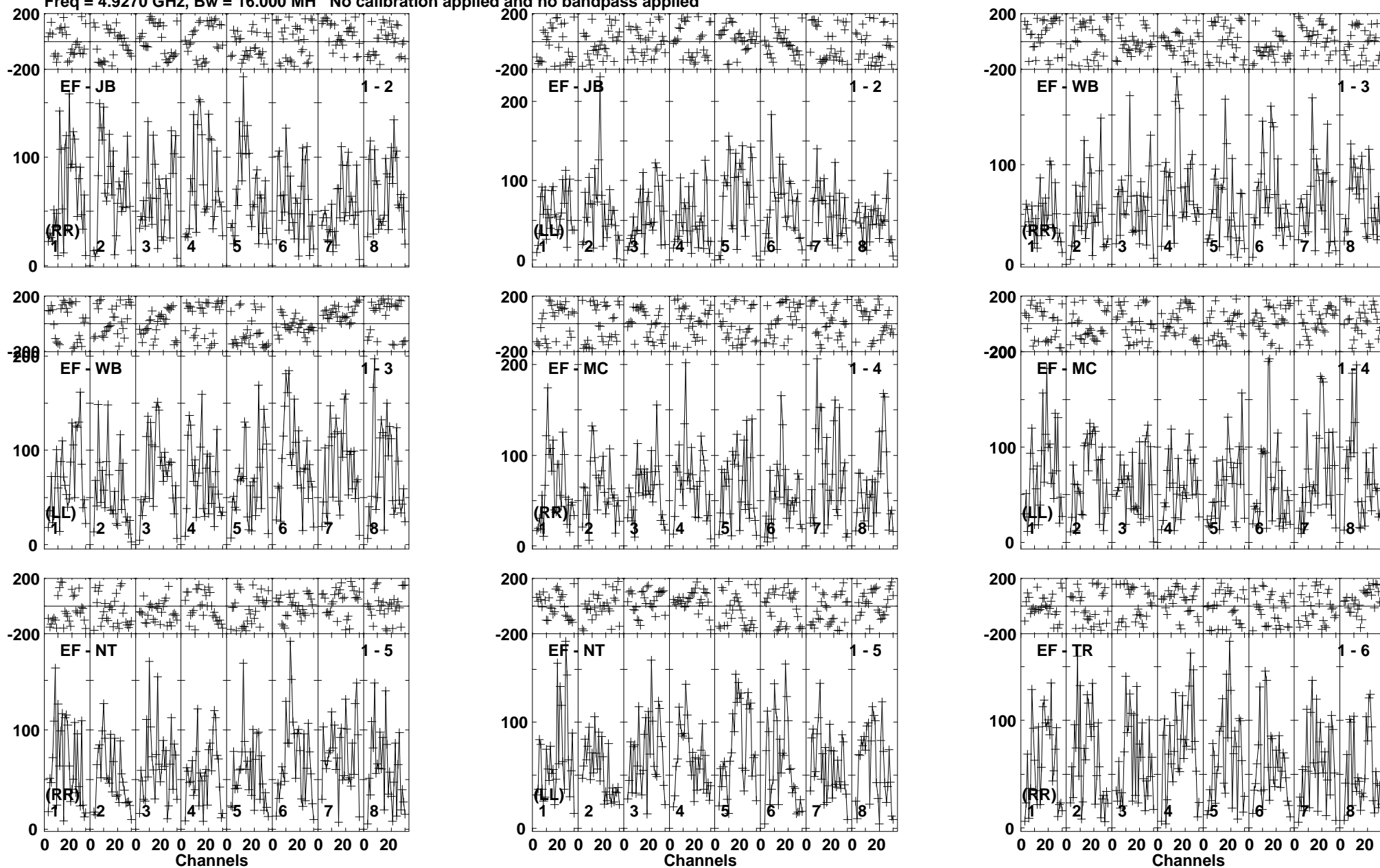
Lower frame: Micro Ampl Jy Top frame: Phas deg Vector averaged cross-power spectrum Baseline: EF (01) - JB (02) Timerange: 00/21:54:00 to 00/22:00:00
