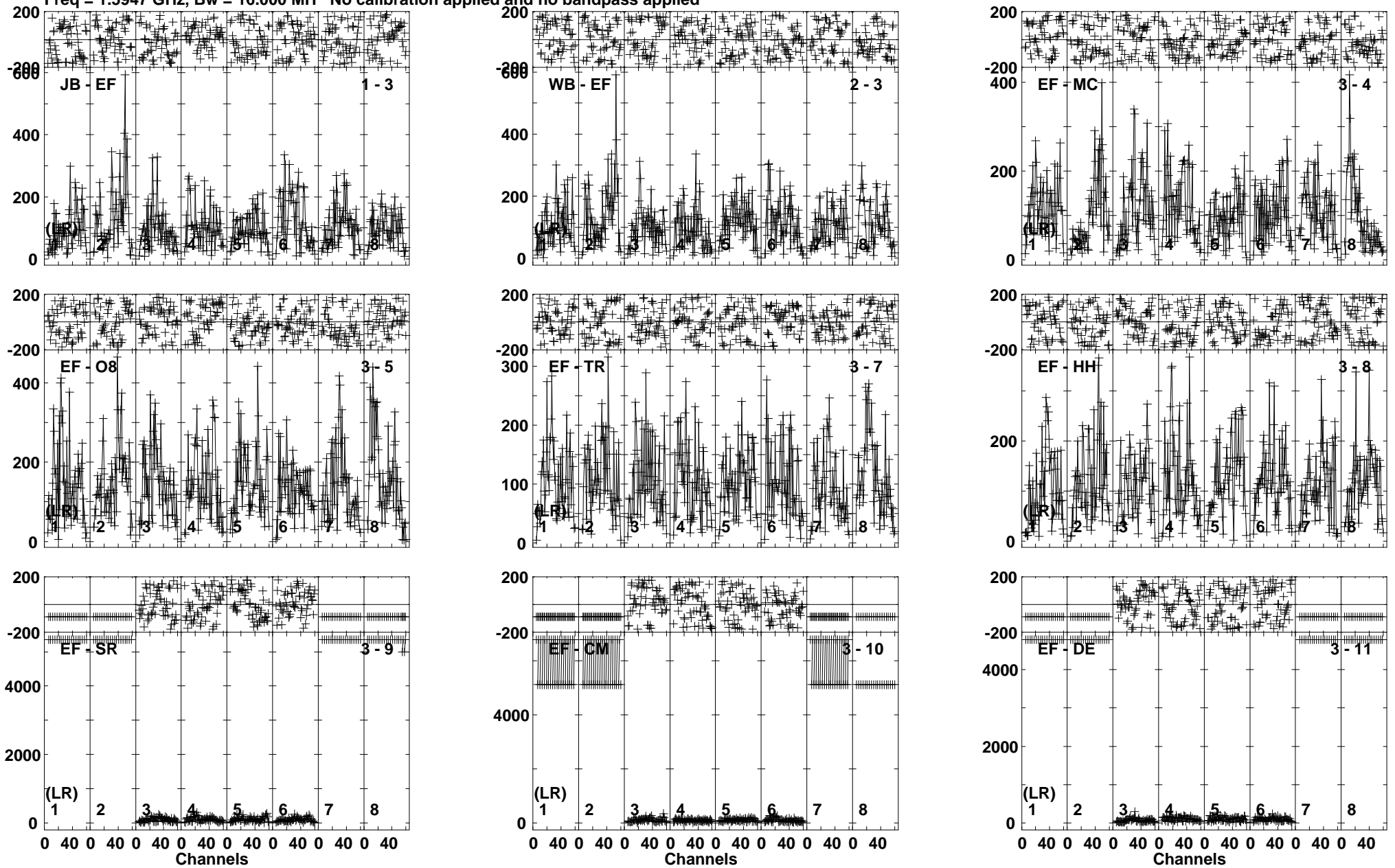
Lower frame: Micro Ampl Jy Top frame: Phas deg Vector averaged cross-power spectrum Baseline: JB (01) - EF (03) Timerange: 00/14:02:18 to 00/14:06:40
