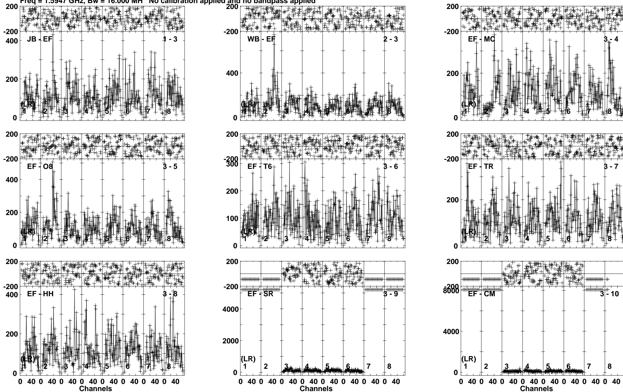
Lower frame: Micro Ampl Jy Top frame: Phas deg Vector averaged cross-power spectrum Baseline: JB (01) - EF (03) Timerange: 00:12:52:56 to 00:12:57:20
