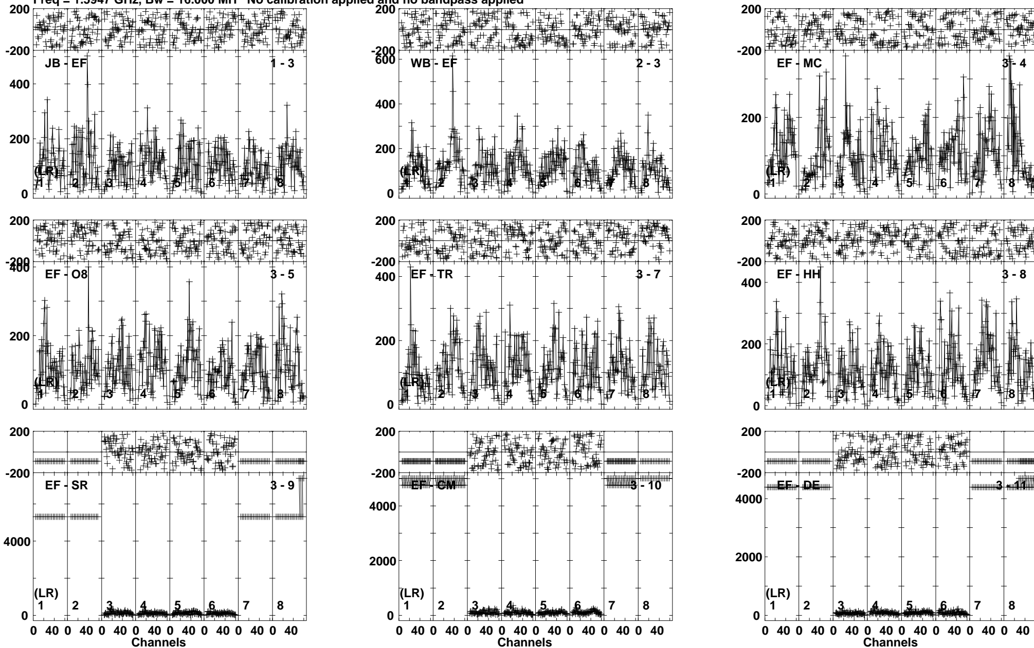
Lower frame: Micro Ampl Jy Top frame: Phas deg Vector averaged cross-power spectrum Baseline: JB (01) - EF (03) Timerange: 00/13:30:56 to 00/13:35:20
