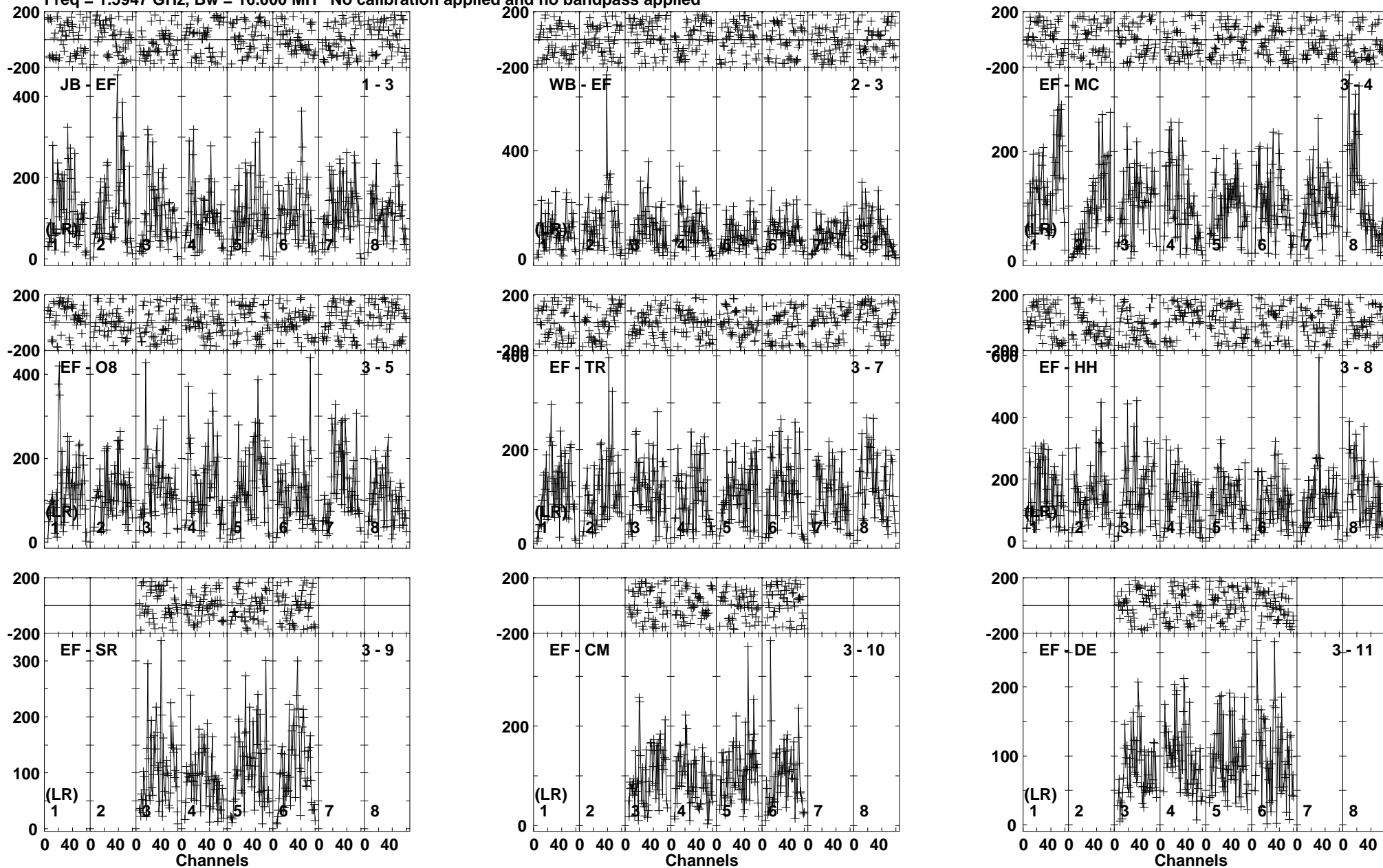
Lower frame: Micro Ampl Jy Top frame: Phas deg Vector averaged cross-power spectrum Baseline: JB (01) - EF (03) Timerange: 00/14:08:59 to 00/14:13:19
