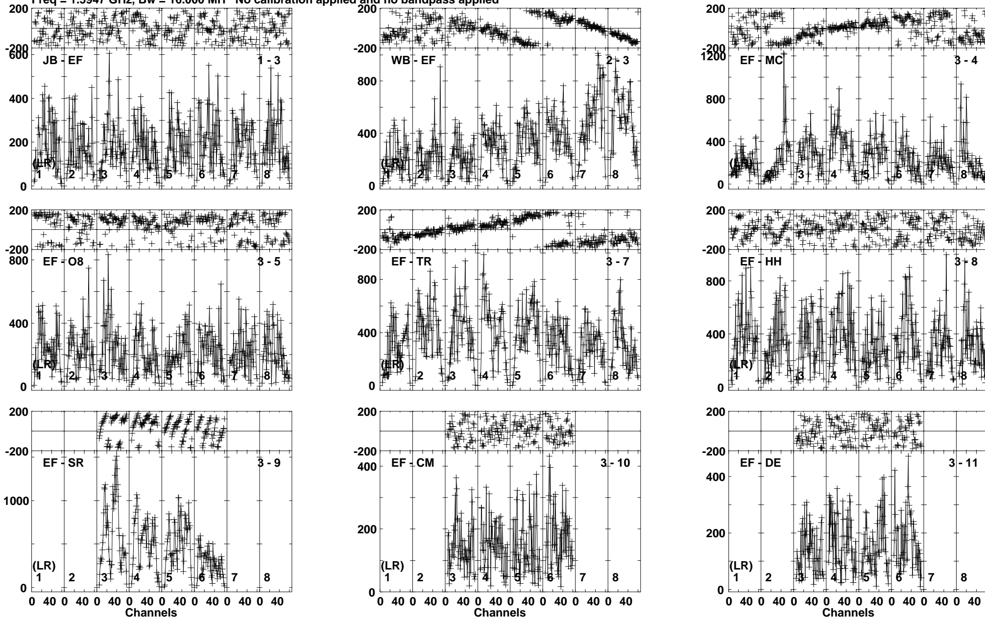
Lower frame: Micro Ampl Jy Top frame: Phas deg Vector averaged cross-power spectrum Baseline: JB (01) - EF (03) Timerange: 00/13:54:41 to 00/13:56:09
