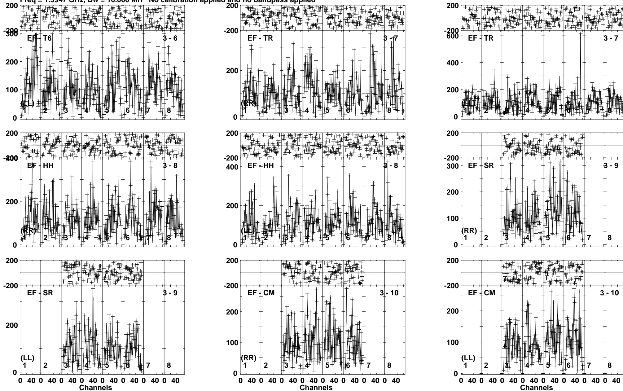
Lower frame: Micro Ampl Jy Top frame: Phas deg Vector averaged cross-power spectrum Baseline: EF (03) - T6 (06) Timerange: 00/12:58:56 to 00/13:03:20
