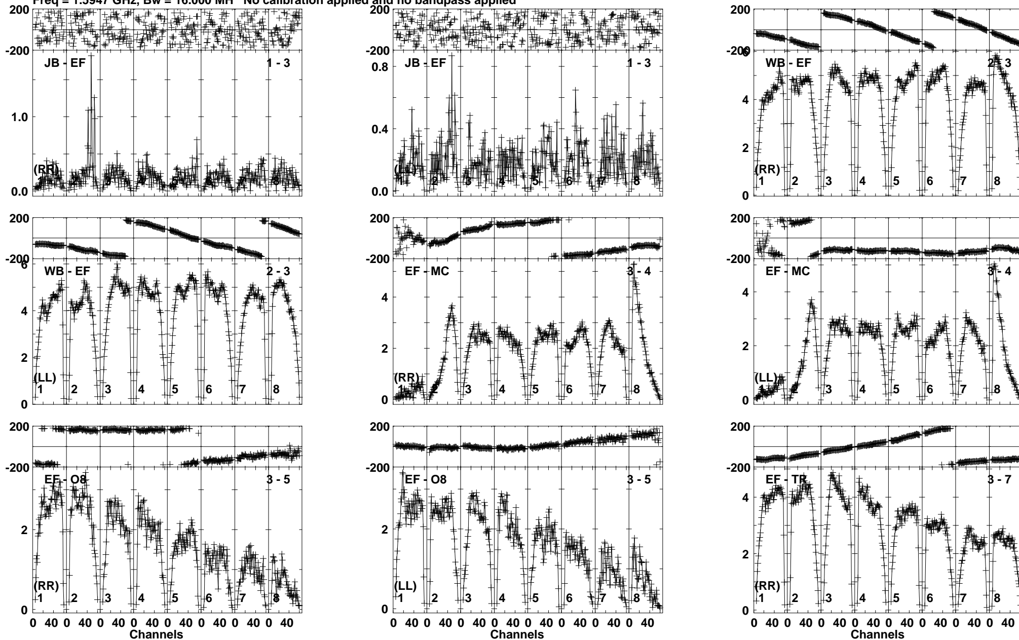
Lower frame: Milli Ampl Jy Top frame: Phas deg Vector averaged cross-power spectrum Baseline: JB (01) - EF (03) Timerange: 00/14:20:00 to 00/14:21:29
