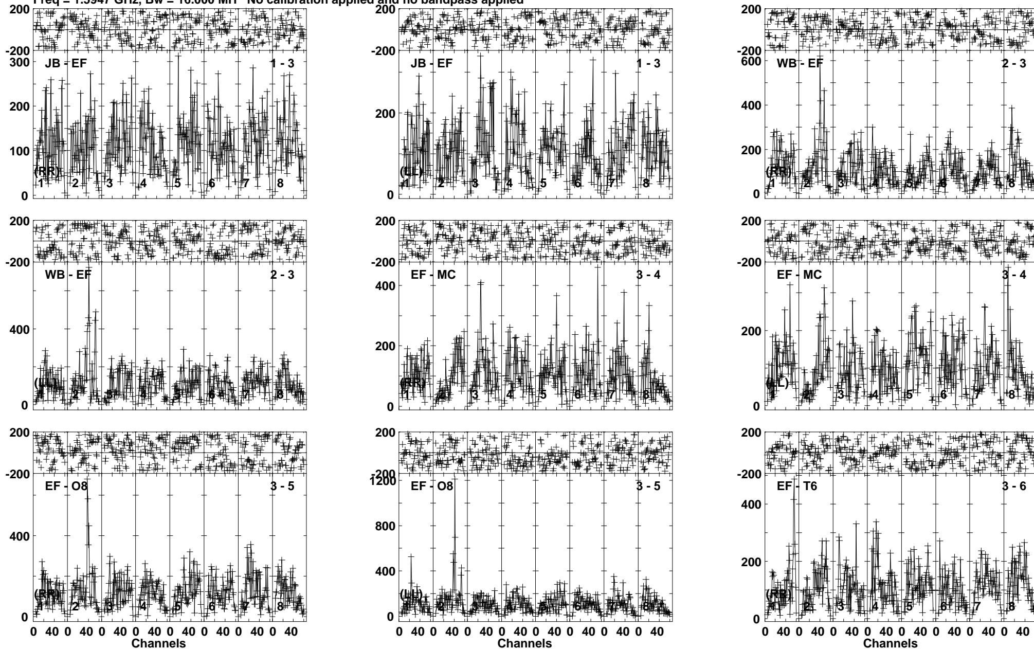
Lower frame: Micro Ampl Jy Top frame: Phas deg Vector averaged cross-power spectrum Baseline: JB (01) - EF (03) Timerange: 00/13:18:17 to 00/13:22:39
