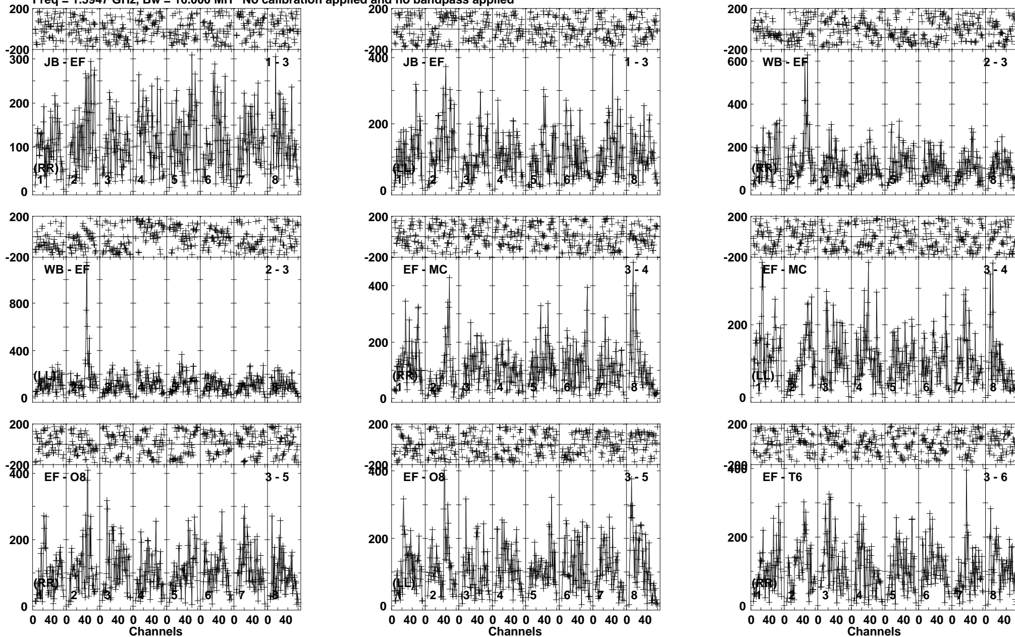
Lower frame: Micro Ampl Jy Top frame: Phas deg Vector averaged cross-power spectrum Baseline: JB (01) - EF (03) Timerange: 00/13:11:37 to 00/13:15:59
